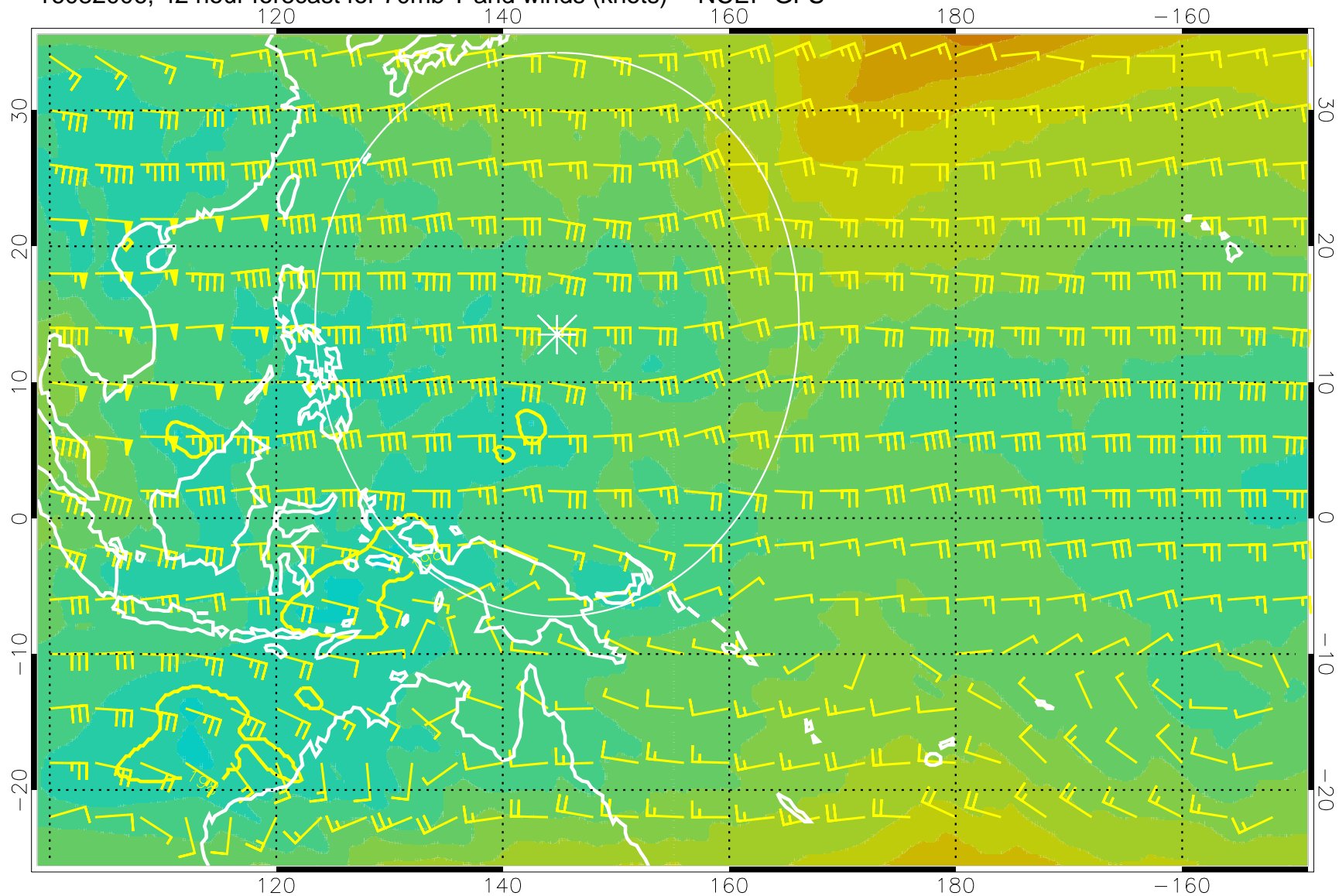
16082006, 42 hour forecast for 70mb T and winds (knots) -- NCEP GFS
