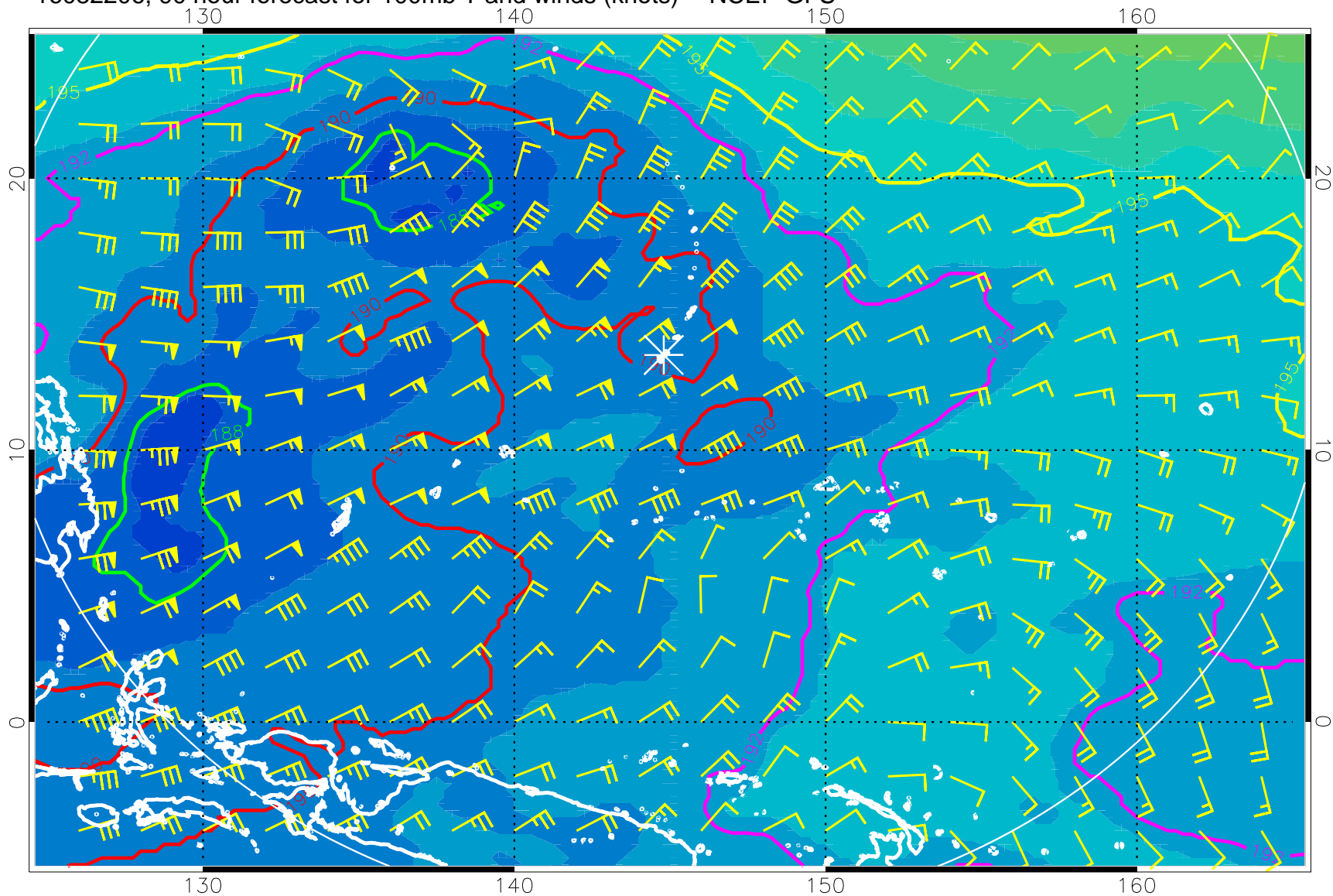
16082206, 90 hour forecast for 100mb T and winds (knots) -- NCEP GFS
