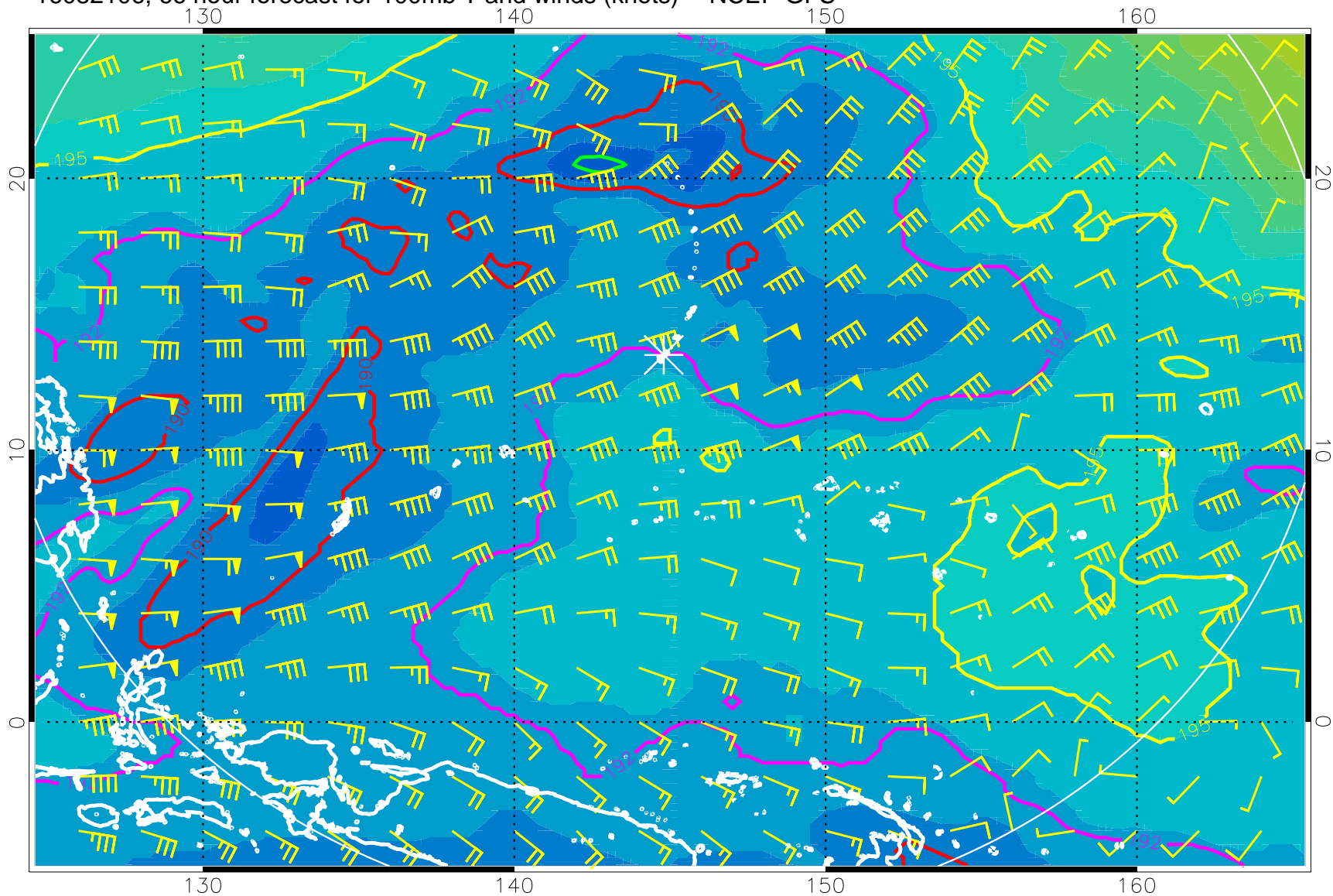
16082106, 66 hour forecast for 100mb T and winds (knots) -- NCEP GFS
