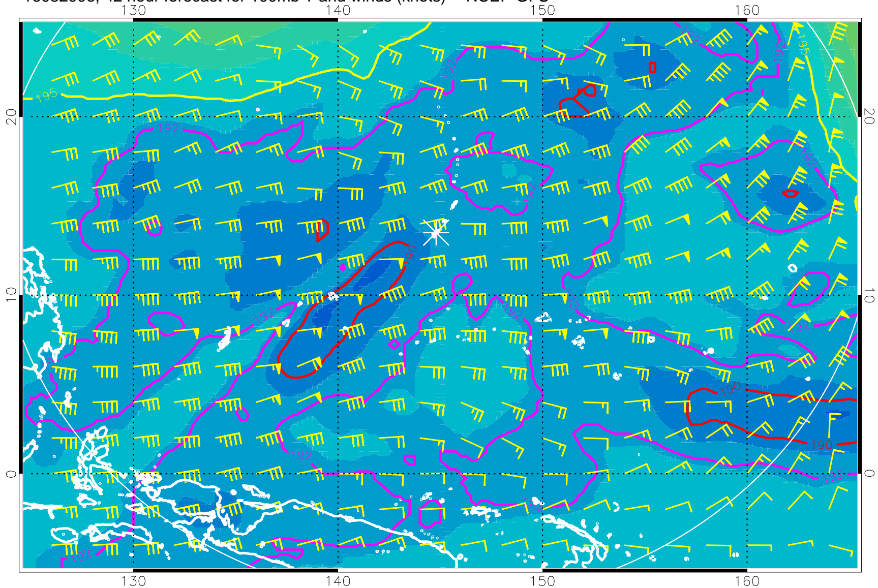
16082006, 42 hour forecast for 100mb T and winds (knots) -- NCEP GFS
