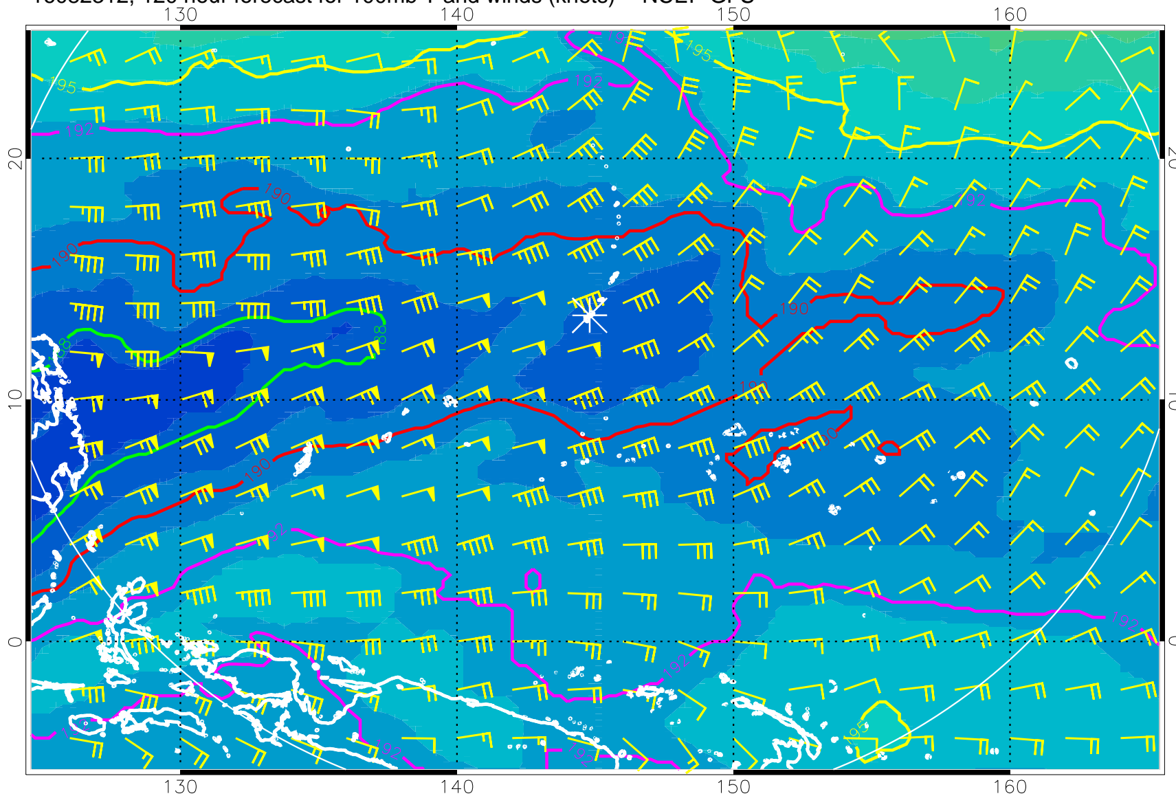
16082312, 120 hour forecast for 100mb T and winds (knots) -- NCEP GFS
