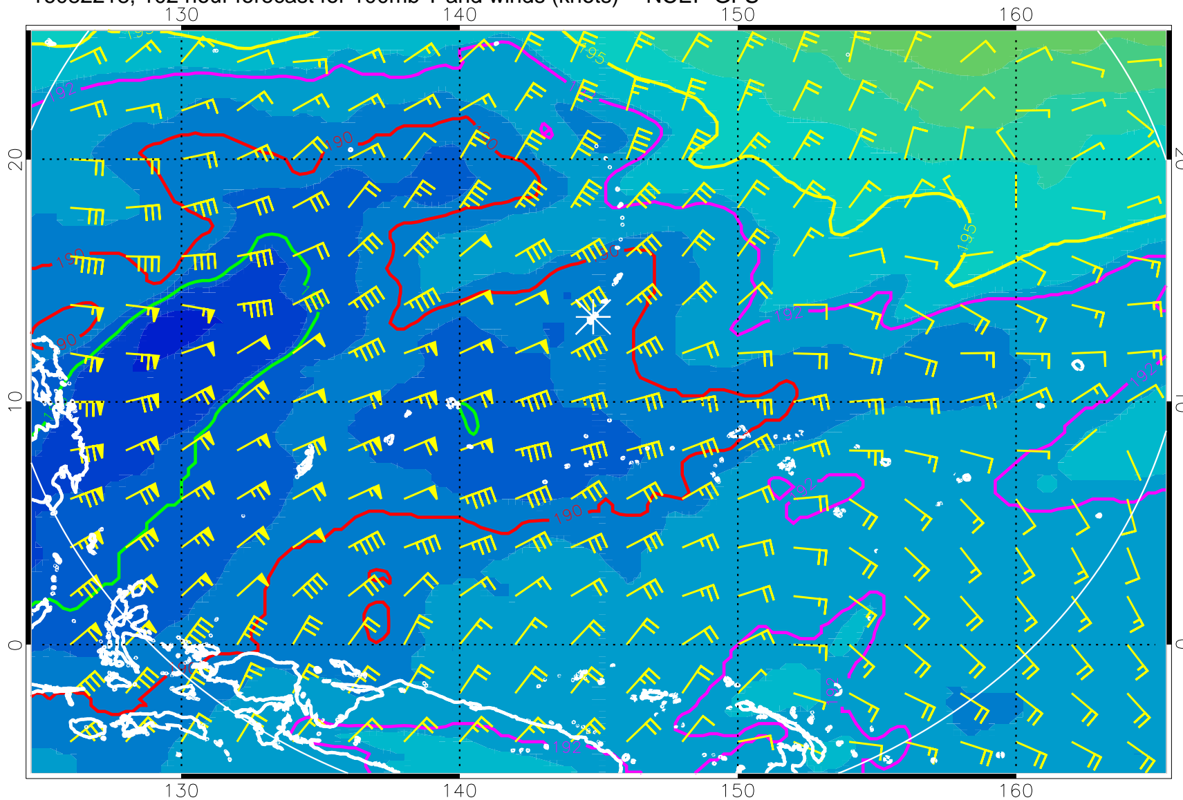
16082218, 102 hour forecast for 100mb T and winds (knots) -- NCEP GFS
