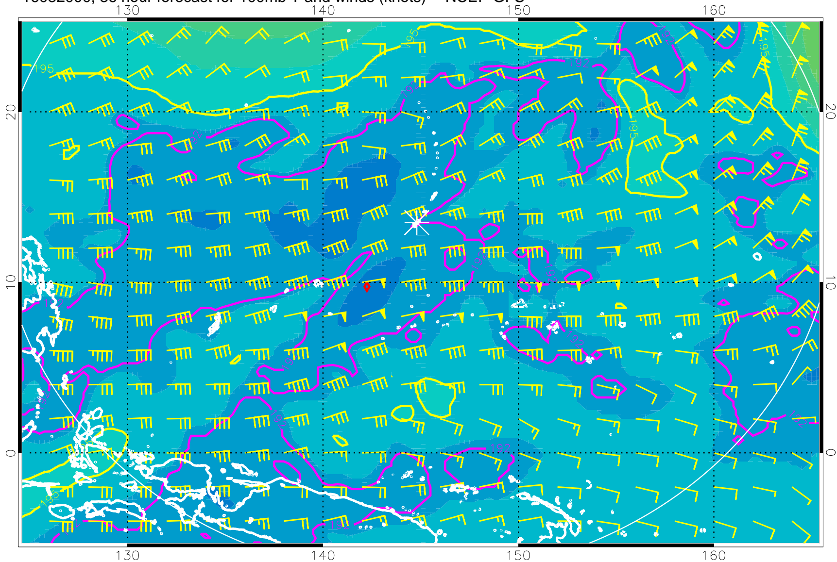
16082000, 36 hour forecast for 100mb T and winds (knots) -- NCEP GFS
