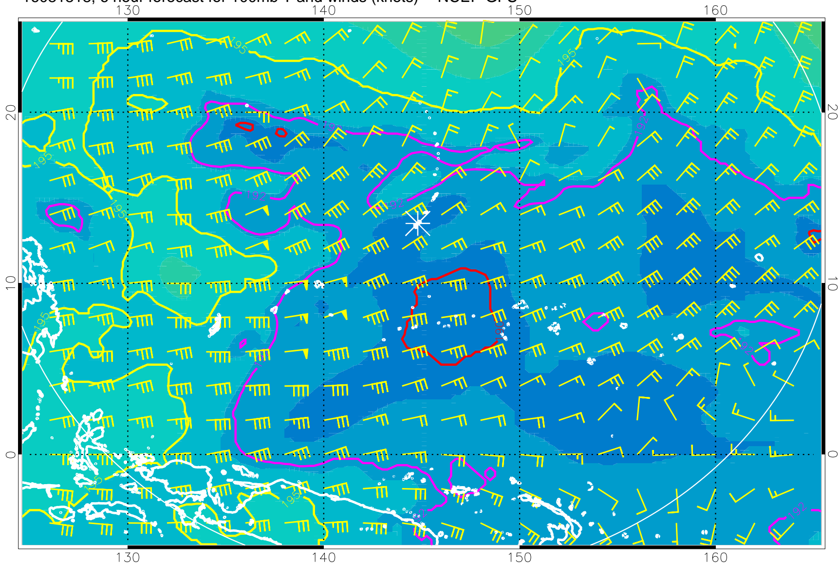
16081818, 6 hour forecast for 100mb T and winds (knots) -- NCEP GFS
