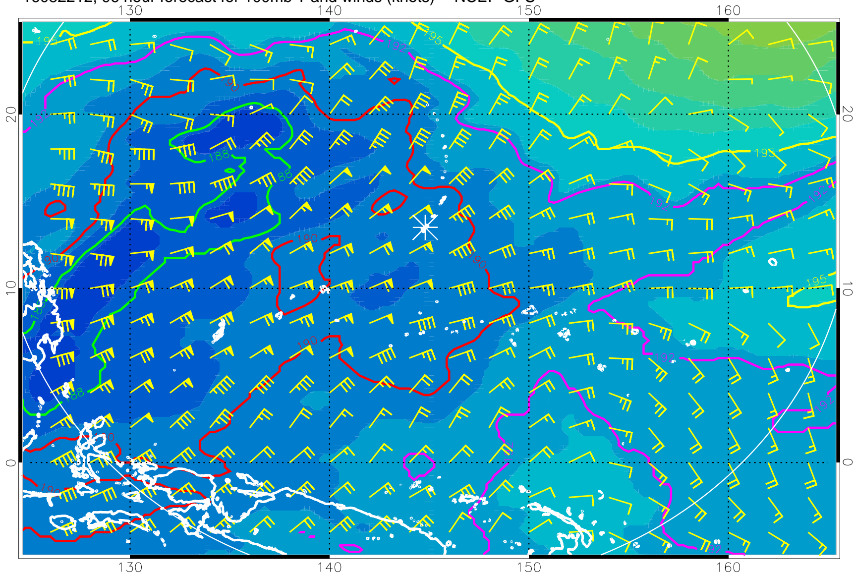
16082212, 96 hour forecast for 100mb T and winds (knots) -- NCEP GFS
