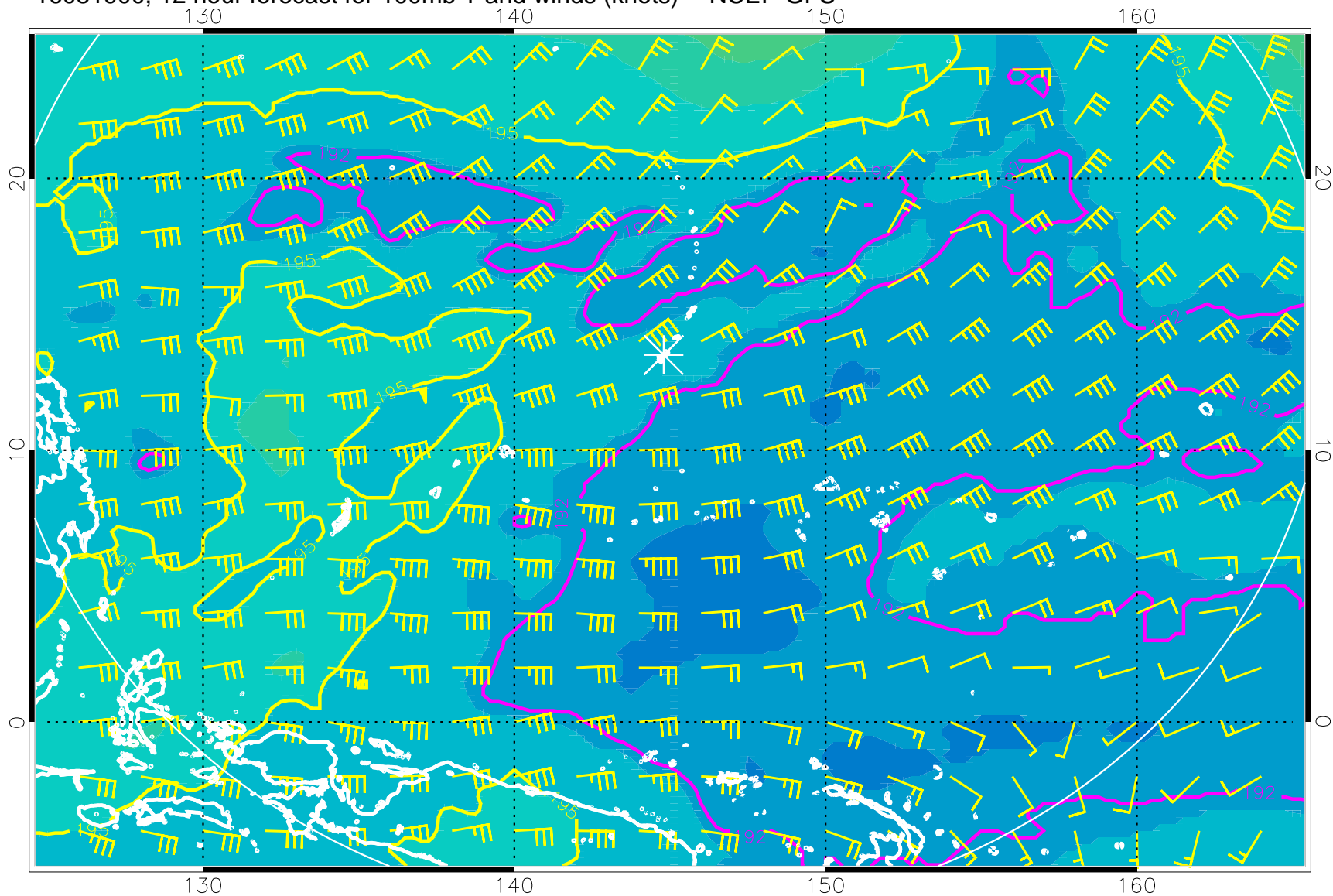
16081900, 12 hour forecast for 100mb T and winds (knots) -- NCEP GFS
