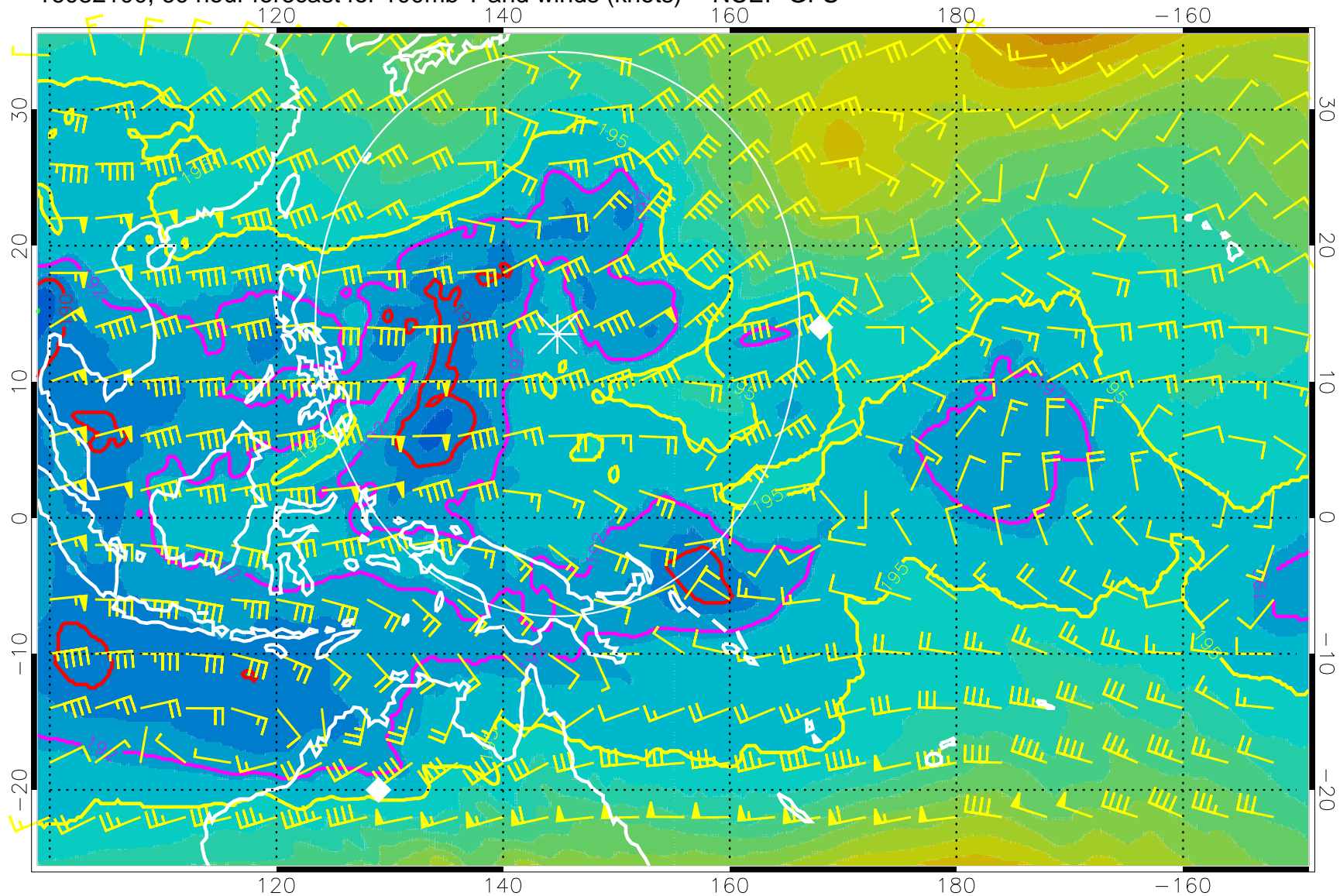
16082100, 60 hour forecast for 100mb T and winds (knots) -- NCEP GFS
