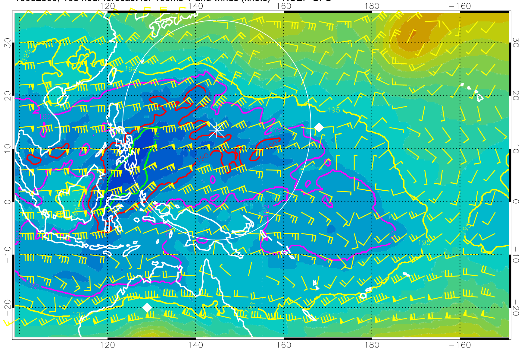
16082300, 108 hour forecast for 100mb T and winds (knots) -- NCEP GFS
