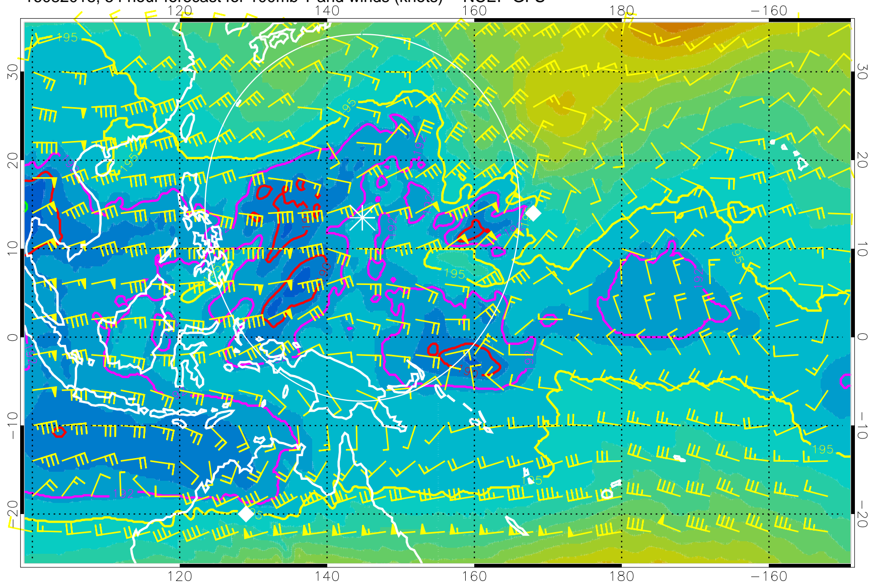
16082018, 54 hour forecast for 100mb T and winds (knots) -- NCEP GFS
