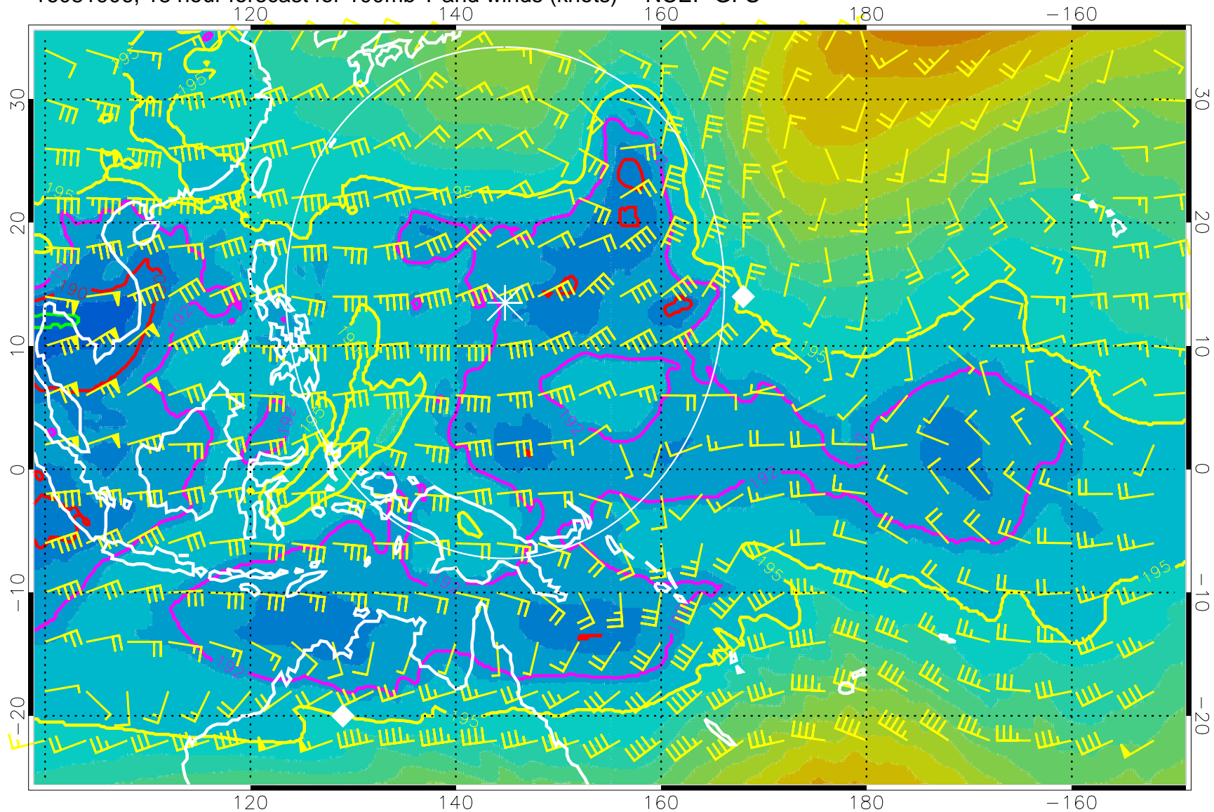
16081906, 18 hour forecast for 100mb T and winds (knots) -- NCEP GFS
