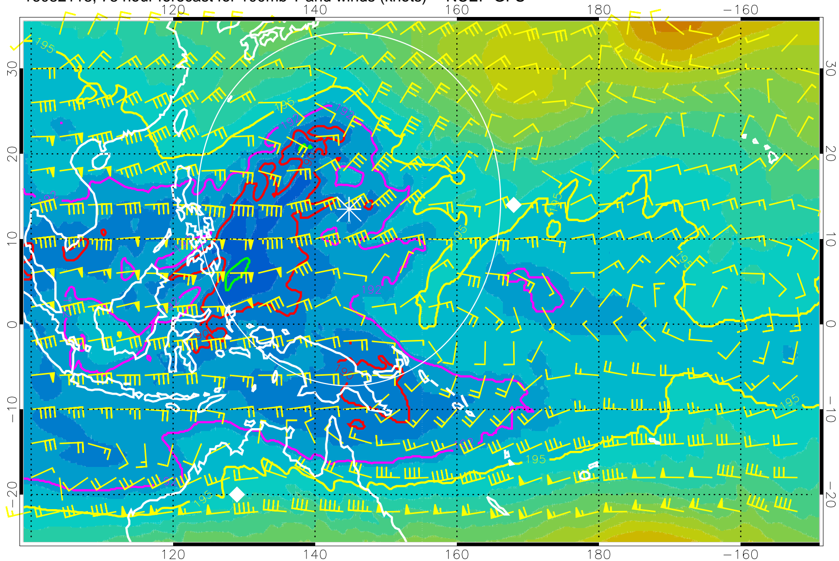
16082118, 78 hour forecast for 100mb T and winds (knots) -- NCEP GFS
