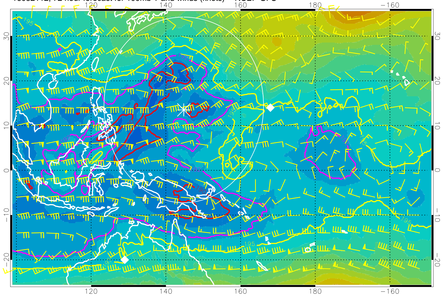
16082112, 72 hour forecast for 100mb T and winds (knots) -- NCEP GFS
