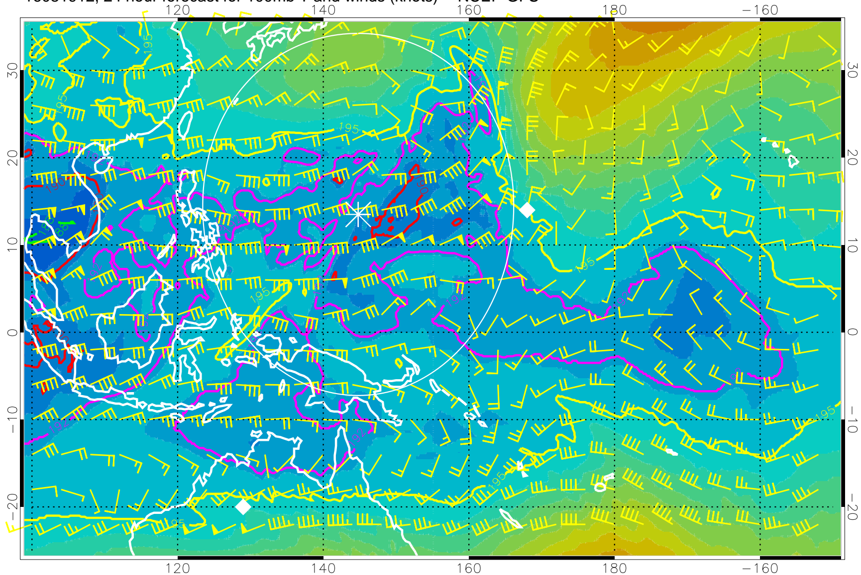
16081912, 24 hour forecast for 100mb T and winds (knots) -- NCEP GFS
