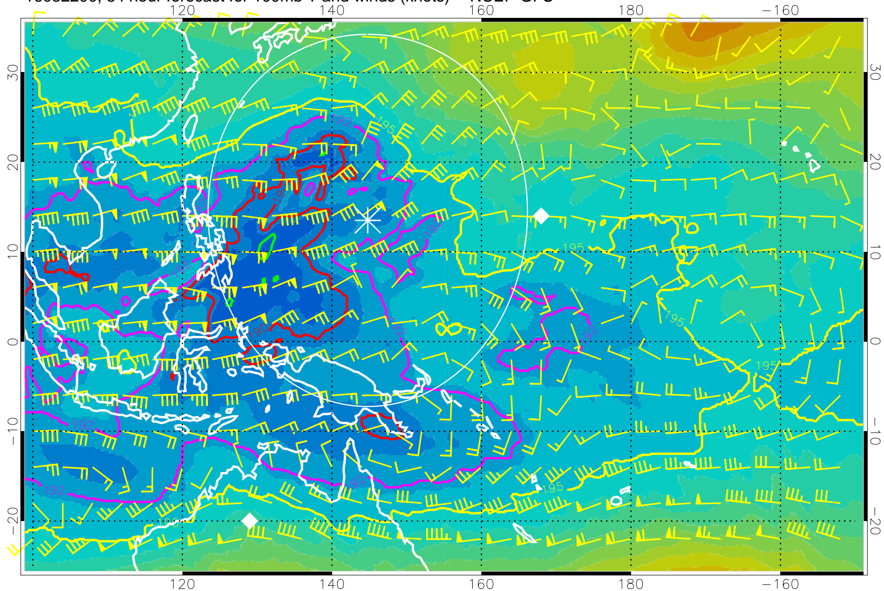
16082200, 84 hour forecast for 100mb T and winds (knots) -- NCEP GFS
