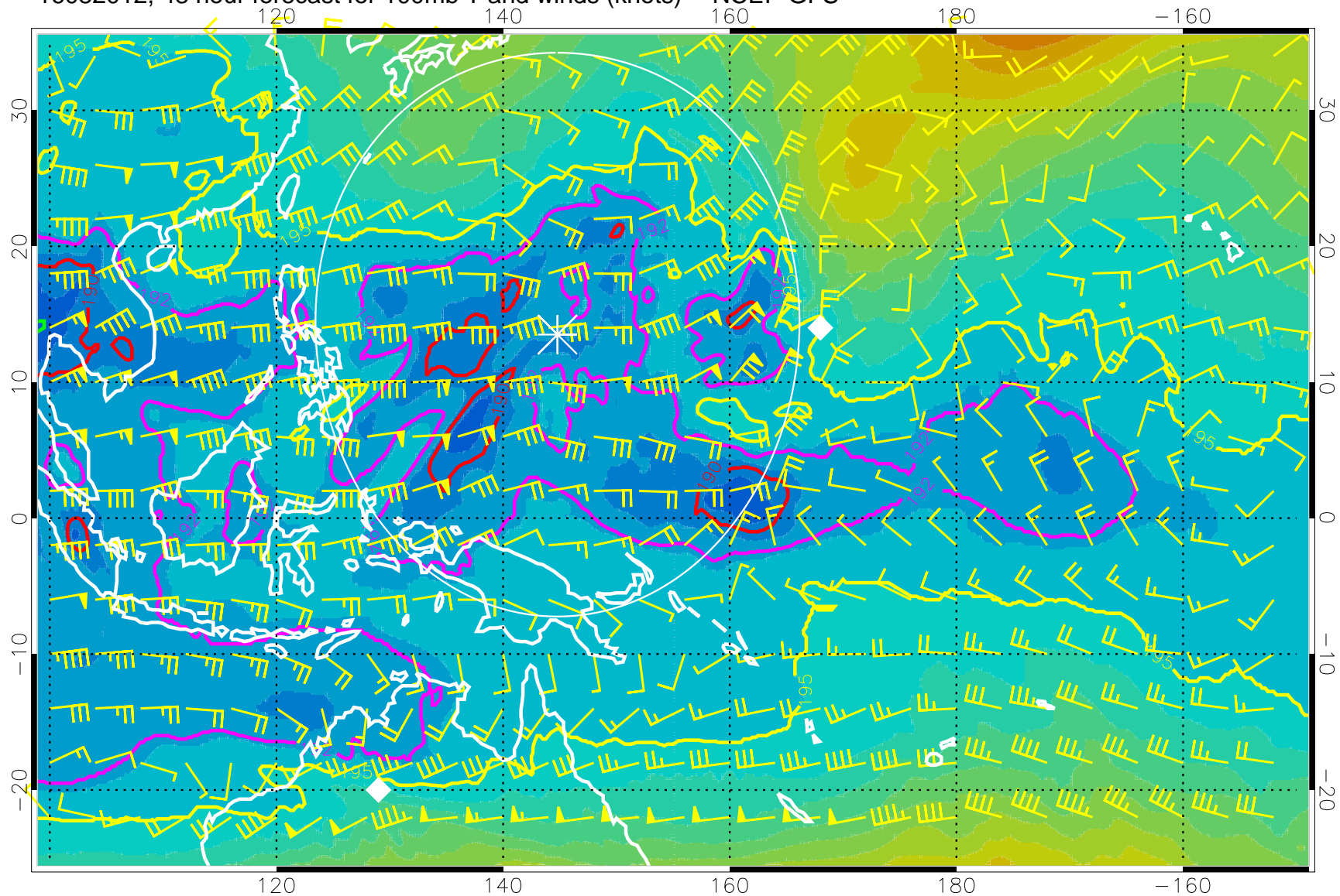
16082012, 48 hour forecast for 100mb T and winds (knots) -- NCEP GFS
