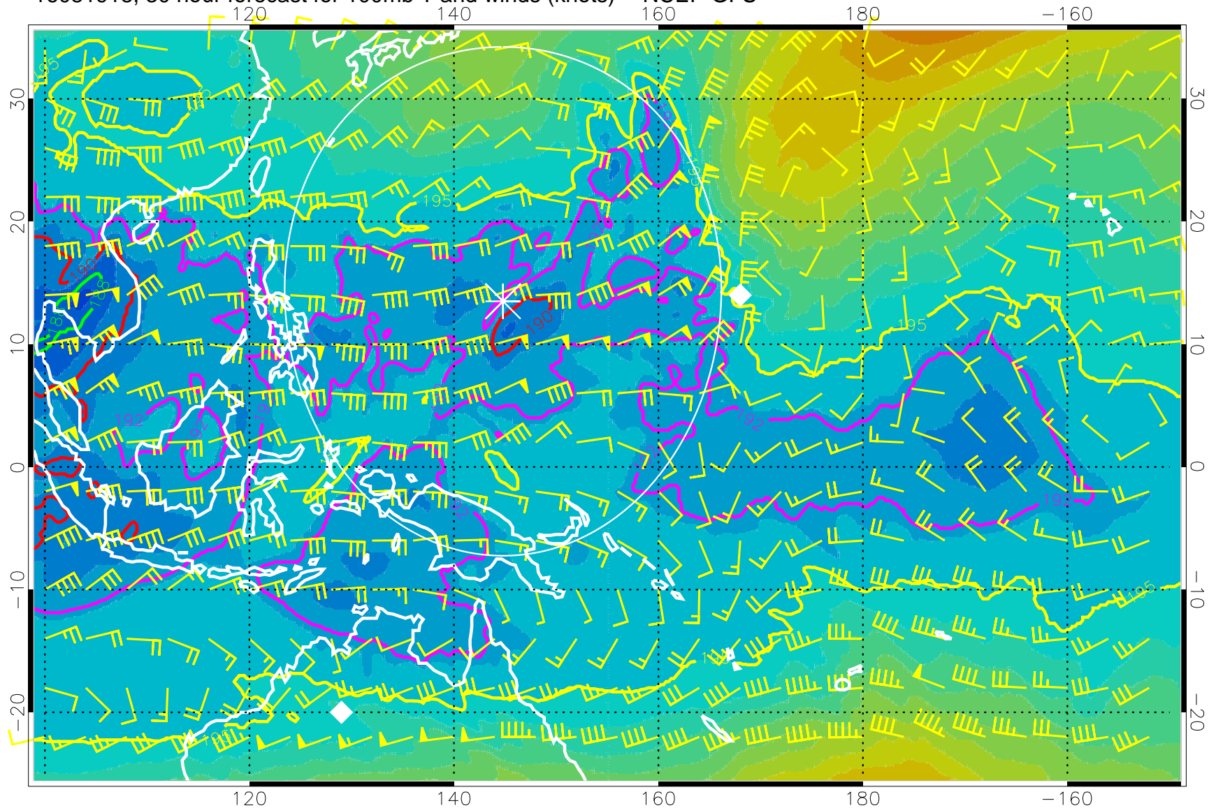
16081918, 30 hour forecast for 100mb T and winds (knots) -- NCEP GFS
