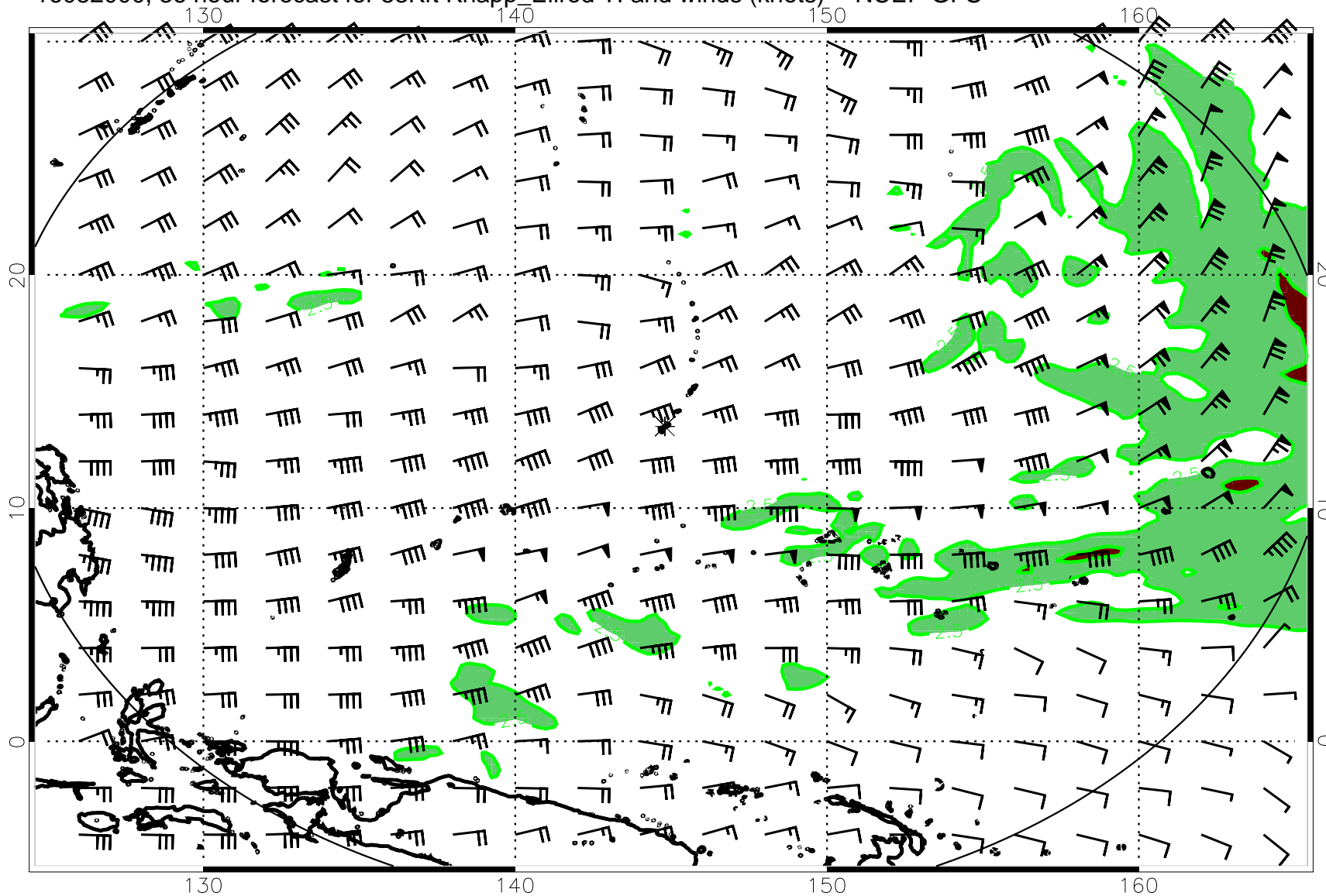
16082000, 36 hour forecast for 53Kft Knapp_Ellrod TI and winds (knots) -- NCEP GFS
