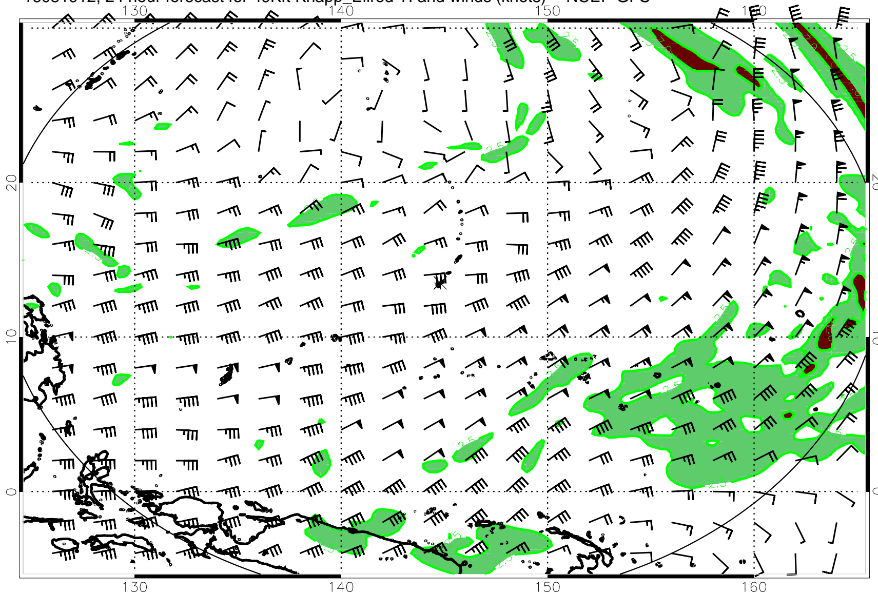
16081912, 24 hour forecast for 49Kft Knapp_Ellrod TI and winds (knots) -- NCEP GFS
