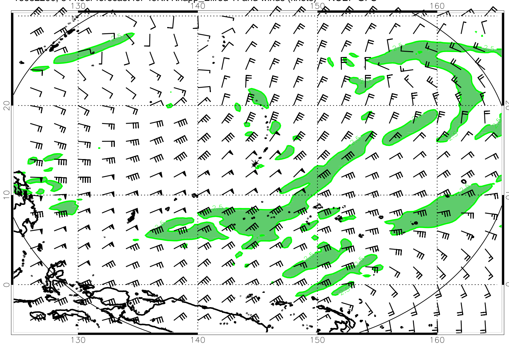
16082200, 84 hour forecast for 49Kft Knapp_Ellrod TI and winds (knots) -- NCEP GFS
