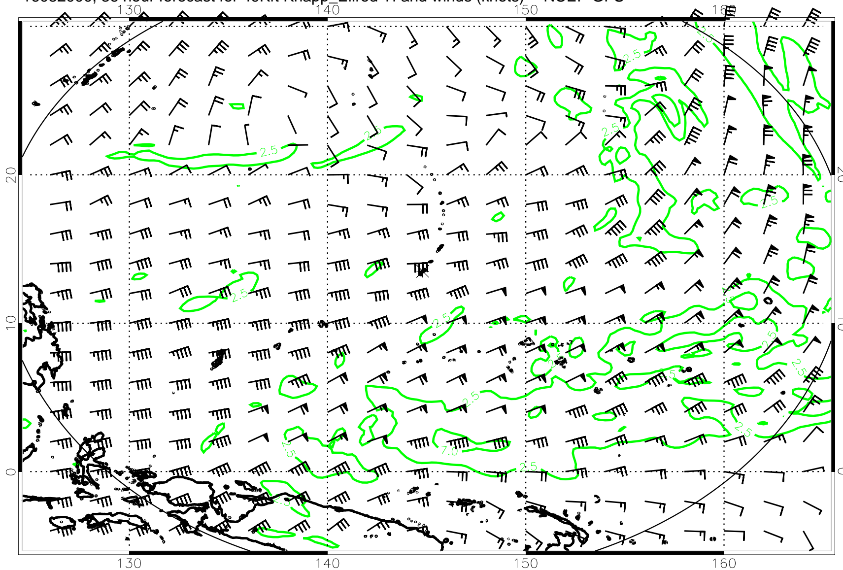
16082000, 36 hour forecast for 49Kft Knapp_Ellrod TI and winds (knots) -- NCEP GFS
