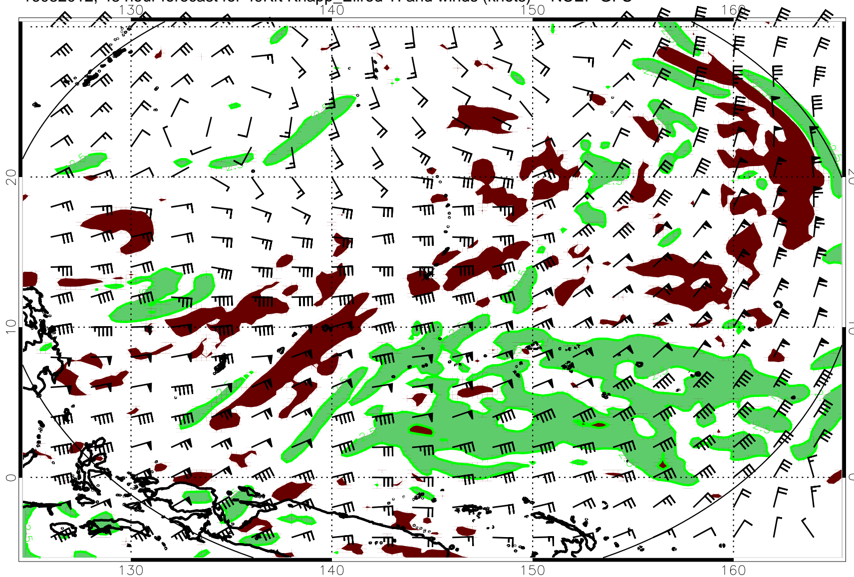
16082012, 48 hour forecast for 49Kft Knapp_Ellrod TI and winds (knots) -- NCEP GFS
