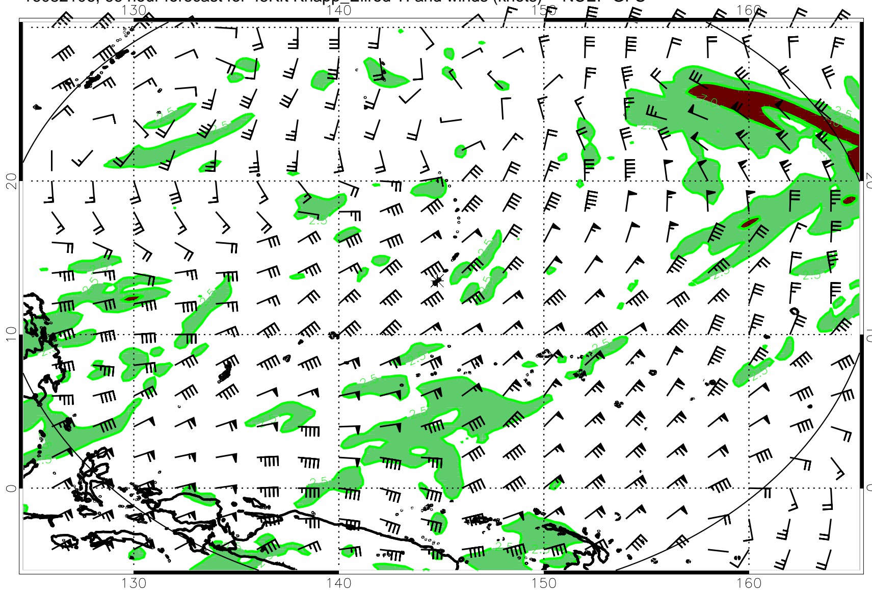
16082106, 66 hour forecast for 45Kft Knapp_Ellrod TI and winds (knots) -- NCEP GFS
