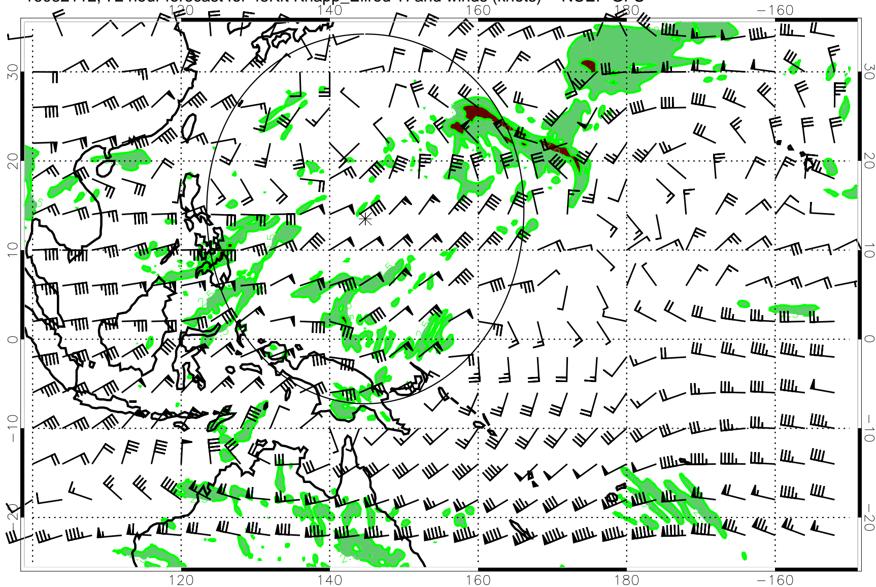
16082112, 72 hour forecast for 45Kft Knapp_Ellrod TI and winds (knots) -- NCEP GFS
