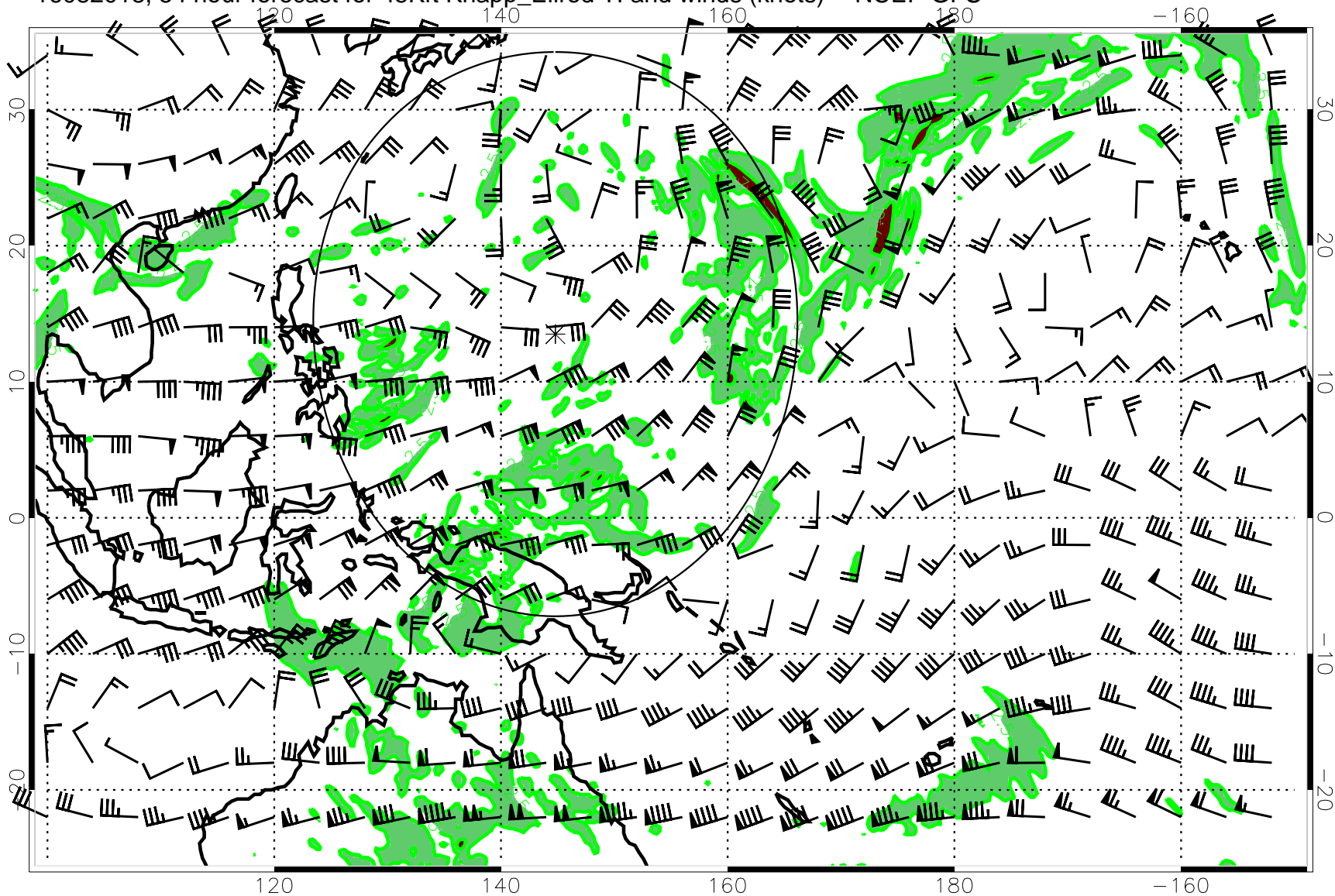
16082018, 54 hour forecast for 45Kft Knapp_Ellrod TI and winds (knots) -- NCEP GFS
