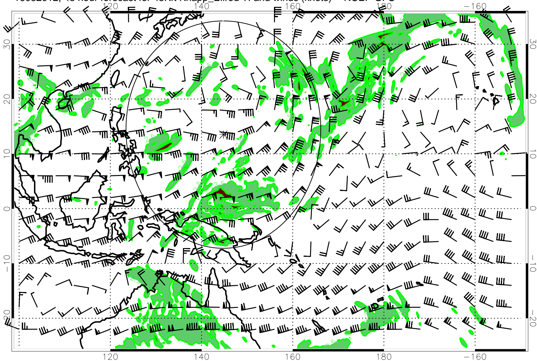
16082012, 48 hour forecast for 45Kft Knapp_Ellrod TI and winds (knots) -- NCEP GFS
