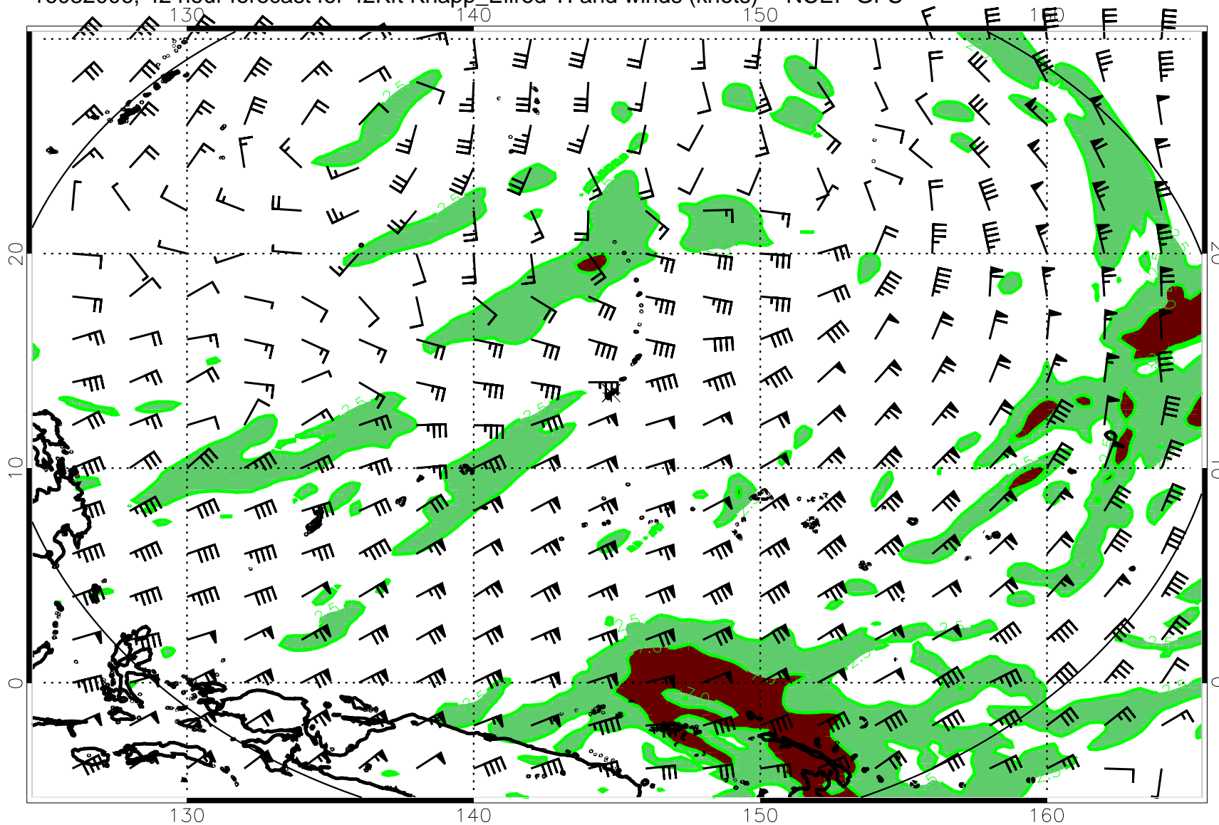
16082006, 42 hour forecast for 42Kft Knapp_Ellrod TI and winds (knots) -- NCEP GFS
