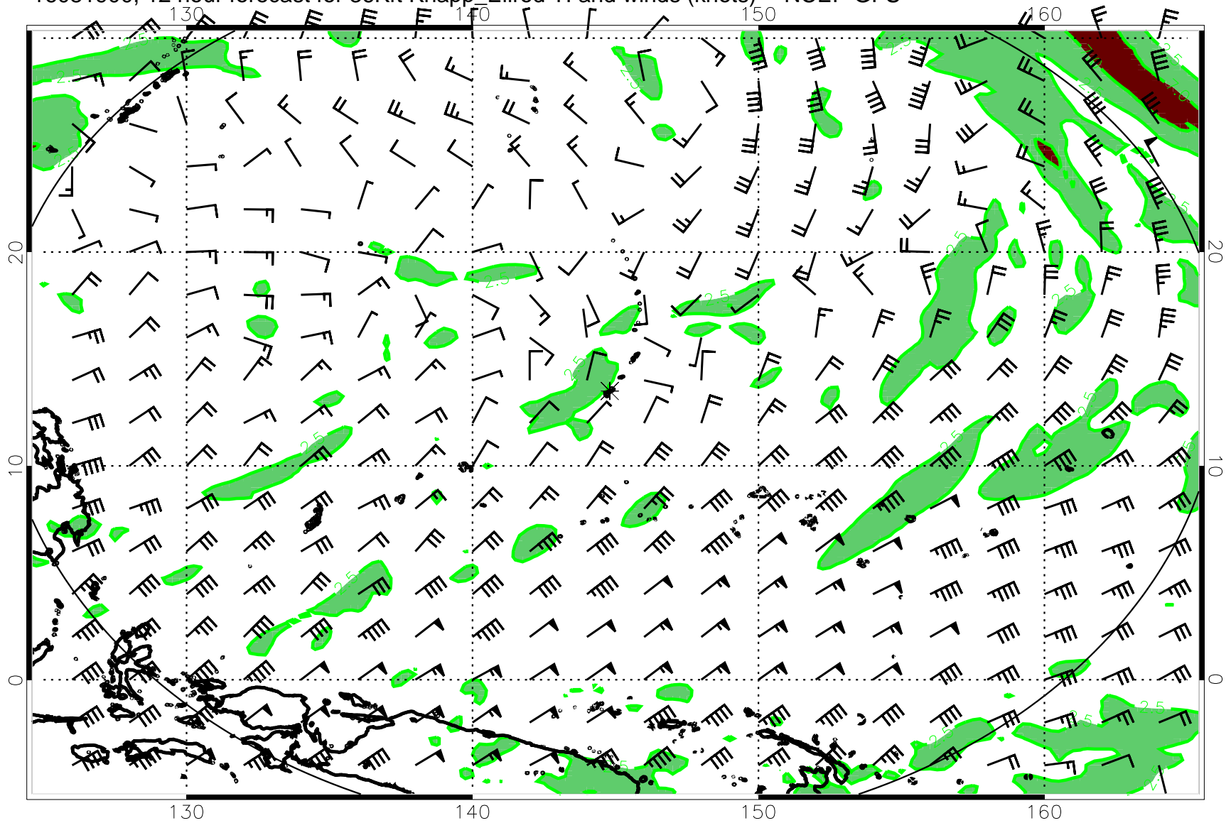
16081900, 12 hour forecast for 36Kft Knapp_Ellrod TI and winds (knots) -- NCEP GFS
