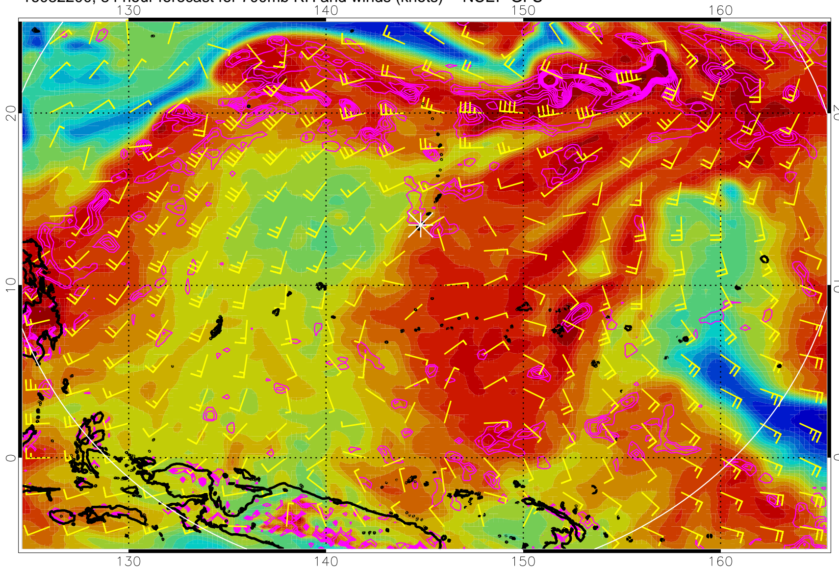
16082200, 84 hour forecast for 700mb RH and winds (knots) -- NCEP GFS
