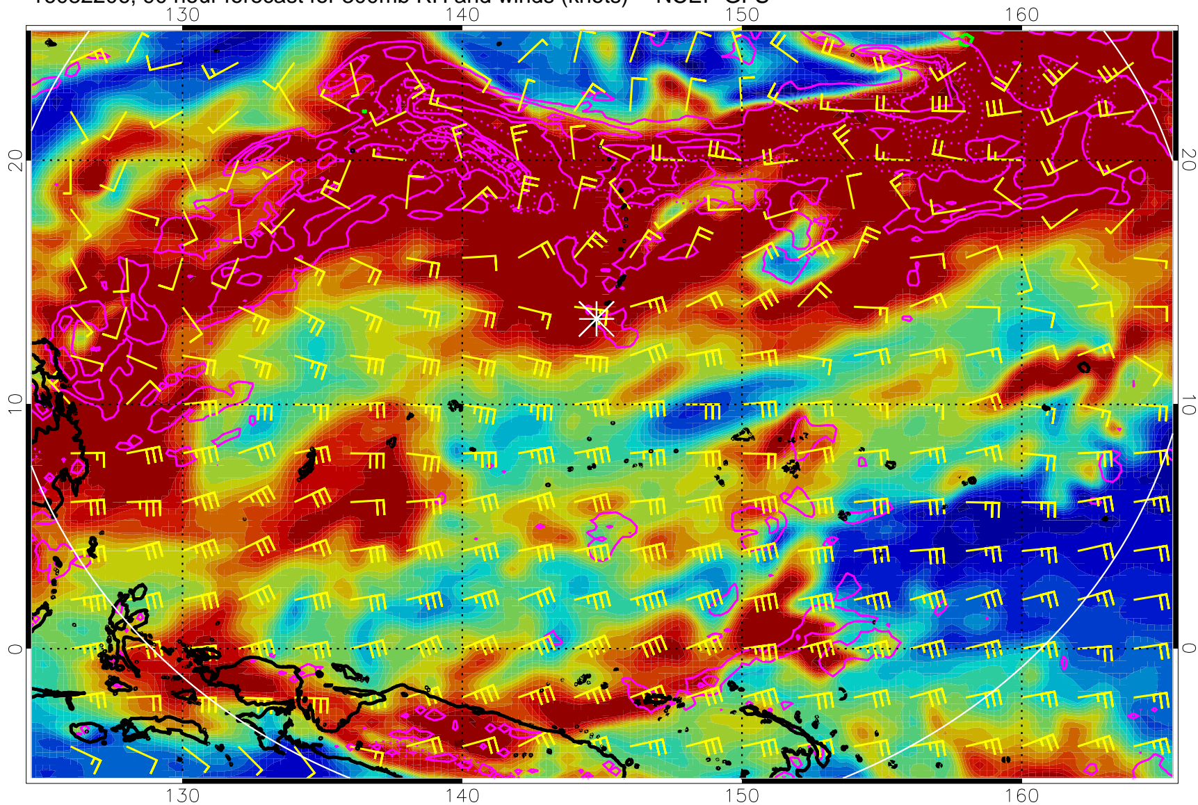
16082206, 90 hour forecast for 300mb RH and winds (knots) -- NCEP GFS
