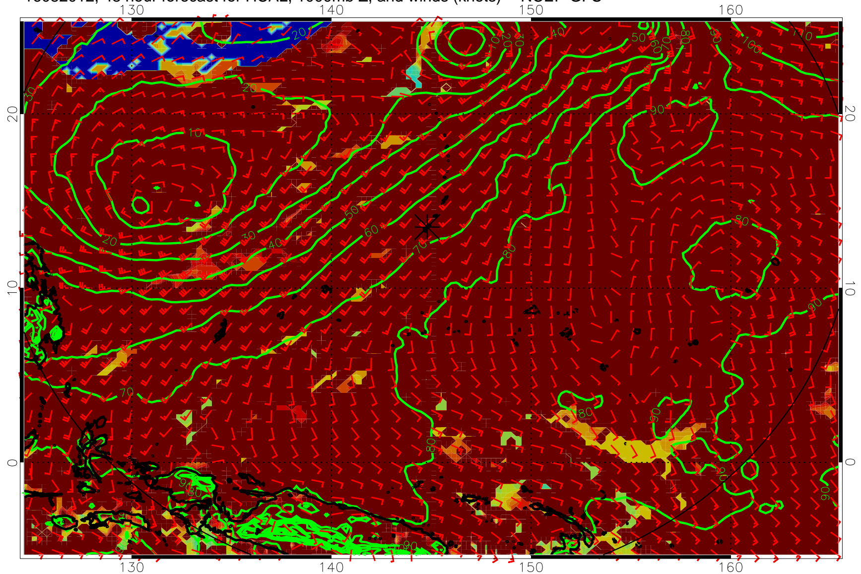
16082012, 48 hour forecast for HCAL, 1000mb Z, and winds (knots) -- NCEP GFS
