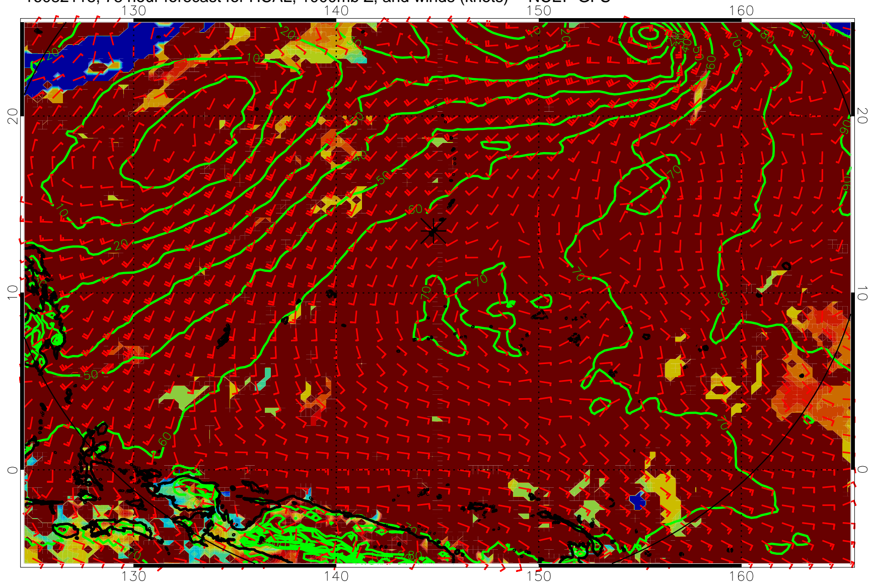
16082118, 78 hour forecast for HCAL, 1000mb Z, and winds (knots) -- NCEP GFS
