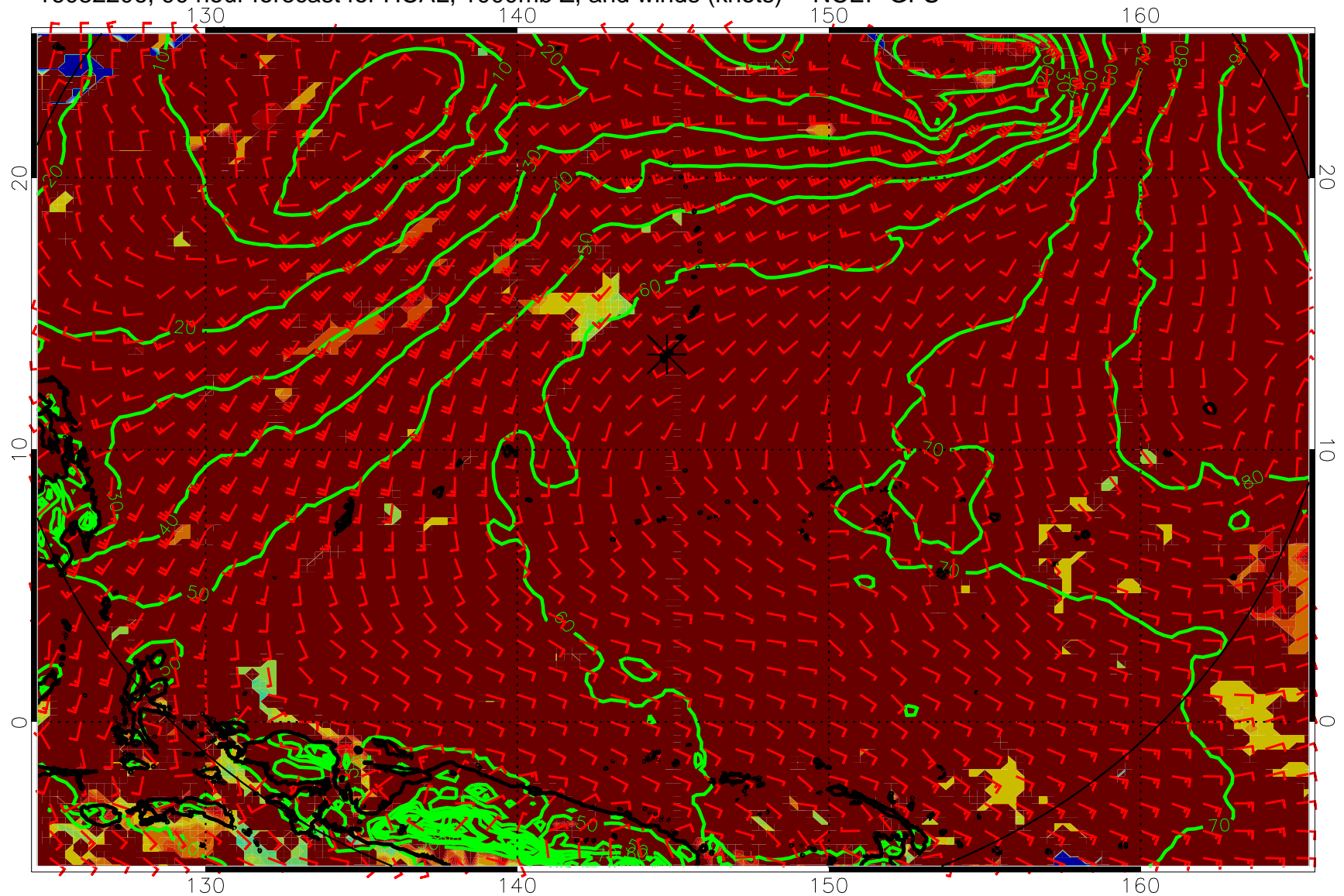
16082206, 90 hour forecast for HCAL, 1000mb Z, and winds (knots) -- NCEP GFS
