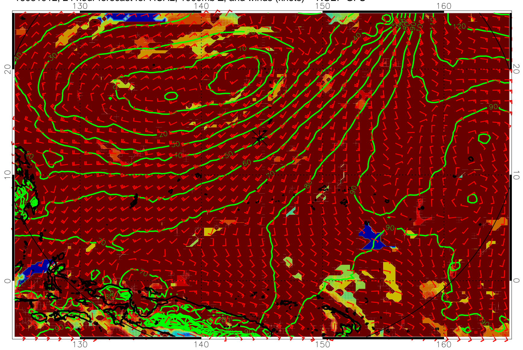
16081912, 24 hour forecast for HCAL, 1000mb Z, and winds (knots) -- NCEP GFS
