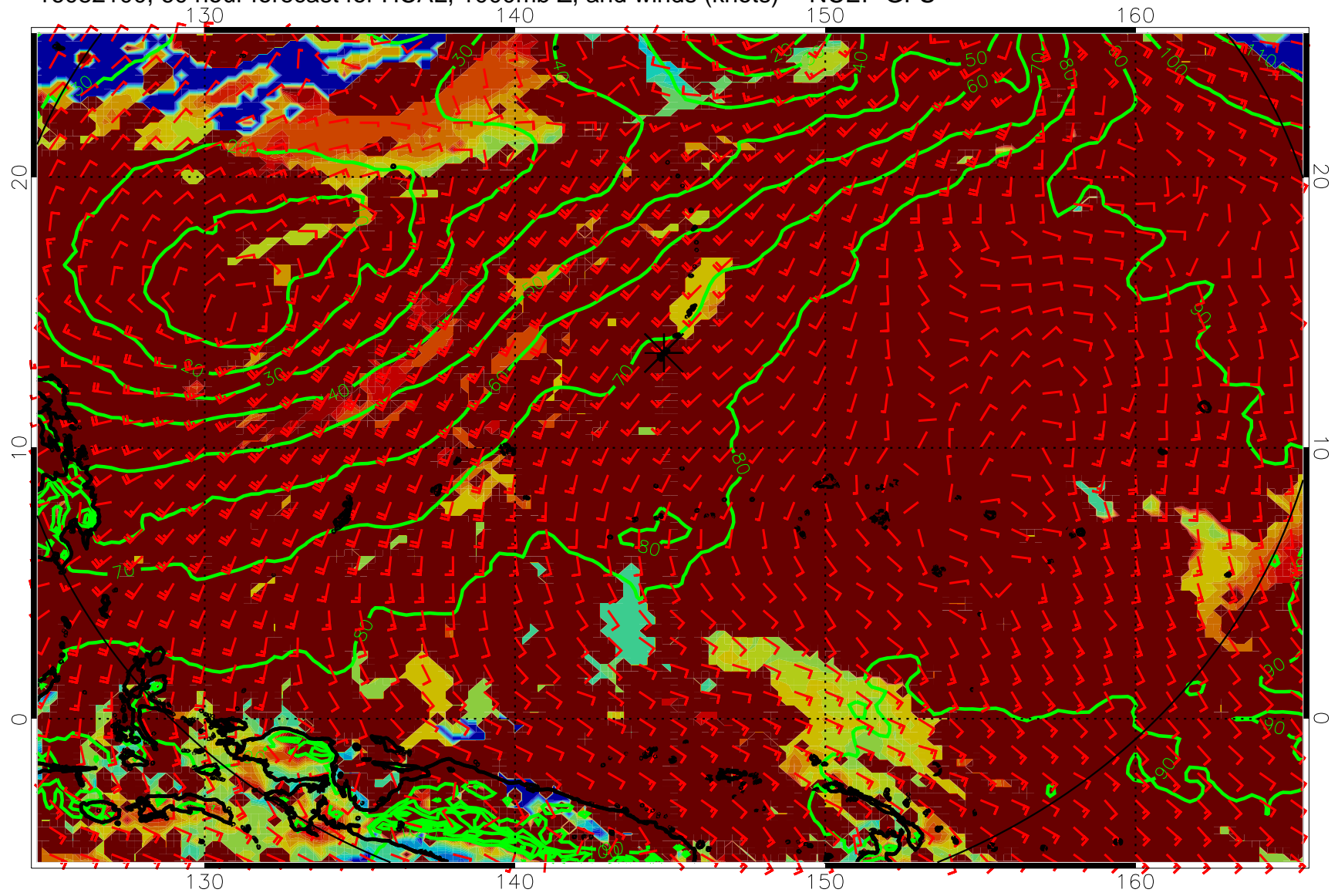
16082100, 60 hour forecast for HCAL, 1000mb Z, and winds (knots) -- NCEP GFS
