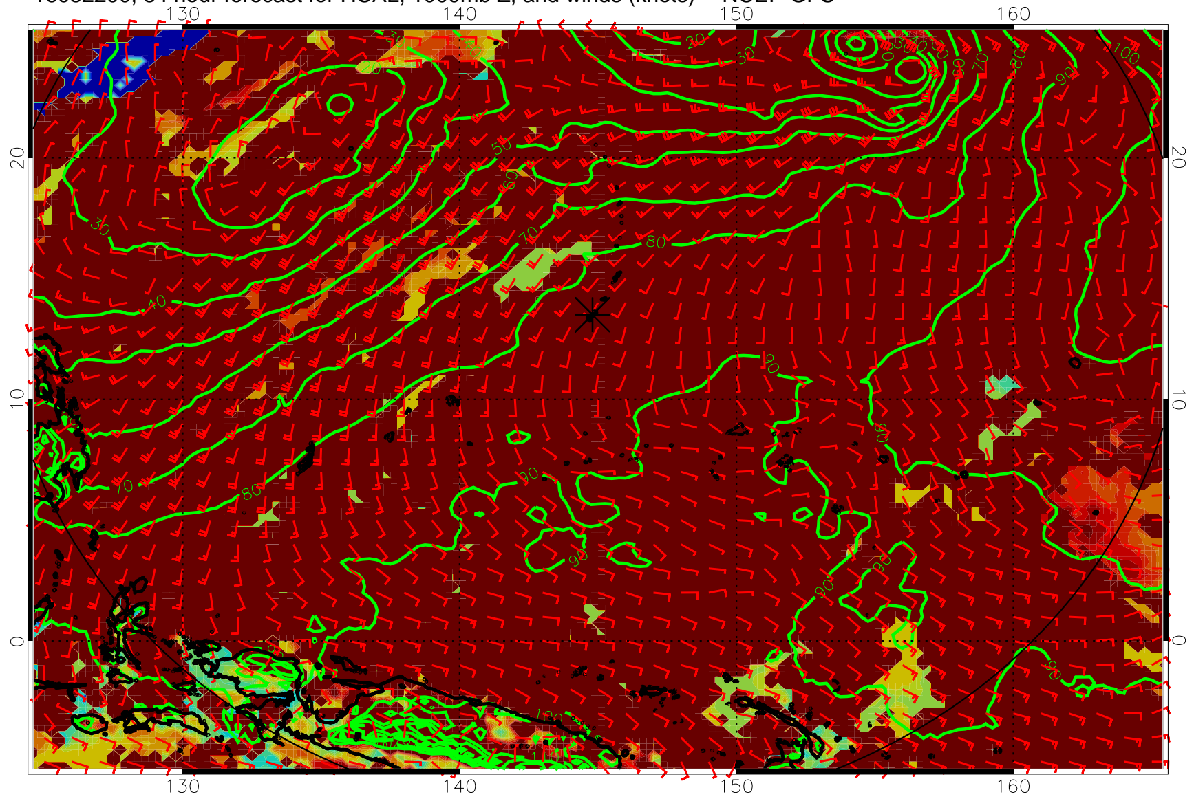
16082200, 84 hour forecast for HCAL, 1000mb Z, and winds (knots) -- NCEP GFS
