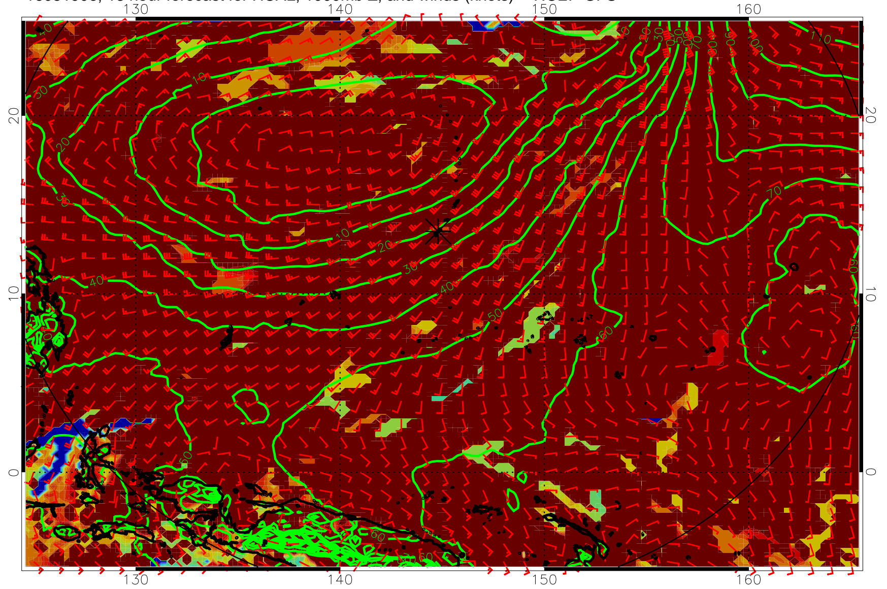
16081906, 18 hour forecast for HCAL, 1000mb Z, and winds (knots) -- NCEP GFS
