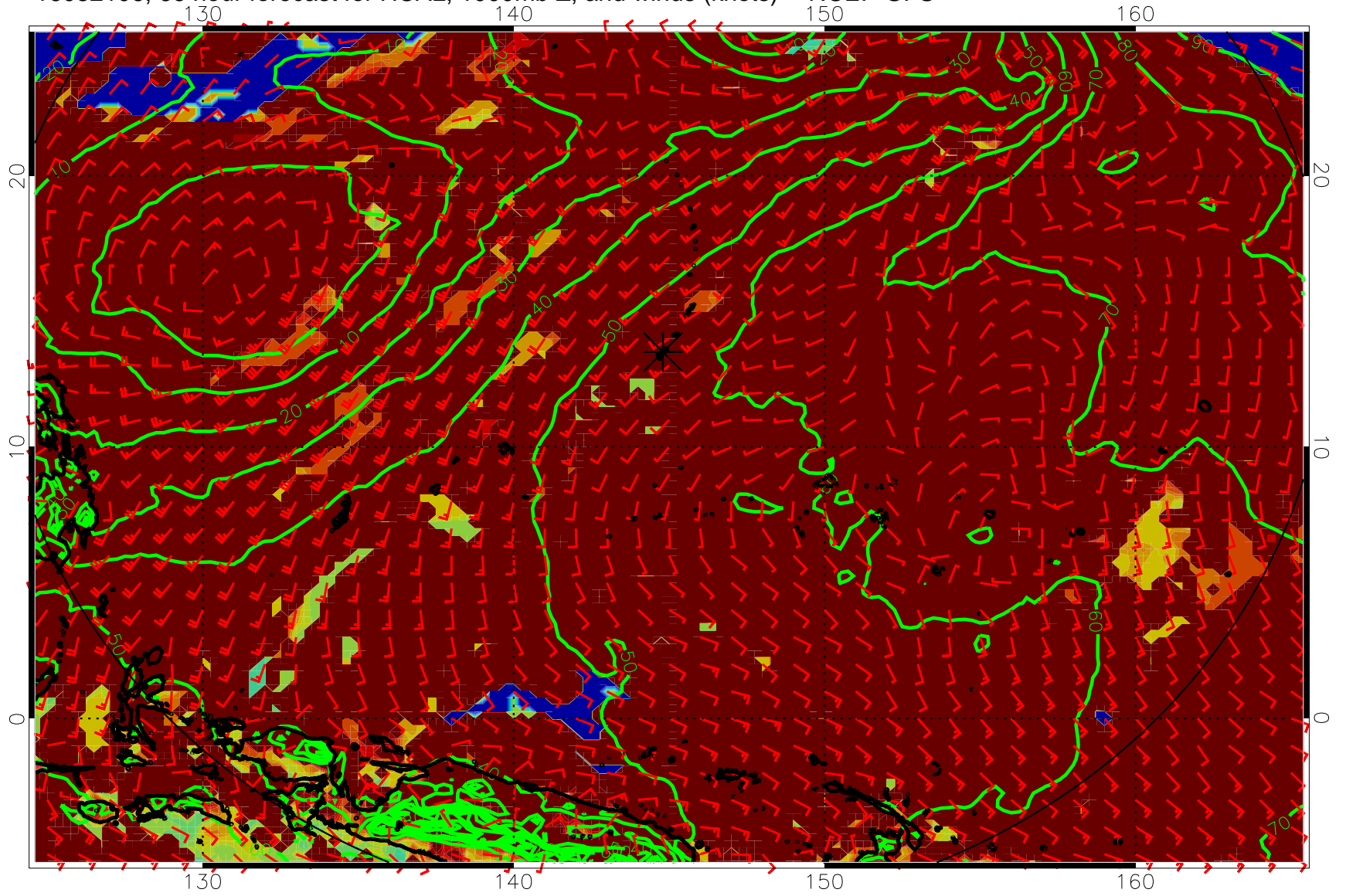
16082106, 66 hour forecast for HCAL, 1000mb Z, and winds (knots) -- NCEP GFS
