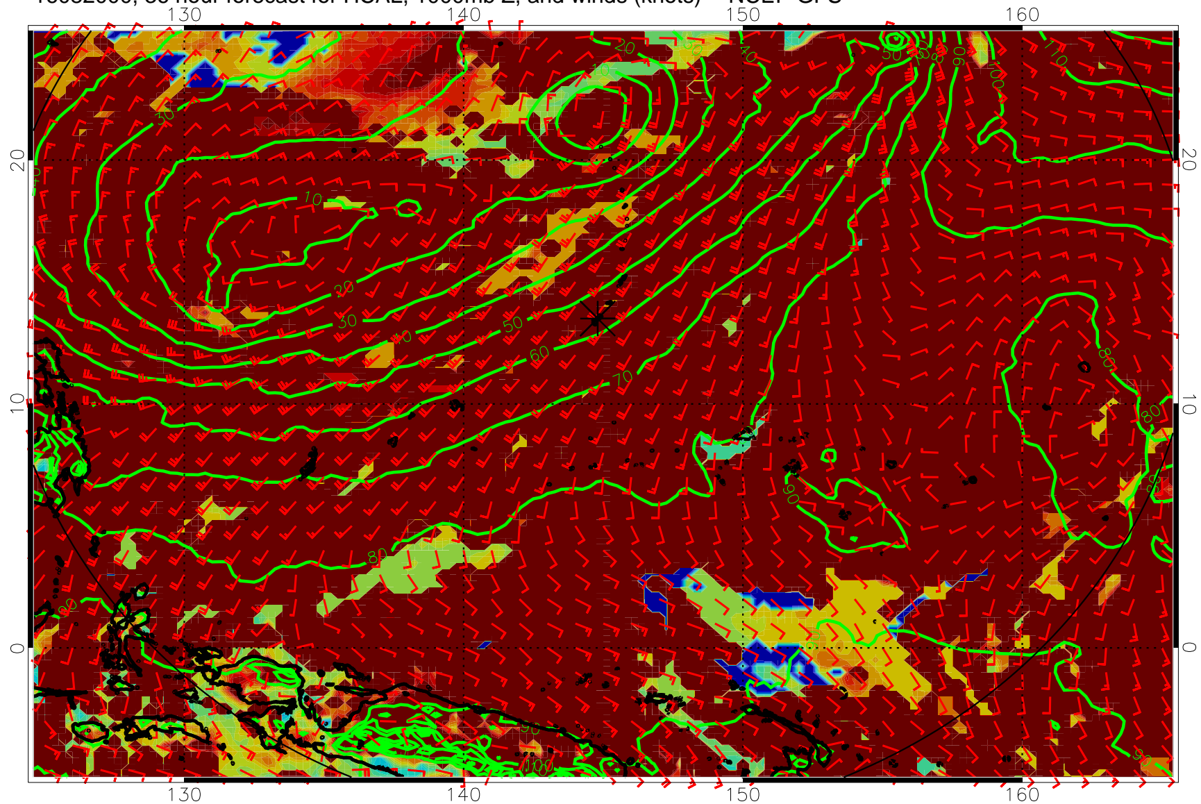
16082000, 36 hour forecast for HCAL, 1000mb Z, and winds (knots) -- NCEP GFS
