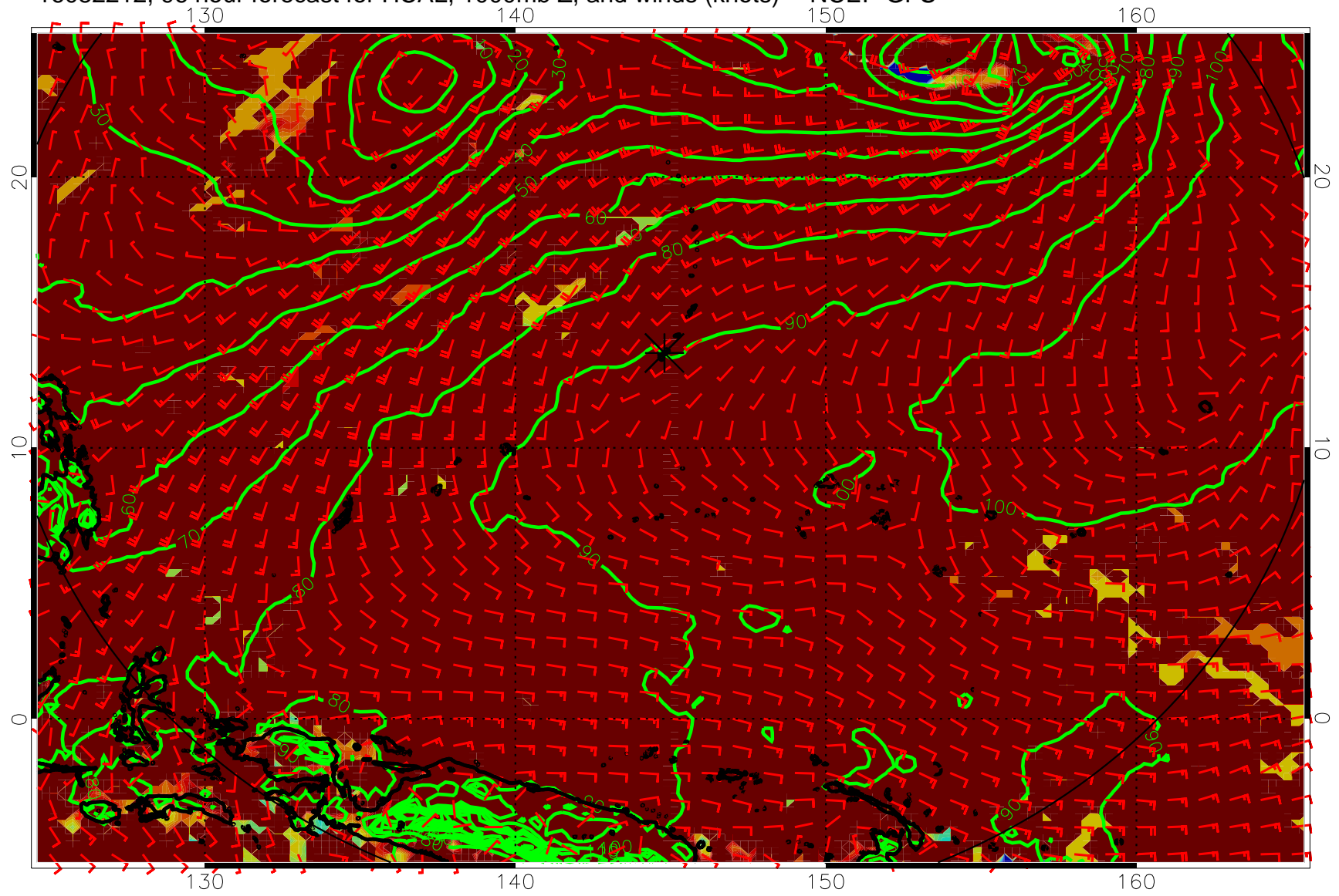
16082212, 96 hour forecast for HCAL, 1000mb Z, and winds (knots) -- NCEP GFS
