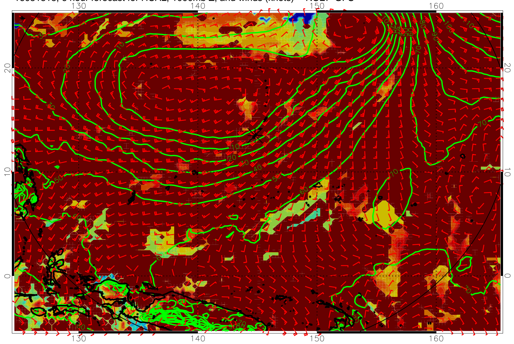
16081818, 6 hour forecast for HCAL, 1000mb Z, and winds (knots) -- NCEP GFS
