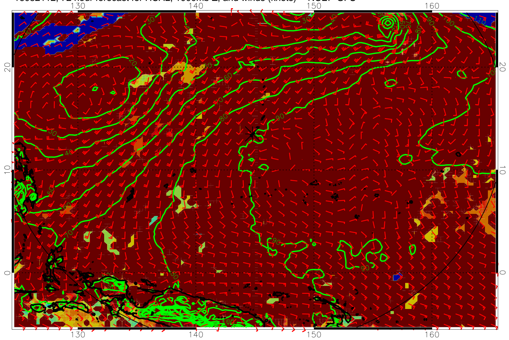
16082112, 72 hour forecast for HCAL, 1000mb Z, and winds (knots) -- NCEP GFS
