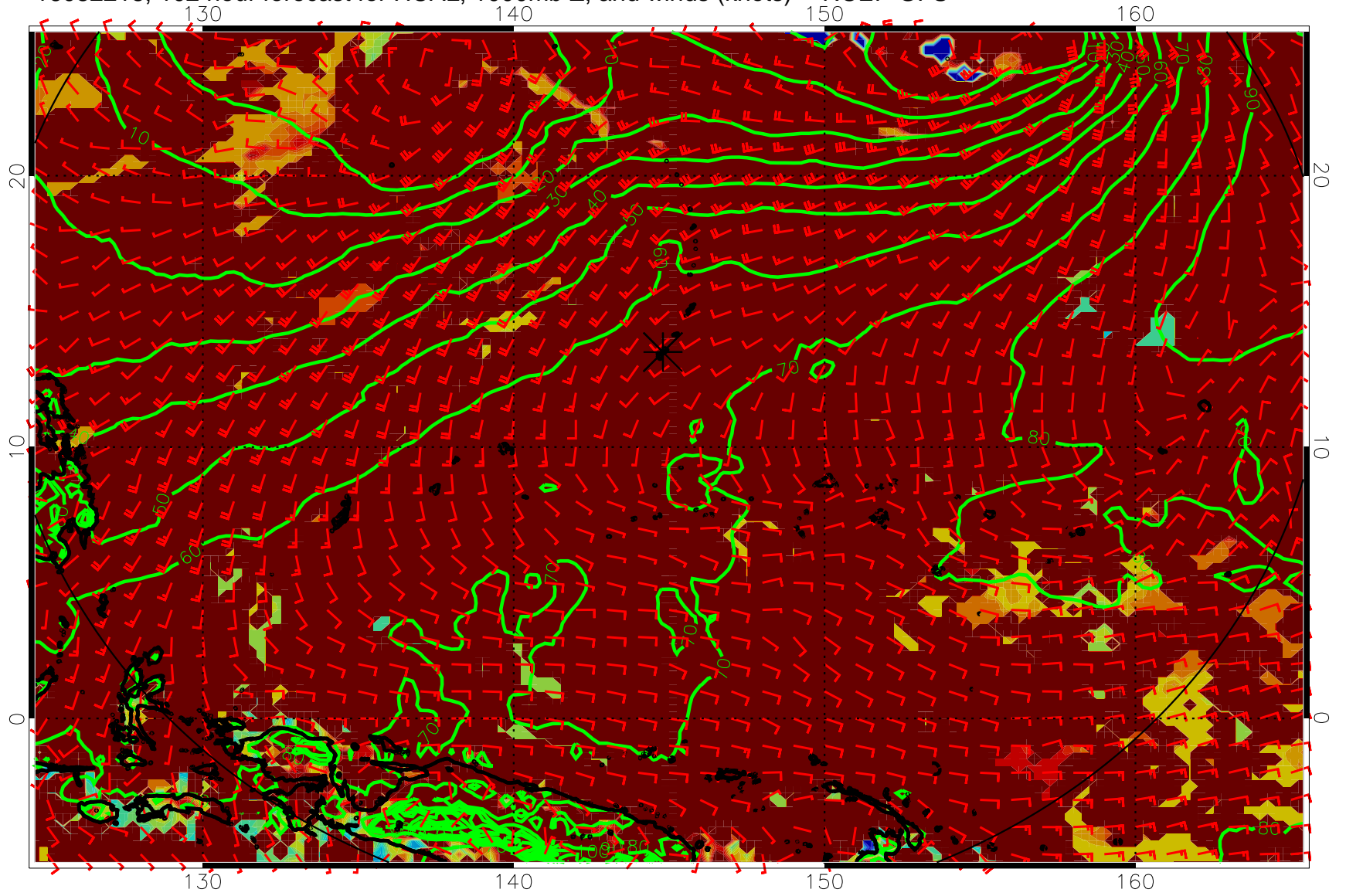
16082218, 102 hour forecast for HCAL, 1000mb Z, and winds (knots) -- NCEP GFS
