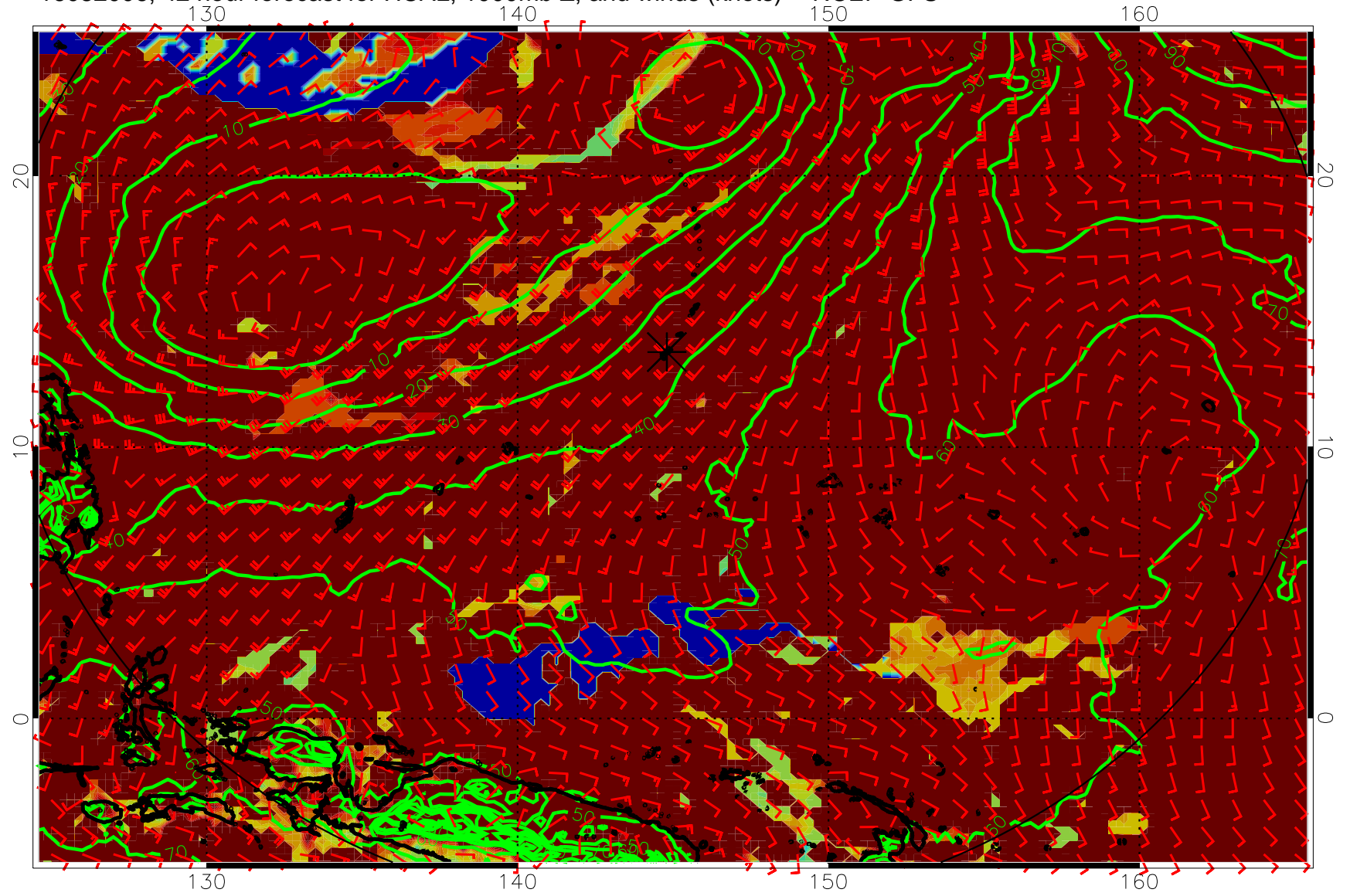
16082006, 42 hour forecast for HCAL, 1000mb Z, and winds (knots) -- NCEP GFS
