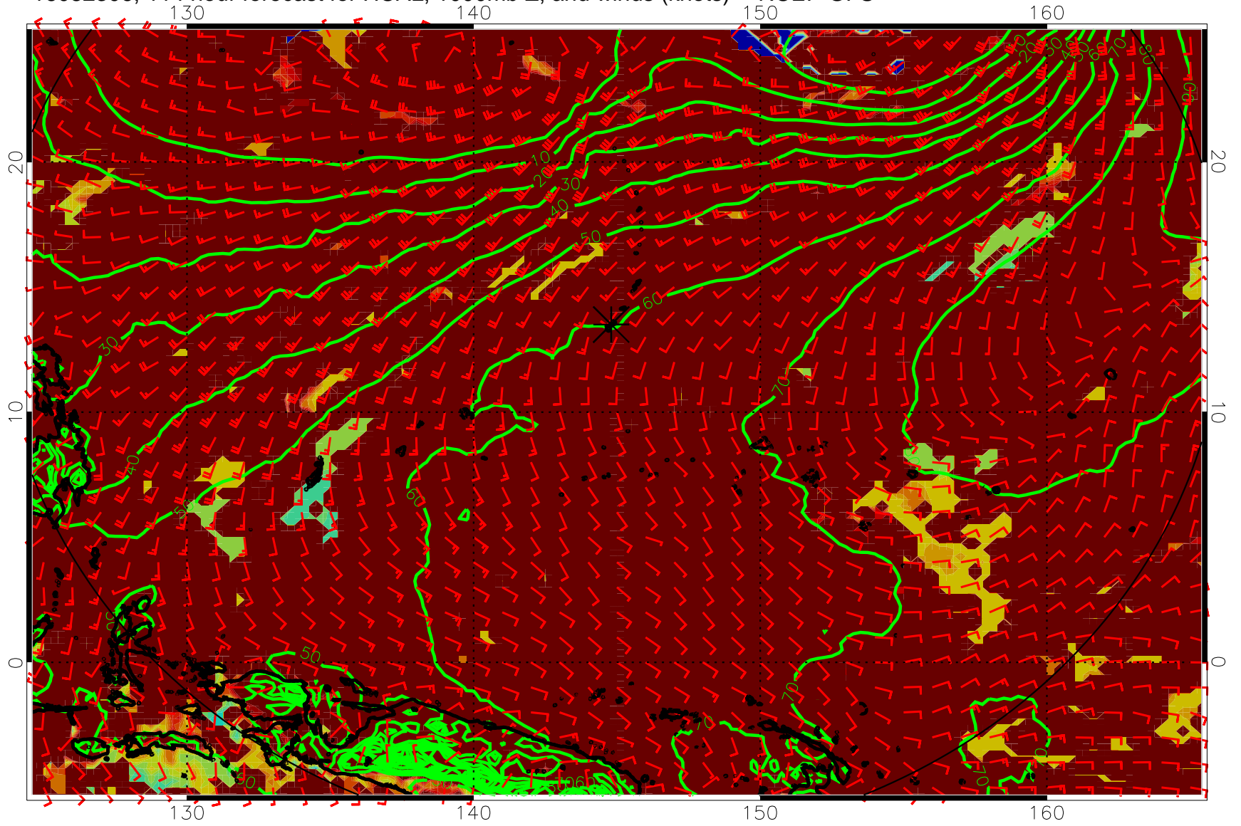
16082306, 114 hour forecast for HCAL, 1000mb Z, and winds (knots) -- NCEP GFS
