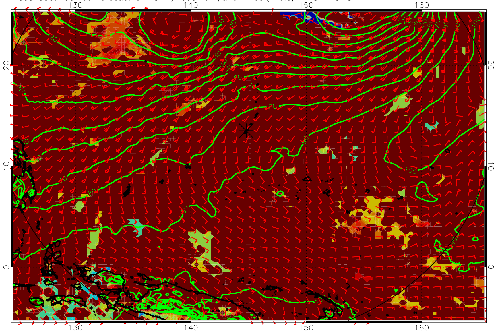
16082300, 108 hour forecast for HCAL, 1000mb Z, and winds (knots) -- NCEP GFS
