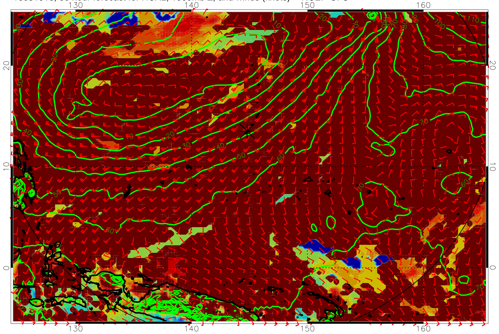
16081918, 30 hour forecast for HCAL, 1000mb Z, and winds (knots) -- NCEP GFS
