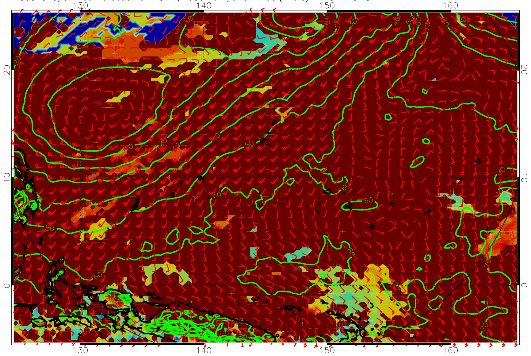
16082018, 54 hour forecast for HCAL, 1000mb Z, and winds (knots) -- NCEP GFS
