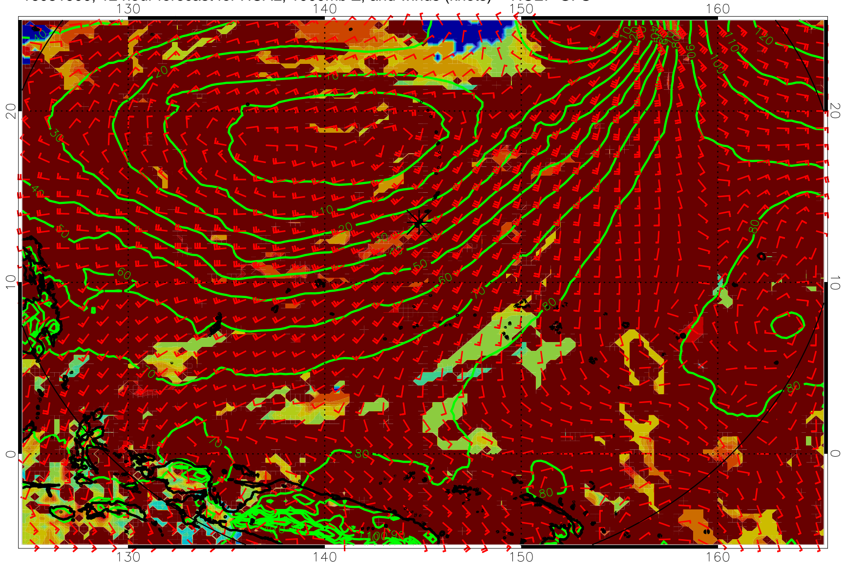
16081900, 12 hour forecast for HCAL, 1000mb Z, and winds (knots) -- NCEP GFS
