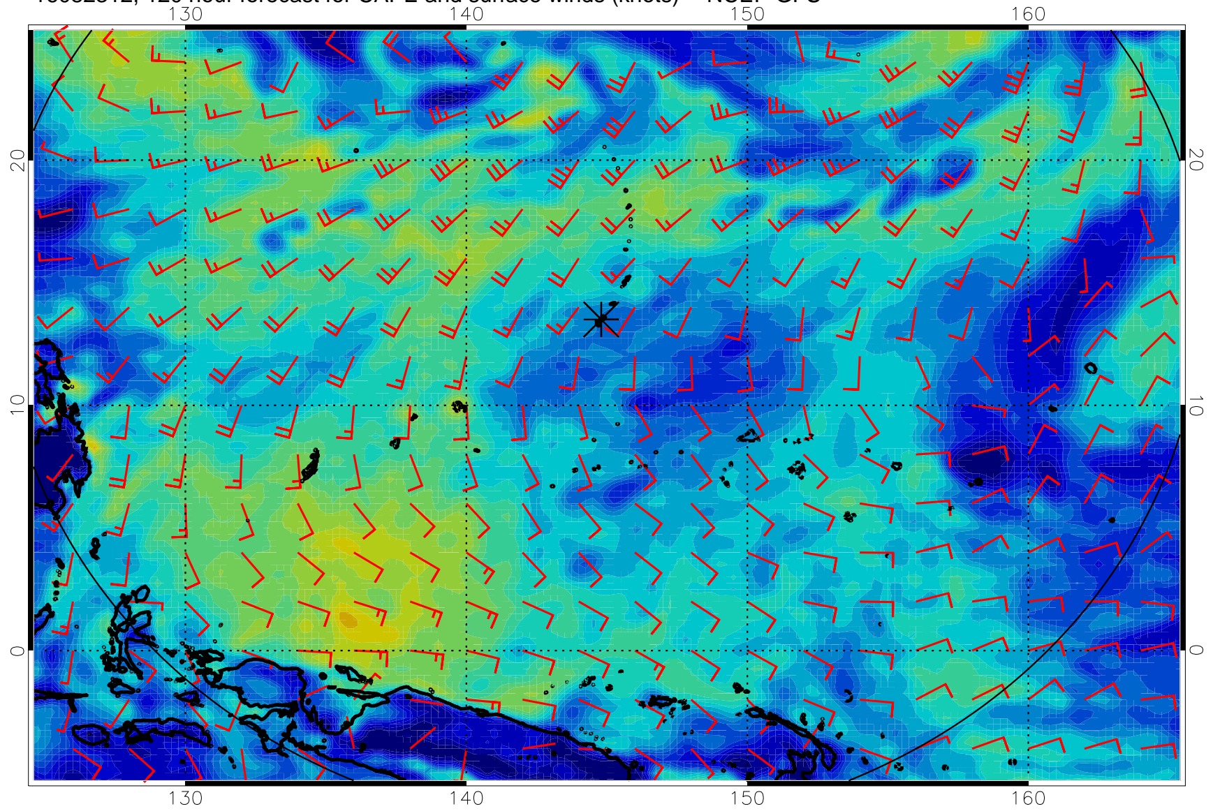
16082312, 120 hour forecast for CAPE and surface winds (knots) -- NCEP GFS
