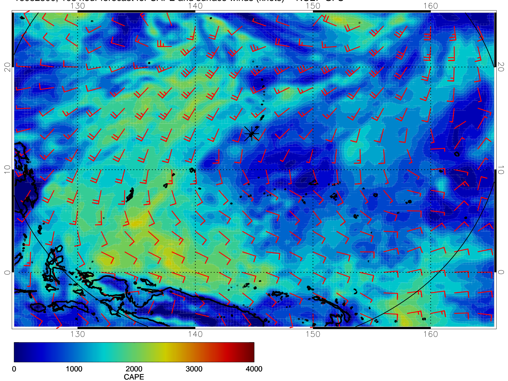
16082300, 108 hour forecast for CAPE and surface winds (knots) -- NCEP GFS
