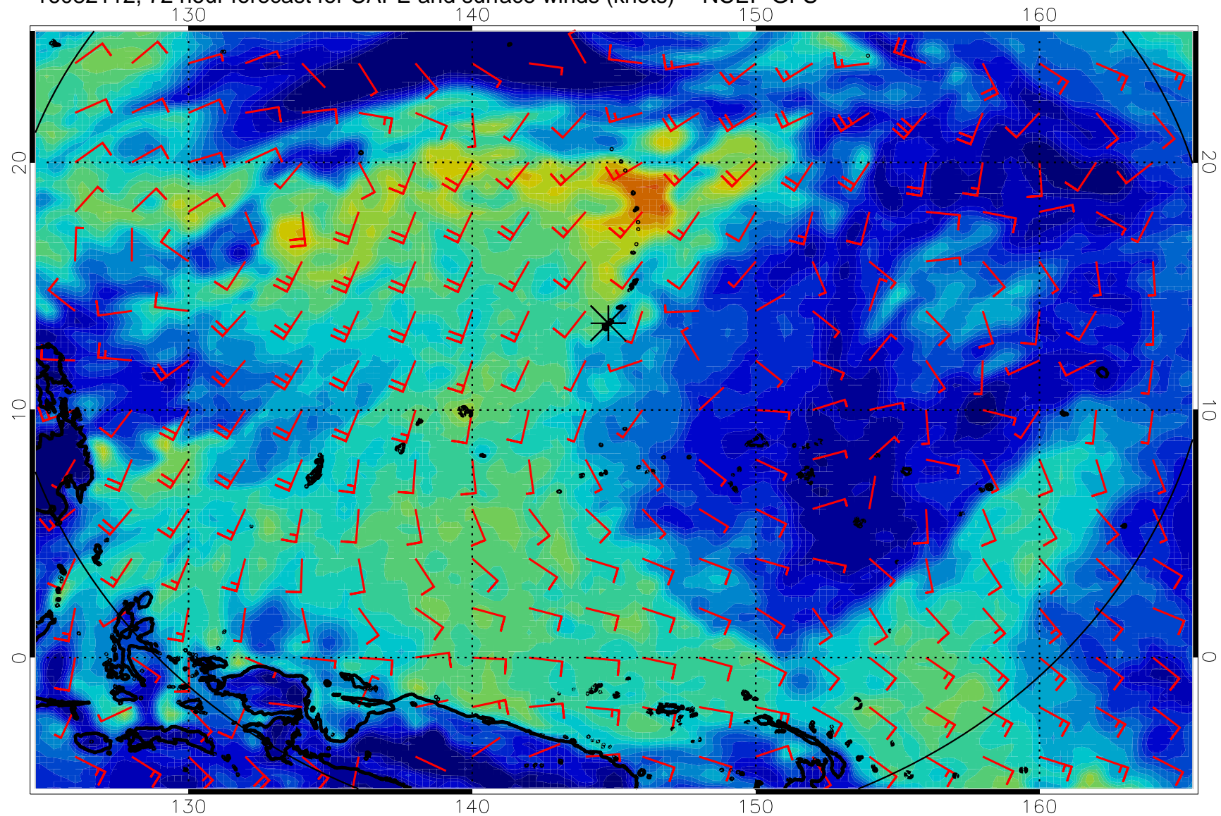
16082112, 72 hour forecast for CAPE and surface winds (knots) -- NCEP GFS
