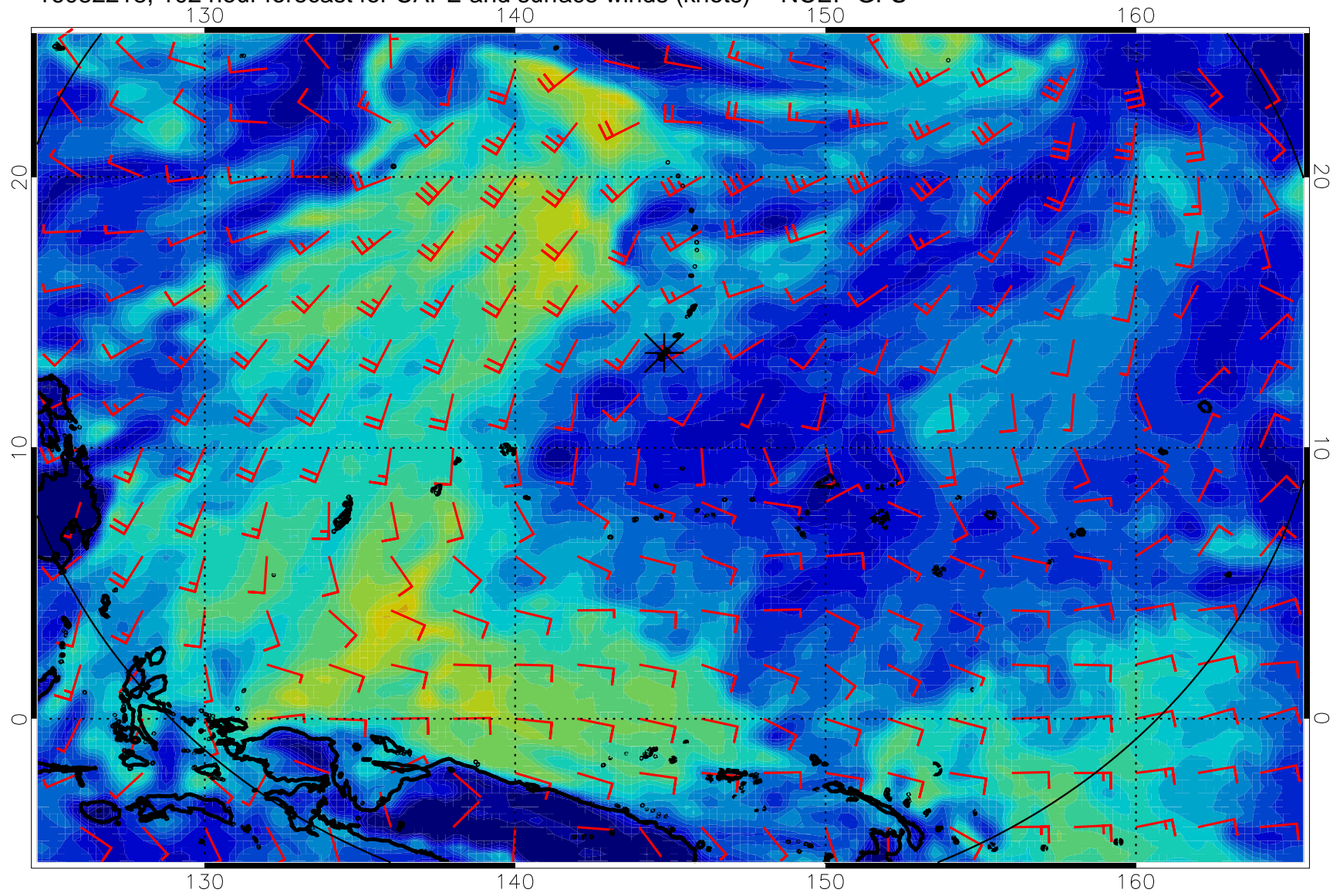
16082218, 102 hour forecast for CAPE and surface winds (knots) -- NCEP GFS
