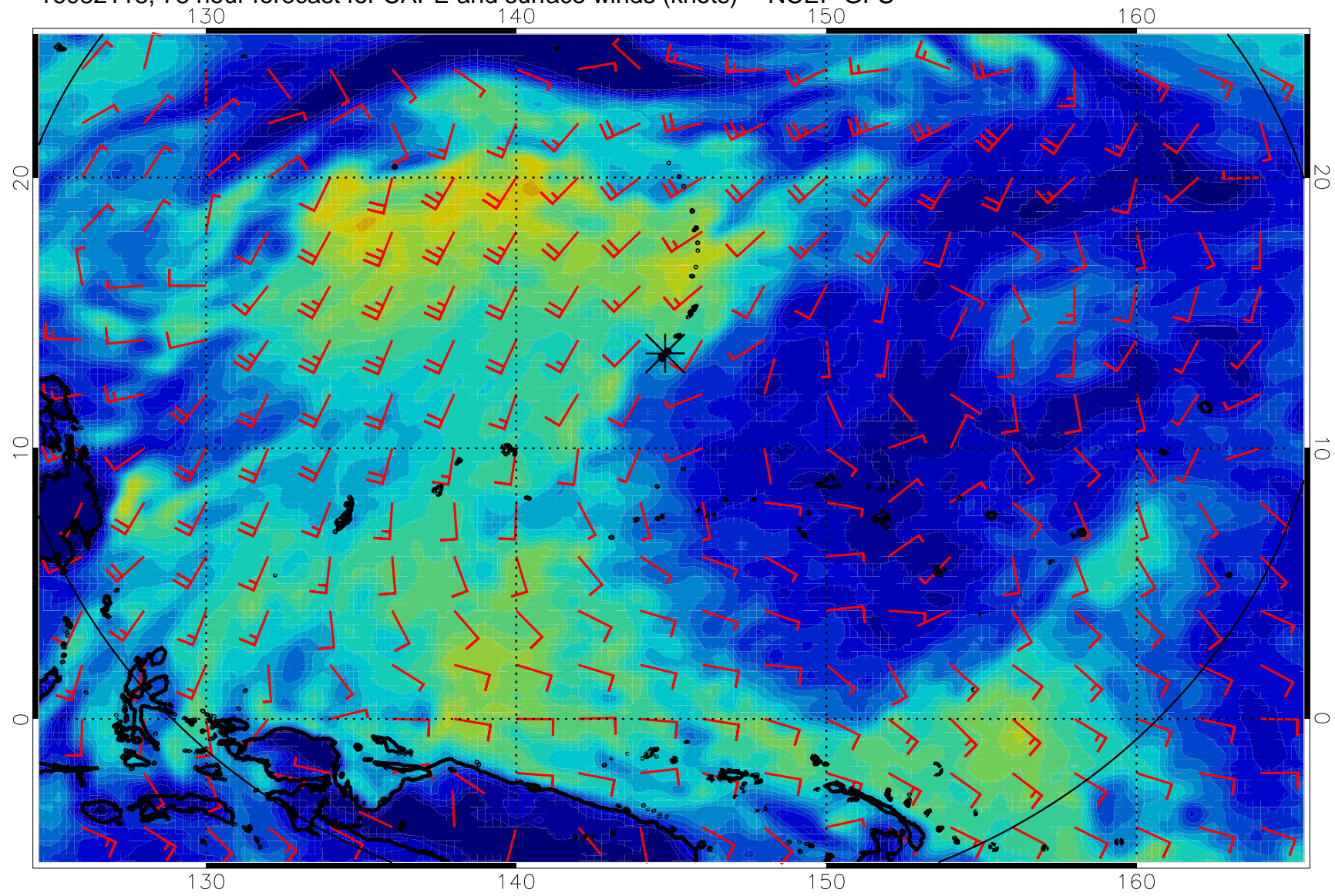
16082118, 78 hour forecast for CAPE and surface winds (knots) -- NCEP GFS
