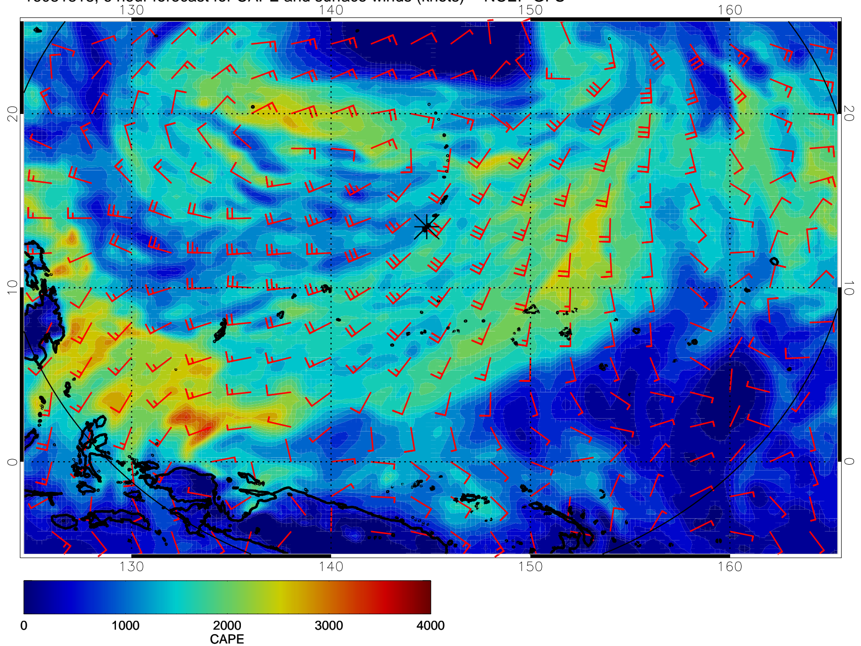
16081818, 6 hour forecast for CAPE and surface winds (knots) -- NCEP GFS
