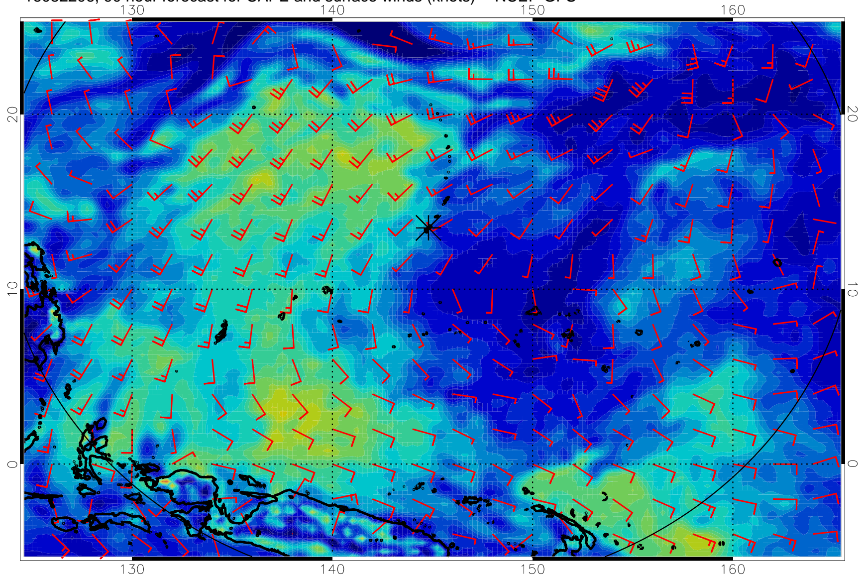
16082206, 90 hour forecast for CAPE and surface winds (knots) -- NCEP GFS
