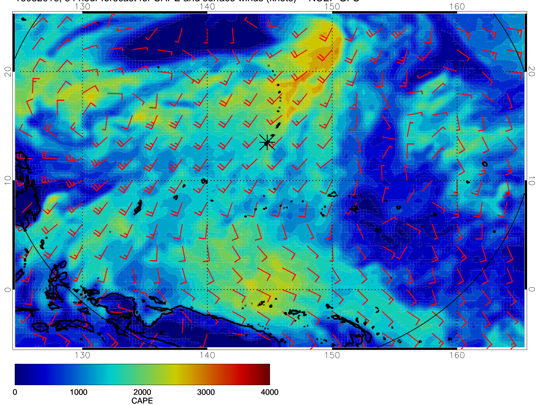
16082018, 54 hour forecast for CAPE and surface winds (knots) -- NCEP GFS
