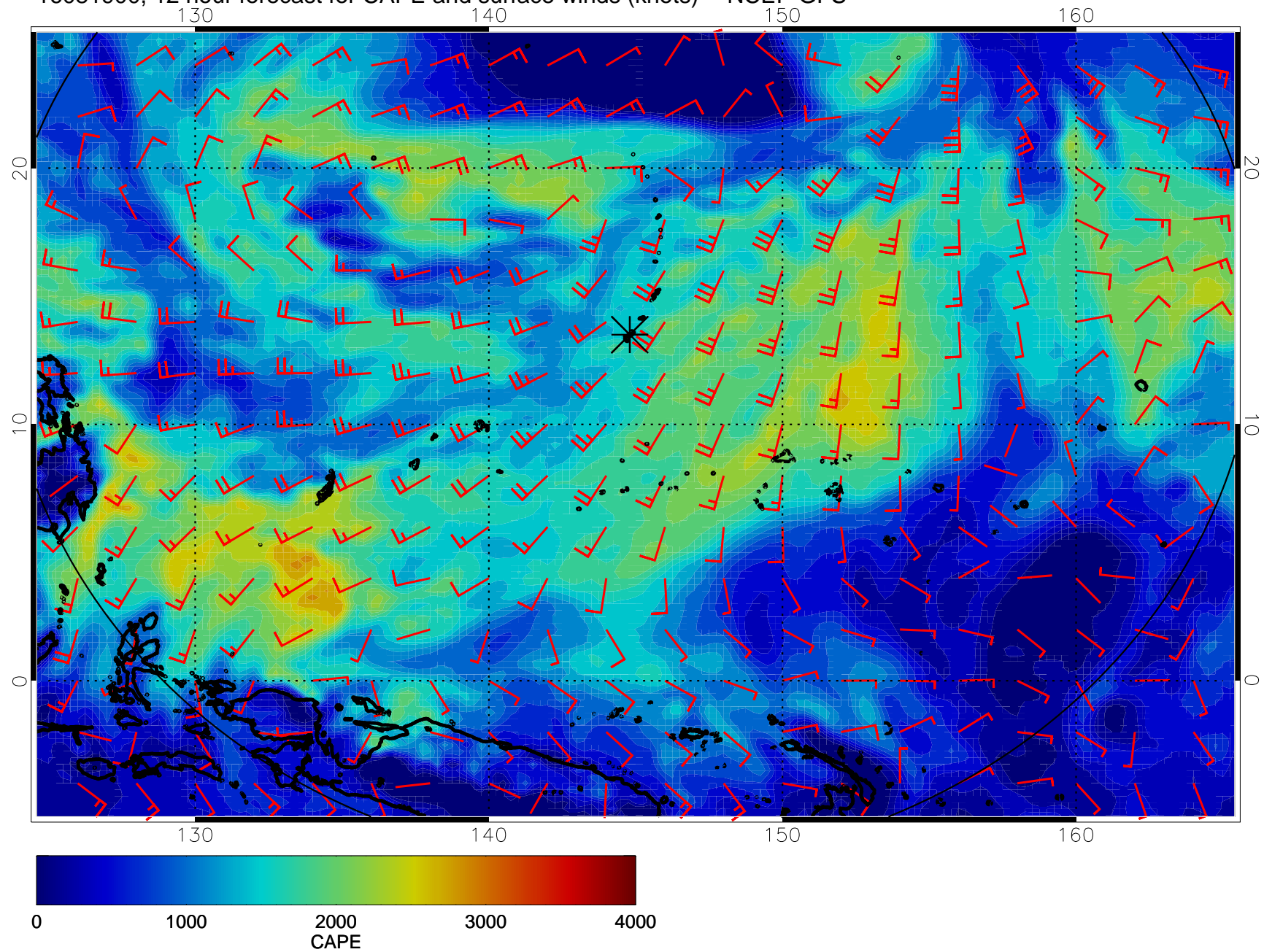
16081900, 12 hour forecast for CAPE and surface winds (knots) -- NCEP GFS
