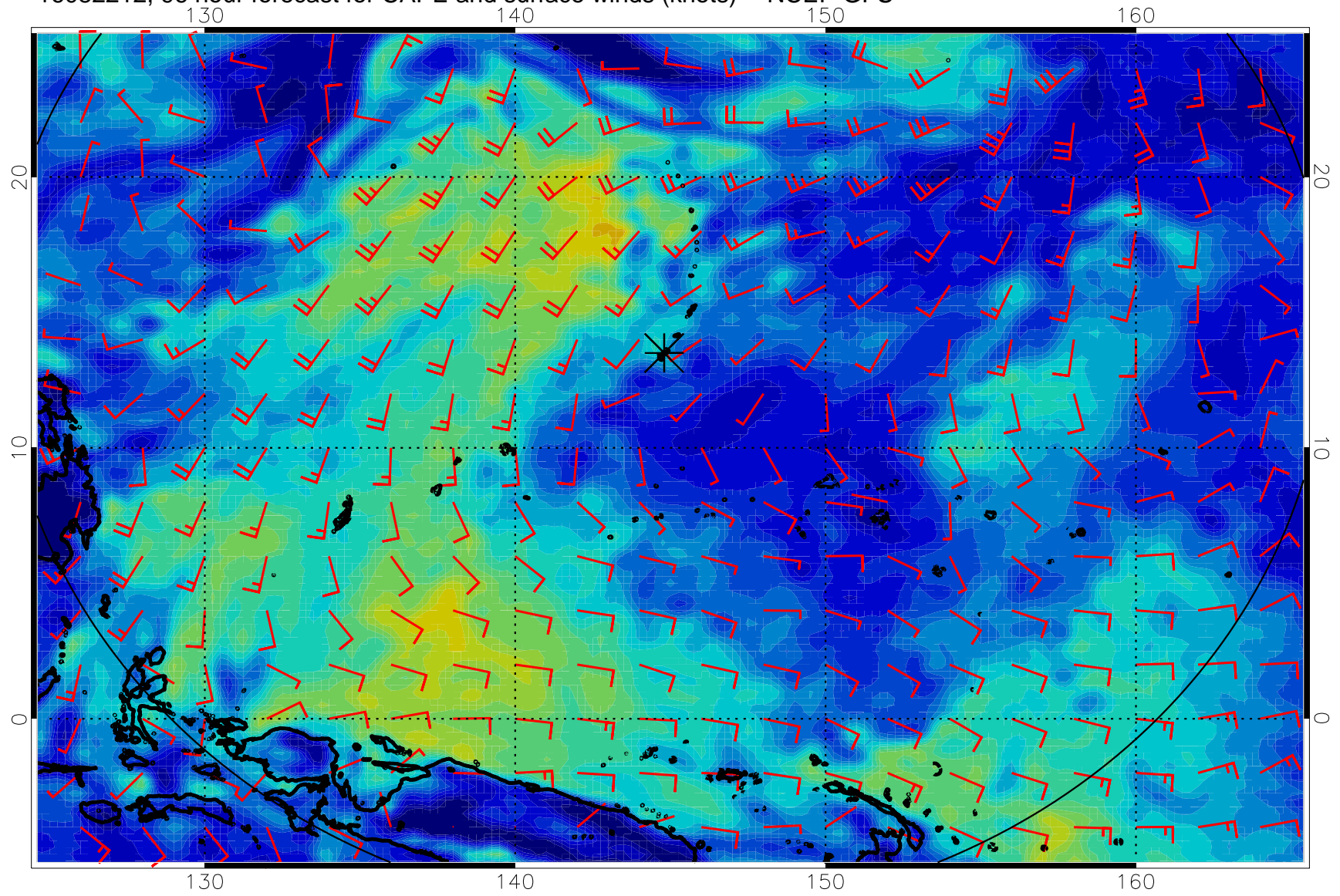
16082212, 96 hour forecast for CAPE and surface winds (knots) -- NCEP GFS
