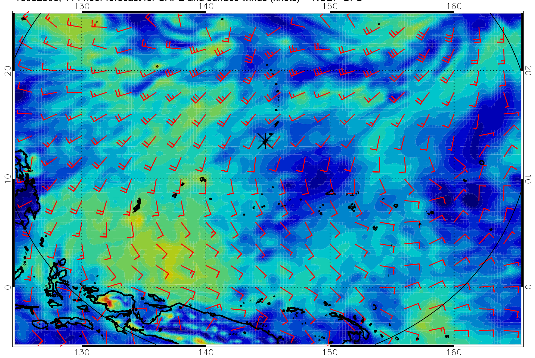
16082306, 114 hour forecast for CAPE and surface winds (knots) -- NCEP GFS
