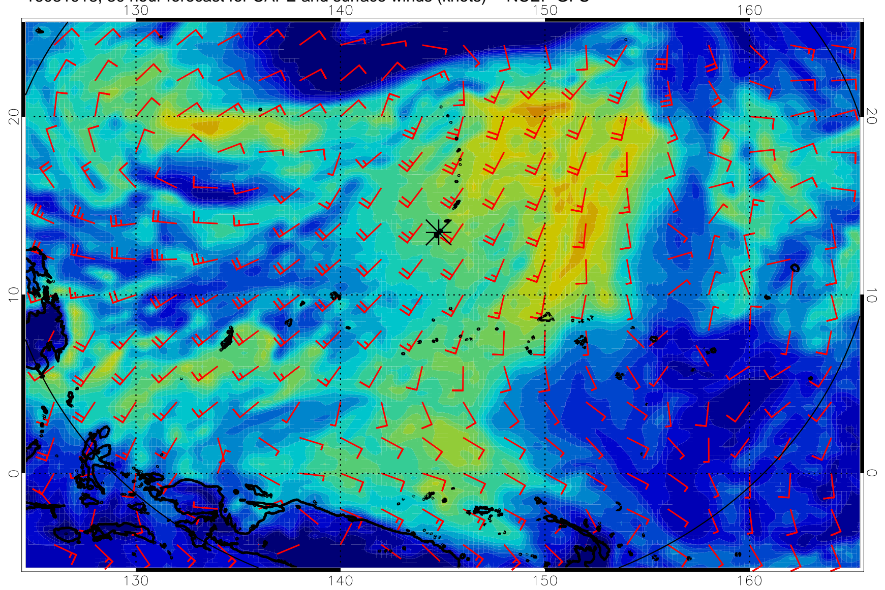
16081918, 30 hour forecast for CAPE and surface winds (knots) -- NCEP GFS
