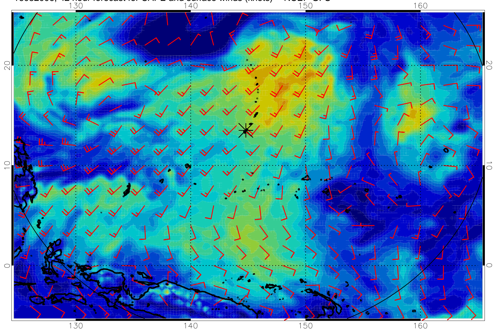
16082006, 42 hour forecast for CAPE and surface winds (knots) -- NCEP GFS
