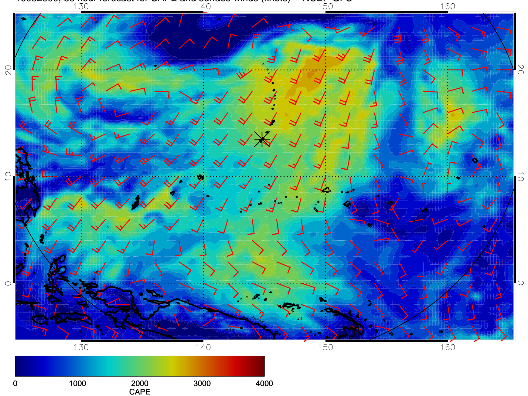
16082000, 36 hour forecast for CAPE and surface winds (knots) -- NCEP GFS
