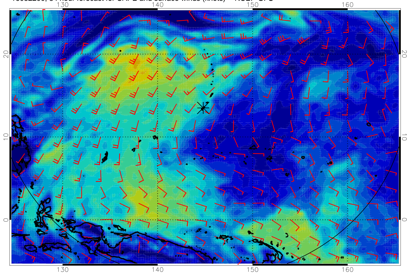
16082200, 84 hour forecast for CAPE and surface winds (knots) -- NCEP GFS
