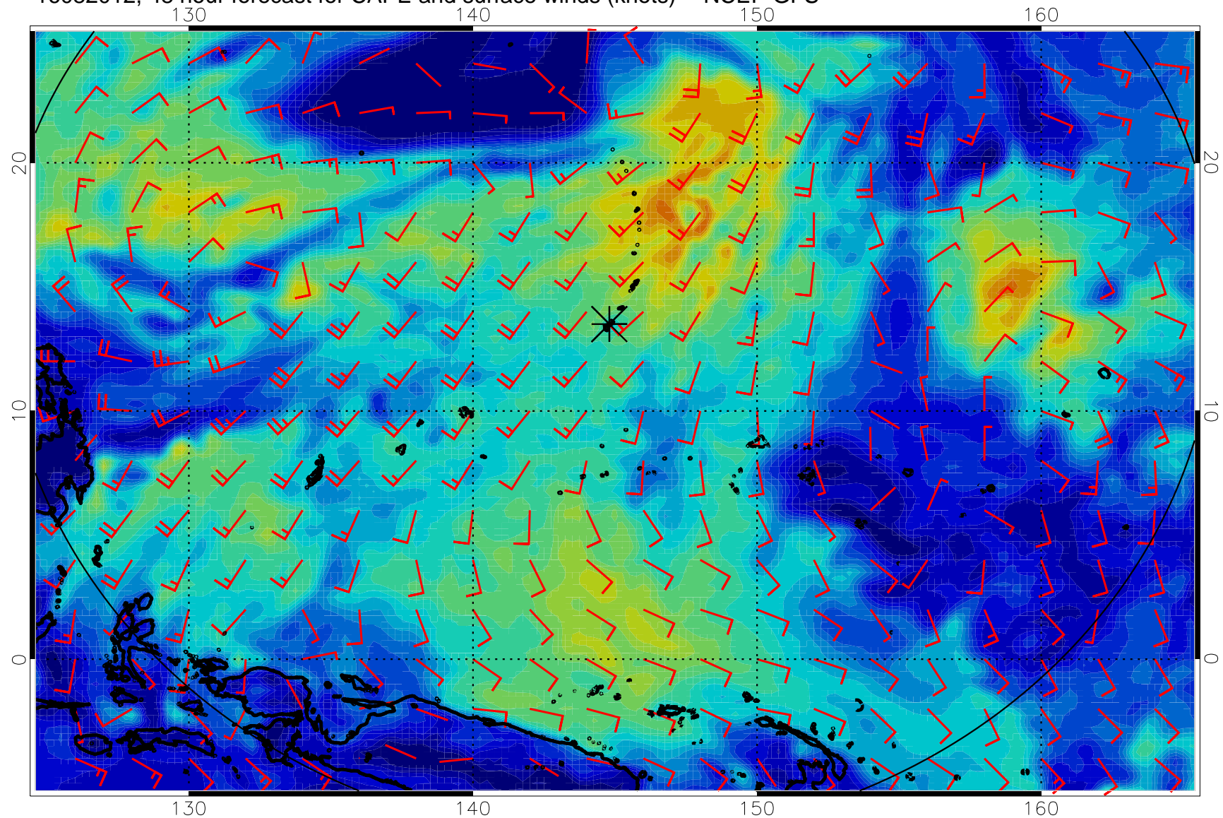
16082012, 48 hour forecast for CAPE and surface winds (knots) -- NCEP GFS
