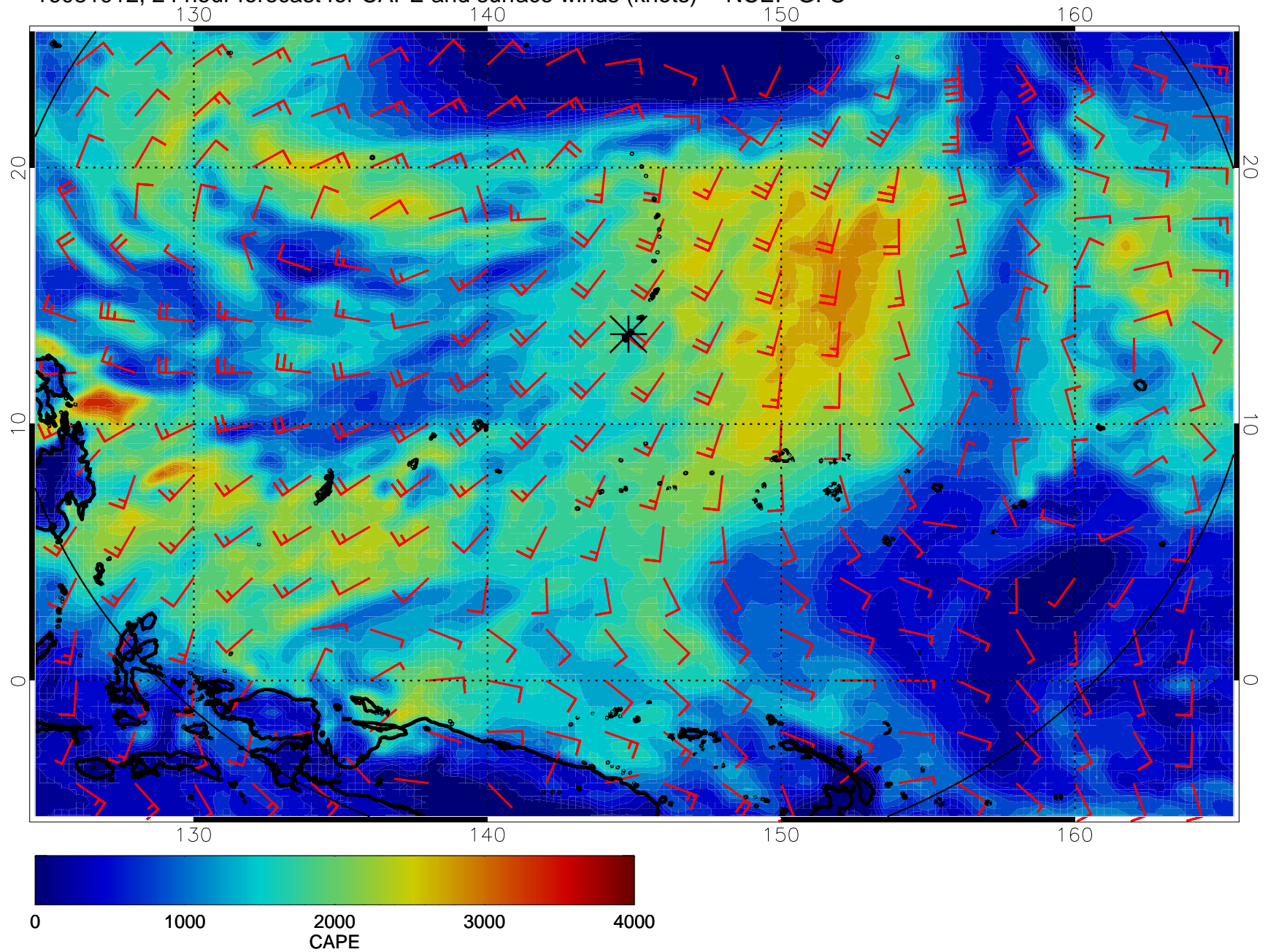
16081912, 24 hour forecast for CAPE and surface winds (knots) -- NCEP GFS
