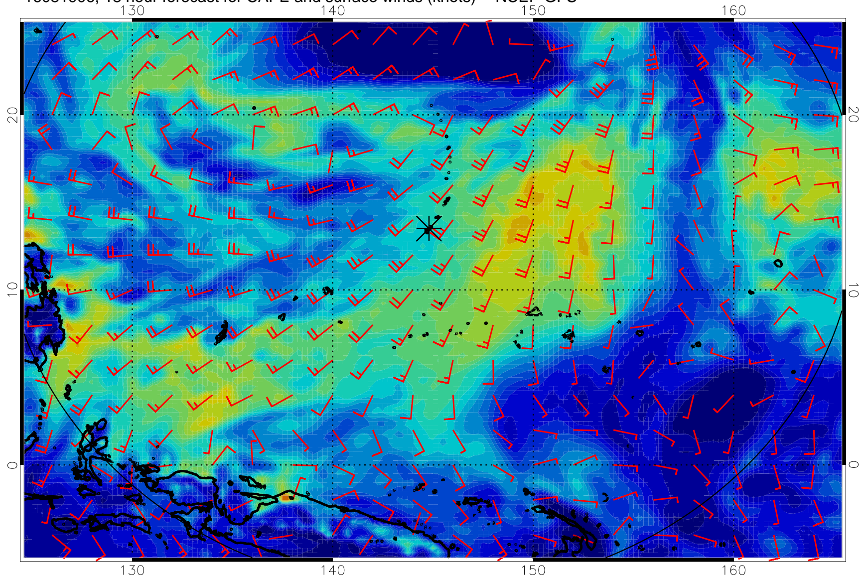
16081906, 18 hour forecast for CAPE and surface winds (knots) -- NCEP GFS
