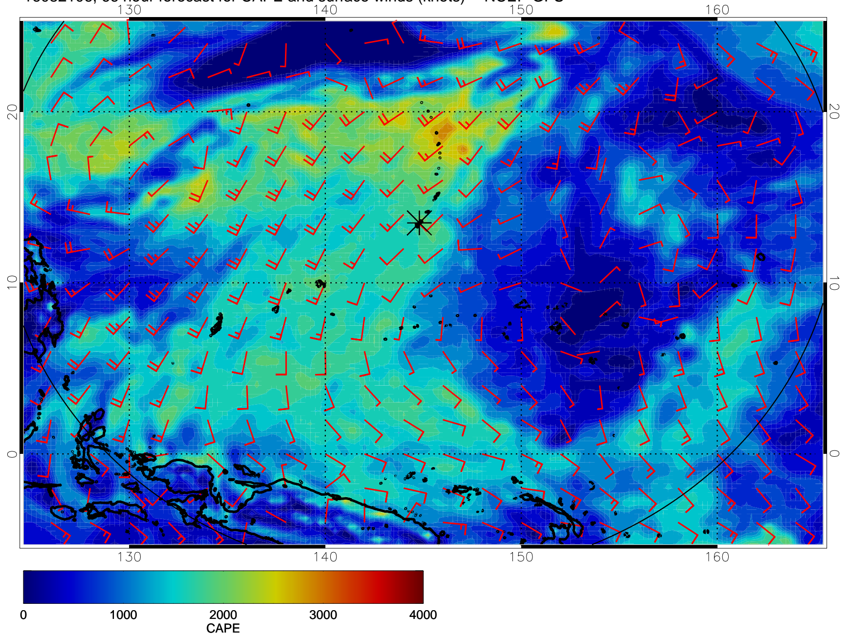
16082106, 66 hour forecast for CAPE and surface winds (knots) -- NCEP GFS
