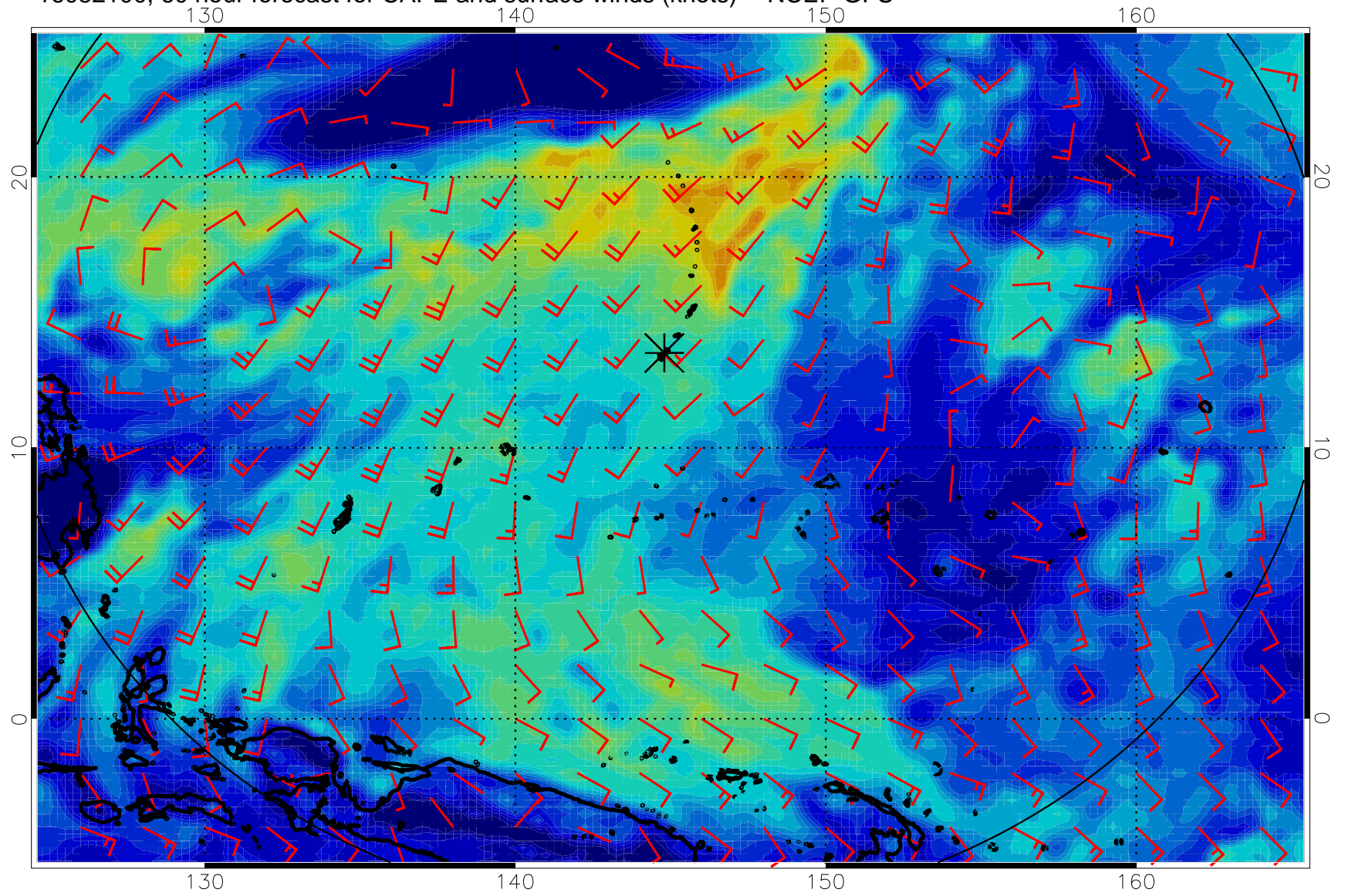
16082100, 60 hour forecast for CAPE and surface winds (knots) -- NCEP GFS
