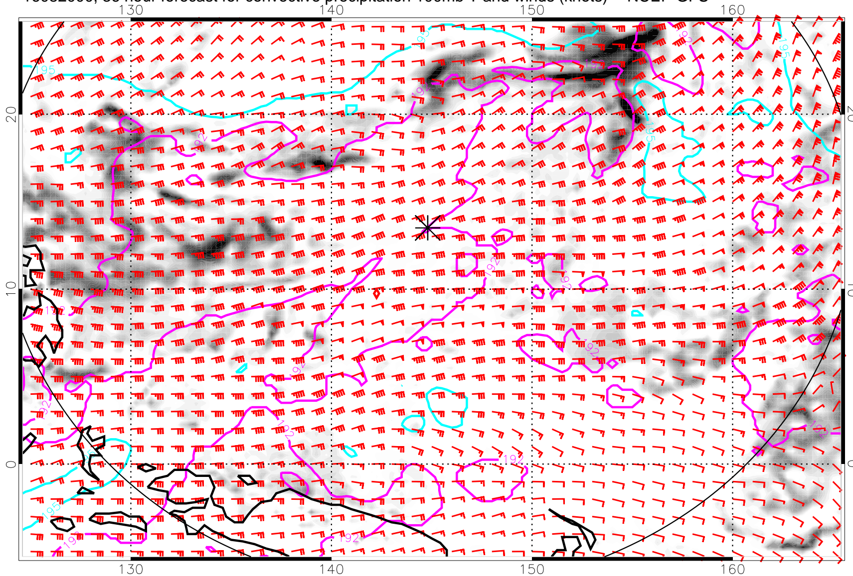
16082000, 36 hour forecast for convective precipitation 100mb T and winds (knots) -- NCEP GFS
