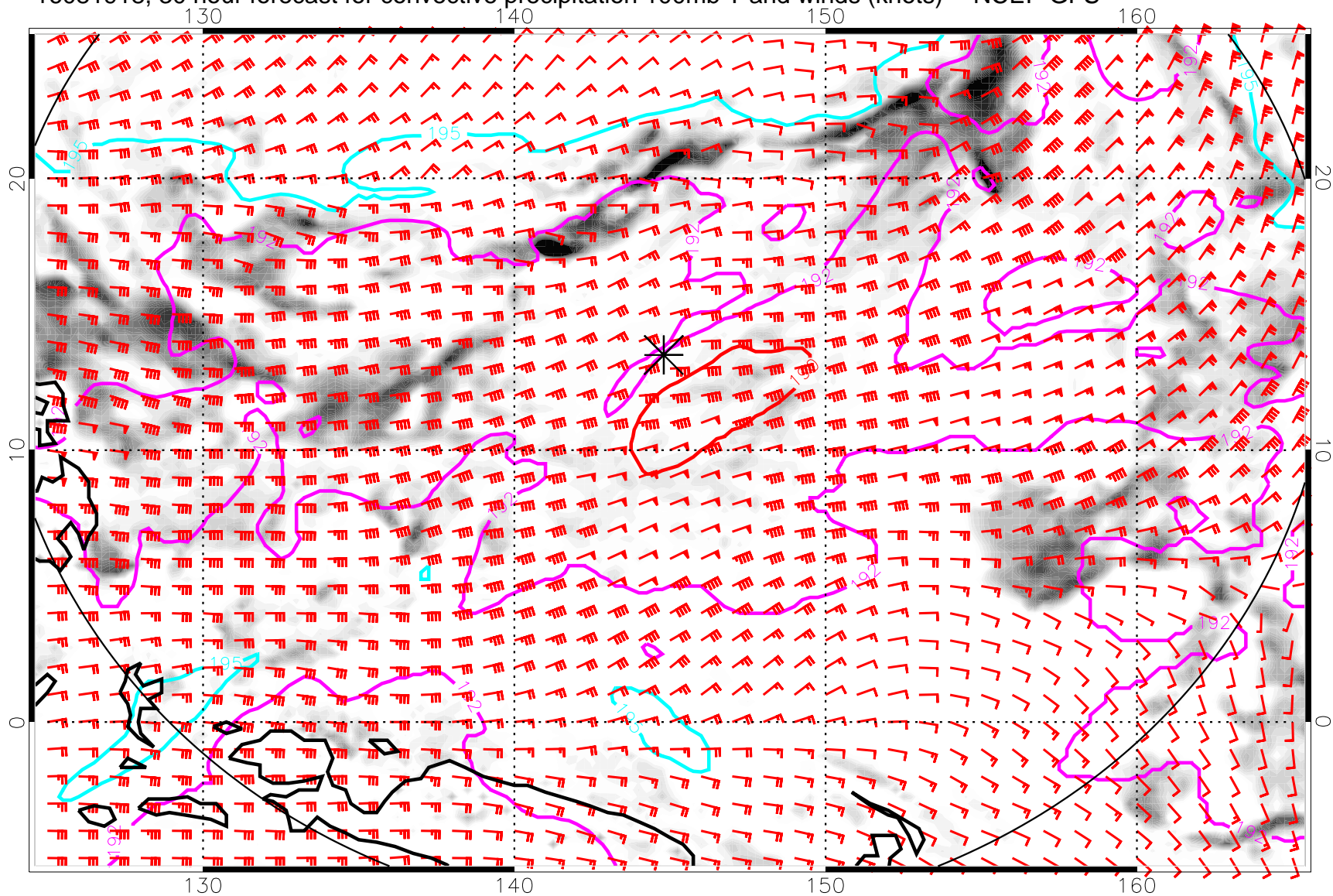
16081918, 30 hour forecast for convective precipitation 100mb T and winds (knots) -- NCEP GFS
