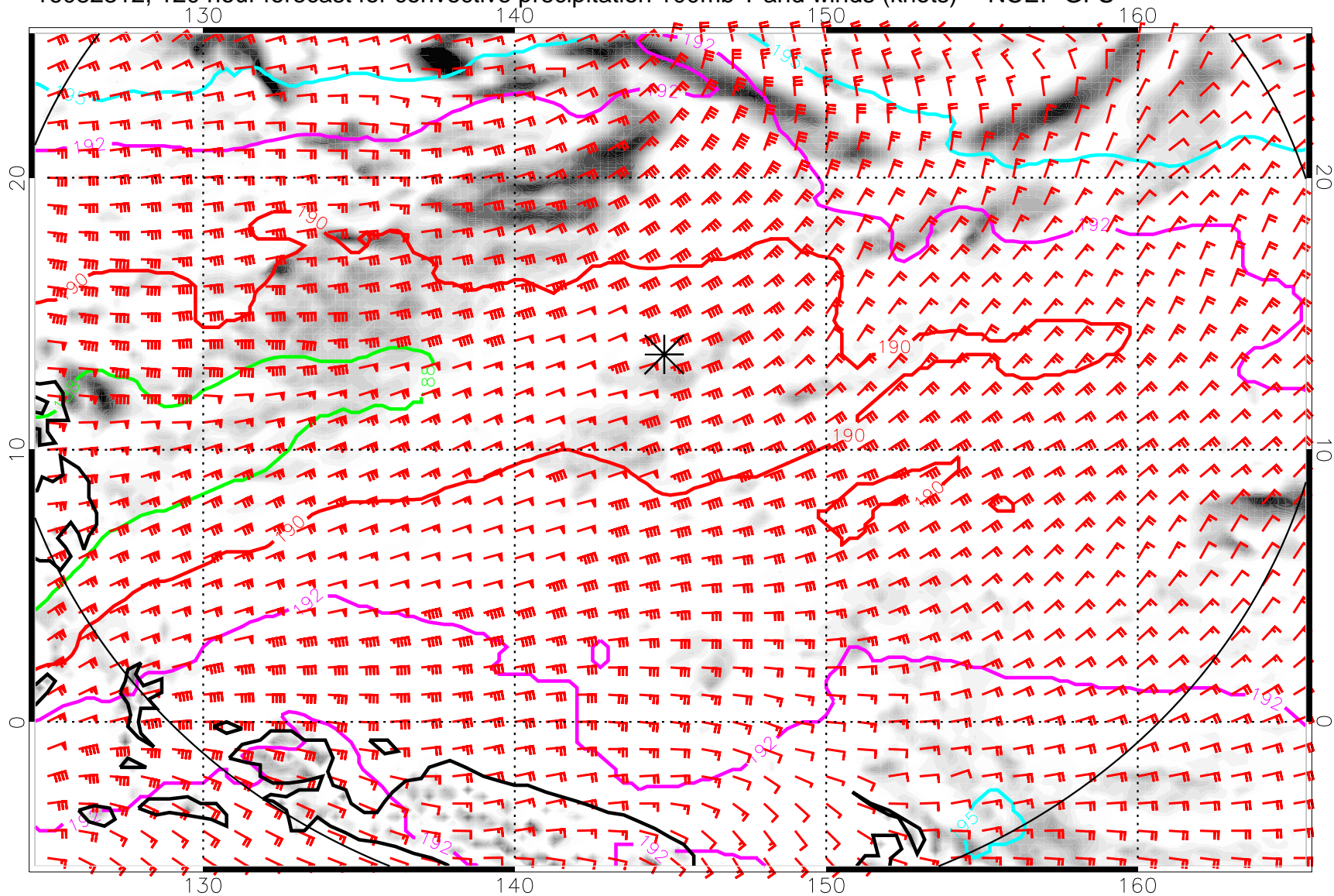
16082312, 120 hour forecast for convective precipitation 100mb T and winds (knots) -- NCEP GFS
