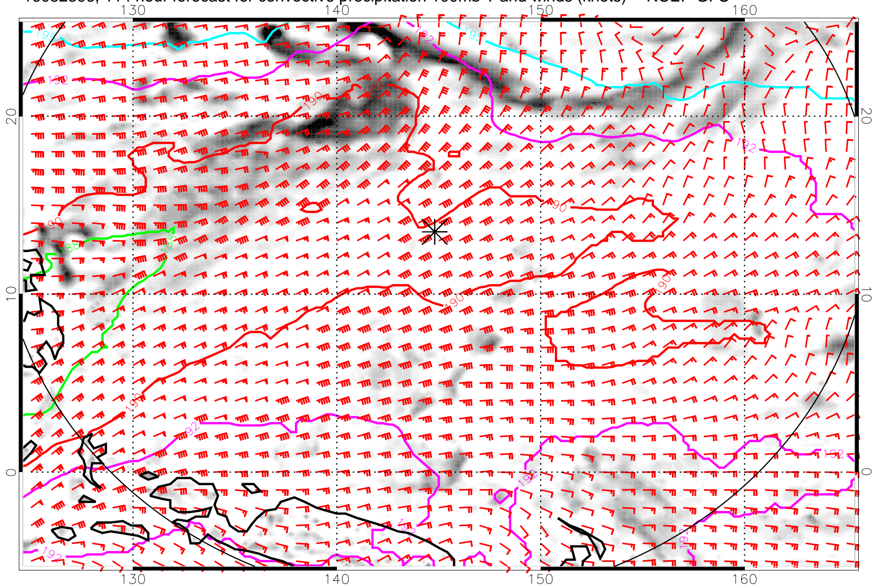
16082306, 114 hour forecast for convective precipitation 100mb T and winds (knots) -- NCEP GFS
