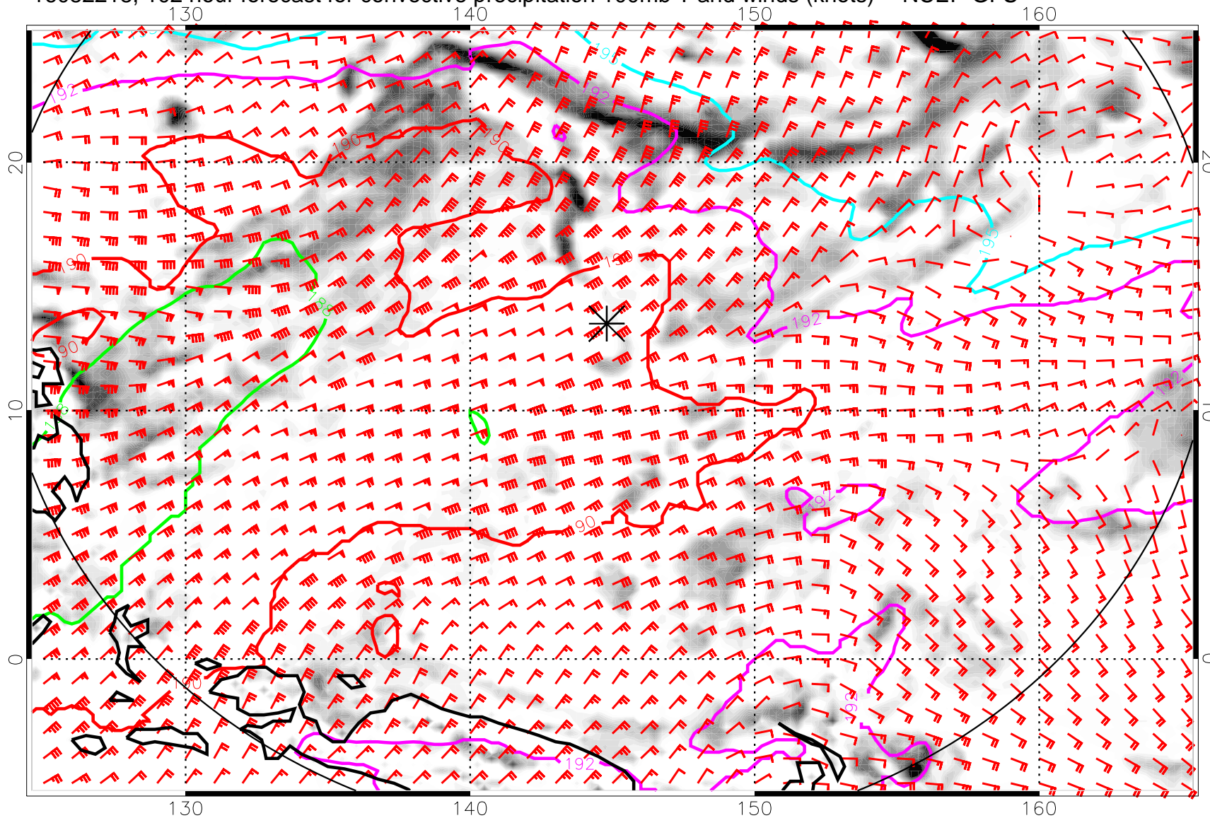
16082218, 102 hour forecast for convective precipitation 100mb T and winds (knots) -- NCEP GFS
