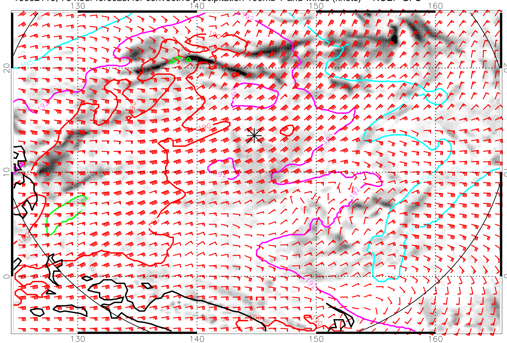
16082118, 78 hour forecast for convective precipitation 100mb T and winds (knots) -- NCEP GFS
