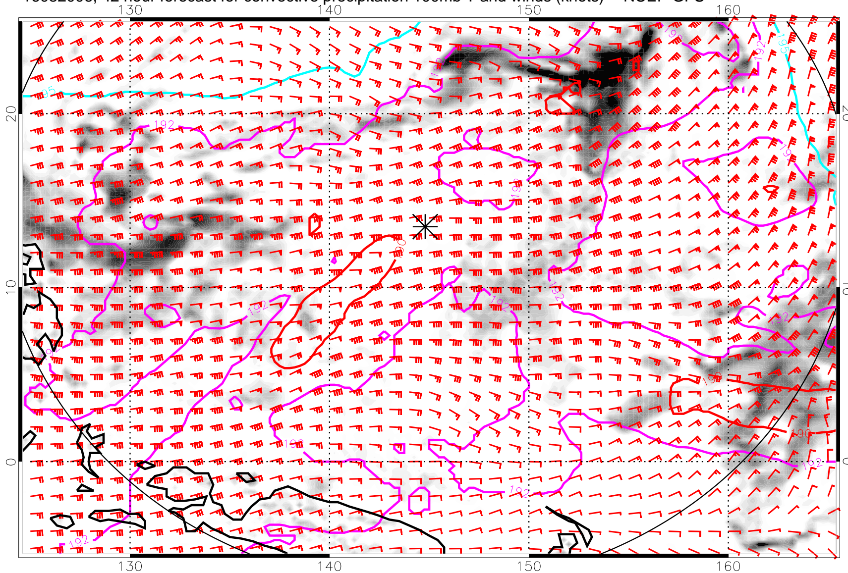
16082006, 42 hour forecast for convective precipitation 100mb T and winds (knots) -- NCEP GFS
