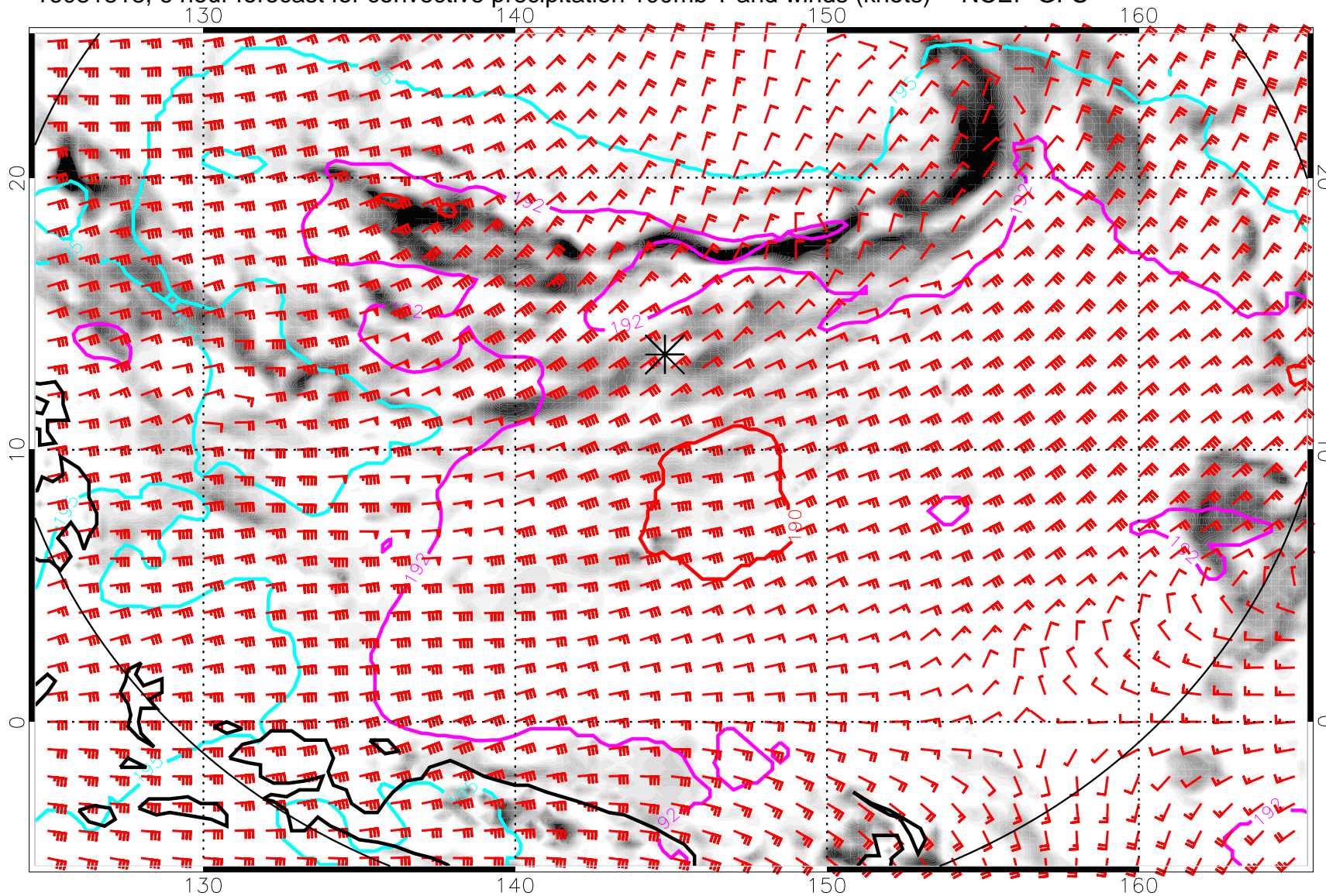
16081818, 6 hour forecast for convective precipitation 100mb T and winds (knots) -- NCEP GFS
