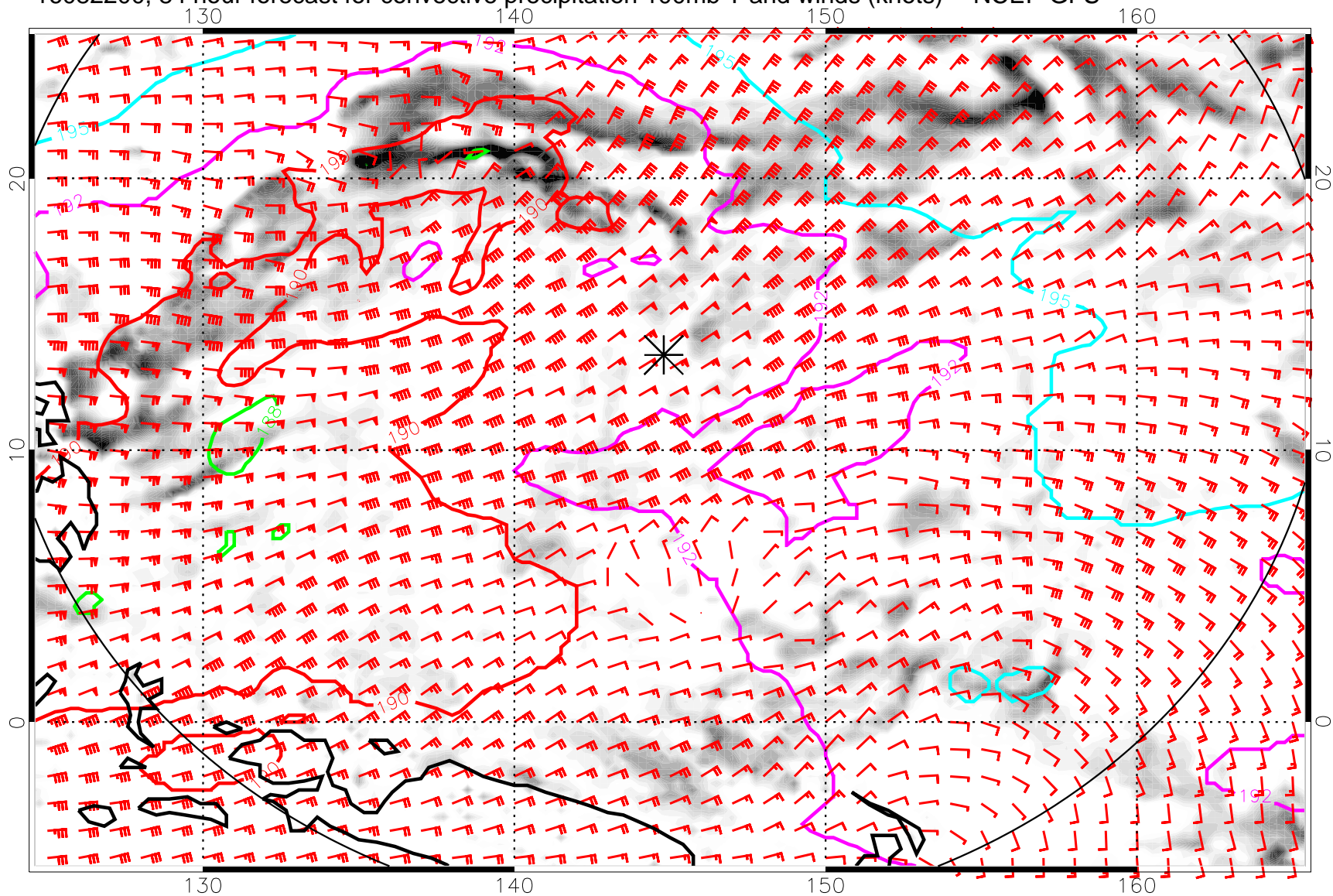
16082200, 84 hour forecast for convective precipitation 100mb T and winds (knots) -- NCEP GFS
