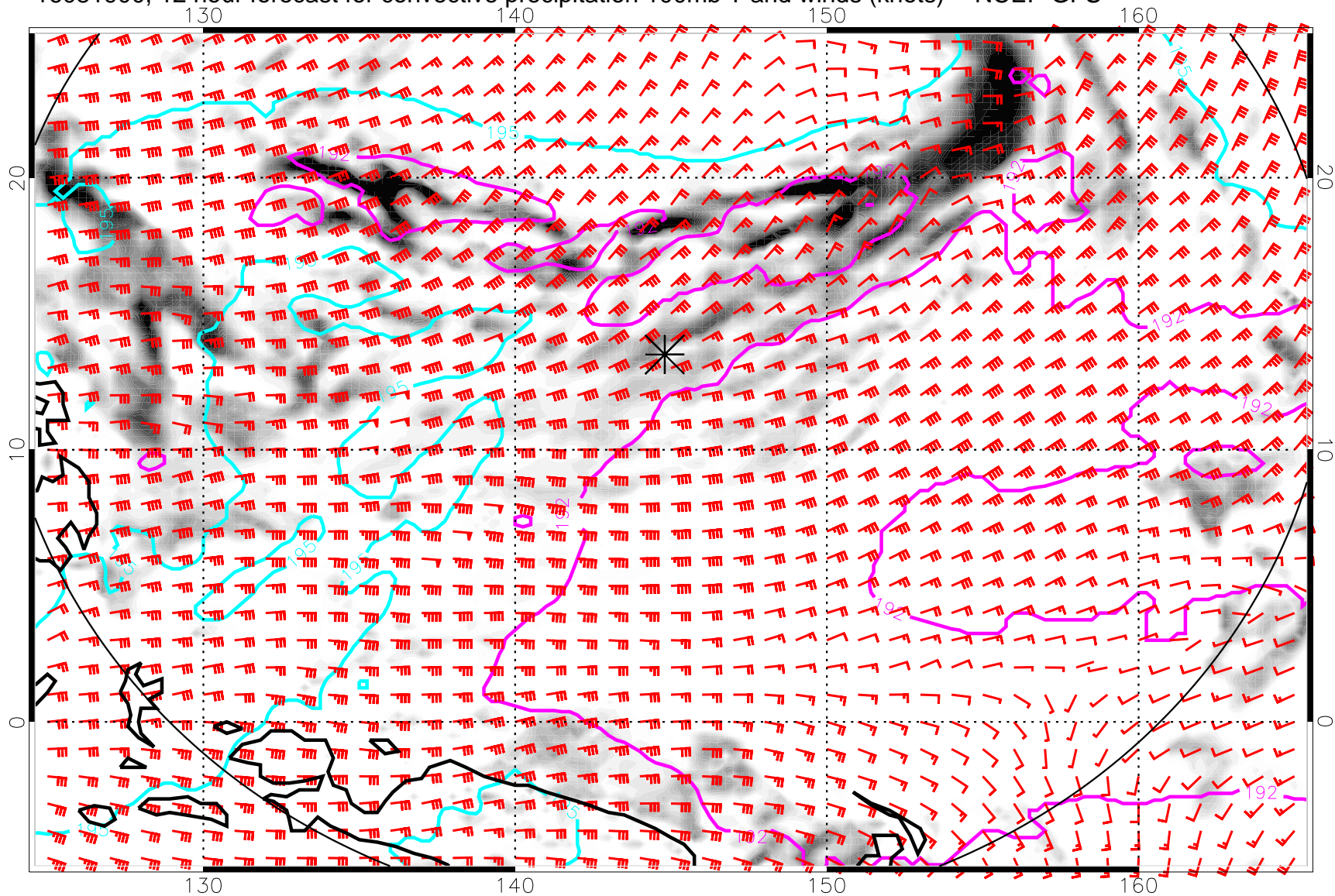
16081900, 12 hour forecast for convective precipitation 100mb T and winds (knots) -- NCEP GFS
