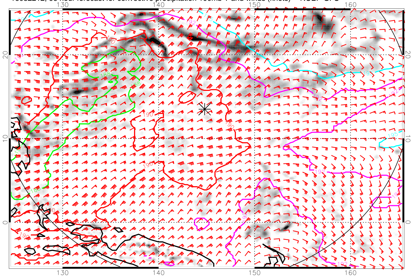
16082212, 96 hour forecast for convective precipitation 100mb T and winds (knots) -- NCEP GFS
