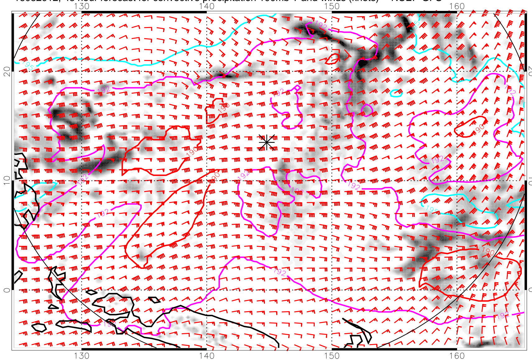
16082012, 48 hour forecast for convective precipitation 100mb T and winds (knots) -- NCEP GFS
