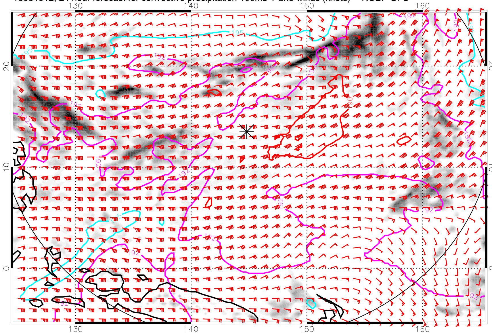
16081912, 24 hour forecast for convective precipitation 100mb T and winds (knots) -- NCEP GFS
