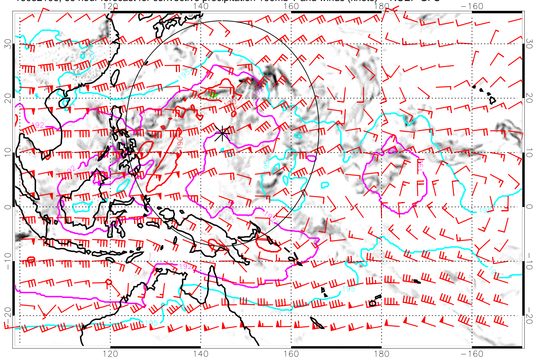
16082106, 66 hour forecast for convective precipitation 100mb T and winds (knots) -- NCEP GFS
