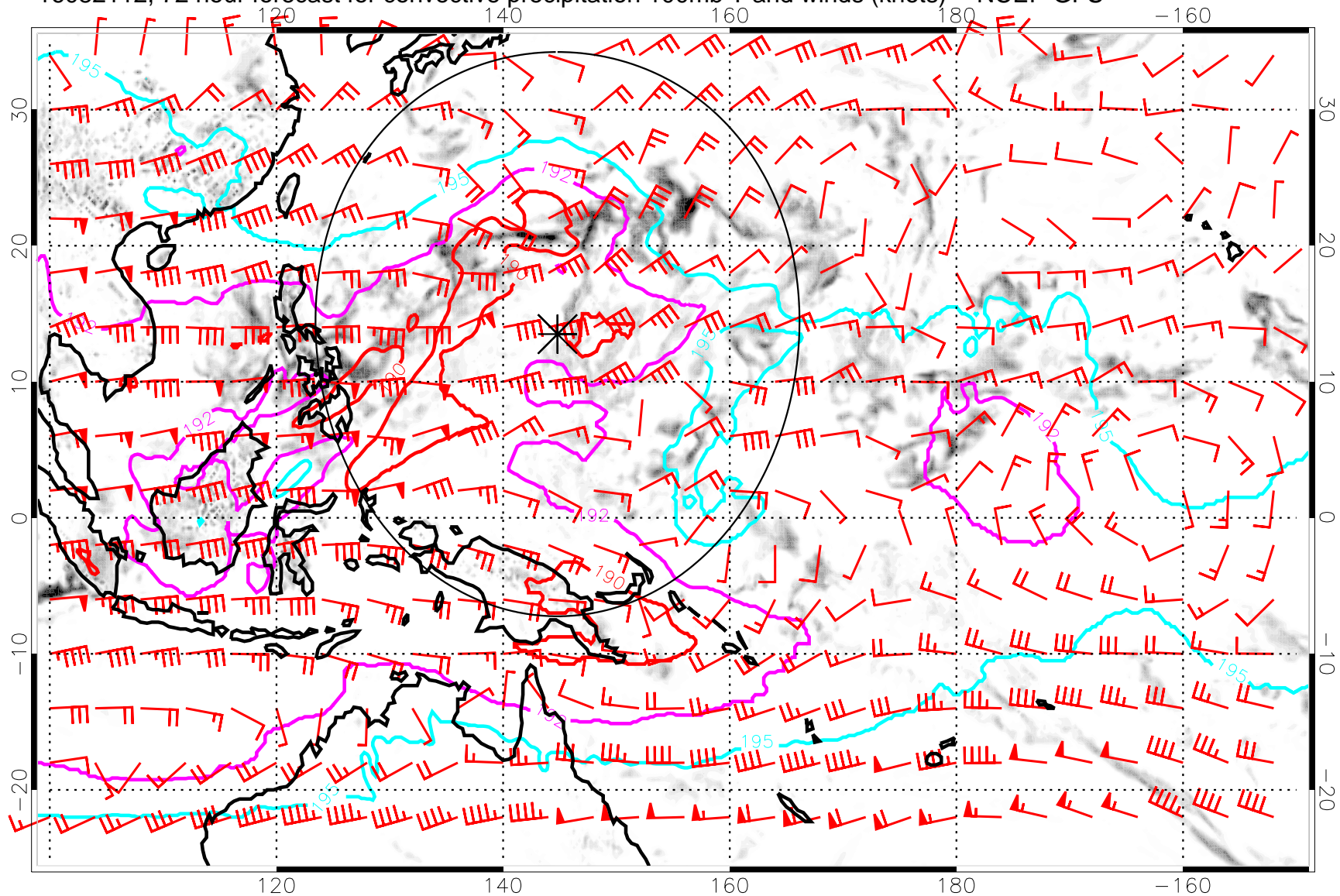
16082112, 72 hour forecast for convective precipitation 100mb T and winds (knots) -- NCEP GFS
