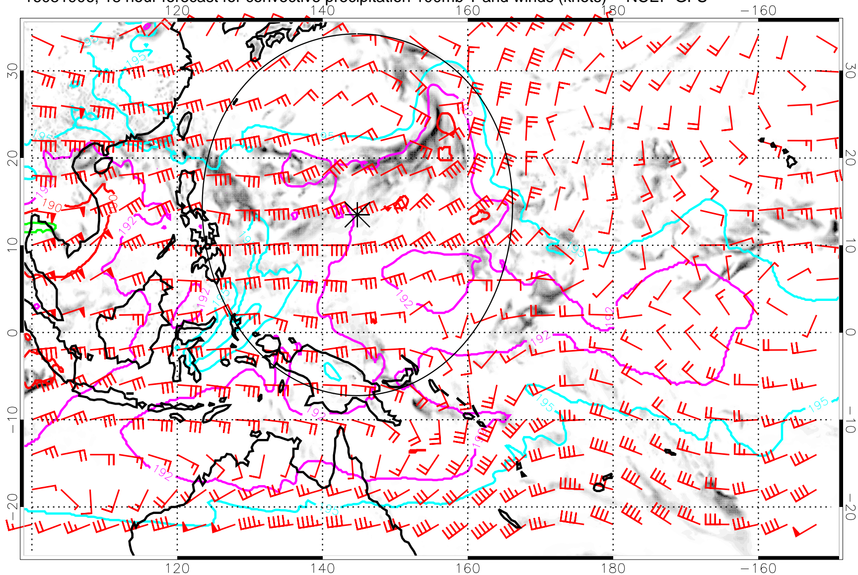
16081906, 18 hour forecast for convective precipitation 100mb T and winds (knots) -- NCEP GFS
