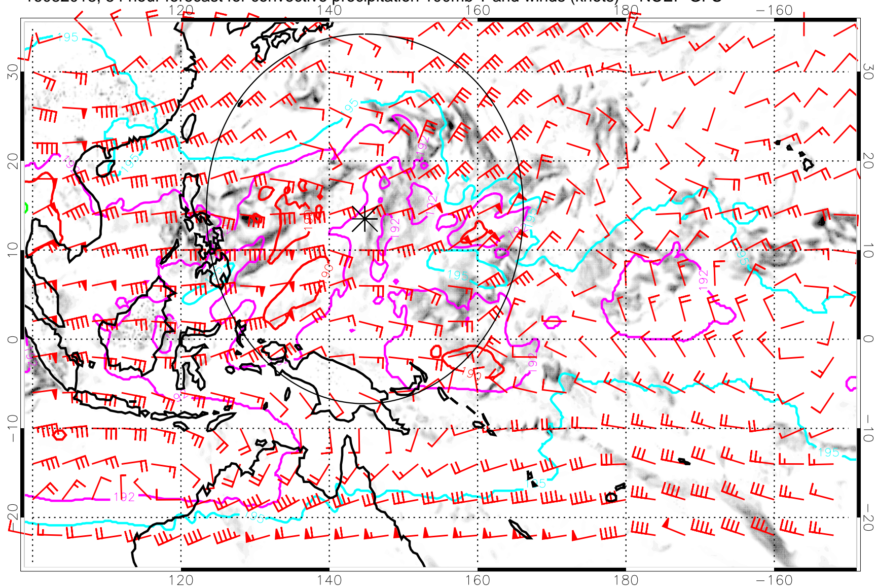
16082018, 54 hour forecast for convective precipitation 100mb T and winds (knots) -- NCEP GFS
