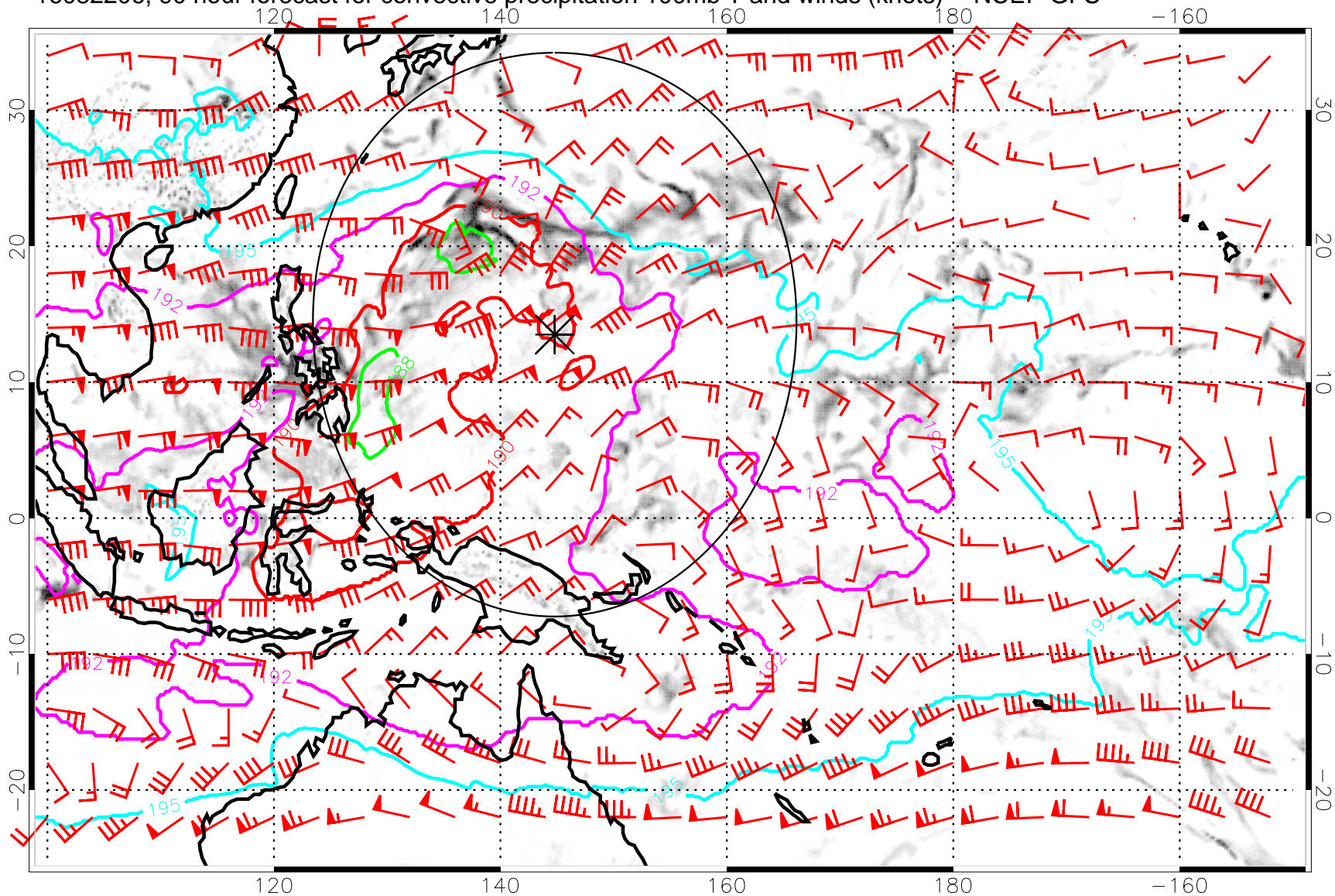
16082206, 90 hour forecast for convective precipitation 100mb T and winds (knots) -- NCEP GFS
