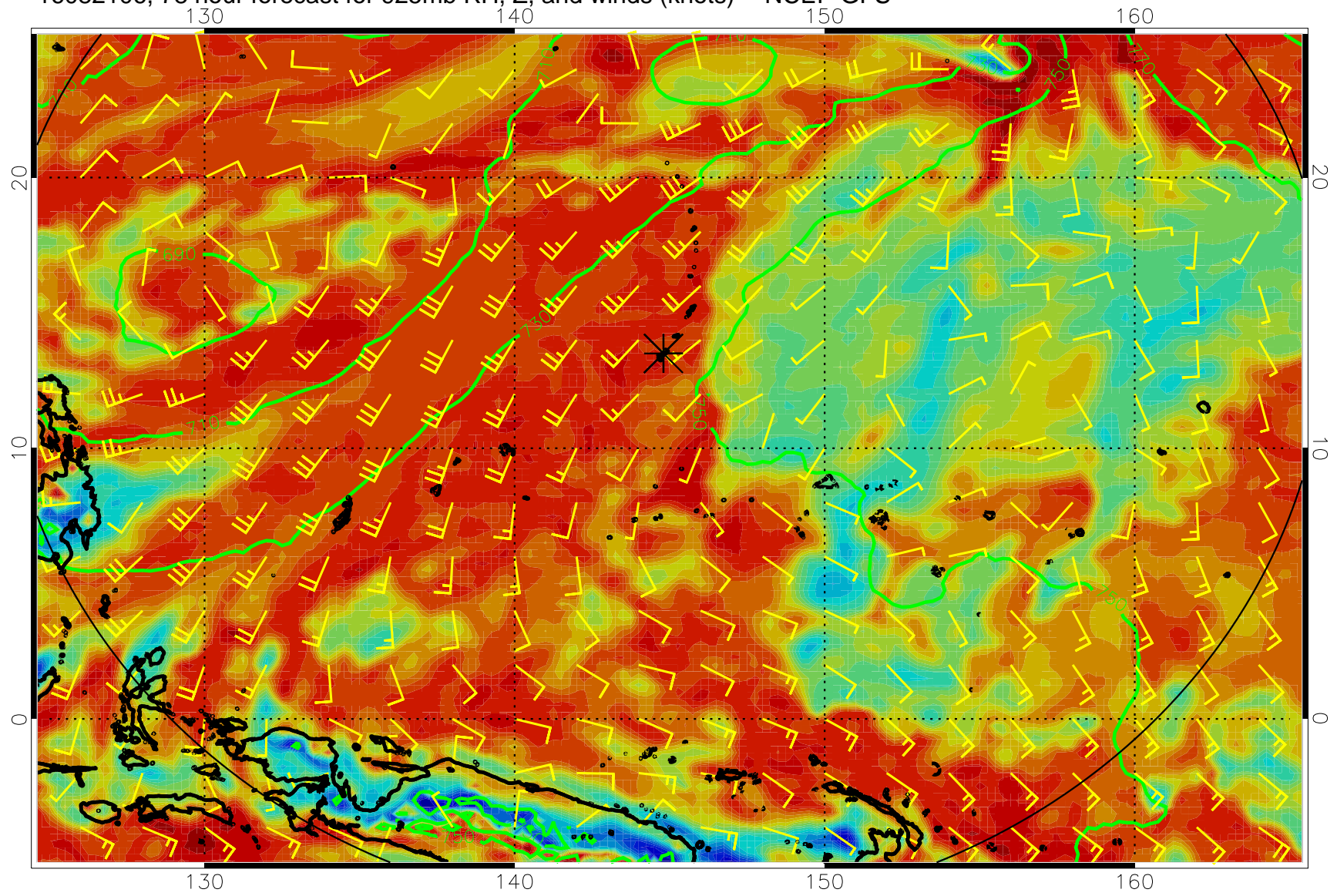
16082106, 78 hour forecast for 925mb RH, Z, and winds (knots) -- NCEP GFS
