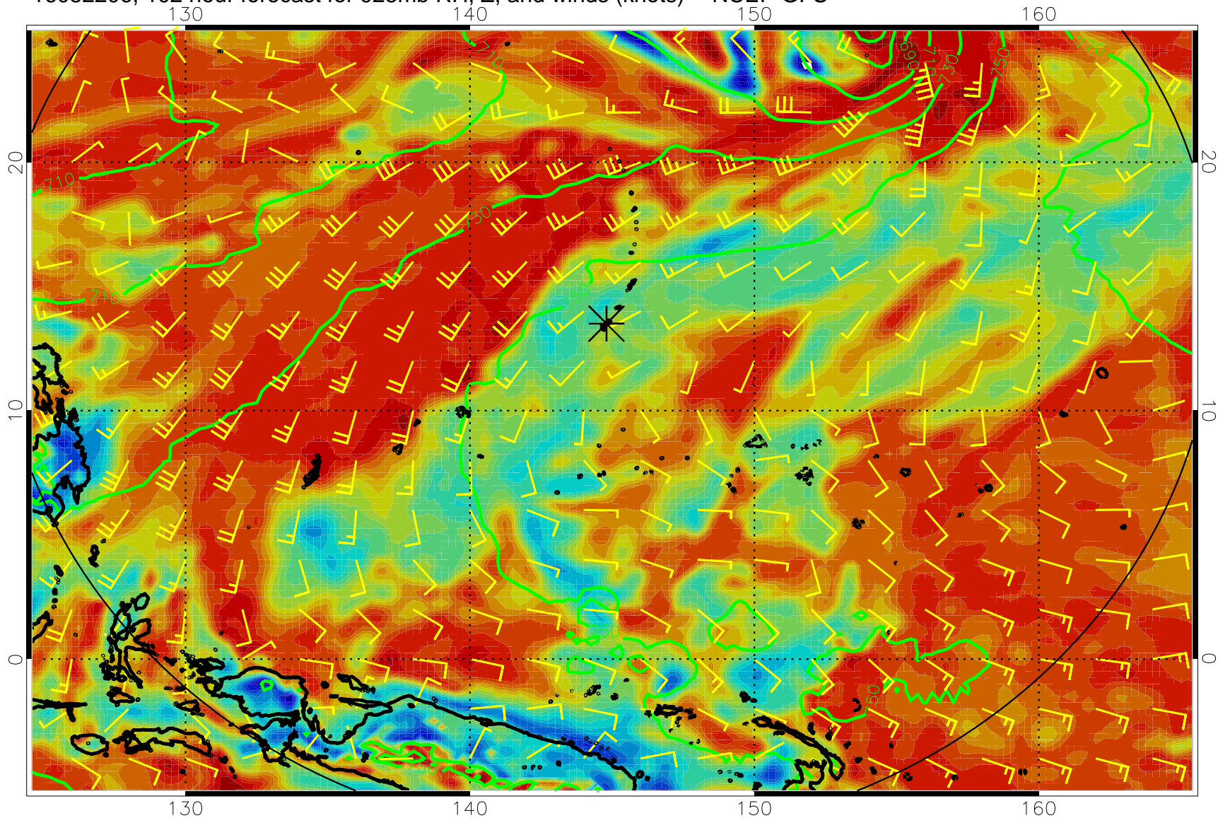
16082206, 102 hour forecast for 925mb RH, Z, and winds (knots) -- NCEP GFS
