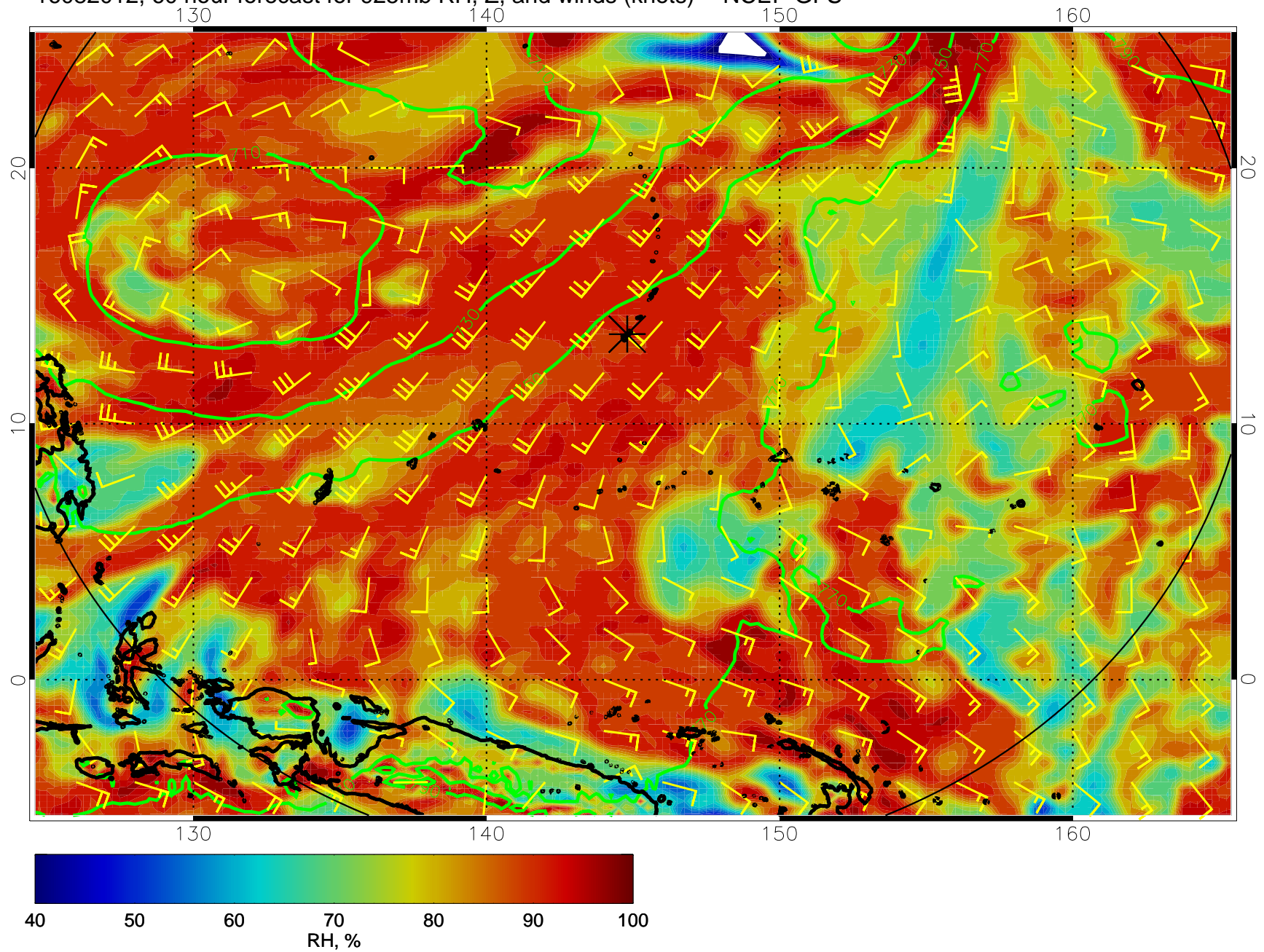
16082012, 60 hour forecast for 925mb RH, Z, and winds (knots) -- NCEP GFS
