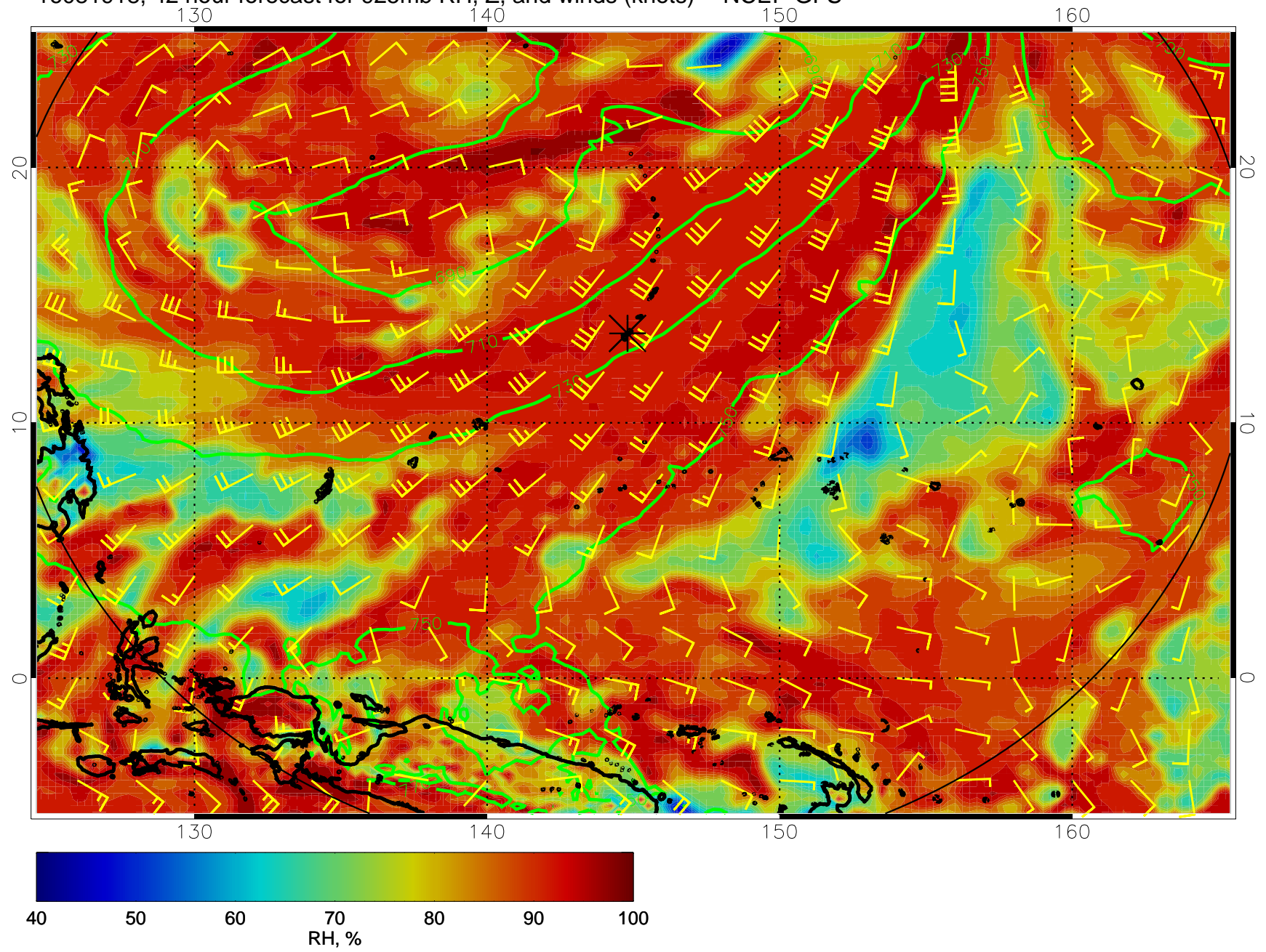
16081918, 42 hour forecast for 925mb RH, Z, and winds (knots) -- NCEP GFS
