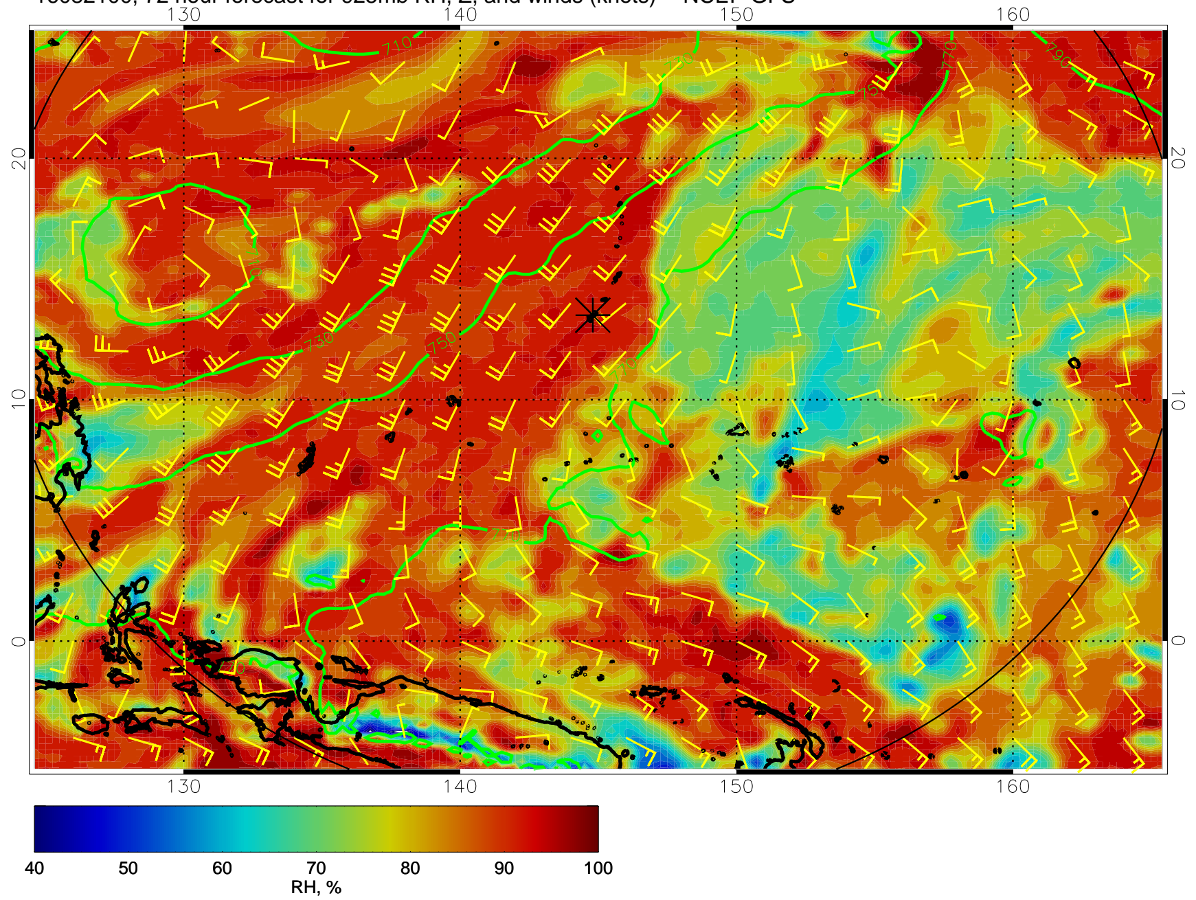
16082100, 72 hour forecast for 925mb RH, Z, and winds (knots) -- NCEP GFS
