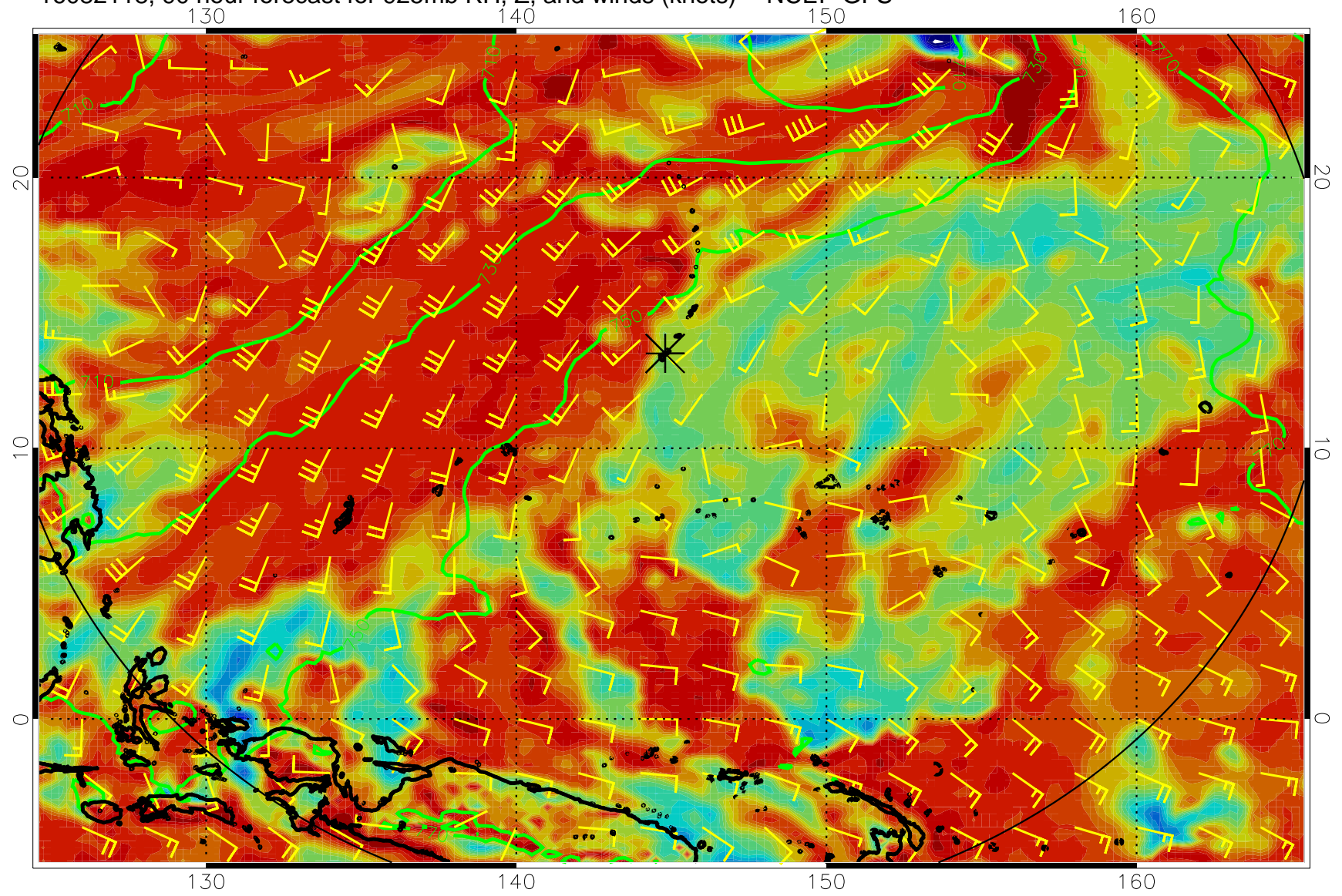
16082118, 90 hour forecast for 925mb RH, Z, and winds (knots) -- NCEP GFS
