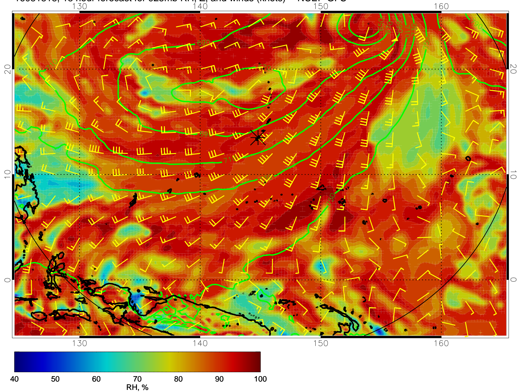
16081818, 18 hour forecast for 925mb RH, Z, and winds (knots) -- NCEP GFS
