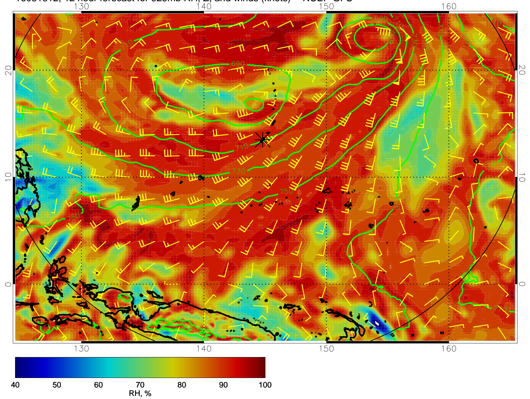
16081812, 12 hour forecast for 925mb RH, Z, and winds (knots) -- NCEP GFS
