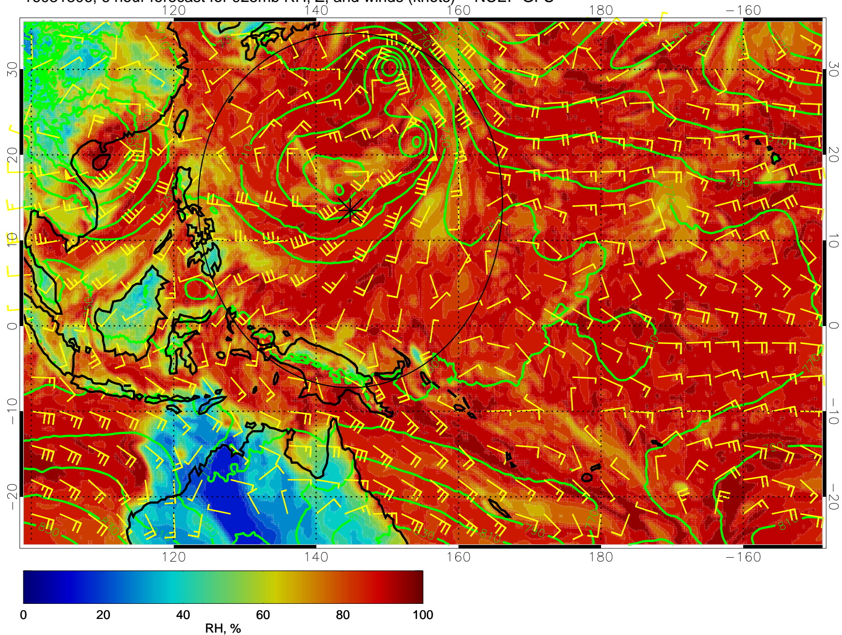
16081806, 6 hour forecast for 925mb RH, Z, and winds (knots) -- NCEP GFS
