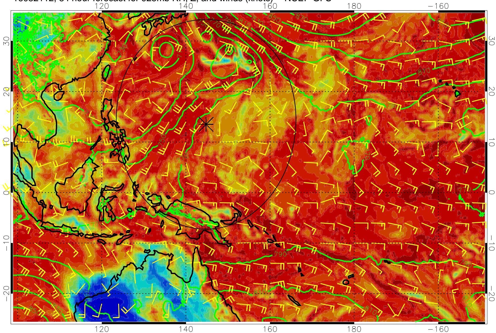
16082112, 84 hour forecast for 925mb RH, Z, and winds (knots) -- NCEP GFS
