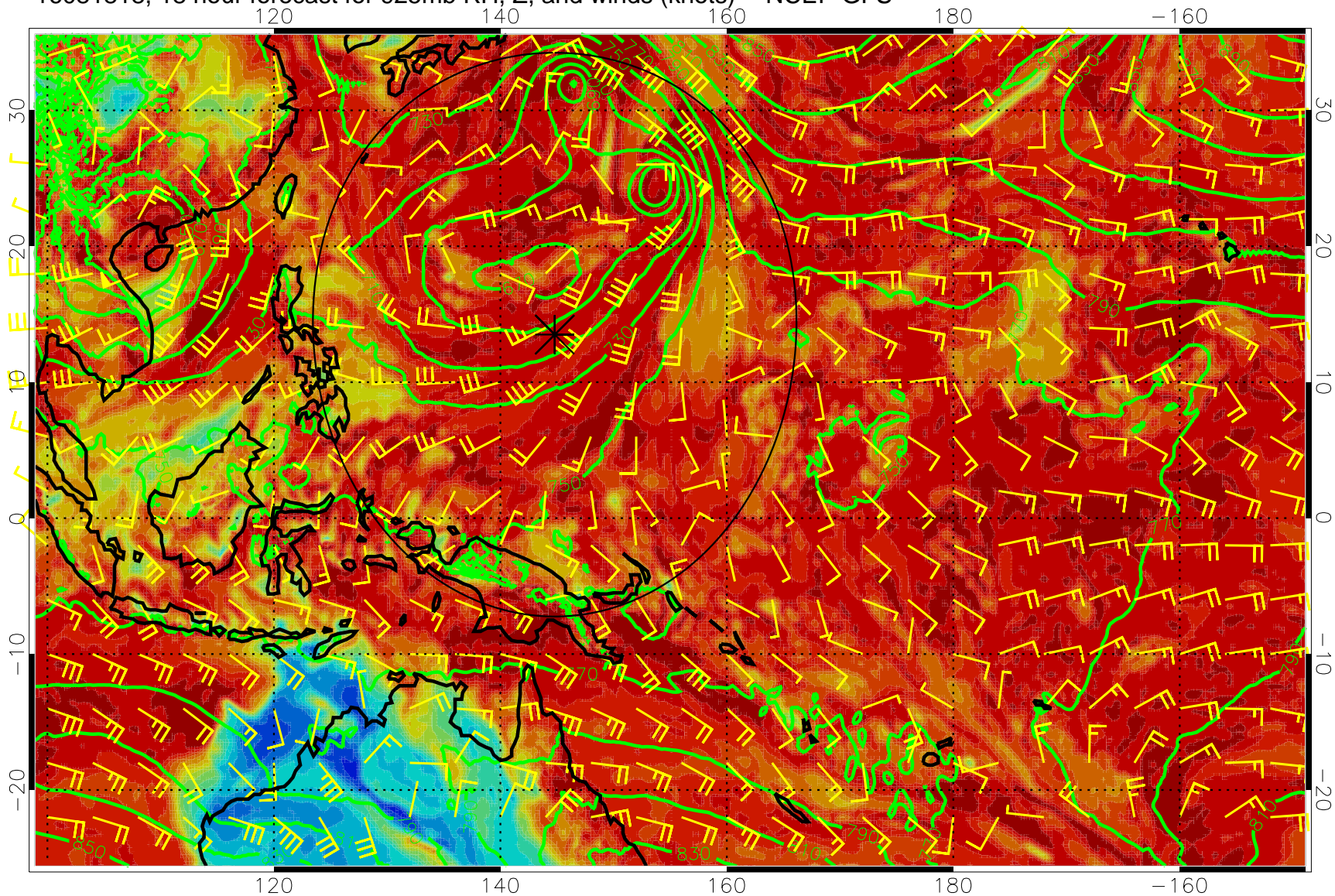
16081818, 18 hour forecast for 925mb RH, Z, and winds (knots) -- NCEP GFS
