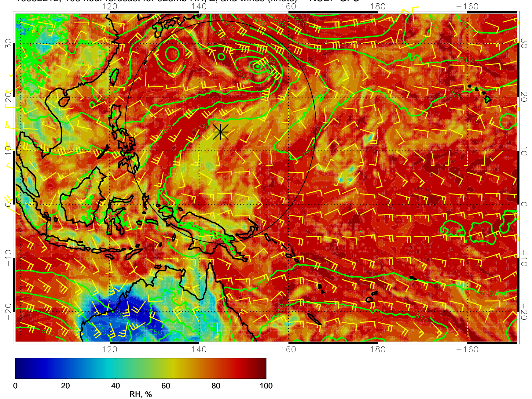
16082212, 108 hour forecast for 925mb RH, Z, and winds (knots) -- NCEP GFS
