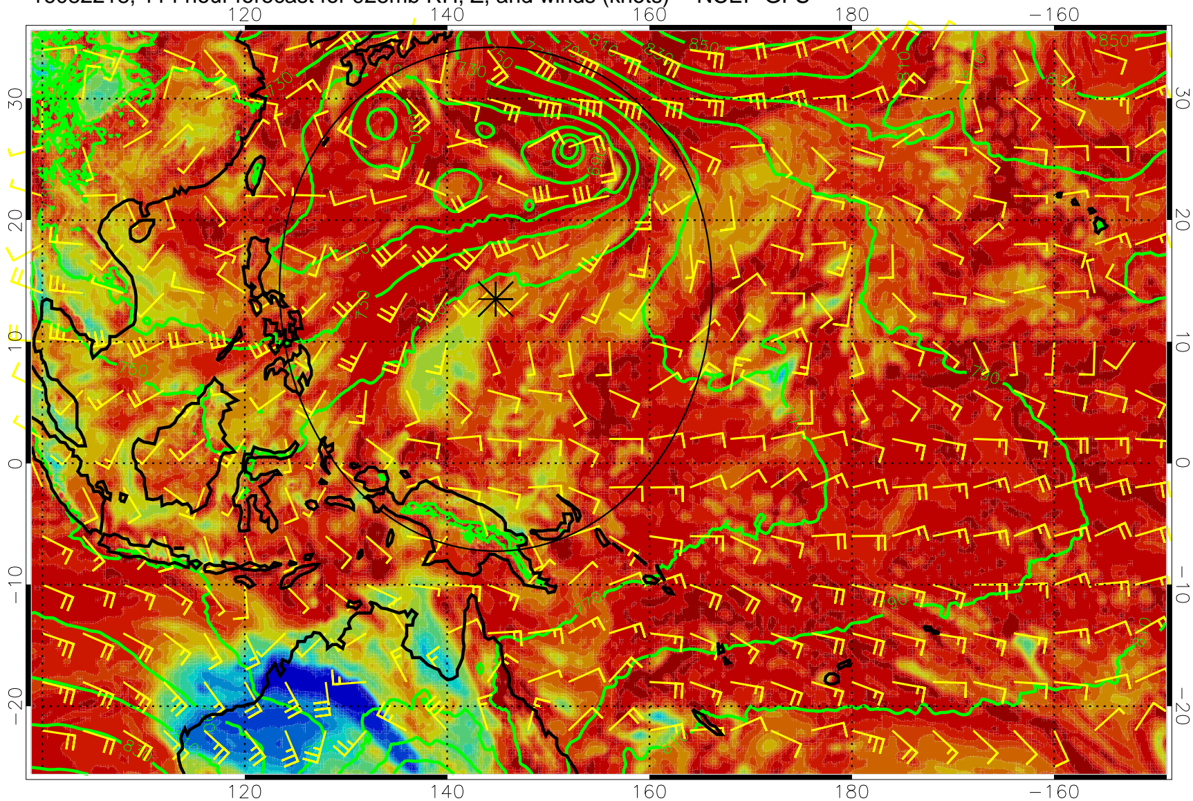
16082218, 114 hour forecast for 925mb RH, Z, and winds (knots) -- NCEP GFS
