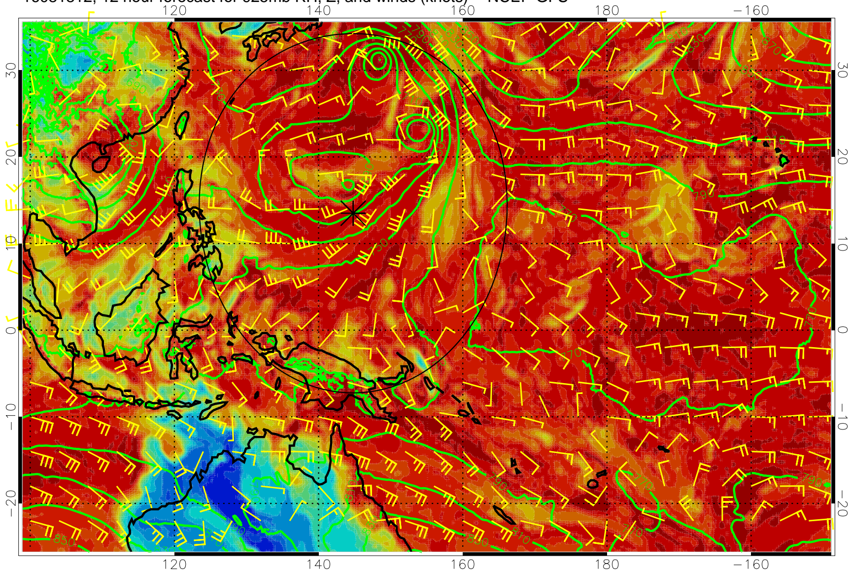
16081812, 12 hour forecast for 925mb RH, Z, and winds (knots) -- NCEP GFS
