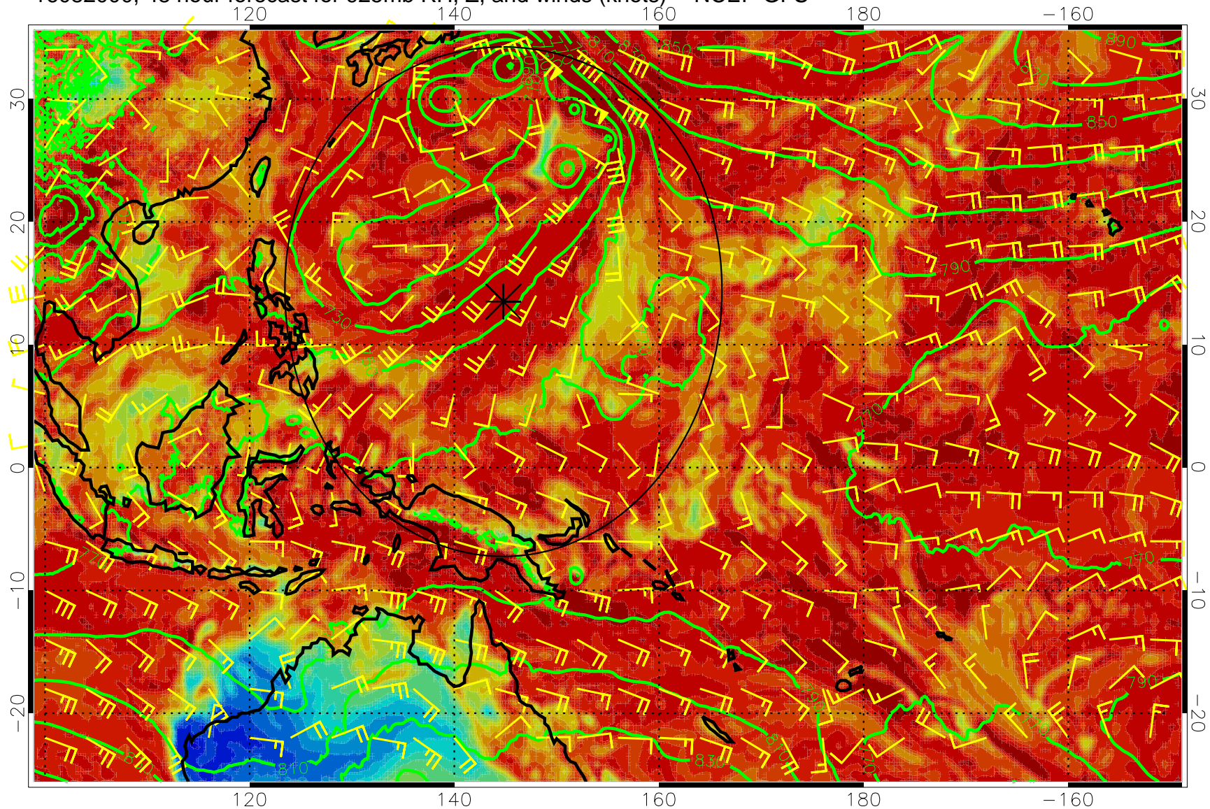
16082000, 48 hour forecast for 925mb RH, Z, and winds (knots) -- NCEP GFS
