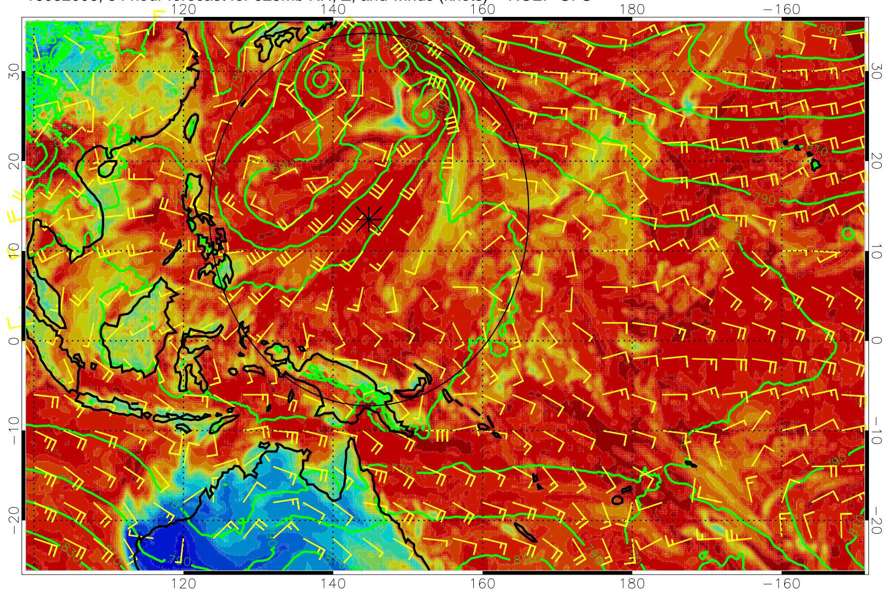
16082006, 54 hour forecast for 925mb RH, Z, and winds (knots) -- NCEP GFS
