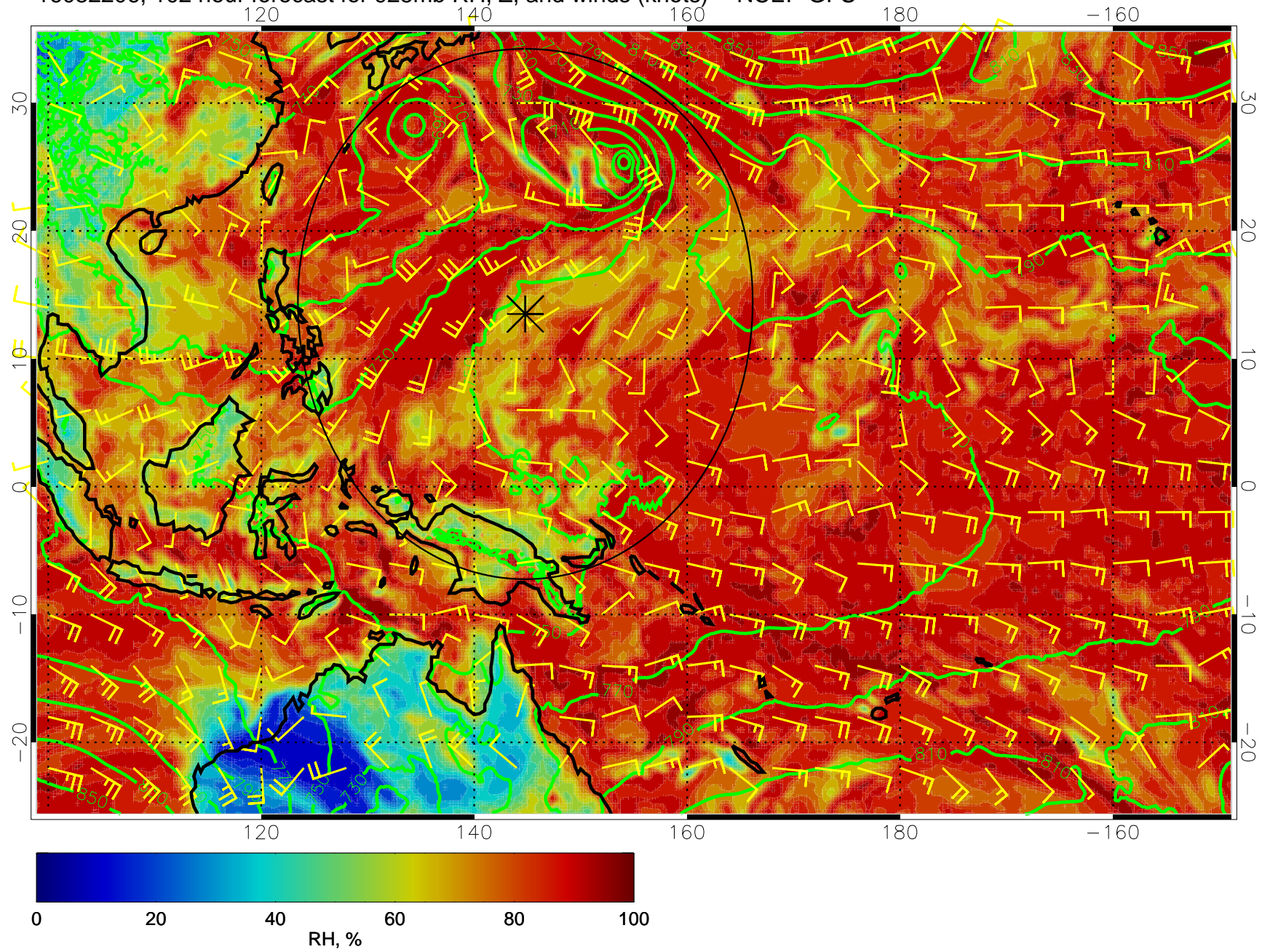
16082206, 102 hour forecast for 925mb RH, Z, and winds (knots) -- NCEP GFS
