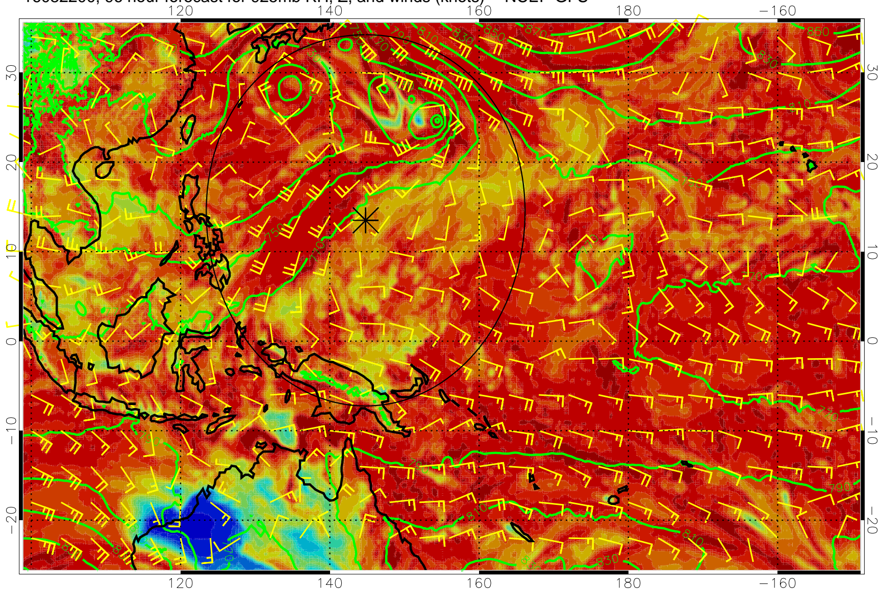
16082200, 96 hour forecast for 925mb RH, Z, and winds (knots) -- NCEP GFS
