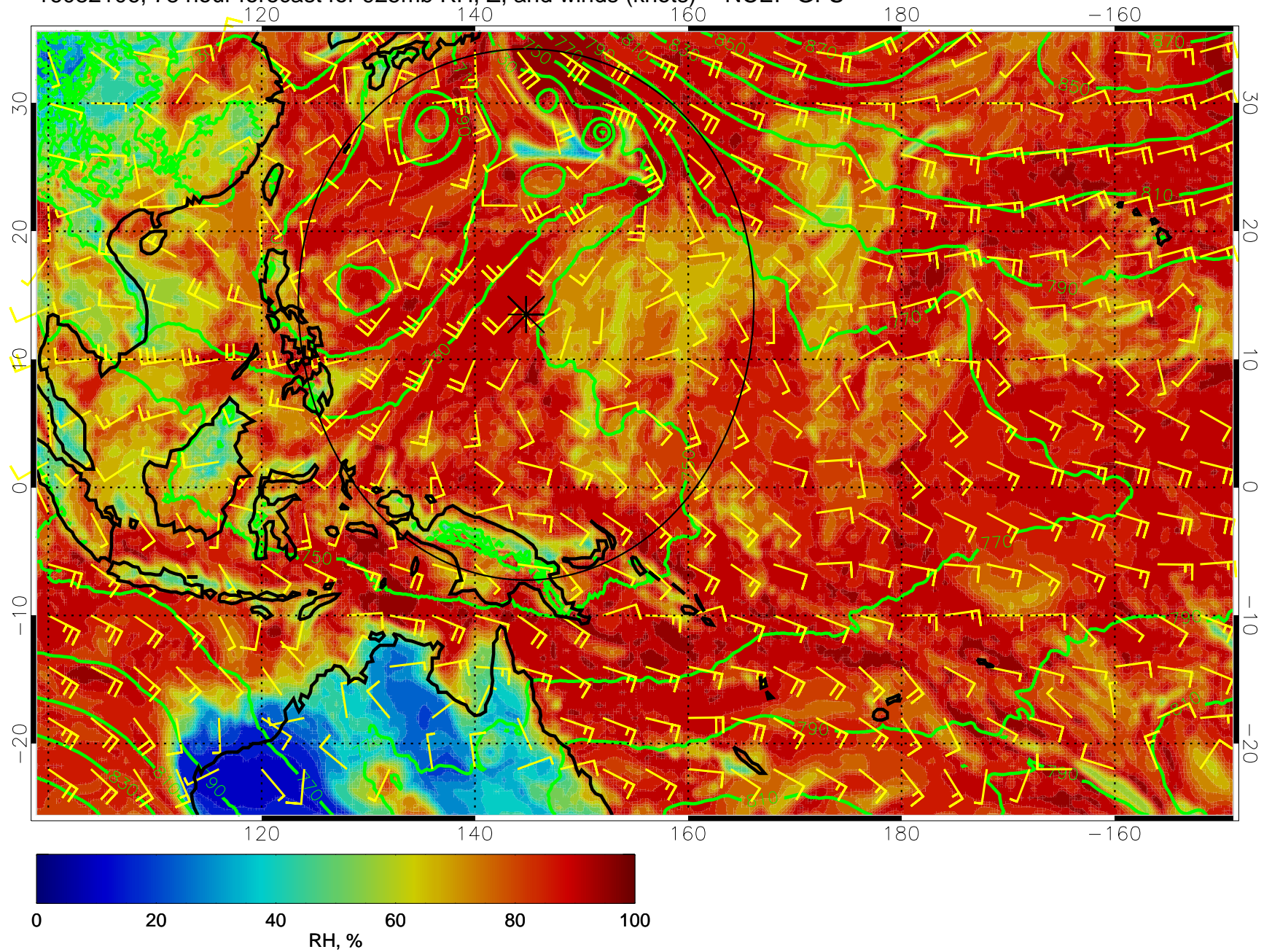
16082106, 78 hour forecast for 925mb RH, Z, and winds (knots) -- NCEP GFS
