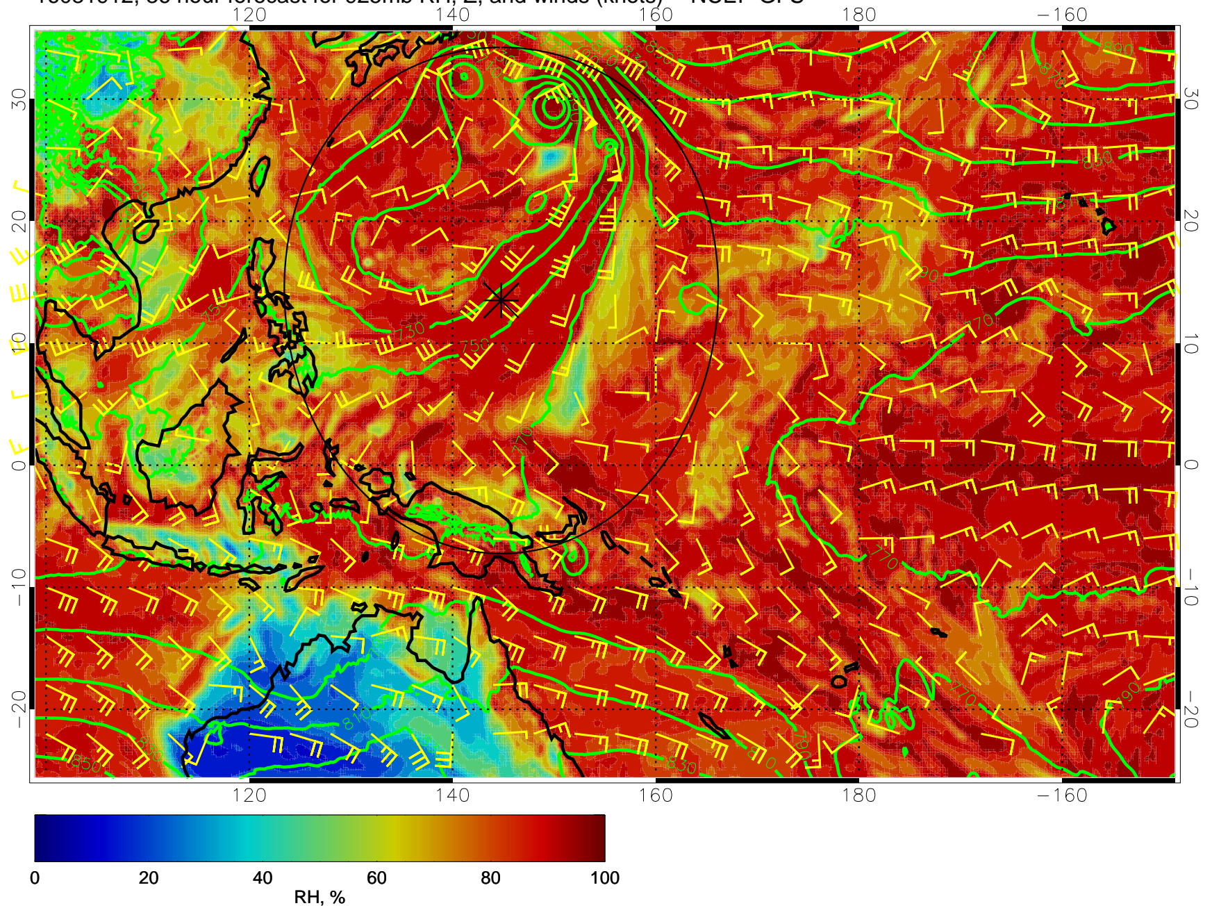
16081912, 36 hour forecast for 925mb RH, Z, and winds (knots) -- NCEP GFS
