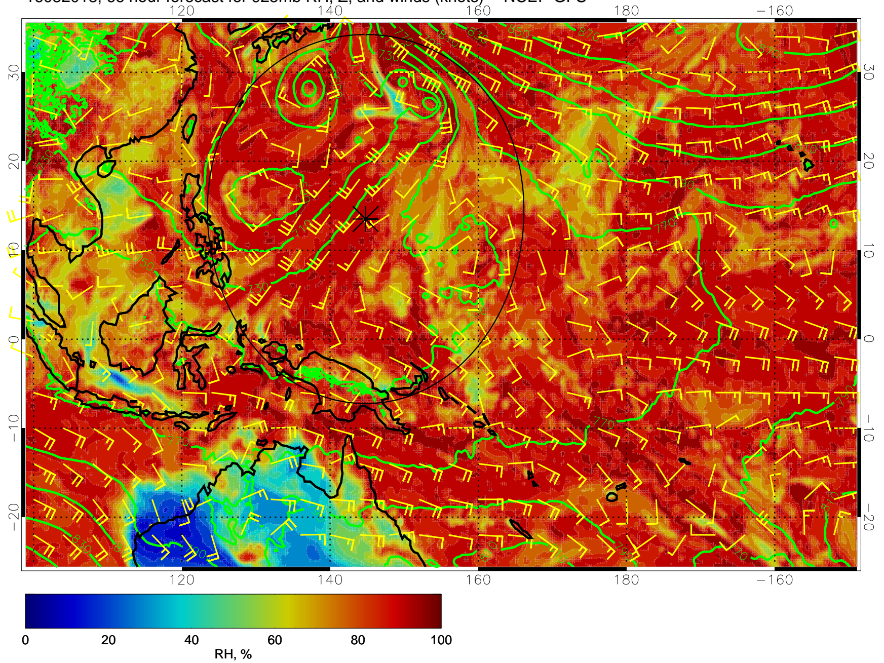
16082018, 66 hour forecast for 925mb RH, Z, and winds (knots) -- NCEP GFS
