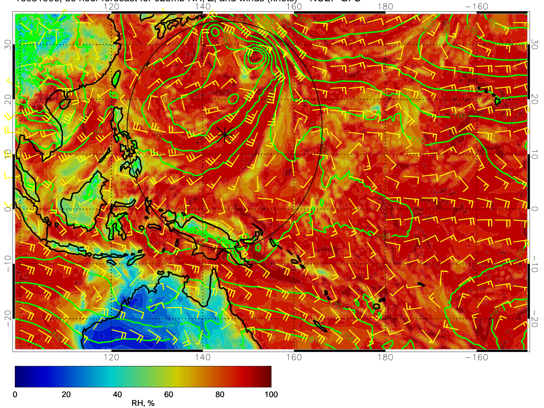
16081906, 30 hour forecast for 925mb RH, Z, and winds (knots) -- NCEP GFS
