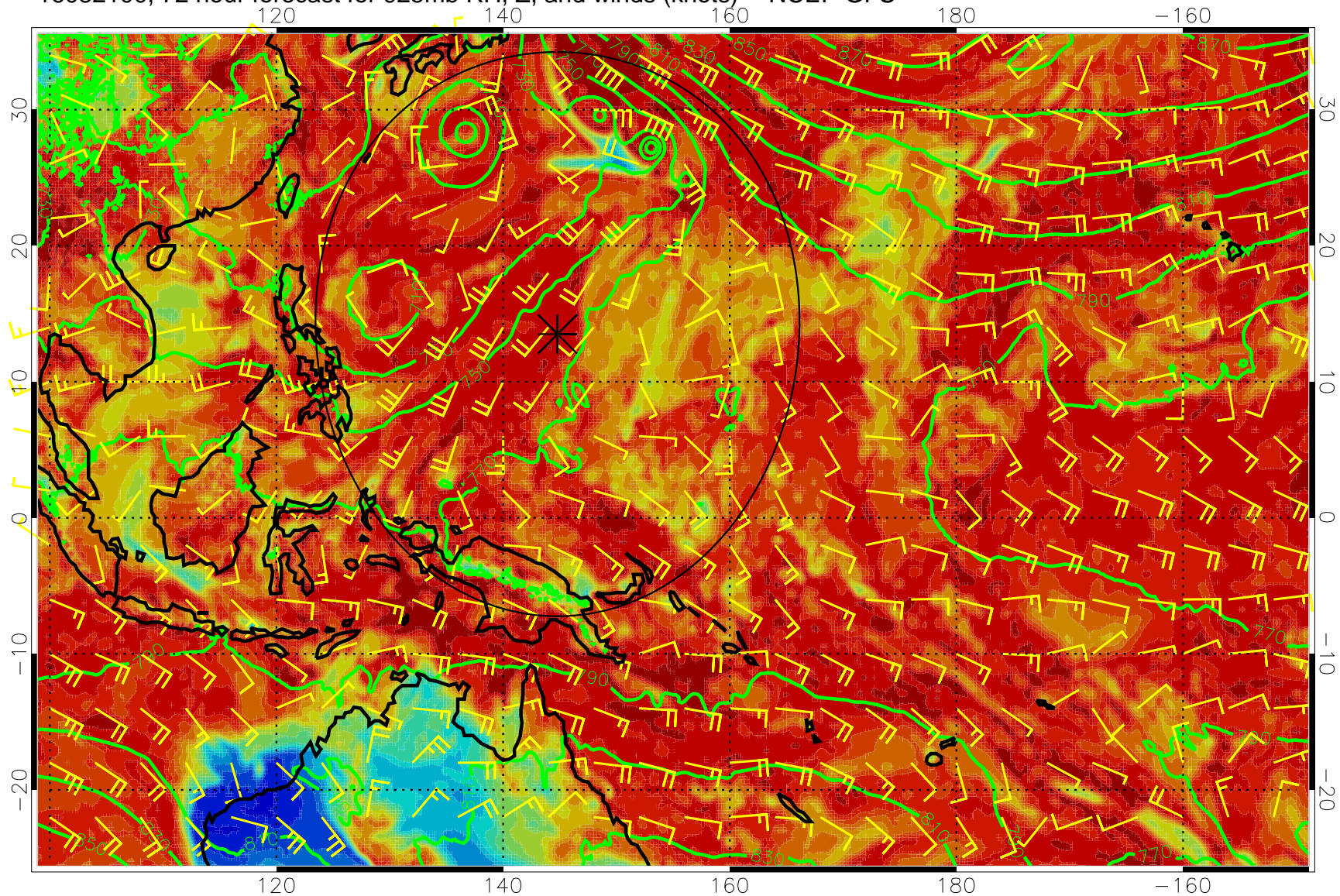
16082100, 72 hour forecast for 925mb RH, Z, and winds (knots) -- NCEP GFS
