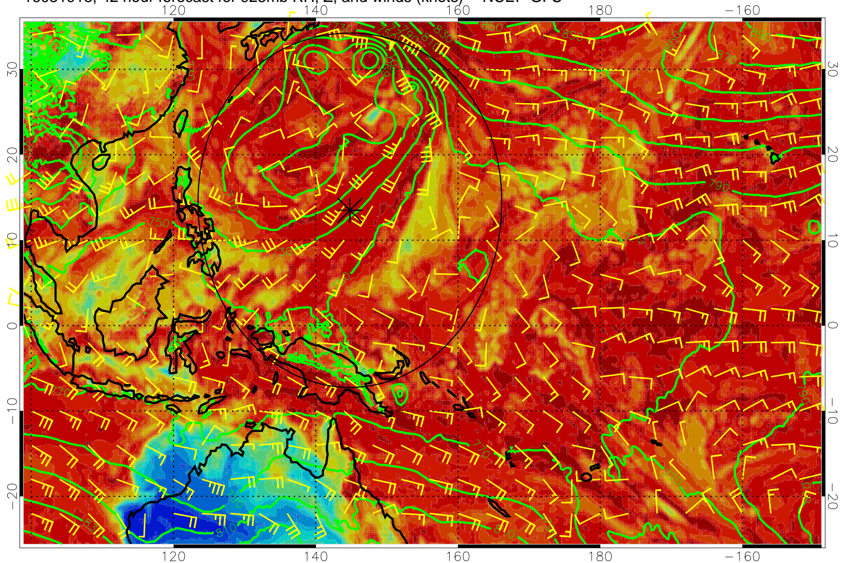
16081918, 42 hour forecast for 925mb RH, Z, and winds (knots) -- NCEP GFS
