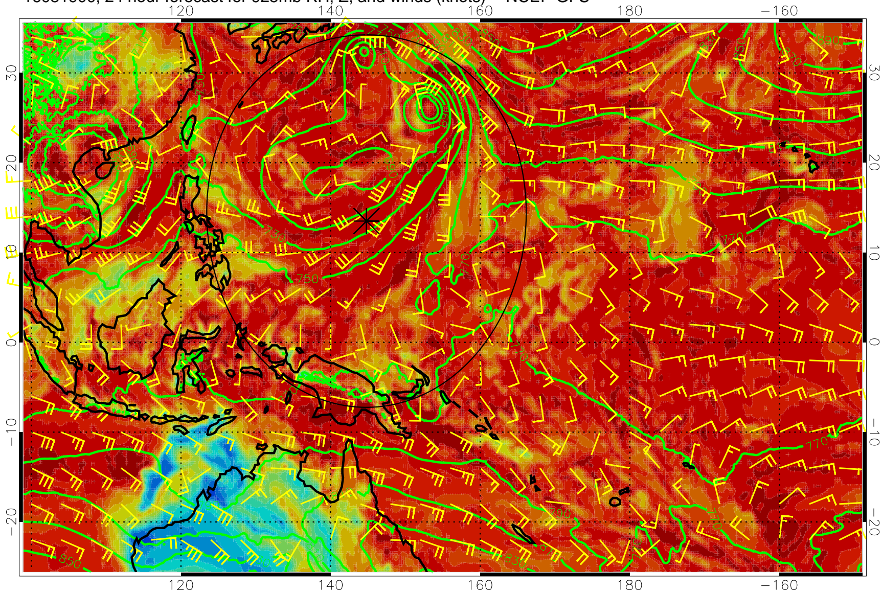
16081900, 24 hour forecast for 925mb RH, Z, and winds (knots) -- NCEP GFS
