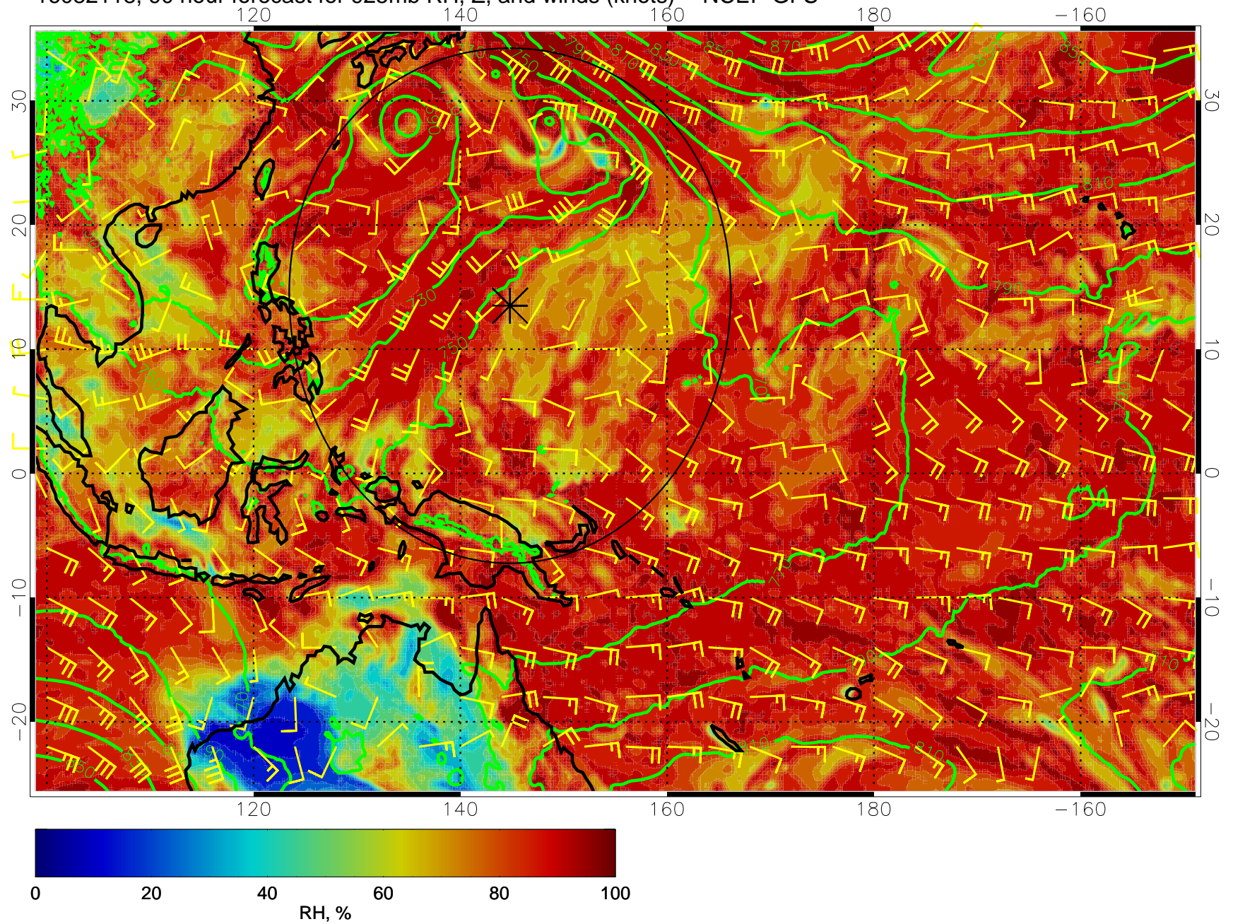
16082118, 90 hour forecast for 925mb RH, Z, and winds (knots) -- NCEP GFS
