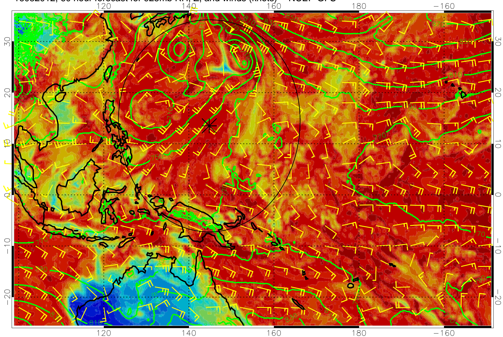
16082012, 60 hour forecast for 925mb RH, Z, and winds (knots) -- NCEP GFS
