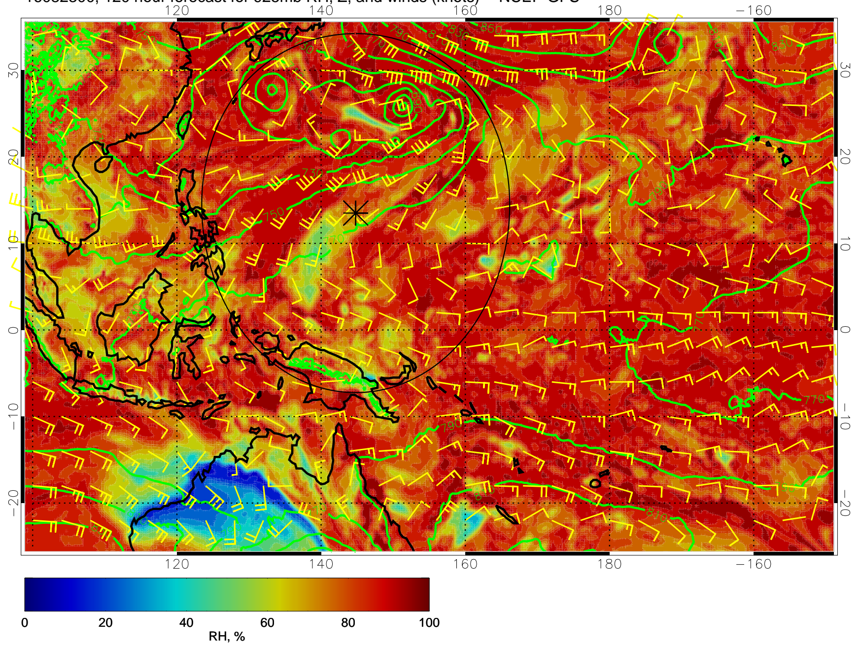
16082300, 120 hour forecast for 925mb RH, Z, and winds (knots) -- NCEP GFS
