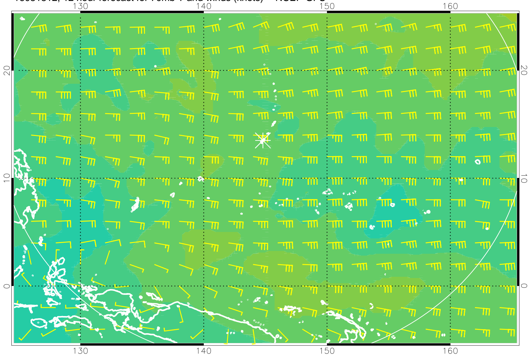
16081812, 12 hour forecast for 70mb T and winds (knots) -- NCEP GFS
