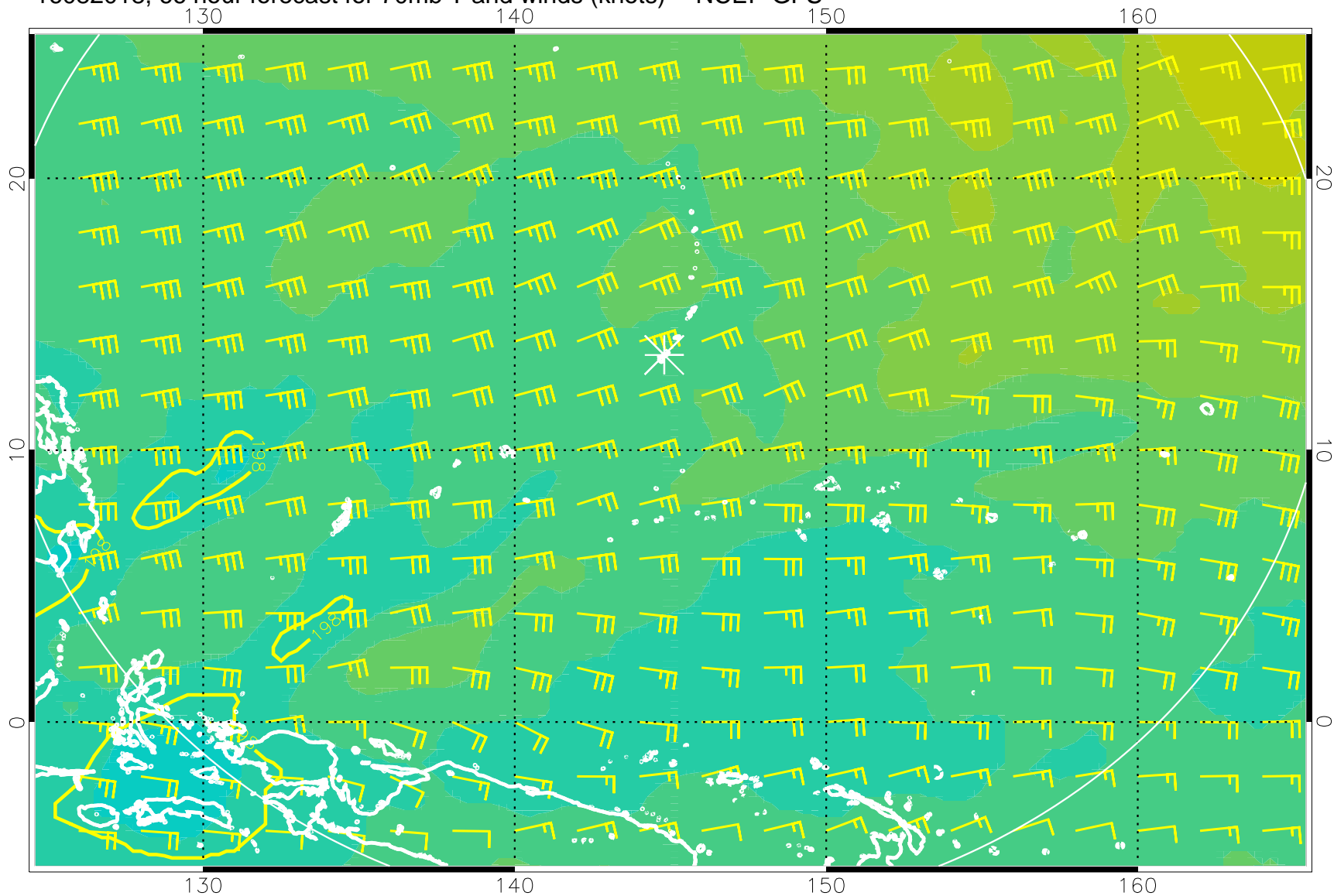
16082018, 66 hour forecast for 70mb T and winds (knots) -- NCEP GFS
