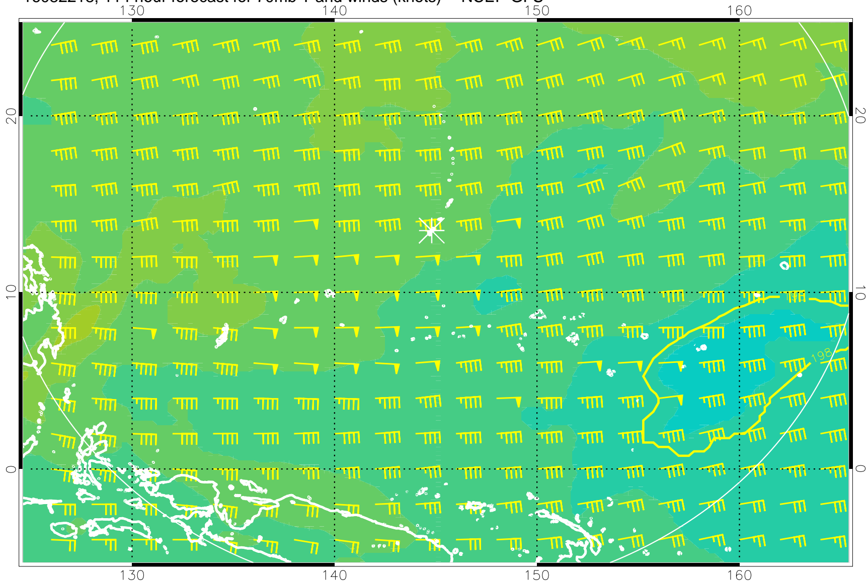
16082218, 114 hour forecast for 70mb T and winds (knots) -- NCEP GFS
