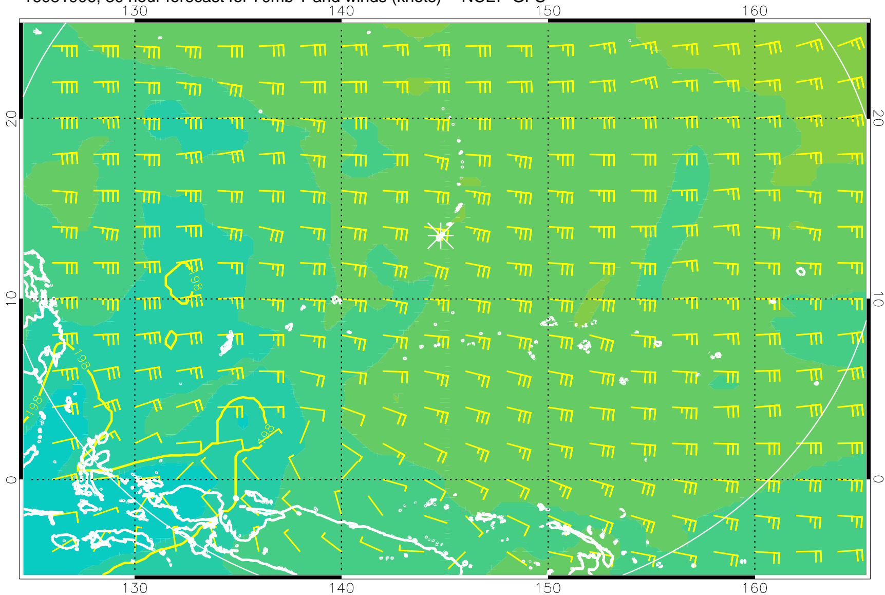
16081906, 30 hour forecast for 70mb T and winds (knots) -- NCEP GFS
