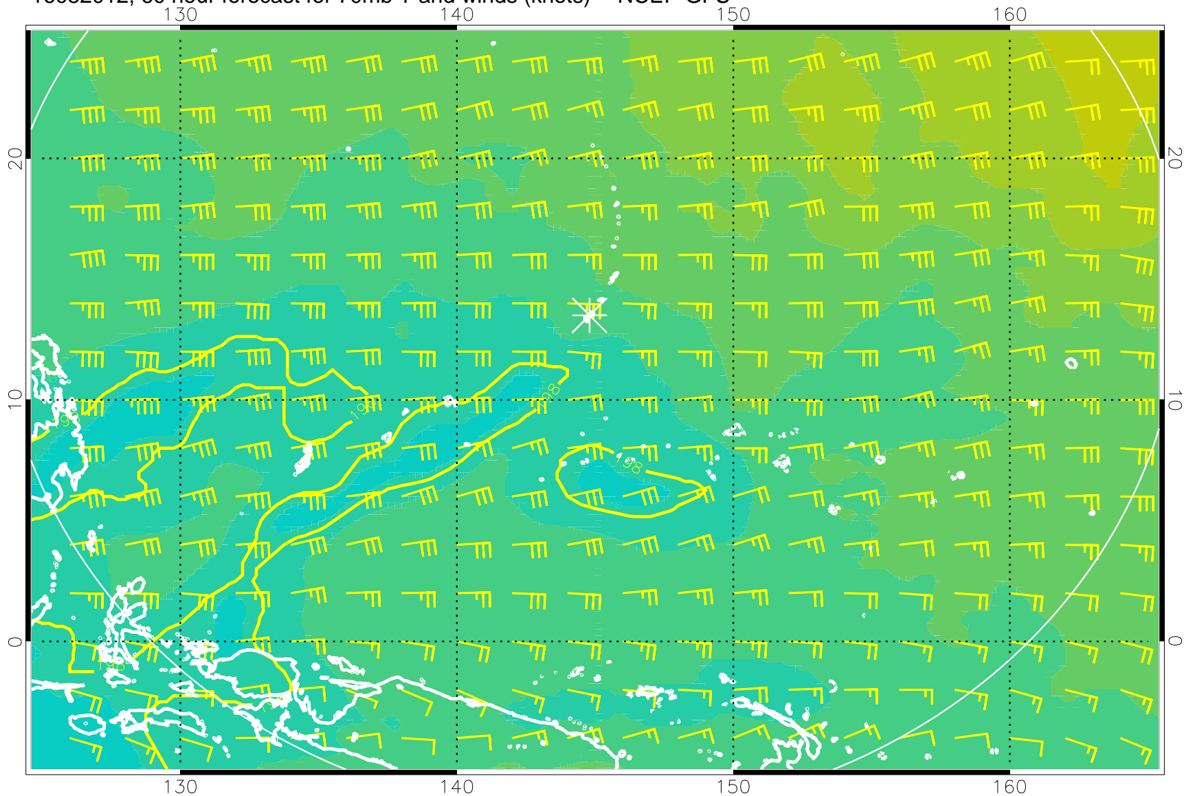
16082012, 60 hour forecast for 70mb T and winds (knots) -- NCEP GFS
