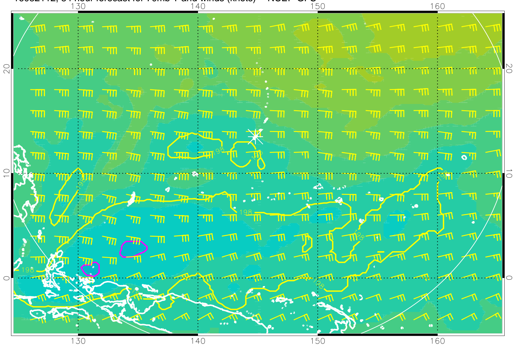
16082112, 84 hour forecast for 70mb T and winds (knots) -- NCEP GFS
