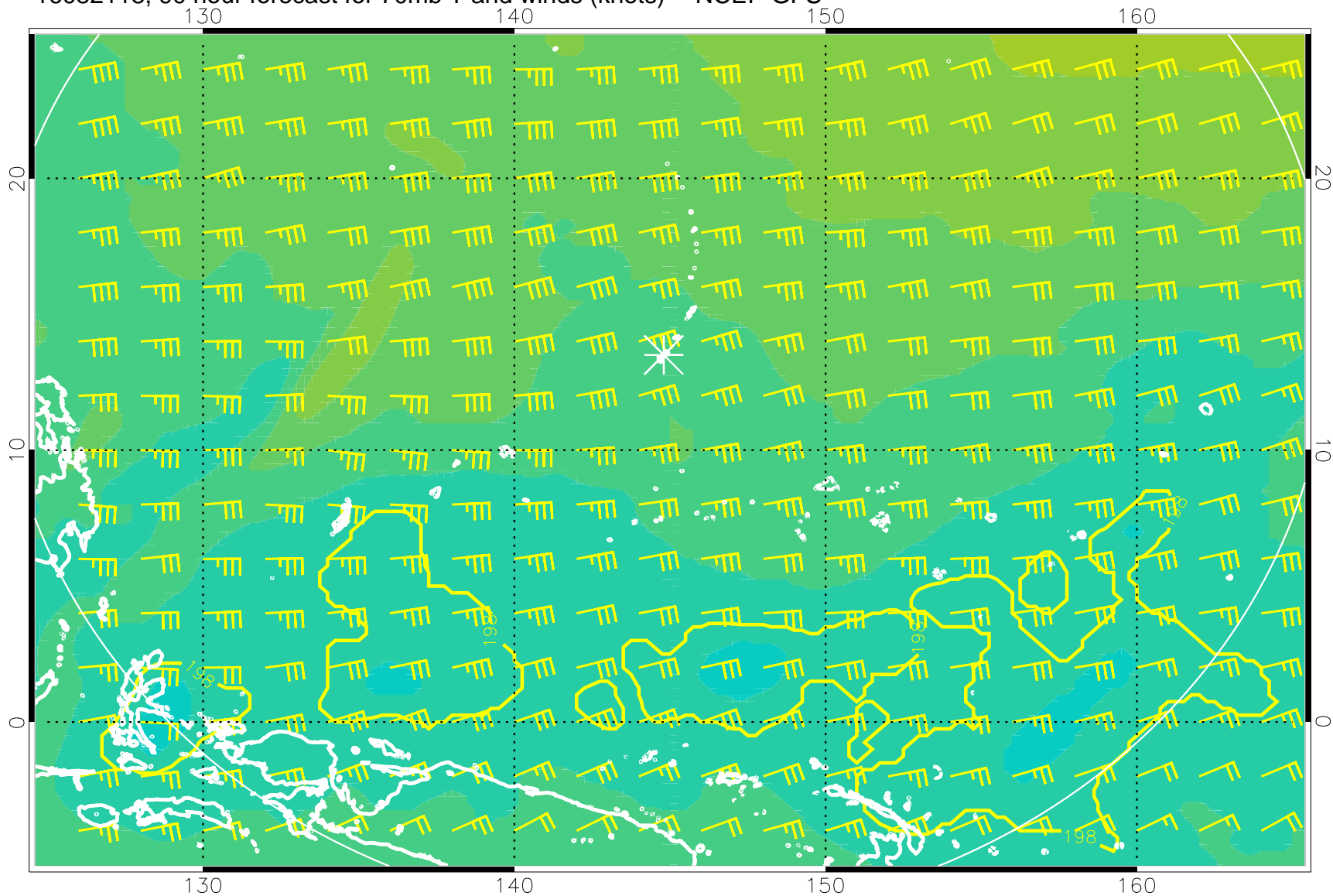
16082118, 90 hour forecast for 70mb T and winds (knots) -- NCEP GFS
