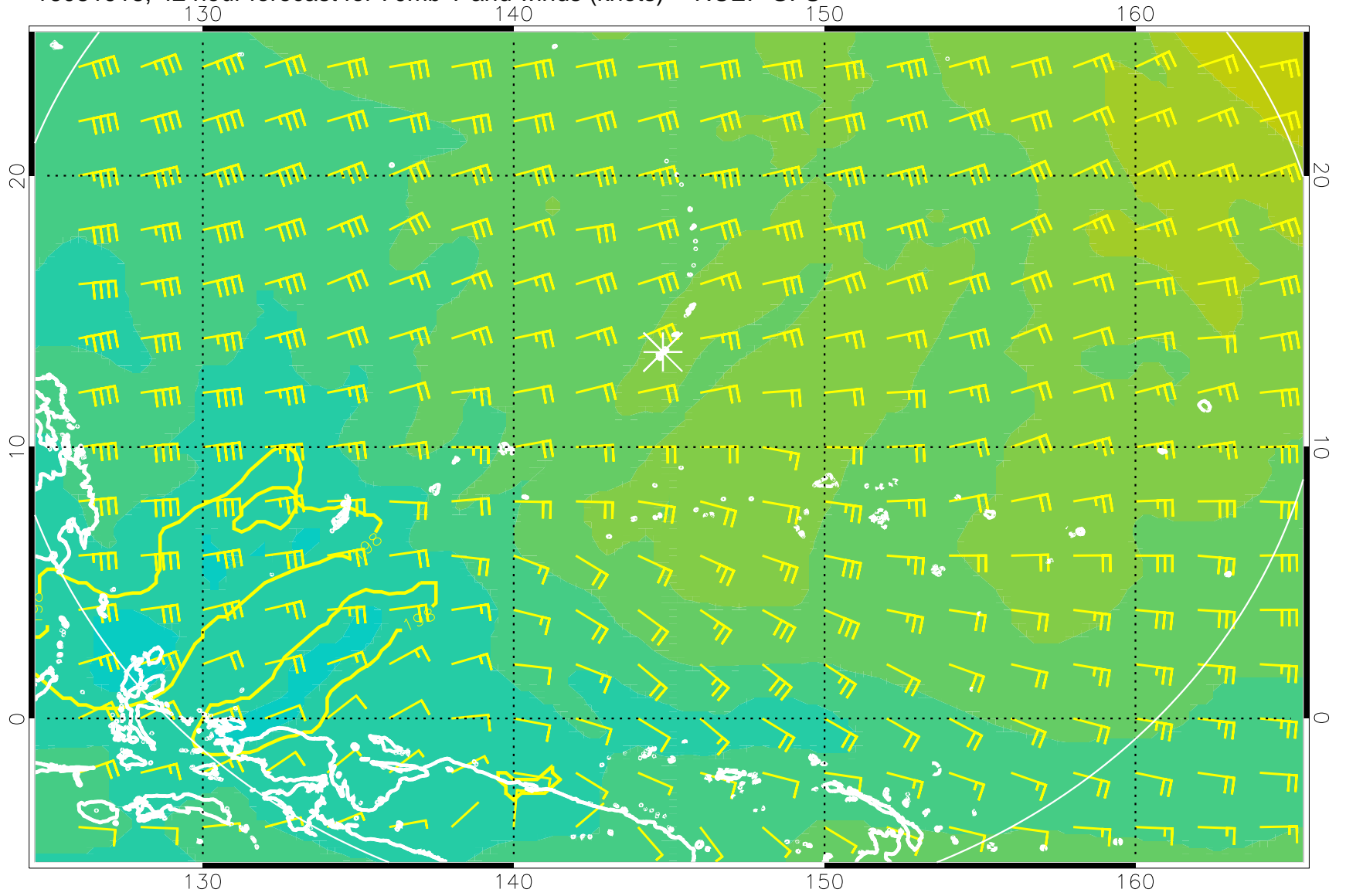
16081918, 42 hour forecast for 70mb T and winds (knots) -- NCEP GFS
