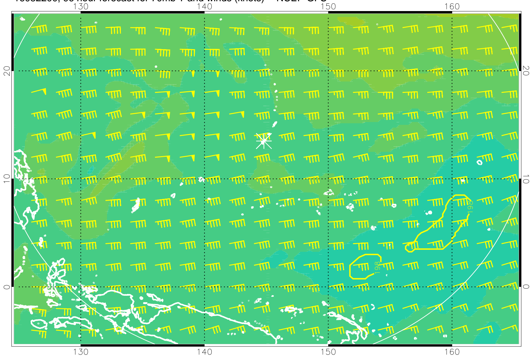
16082200, 96 hour forecast for 70mb T and winds (knots) -- NCEP GFS
