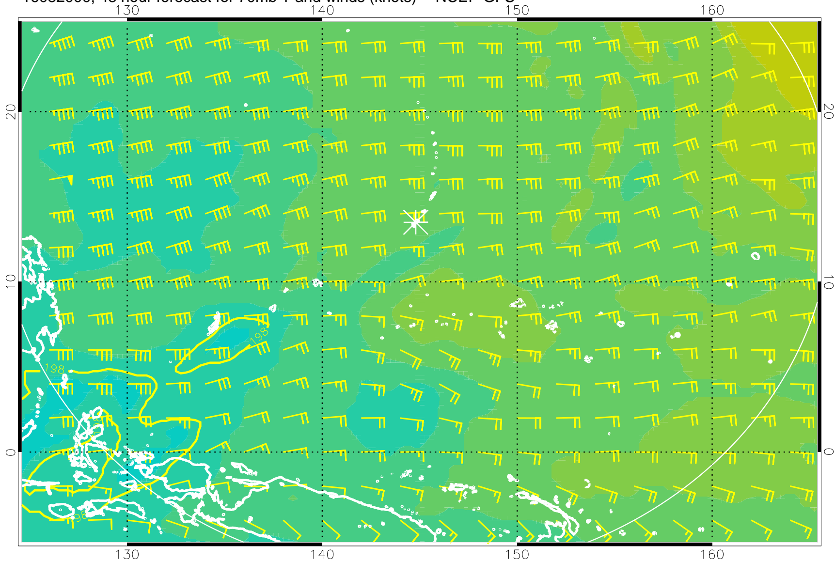
16082000, 48 hour forecast for 70mb T and winds (knots) -- NCEP GFS
