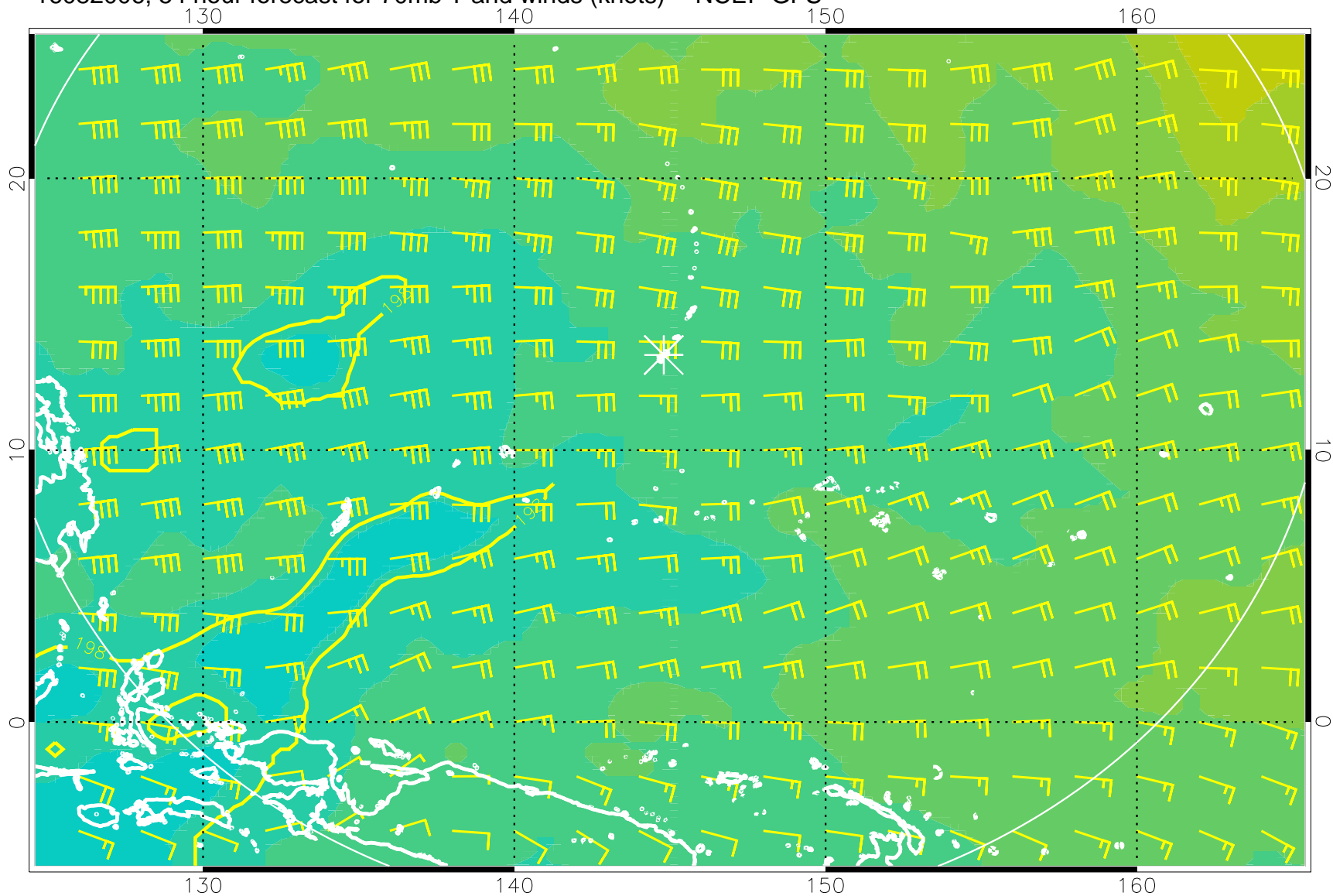
16082006, 54 hour forecast for 70mb T and winds (knots) -- NCEP GFS
