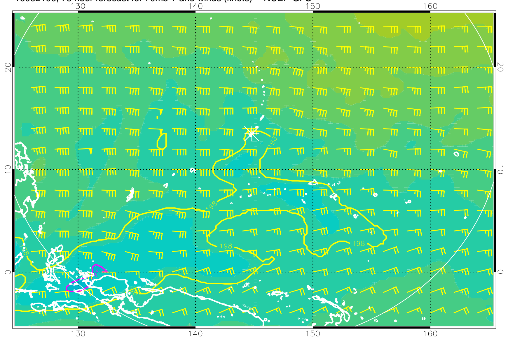
16082106, 78 hour forecast for 70mb T and winds (knots) -- NCEP GFS
