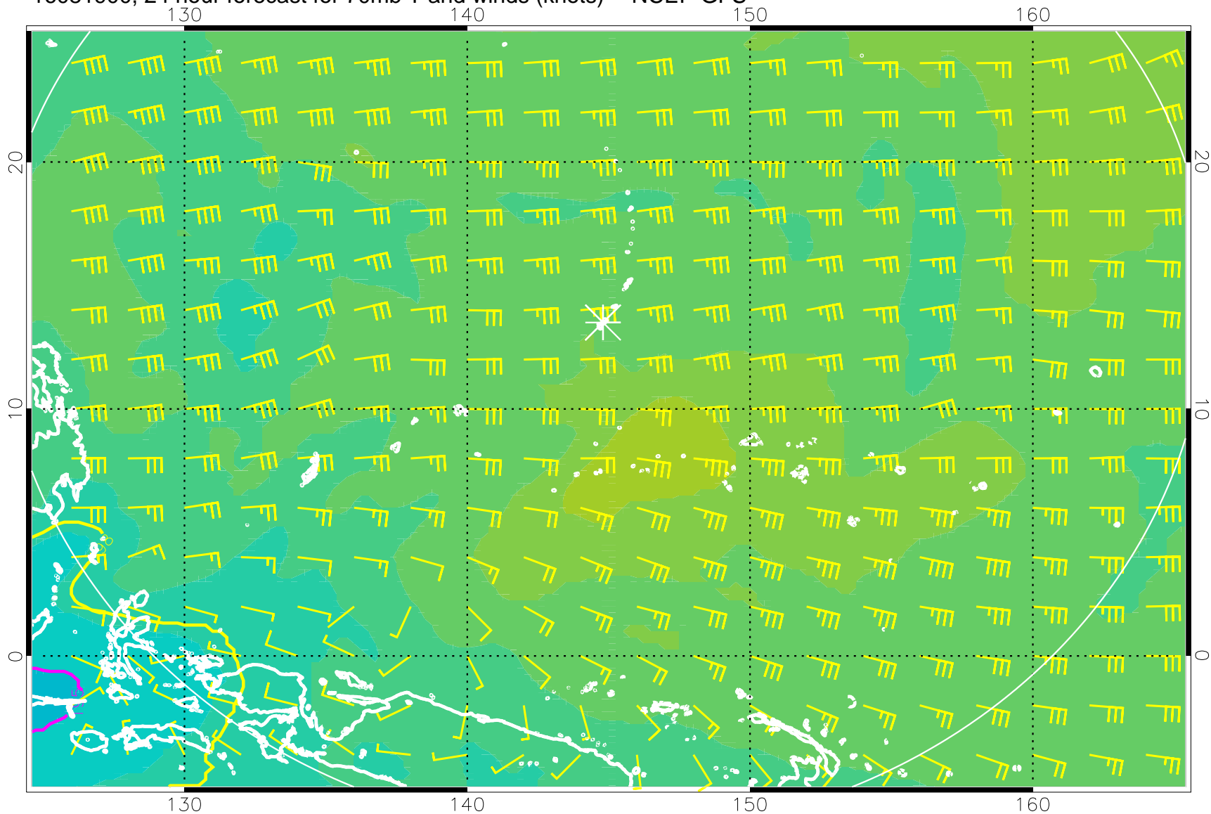
16081900, 24 hour forecast for 70mb T and winds (knots) -- NCEP GFS
