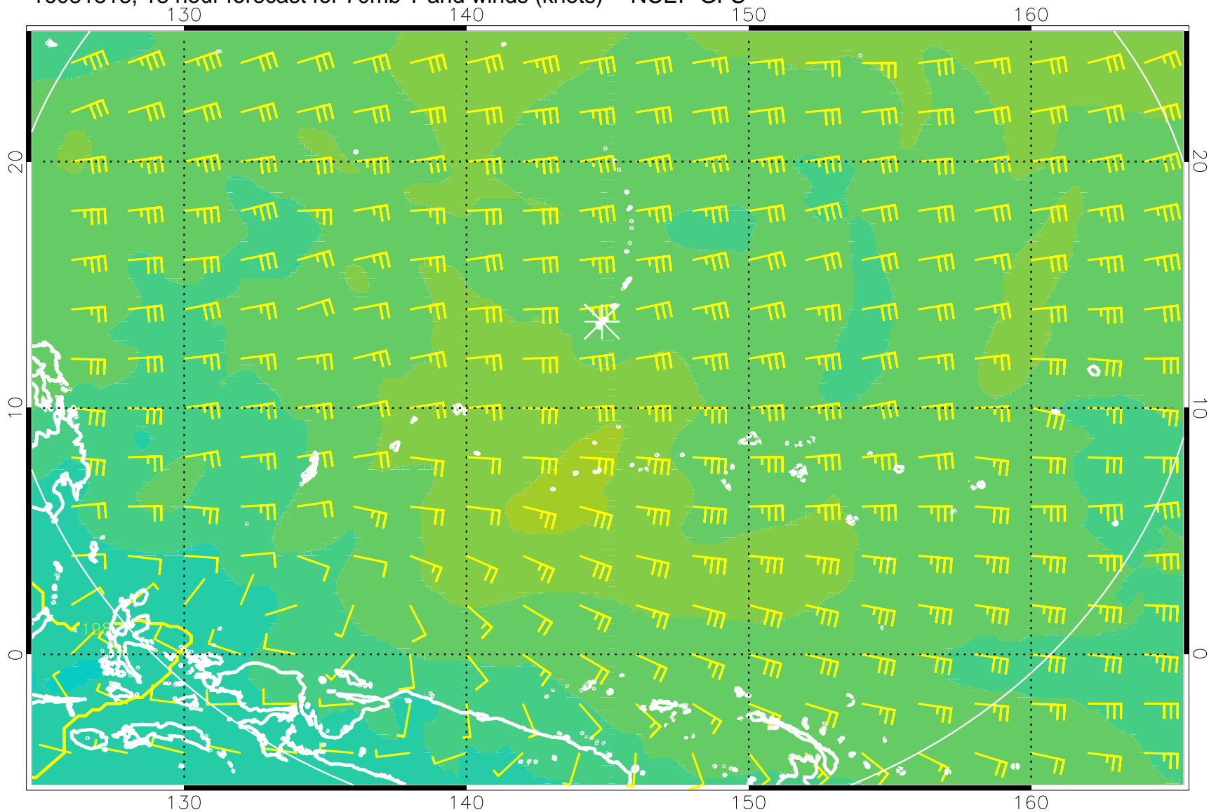
16081818, 18 hour forecast for 70mb T and winds (knots) -- NCEP GFS
