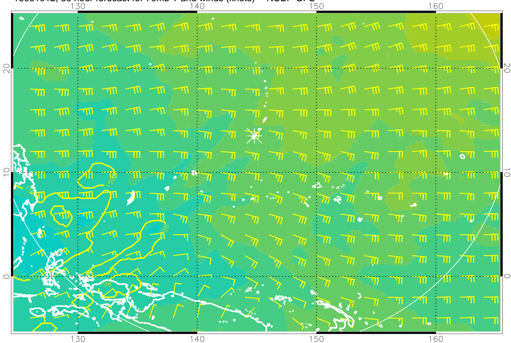
16081912, 36 hour forecast for 70mb T and winds (knots) -- NCEP GFS
