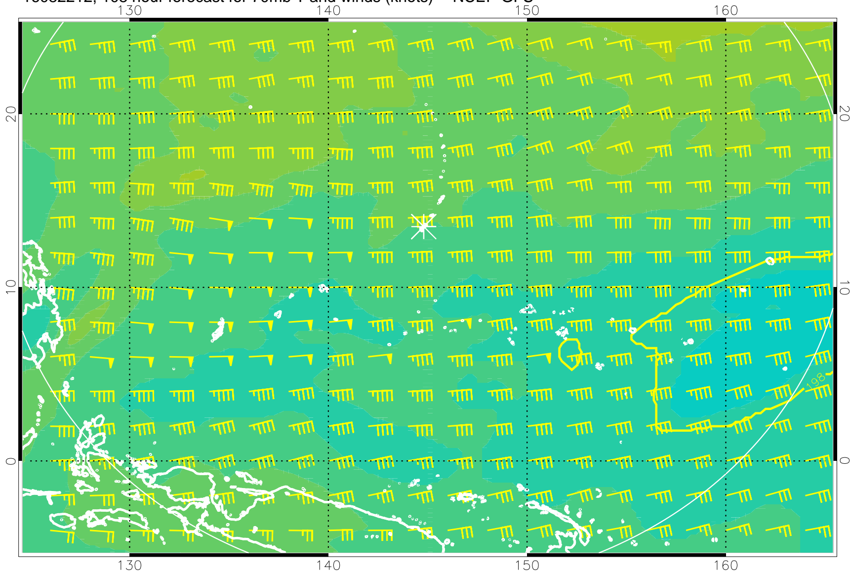
16082212, 108 hour forecast for 70mb T and winds (knots) -- NCEP GFS
