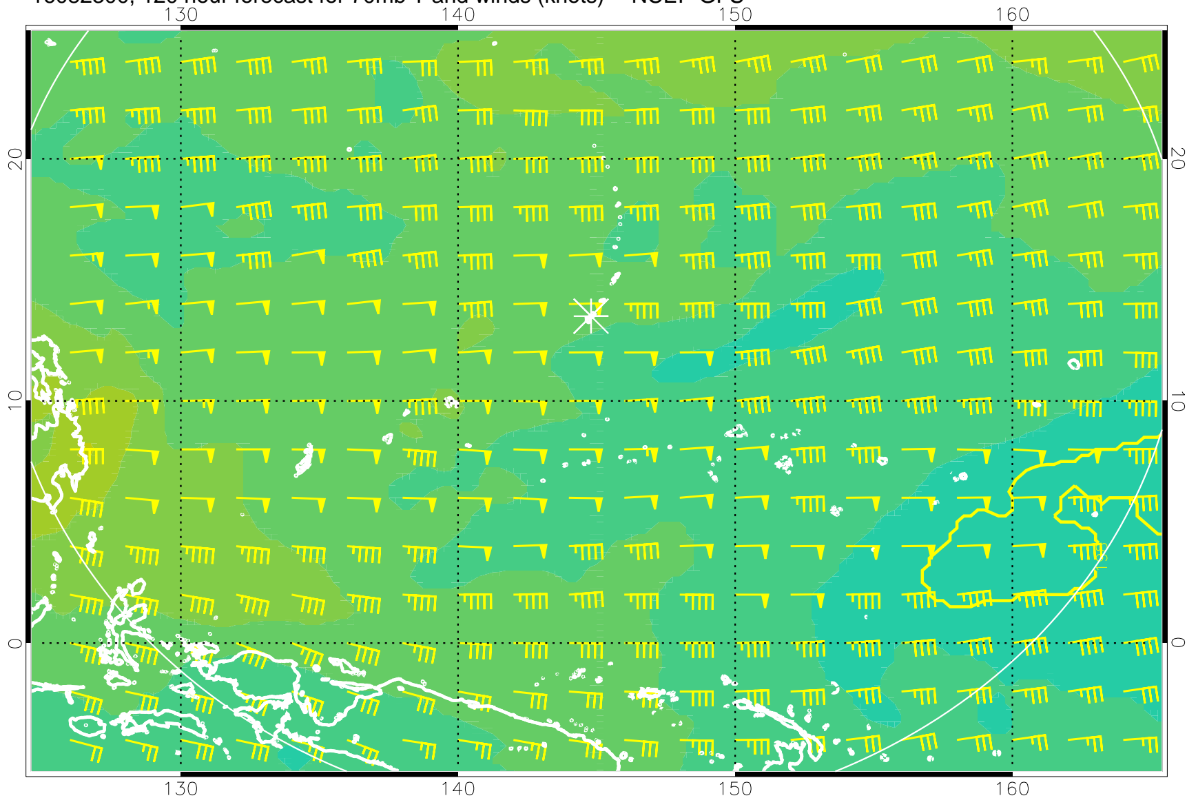
16082300, 120 hour forecast for 70mb T and winds (knots) -- NCEP GFS
