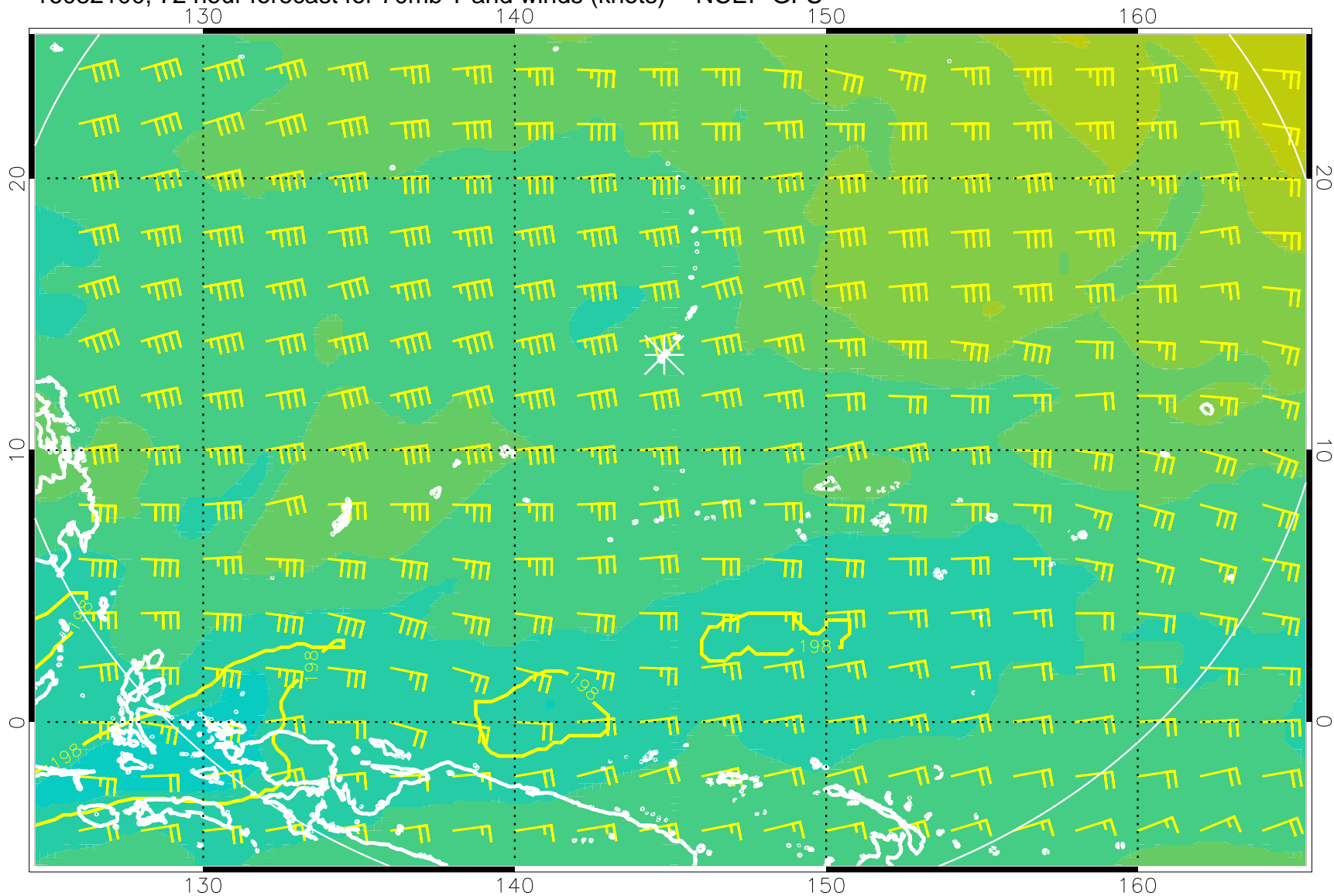
16082100, 72 hour forecast for 70mb T and winds (knots) -- NCEP GFS
