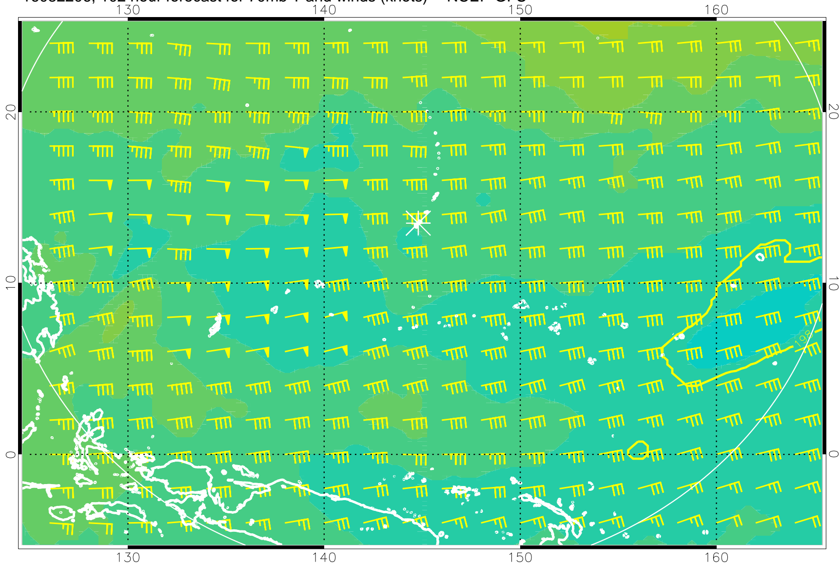
16082206, 102 hour forecast for 70mb T and winds (knots) -- NCEP GFS
