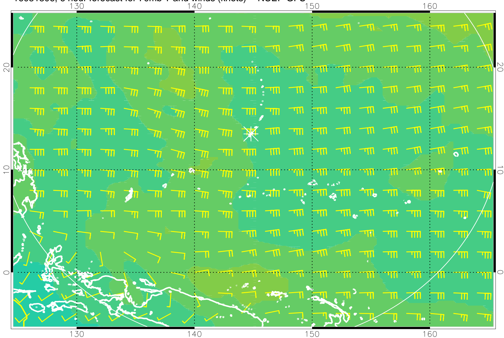
16081806, 6 hour forecast for 70mb T and winds (knots) -- NCEP GFS
