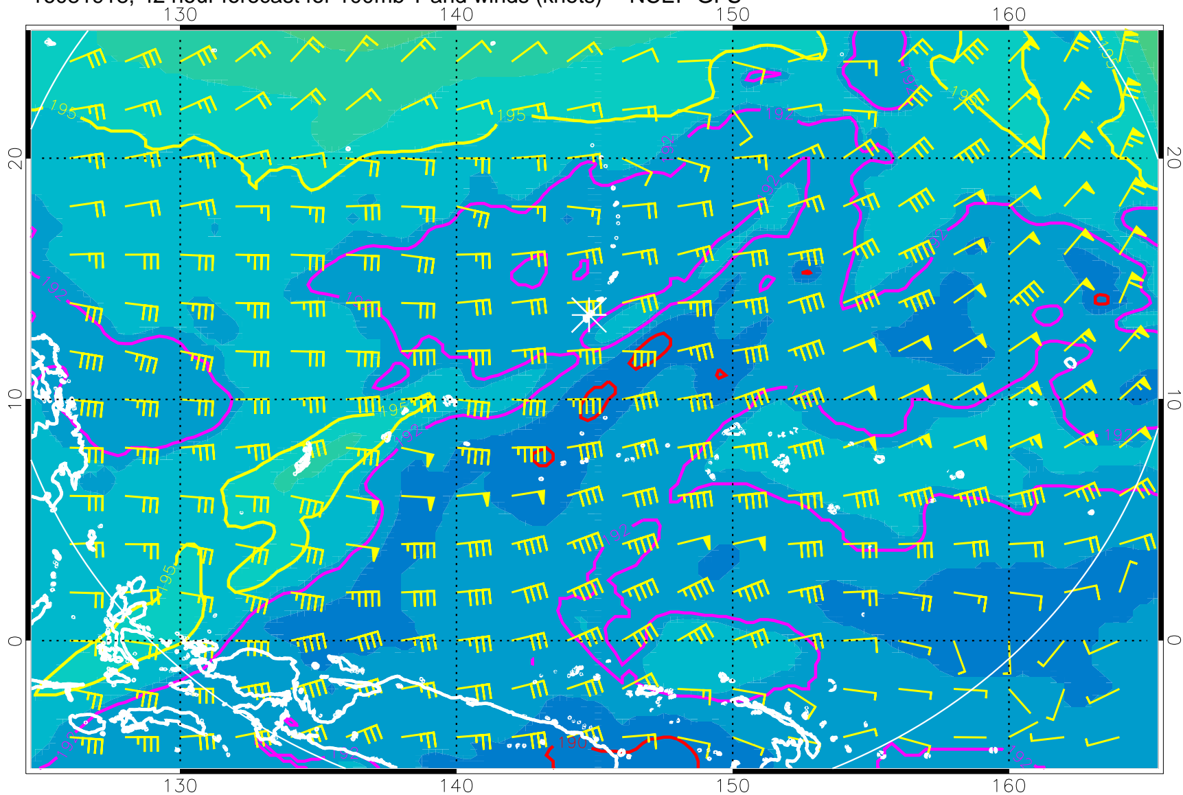
16081918, 42 hour forecast for 100mb T and winds (knots) -- NCEP GFS
