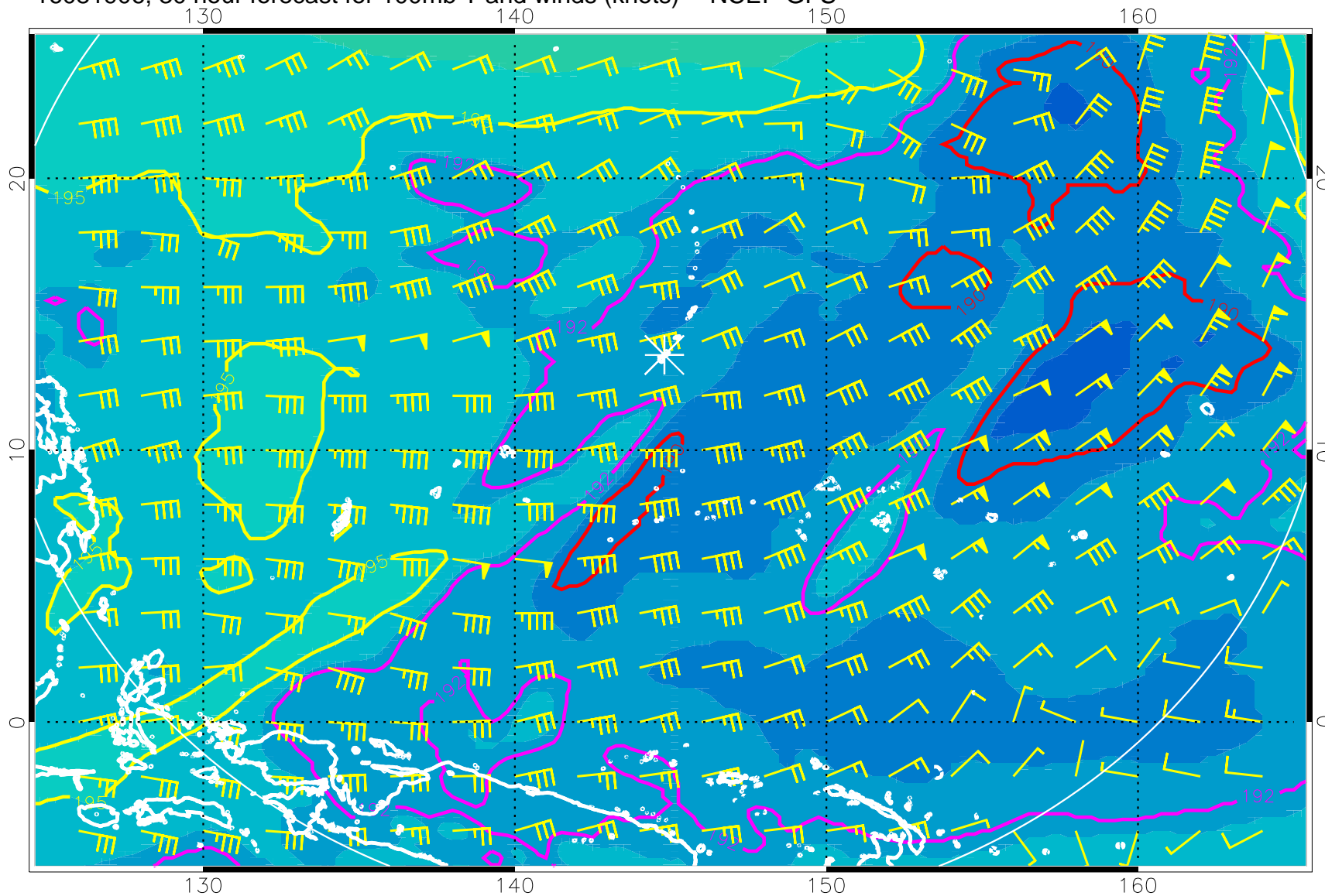
16081906, 30 hour forecast for 100mb T and winds (knots) -- NCEP GFS
