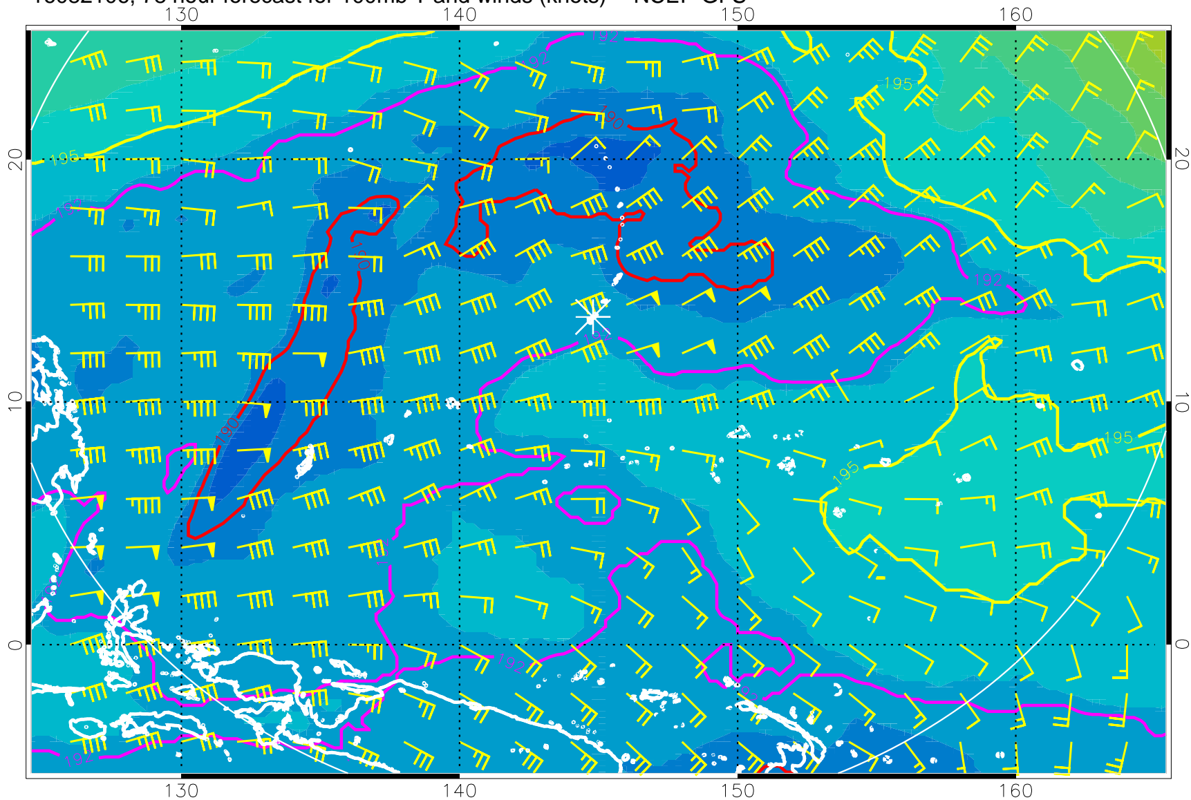
16082106, 78 hour forecast for 100mb T and winds (knots) -- NCEP GFS
