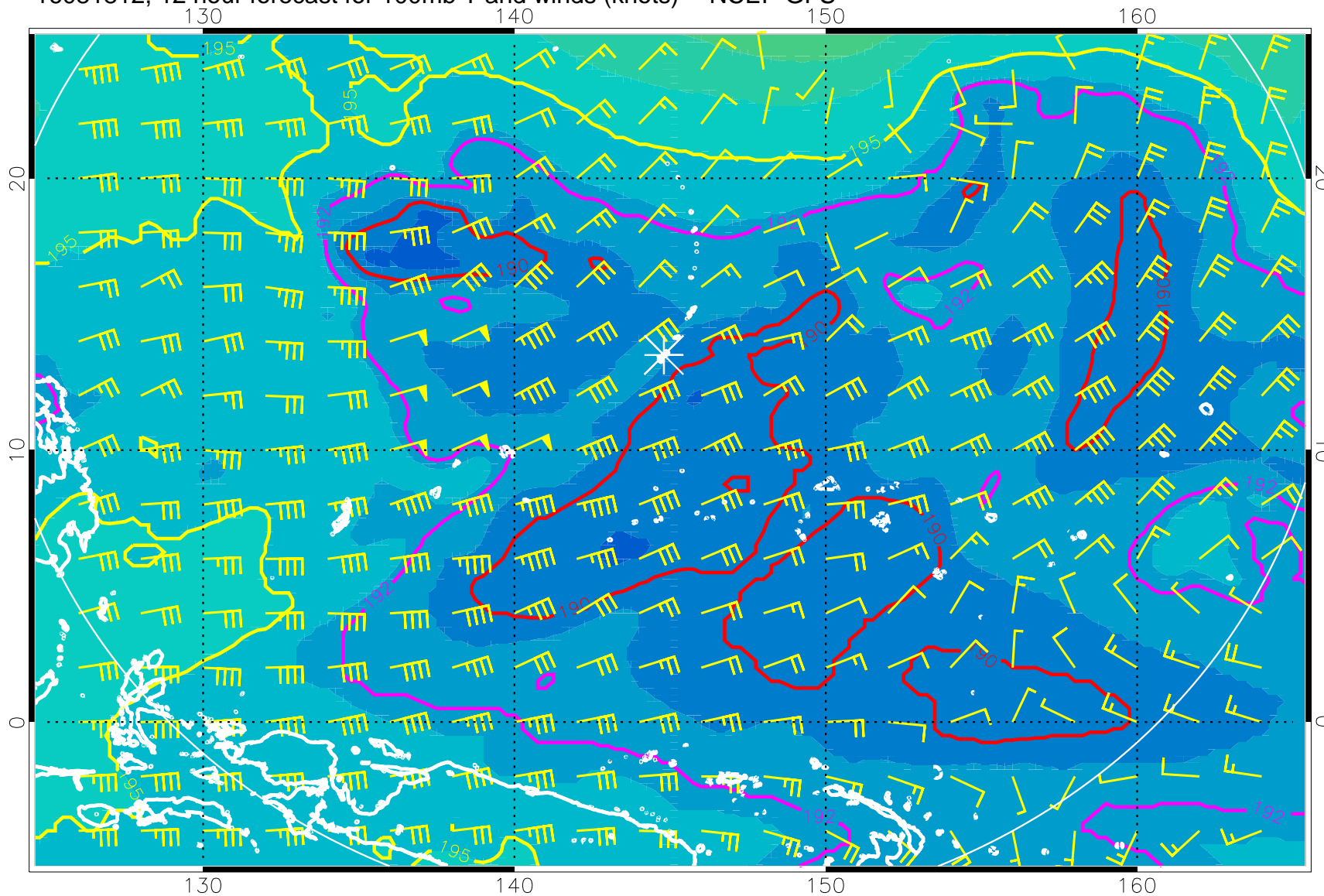
16081812, 12 hour forecast for 100mb T and winds (knots) -- NCEP GFS
