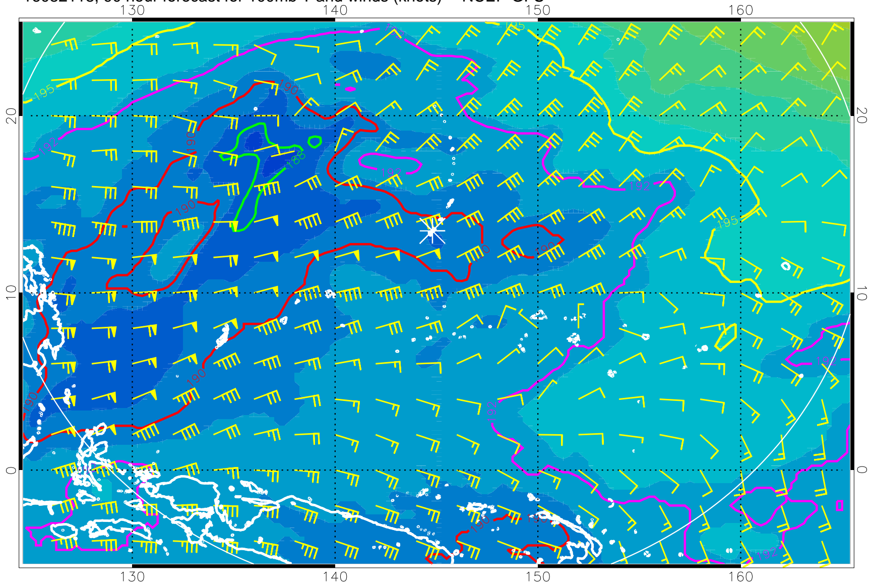
16082118, 90 hour forecast for 100mb T and winds (knots) -- NCEP GFS
