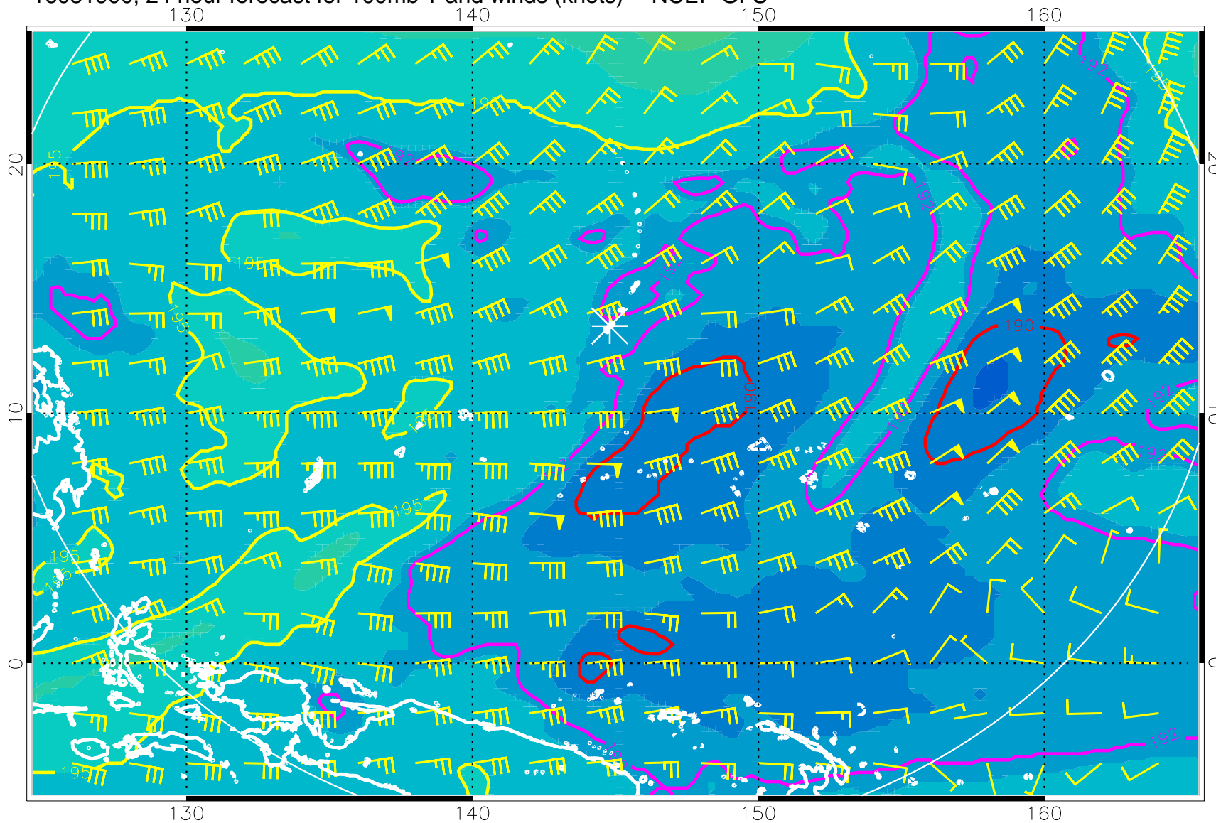
16081900, 24 hour forecast for 100mb T and winds (knots) -- NCEP GFS
