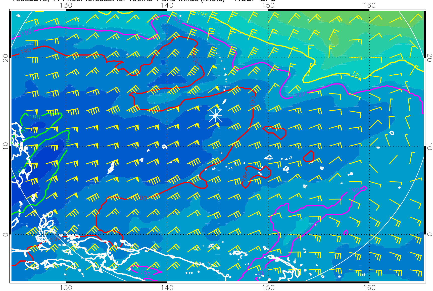
16082218, 114 hour forecast for 100mb T and winds (knots) -- NCEP GFS
