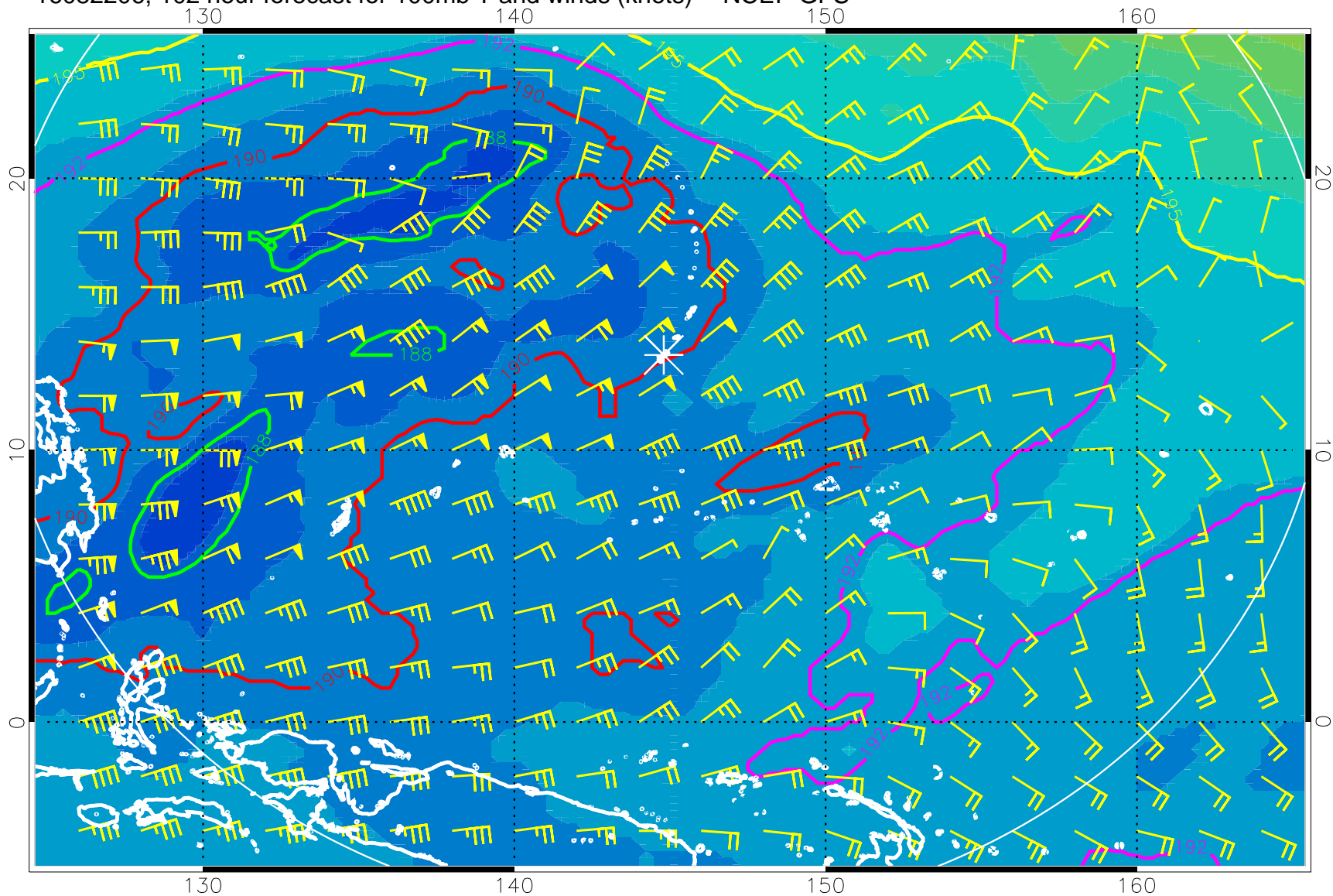
16082206, 102 hour forecast for 100mb T and winds (knots) -- NCEP GFS
