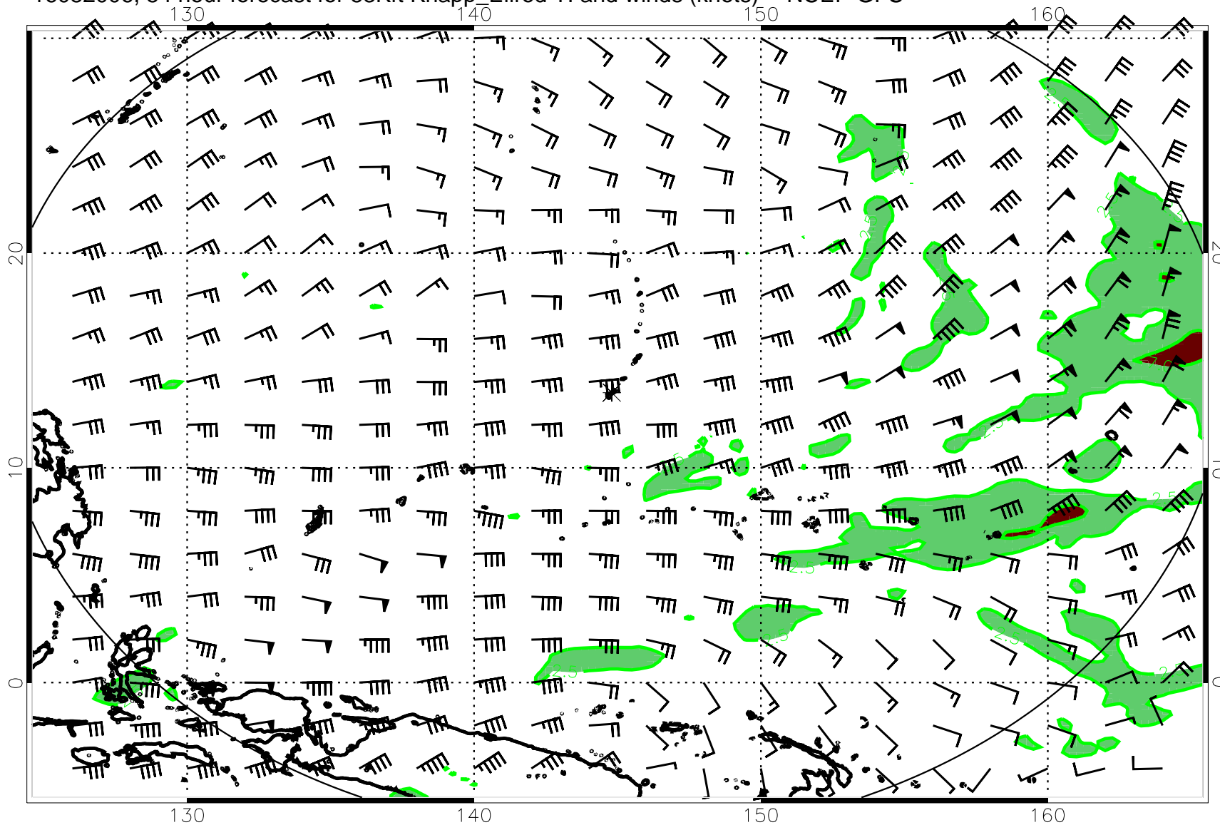
16082006, 54 hour forecast for 53Kft Knapp_Ellrod TI and winds (knots) -- NCEP GFS
