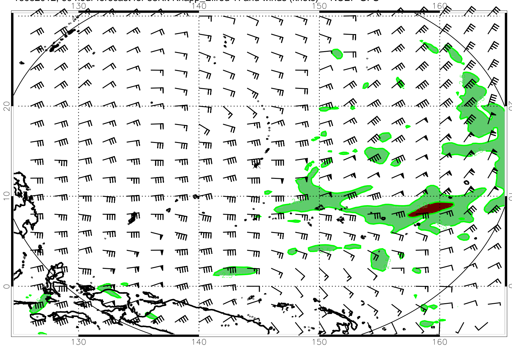
16082012, 60 hour forecast for 53Kft Knapp_Ellrod TI and winds (knots) -- NCEP GFS
