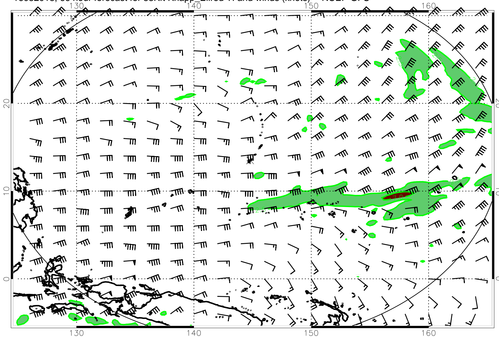
16082018, 66 hour forecast for 53Kft Knapp_Ellrod TI and winds (knots) -- NCEP GFS
