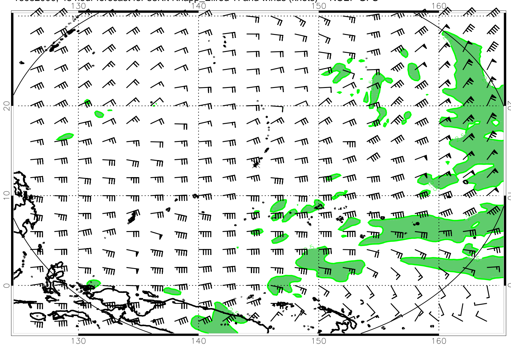
16082000, 48 hour forecast for 53Kft Knapp_Ellrod TI and winds (knots) -- NCEP GFS
