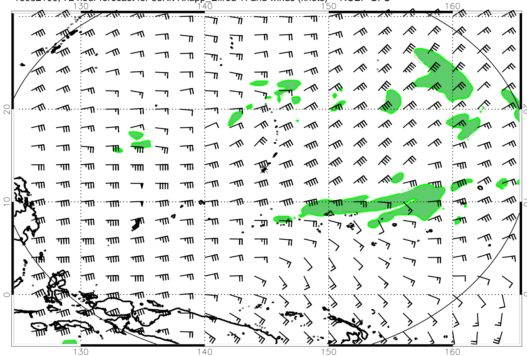
16082100, 72 hour forecast for 53Kft Knapp_Ellrod TI and winds (knots) -- NCEP GFS
