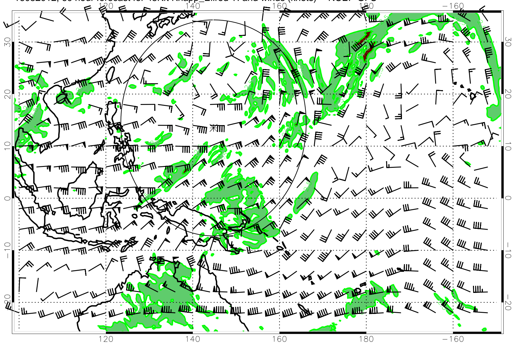
16082012, 60 hour forecast for 45Kft Knapp_Ellrod TI and winds (knots) -- NCEP GFS
