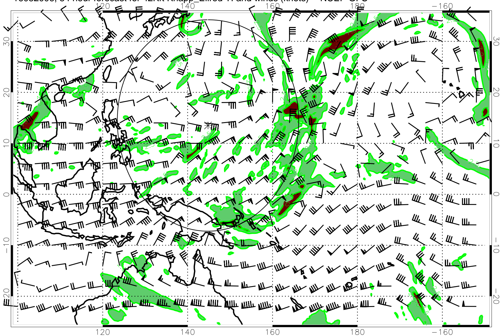
16082006, 54 hour forecast for 42Kft Knapp_Ellrod TI and winds (knots) -- NCEP GFS
