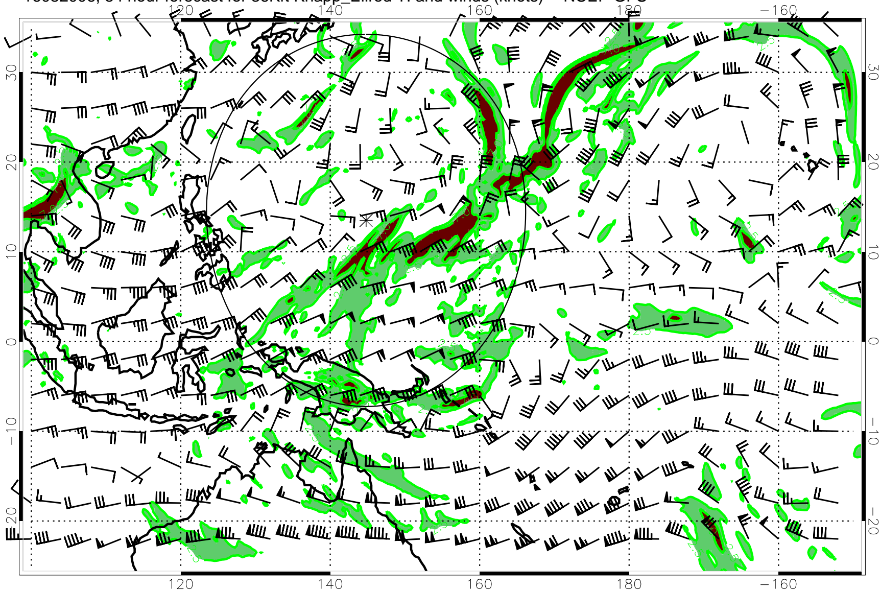
16082006, 54 hour forecast for 36Kft Knapp_Ellrod TI and winds (knots) -- NCEP GFS
