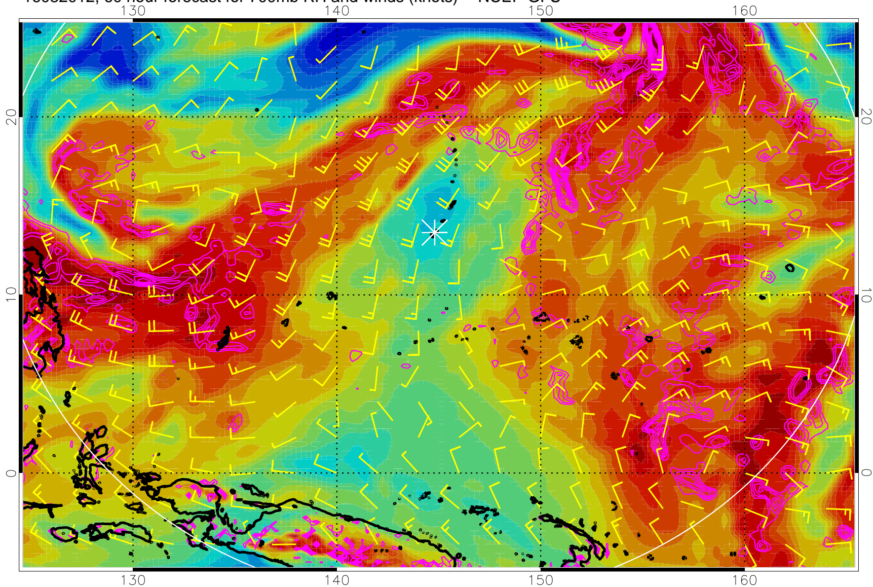
16082012, 60 hour forecast for 700mb RH and winds (knots) -- NCEP GFS
