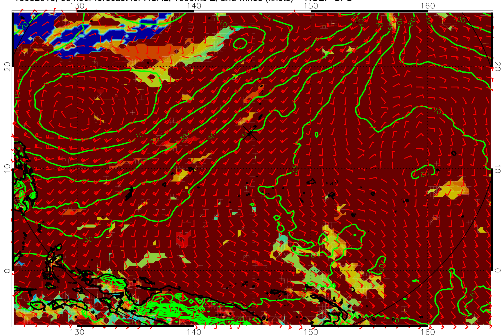
16082018, 66 hour forecast for HCAL, 1000mb Z, and winds (knots) -- NCEP GFS
