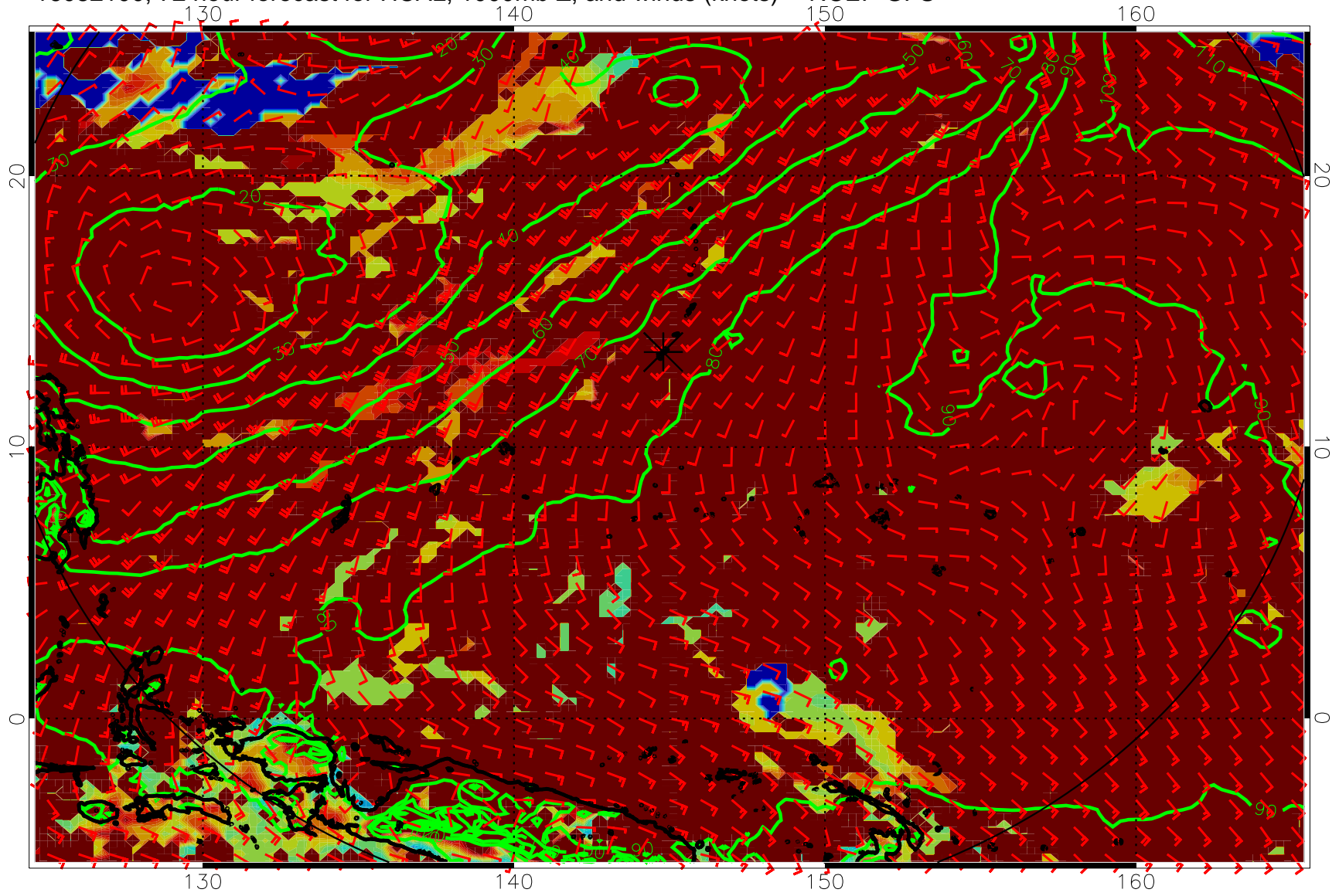
16082100, 72 hour forecast for HCAL, 1000mb Z, and winds (knots) -- NCEP GFS
