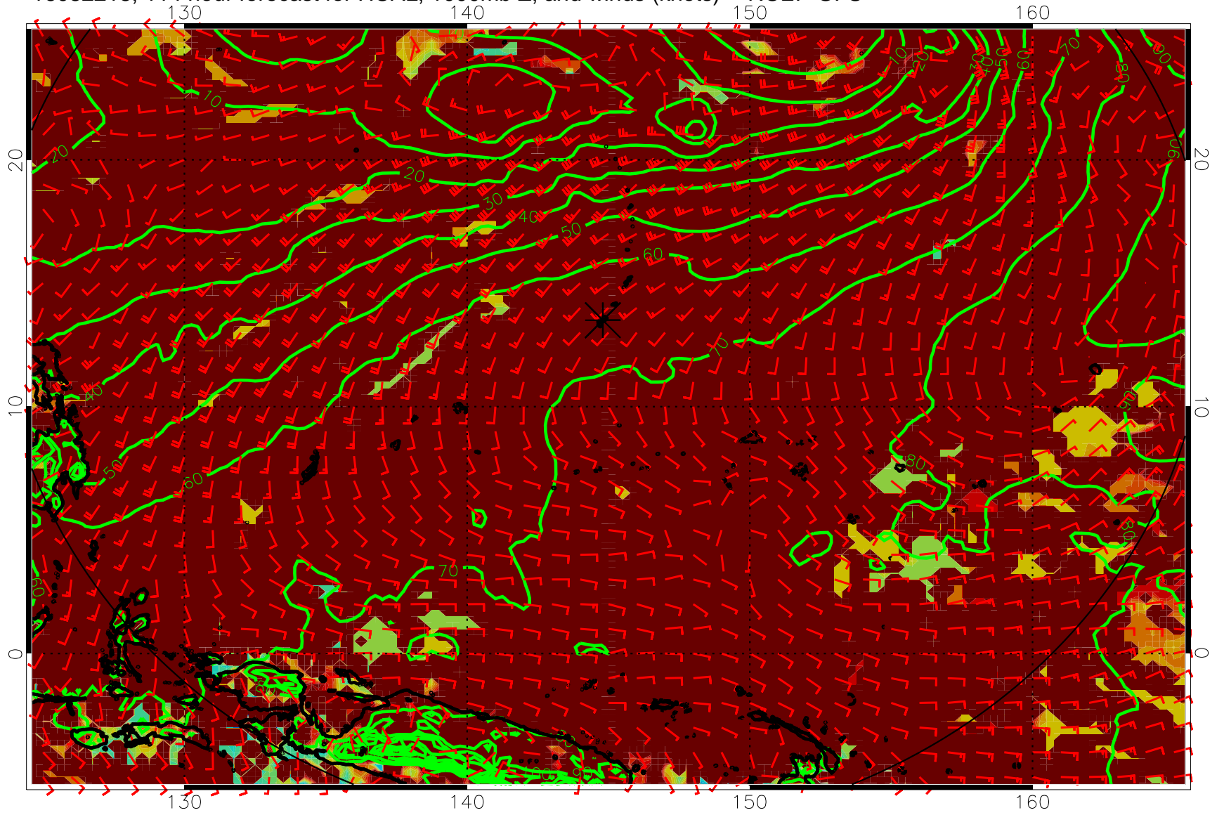
16082218, 114 hour forecast for HCAL, 1000mb Z, and winds (knots) -- NCEP GFS
