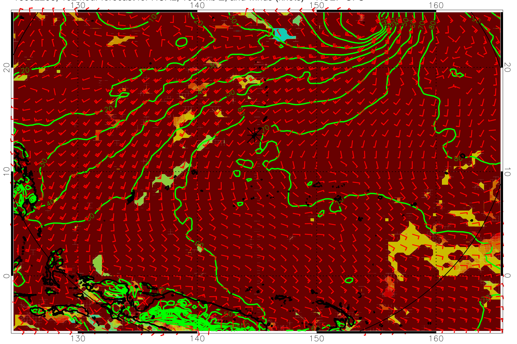
16082206, 102 hour forecast for HCAL, 1000mb Z, and winds (knots) -- NCEP GFS
