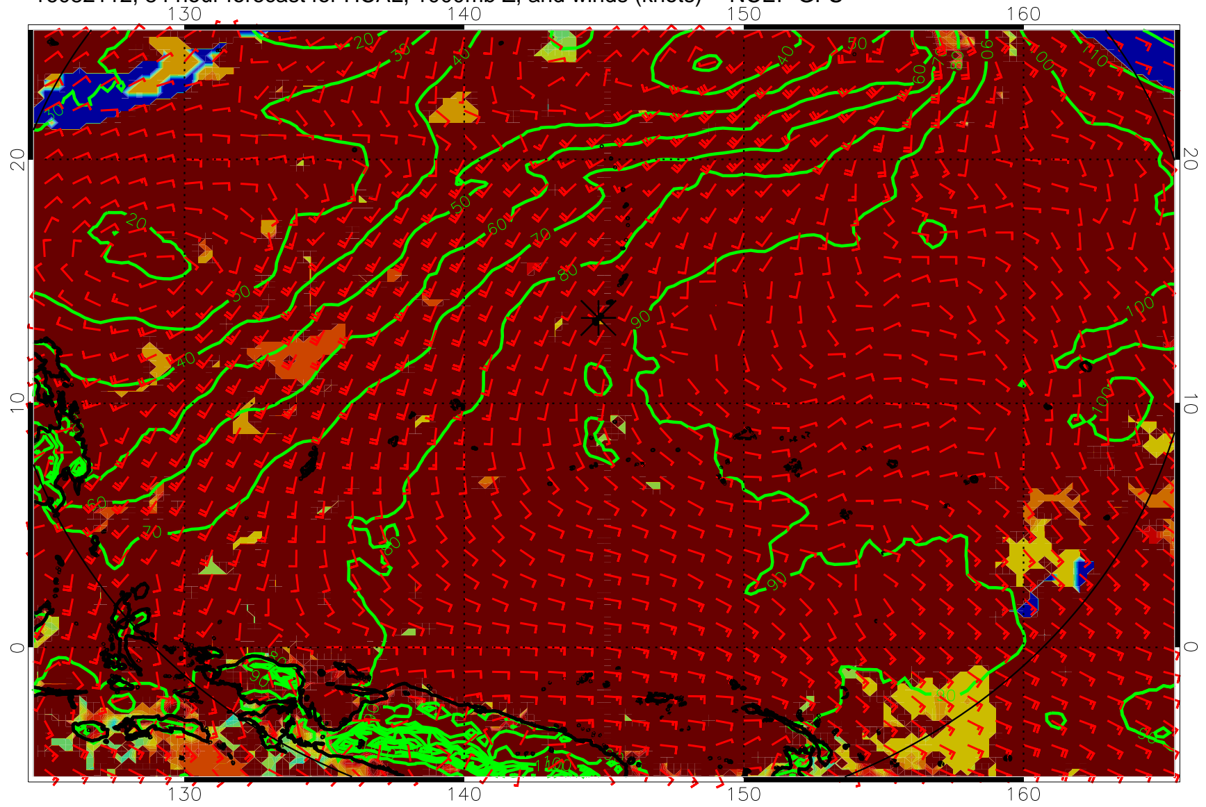
16082112, 84 hour forecast for HCAL, 1000mb Z, and winds (knots) -- NCEP GFS
