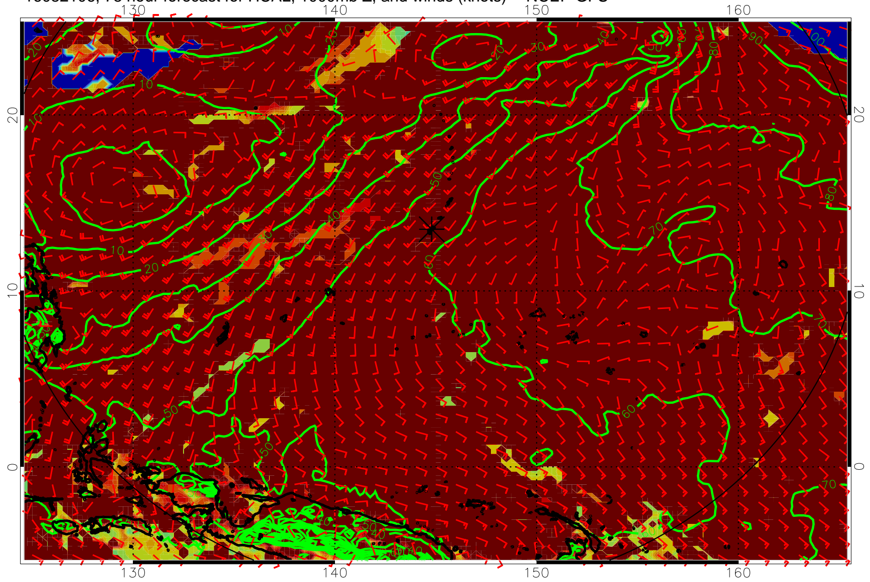
16082106, 78 hour forecast for HCAL, 1000mb Z, and winds (knots) -- NCEP GFS
