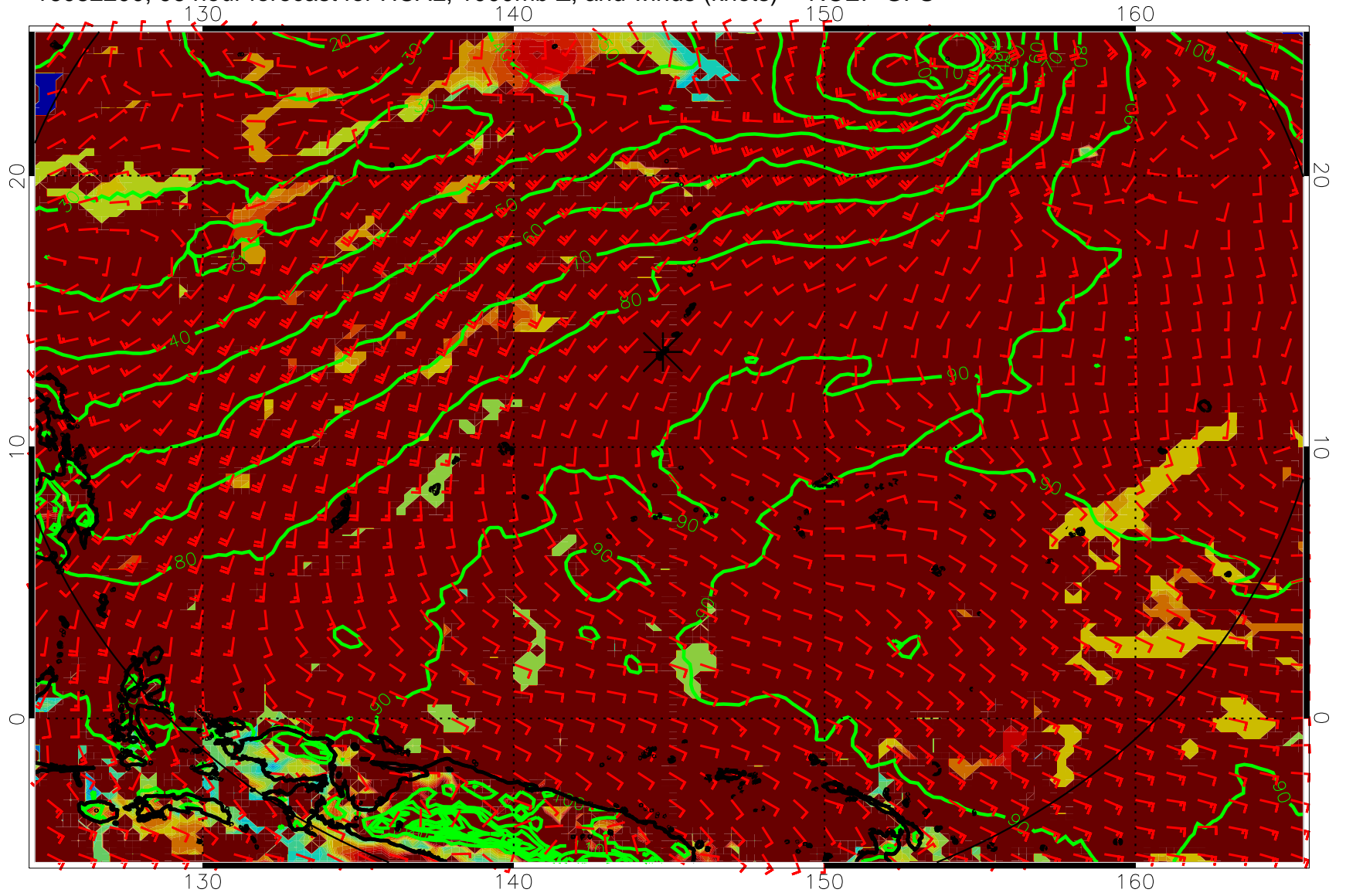
16082200, 96 hour forecast for HCAL, 1000mb Z, and winds (knots) -- NCEP GFS
