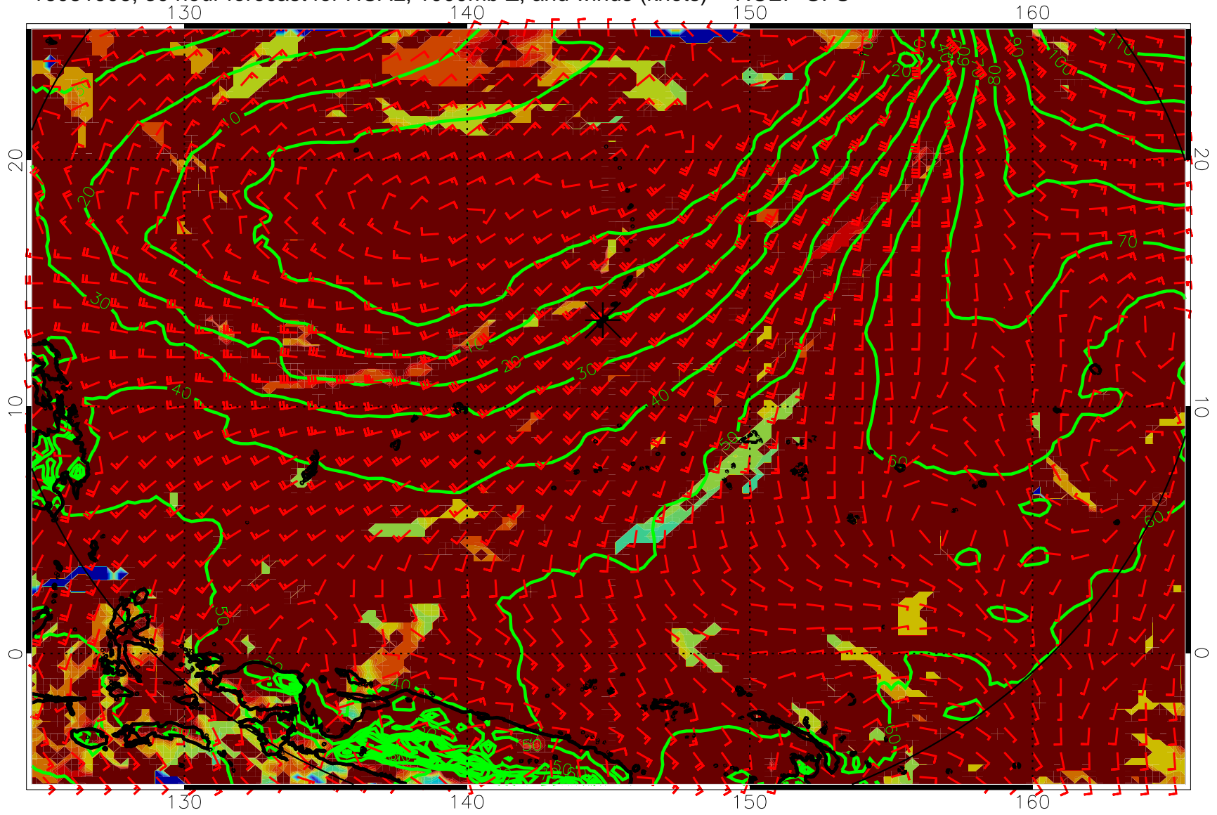
16081906, 30 hour forecast for HCAL, 1000mb Z, and winds (knots) -- NCEP GFS
