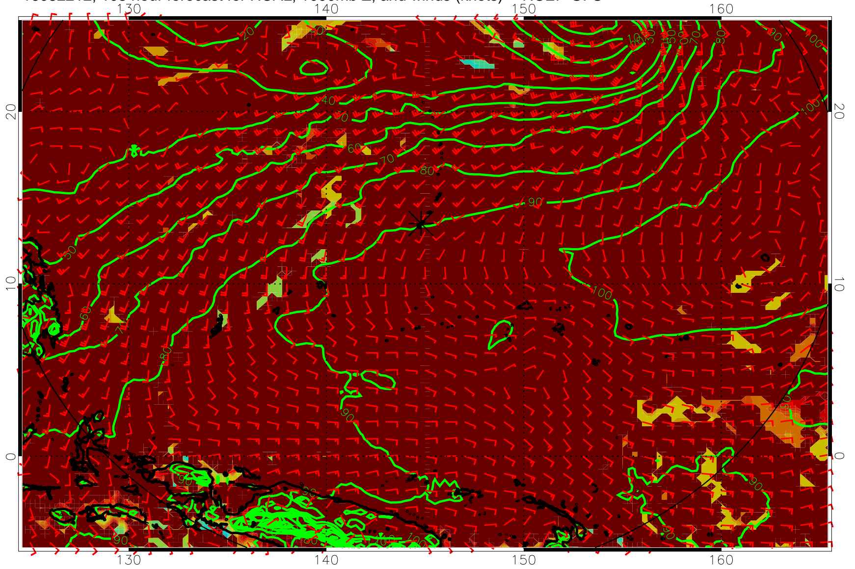
16082212, 108 hour forecast for HCAL, 1000mb Z, and winds (knots) -- NCEP GFS
