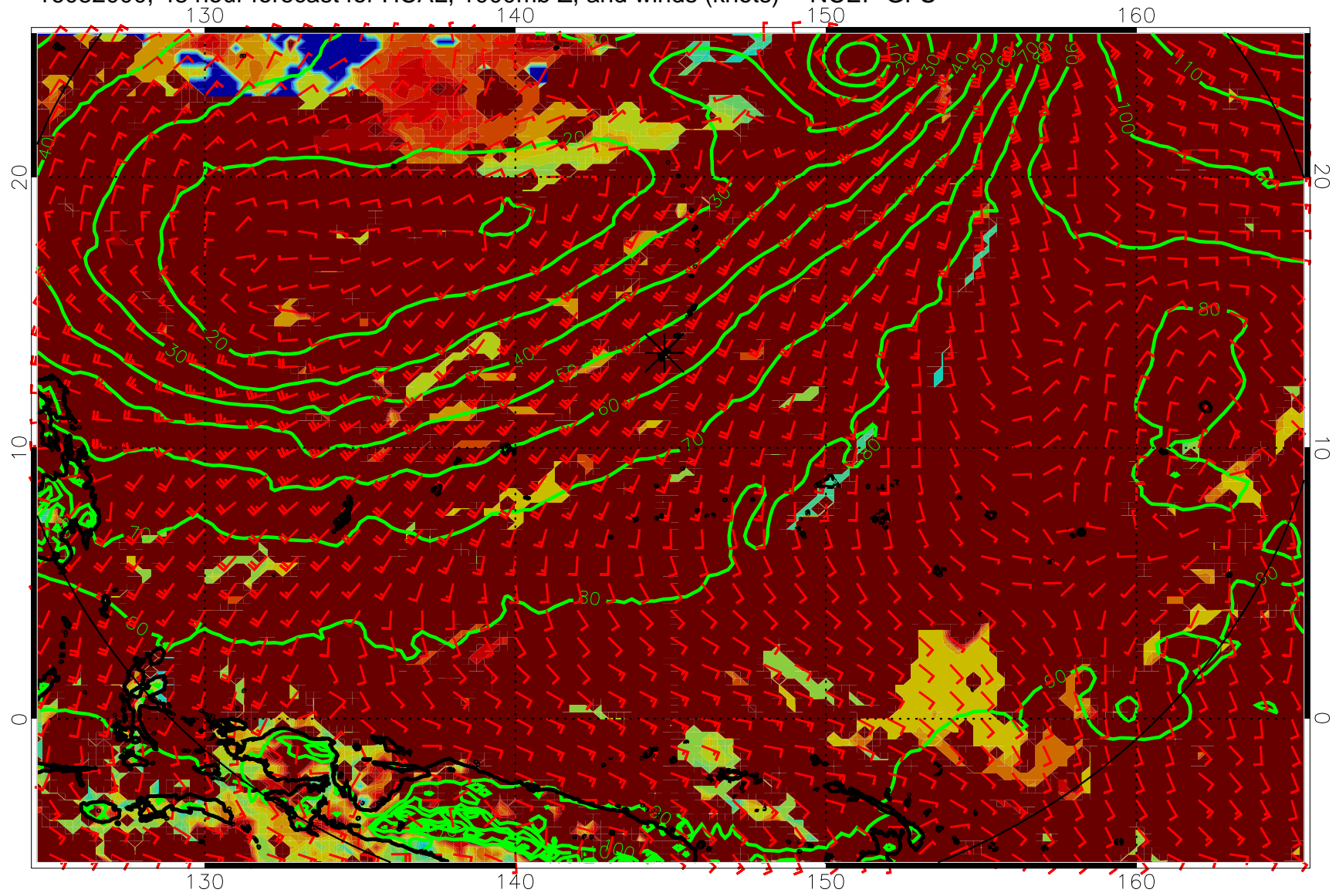
16082000, 48 hour forecast for HCAL, 1000mb Z, and winds (knots) -- NCEP GFS
