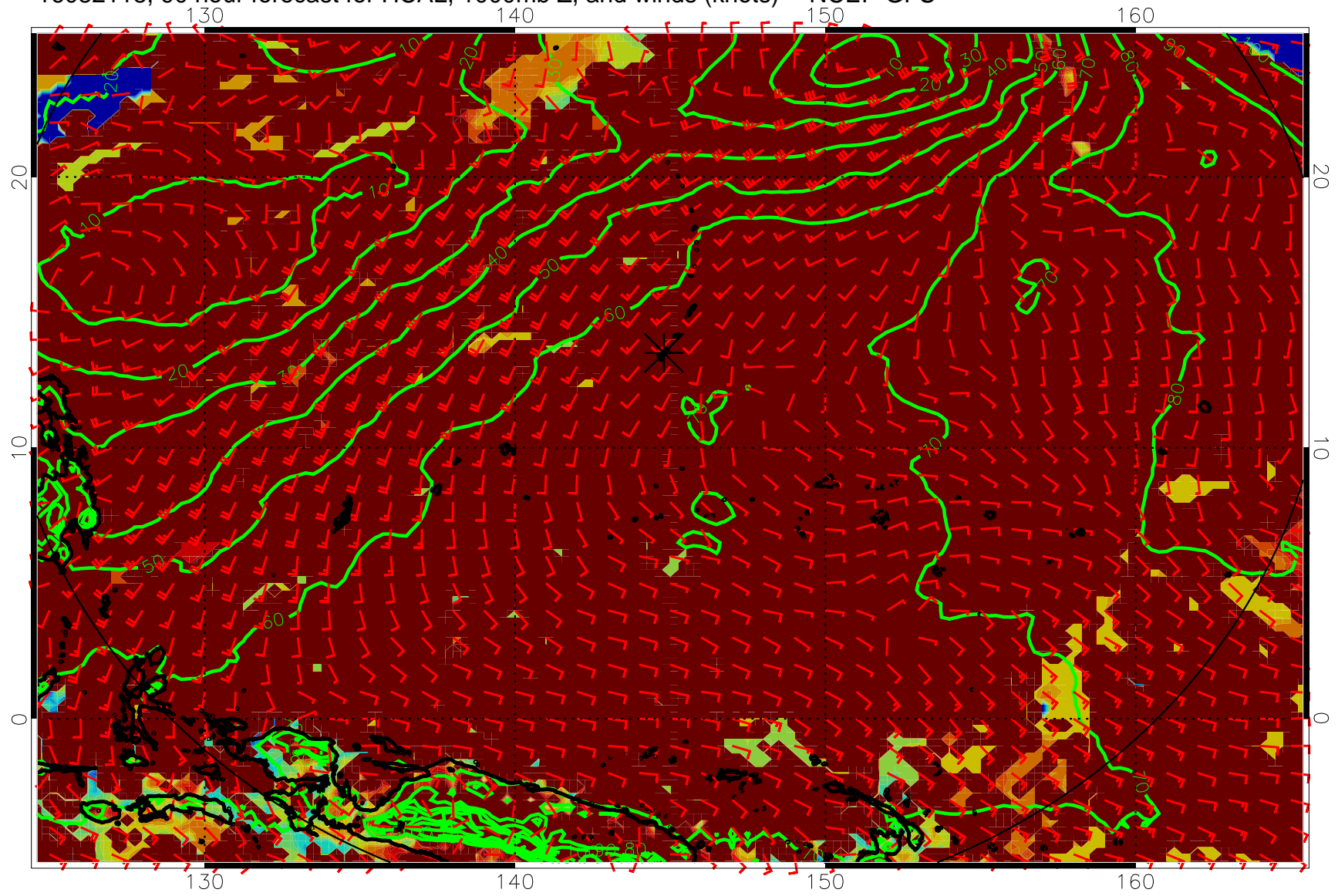
16082118, 90 hour forecast for HCAL, 1000mb Z, and winds (knots) -- NCEP GFS
