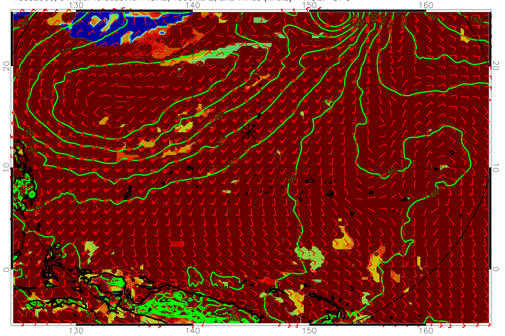
16082006, 54 hour forecast for HCAL, 1000mb Z, and winds (knots) -- NCEP GFS
