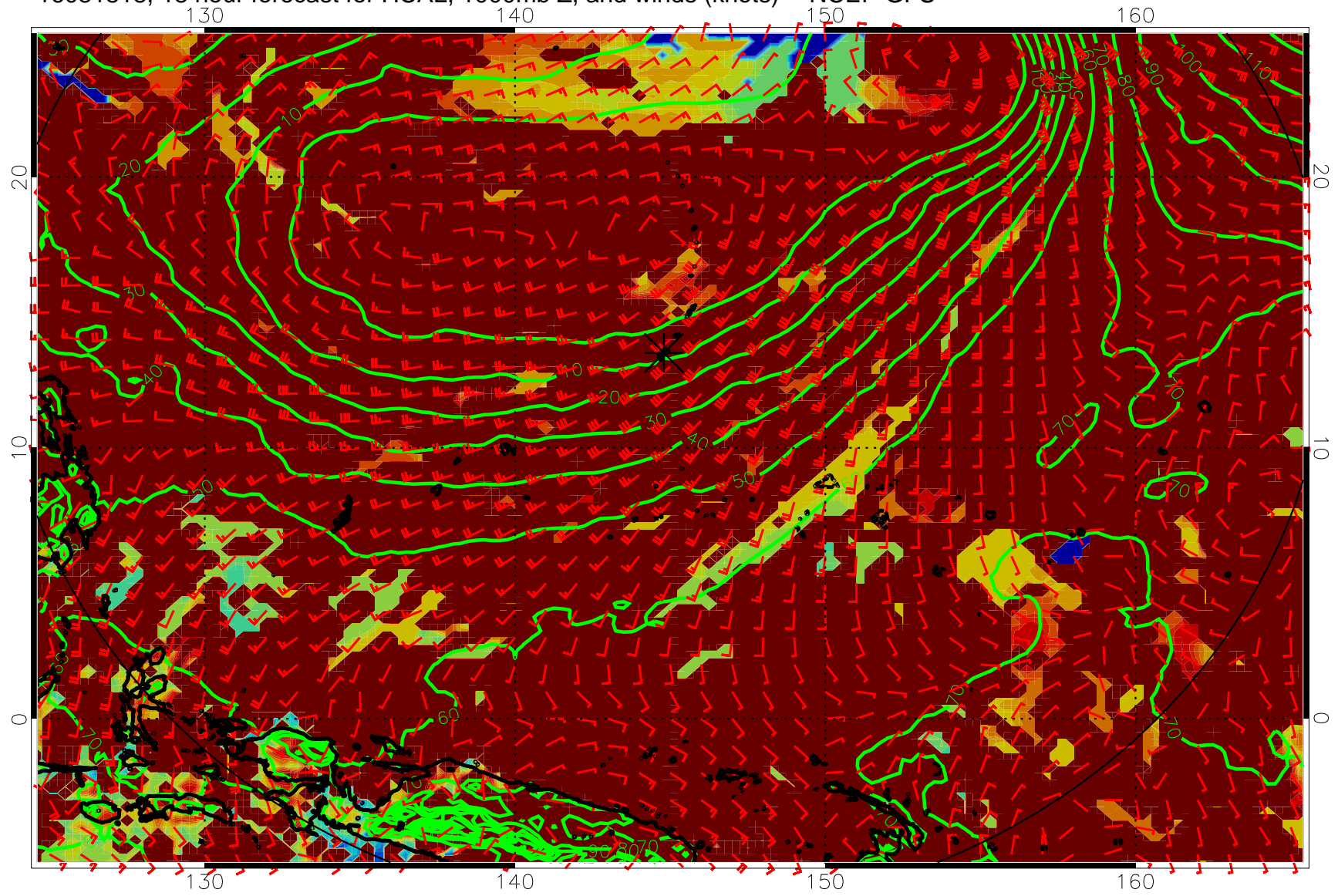
16081818, 18 hour forecast for HCAL, 1000mb Z, and winds (knots) -- NCEP GFS
