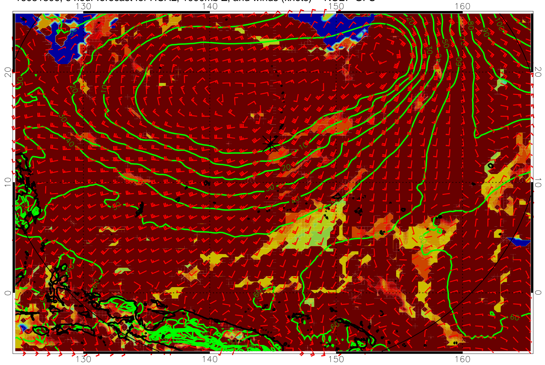
16081806, 6 hour forecast for HCAL, 1000mb Z, and winds (knots) -- NCEP GFS
