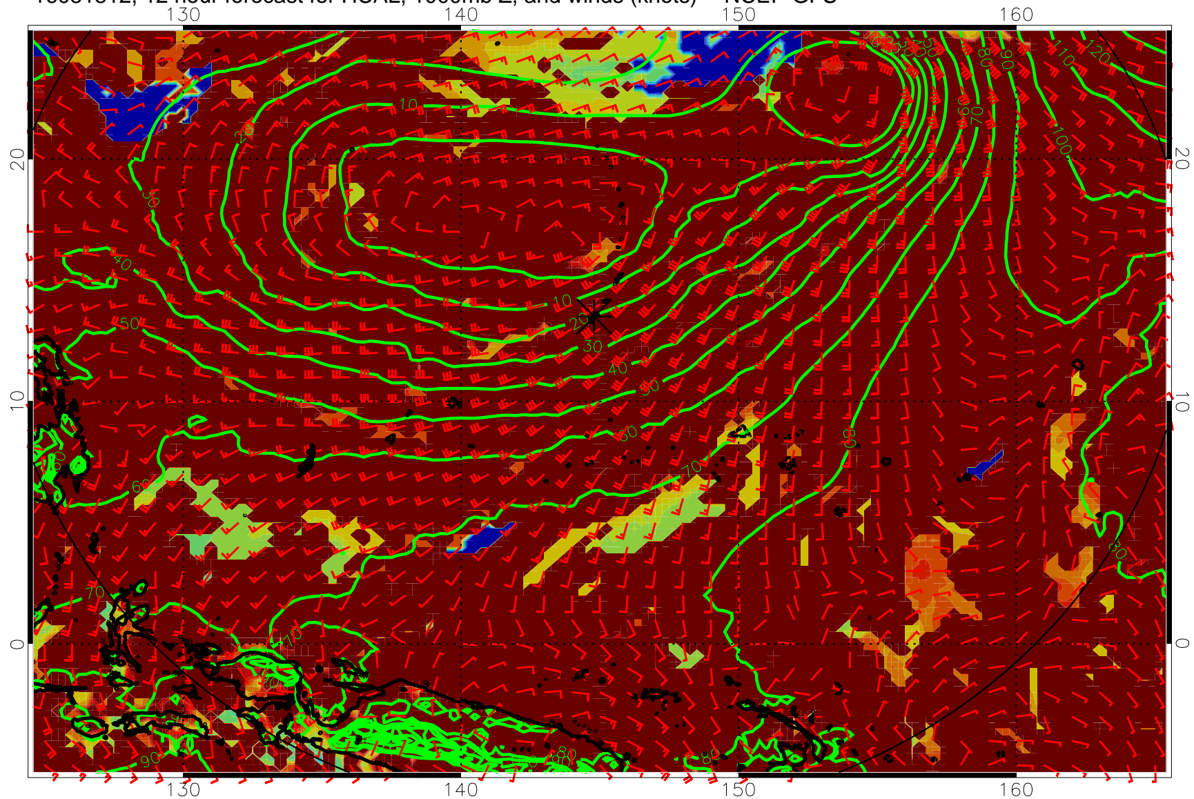
16081812, 12 hour forecast for HCAL, 1000mb Z, and winds (knots) -- NCEP GFS
