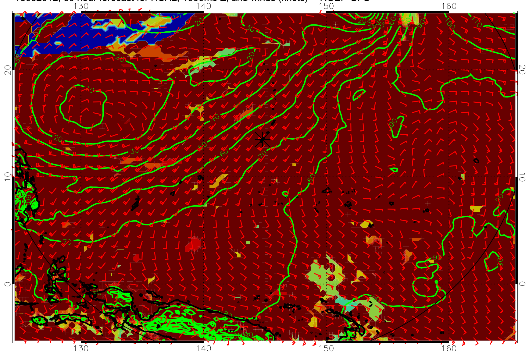
16082012, 60 hour forecast for HCAL, 1000mb Z, and winds (knots) -- NCEP GFS
