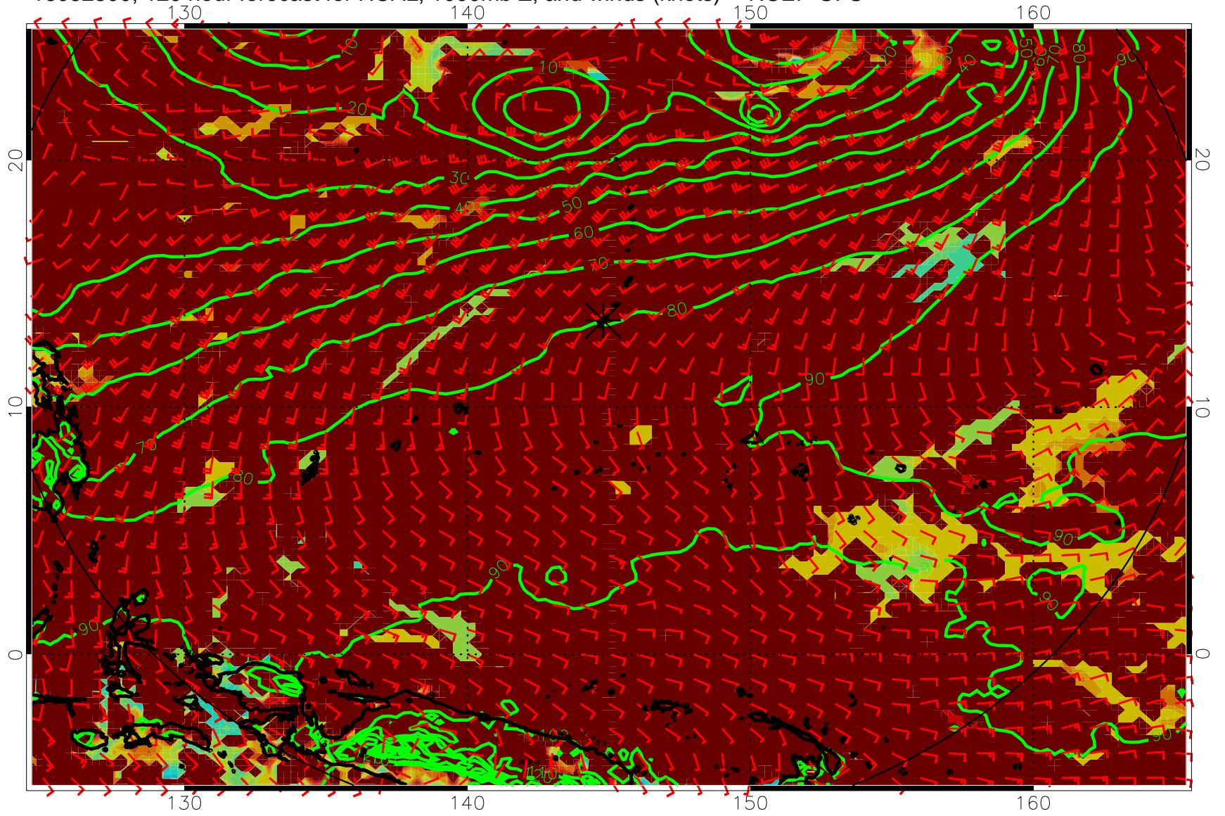
16082300, 120 hour forecast for HCAL, 1000mb Z, and winds (knots) -- NCEP GFS
