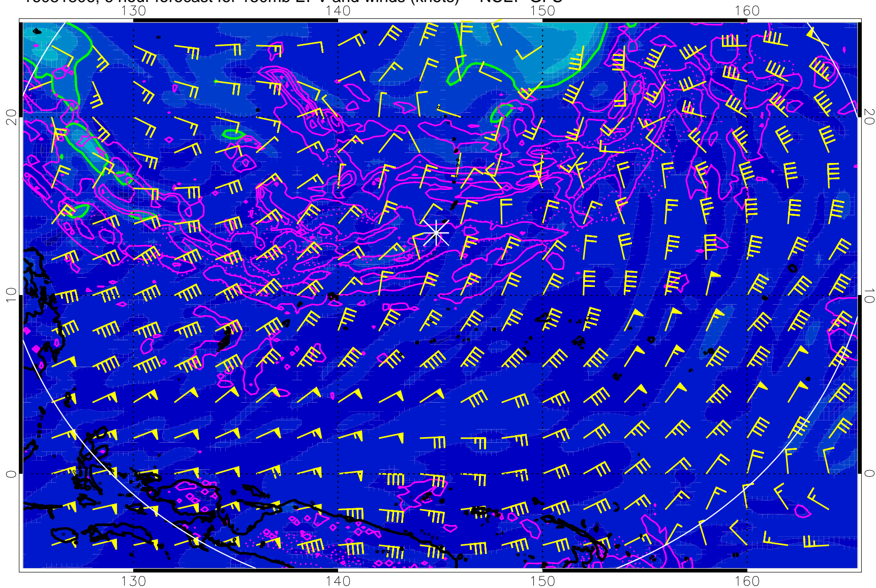
16081806, 6 hour forecast for 150mb EPV and winds (knots) -- NCEP GFS
