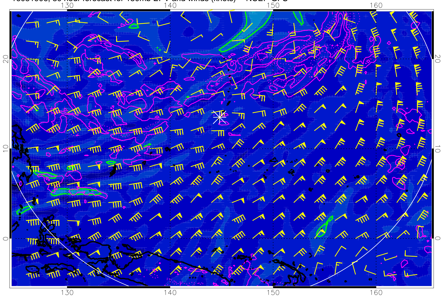
16081906, 30 hour forecast for 150mb EPV and winds (knots) -- NCEP GFS
