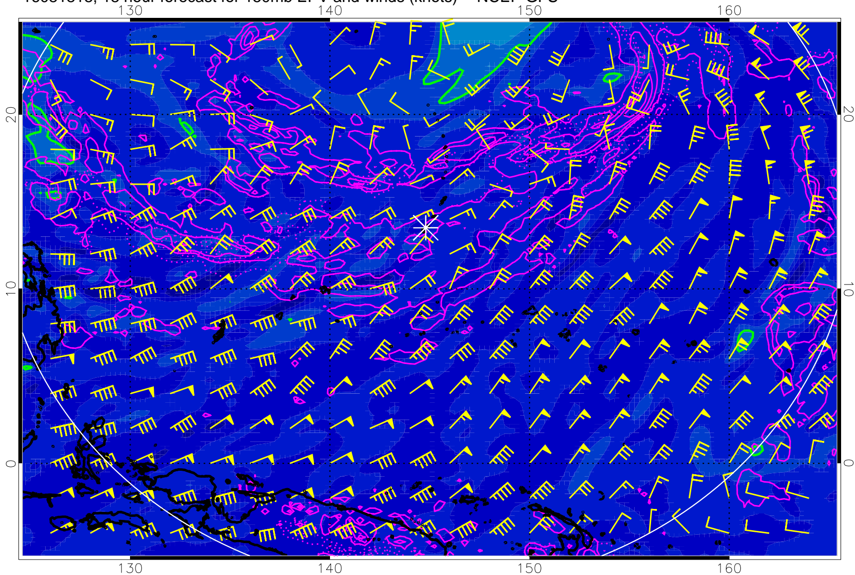
16081818, 18 hour forecast for 150mb EPV and winds (knots) -- NCEP GFS
