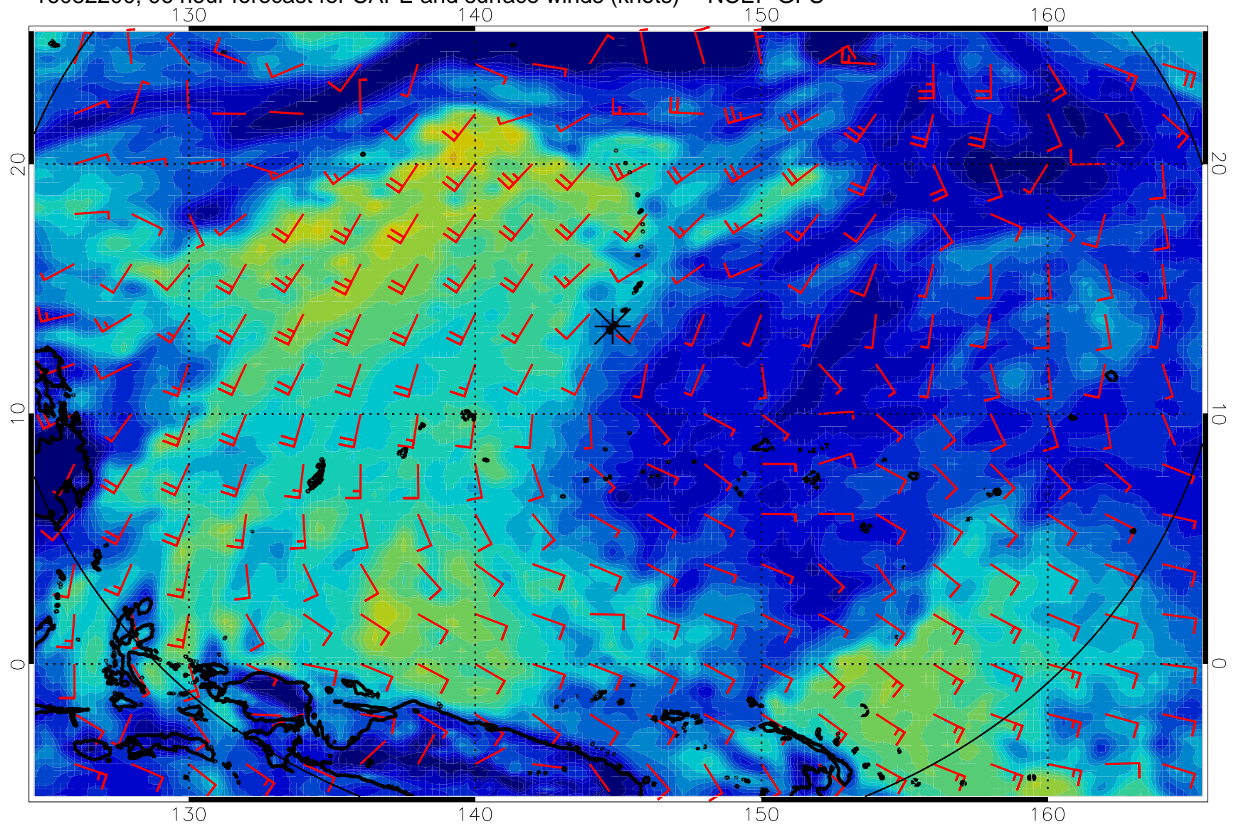
16082200, 96 hour forecast for CAPE and surface winds (knots) -- NCEP GFS
