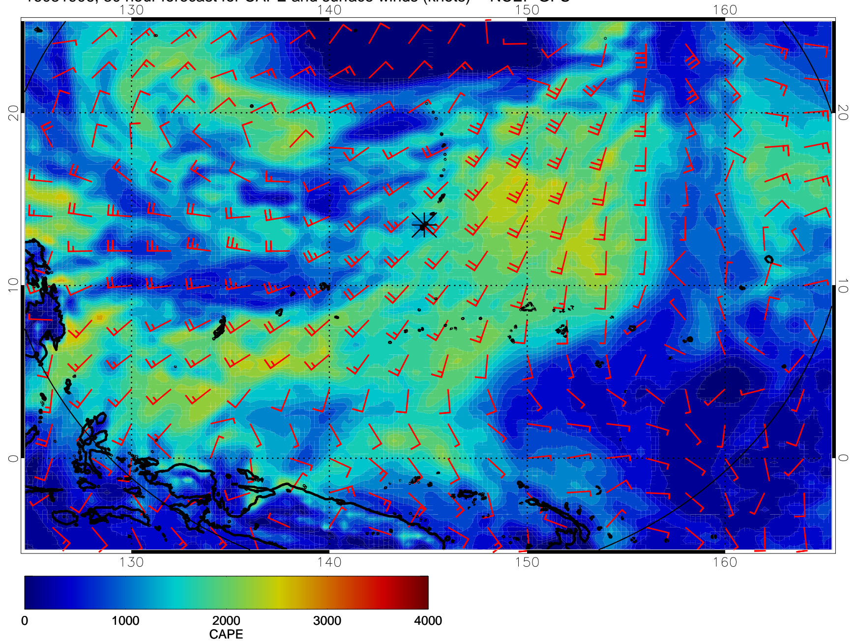
16081906, 30 hour forecast for CAPE and surface winds (knots) -- NCEP GFS
