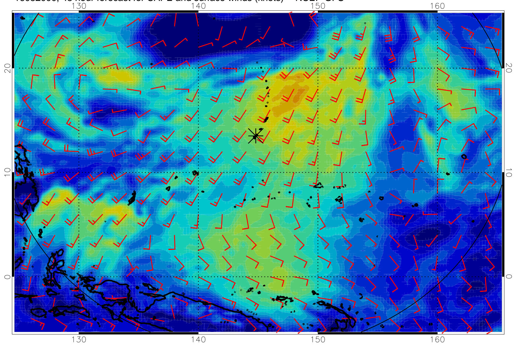
16082000, 48 hour forecast for CAPE and surface winds (knots) -- NCEP GFS
