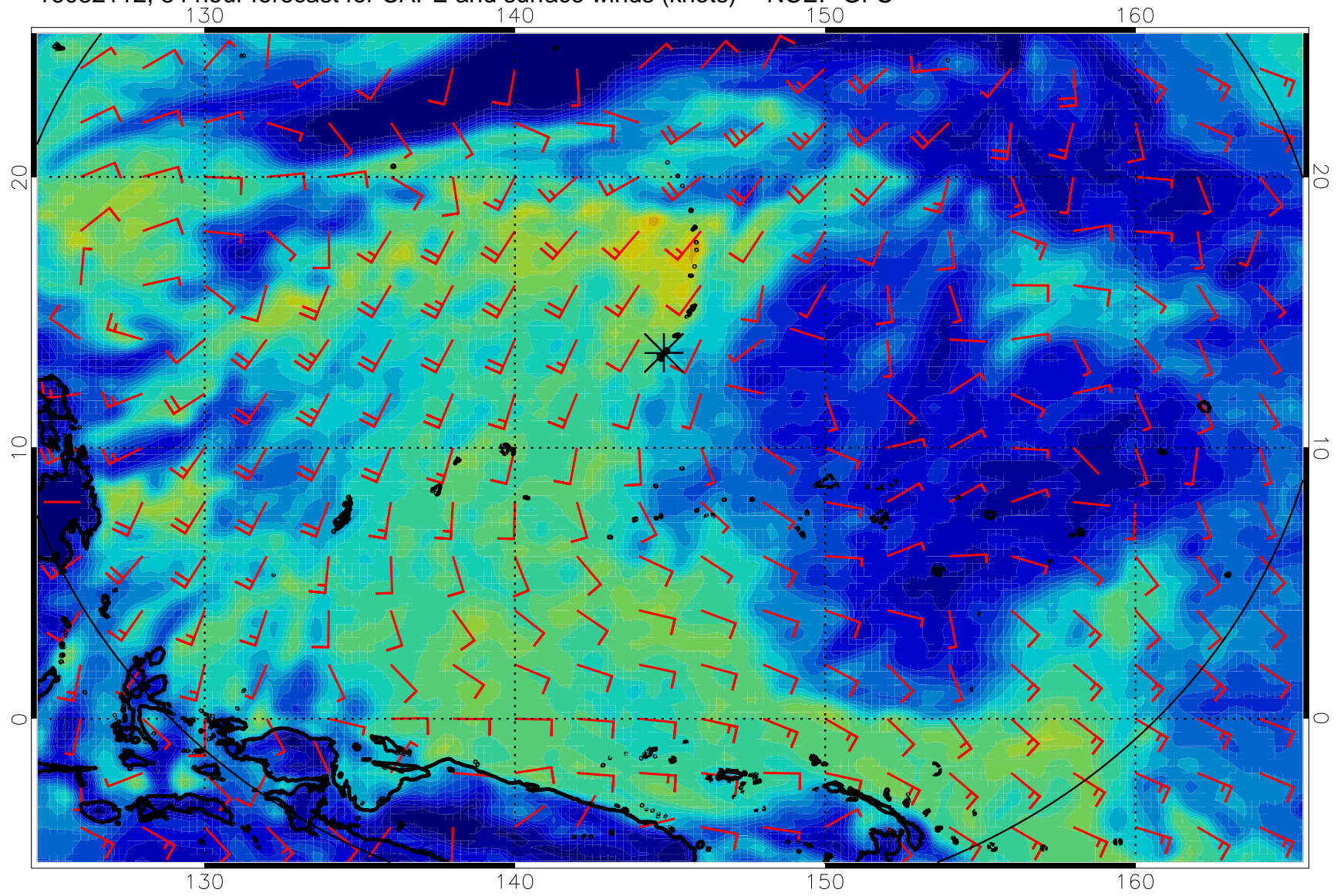
16082112, 84 hour forecast for CAPE and surface winds (knots) -- NCEP GFS
