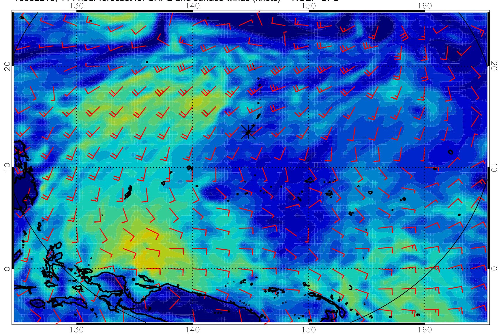
16082218, 114 hour forecast for CAPE and surface winds (knots) -- NCEP GFS
