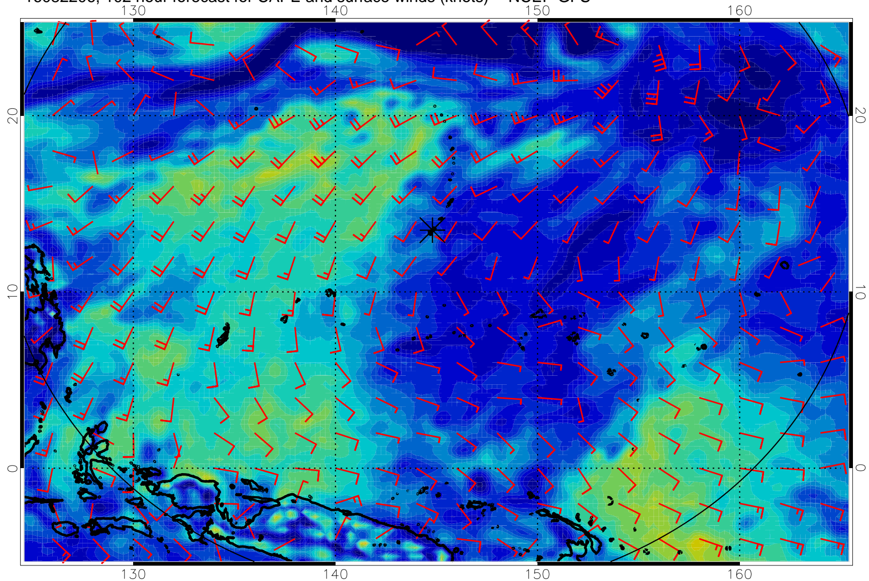
16082206, 102 hour forecast for CAPE and surface winds (knots) -- NCEP GFS
