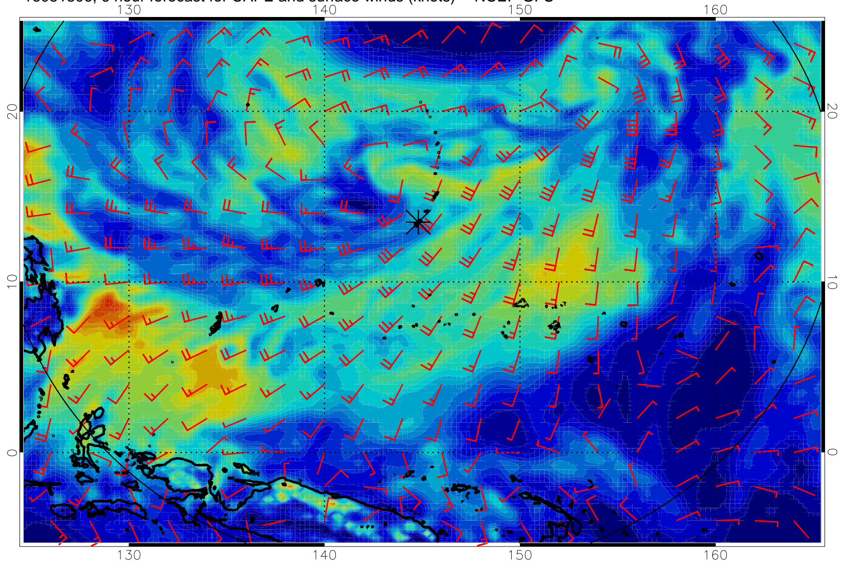
16081806, 6 hour forecast for CAPE and surface winds (knots) -- NCEP GFS
