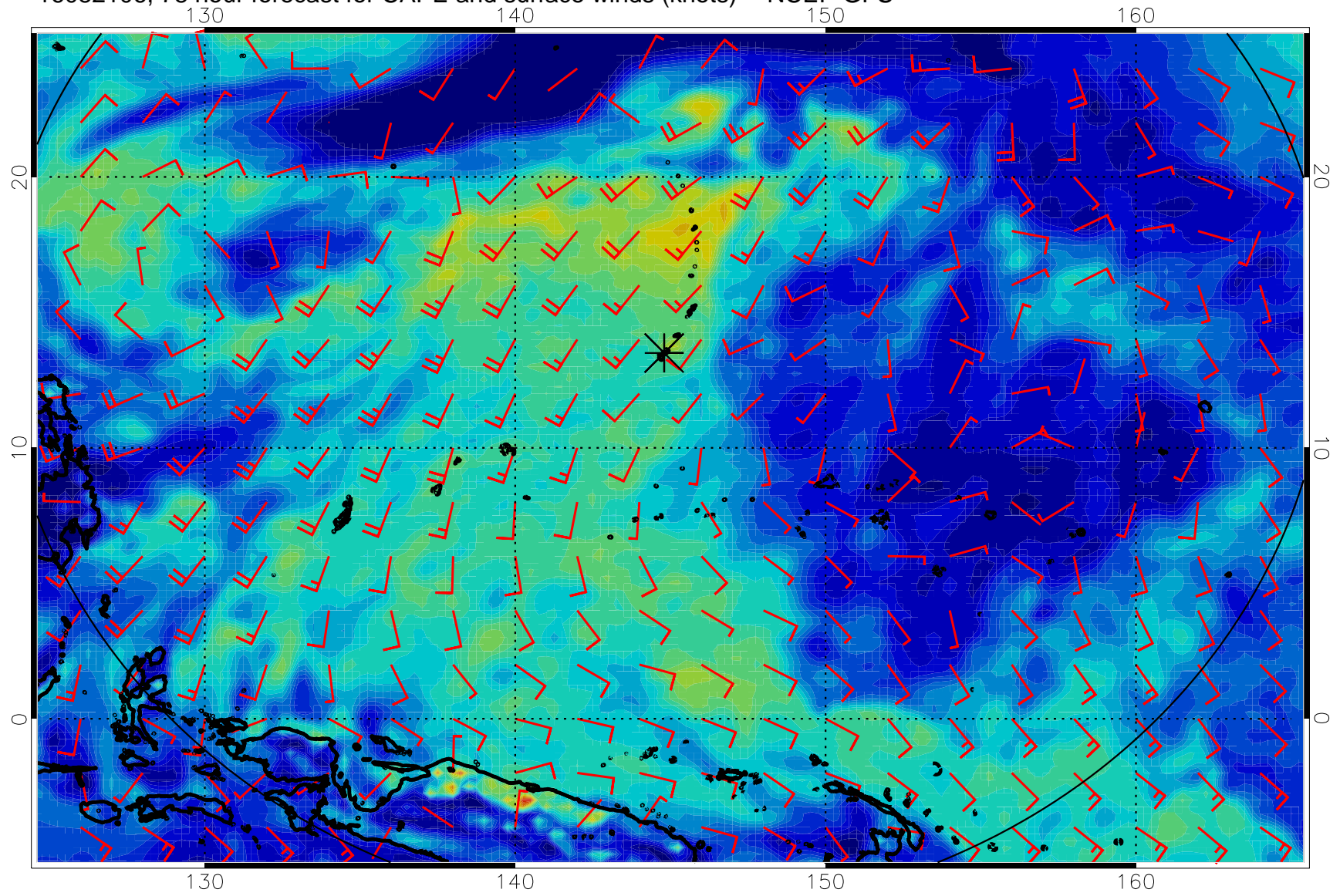
16082106, 78 hour forecast for CAPE and surface winds (knots) -- NCEP GFS
