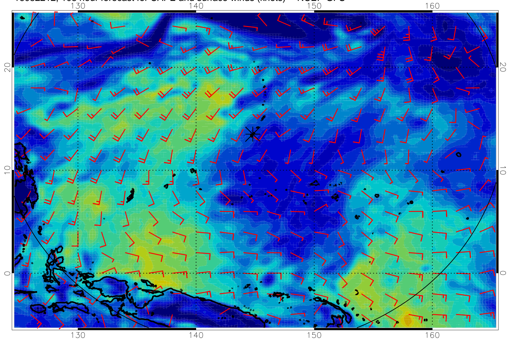
16082212, 108 hour forecast for CAPE and surface winds (knots) -- NCEP GFS
