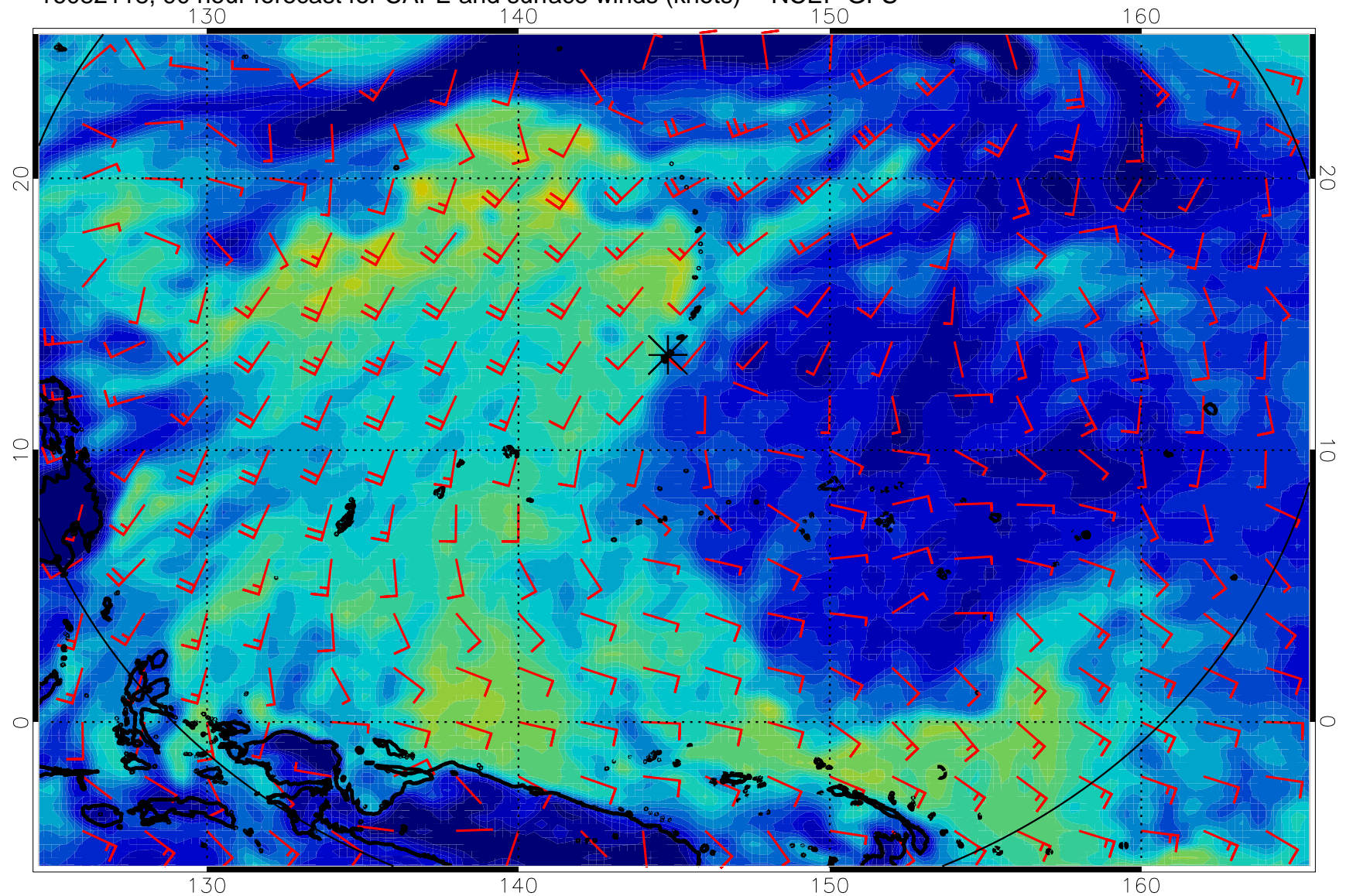
16082118, 90 hour forecast for CAPE and surface winds (knots) -- NCEP GFS
