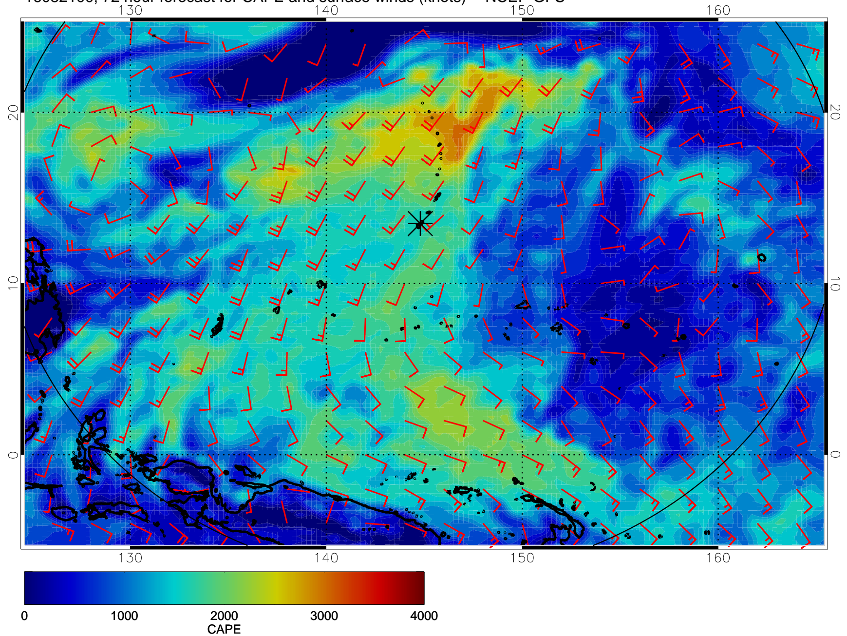
16082100, 72 hour forecast for CAPE and surface winds (knots) -- NCEP GFS
