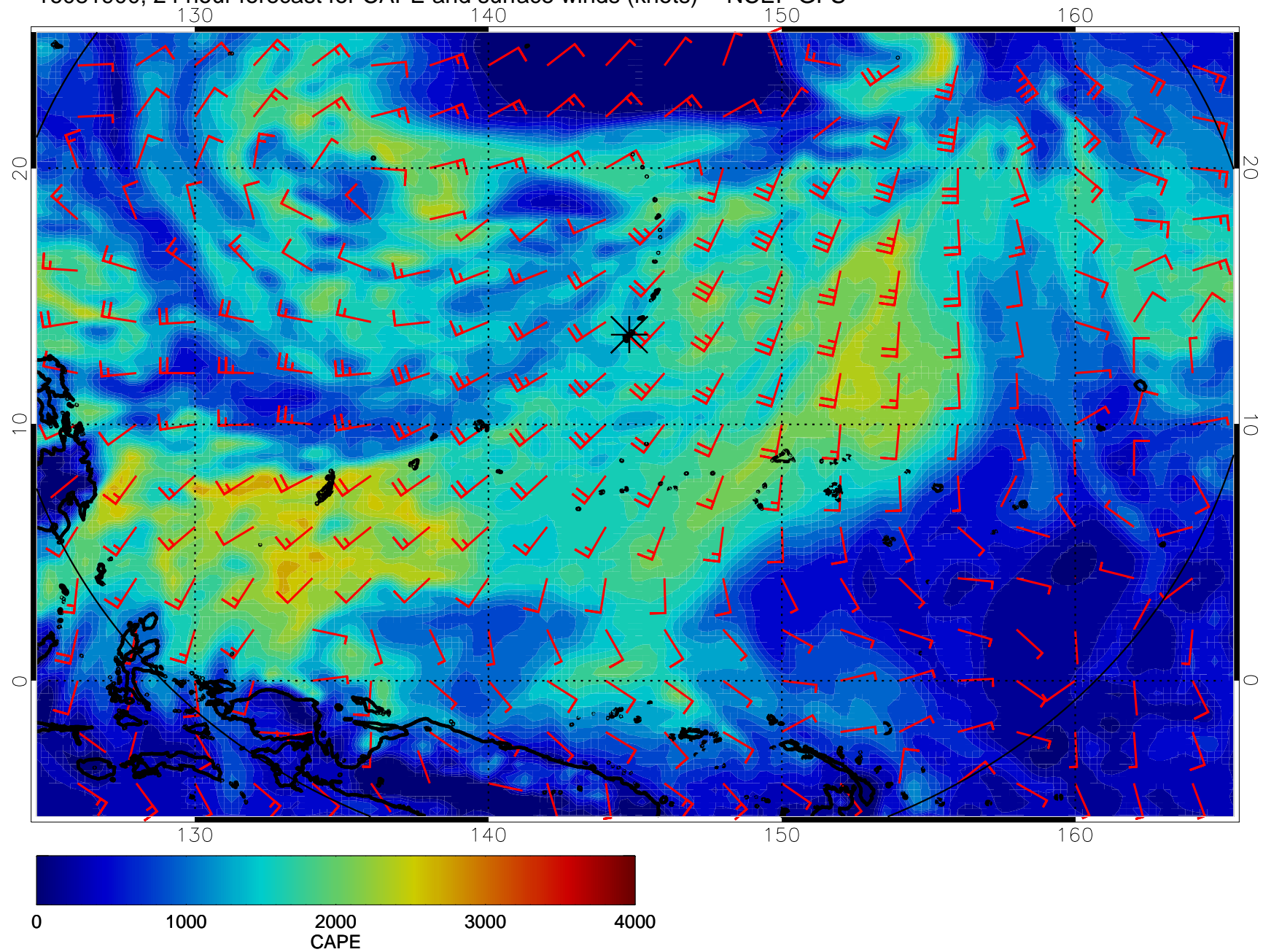
16081900, 24 hour forecast for CAPE and surface winds (knots) -- NCEP GFS
