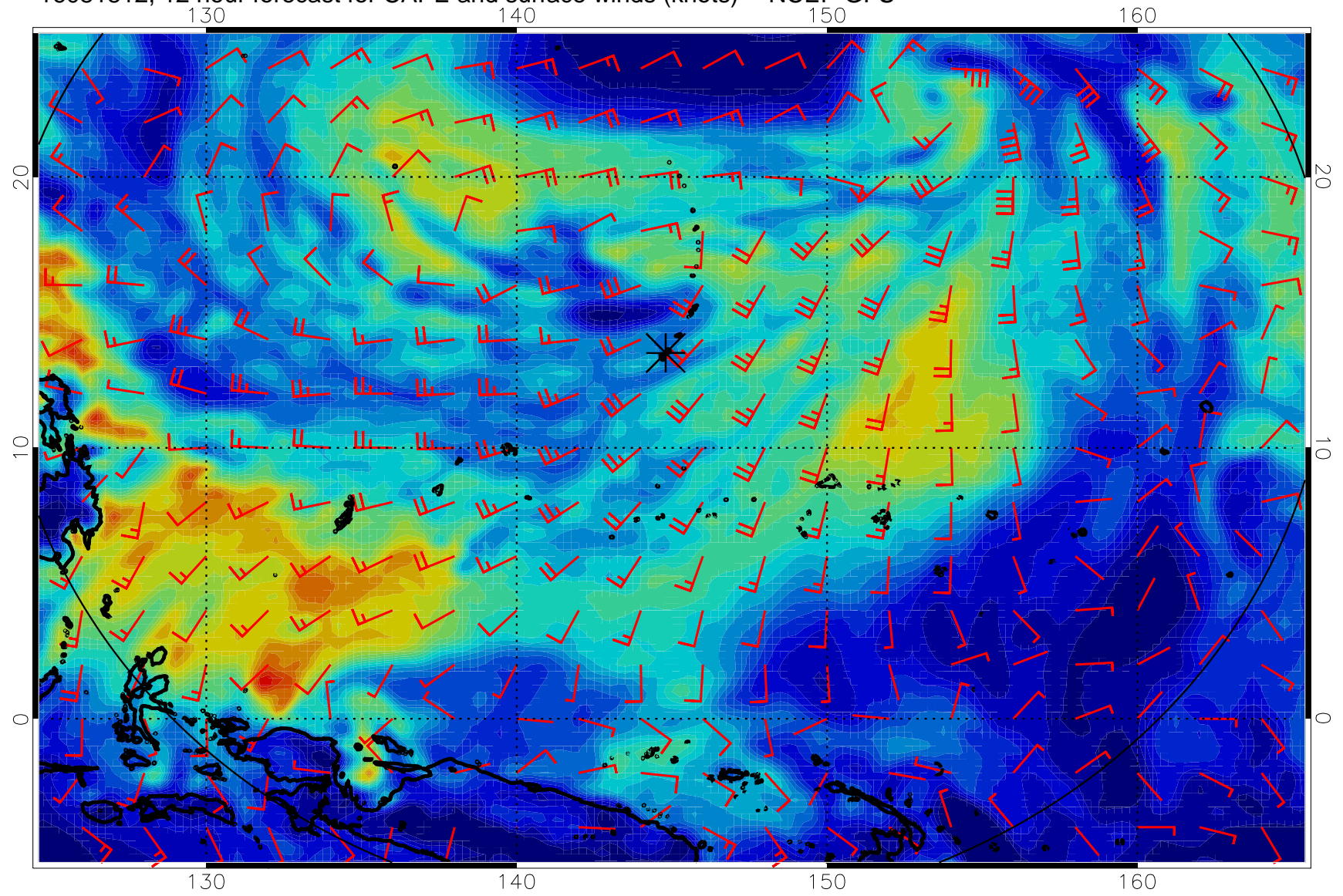
16081812, 12 hour forecast for CAPE and surface winds (knots) -- NCEP GFS
