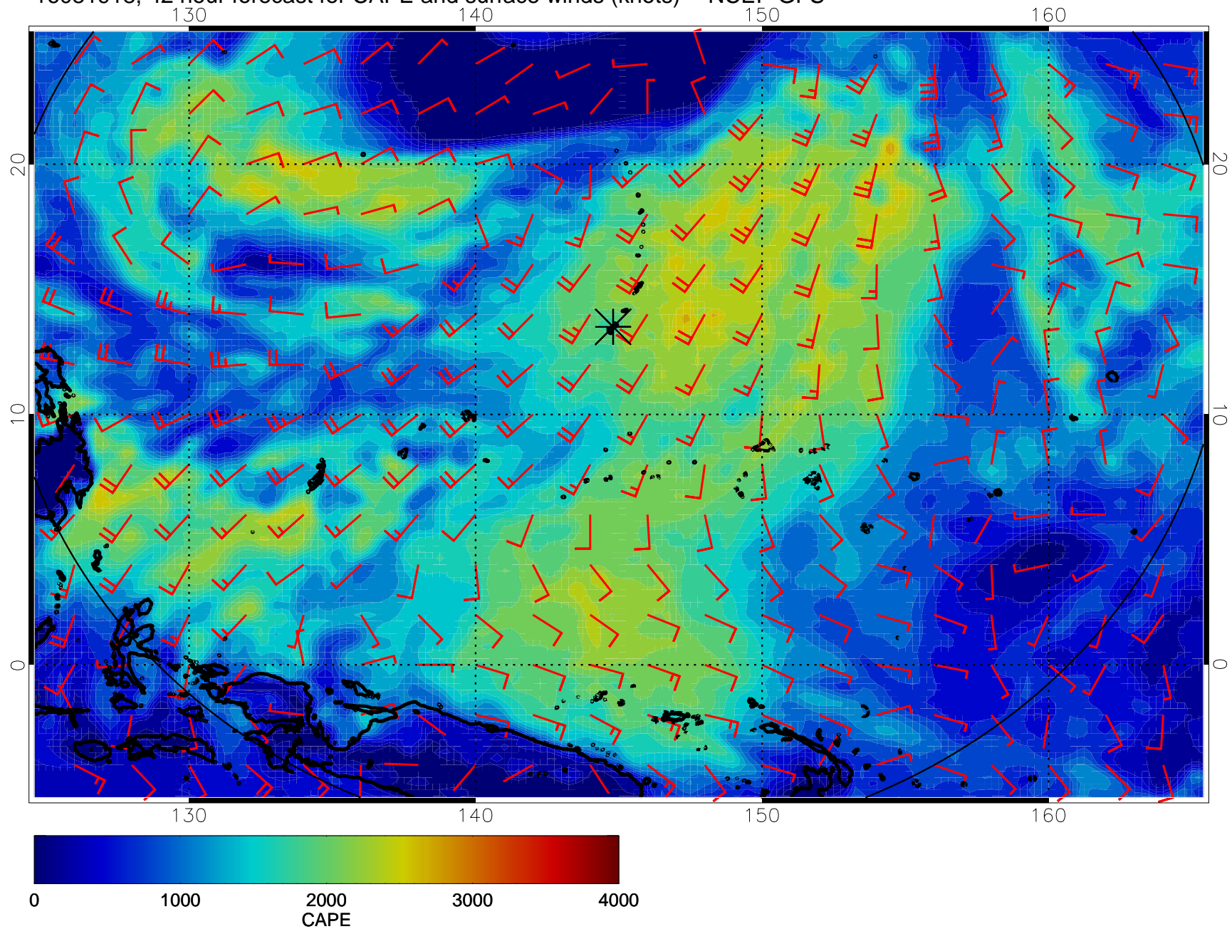
16081918, 42 hour forecast for CAPE and surface winds (knots) -- NCEP GFS
