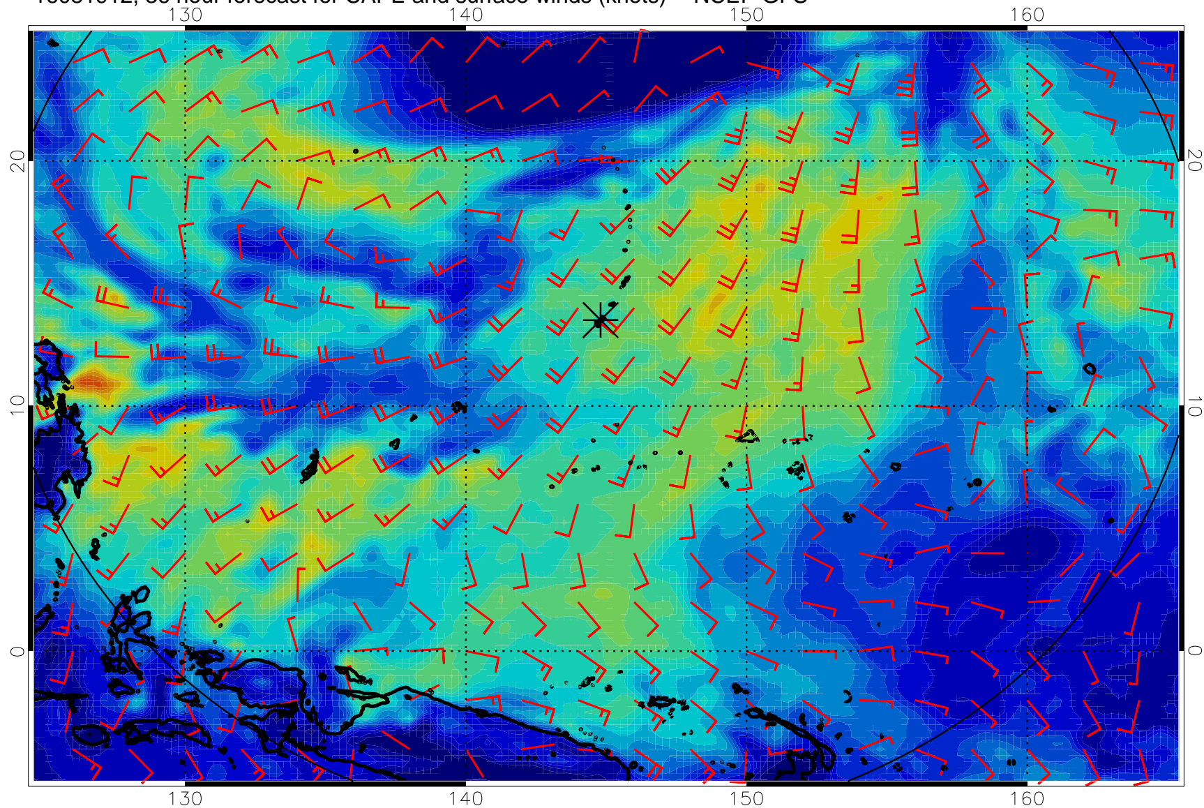
16081912, 36 hour forecast for CAPE and surface winds (knots) -- NCEP GFS
