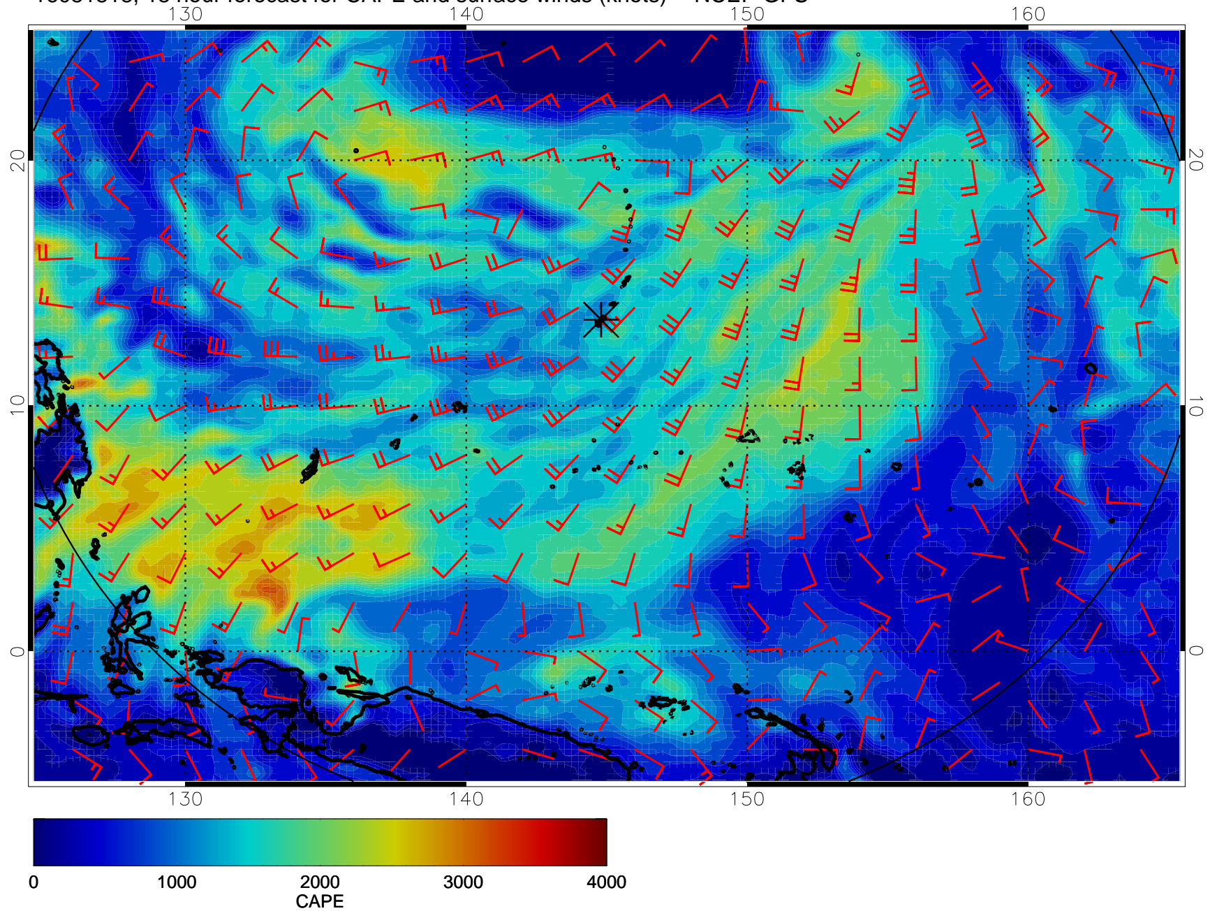
16081818, 18 hour forecast for CAPE and surface winds (knots) -- NCEP GFS
