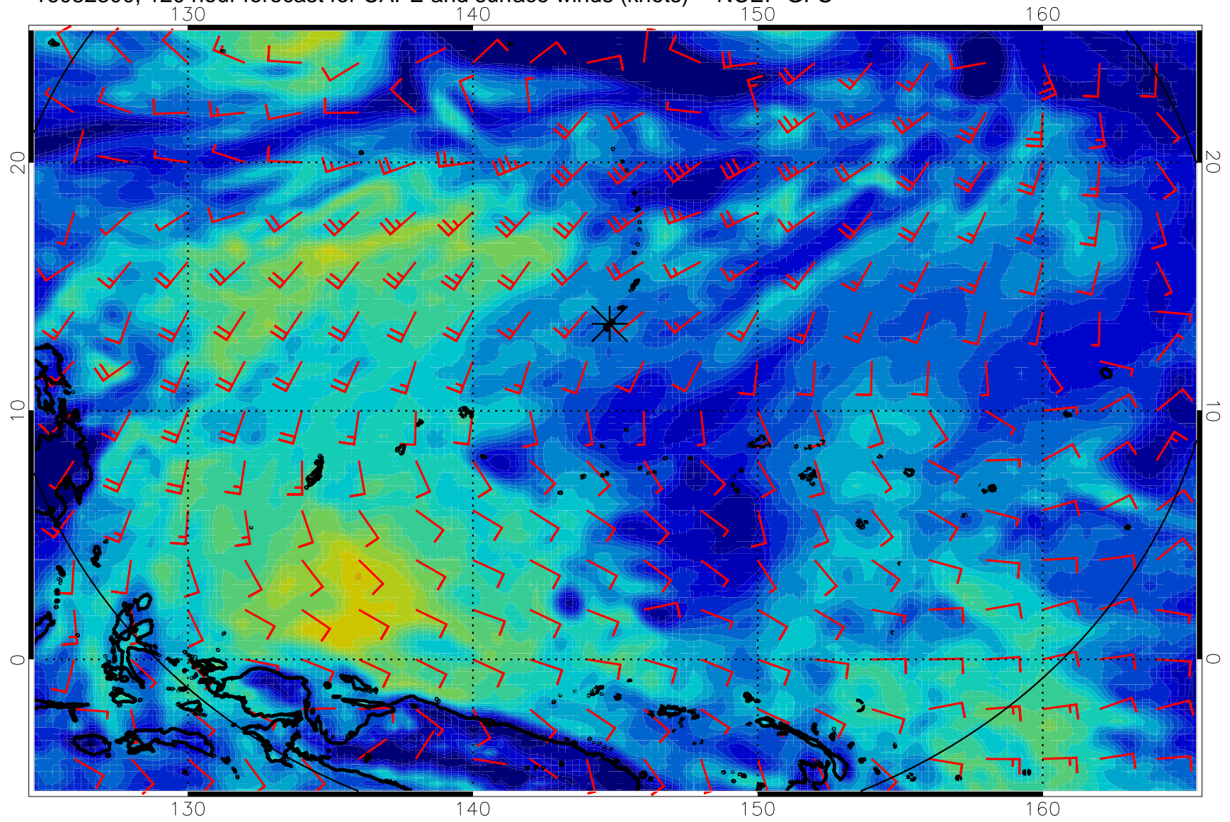
16082300, 120 hour forecast for CAPE and surface winds (knots) -- NCEP GFS
