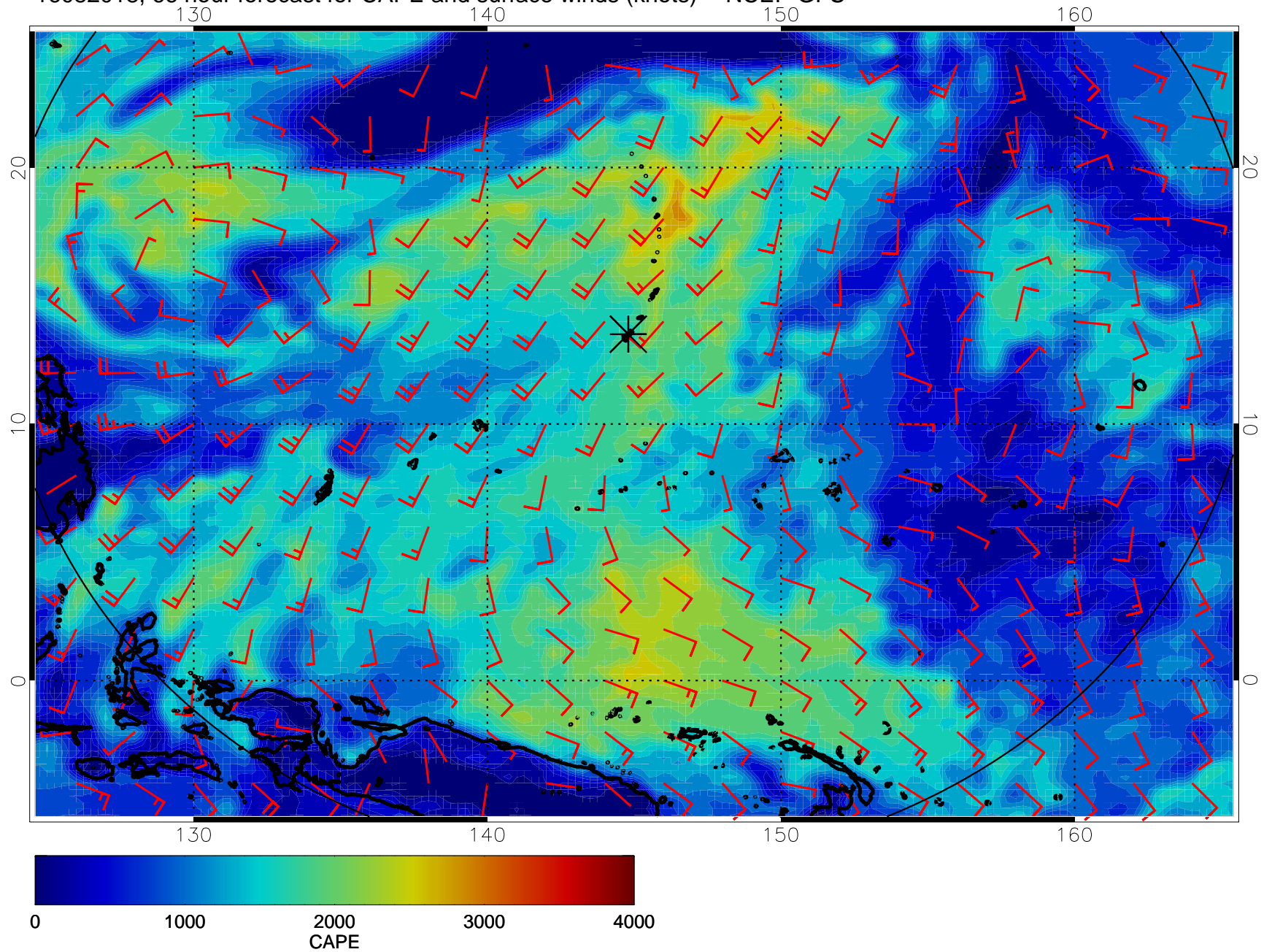
16082018, 66 hour forecast for CAPE and surface winds (knots) -- NCEP GFS
