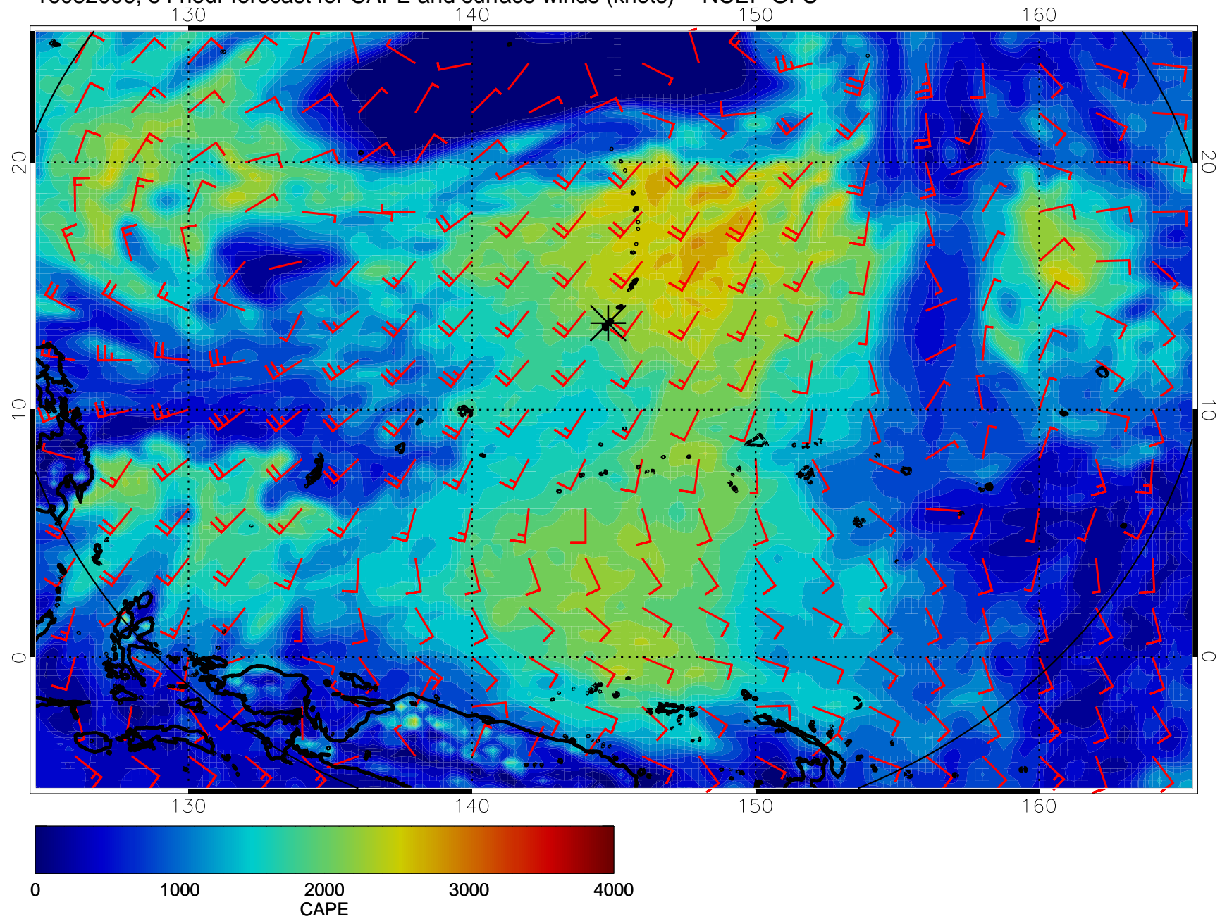
16082006, 54 hour forecast for CAPE and surface winds (knots) -- NCEP GFS
