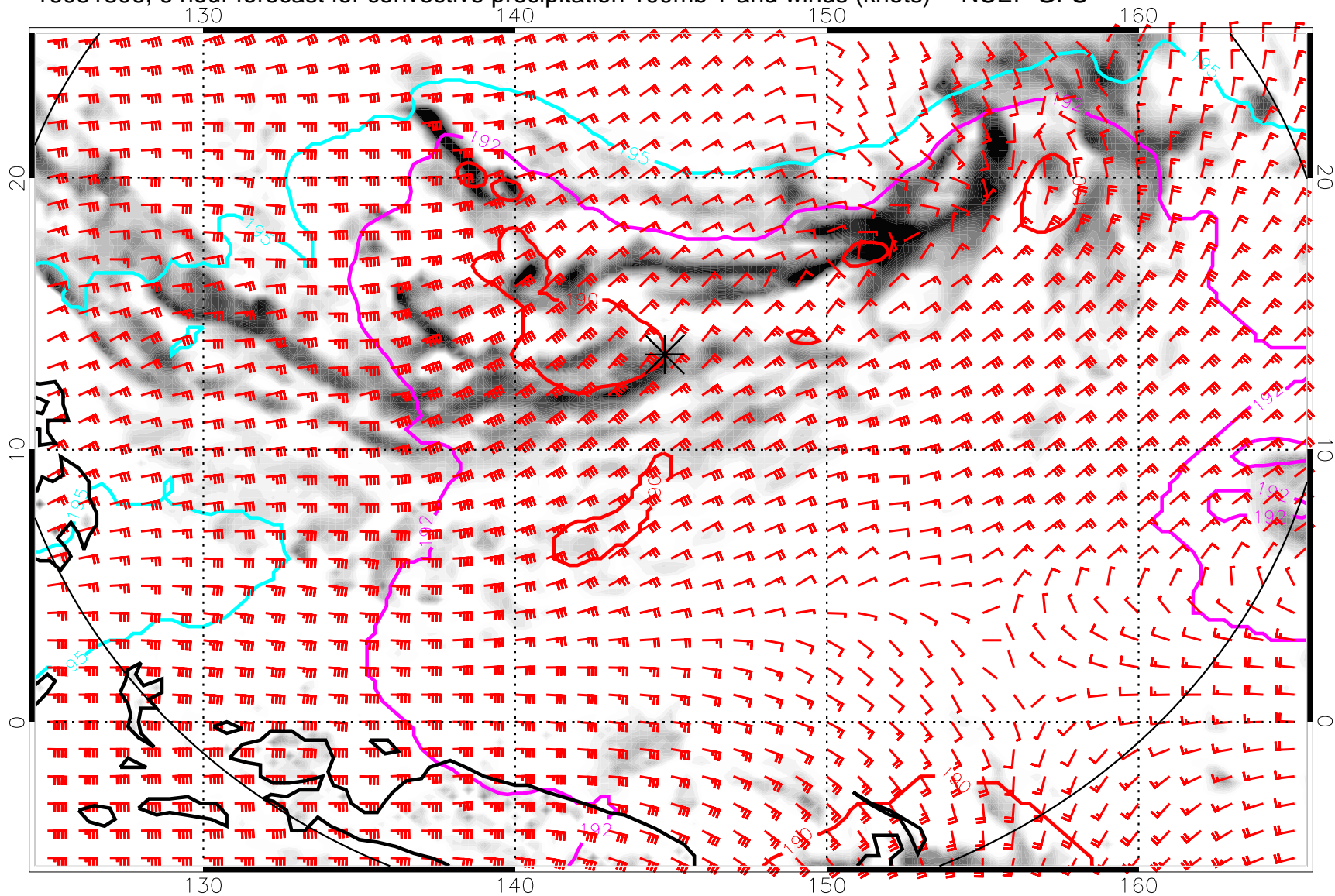
16081806, 6 hour forecast for convective precipitation 100mb T and winds (knots) -- NCEP GFS
