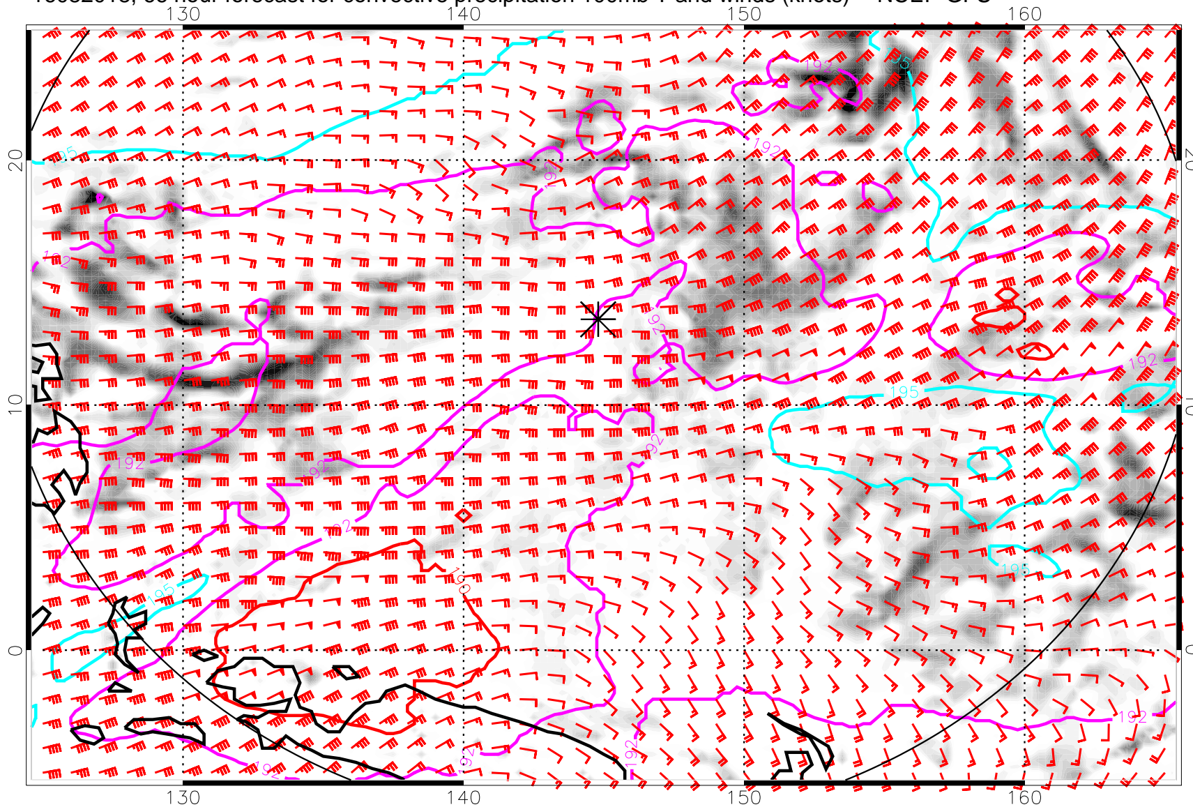
16082018, 66 hour forecast for convective precipitation 100mb T and winds (knots) -- NCEP GFS
