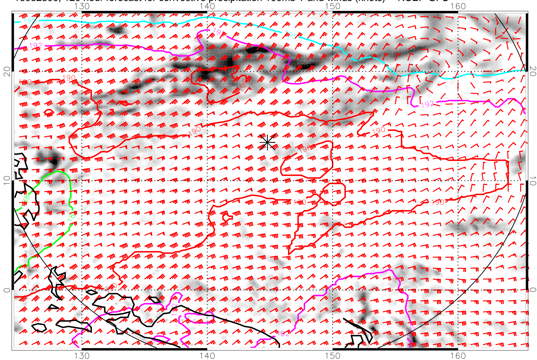
16082300, 120 hour forecast for convective precipitation 100mb T and winds (knots) -- NCEP GFS
