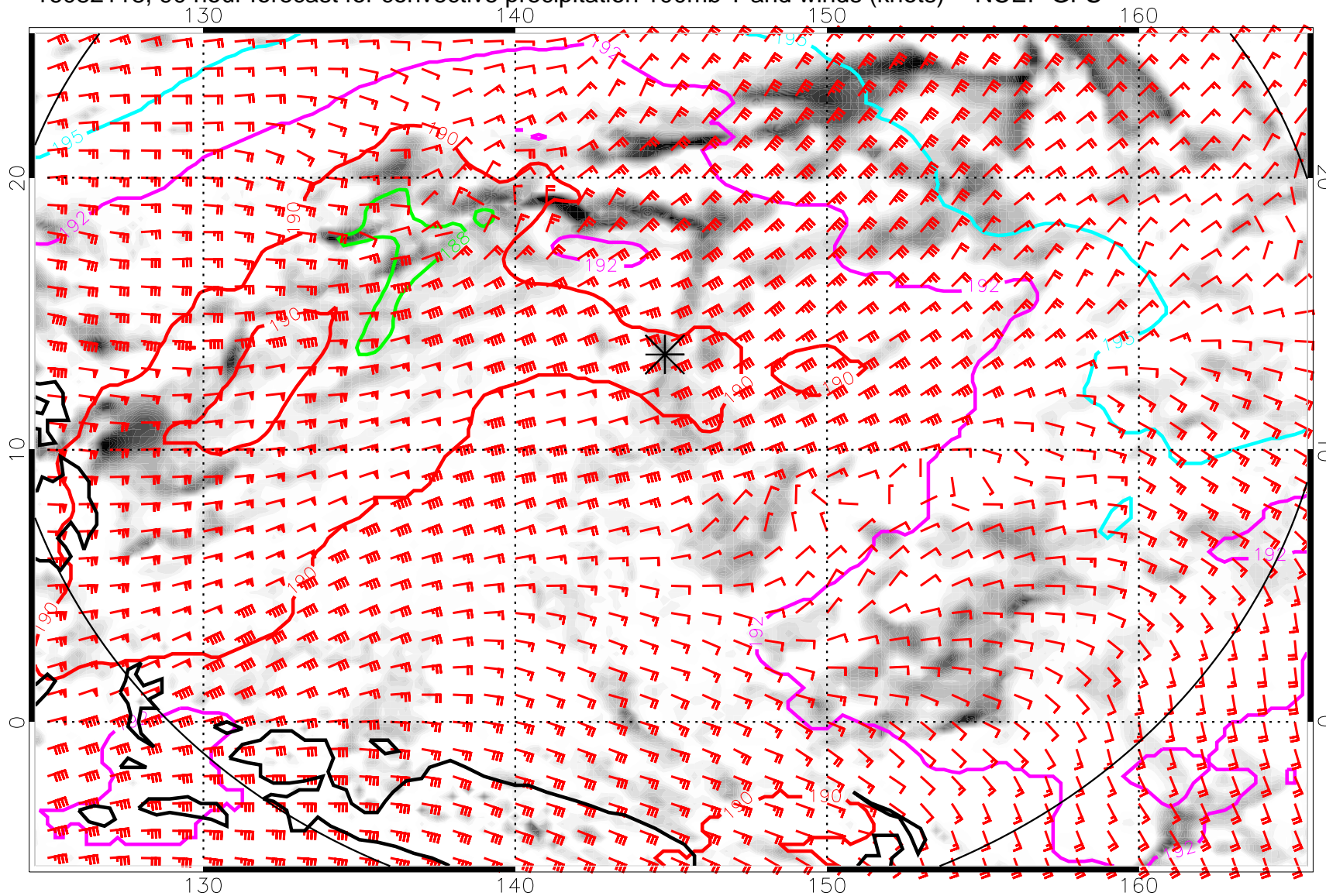
16082118, 90 hour forecast for convective precipitation 100mb T and winds (knots) -- NCEP GFS
