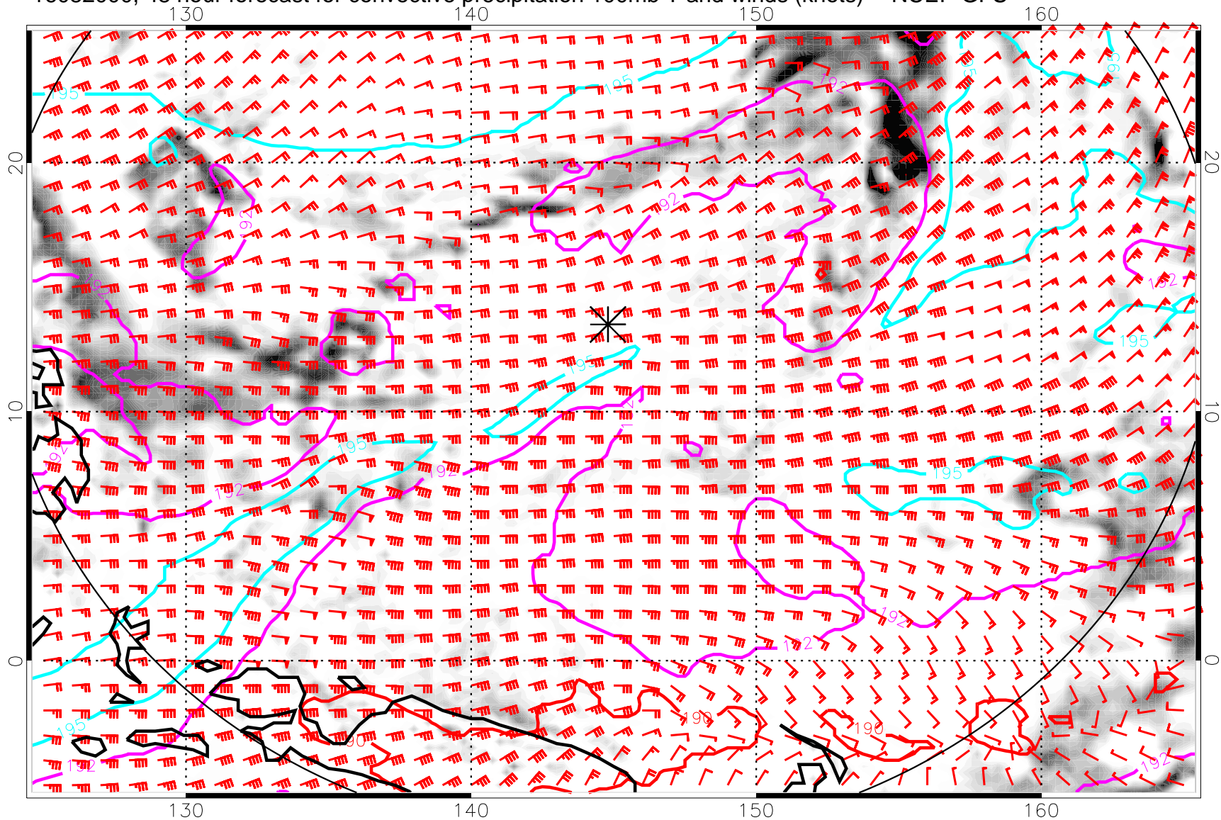
16082000, 48 hour forecast for convective precipitation 100mb T and winds (knots) -- NCEP GFS
