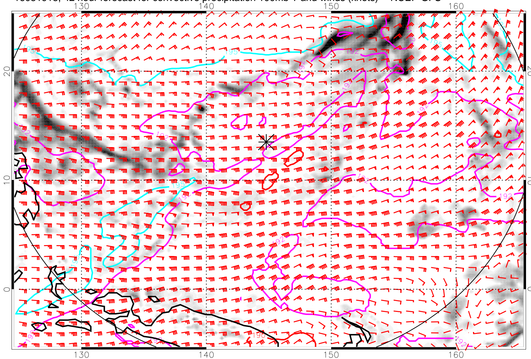
16081918, 42 hour forecast for convective precipitation 100mb T and winds (knots) -- NCEP GFS
