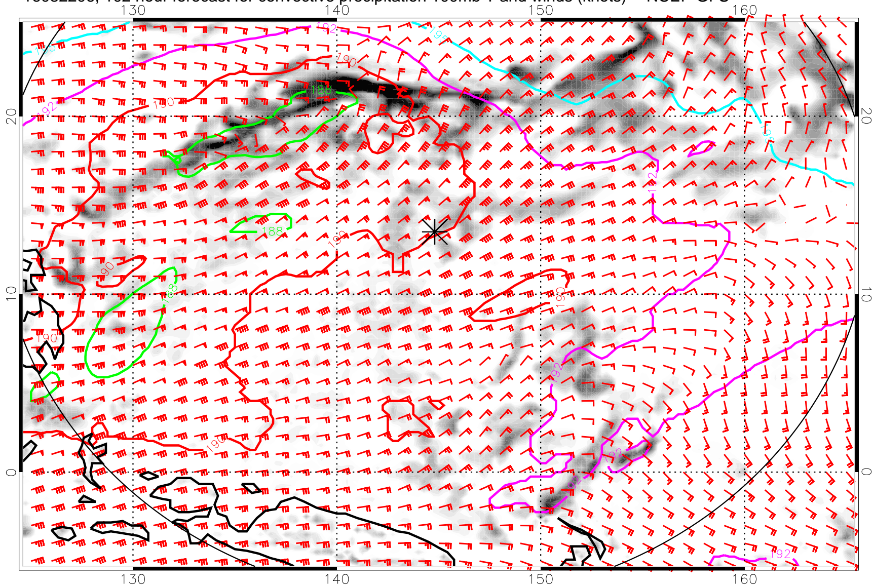
16082206, 102 hour forecast for convective precipitation 100mb T and winds (knots) -- NCEP GFS
