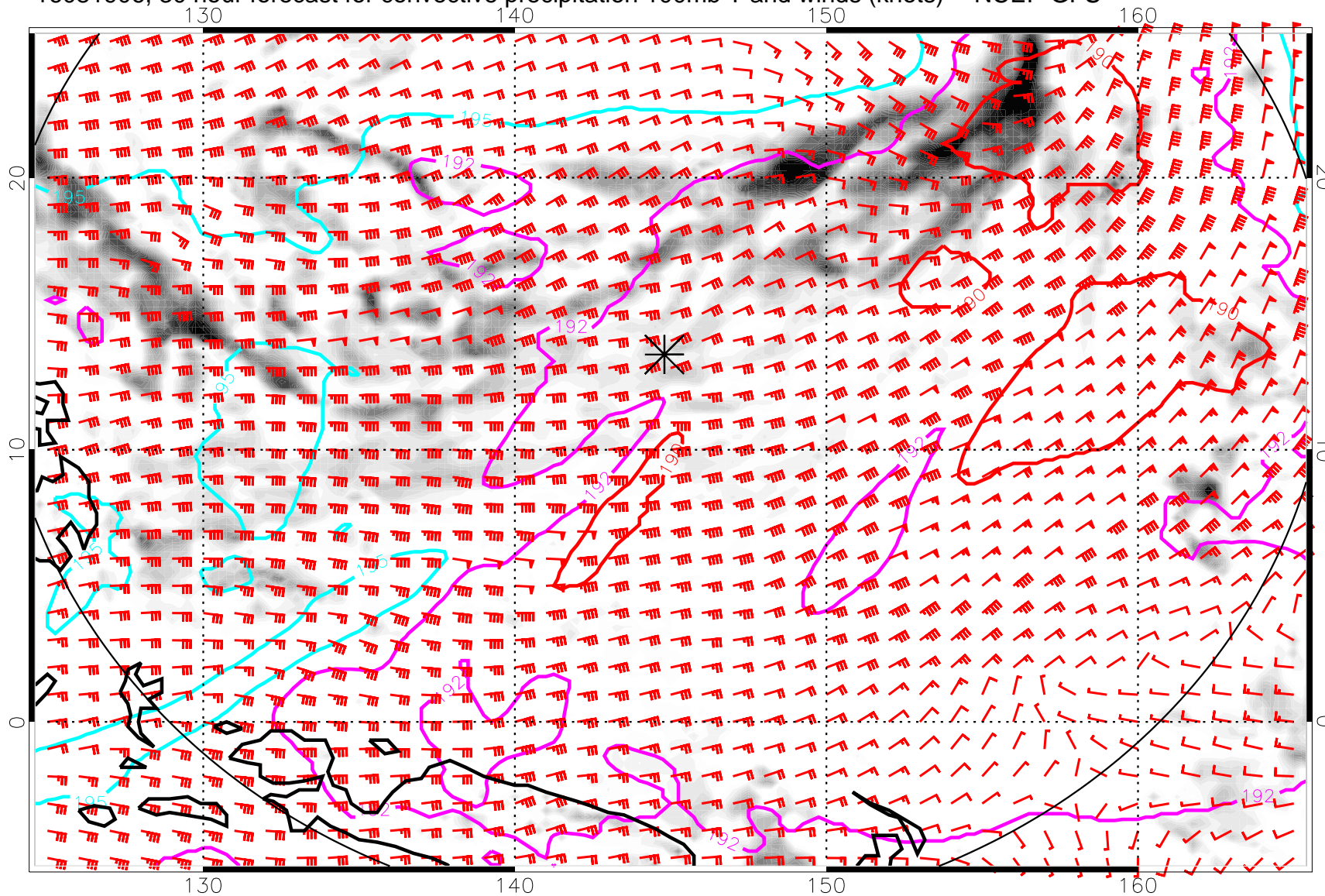
16081906, 30 hour forecast for convective precipitation 100mb T and winds (knots) -- NCEP GFS
