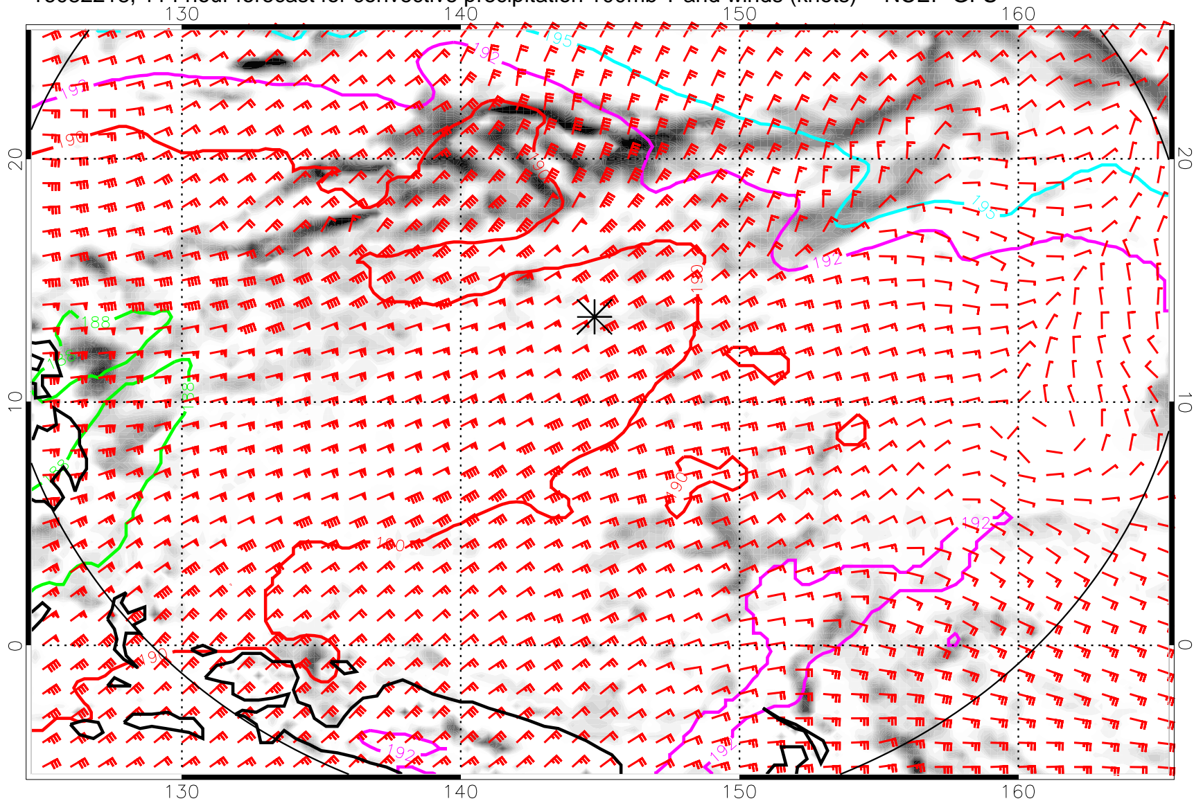
16082218, 114 hour forecast for convective precipitation 100mb T and winds (knots) -- NCEP GFS
