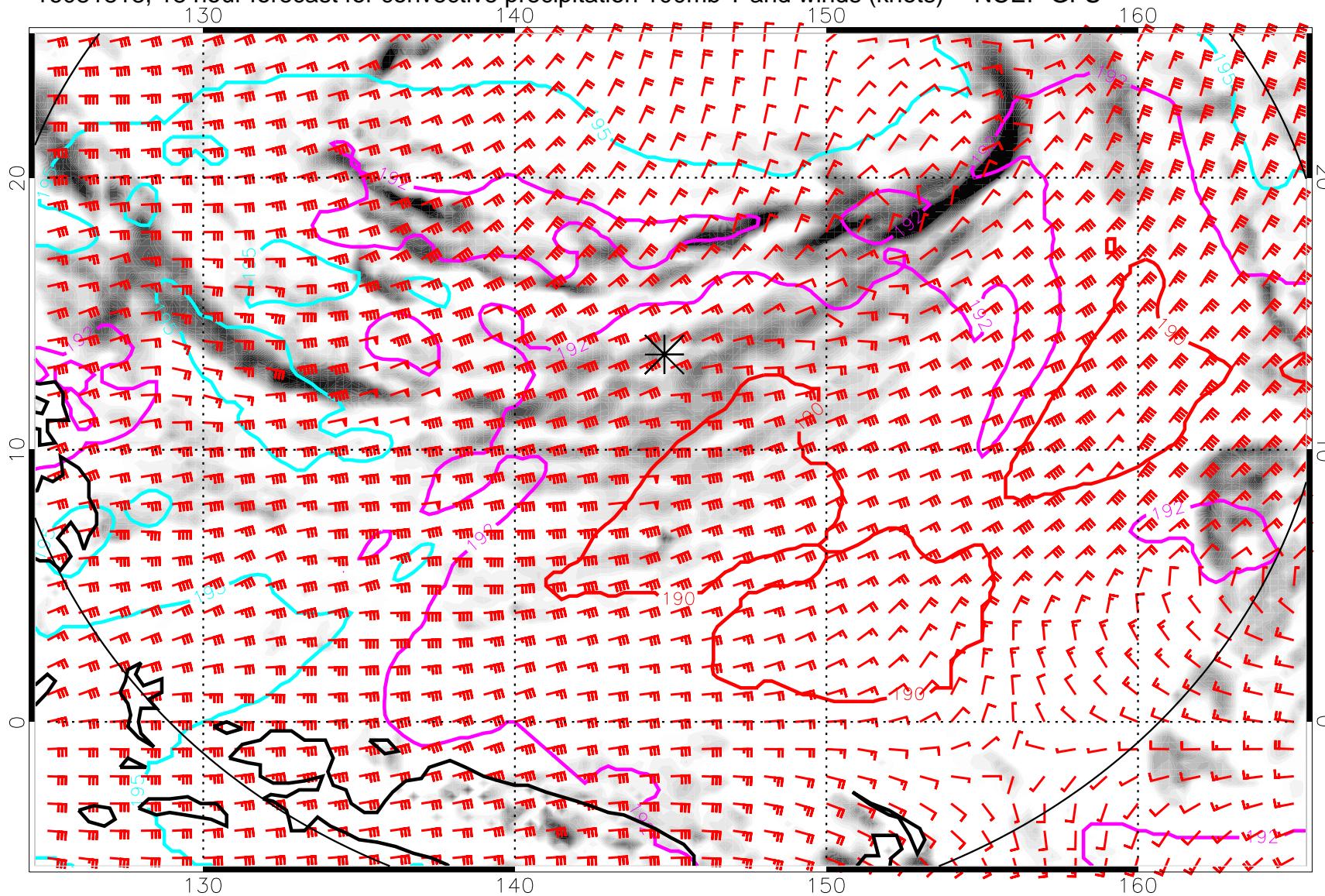
16081818, 18 hour forecast for convective precipitation 100mb T and winds (knots) -- NCEP GFS
