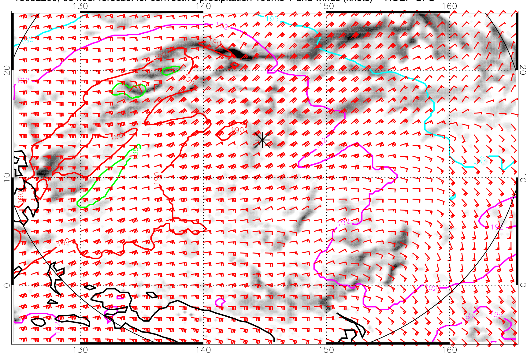
16082200, 96 hour forecast for convective precipitation 100mb T and winds (knots) -- NCEP GFS
