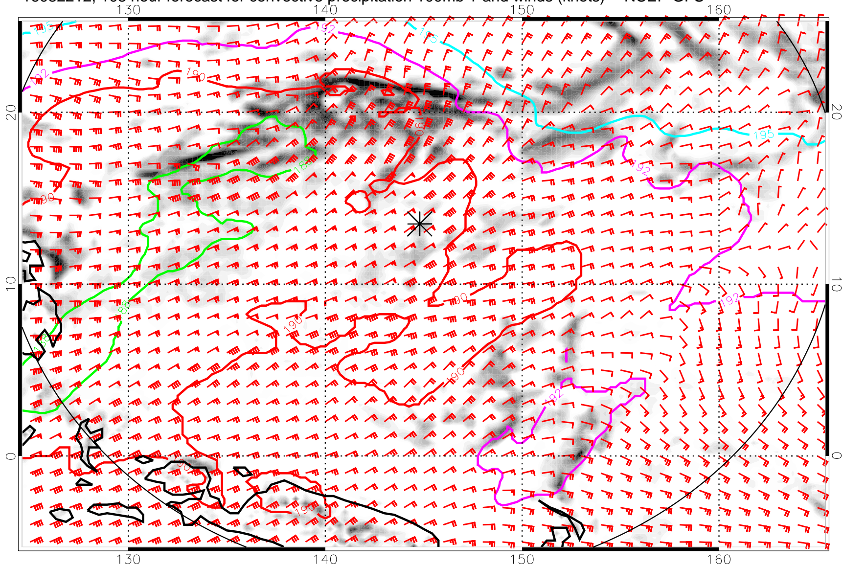
16082212, 108 hour forecast for convective precipitation 100mb T and winds (knots) -- NCEP GFS
