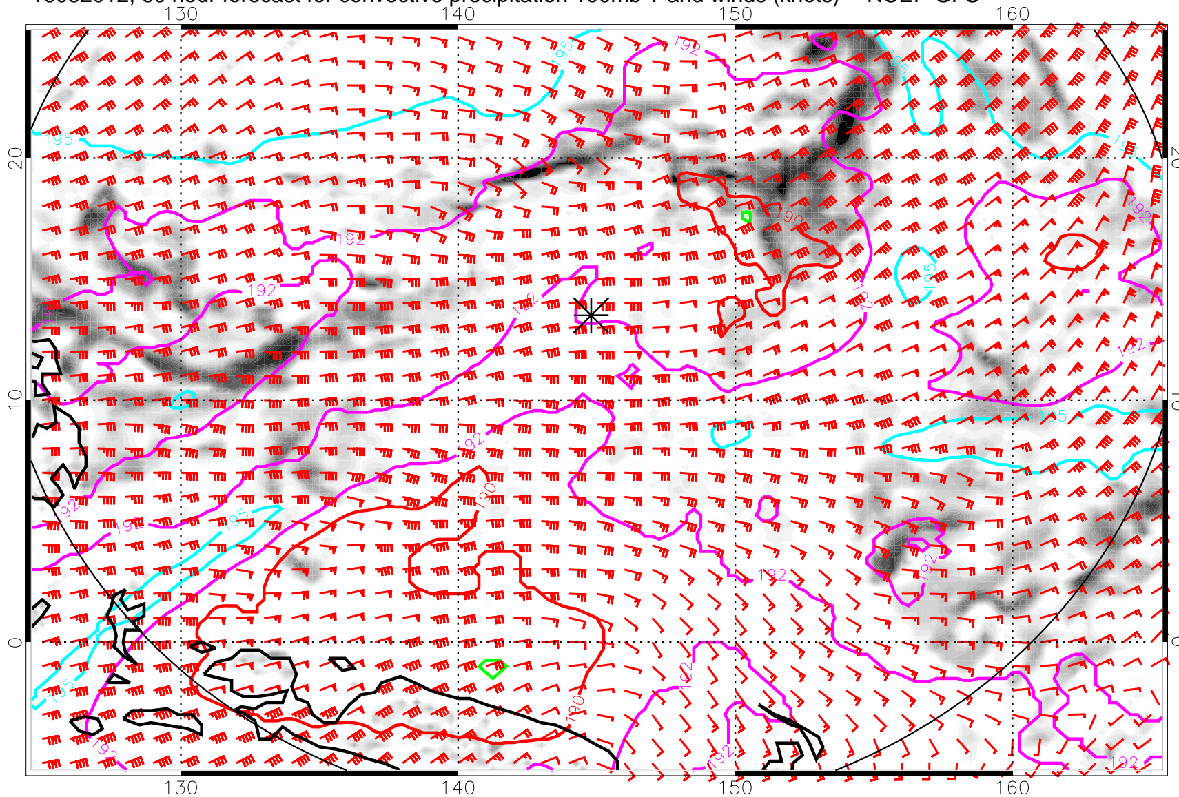
16082012, 60 hour forecast for convective precipitation 100mb T and winds (knots) -- NCEP GFS
