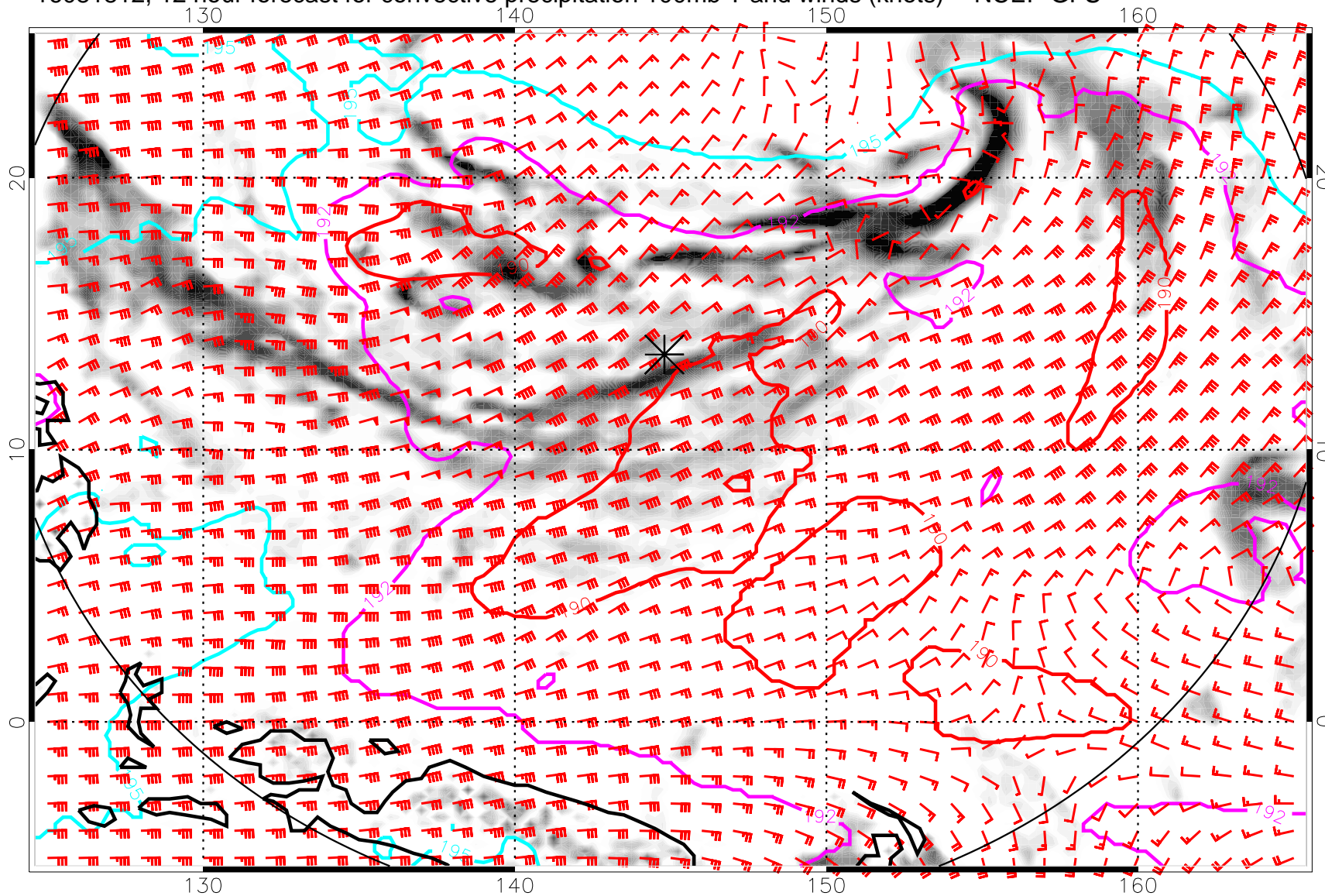
16081812, 12 hour forecast for convective precipitation 100mb T and winds (knots) -- NCEP GFS
