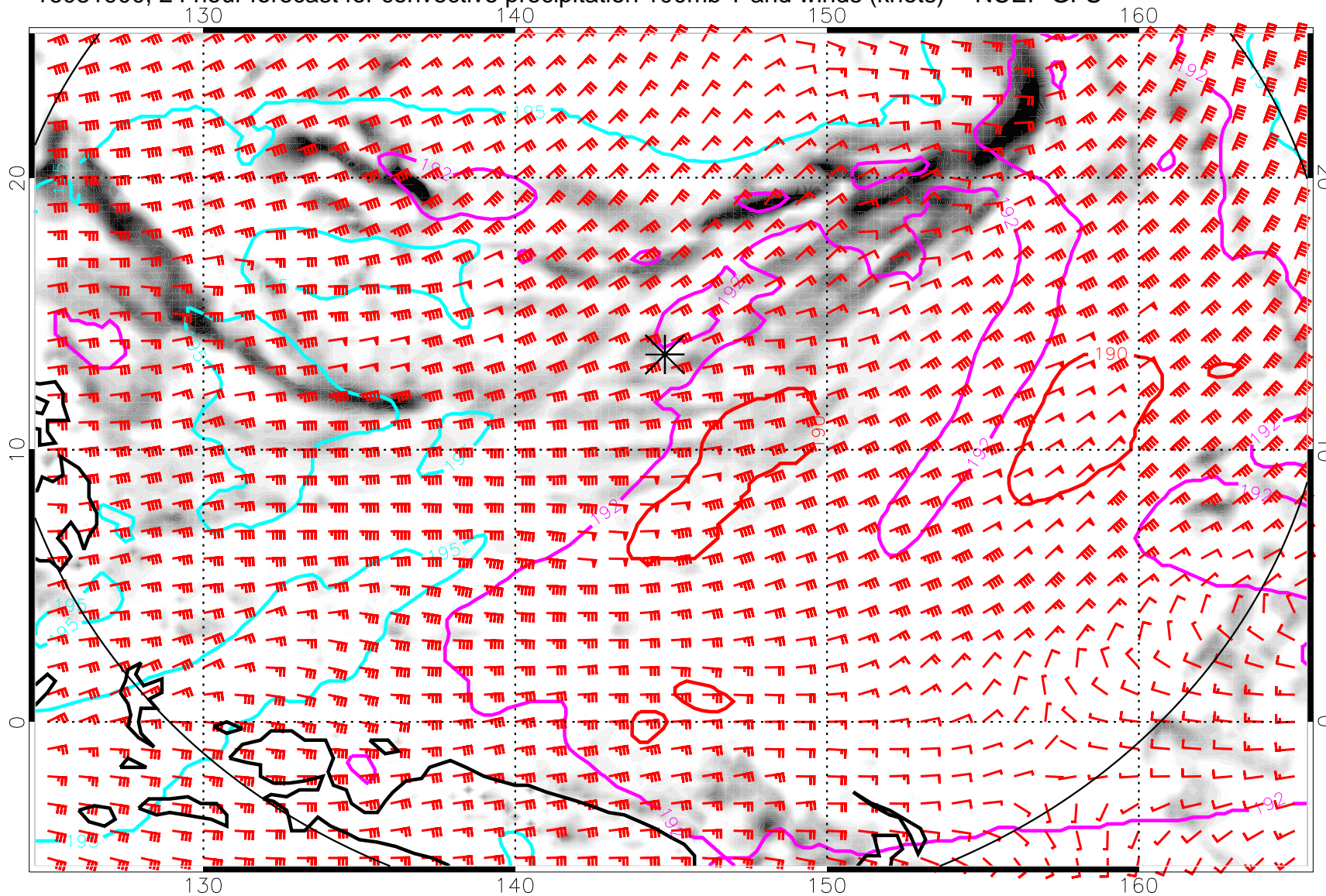
16081900, 24 hour forecast for convective precipitation 100mb T and winds (knots) -- NCEP GFS
