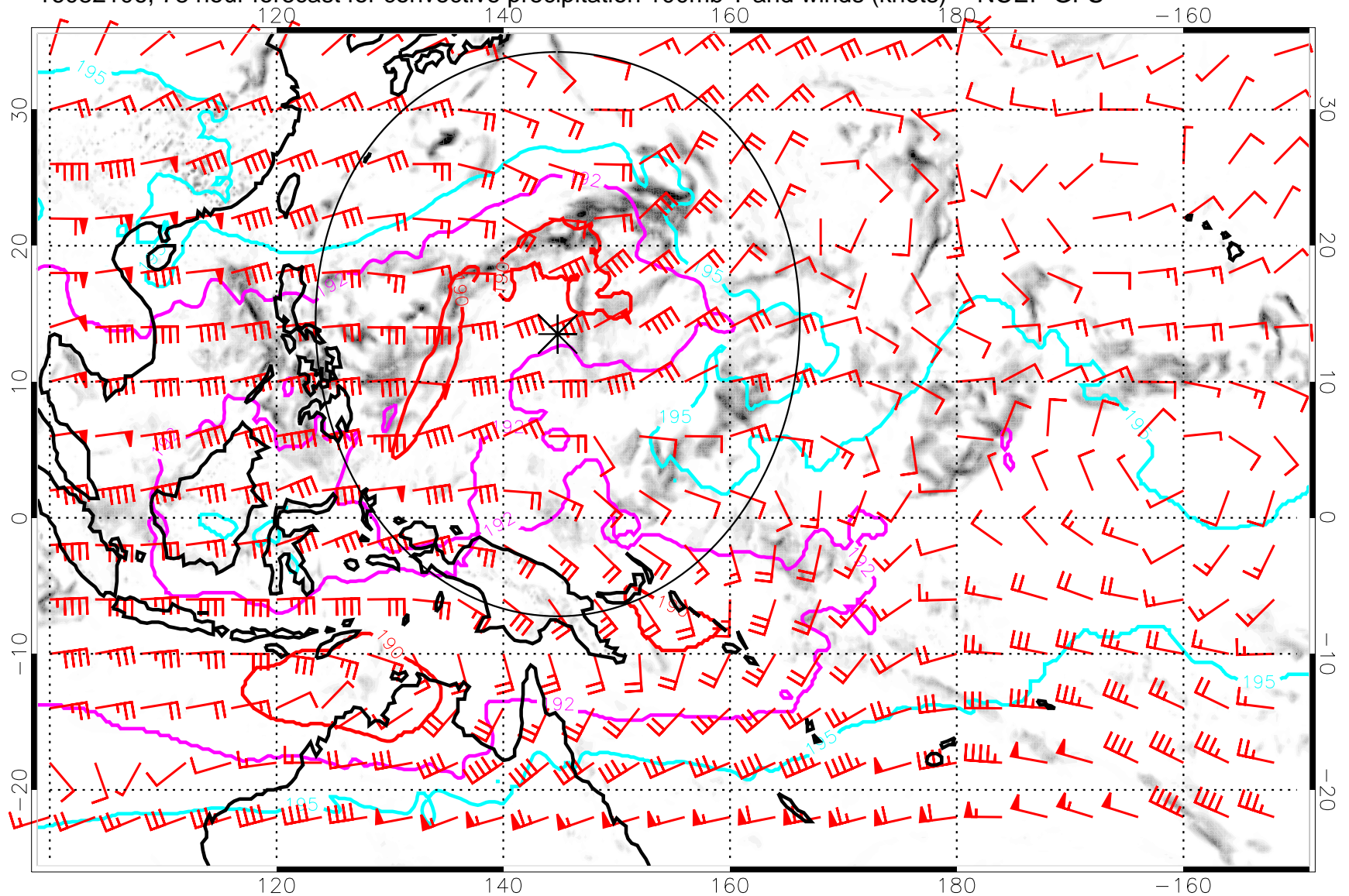
16082106, 78 hour forecast for convective precipitation 100mb T and winds (knots) -- NCEP GFS
