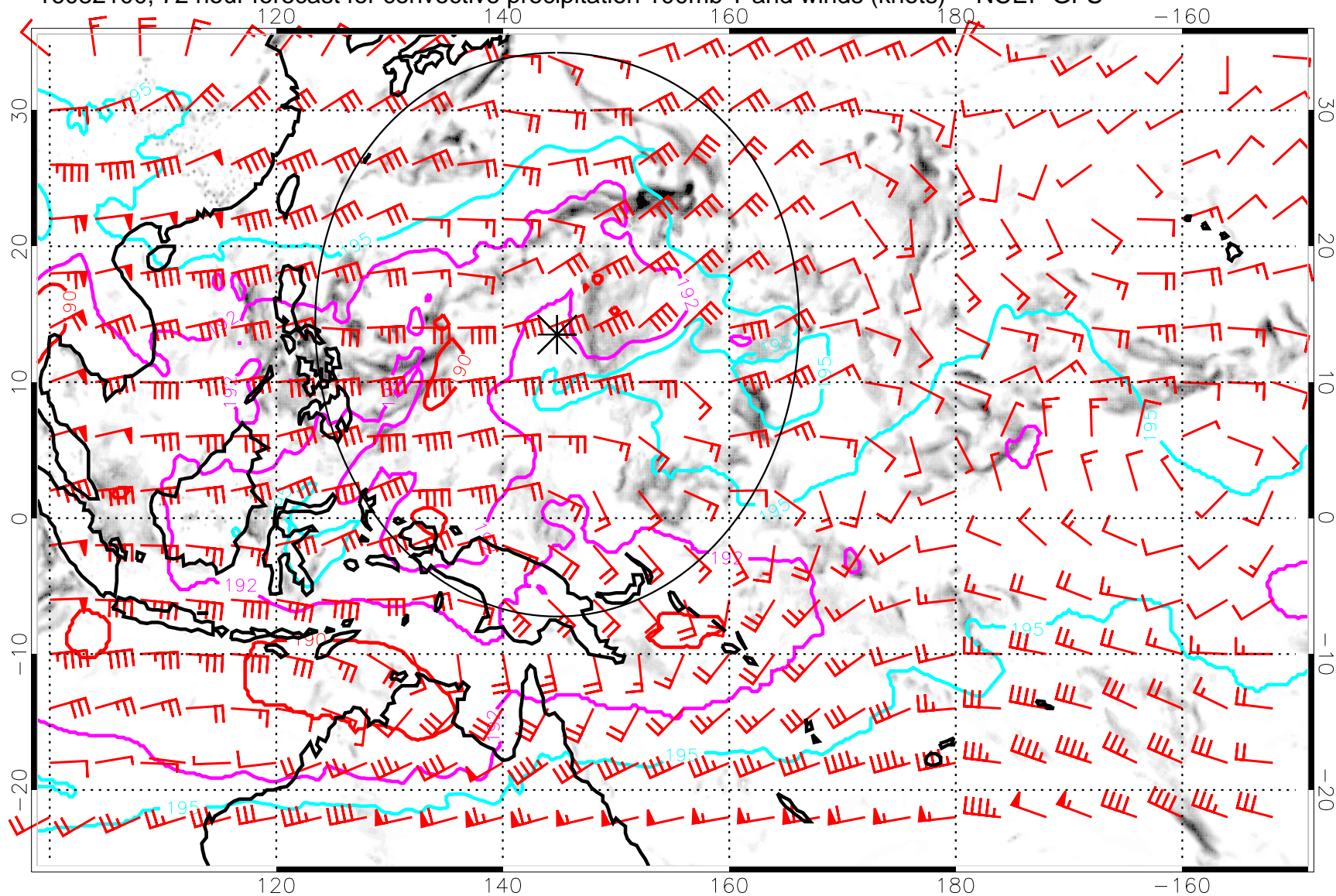
16082100, 72 hour forecast for convective precipitation 100mb T and winds (knots) -- NCEP GFS
