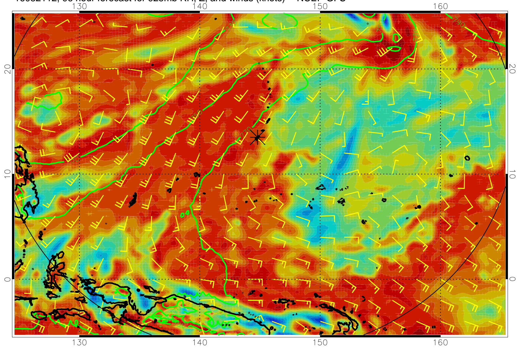
16082112, 96 hour forecast for 925mb RH, Z, and winds (knots) -- NCEP GFS
