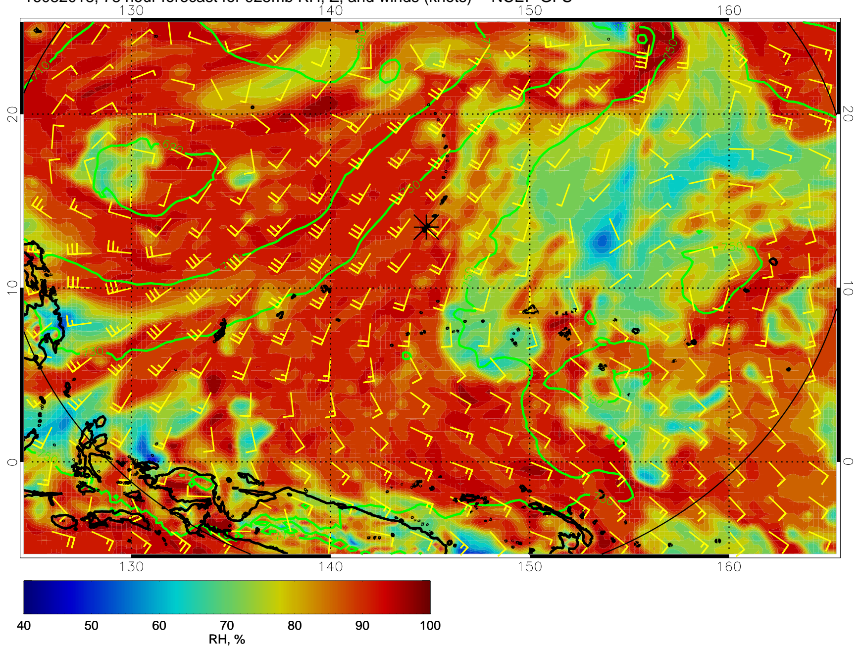
16082018, 78 hour forecast for 925mb RH, Z, and winds (knots) -- NCEP GFS
