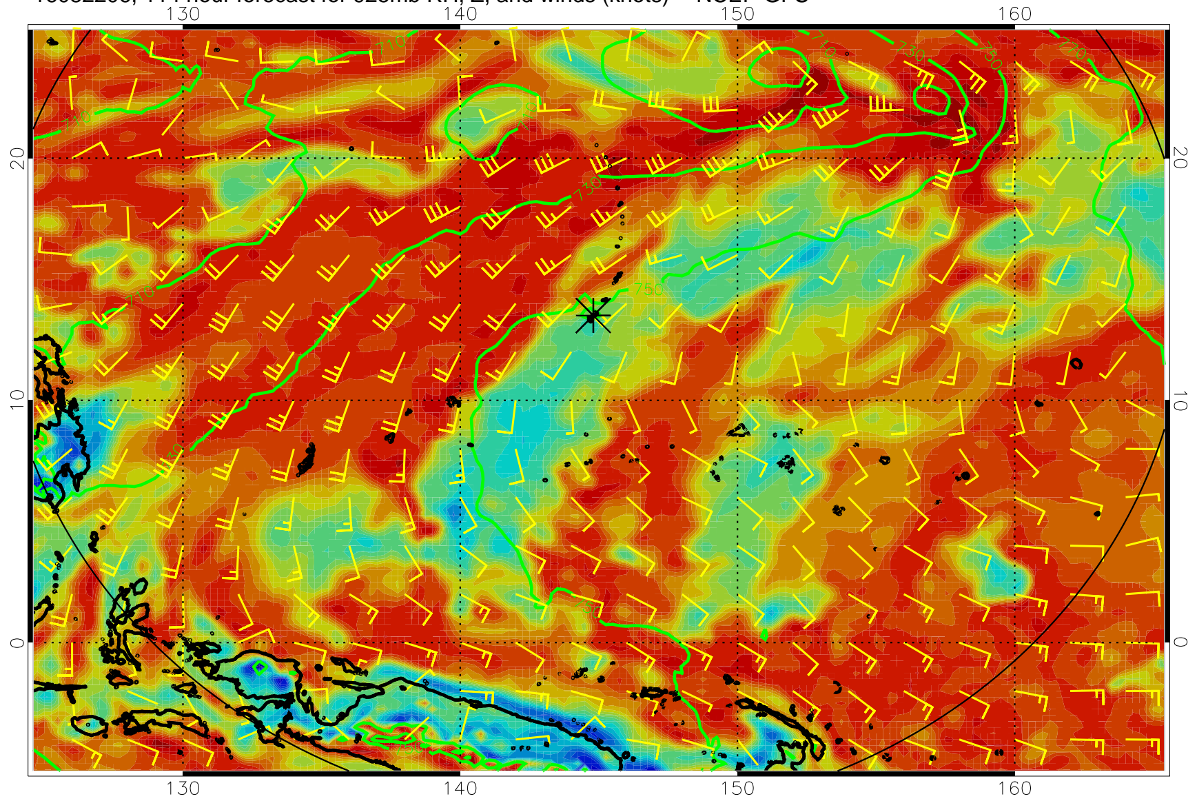
16082206, 114 hour forecast for 925mb RH, Z, and winds (knots) -- NCEP GFS
