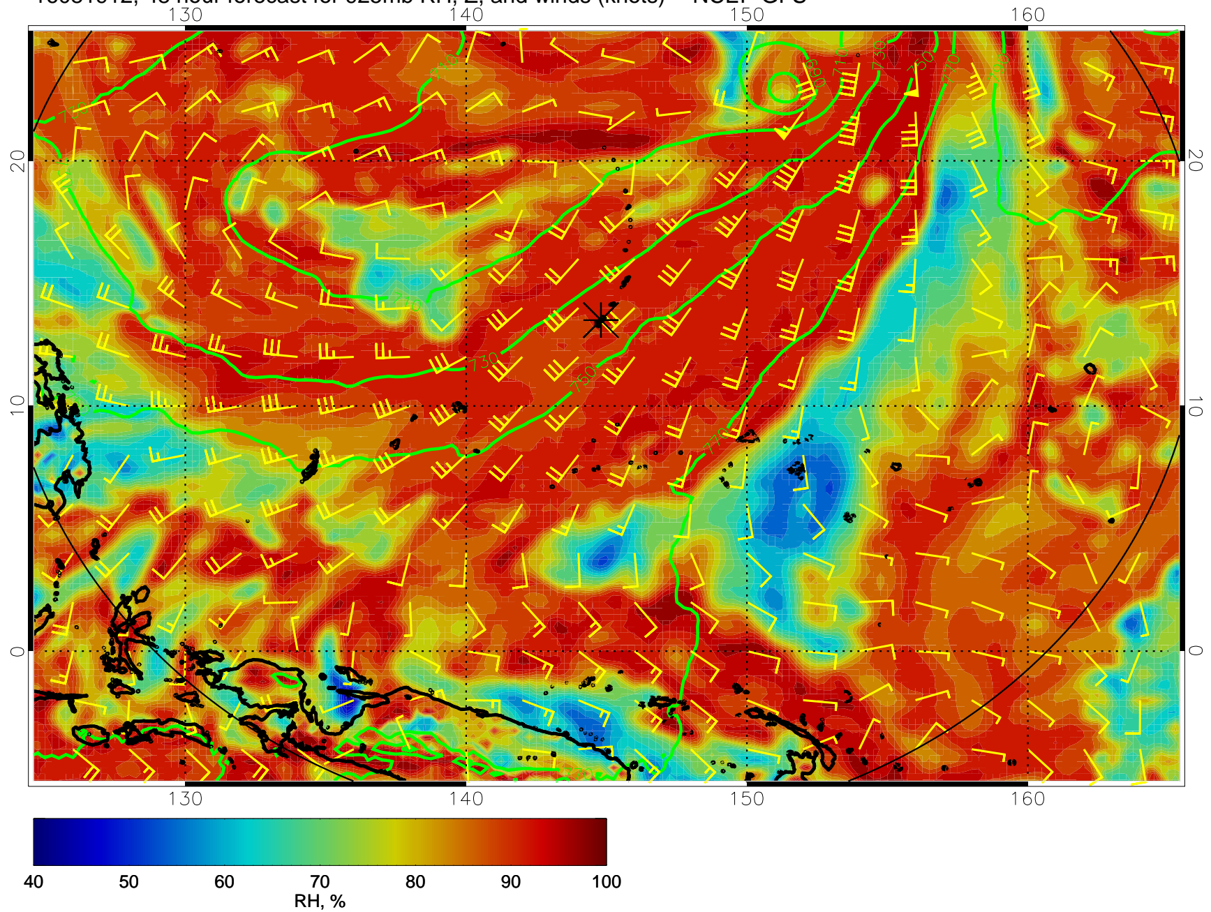
16081912, 48 hour forecast for 925mb RH, Z, and winds (knots) -- NCEP GFS
