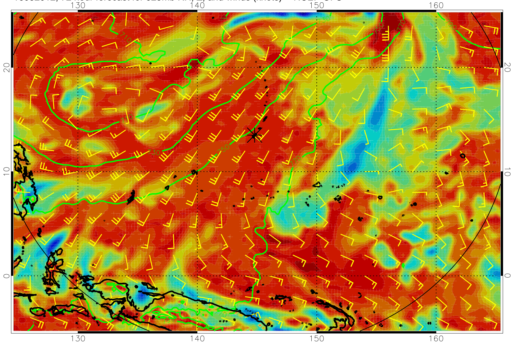
16082012, 72 hour forecast for 925mb RH, Z, and winds (knots) -- NCEP GFS
