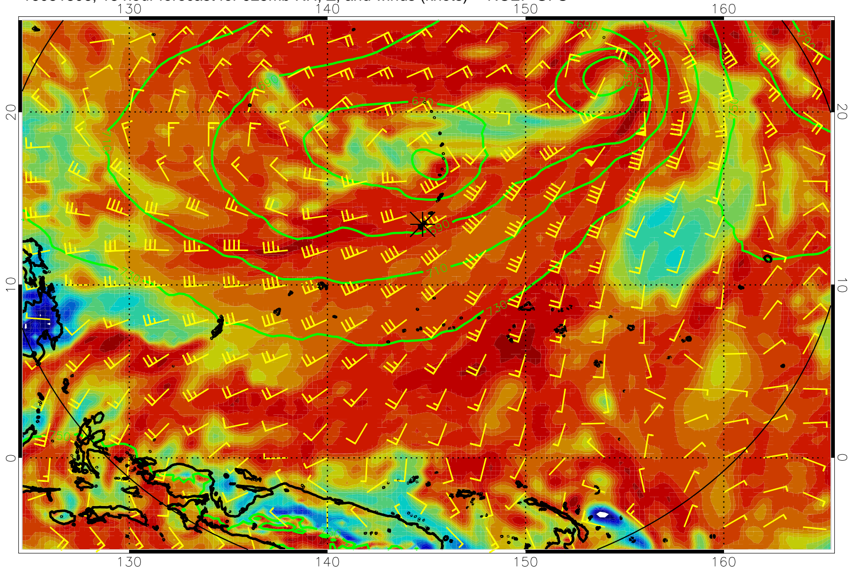
16081806, 18 hour forecast for 925mb RH, Z, and winds (knots) -- NCEP GFS
