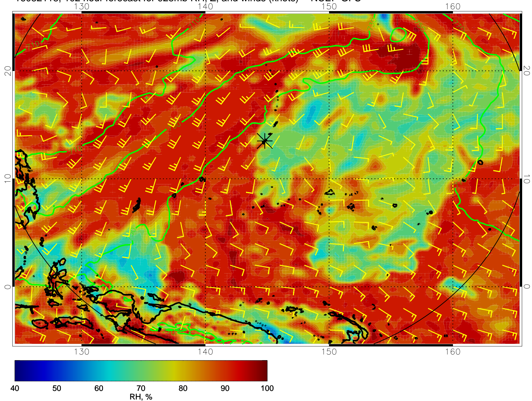
16082118, 102 hour forecast for 925mb RH, Z, and winds (knots) -- NCEP GFS
