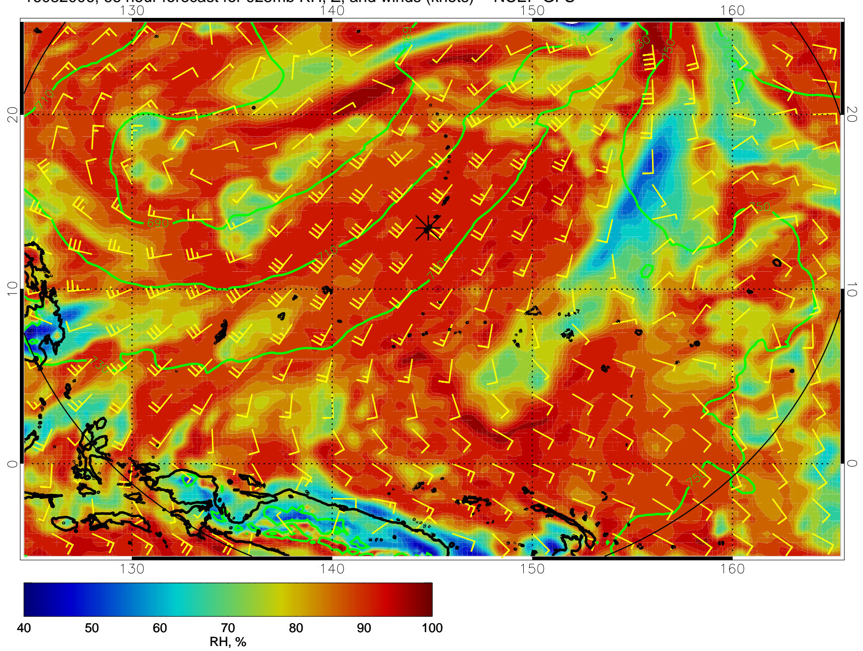
16082006, 66 hour forecast for 925mb RH, Z, and winds (knots) -- NCEP GFS
