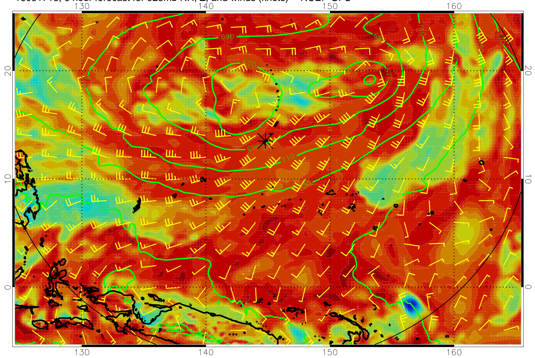
16081718, 6 hour forecast for 925mb RH, Z, and winds (knots) -- NCEP GFS
