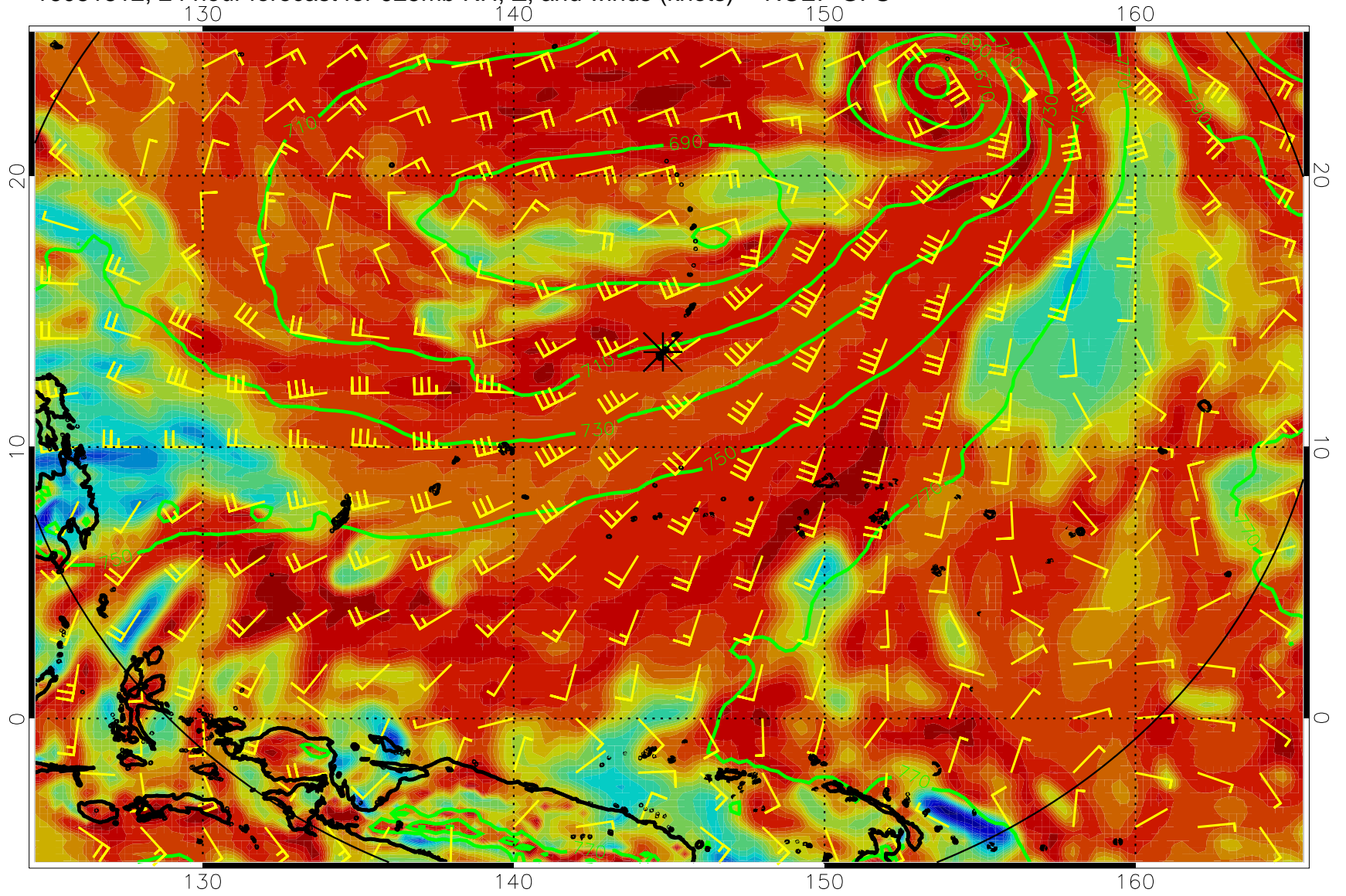
16081812, 24 hour forecast for 925mb RH, Z, and winds (knots) -- NCEP GFS
