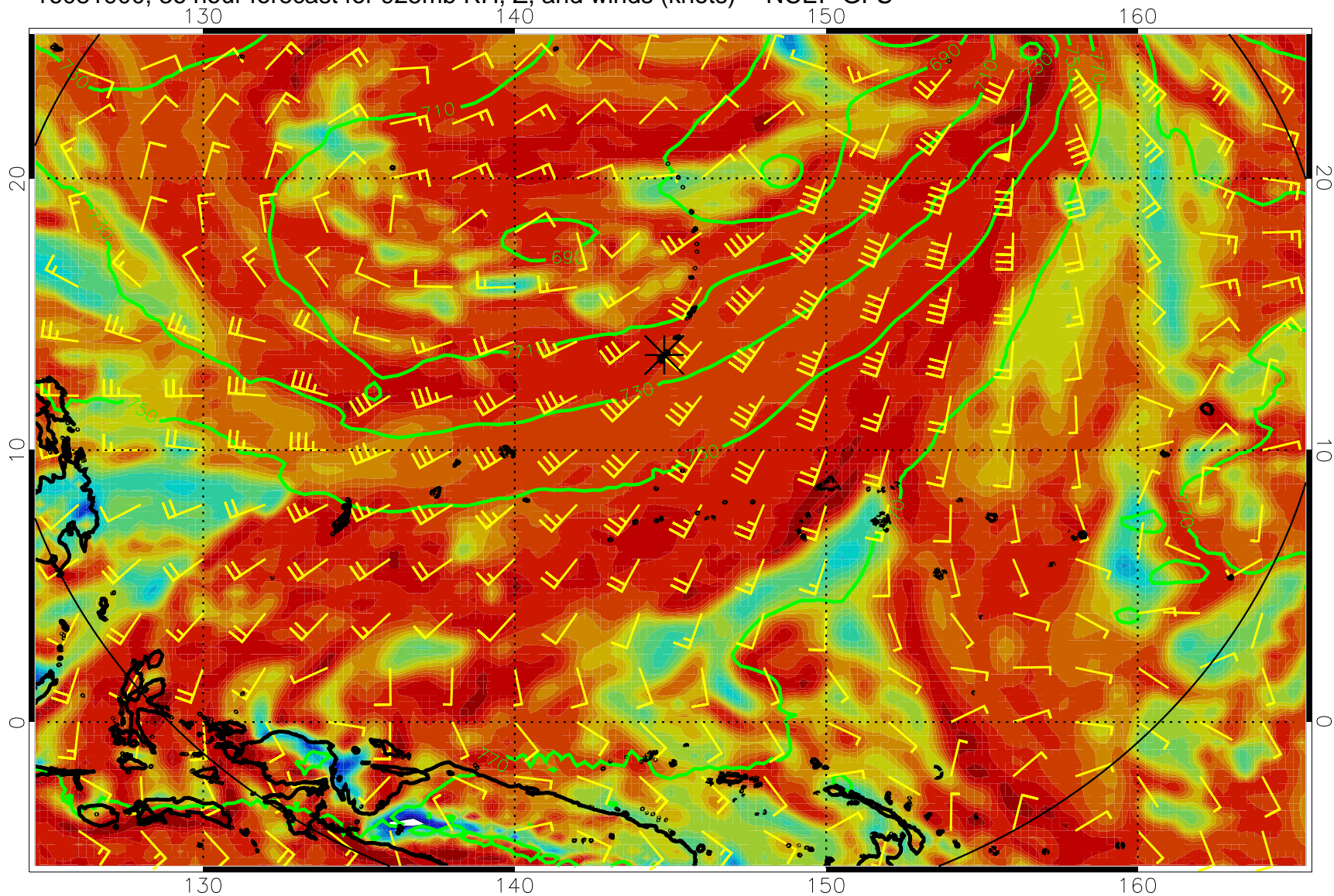
16081900, 36 hour forecast for 925mb RH, Z, and winds (knots) -- NCEP GFS
