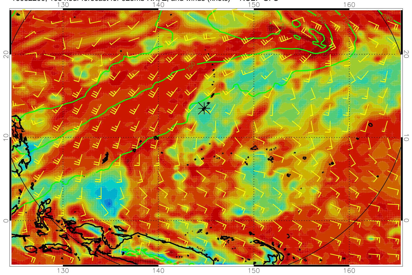
16082200, 108 hour forecast for 925mb RH, Z, and winds (knots) -- NCEP GFS
