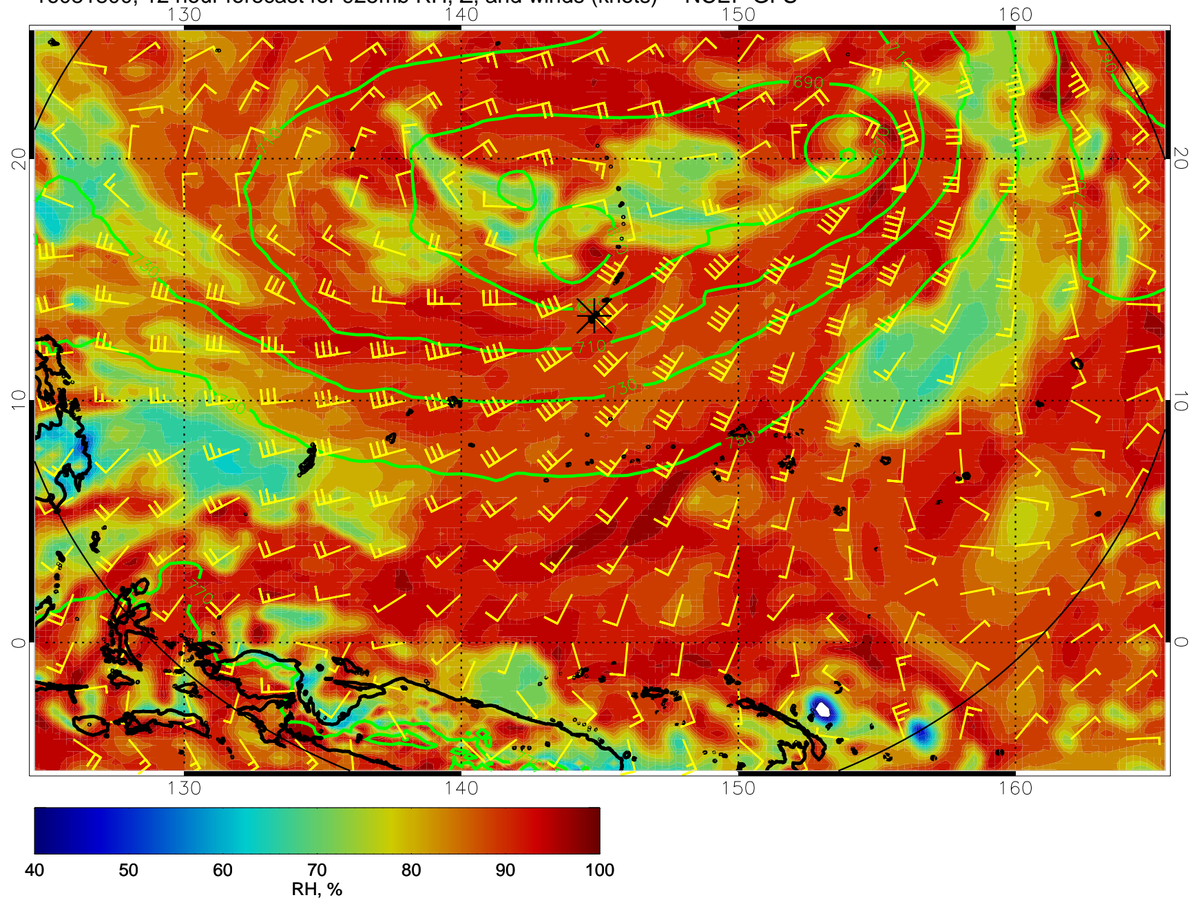
16081800, 12 hour forecast for 925mb RH, Z, and winds (knots) -- NCEP GFS
