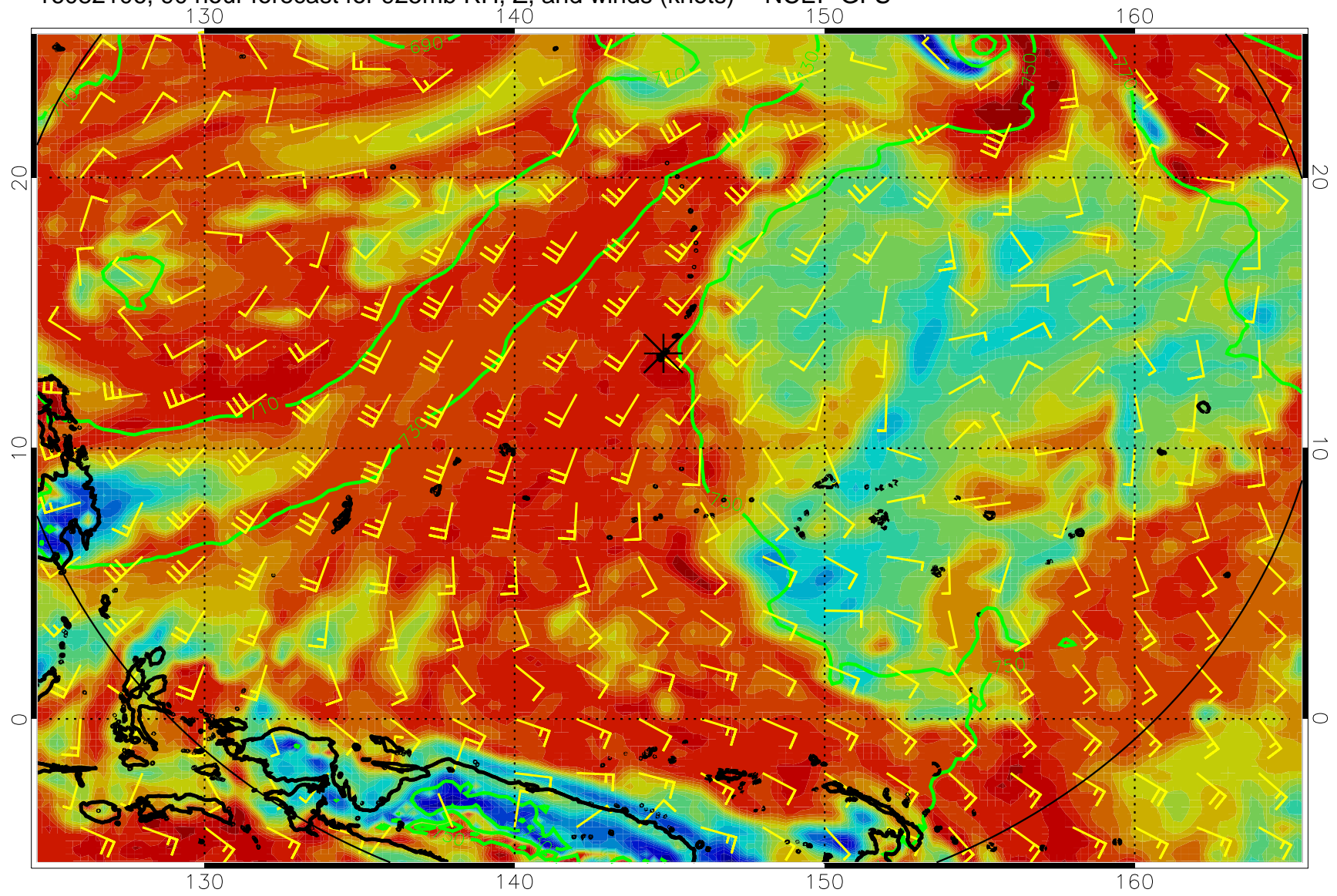
16082106, 90 hour forecast for 925mb RH, Z, and winds (knots) -- NCEP GFS
