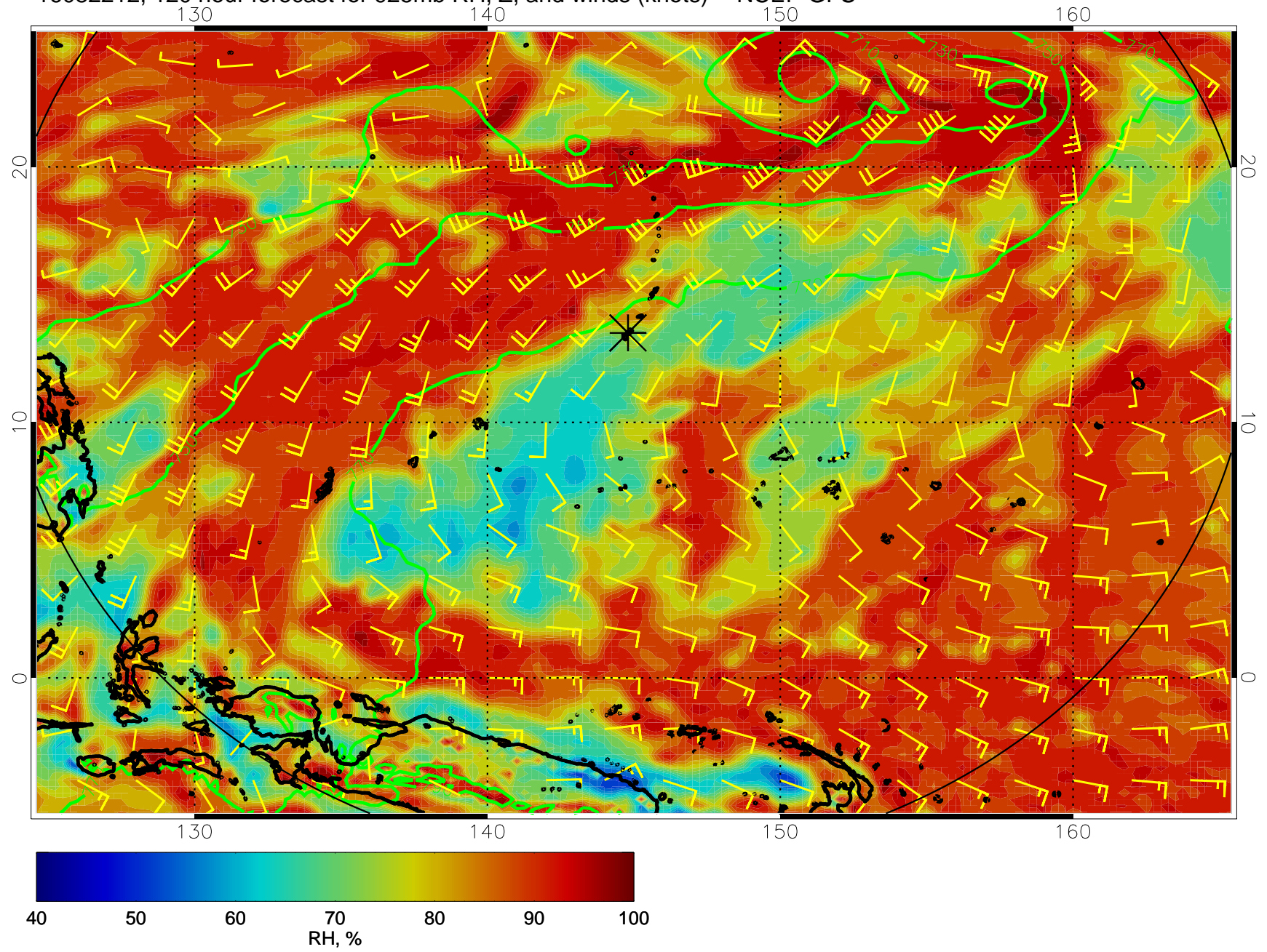
16082212, 120 hour forecast for 925mb RH, Z, and winds (knots) -- NCEP GFS
