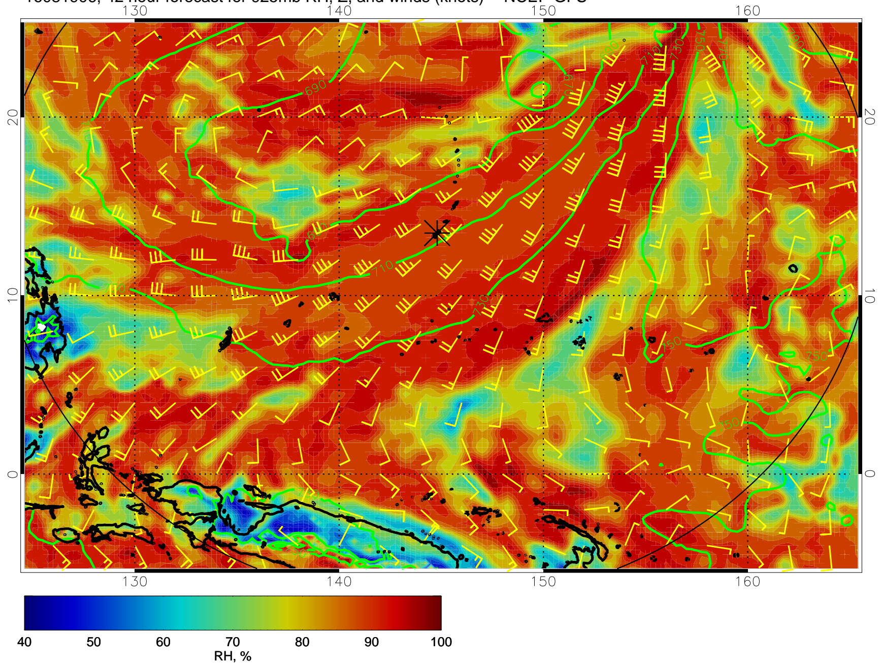
16081906, 42 hour forecast for 925mb RH, Z, and winds (knots) -- NCEP GFS
