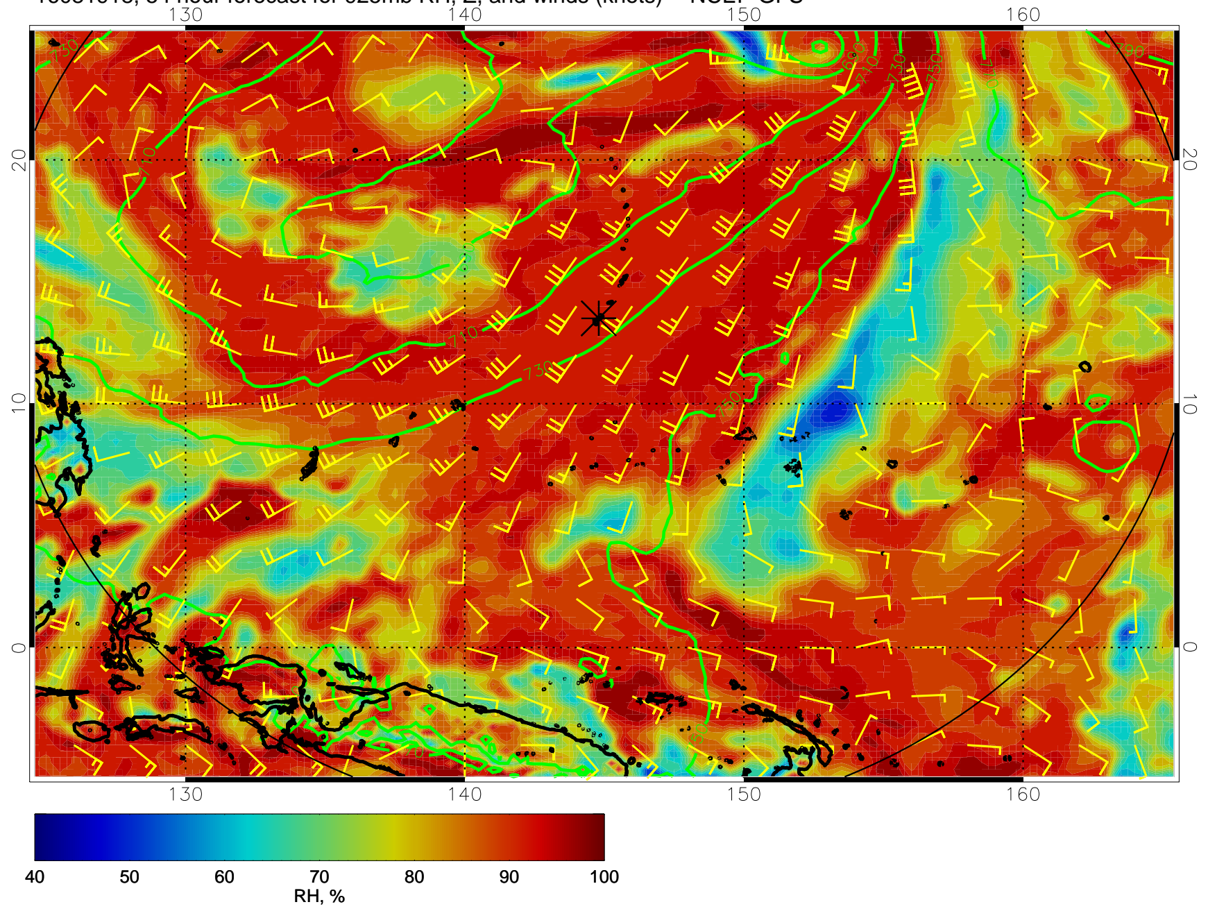
16081918, 54 hour forecast for 925mb RH, Z, and winds (knots) -- NCEP GFS
