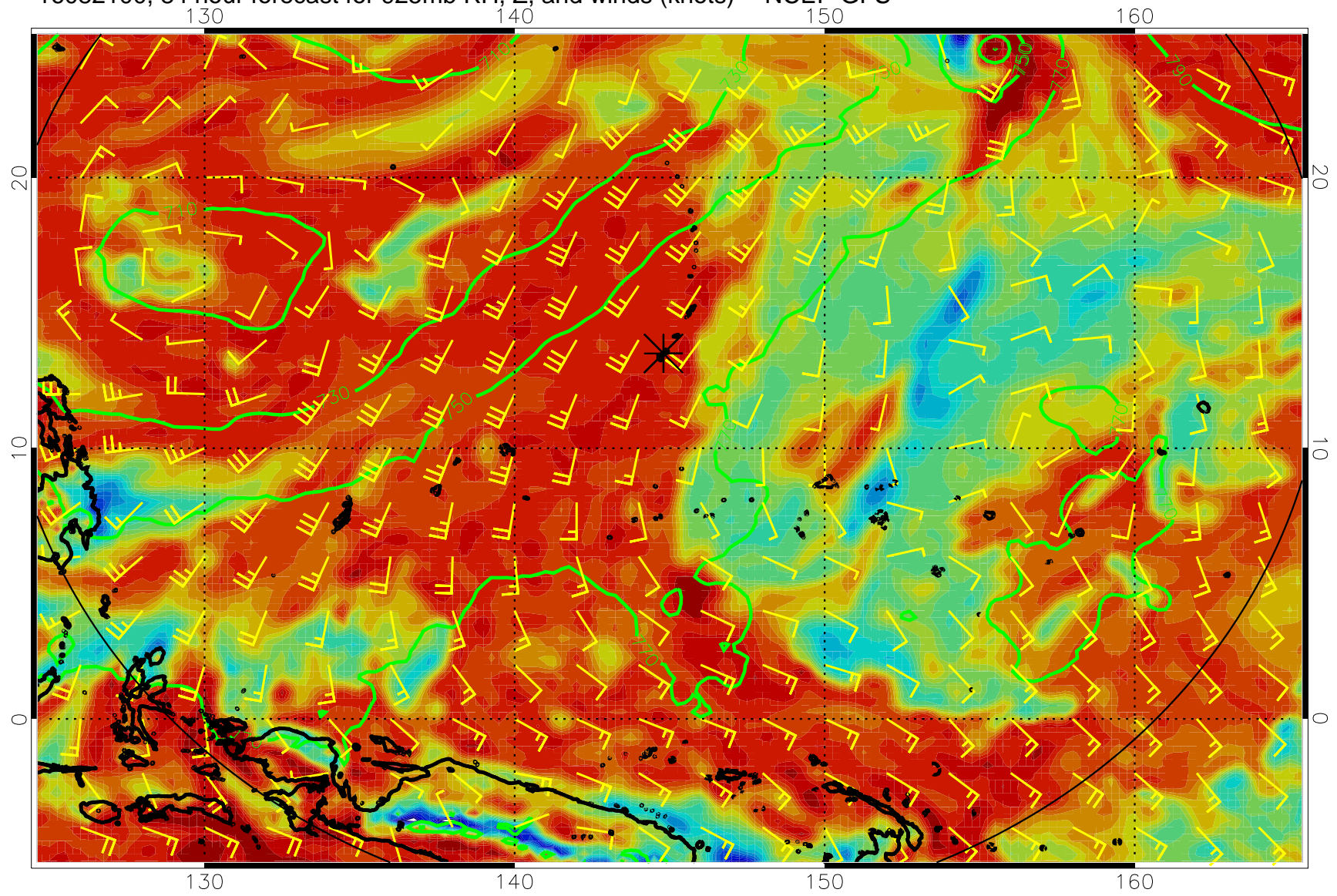
16082100, 84 hour forecast for 925mb RH, Z, and winds (knots) -- NCEP GFS
