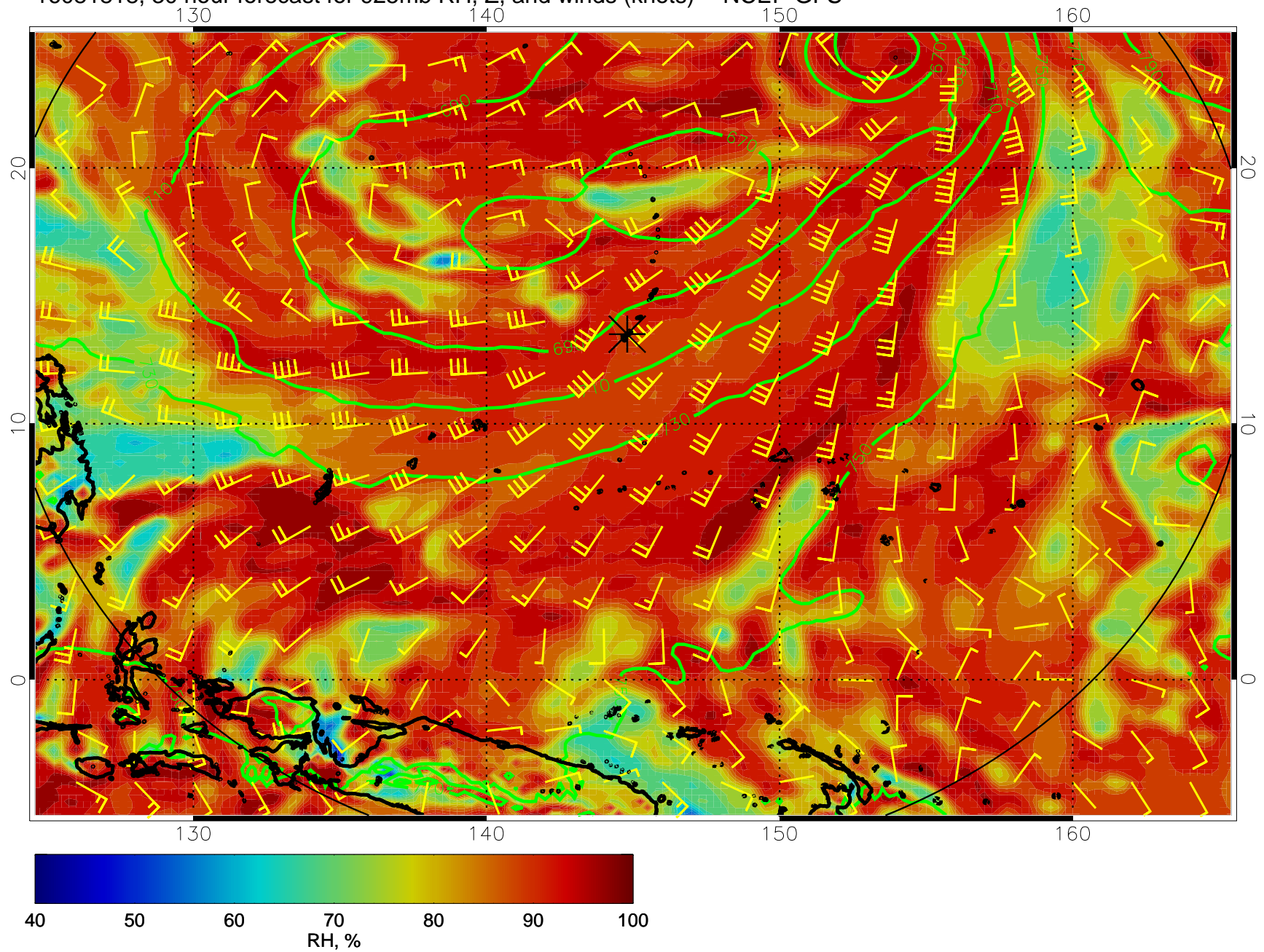
16081818, 30 hour forecast for 925mb RH, Z, and winds (knots) -- NCEP GFS
