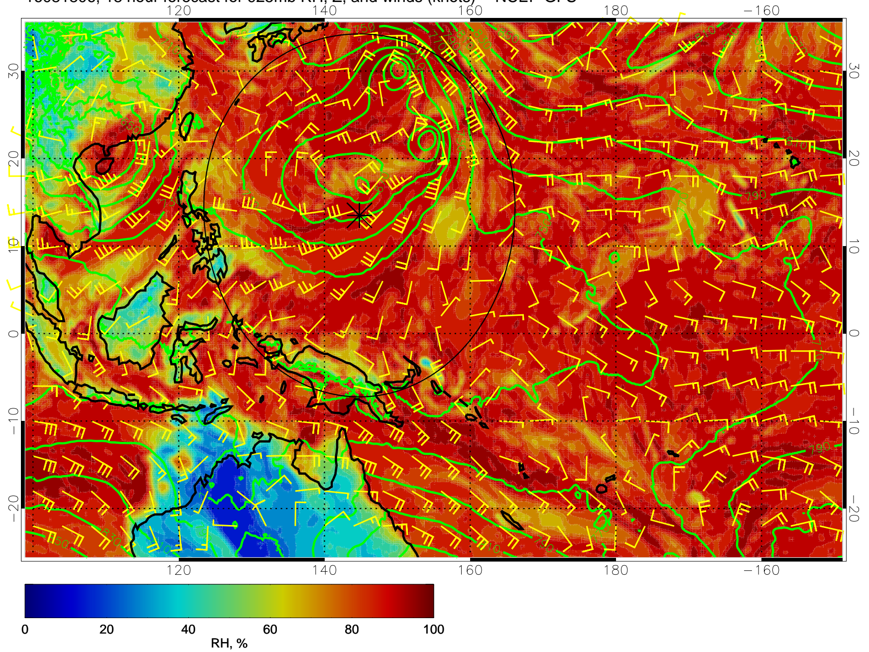
16081806, 18 hour forecast for 925mb RH, Z, and winds (knots) -- NCEP GFS
