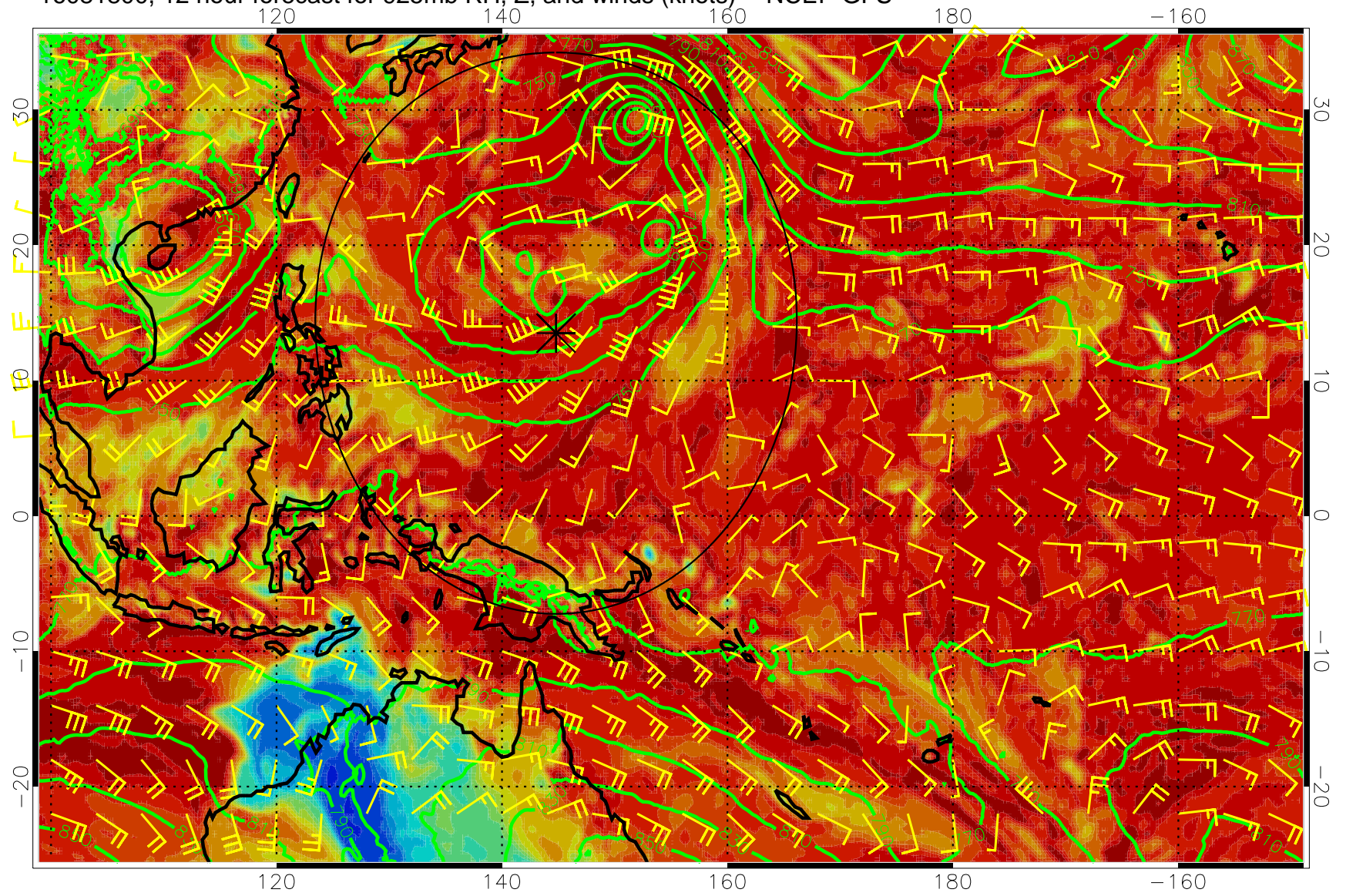
16081800, 12 hour forecast for 925mb RH, Z, and winds (knots) -- NCEP GFS
