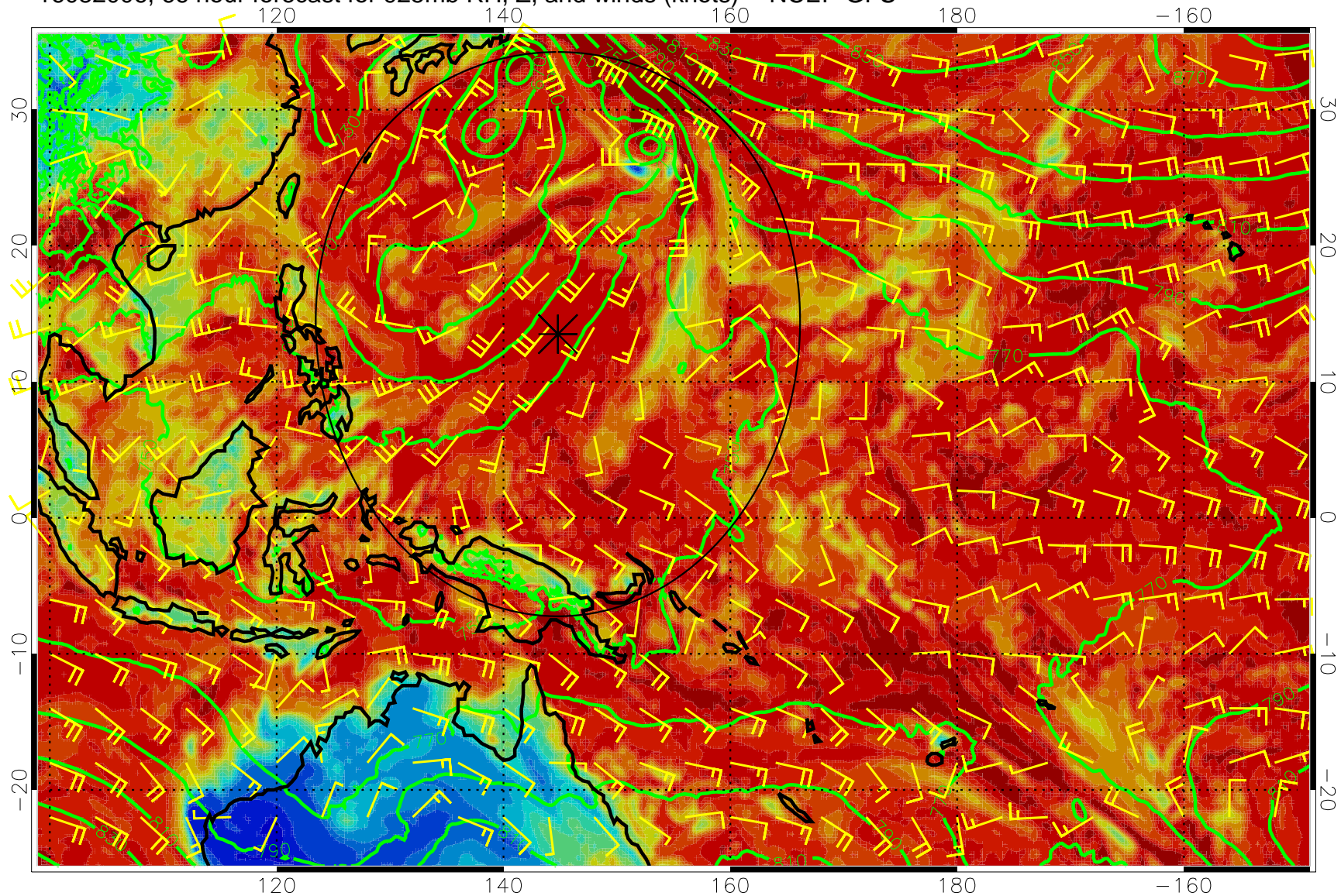
16082006, 66 hour forecast for 925mb RH, Z, and winds (knots) -- NCEP GFS
