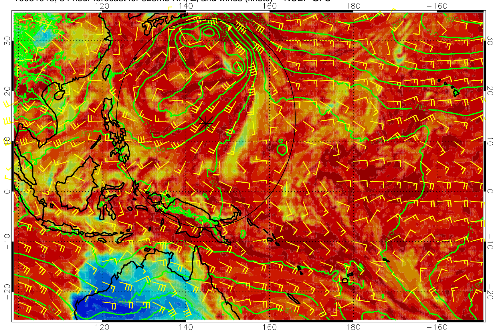
16081918, 54 hour forecast for 925mb RH, Z, and winds (knots) -- NCEP GFS
