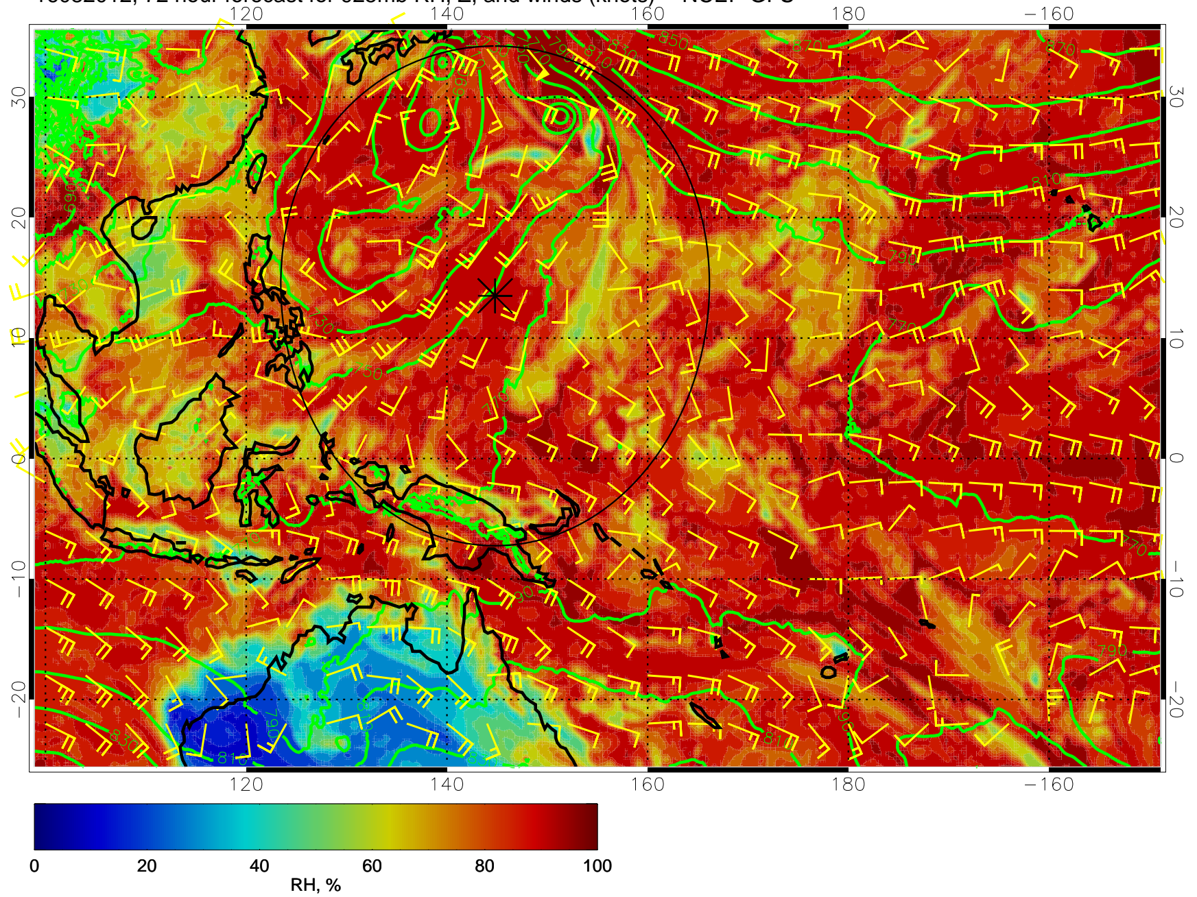
16082012, 72 hour forecast for 925mb RH, Z, and winds (knots) -- NCEP GFS
