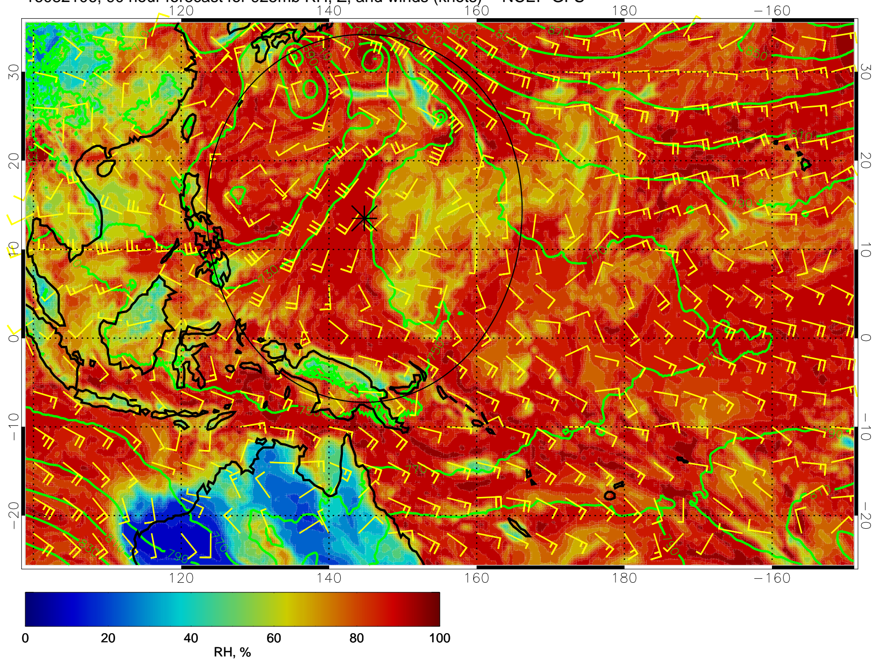
16082106, 90 hour forecast for 925mb RH, Z, and winds (knots) -- NCEP GFS
