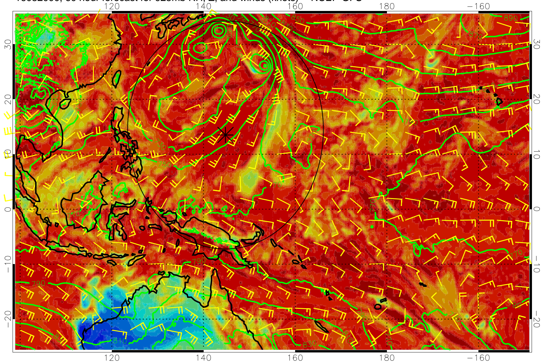
16082000, 60 hour forecast for 925mb RH, Z, and winds (knots) -- NCEP GFS
