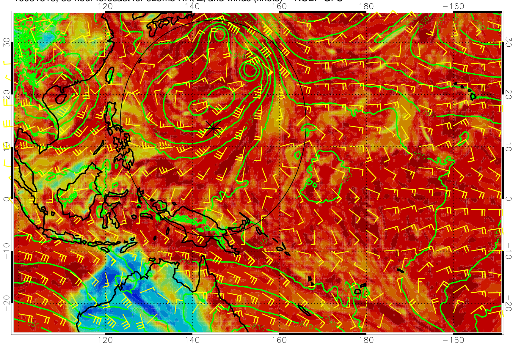
16081818, 30 hour forecast for 925mb RH, Z, and winds (knots) -- NCEP GFS
