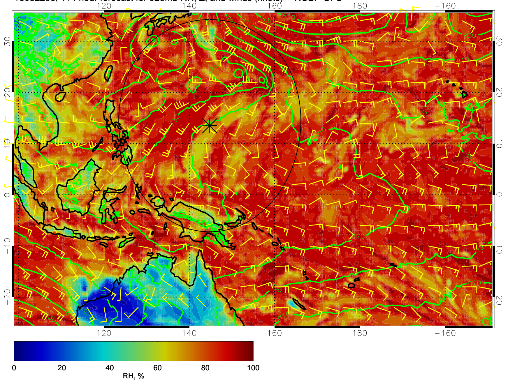
16082206, 114 hour forecast for 925mb RH, Z, and winds (knots) -- NCEP GFS
