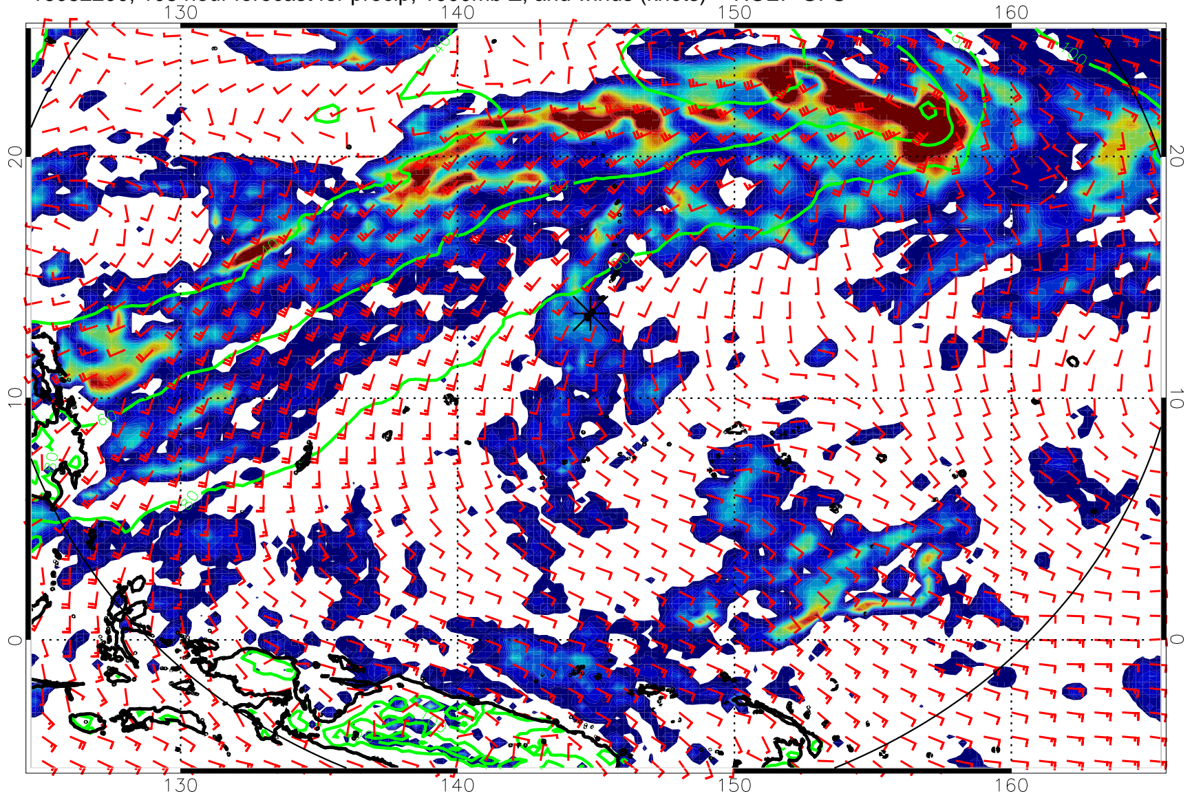
16082200, 108 hour forecast for precip, 1000mb Z, and winds (knots) -- NCEP GFS
