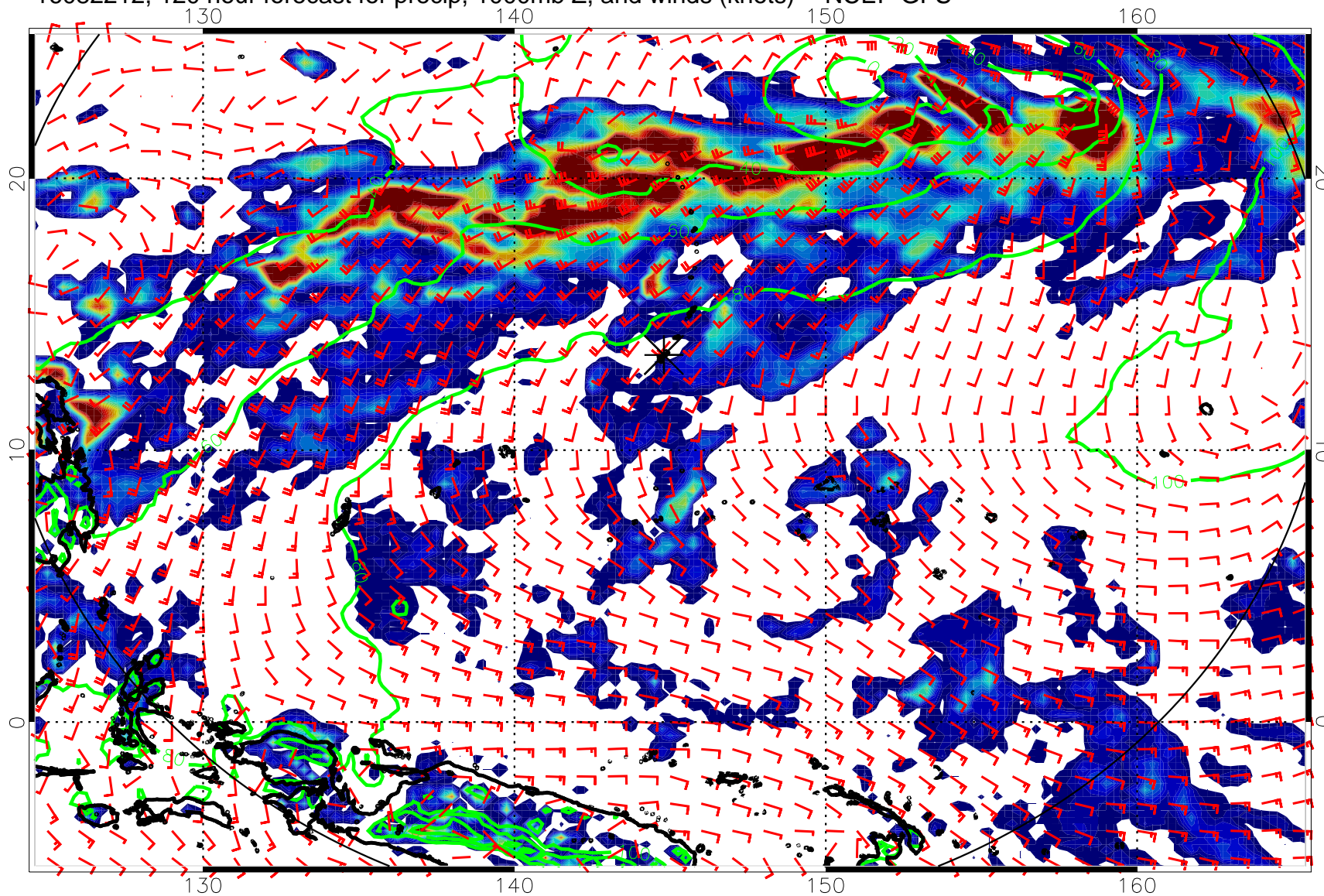
16082212, 120 hour forecast for precip, 1000mb Z, and winds (knots) -- NCEP GFS
