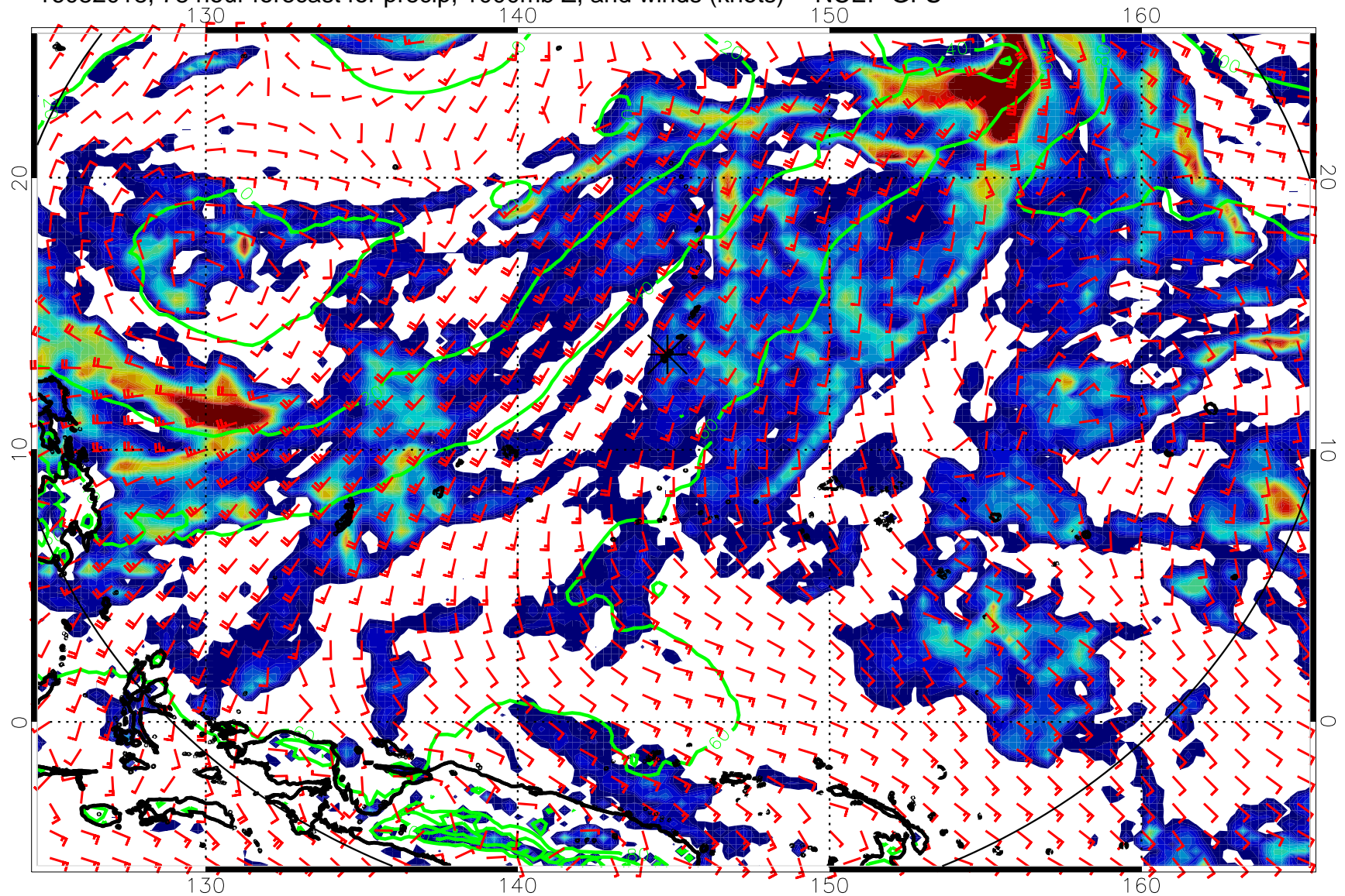
16082018, 78 hour forecast for precip, 1000mb Z, and winds (knots) -- NCEP GFS
