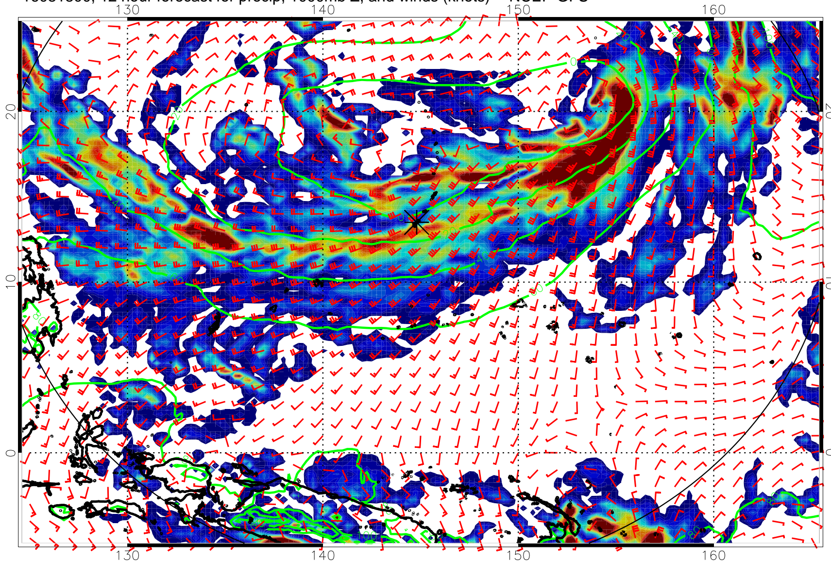
16081800, 12 hour forecast for precip, 1000mb Z, and winds (knots) -- NCEP GFS
