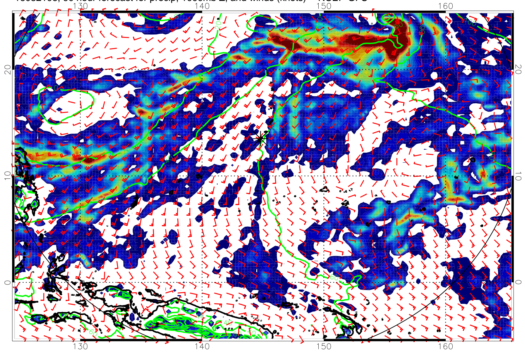
16082106, 90 hour forecast for precip, 1000mb Z, and winds (knots) -- NCEP GFS
