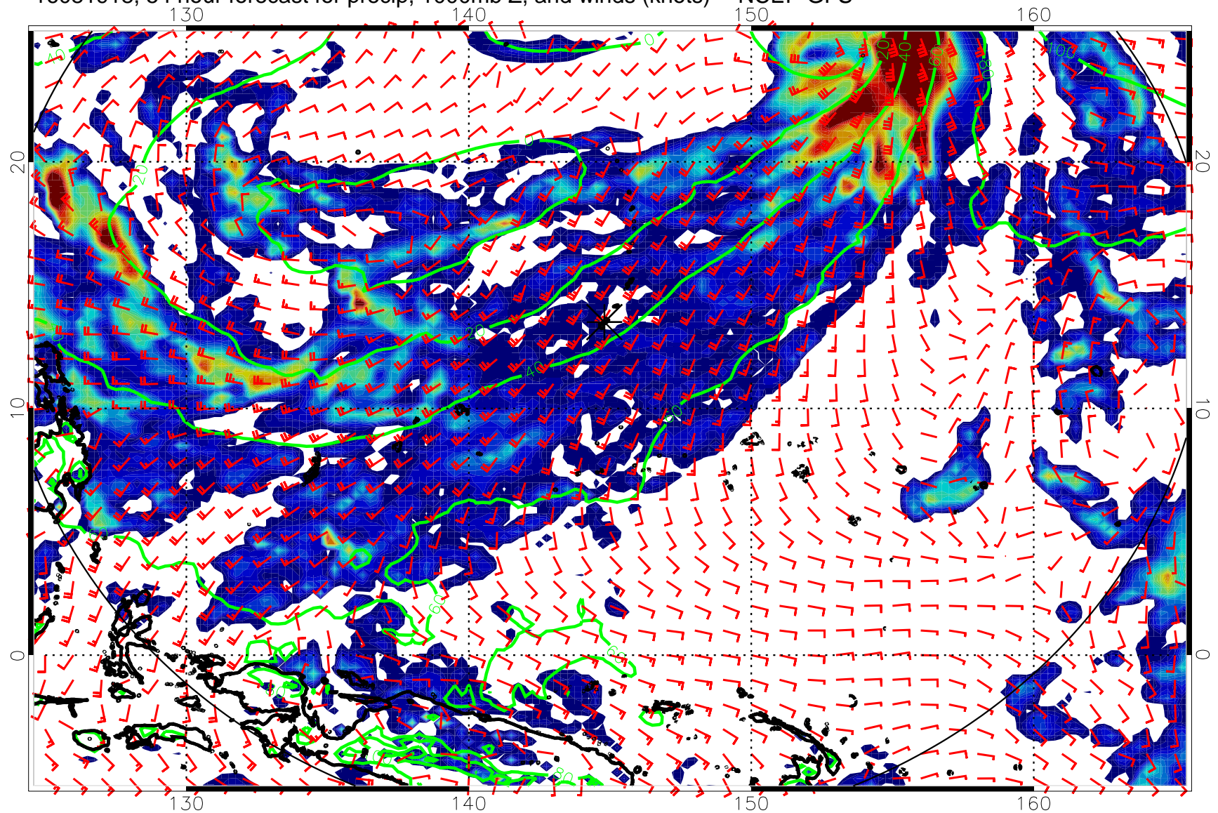
16081918, 54 hour forecast for precip, 1000mb Z, and winds (knots) -- NCEP GFS
