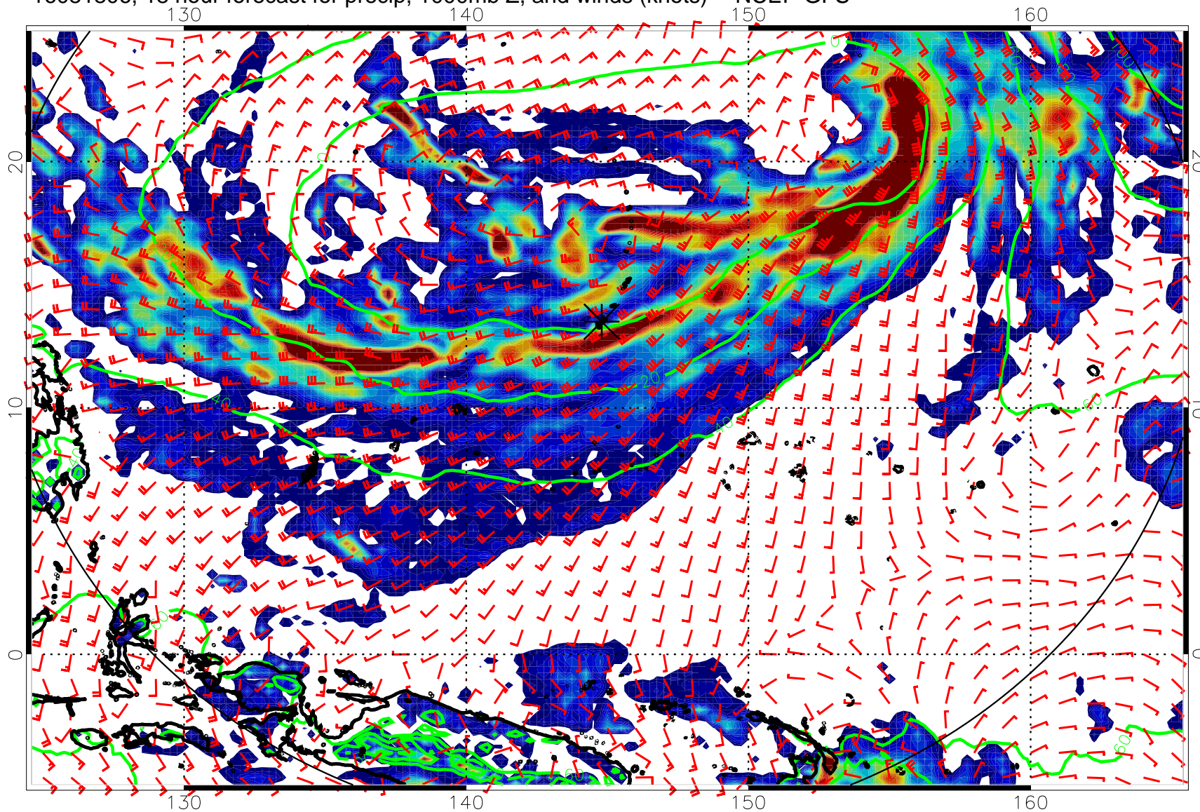
16081806, 18 hour forecast for precip, 1000mb Z, and winds (knots) -- NCEP GFS
