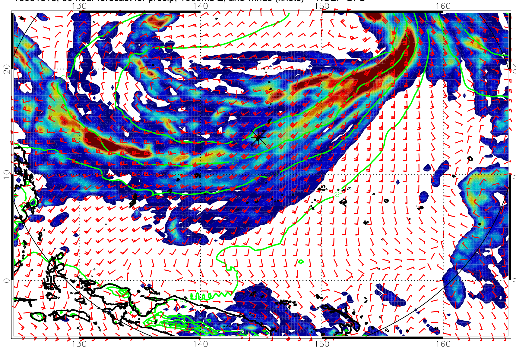
16081818, 30 hour forecast for precip, 1000mb Z, and winds (knots) -- NCEP GFS
