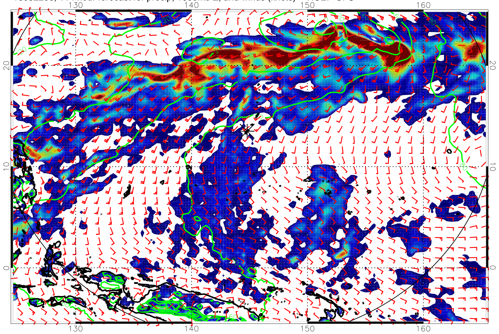
16082206, 114 hour forecast for precip, 1000mb Z, and winds (knots) -- NCEP GFS
