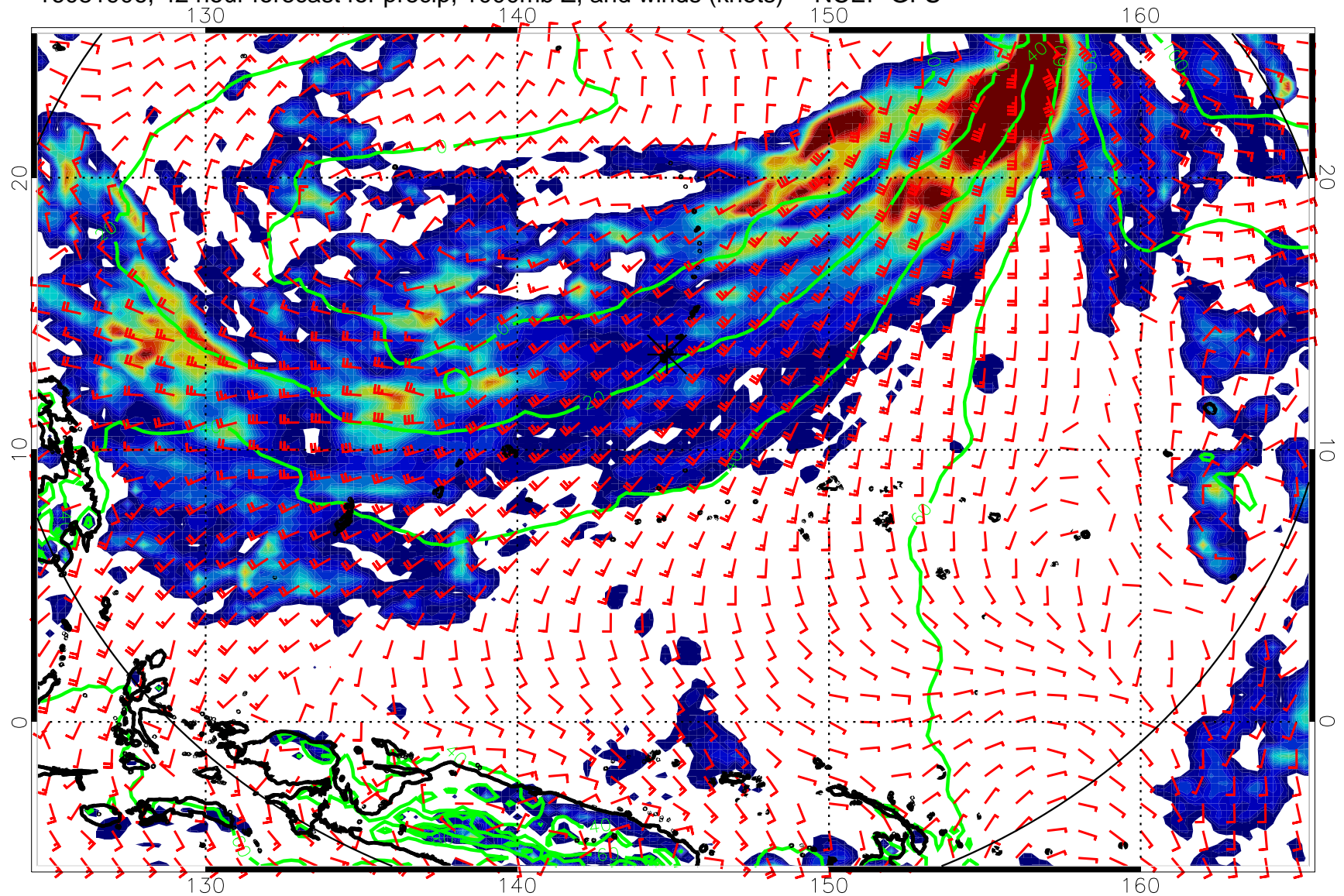
16081906, 42 hour forecast for precip, 1000mb Z, and winds (knots) -- NCEP GFS
