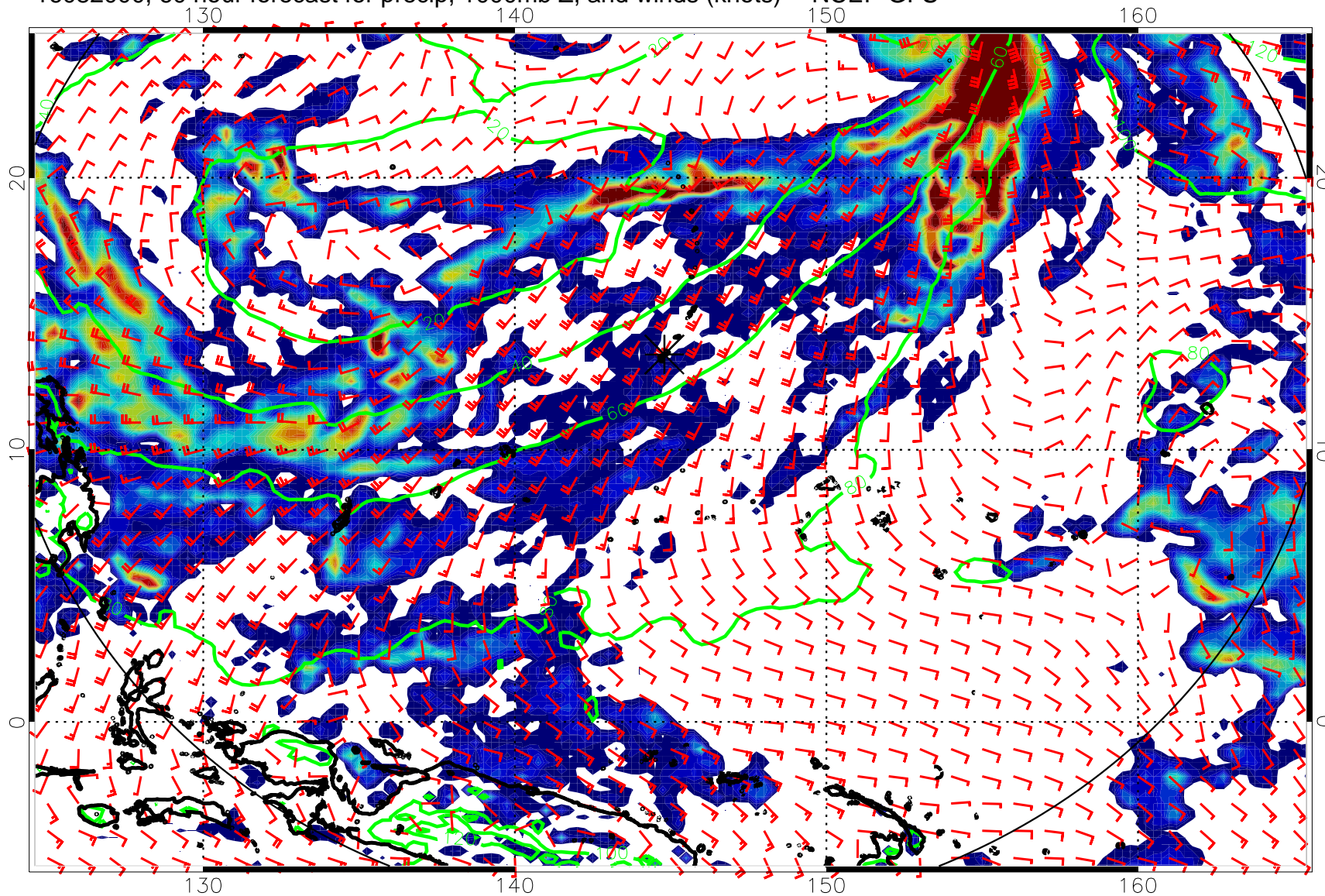
16082000, 60 hour forecast for precip, 1000mb Z, and winds (knots) -- NCEP GFS
