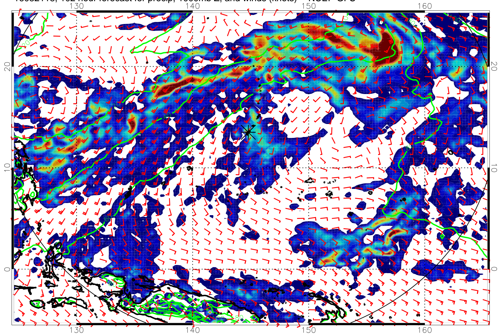
16082118, 102 hour forecast for precip, 1000mb Z, and winds (knots) -- NCEP GFS
