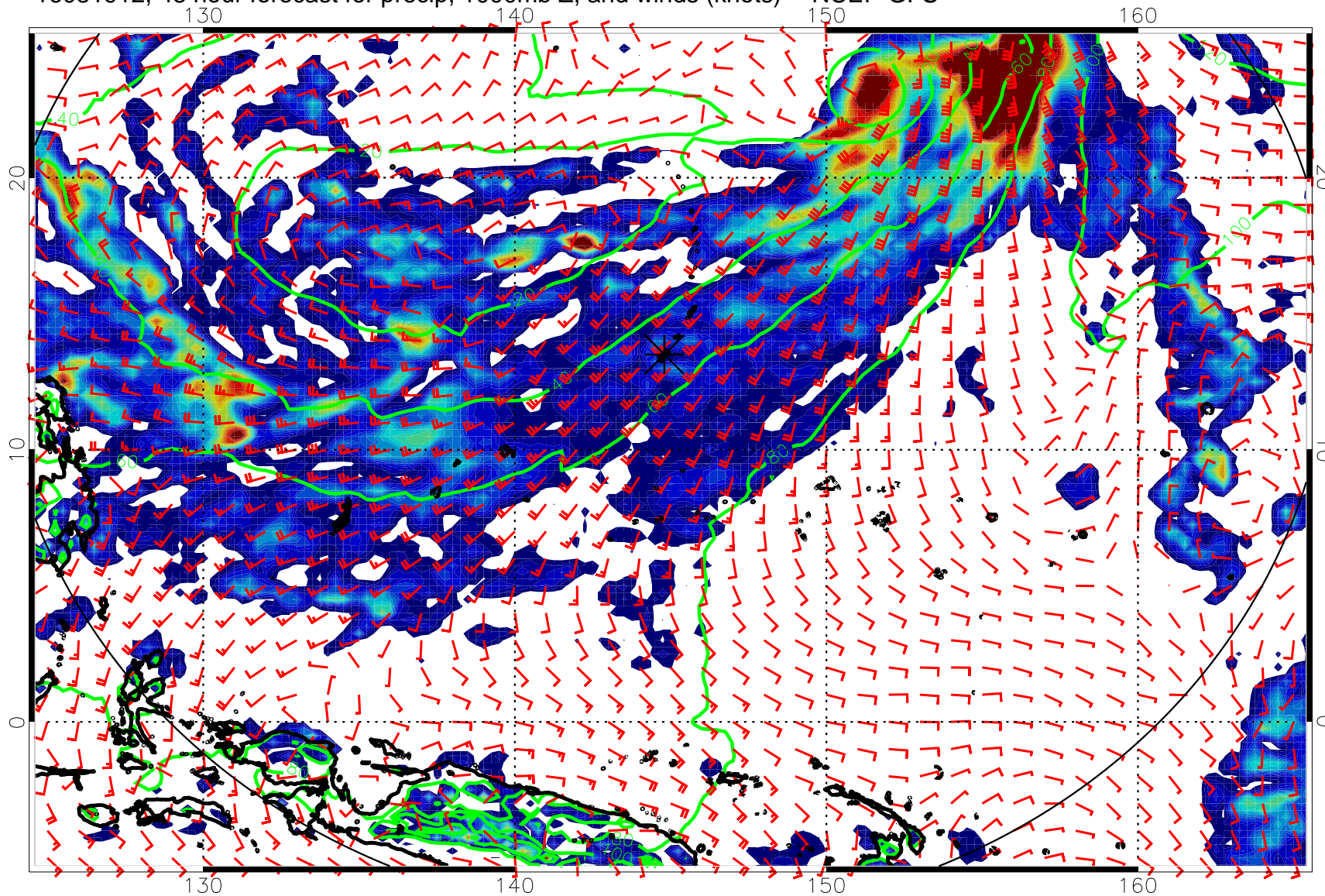
16081912, 48 hour forecast for precip, 1000mb Z, and winds (knots) -- NCEP GFS
