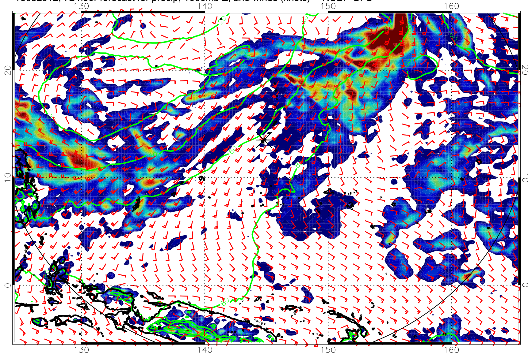
16082012, 72 hour forecast for precip, 1000mb Z, and winds (knots) -- NCEP GFS
