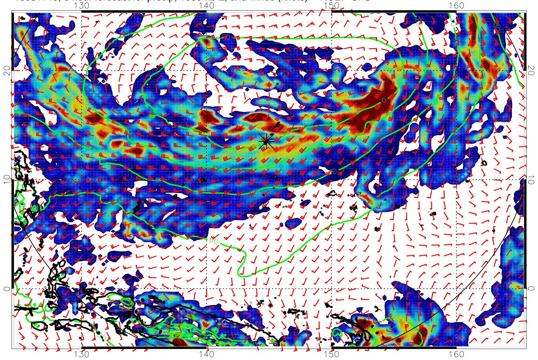
16081718, 6 hour forecast for precip, 1000mb Z, and winds (knots) -- NCEP GFS
