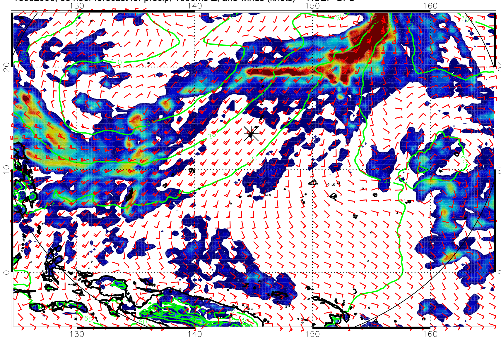
16082006, 66 hour forecast for precip, 1000mb Z, and winds (knots) -- NCEP GFS
