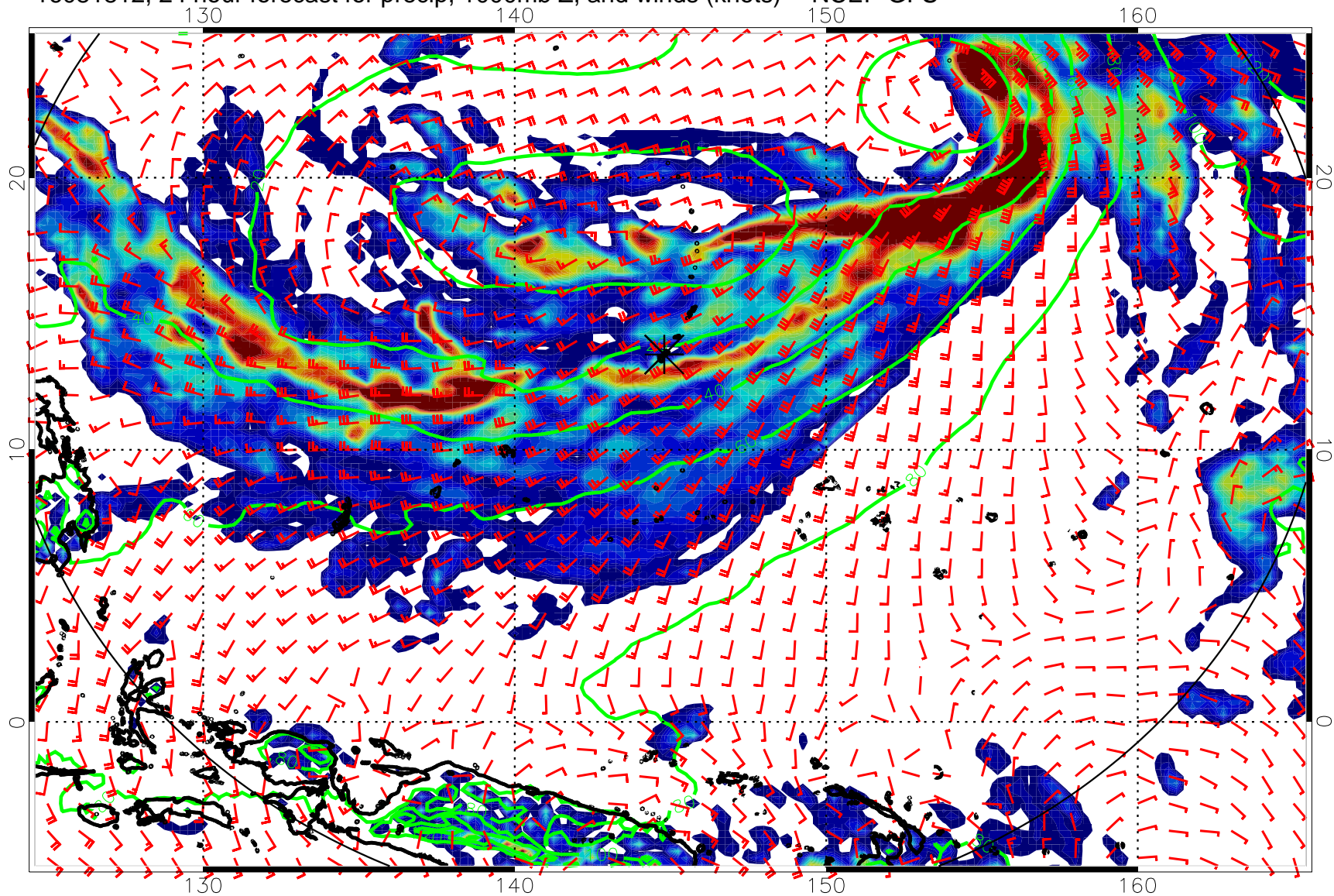
16081812, 24 hour forecast for precip, 1000mb Z, and winds (knots) -- NCEP GFS
