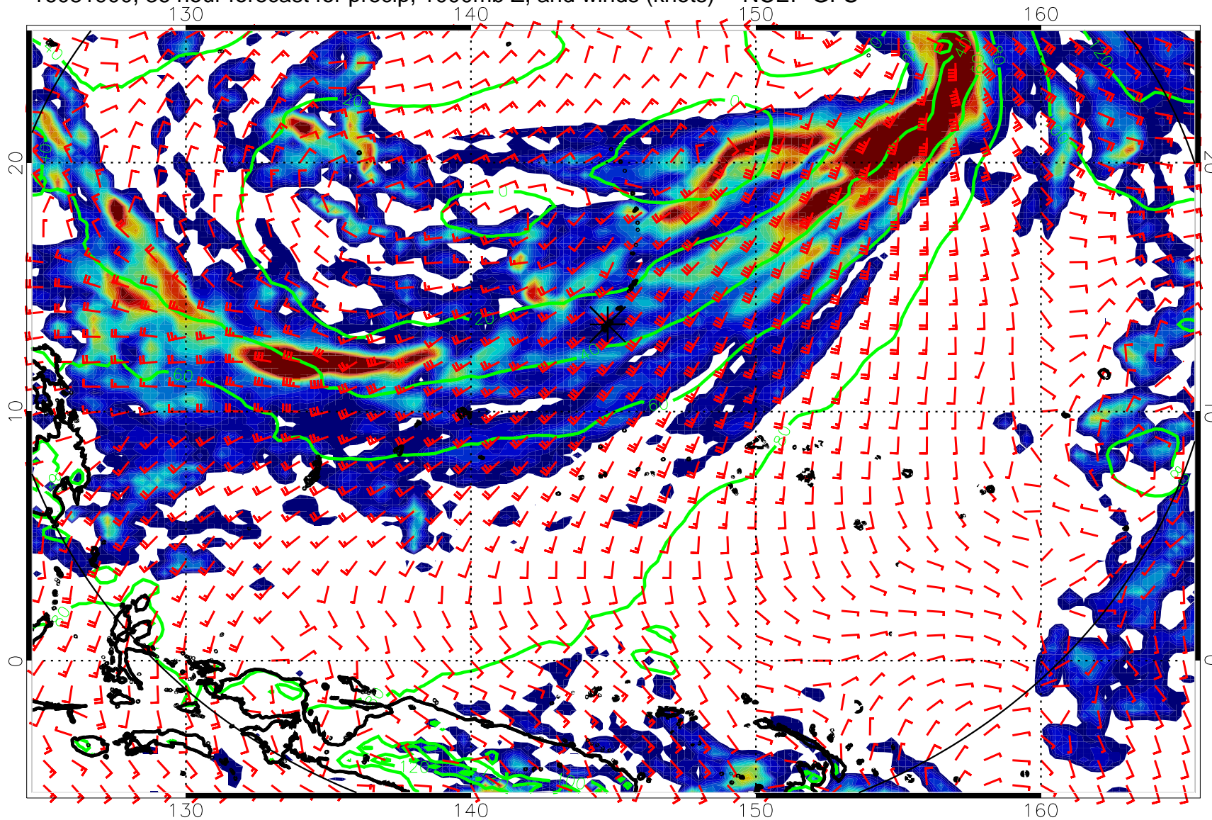
16081900, 36 hour forecast for precip, 1000mb Z, and winds (knots) -- NCEP GFS
