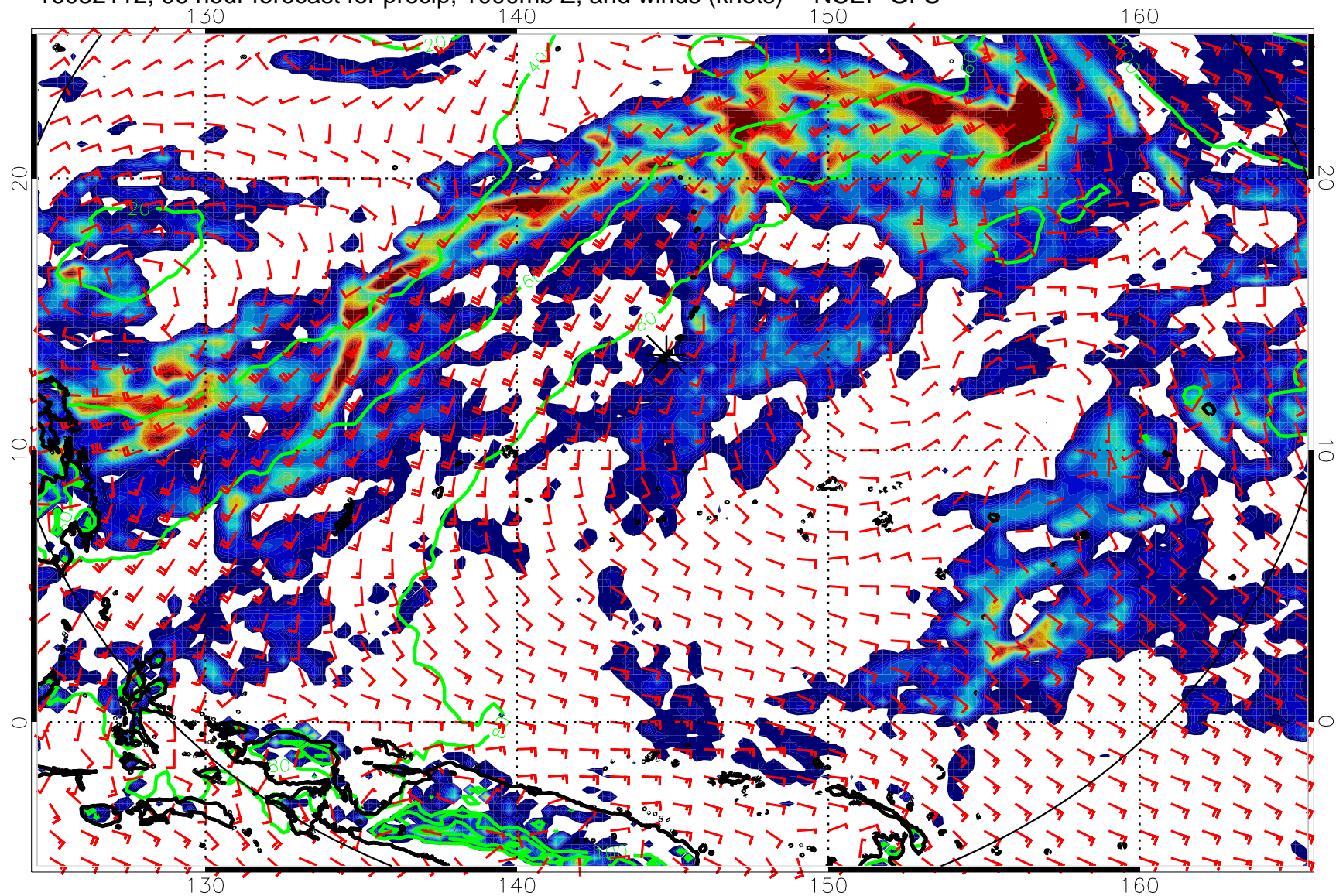
16082112, 96 hour forecast for precip, 1000mb Z, and winds (knots) -- NCEP GFS
