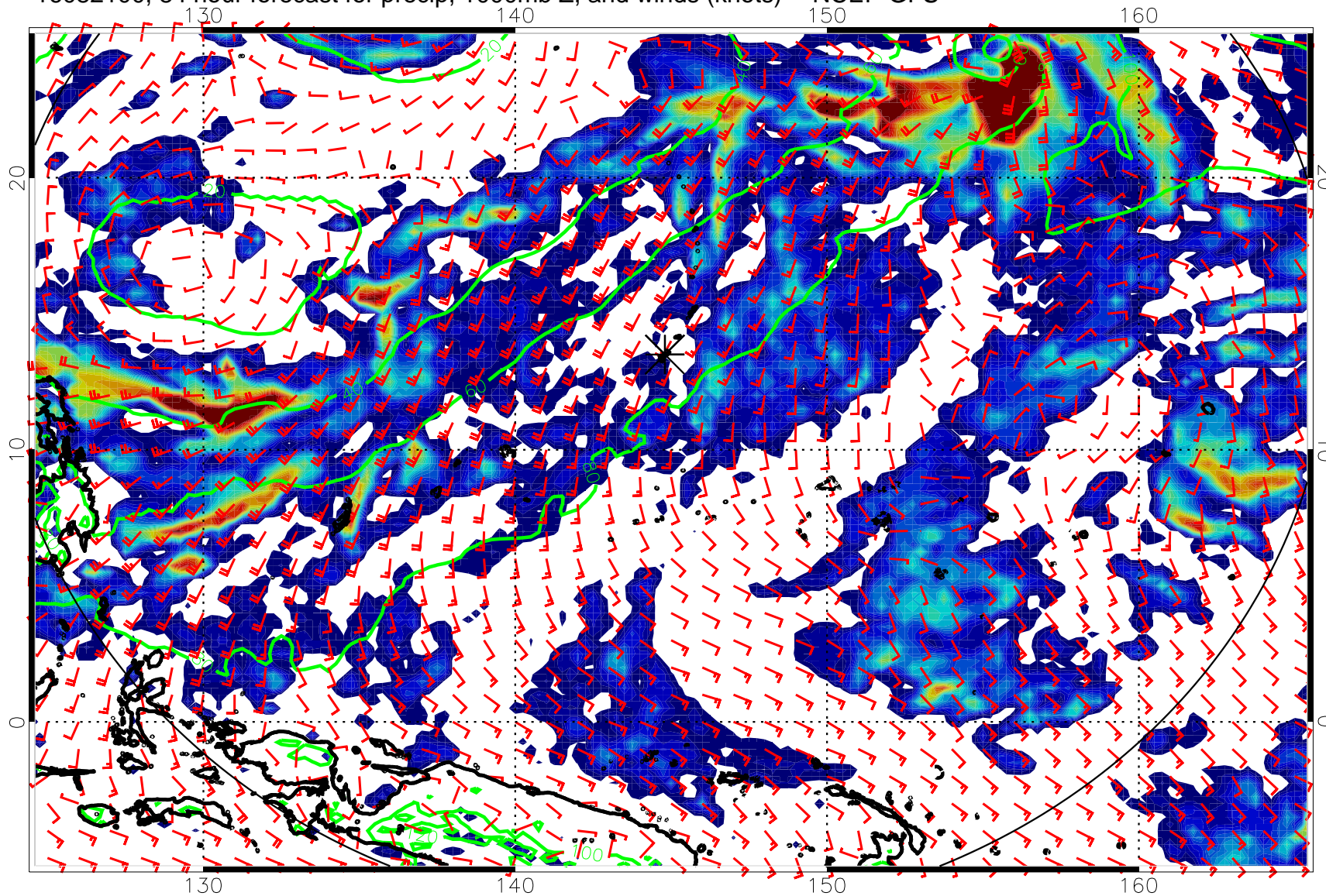
16082100, 84 hour forecast for precip, 1000mb Z, and winds (knots) -- NCEP GFS
