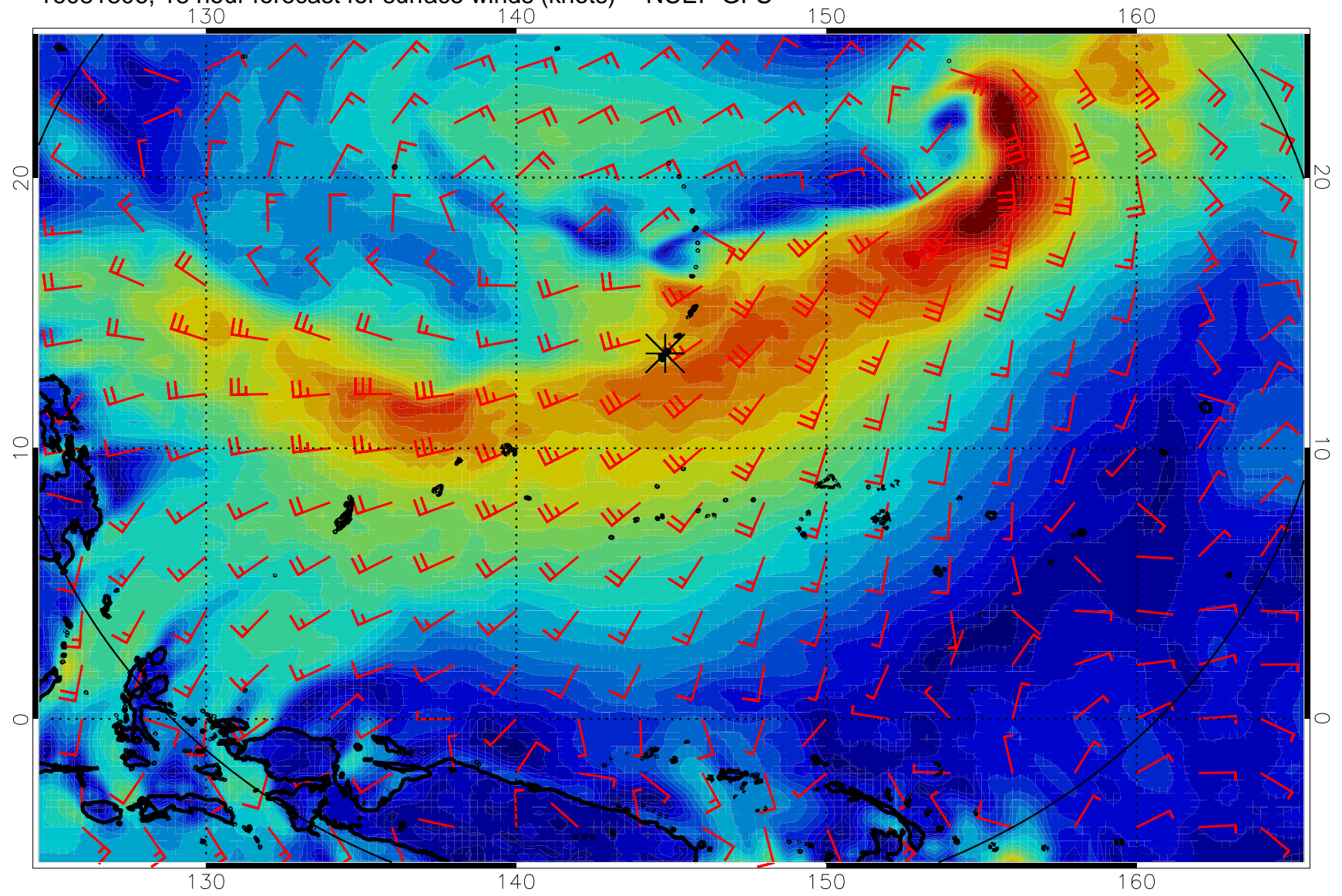
16081806, 18 hour forecast for surface winds (knots) -- NCEP GFS
