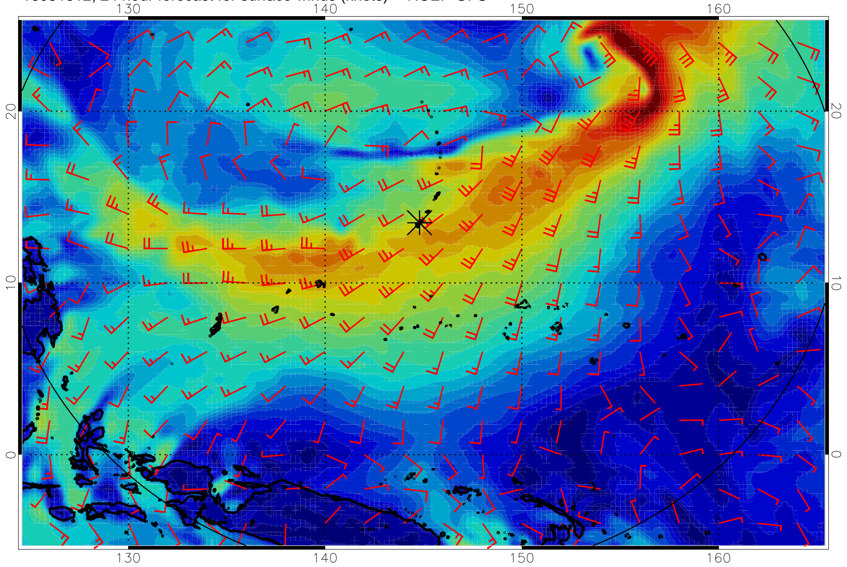
16081812, 24 hour forecast for surface winds (knots) -- NCEP GFS
