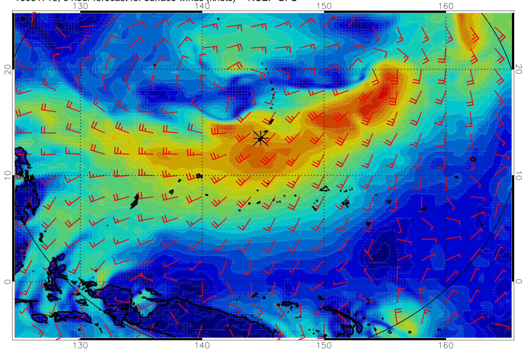
16081718, 6 hour forecast for surface winds (knots) -- NCEP GFS
