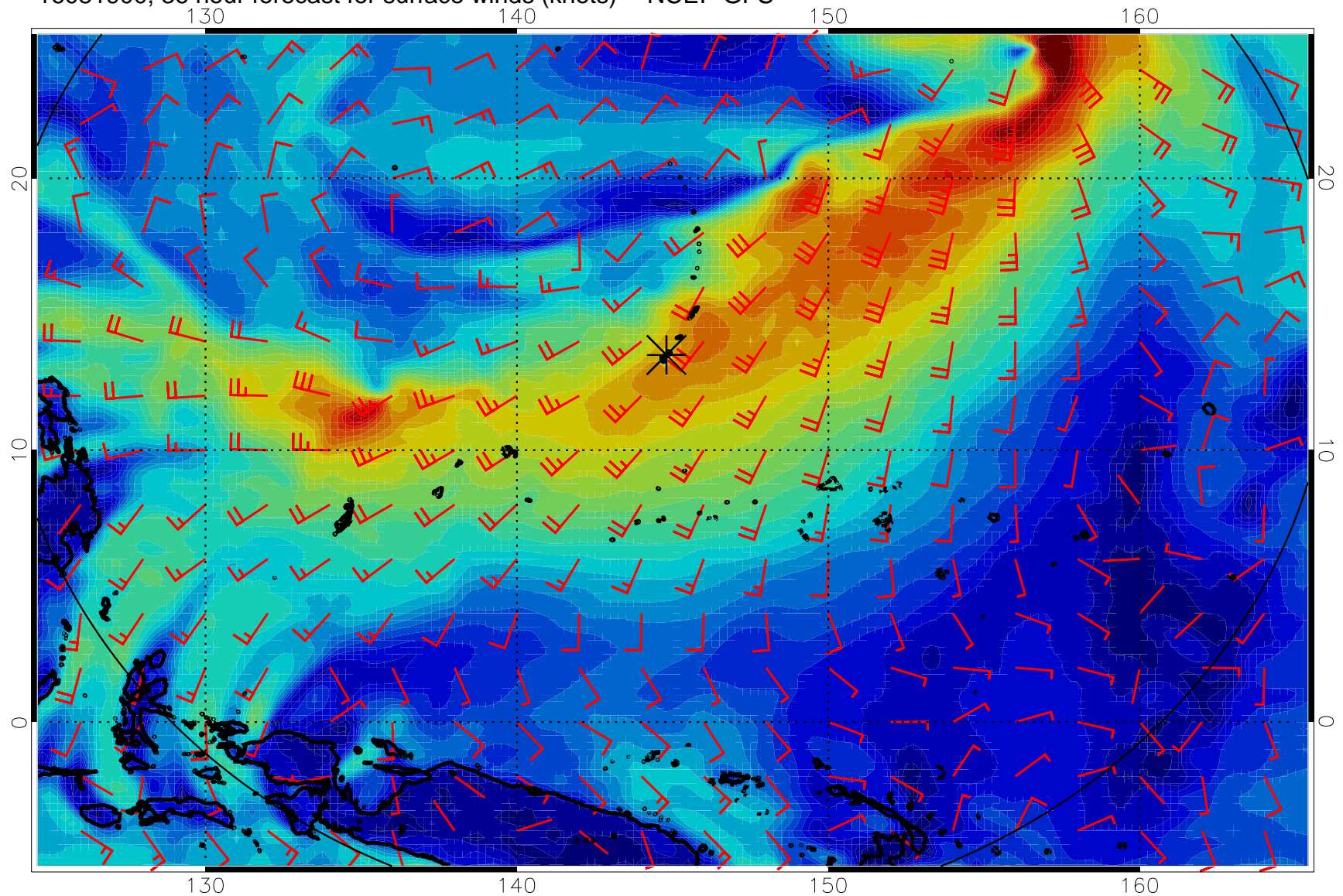
16081900, 36 hour forecast for surface winds (knots) -- NCEP GFS
