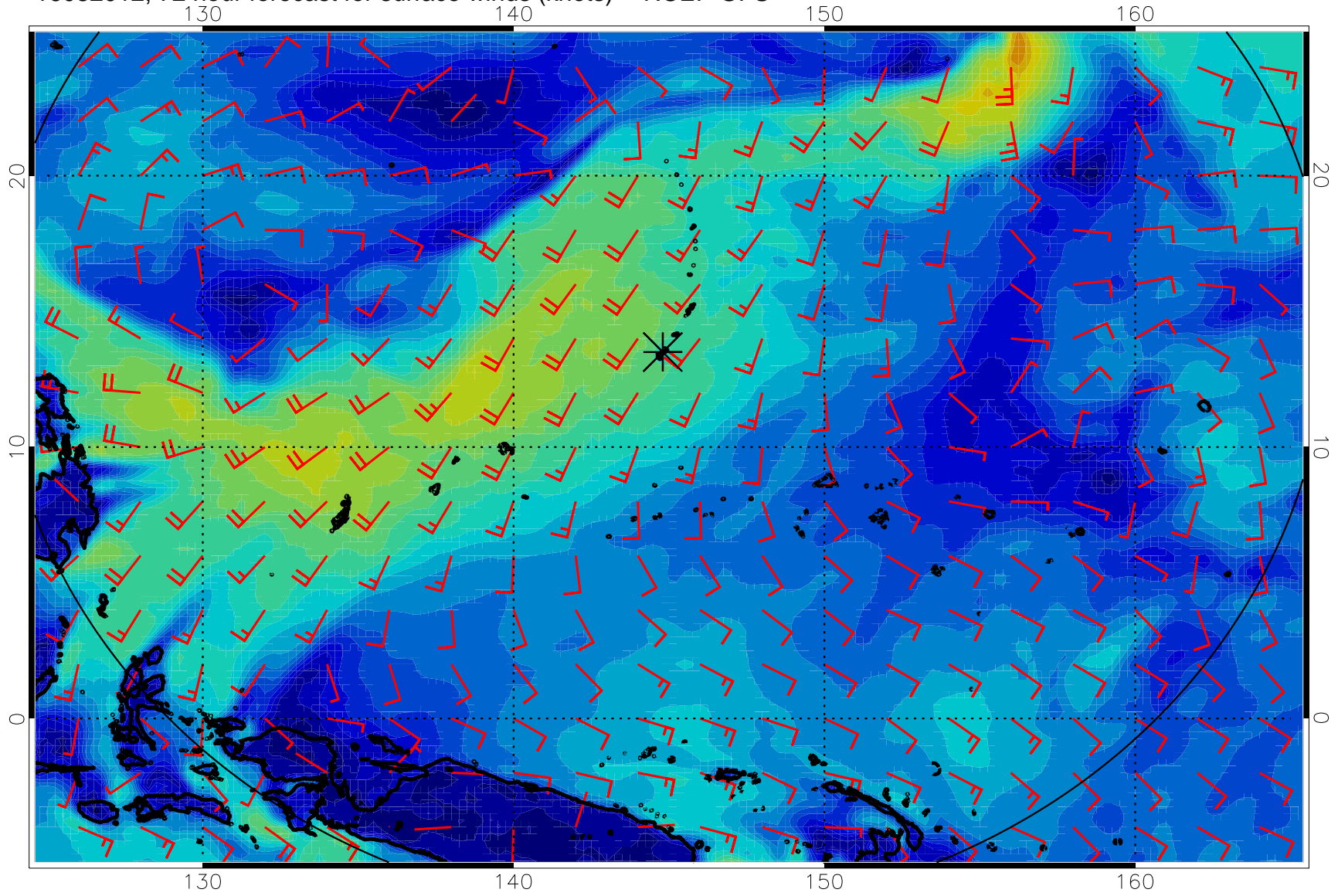
16082012, 72 hour forecast for surface winds (knots) -- NCEP GFS
