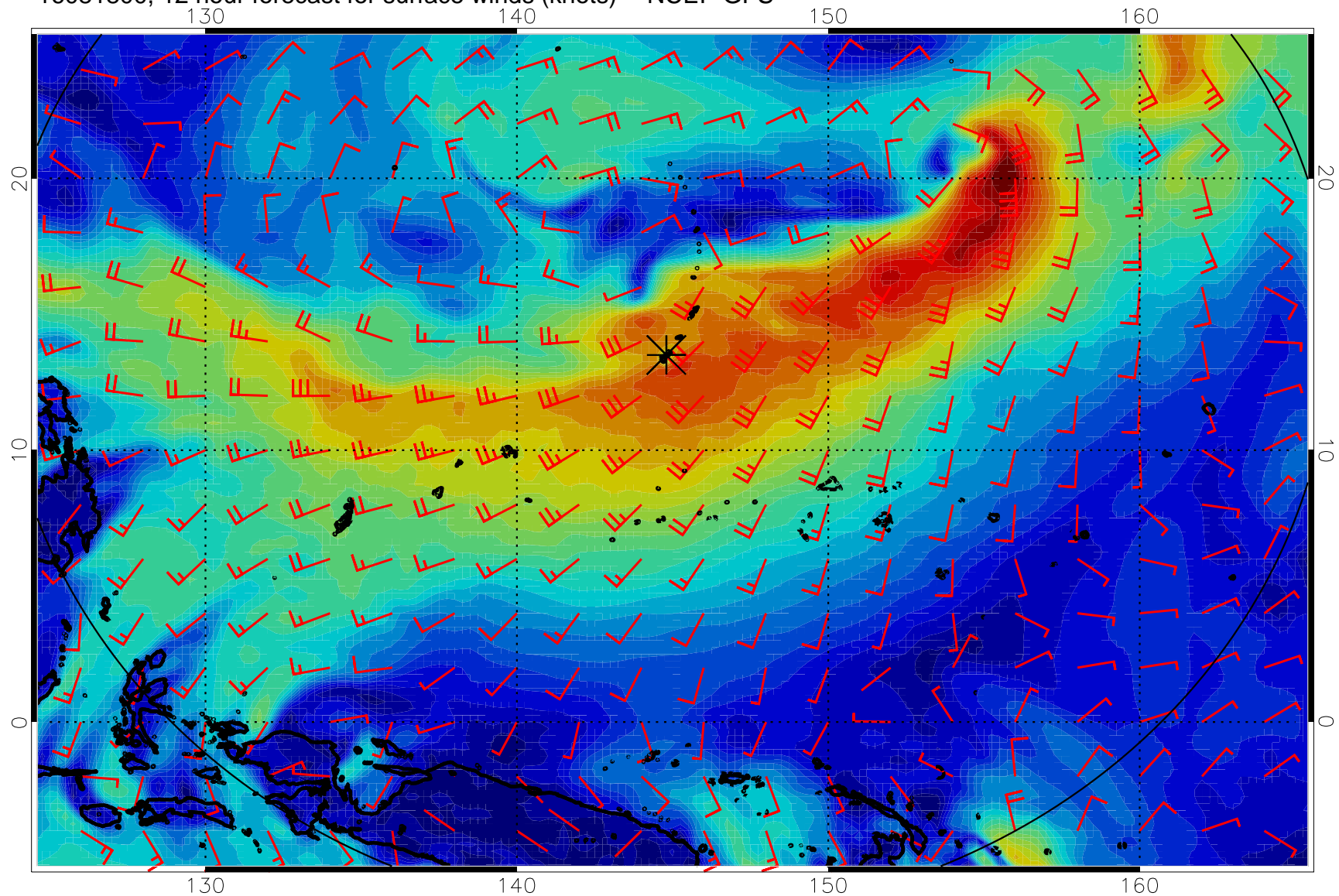
16081800, 12 hour forecast for surface winds (knots) -- NCEP GFS
