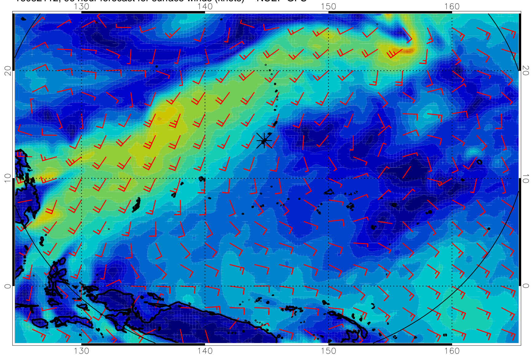
16082112, 96 hour forecast for surface winds (knots) -- NCEP GFS
