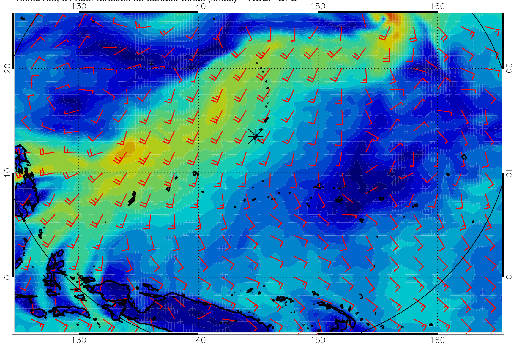
16082100, 84 hour forecast for surface winds (knots) -- NCEP GFS
