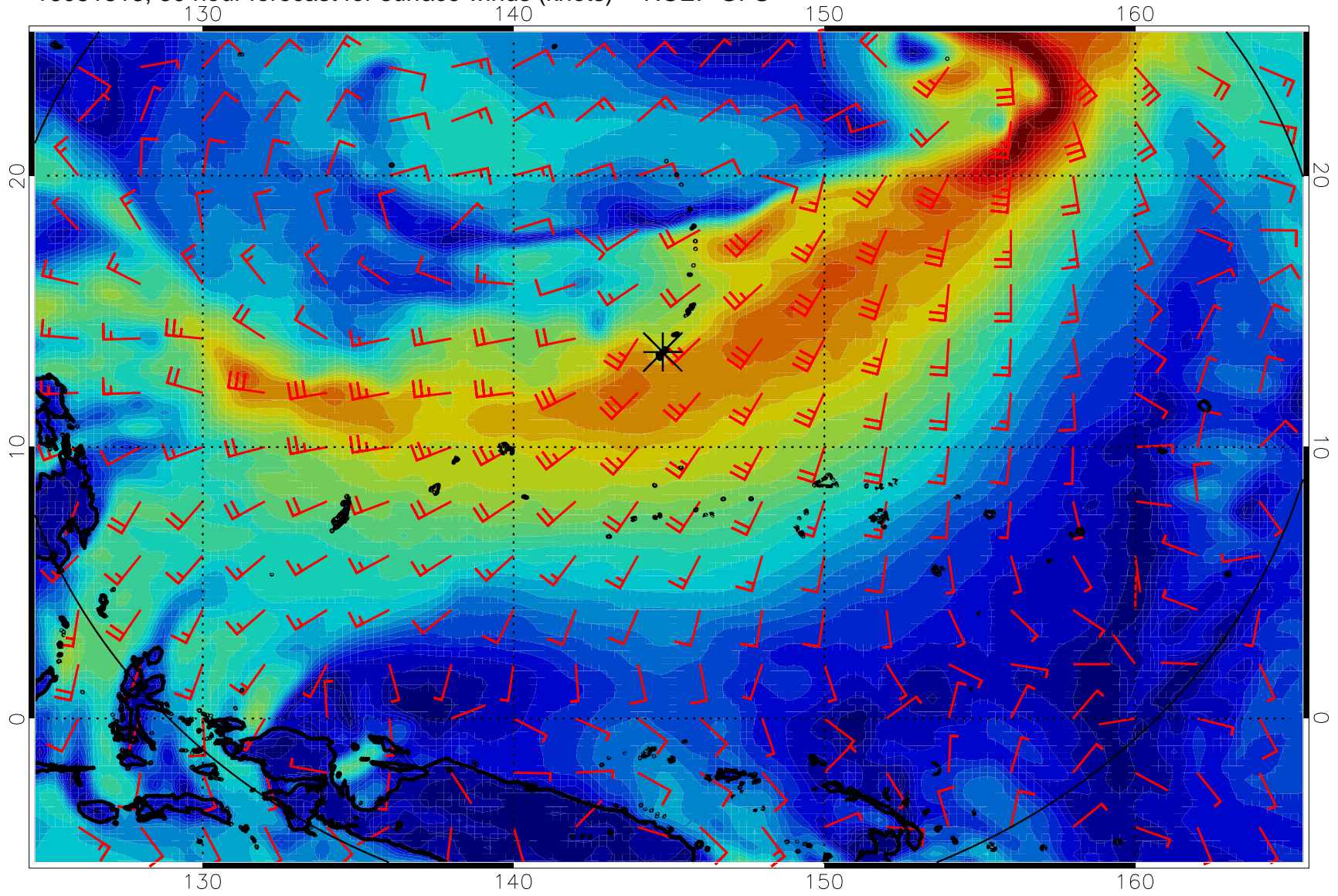
16081818, 30 hour forecast for surface winds (knots) -- NCEP GFS
