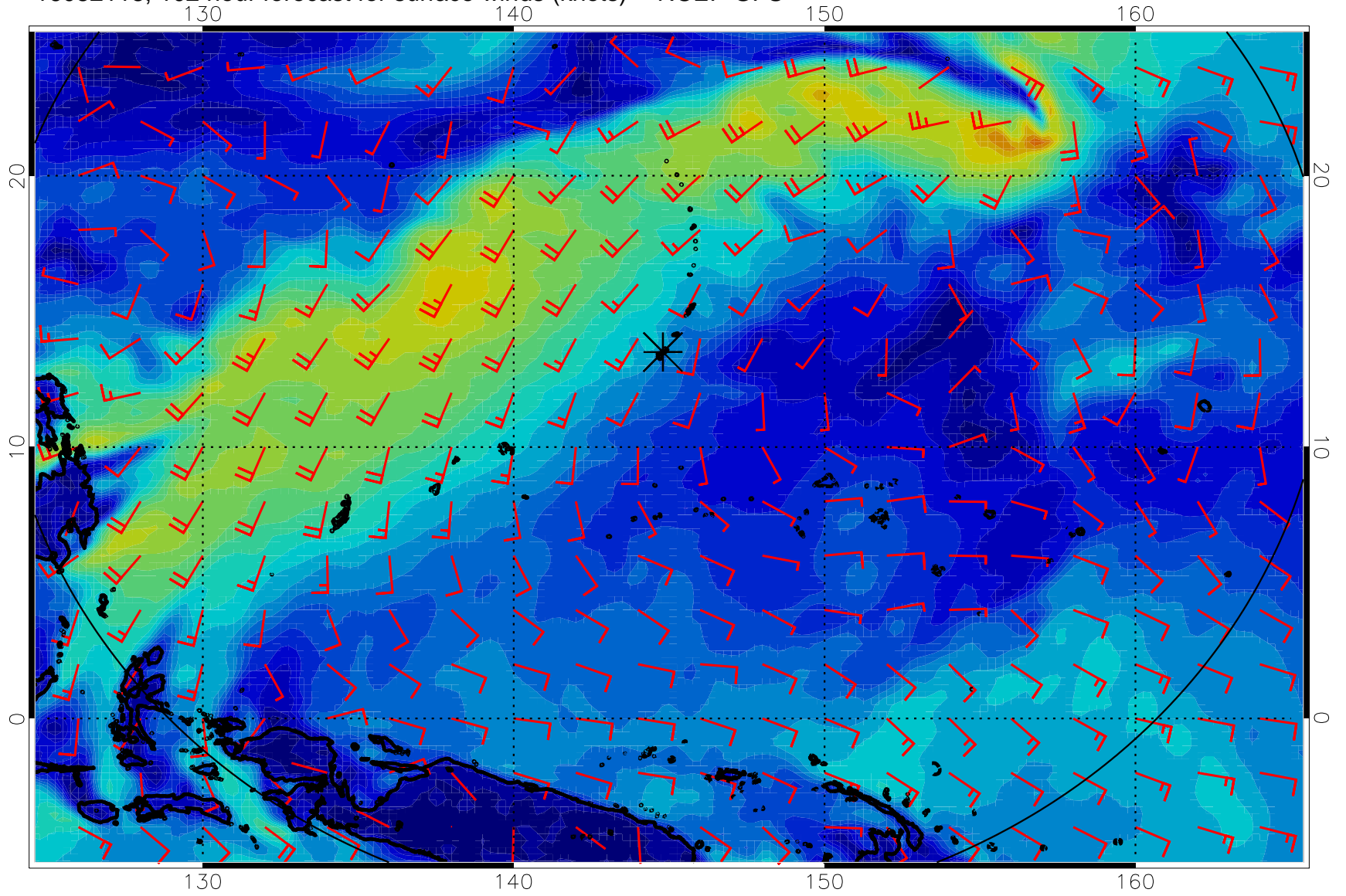
16082118, 102 hour forecast for surface winds (knots) -- NCEP GFS
