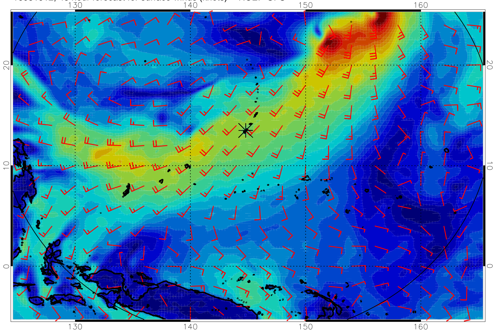
16081912, 48 hour forecast for surface winds (knots) -- NCEP GFS
