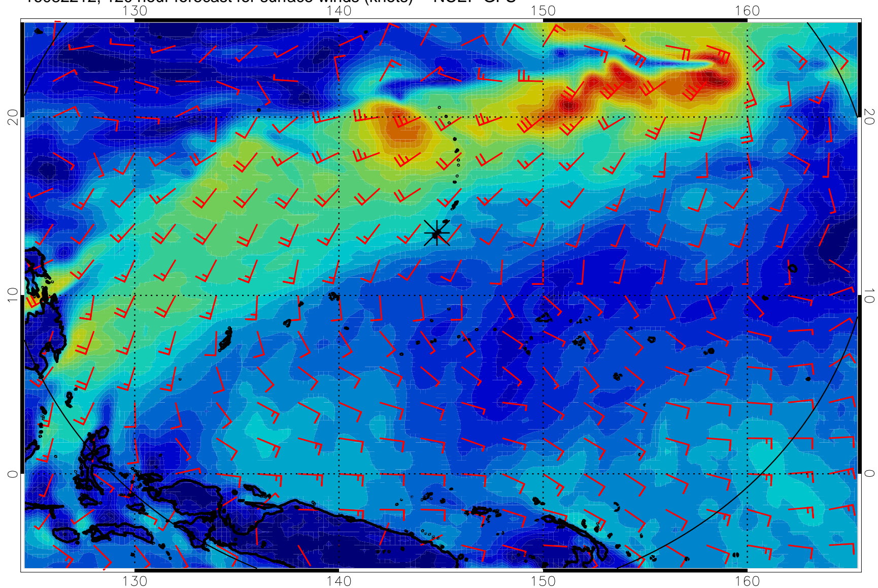
16082212, 120 hour forecast for surface winds (knots) -- NCEP GFS
