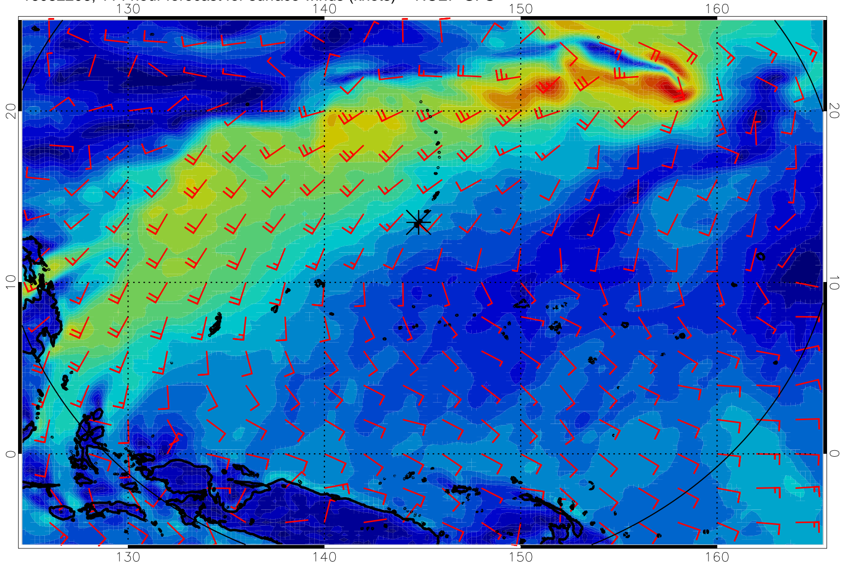
16082206, 114 hour forecast for surface winds (knots) -- NCEP GFS
