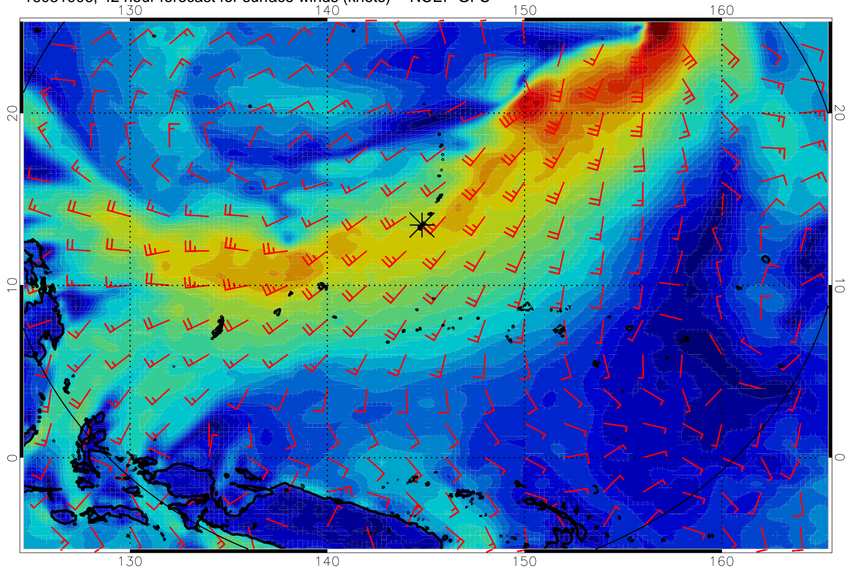
16081906, 42 hour forecast for surface winds (knots) -- NCEP GFS
