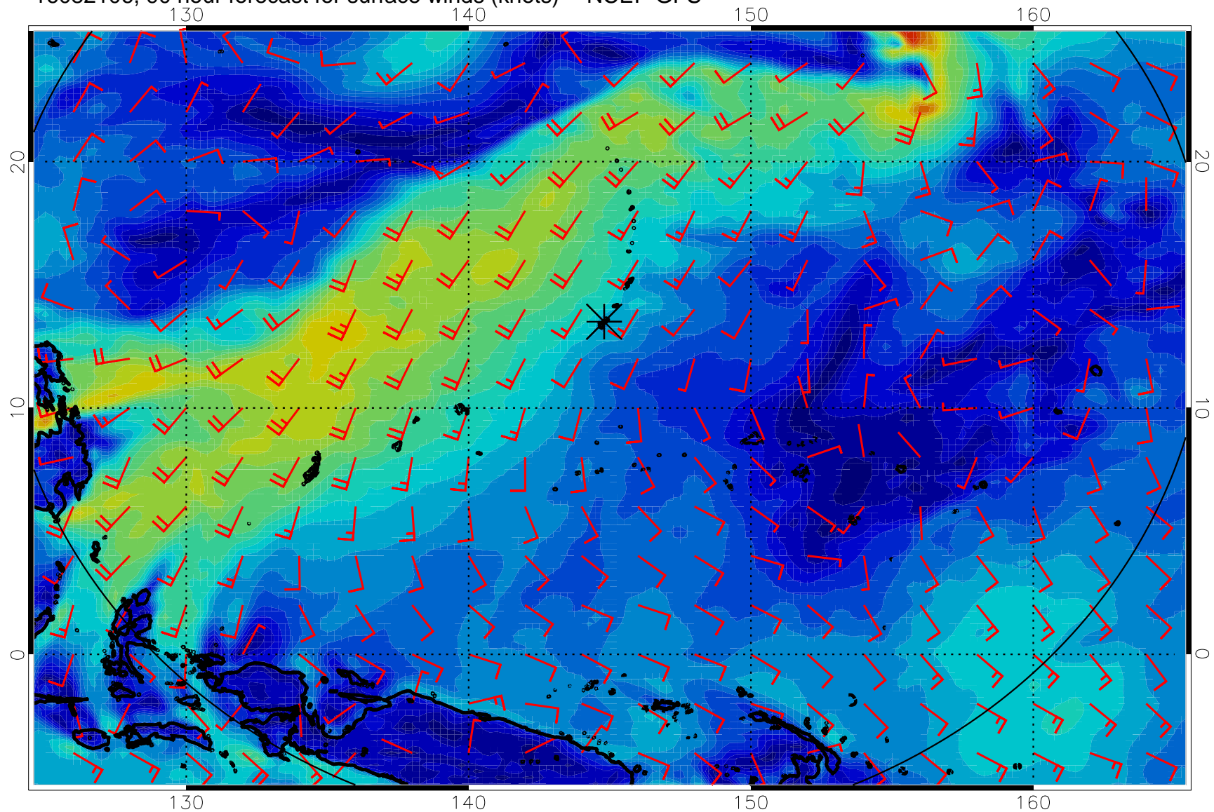
16082106, 90 hour forecast for surface winds (knots) -- NCEP GFS
