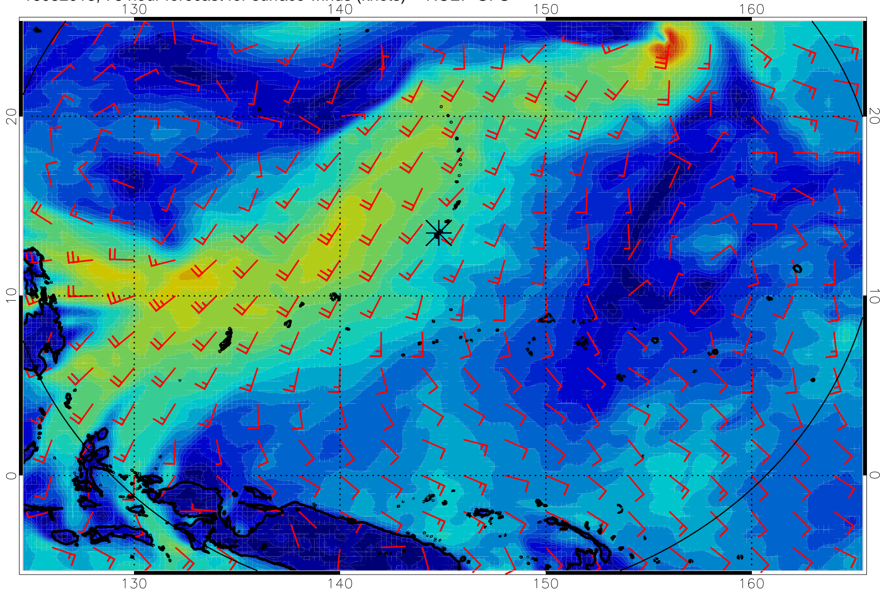
16082018, 78 hour forecast for surface winds (knots) -- NCEP GFS
