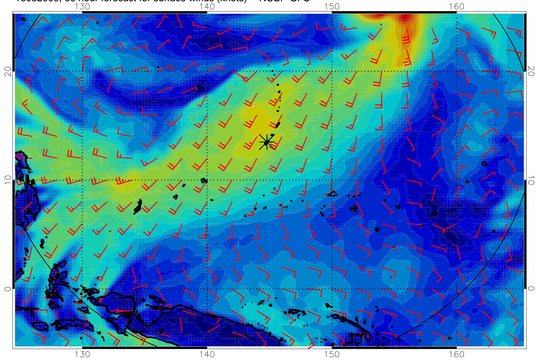
16082000, 60 hour forecast for surface winds (knots) -- NCEP GFS
