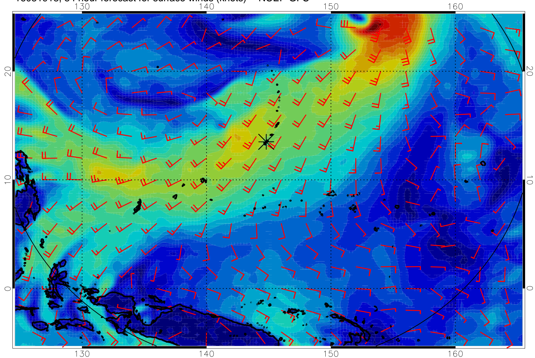
16081918, 54 hour forecast for surface winds (knots) -- NCEP GFS
