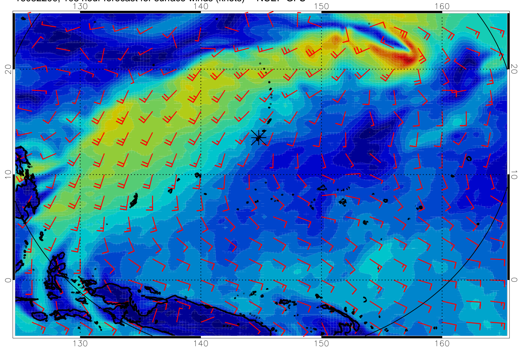
16082200, 108 hour forecast for surface winds (knots) -- NCEP GFS
