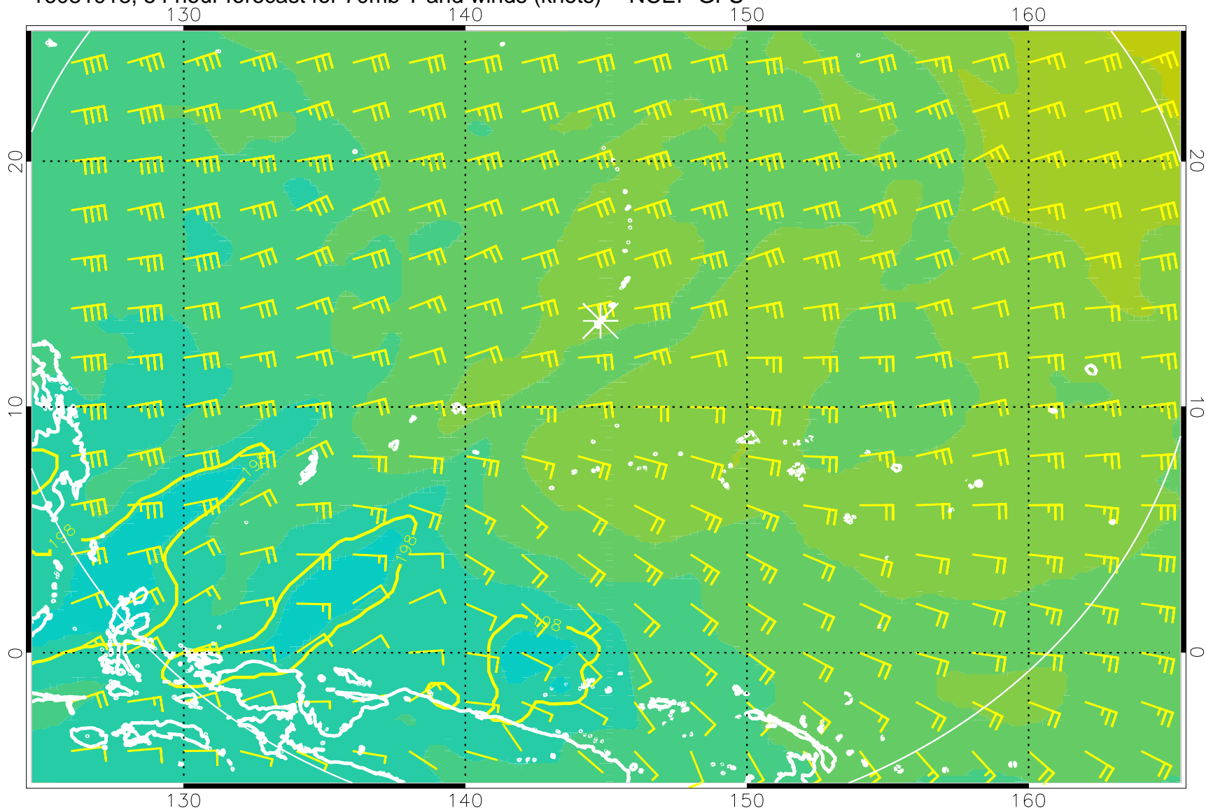
16081918, 54 hour forecast for 70mb T and winds (knots) -- NCEP GFS
