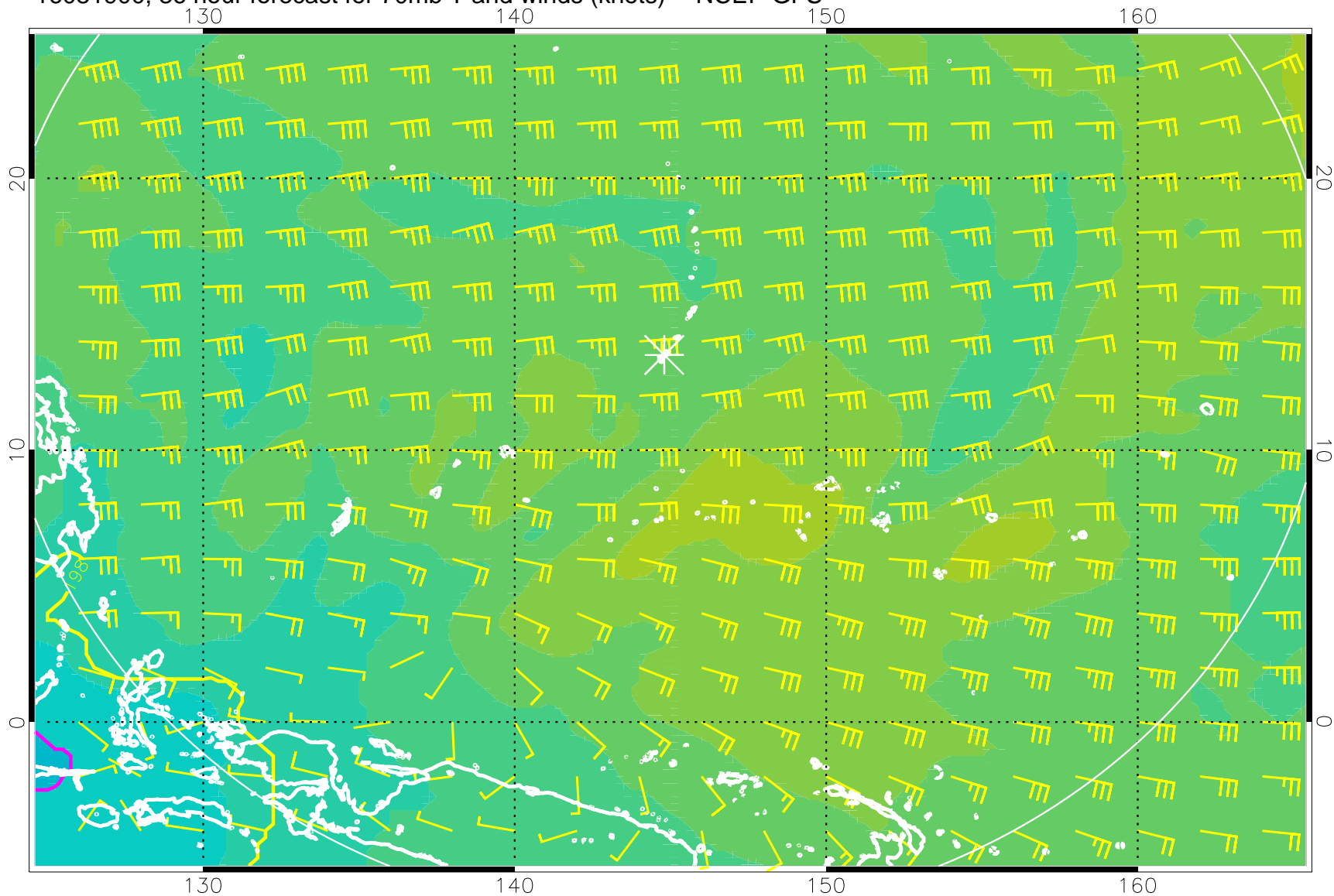
16081900, 36 hour forecast for 70mb T and winds (knots) -- NCEP GFS
