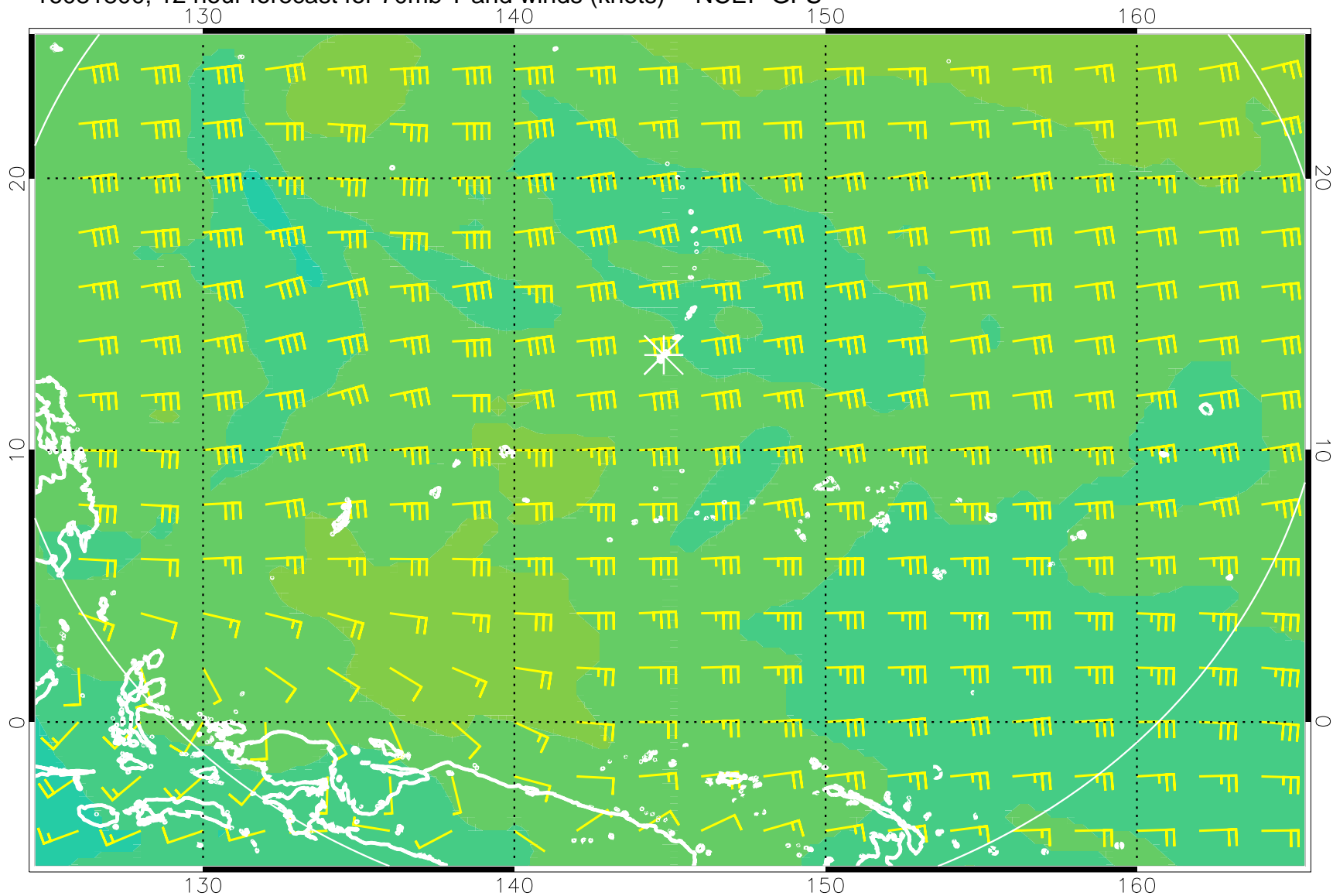
16081800, 12 hour forecast for 70mb T and winds (knots) -- NCEP GFS
