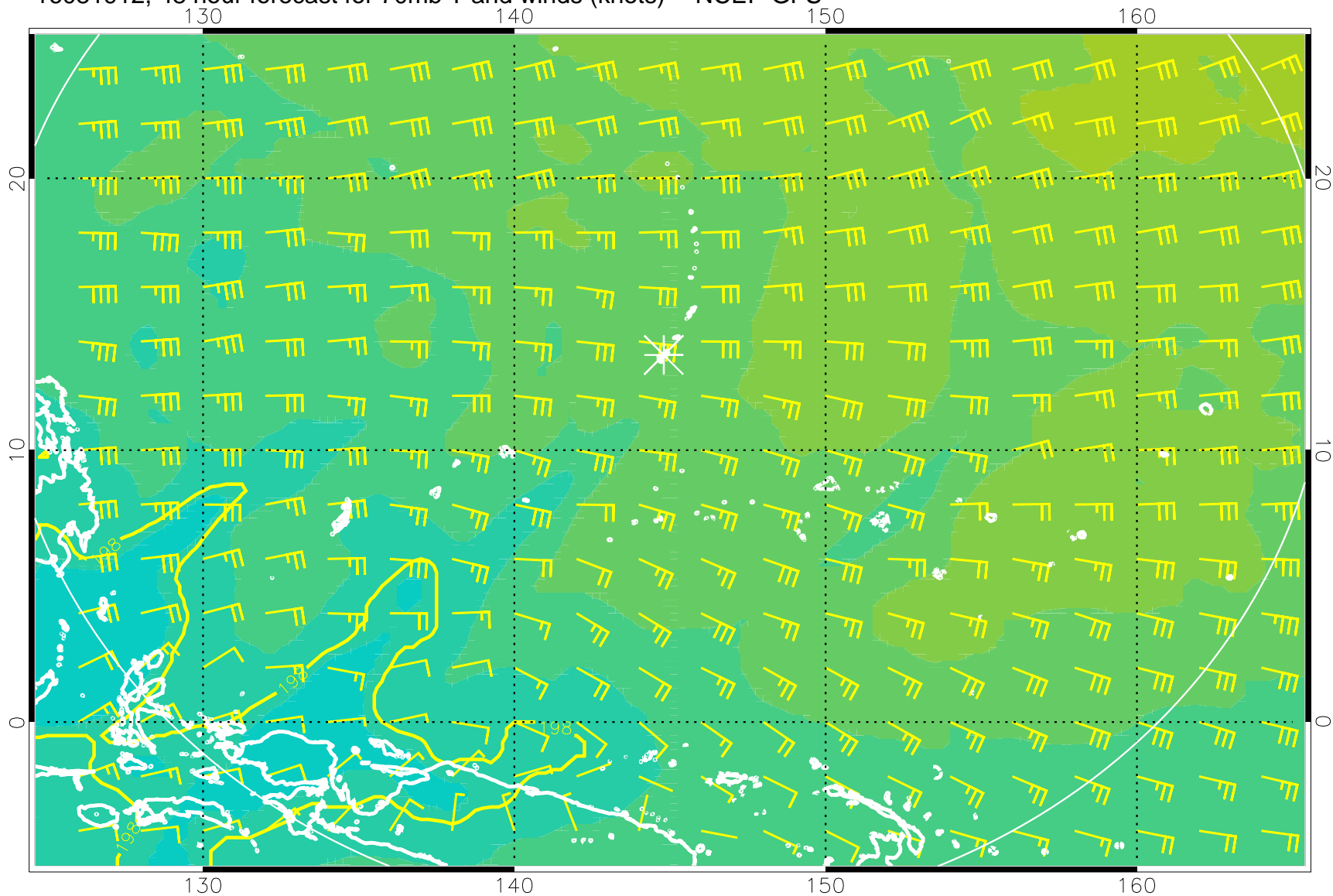
16081912, 48 hour forecast for 70mb T and winds (knots) -- NCEP GFS
