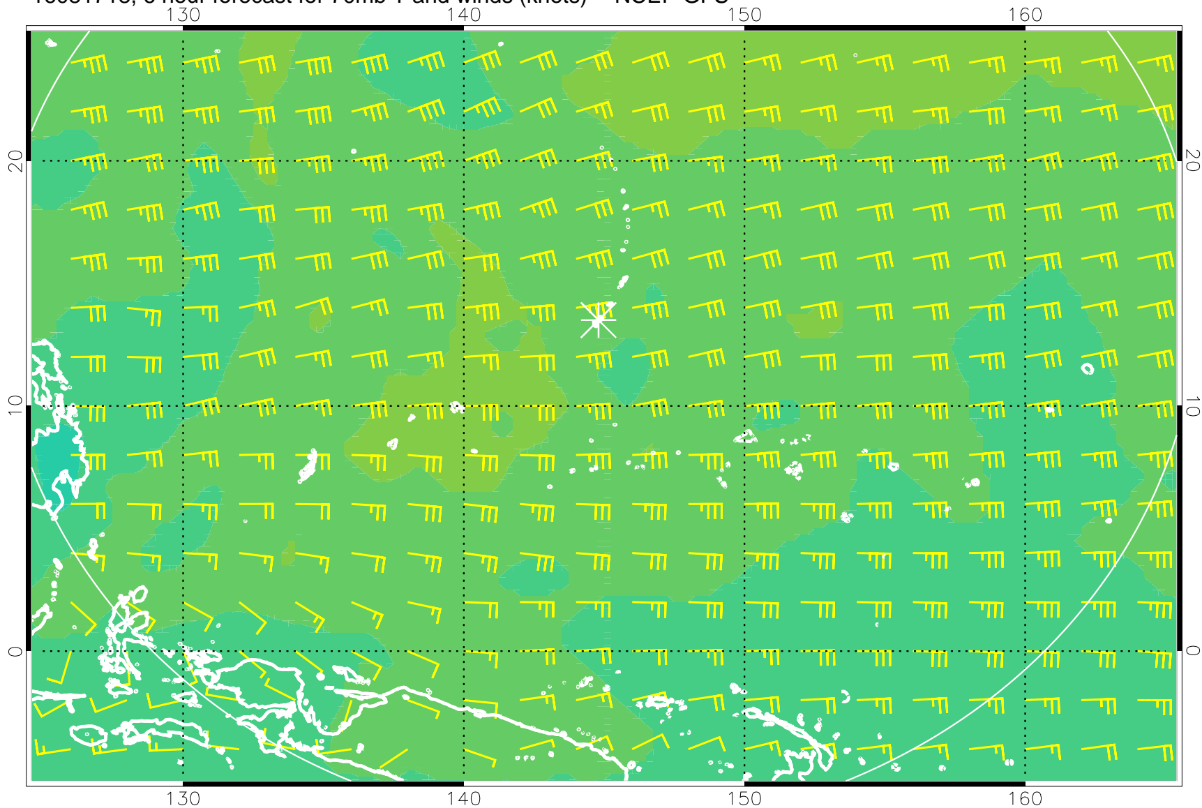
16081718, 6 hour forecast for 70mb T and winds (knots) -- NCEP GFS
