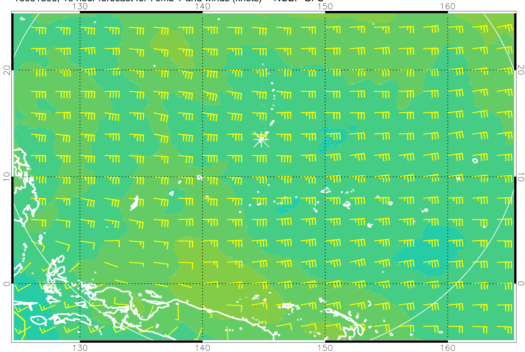
16081806, 18 hour forecast for 70mb T and winds (knots) -- NCEP GFS
