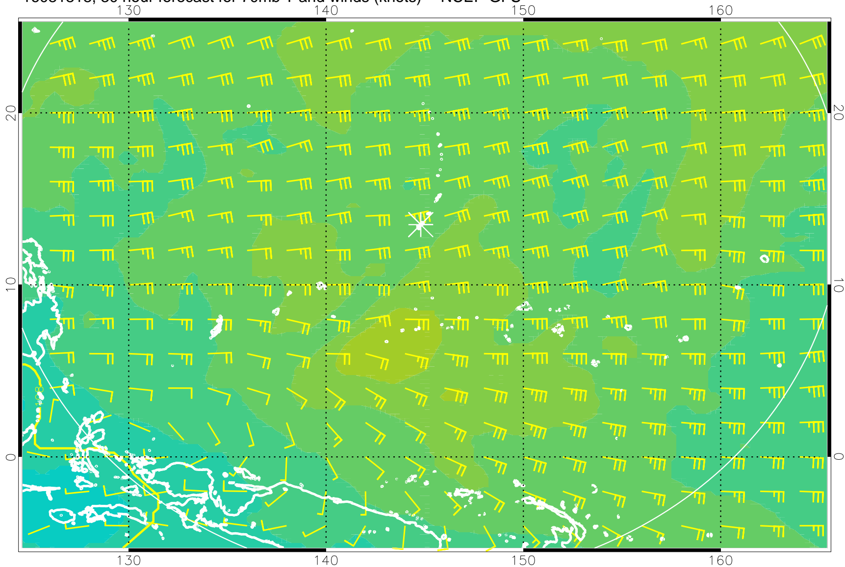
16081818, 30 hour forecast for 70mb T and winds (knots) -- NCEP GFS
