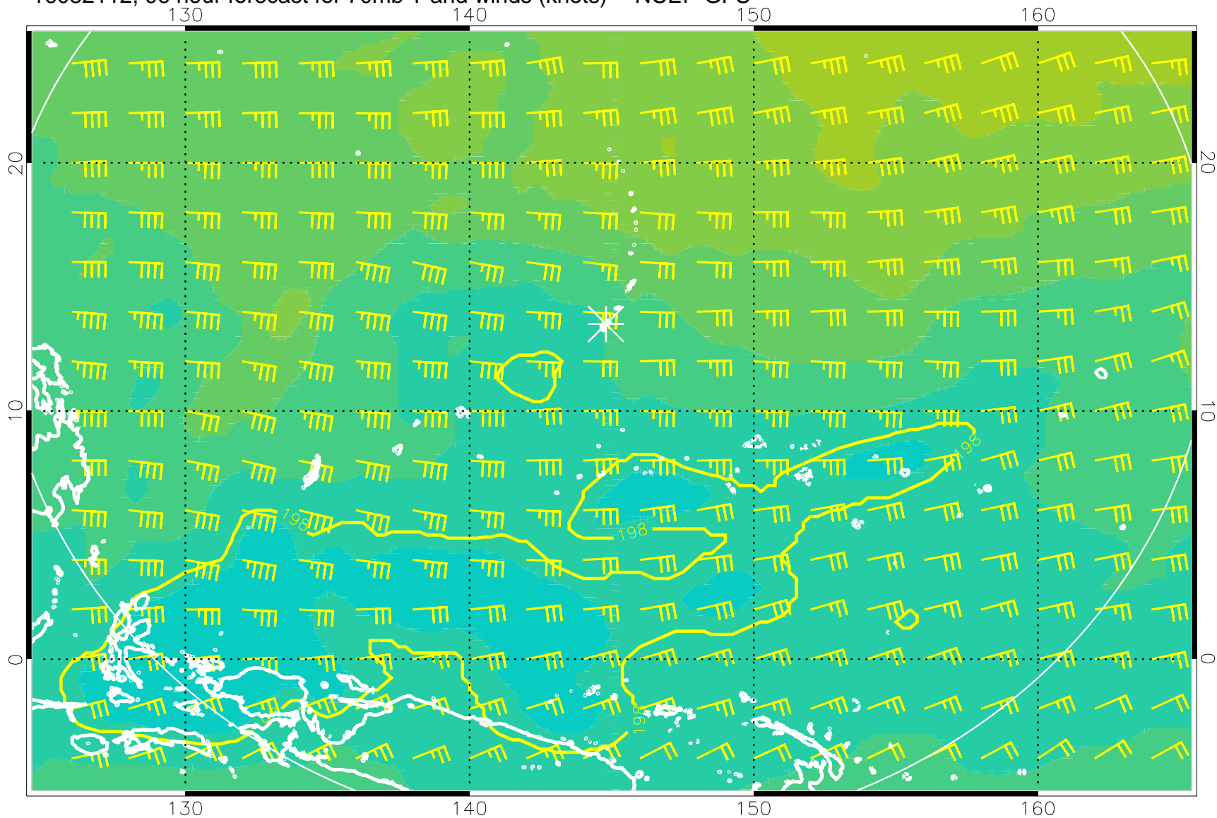
16082112, 96 hour forecast for 70mb T and winds (knots) -- NCEP GFS
