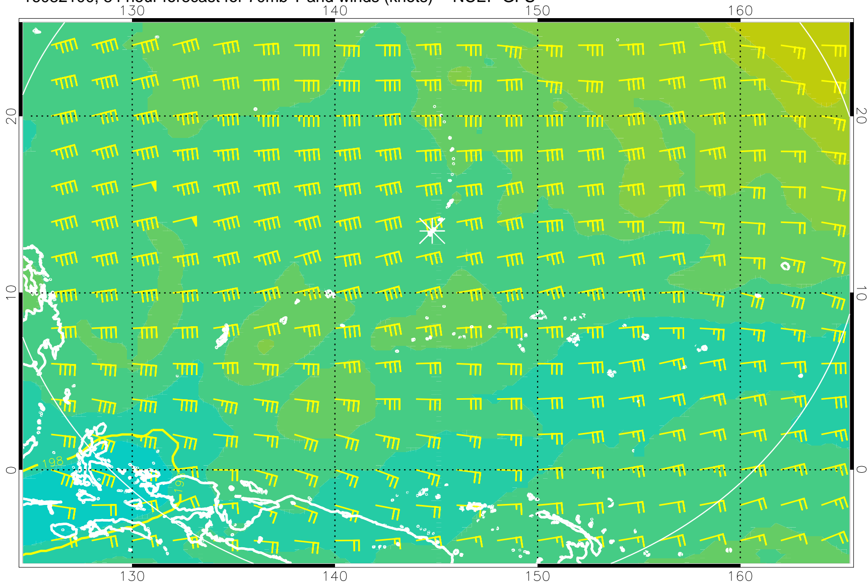
16082100, 84 hour forecast for 70mb T and winds (knots) -- NCEP GFS
