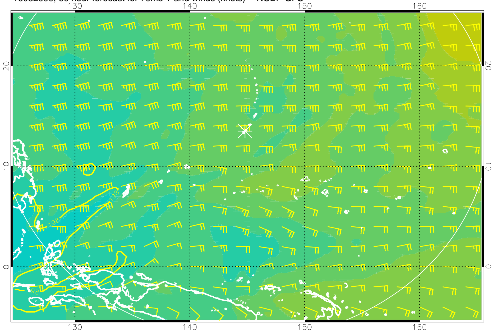
16082000, 60 hour forecast for 70mb T and winds (knots) -- NCEP GFS
