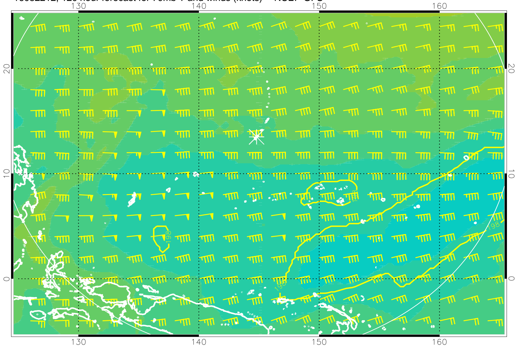
16082212, 120 hour forecast for 70mb T and winds (knots) -- NCEP GFS
