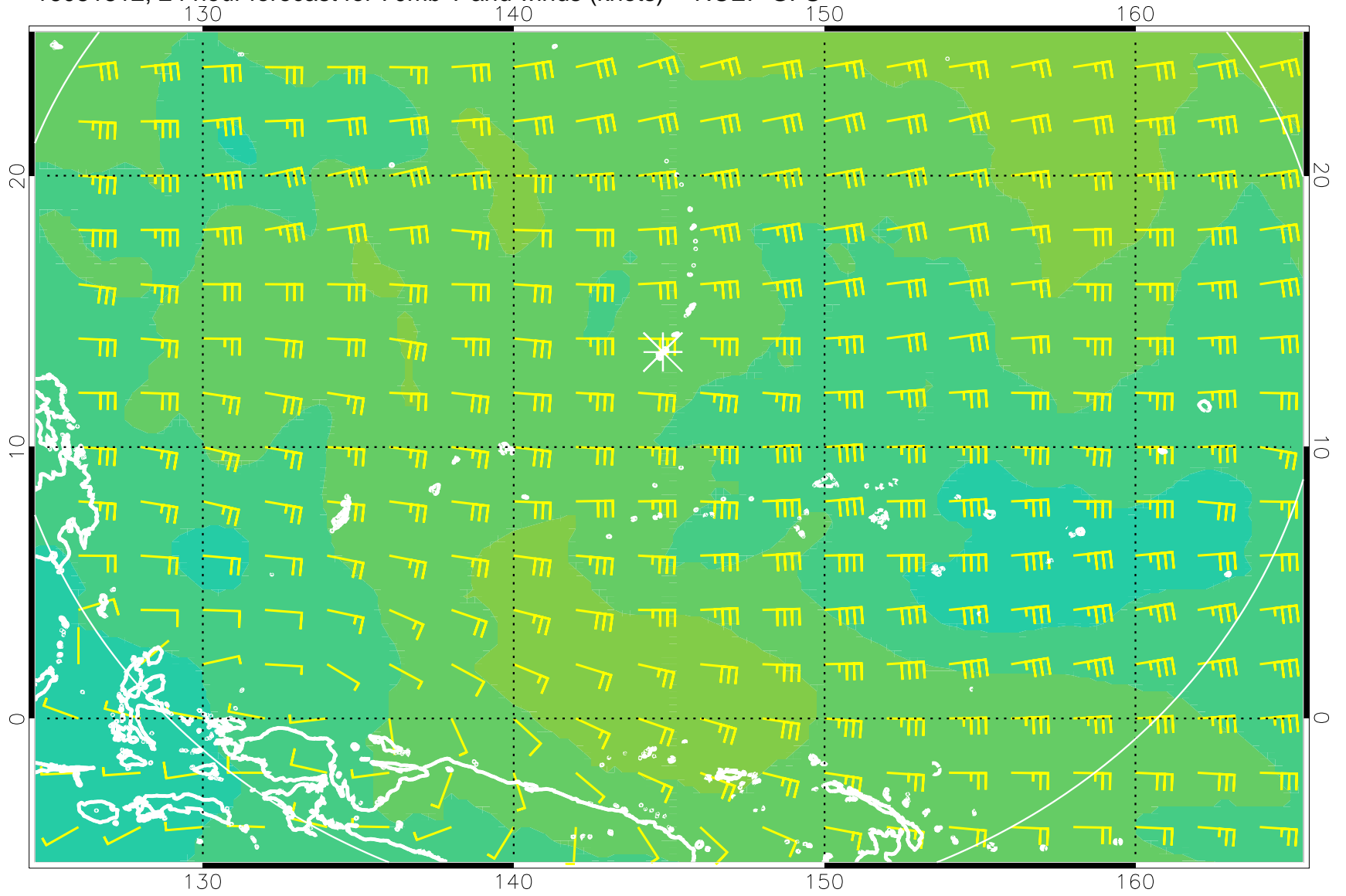
16081812, 24 hour forecast for 70mb T and winds (knots) -- NCEP GFS
