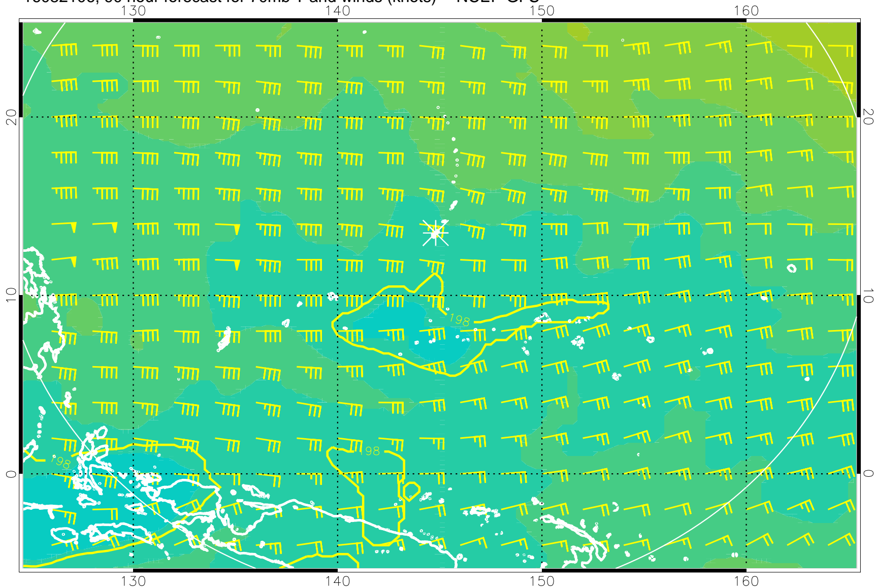
16082106, 90 hour forecast for 70mb T and winds (knots) -- NCEP GFS
