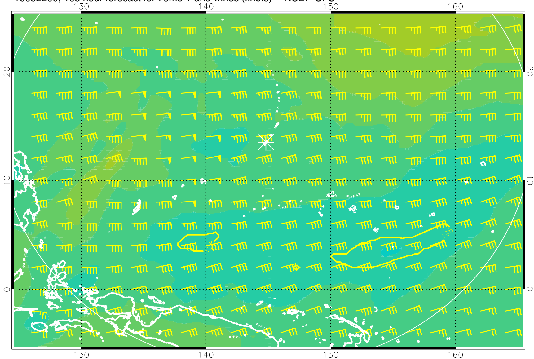
16082200, 108 hour forecast for 70mb T and winds (knots) -- NCEP GFS
