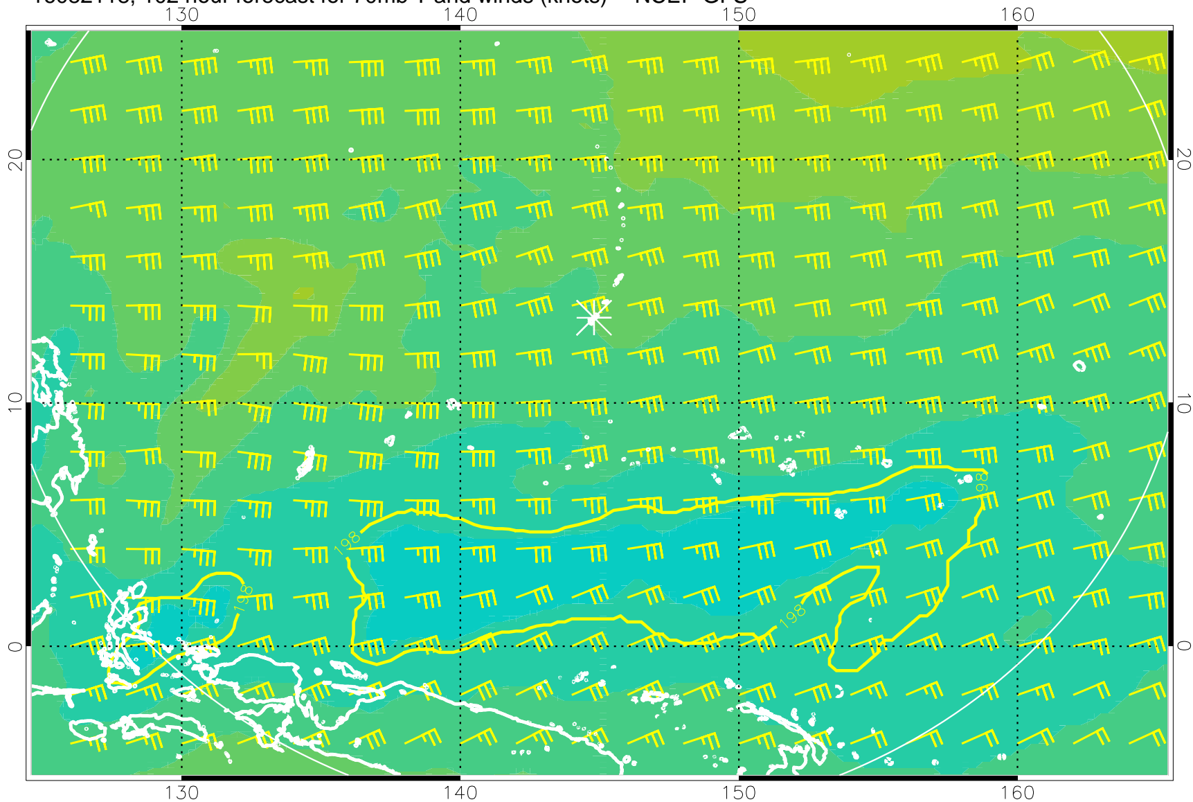
16082118, 102 hour forecast for 70mb T and winds (knots) -- NCEP GFS
