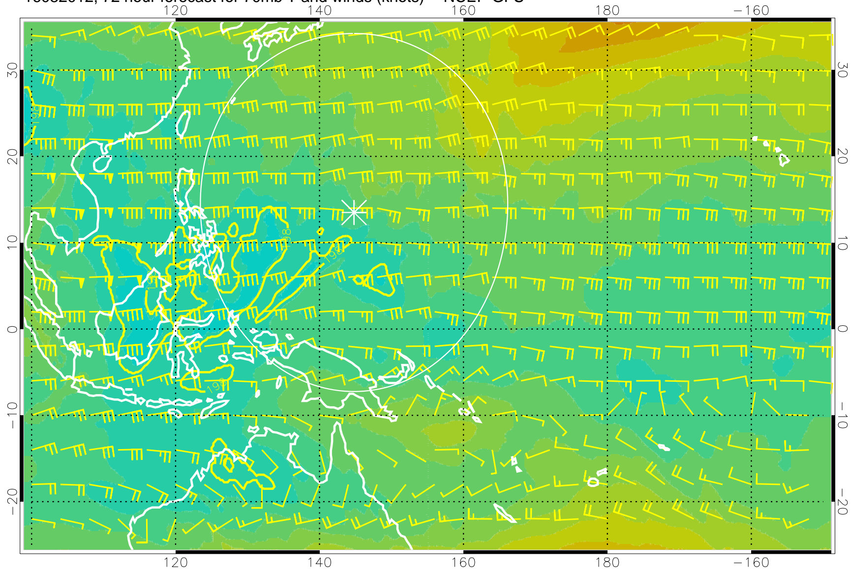
16082012, 72 hour forecast for 70mb T and winds (knots) -- NCEP GFS
