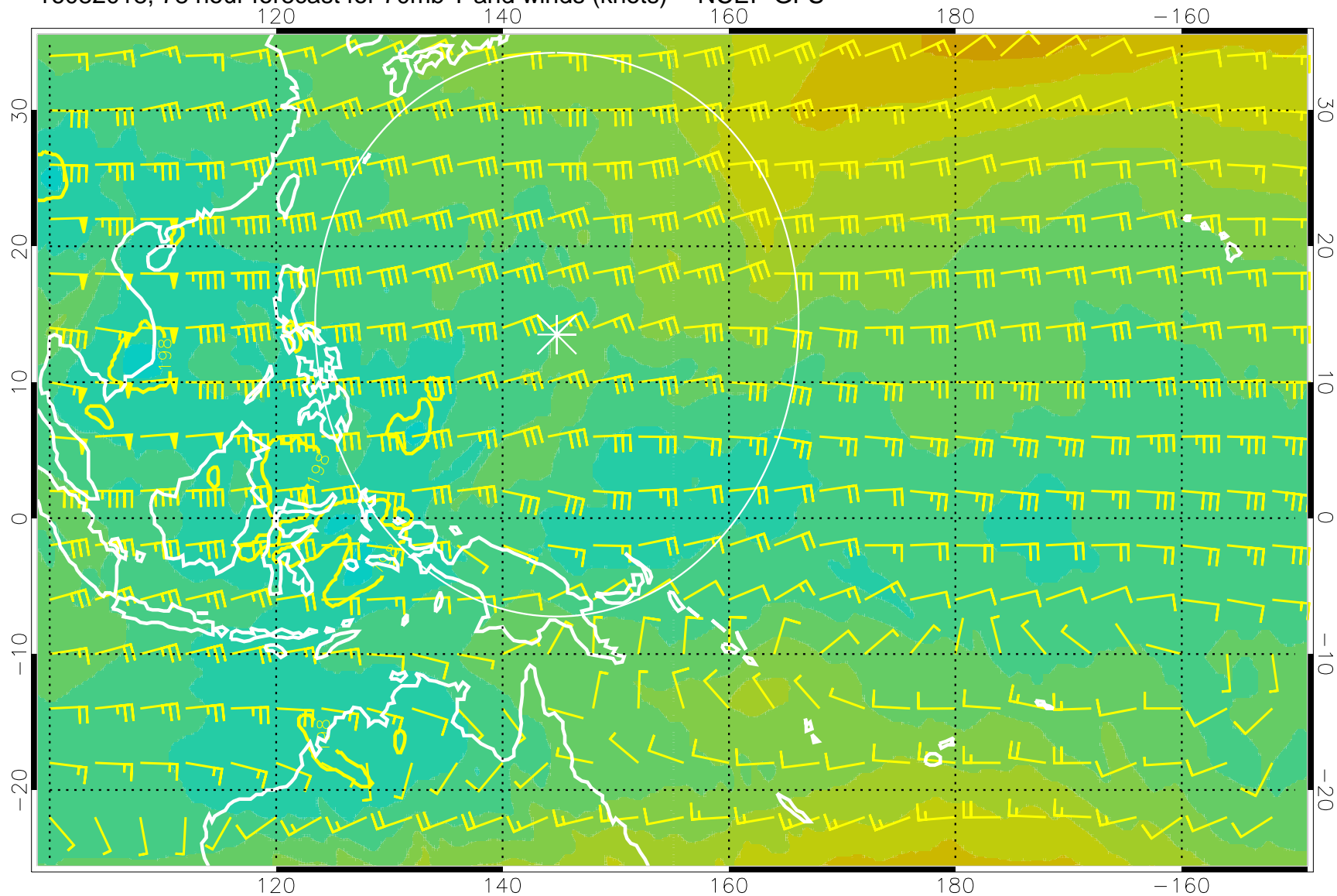
16082018, 78 hour forecast for 70mb T and winds (knots) -- NCEP GFS
