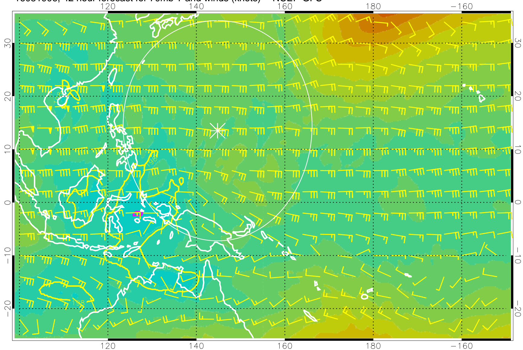
16081906, 42 hour forecast for 70mb T and winds (knots) -- NCEP GFS
