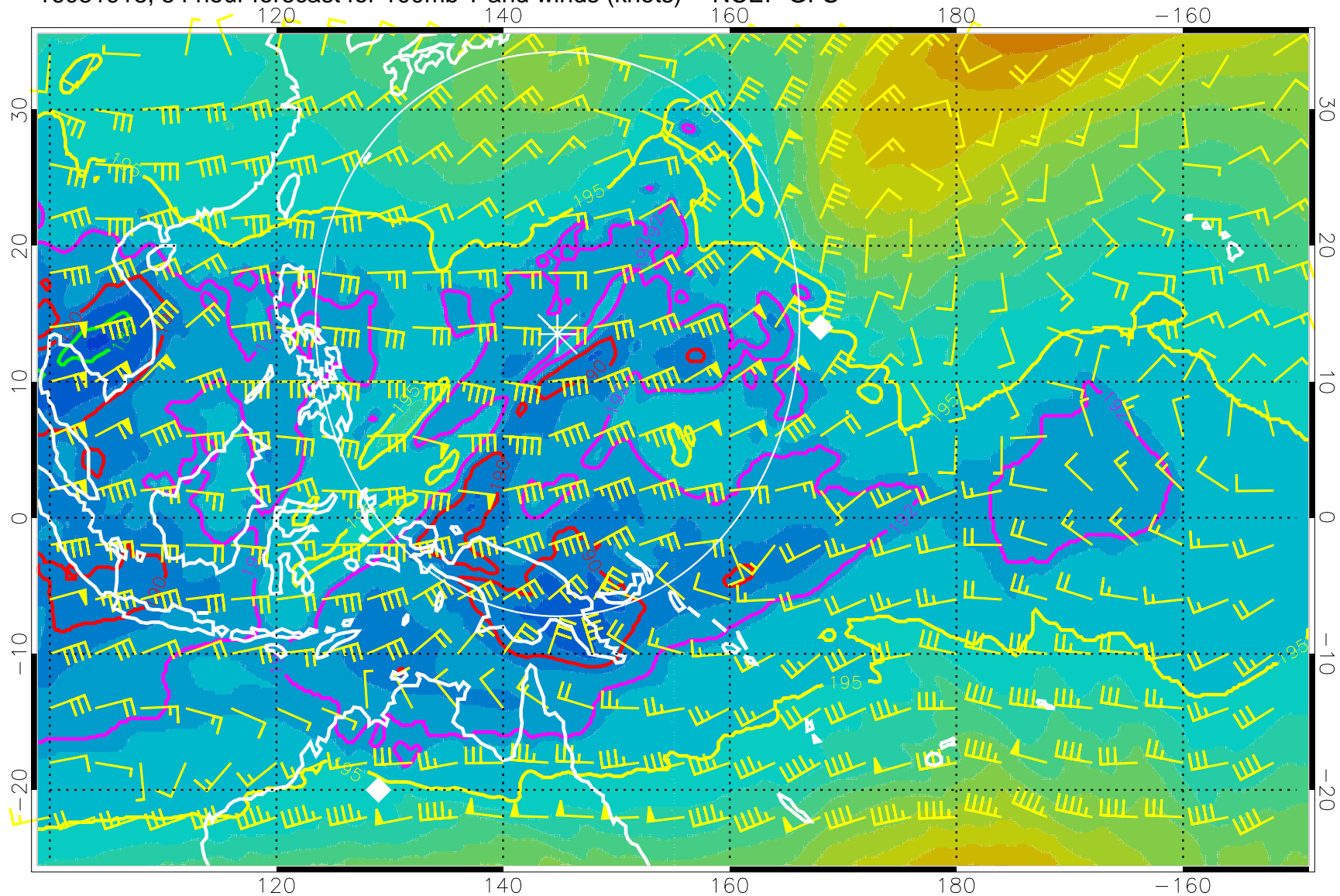
16081918, 54 hour forecast for 100mb T and winds (knots) -- NCEP GFS
