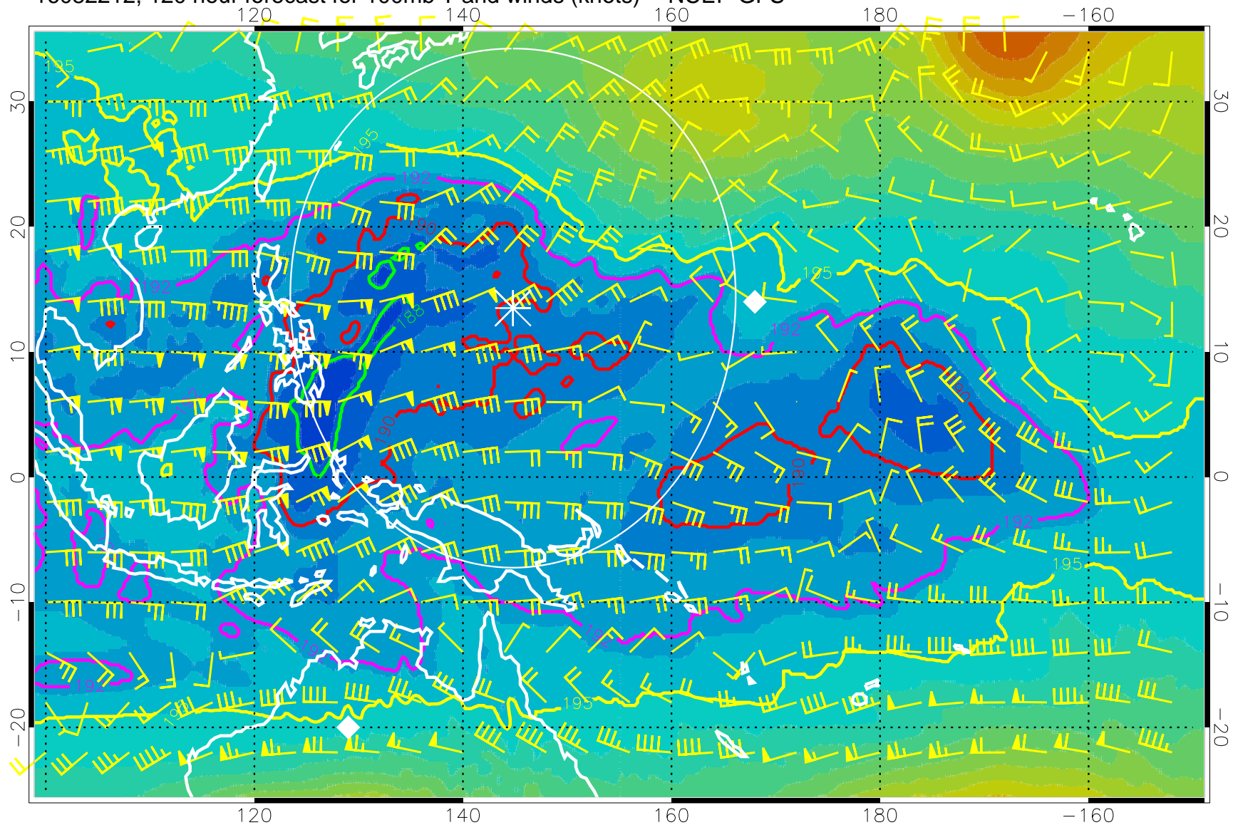
16082212, 120 hour forecast for 100mb T and winds (knots) -- NCEP GFS
