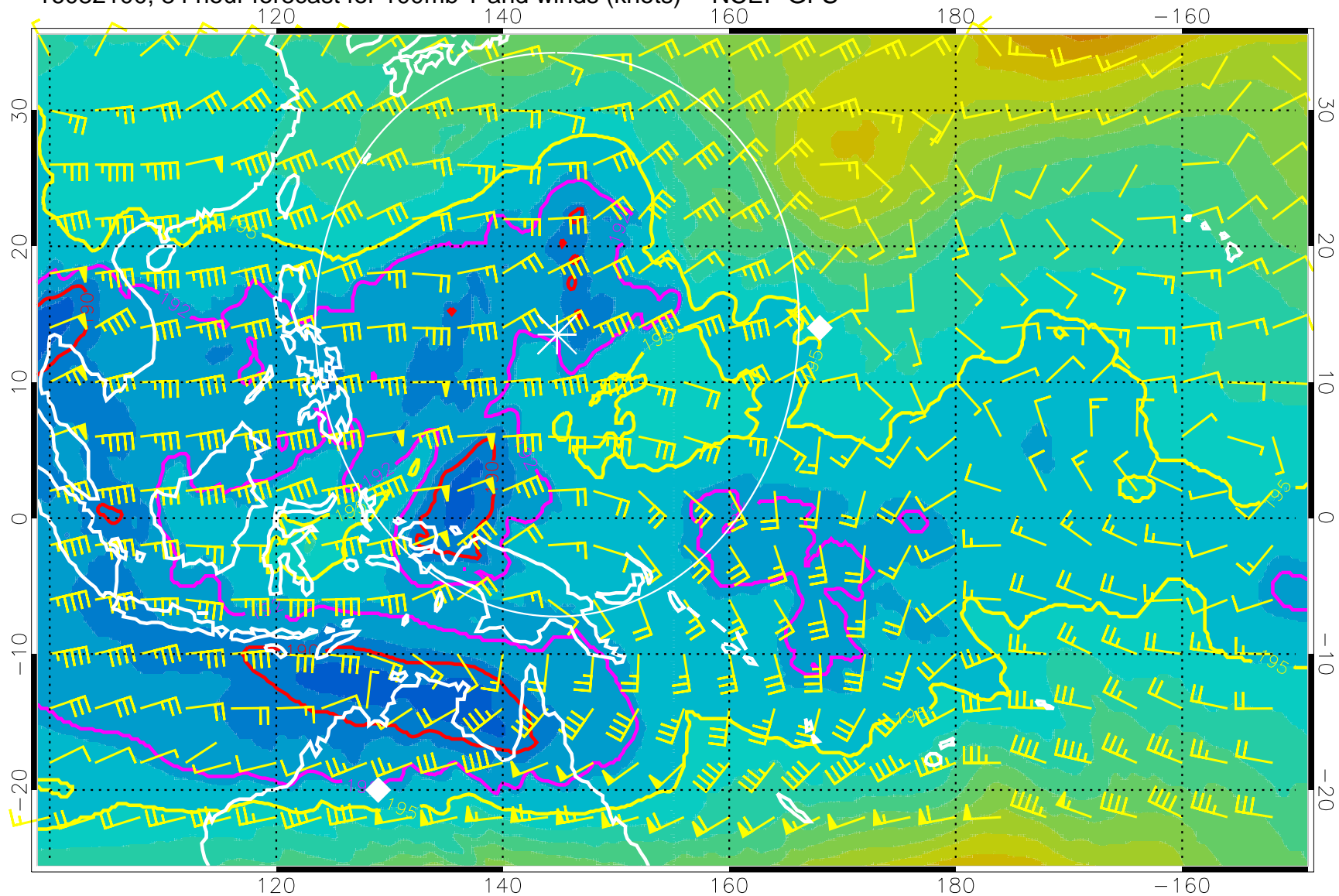
16082100, 84 hour forecast for 100mb T and winds (knots) -- NCEP GFS
