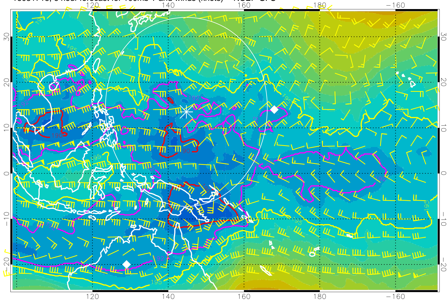
16081718, 6 hour forecast for 100mb T and winds (knots) -- NCEP GFS
