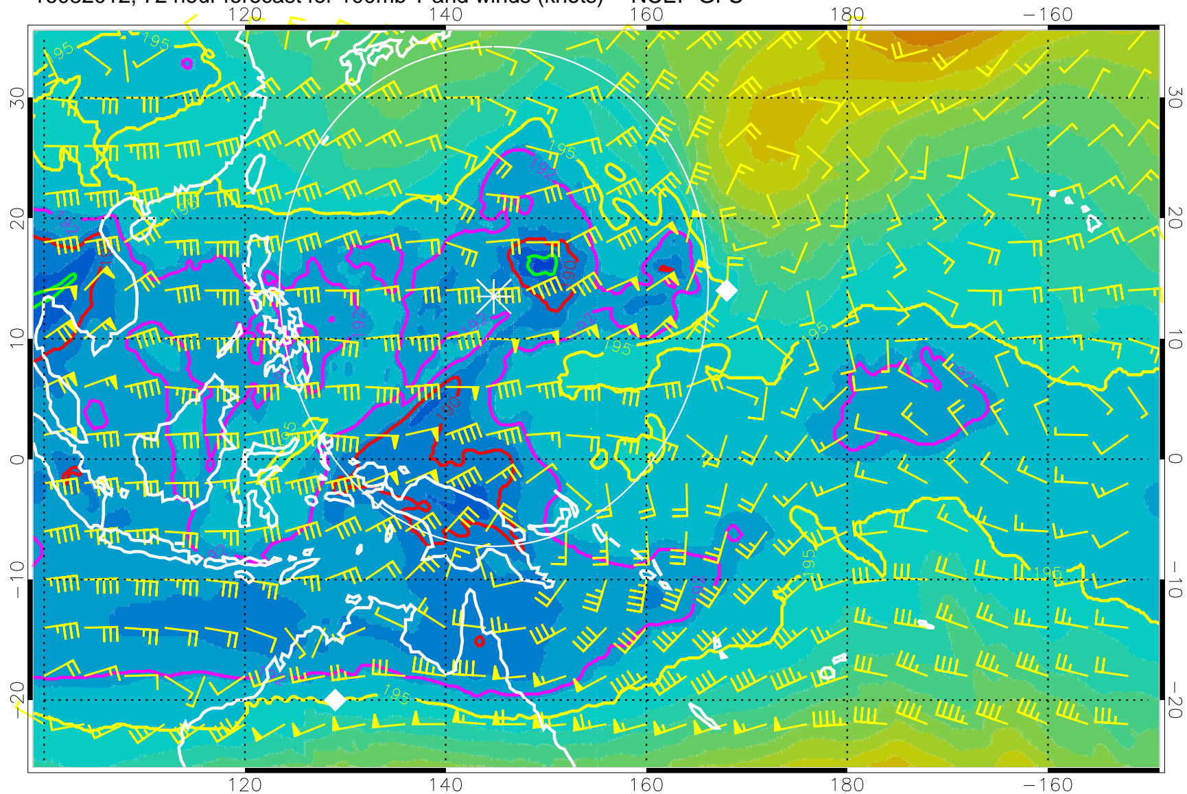
16082012, 72 hour forecast for 100mb T and winds (knots) -- NCEP GFS
