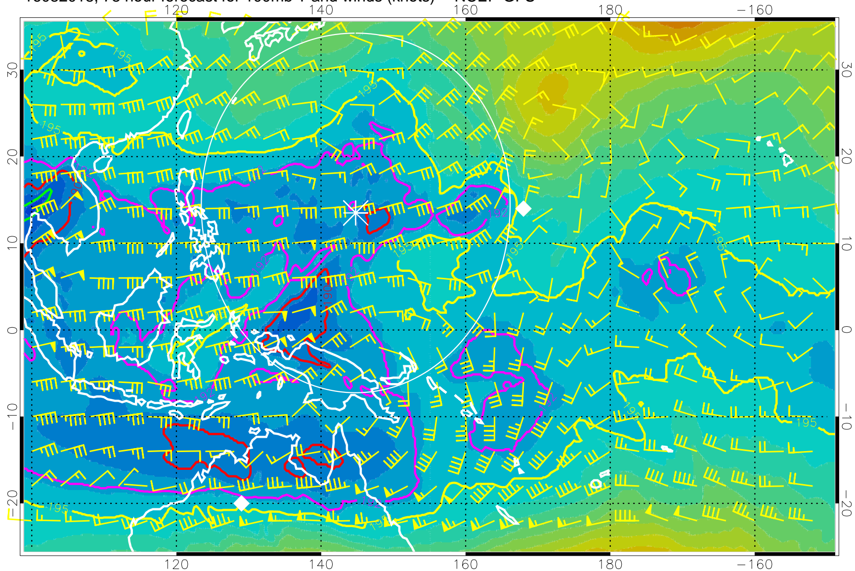
16082018, 78 hour forecast for 100mb T and winds (knots) -- NCEP GFS
