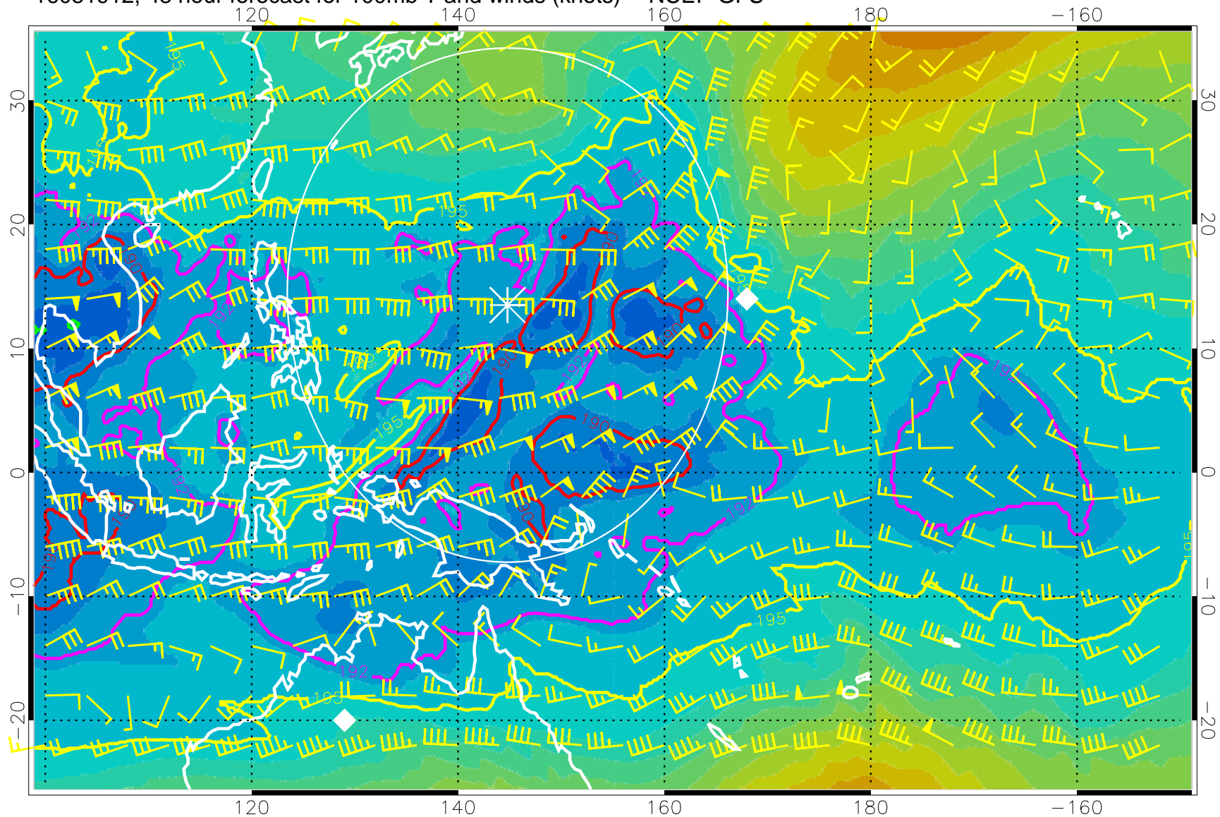
16081912, 48 hour forecast for 100mb T and winds (knots) -- NCEP GFS
