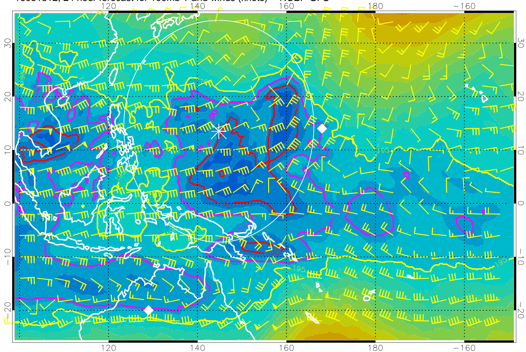
16081812, 24 hour forecast for 100mb T and winds (knots) -- NCEP GFS
