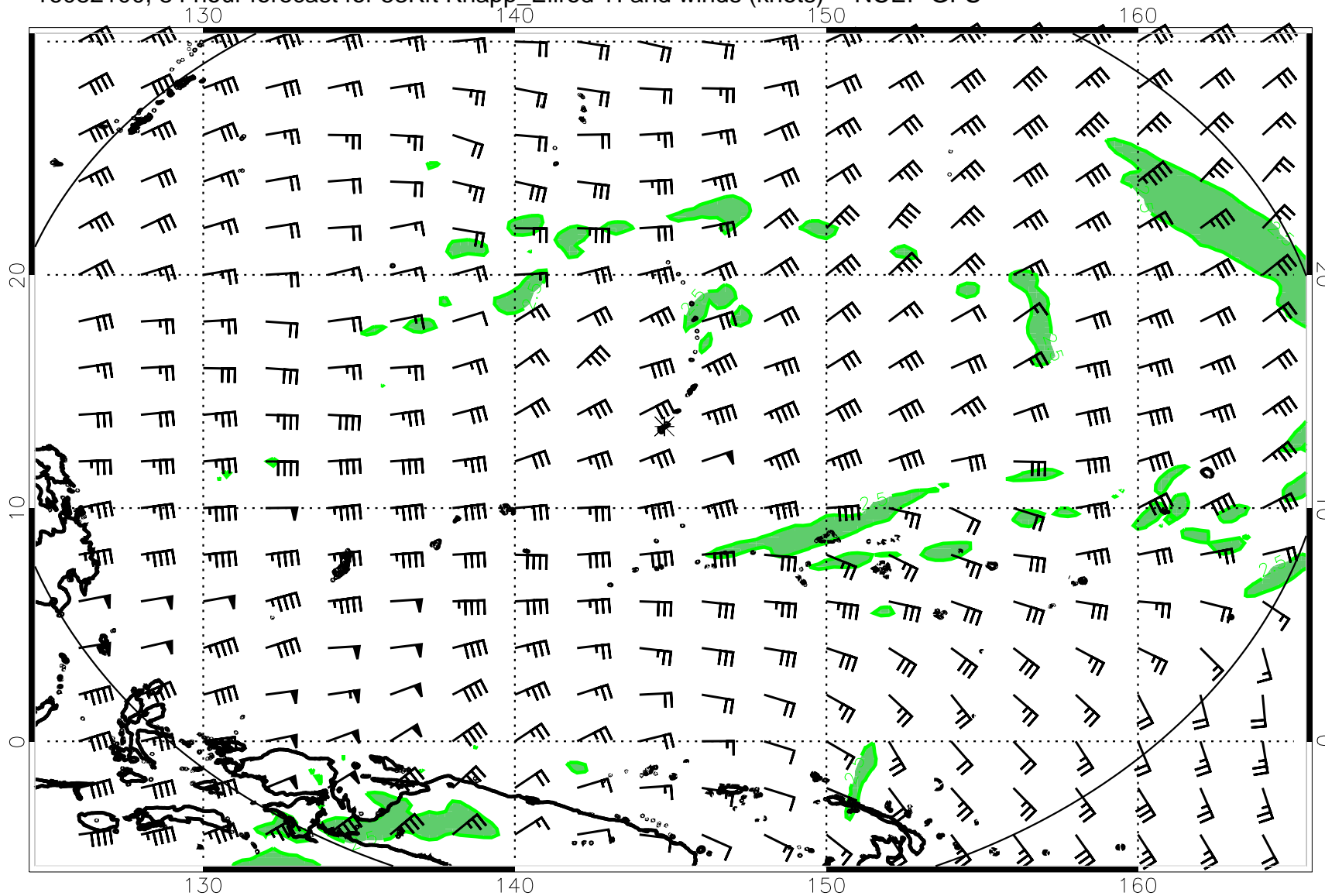
16082100, 84 hour forecast for 53Kft Knapp_Ellrod TI and winds (knots) -- NCEP GFS
