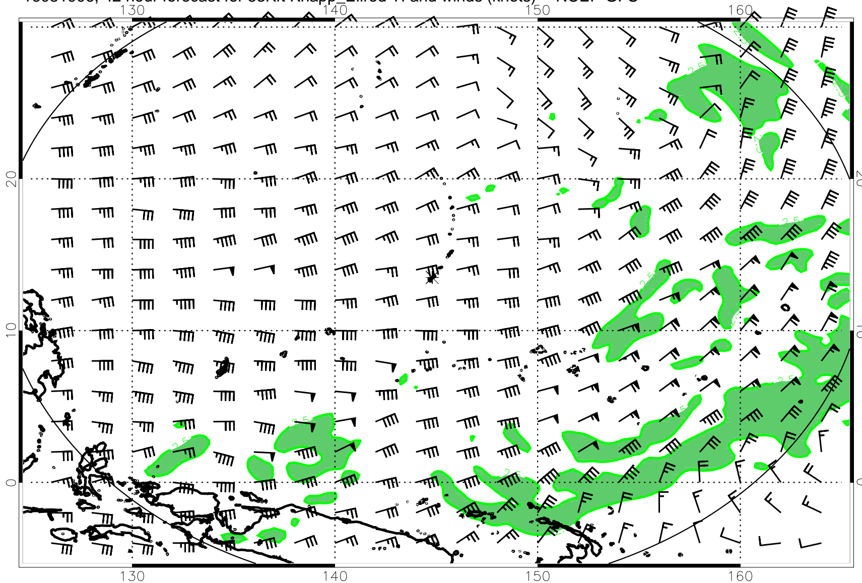
16081906, 42 hour forecast for 53Kft Knapp_Ellrod TI and winds (knots) -- NCEP GFS
