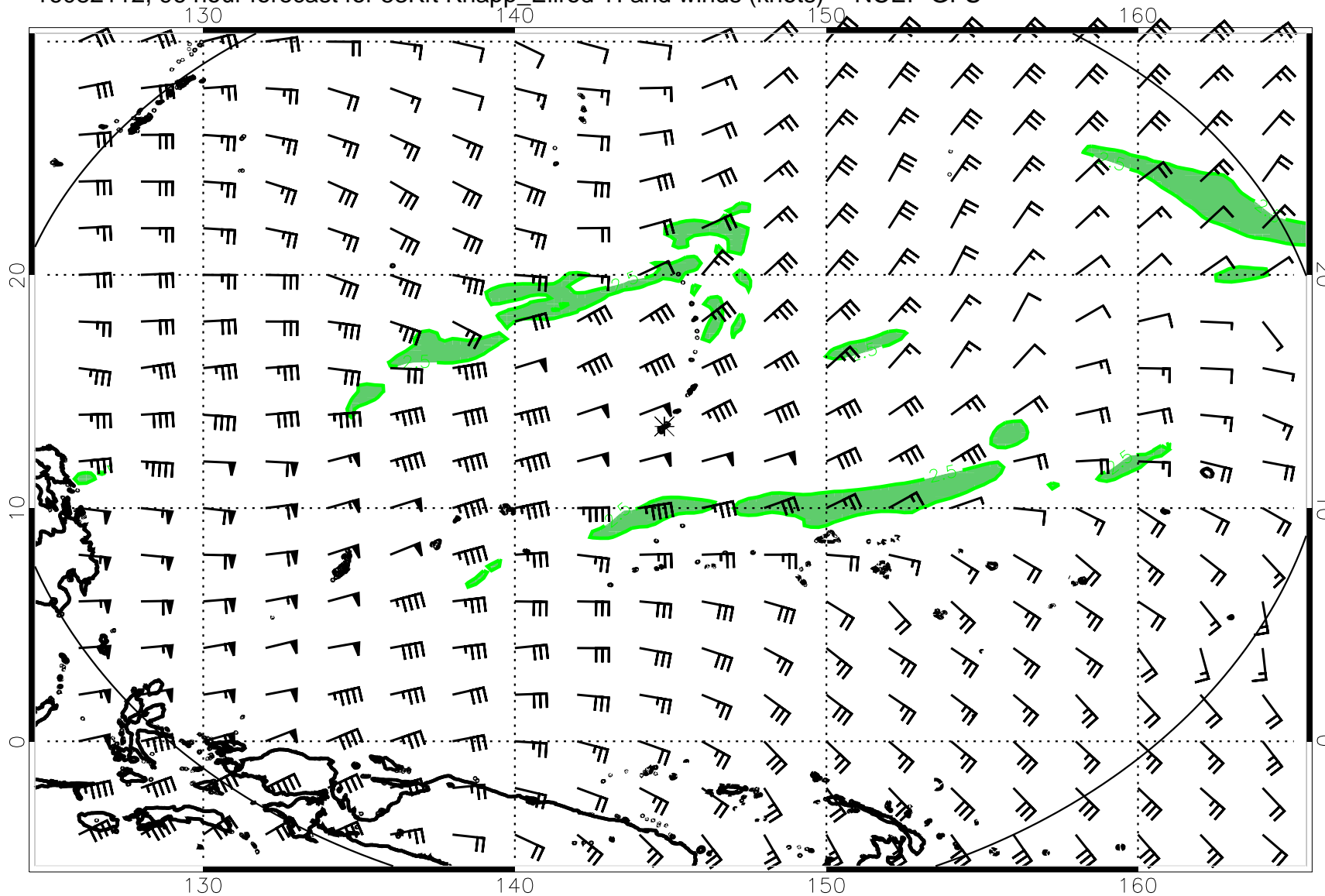
16082112, 96 hour forecast for 53Kft Knapp_Ellrod TI and winds (knots) -- NCEP GFS
