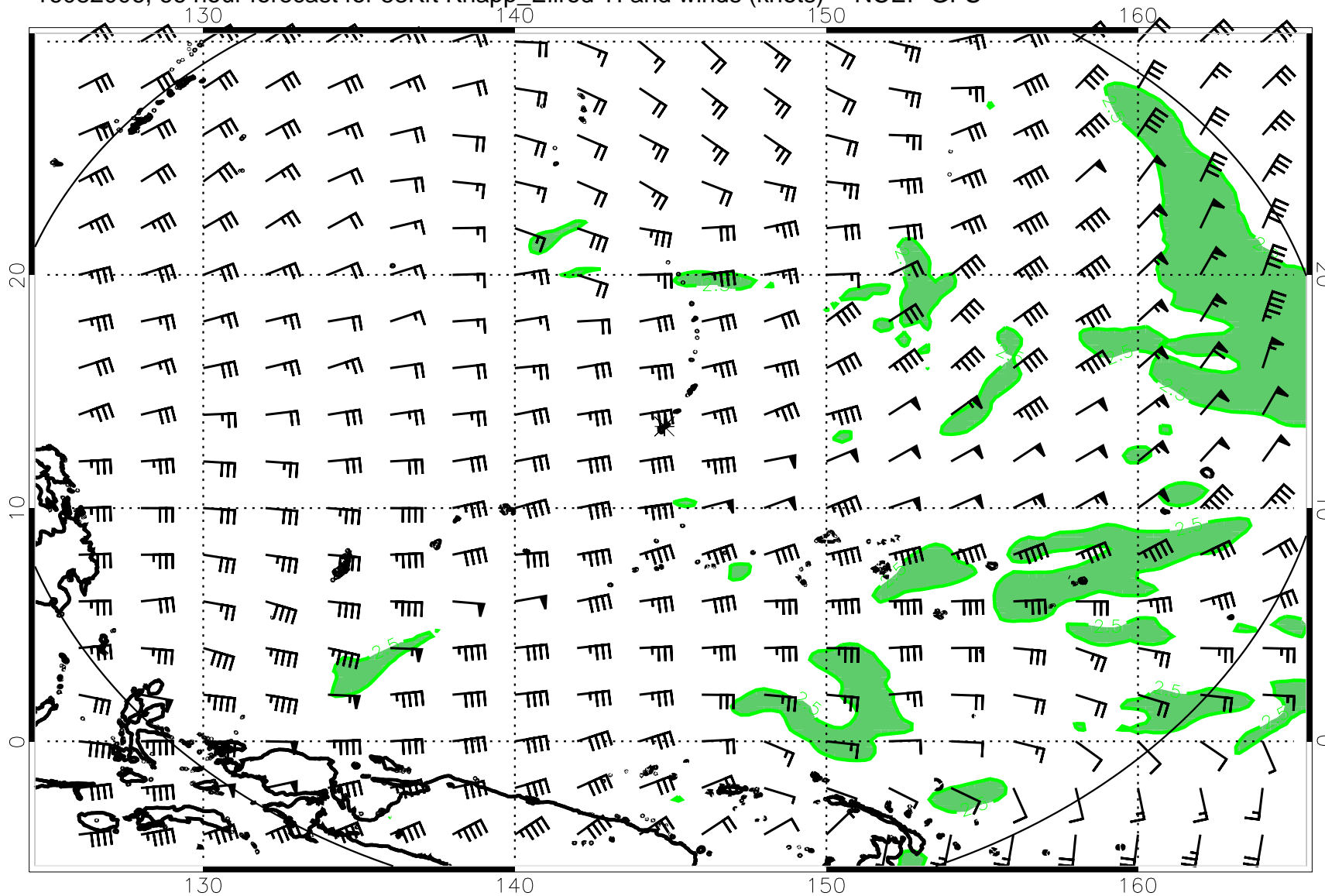
16082006, 66 hour forecast for 53Kft Knapp_Ellrod TI and winds (knots) -- NCEP GFS
