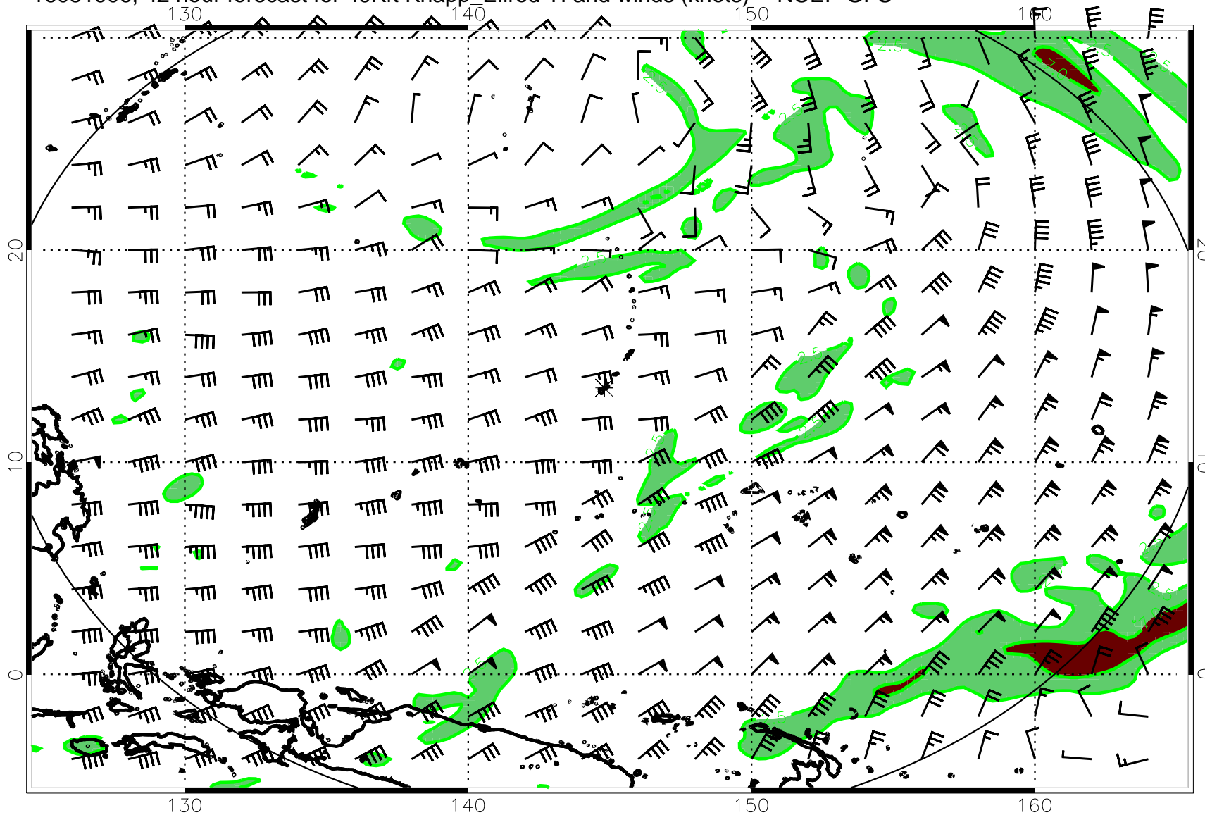
16081906, 42 hour forecast for 49Kft Knapp_Ellrod TI and winds (knots) -- NCEP GFS
