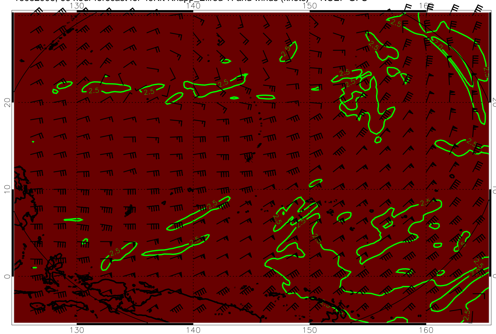
16082006, 66 hour forecast for 49Kft Knapp_Ellrod TI and winds (knots) -- NCEP GFS
