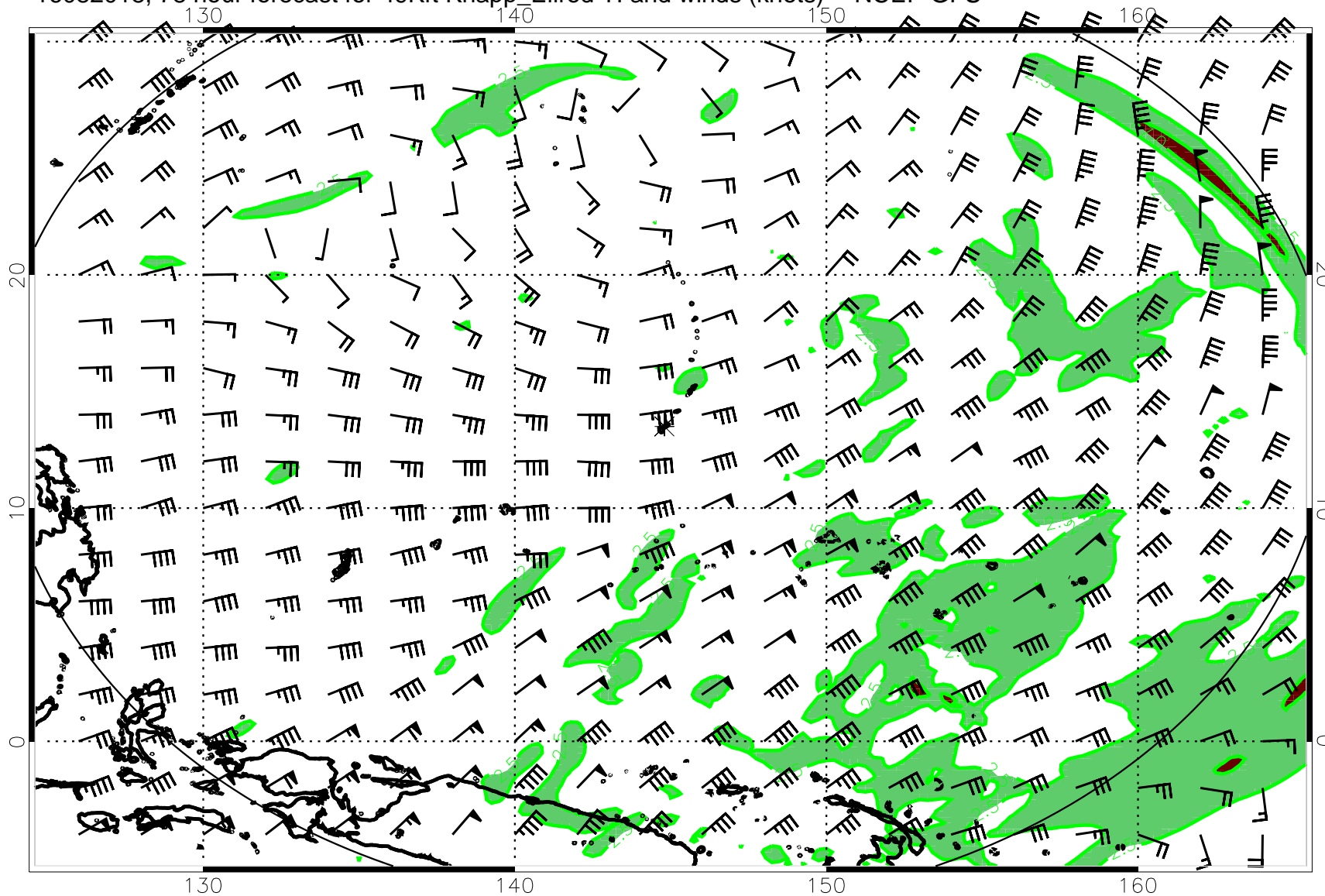
16082018, 78 hour forecast for 49Kft Knapp_Ellrod TI and winds (knots) -- NCEP GFS
