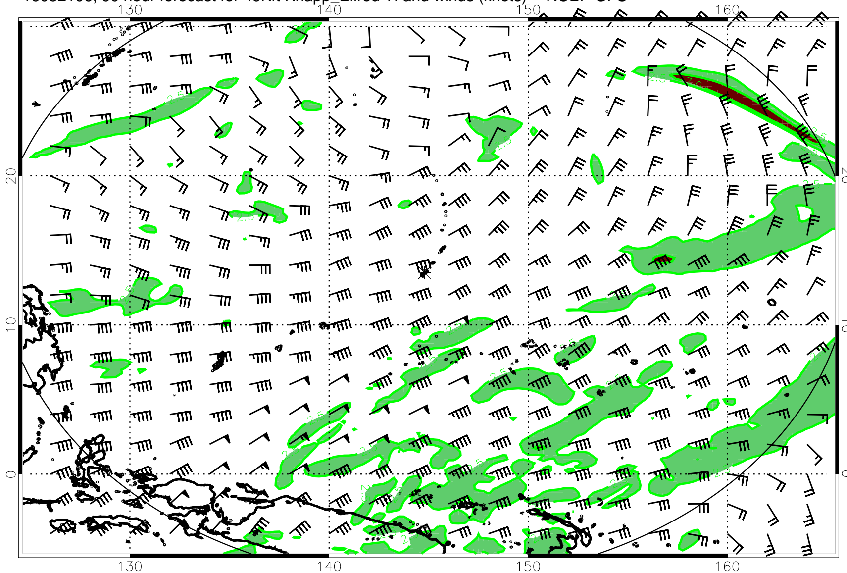
16082106, 90 hour forecast for 49Kft Knapp_Ellrod TI and winds (knots) -- NCEP GFS
