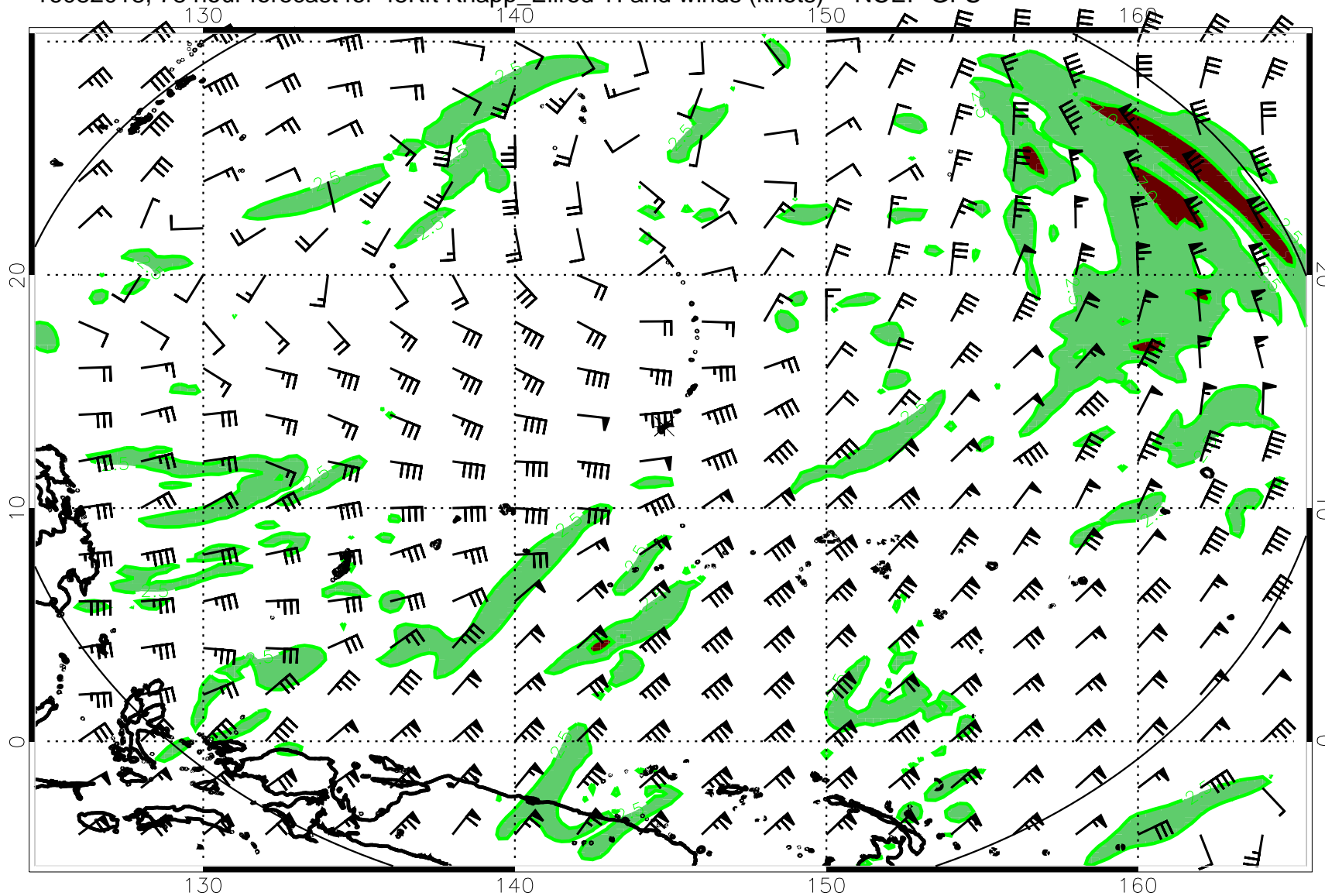
16082018, 78 hour forecast for 45Kft Knapp_Ellrod TI and winds (knots) -- NCEP GFS
