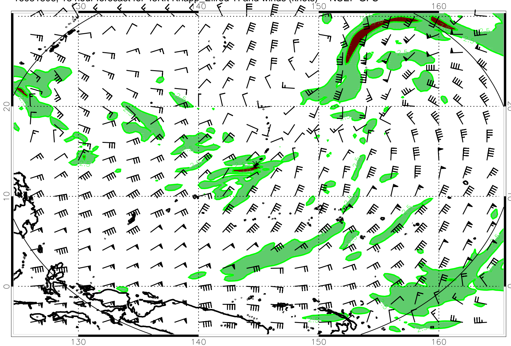
16081806, 18 hour forecast for 45Kft Knapp_Ellrod TI and winds (knots) -- NCEP GFS
