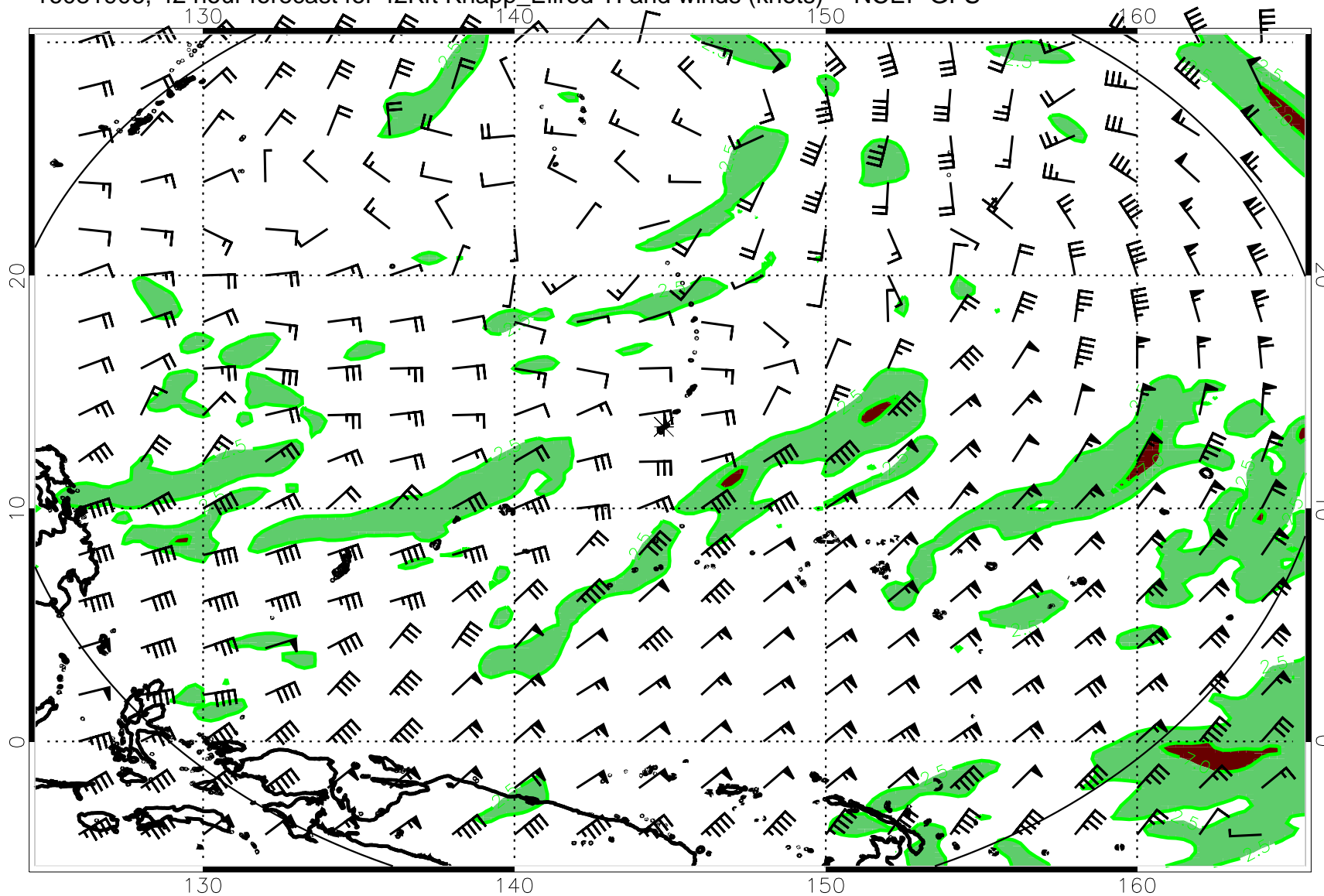
16081906, 42 hour forecast for 42Kft Knapp_Ellrod TI and winds (knots) -- NCEP GFS
