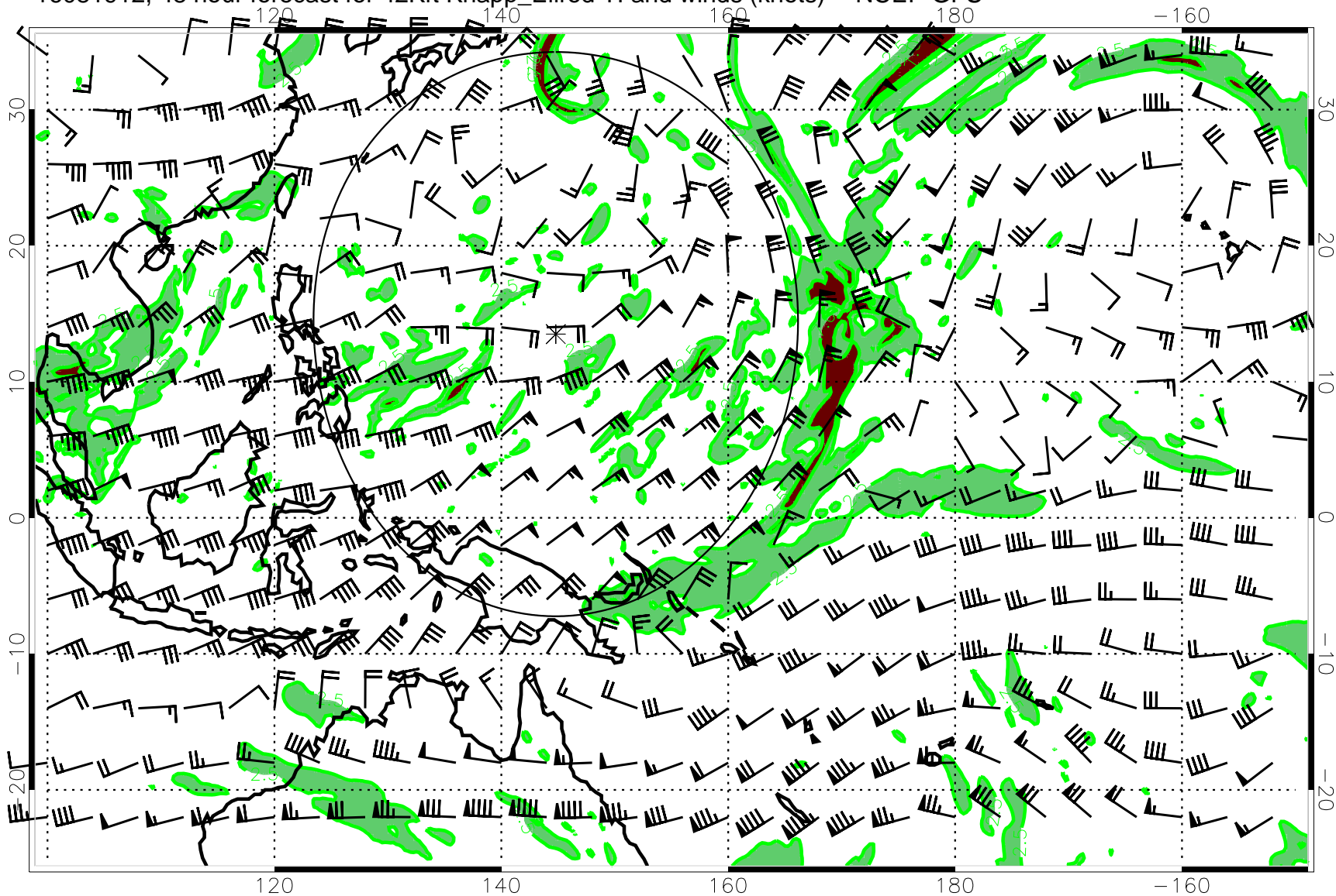
16081912, 48 hour forecast for 42Kft Knapp_Ellrod TI and winds (knots) -- NCEP GFS
