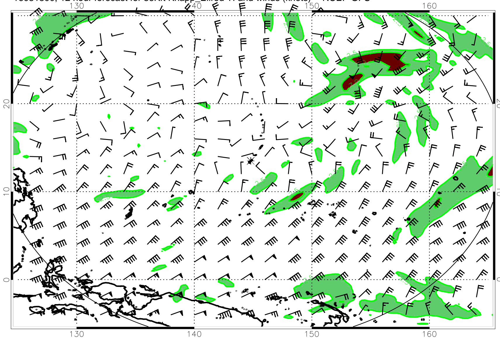
16081800, 12 hour forecast for 36Kft Knapp_Ellrod TI and winds (knots) -- NCEP GFS
