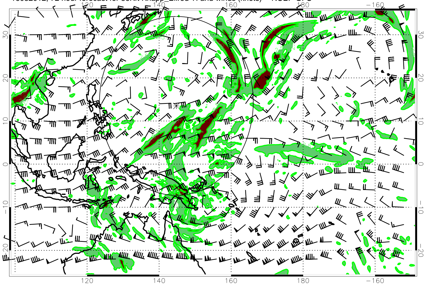
16082012, 72 hour forecast for 36Kft Knapp_Ellrod TI and winds (knots) -- NCEP GFS
