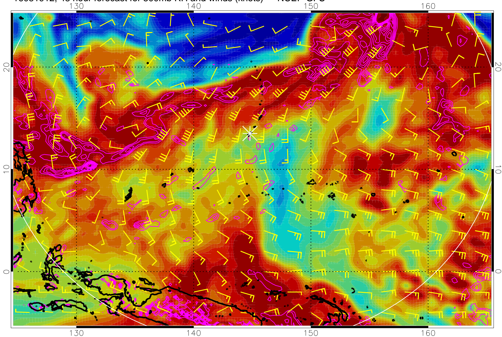
16081912, 48 hour forecast for 500mb RH and winds (knots) -- NCEP GFS
