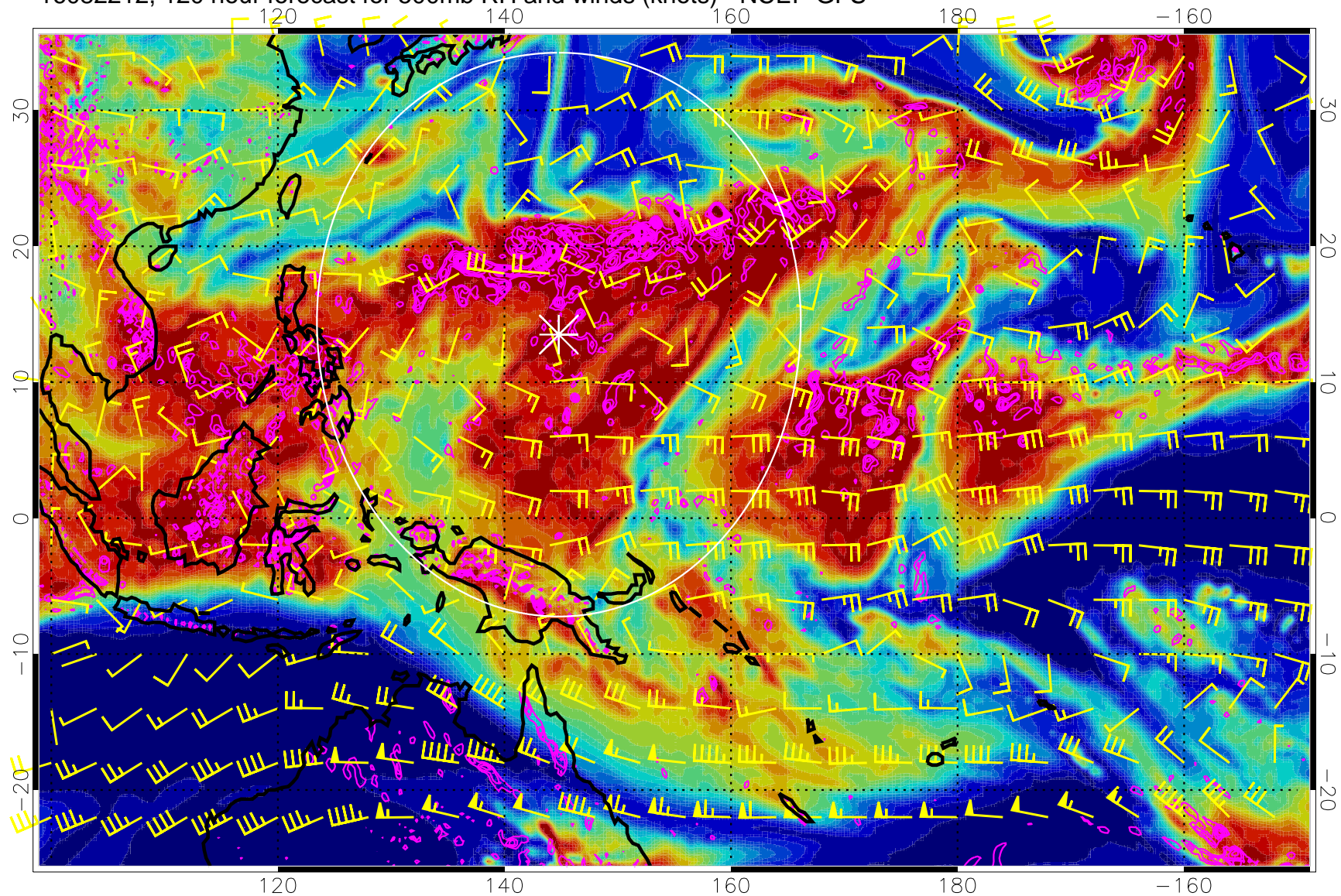
16082212, 120 hour forecast for 500mb RH and winds (knots) - NCEP GFS
