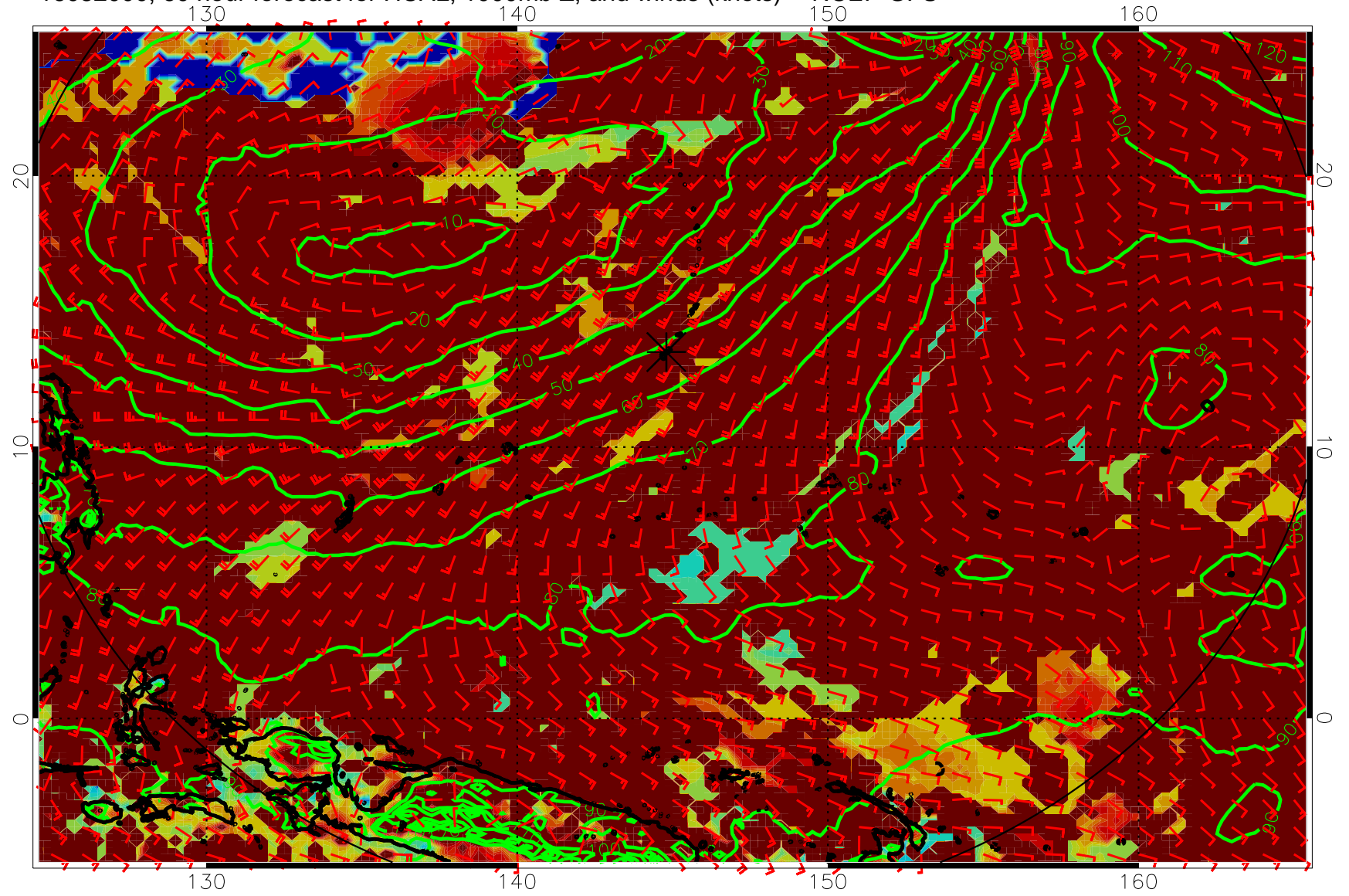
16082000, 60 hour forecast for HCAL, 1000mb Z, and winds (knots) -- NCEP GFS
