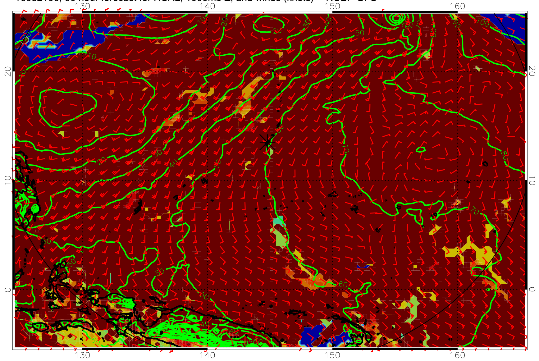
16082106, 90 hour forecast for HCAL, 1000mb Z, and winds (knots) -- NCEP GFS
