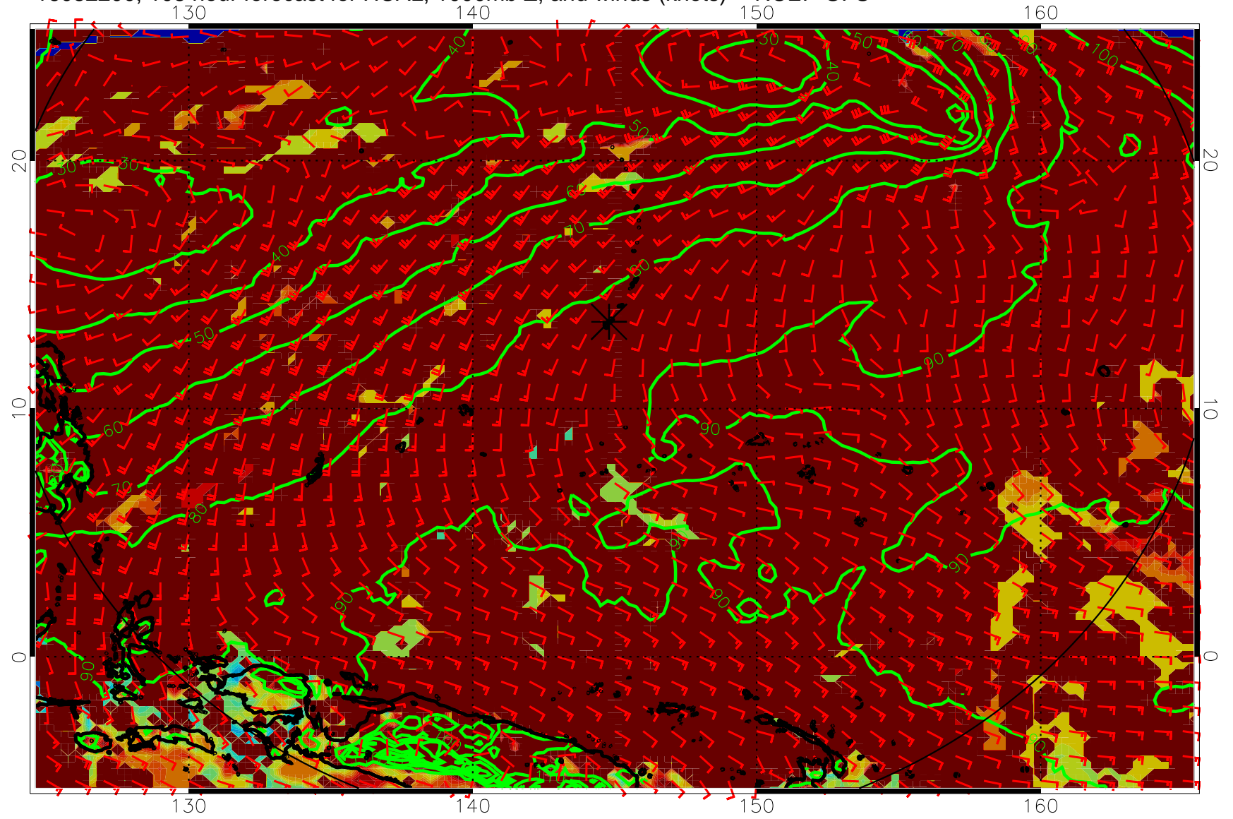
16082200, 108 hour forecast for HCAL, 1000mb Z, and winds (knots) -- NCEP GFS
