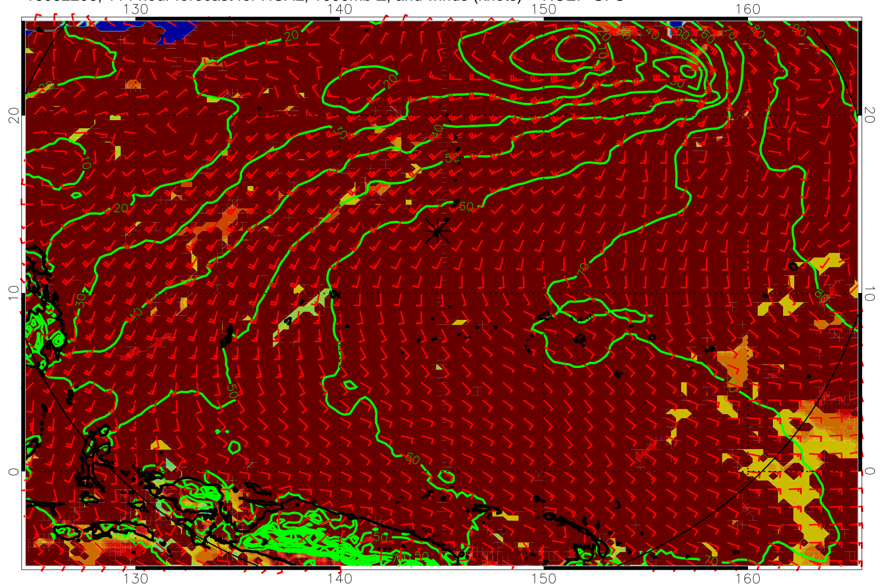
16082206, 114 hour forecast for HCAL, 1000mb Z, and winds (knots) -- NCEP GFS
