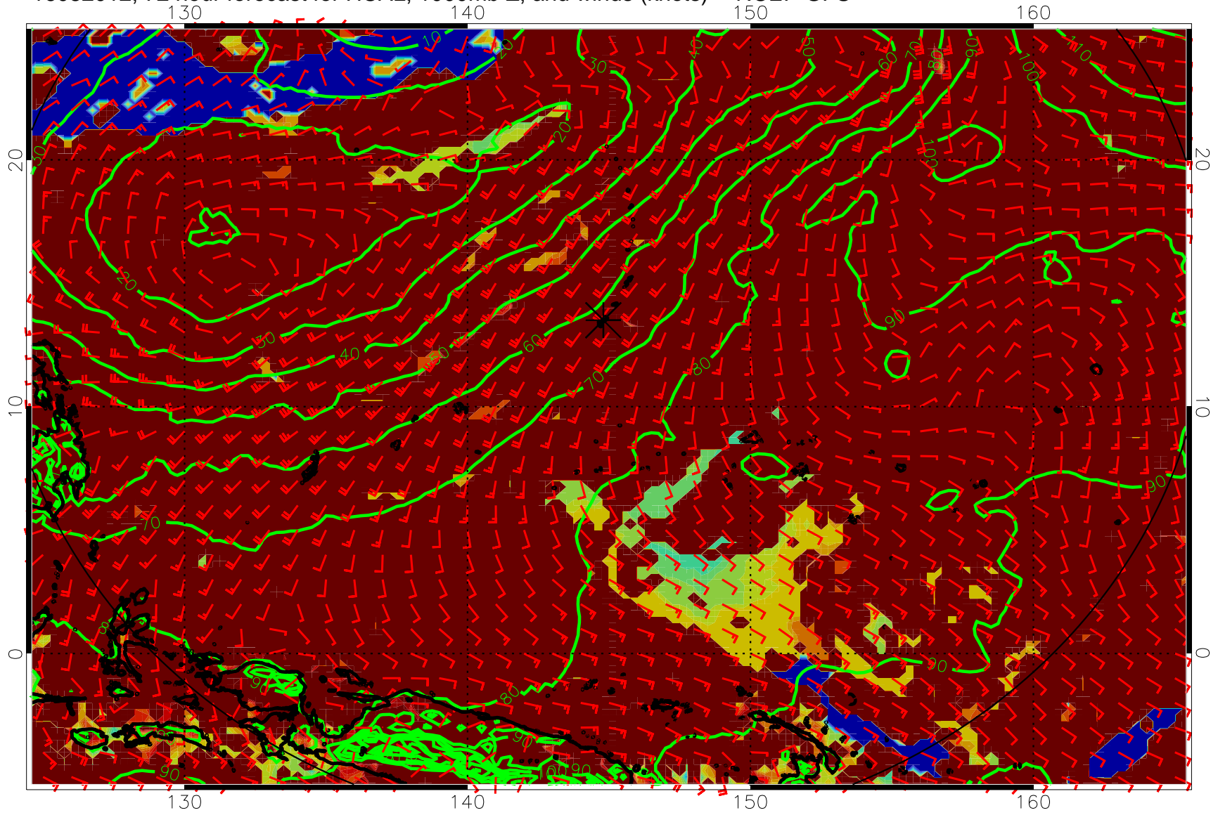
16082012, 72 hour forecast for HCAL, 1000mb Z, and winds (knots) -- NCEP GFS
