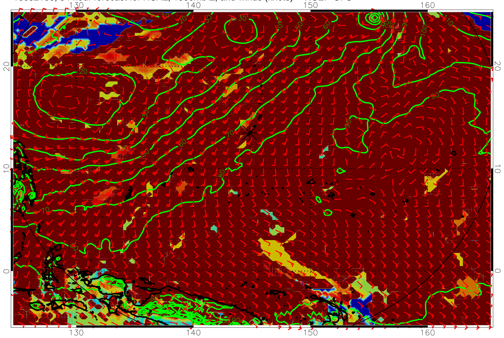
16082100, 84 hour forecast for HCAL, 1000mb Z, and winds (knots) -- NCEP GFS
