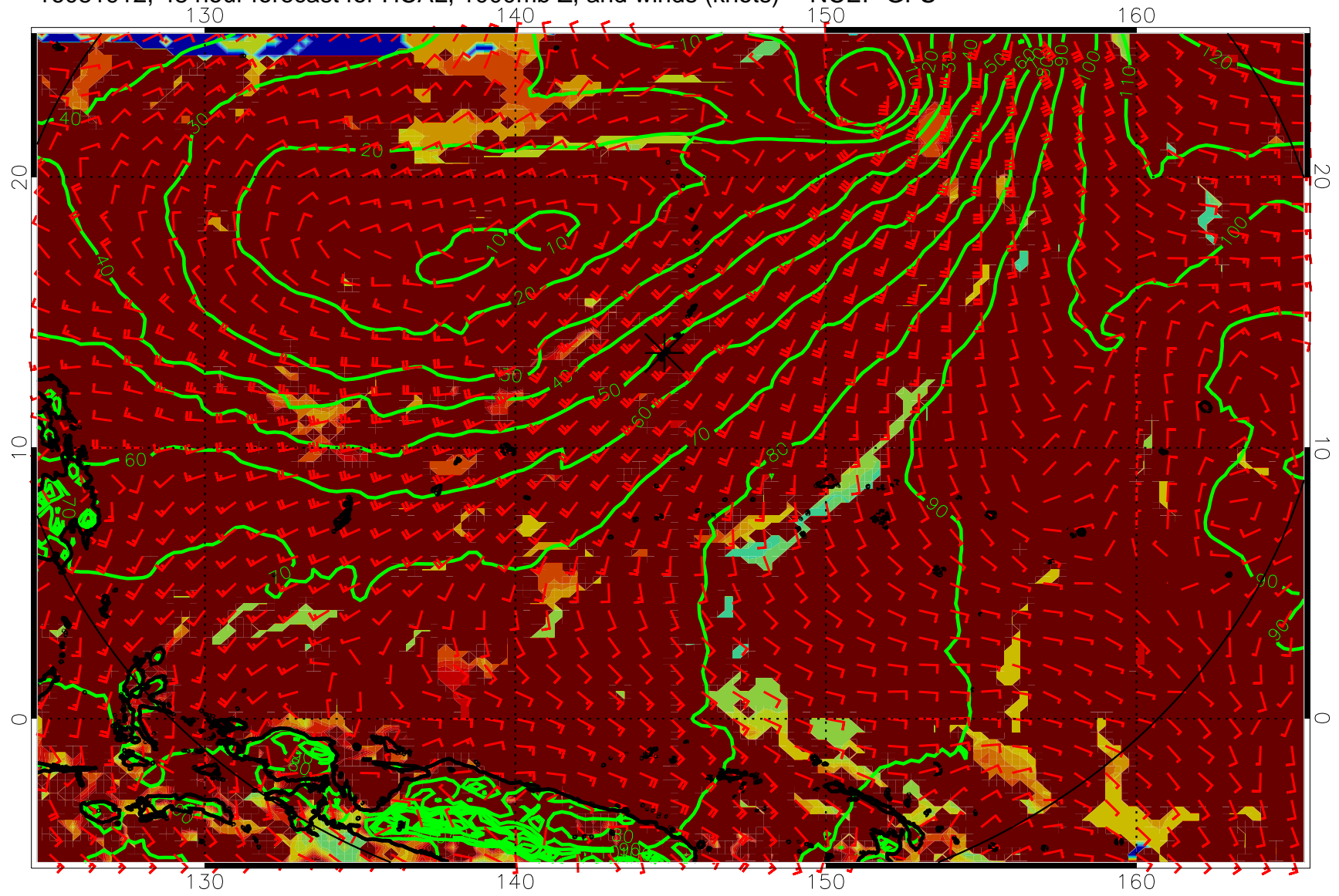
16081912, 48 hour forecast for HCAL, 1000mb Z, and winds (knots) -- NCEP GFS
