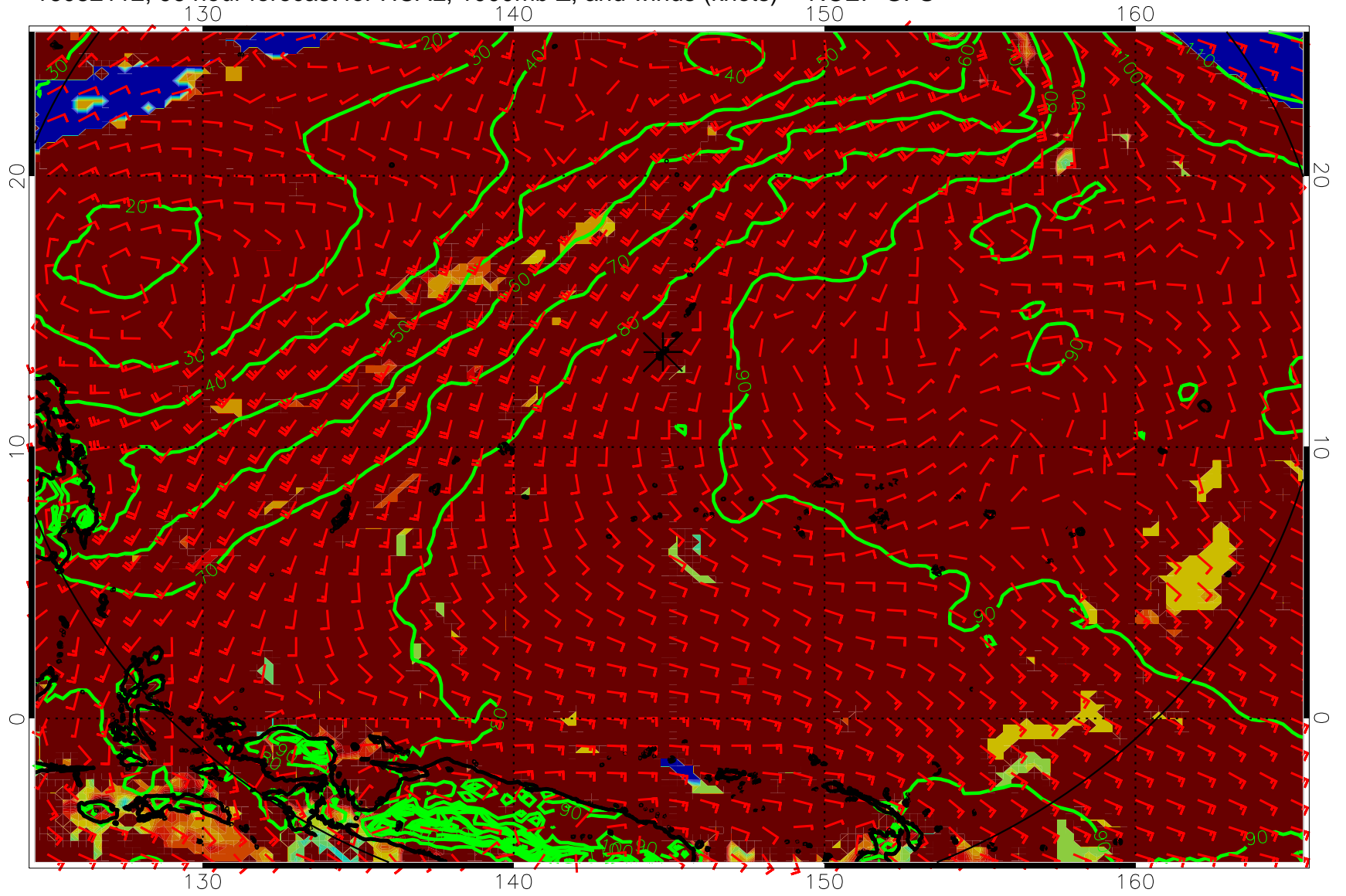
16082112, 96 hour forecast for HCAL, 1000mb Z, and winds (knots) -- NCEP GFS
