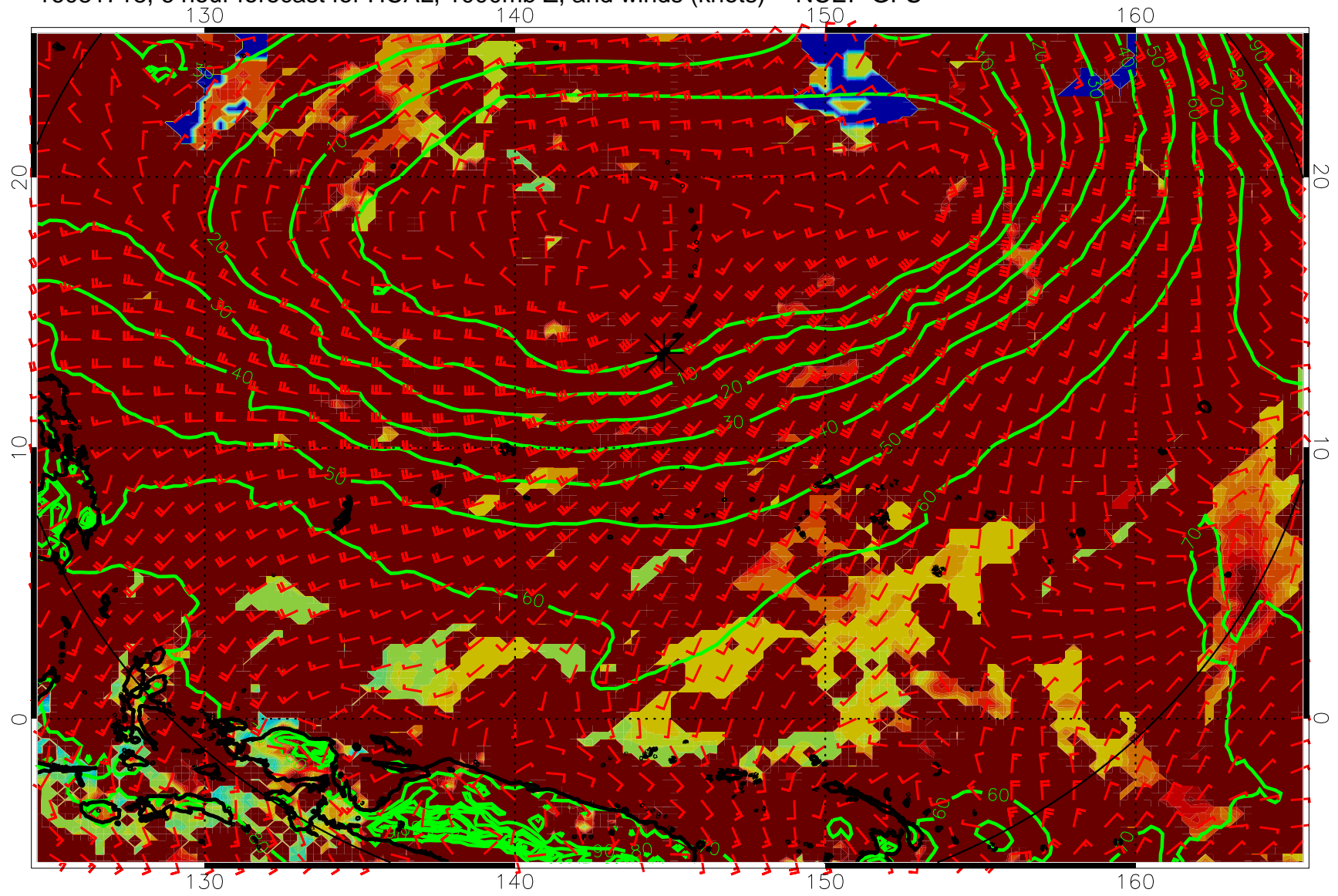
16081718, 6 hour forecast for HCAL, 1000mb Z, and winds (knots) -- NCEP GFS
