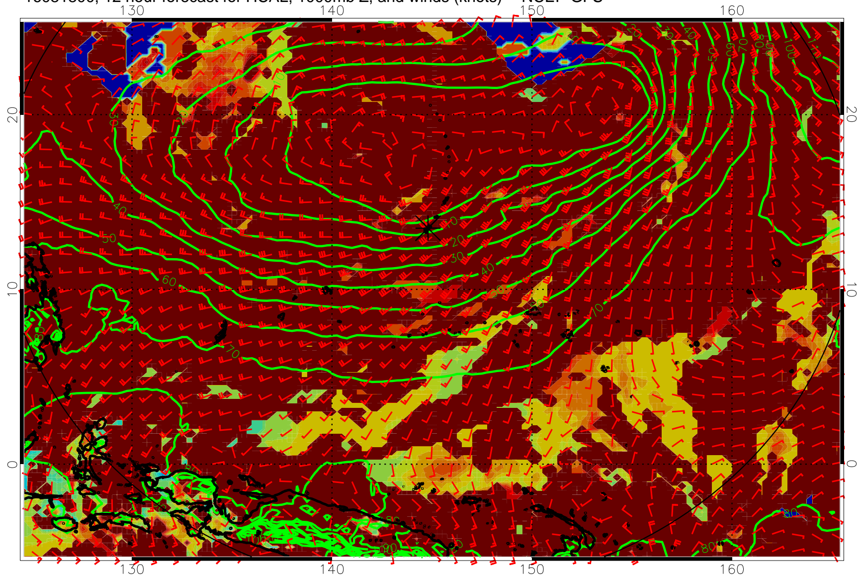
16081800, 12 hour forecast for HCAL, 1000mb Z, and winds (knots) -- NCEP GFS
