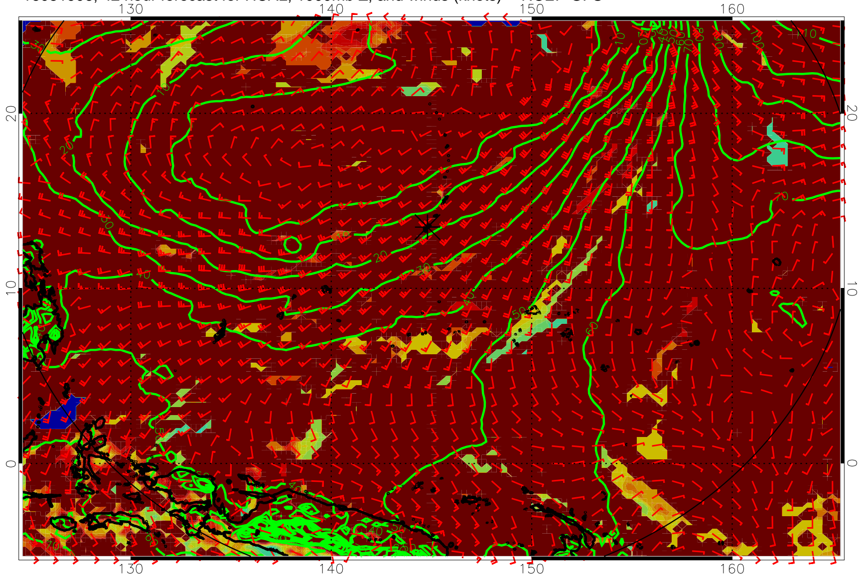
16081906, 42 hour forecast for HCAL, 1000mb Z, and winds (knots) -- NCEP GFS
