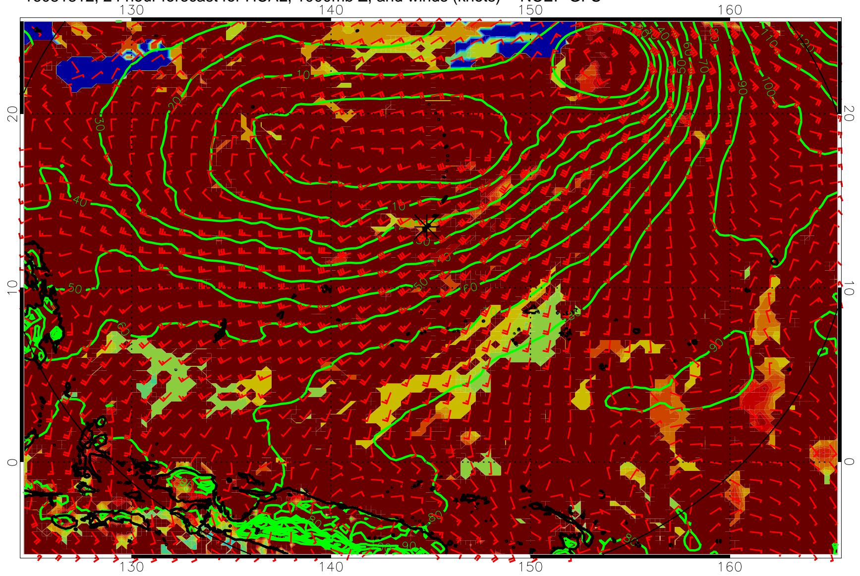
16081812, 24 hour forecast for HCAL, 1000mb Z, and winds (knots) -- NCEP GFS
