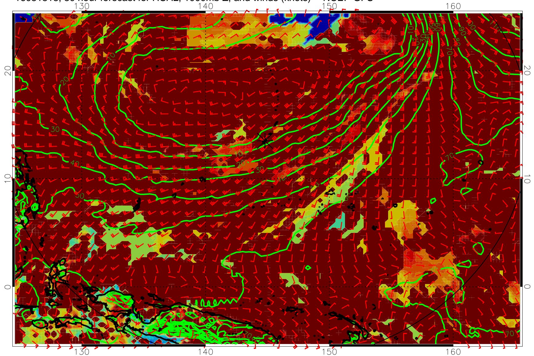
16081818, 30 hour forecast for HCAL, 1000mb Z, and winds (knots) -- NCEP GFS
