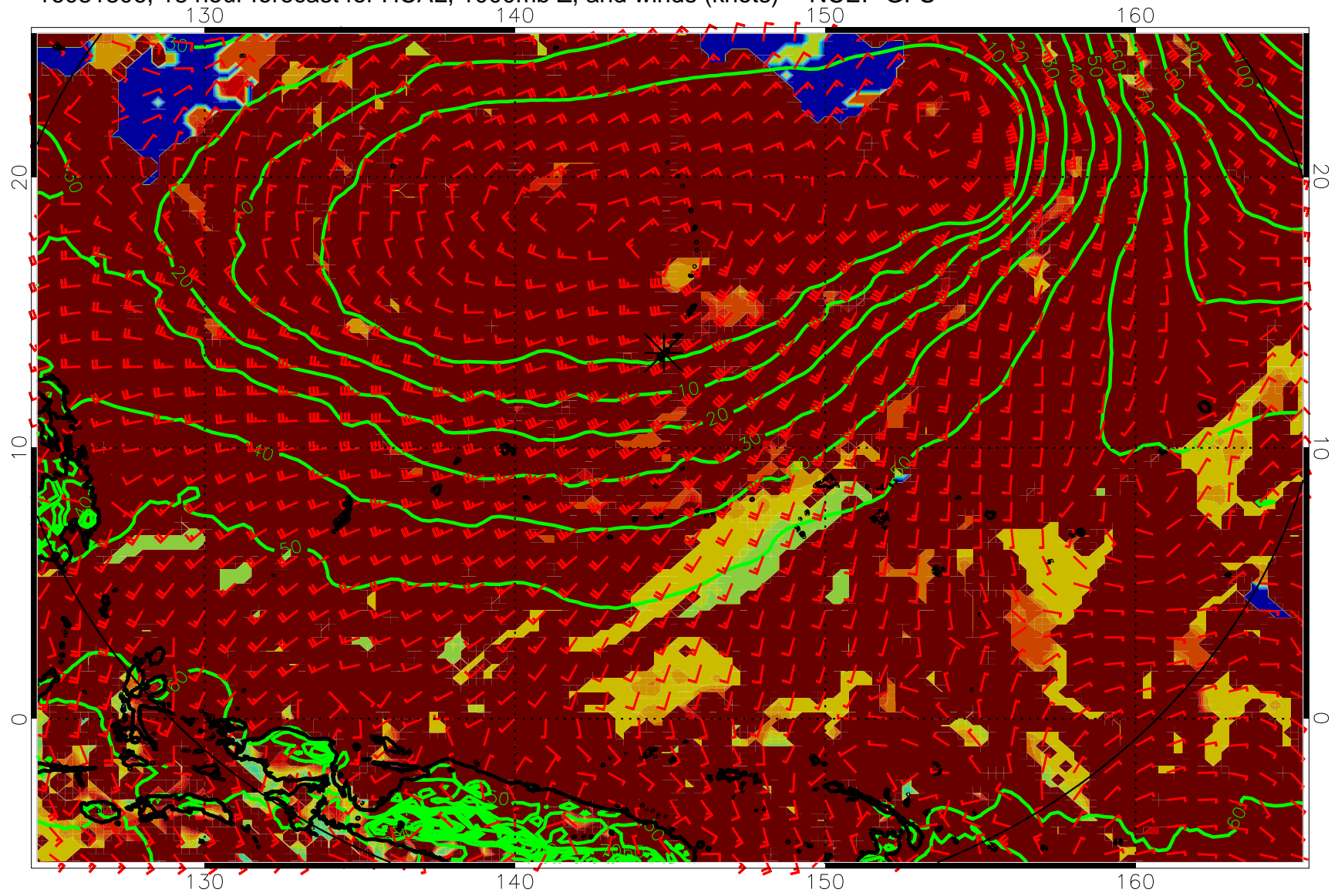
16081806, 18 hour forecast for HCAL, 1000mb Z, and winds (knots) -- NCEP GFS
