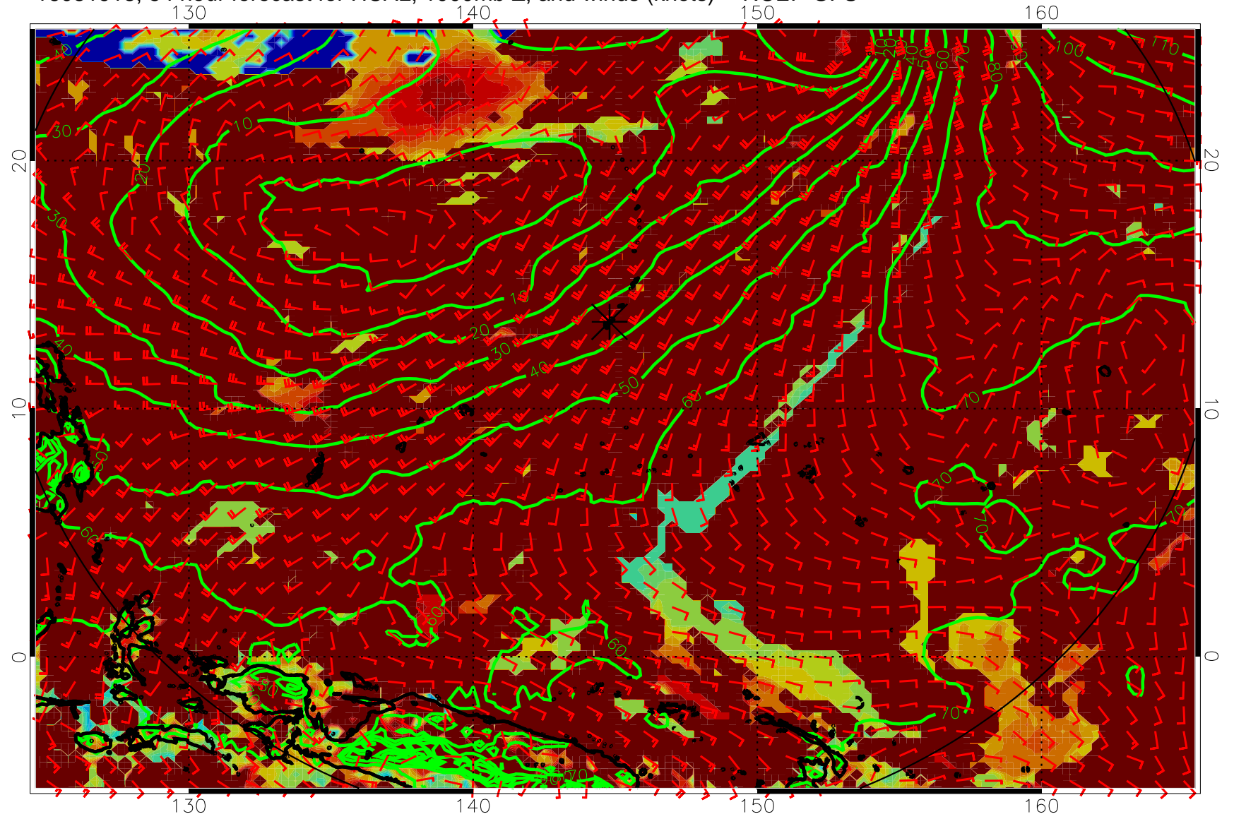
16081918, 54 hour forecast for HCAL, 1000mb Z, and winds (knots) -- NCEP GFS
