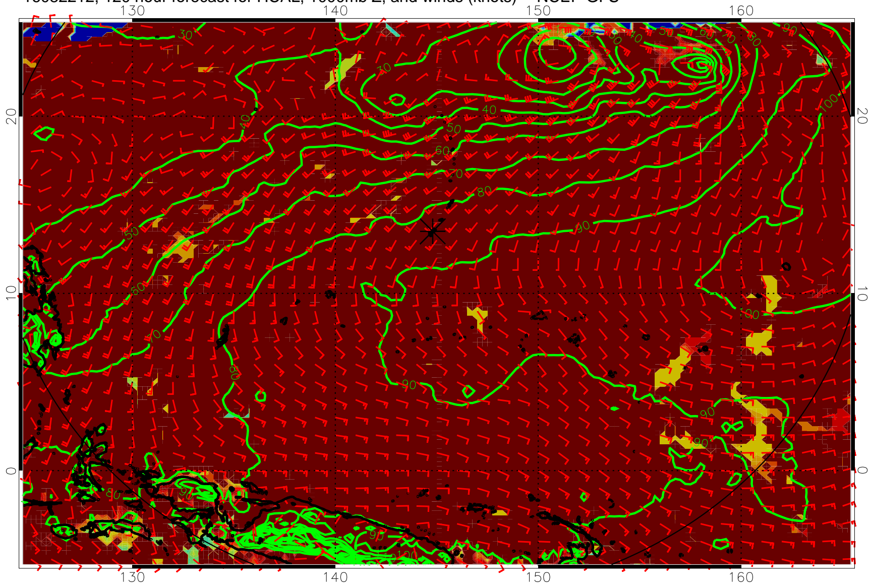
16082212, 120 hour forecast for HCAL, 1000mb Z, and winds (knots) -- NCEP GFS
