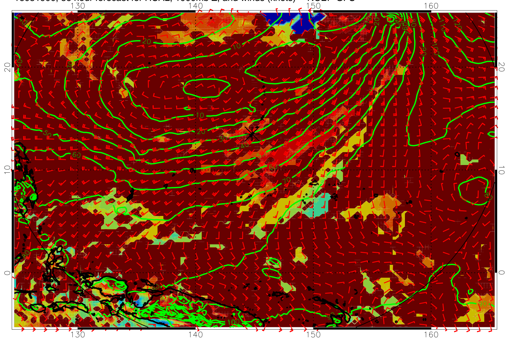
16081900, 36 hour forecast for HCAL, 1000mb Z, and winds (knots) -- NCEP GFS
