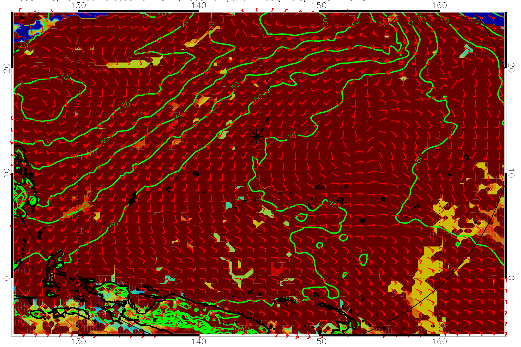
16082118, 102 hour forecast for HCAL, 1000mb Z, and winds (knots) -- NCEP GFS
