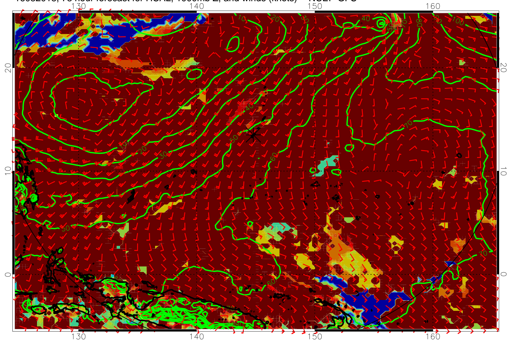
16082018, 78 hour forecast for HCAL, 1000mb Z, and winds (knots) -- NCEP GFS
