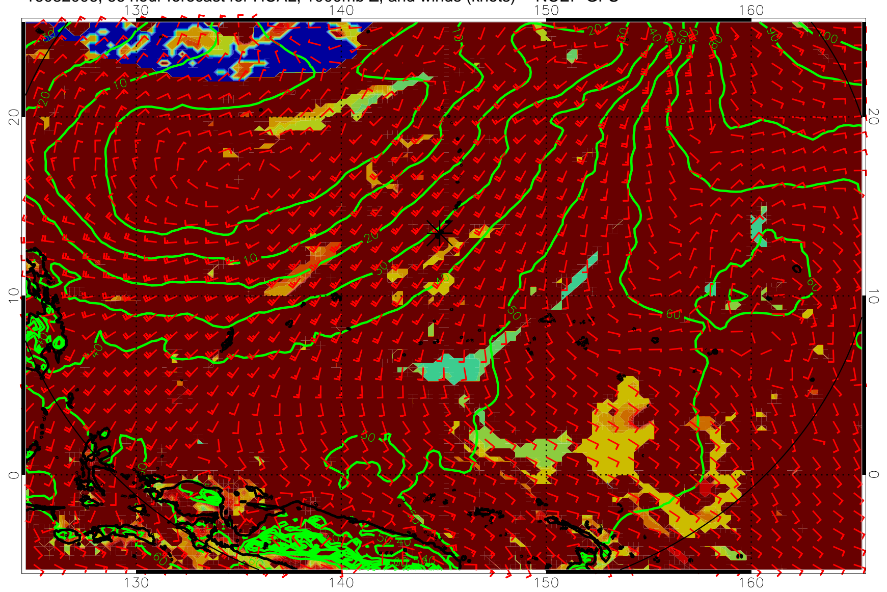
16082006, 66 hour forecast for HCAL, 1000mb Z, and winds (knots) -- NCEP GFS
