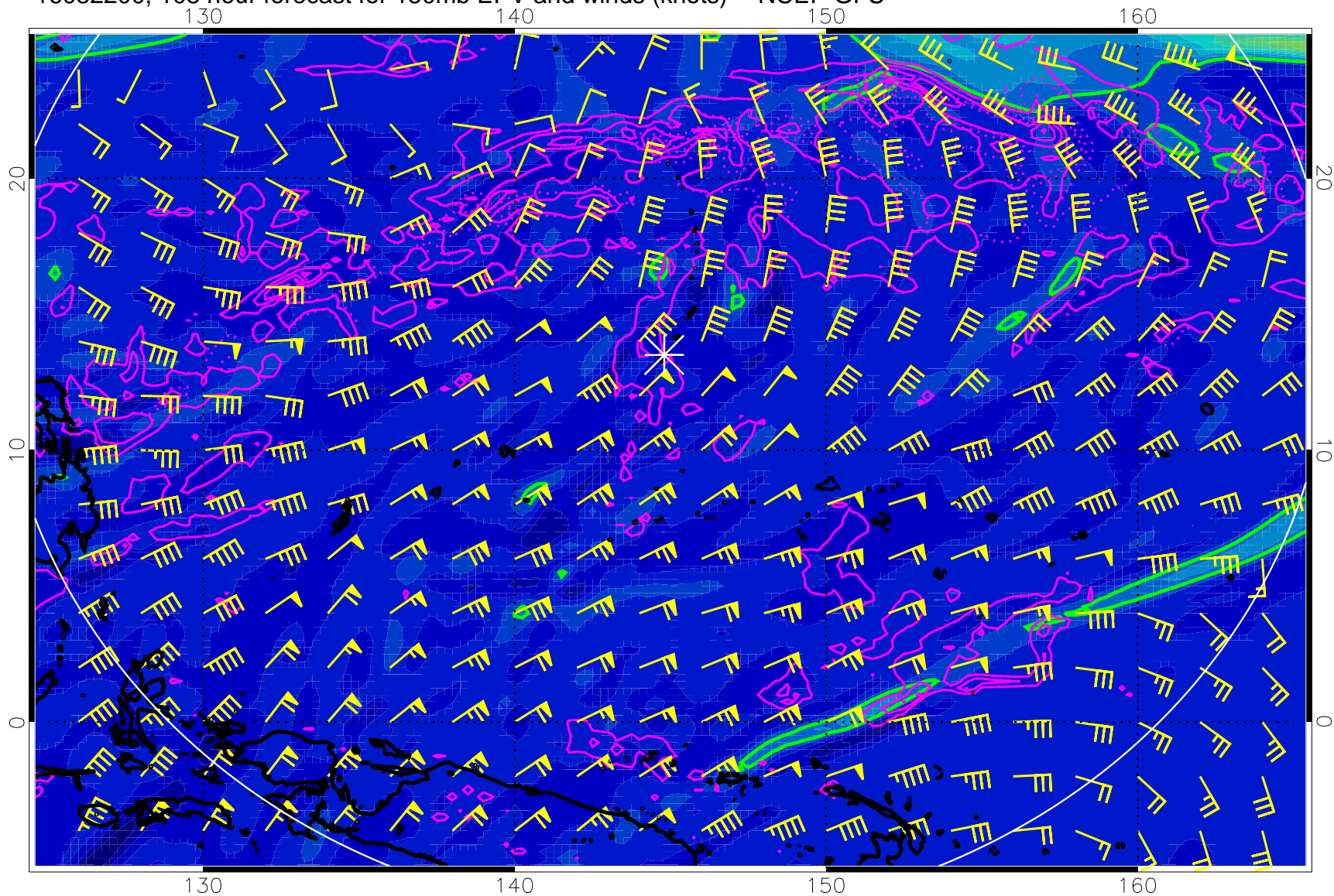
16082200, 108 hour forecast for 150mb EPV and winds (knots) -- NCEP GFS
