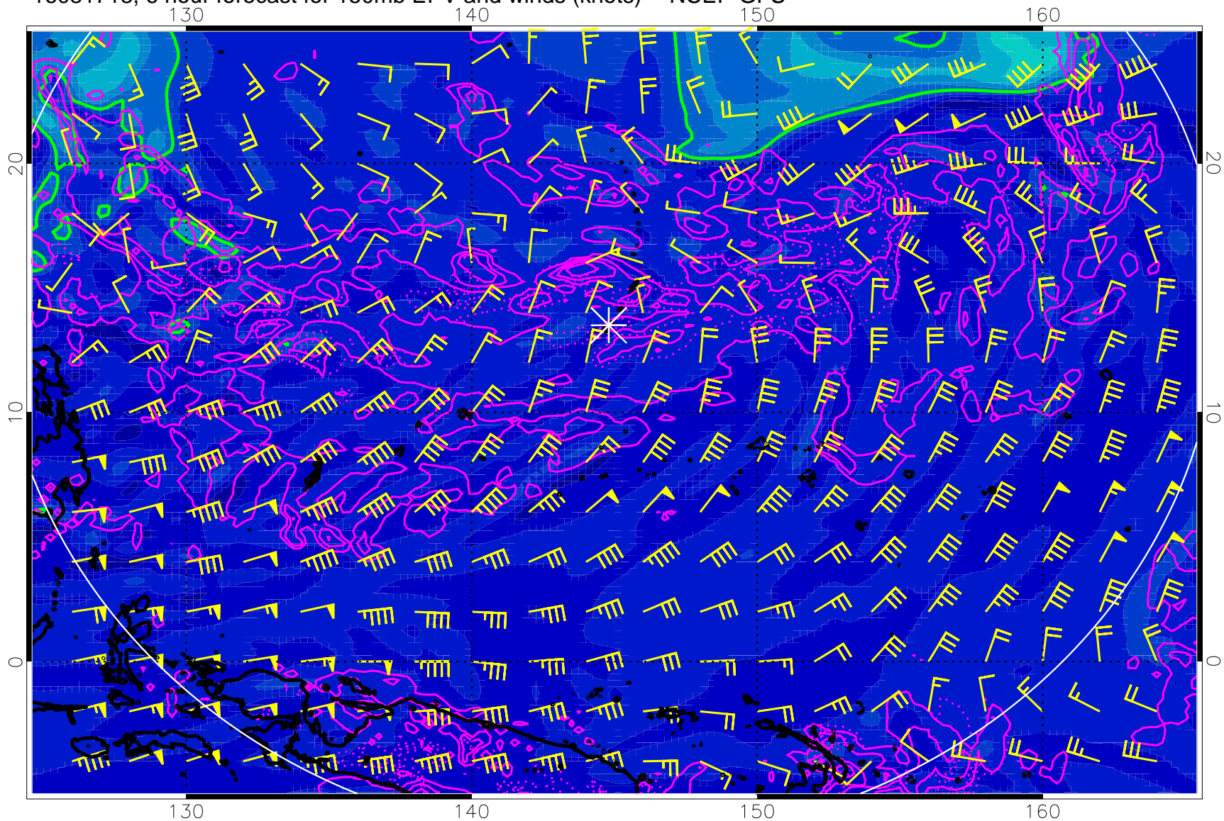
16081718, 6 hour forecast for 150mb EPV and winds (knots) -- NCEP GFS
