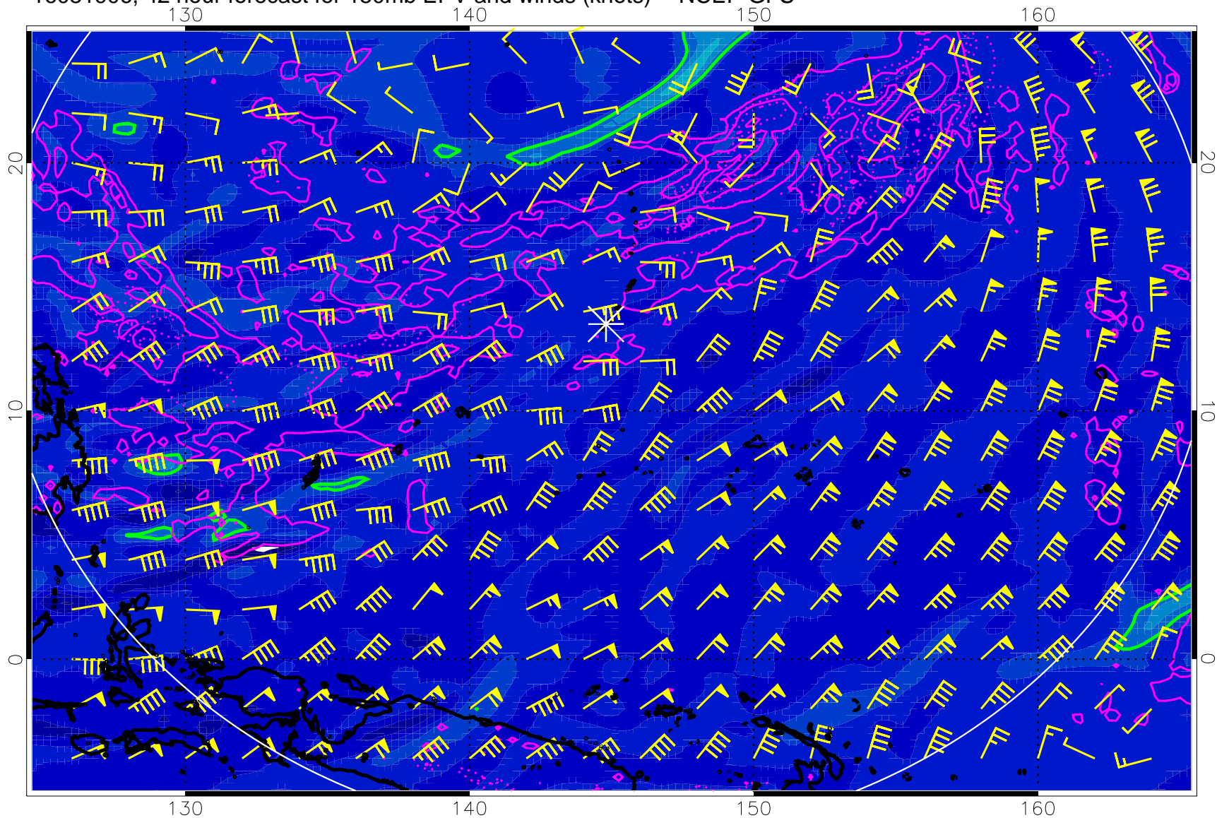
16081906, 42 hour forecast for 150mb EPV and winds (knots) -- NCEP GFS
