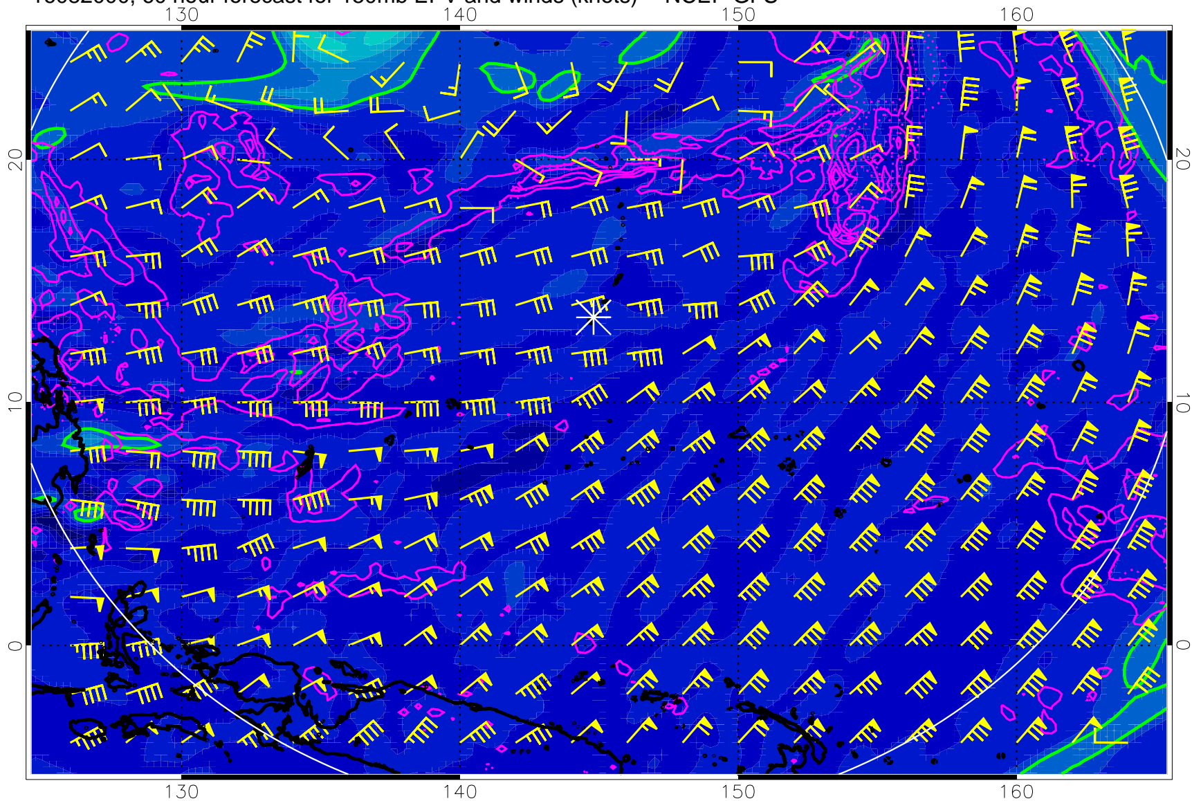
16082000, 60 hour forecast for 150mb EPV and winds (knots) -- NCEP GFS
