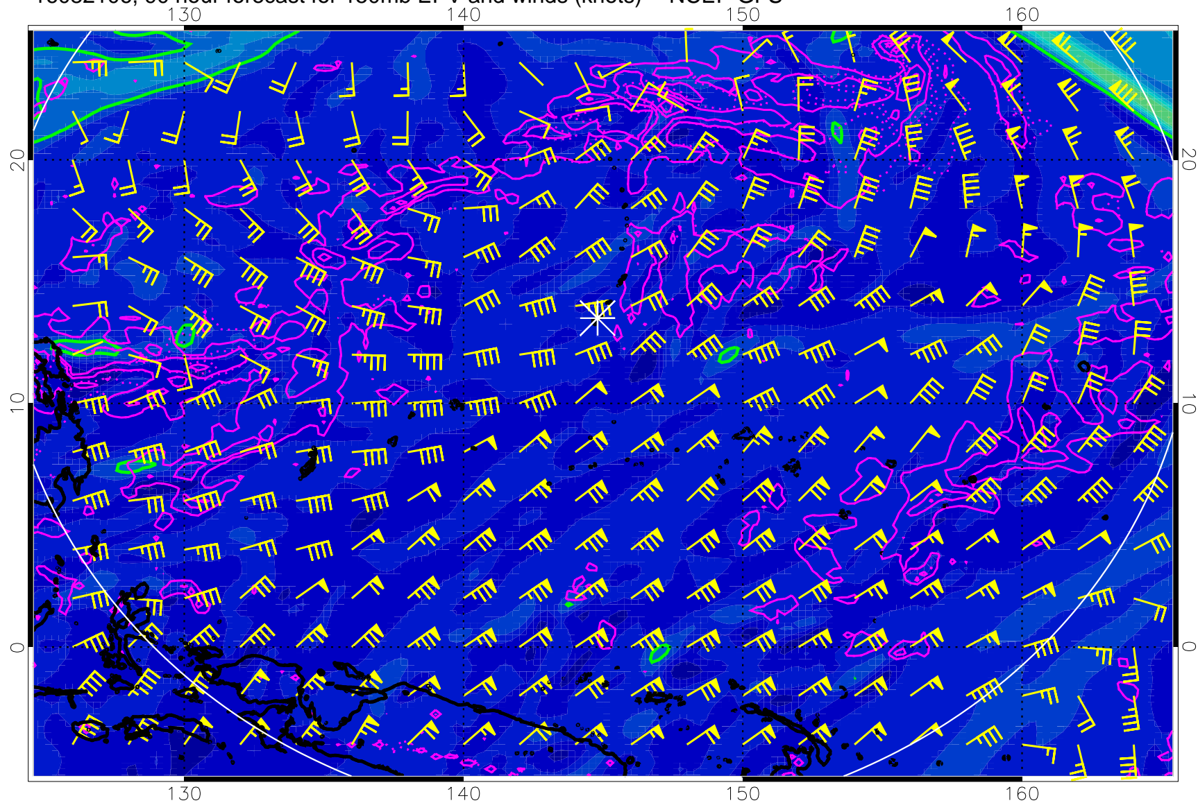
16082106, 90 hour forecast for 150mb EPV and winds (knots) -- NCEP GFS
