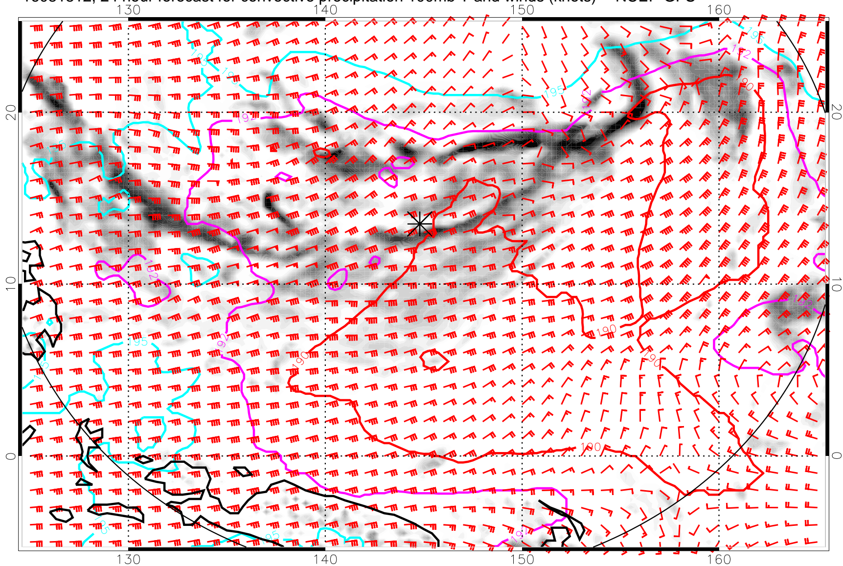
16081812, 24 hour forecast for convective precipitation 100mb T and winds (knots) -- NCEP GFS
