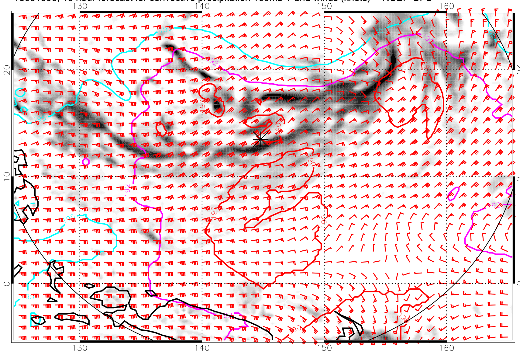
16081806, 18 hour forecast for convective precipitation 100mb T and winds (knots) -- NCEP GFS
