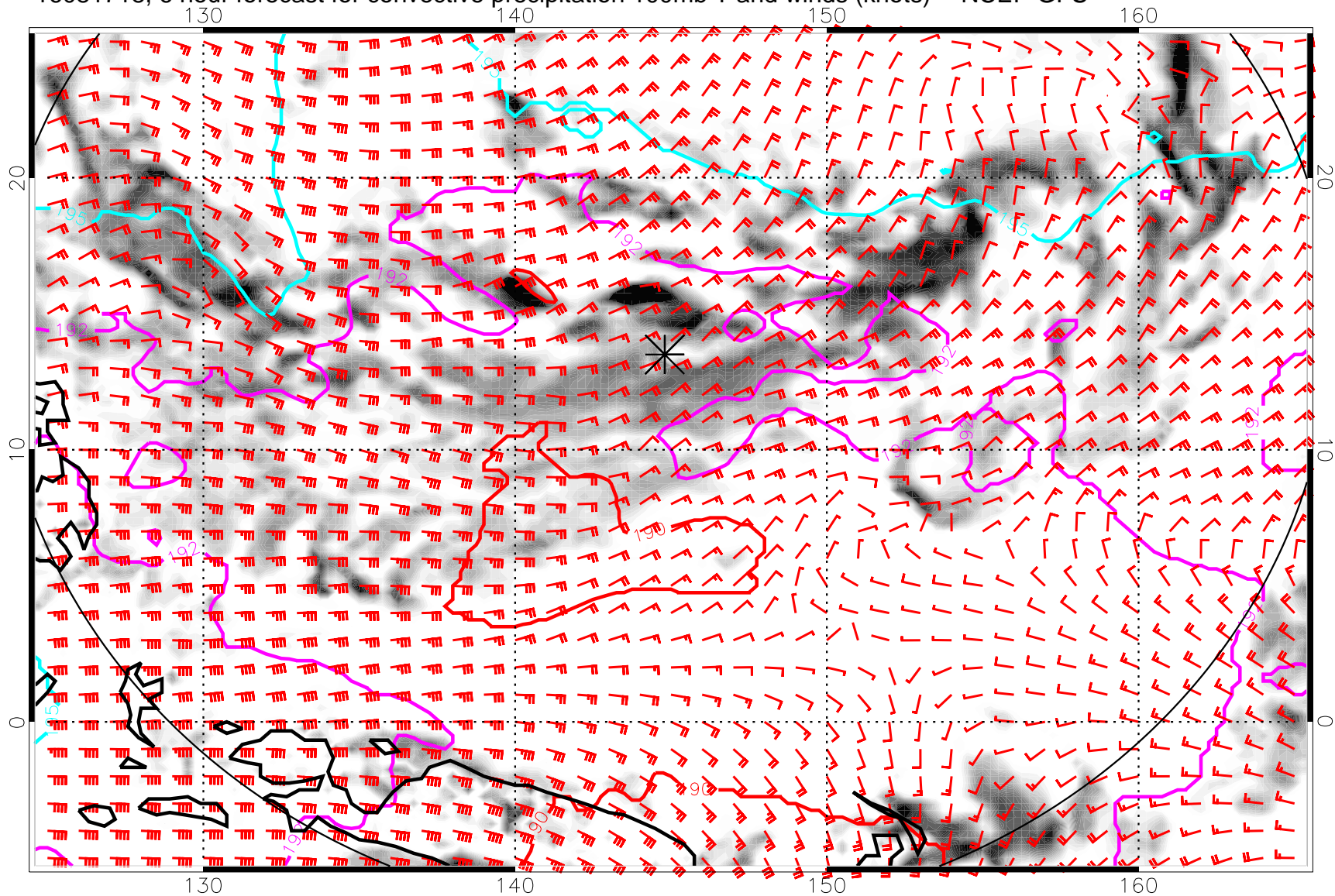
16081718, 6 hour forecast for convective precipitation 100mb T and winds (knots) -- NCEP GFS
