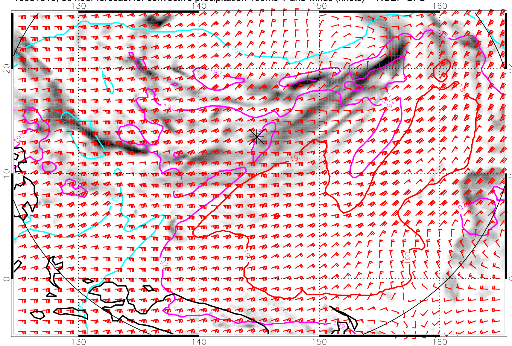
16081818, 30 hour forecast for convective precipitation 100mb T and winds (knots) -- NCEP GFS
