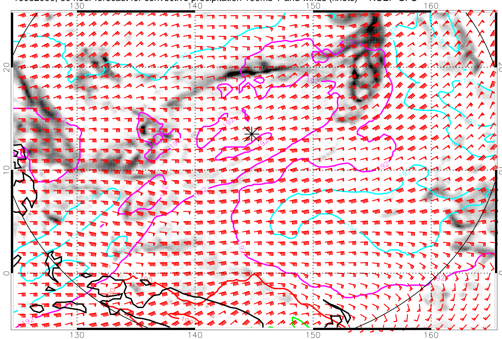
16082000, 60 hour forecast for convective precipitation 100mb T and winds (knots) -- NCEP GFS
