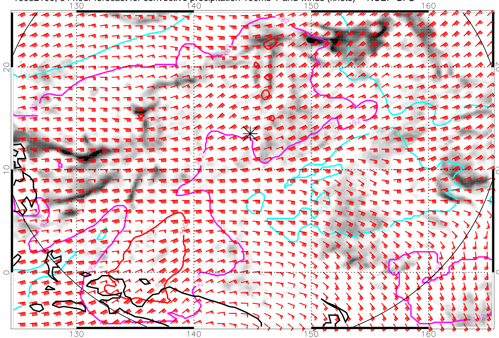
16082100, 84 hour forecast for convective precipitation 100mb T and winds (knots) -- NCEP GFS
