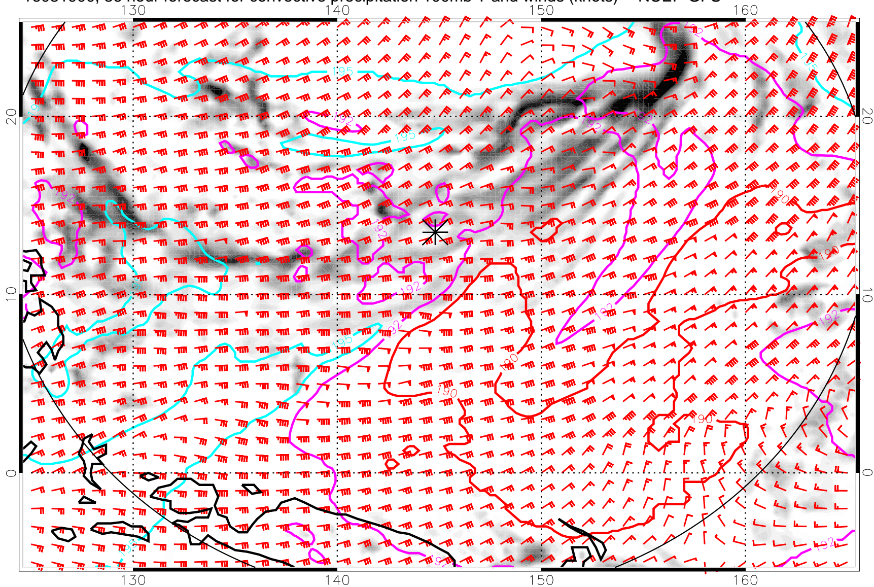
16081900, 36 hour forecast for convective precipitation 100mb T and winds (knots) -- NCEP GFS
