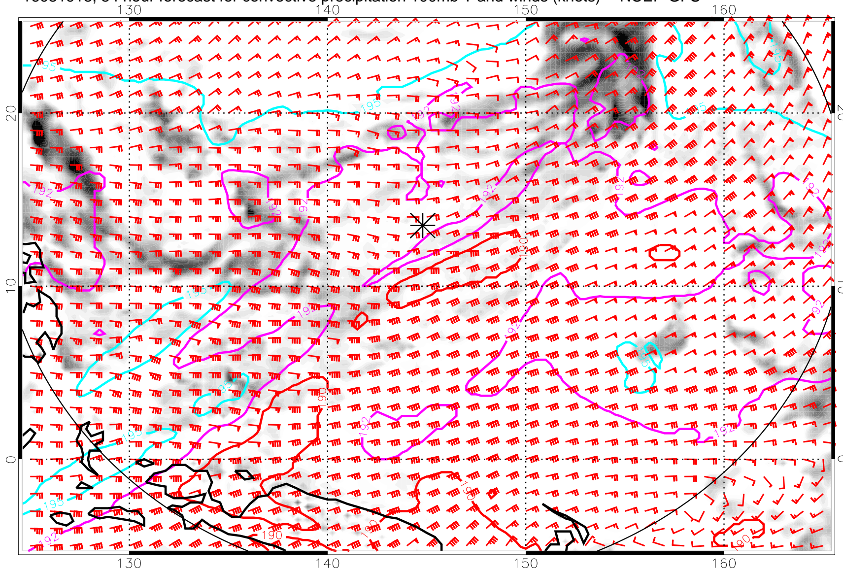
16081918, 54 hour forecast for convective precipitation 100mb T and winds (knots) -- NCEP GFS
