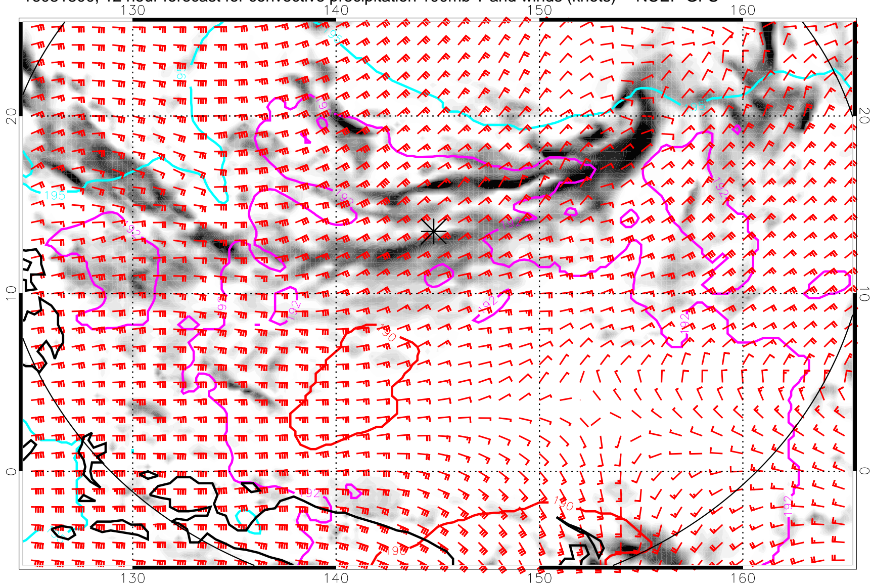
16081800, 12 hour forecast for convective precipitation 100mb T and winds (knots) -- NCEP GFS
