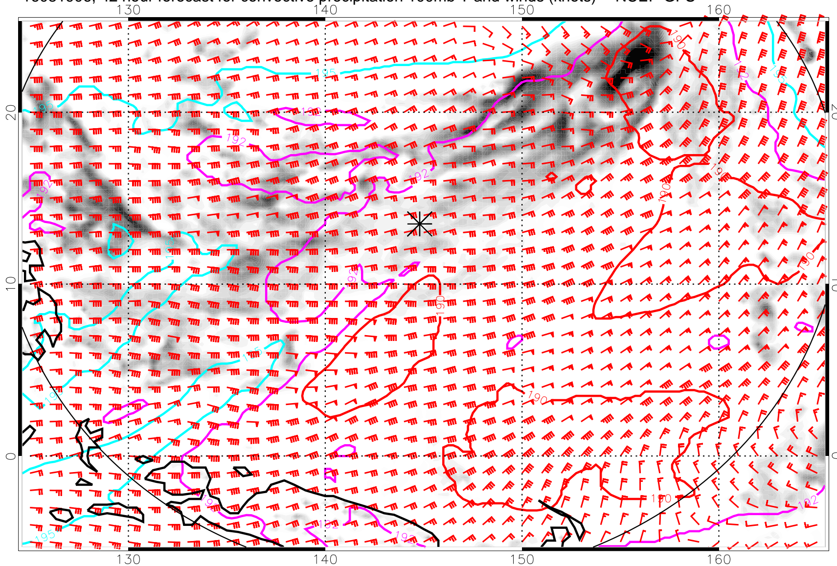
16081906, 42 hour forecast for convective precipitation 100mb T and winds (knots) -- NCEP GFS
