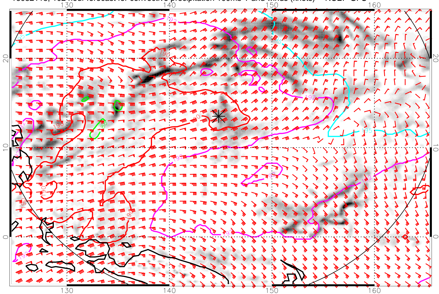
16082118, 102 hour forecast for convective precipitation 100mb T and winds (knots) -- NCEP GFS
