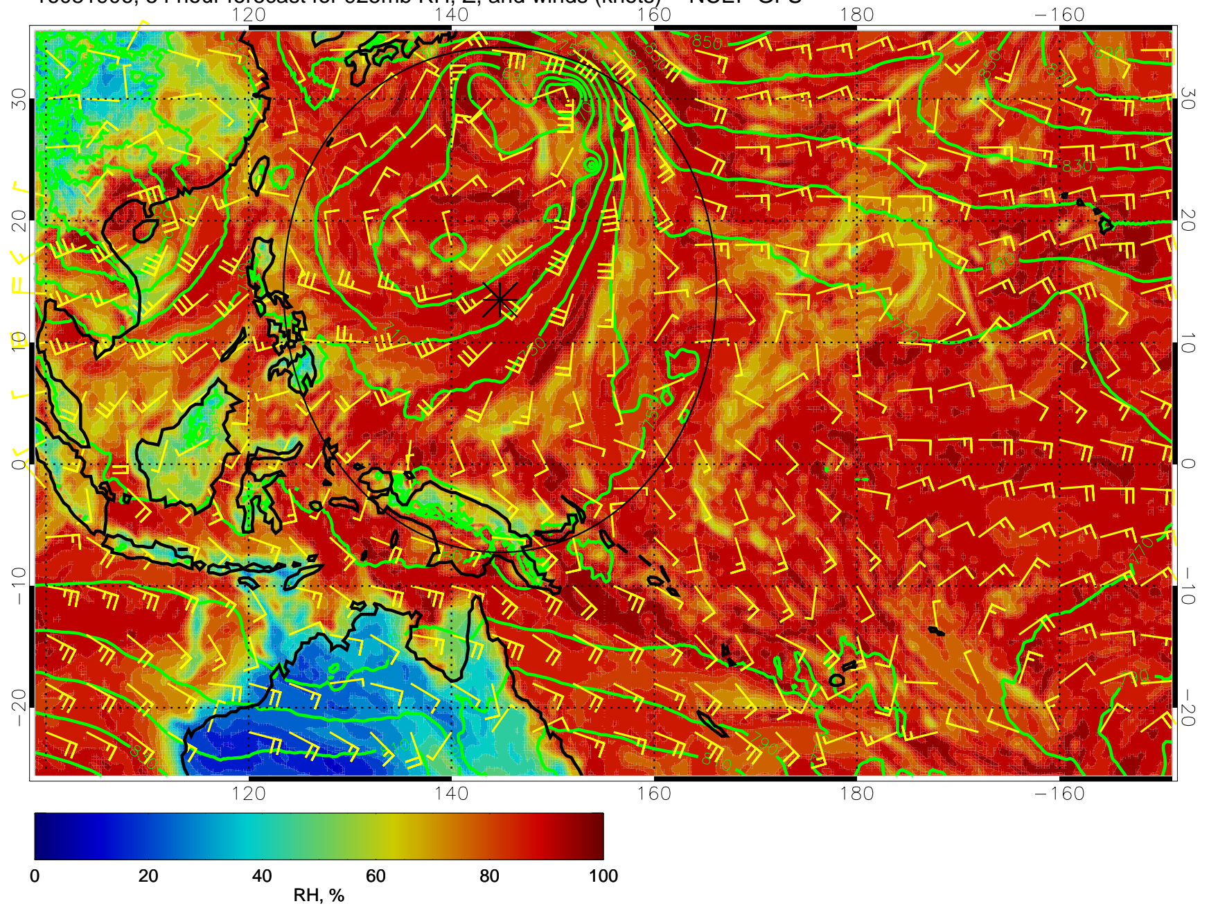
16081906, 54 hour forecast for 925mb RH, Z, and winds (knots) -- NCEP GFS
