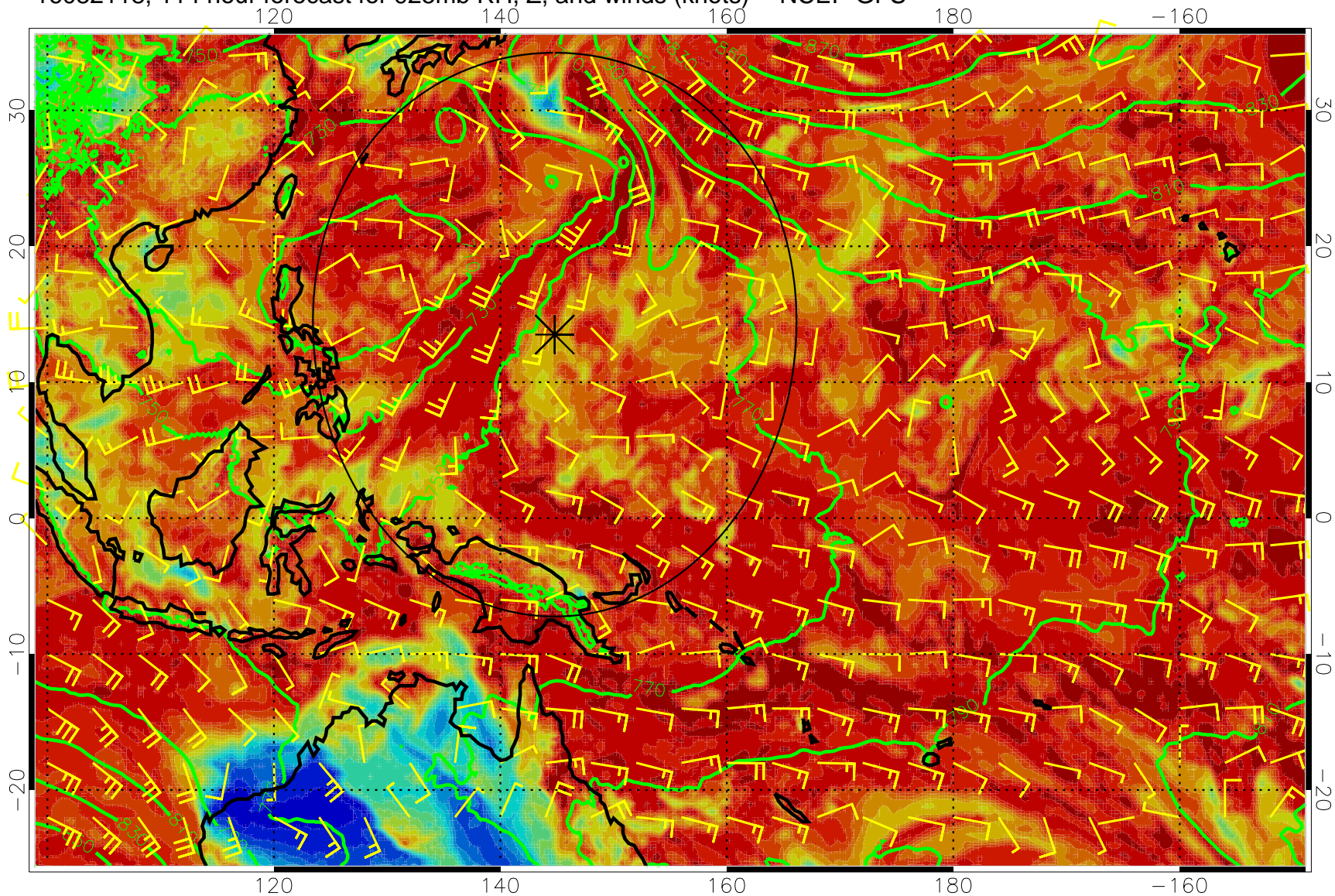
16082118, 114 hour forecast for 925mb RH, Z, and winds (knots) -- NCEP GFS
