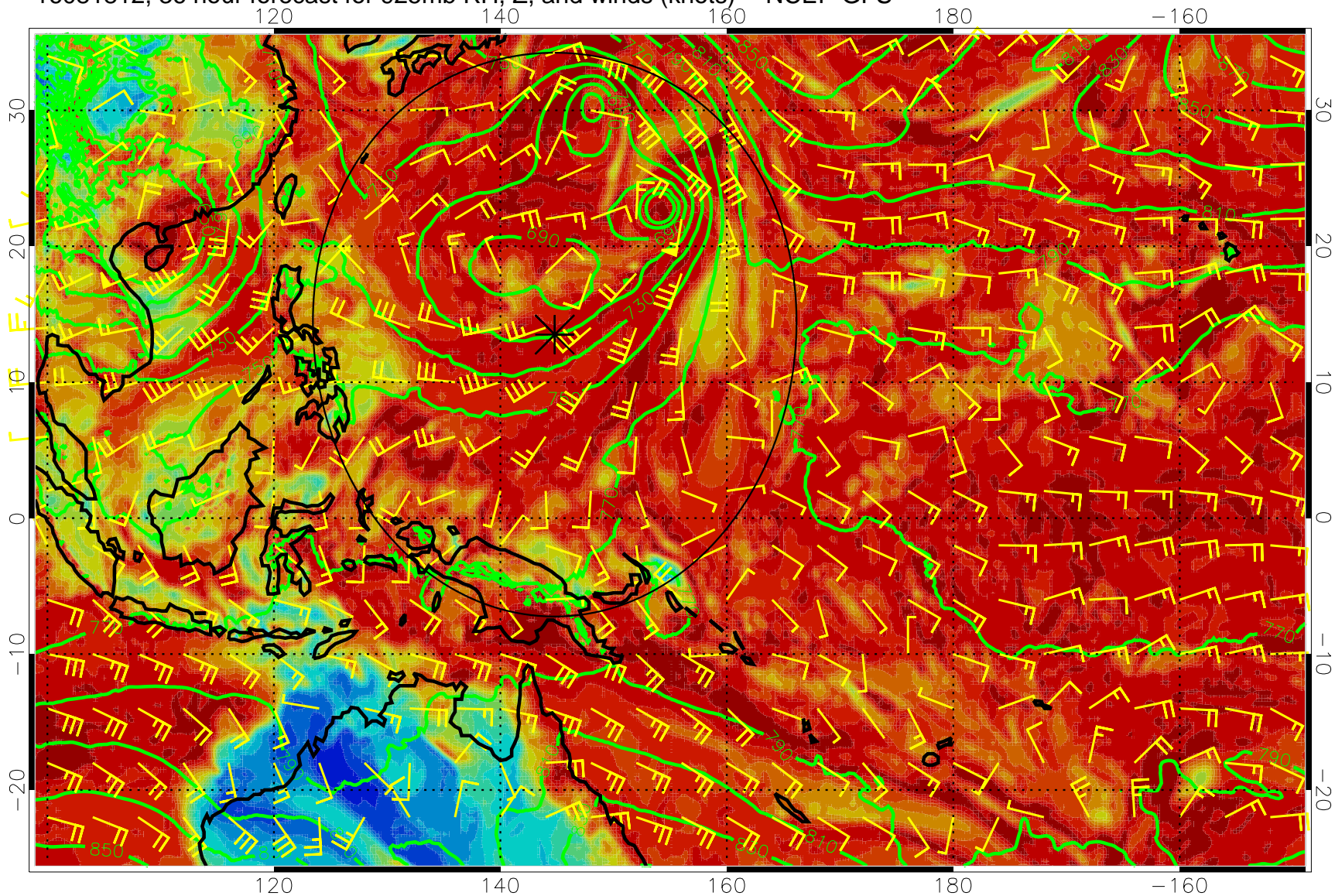
16081812, 36 hour forecast for 925mb RH, Z, and winds (knots) -- NCEP GFS
