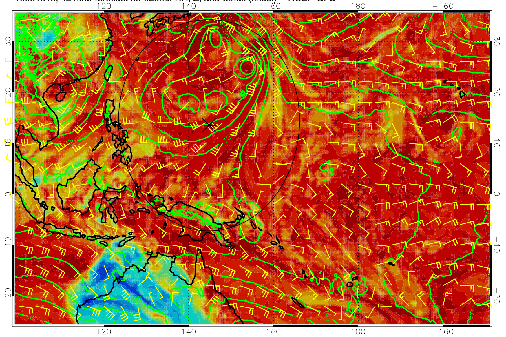
16081818, 42 hour forecast for 925mb RH, Z, and winds (knots) -- NCEP GFS
