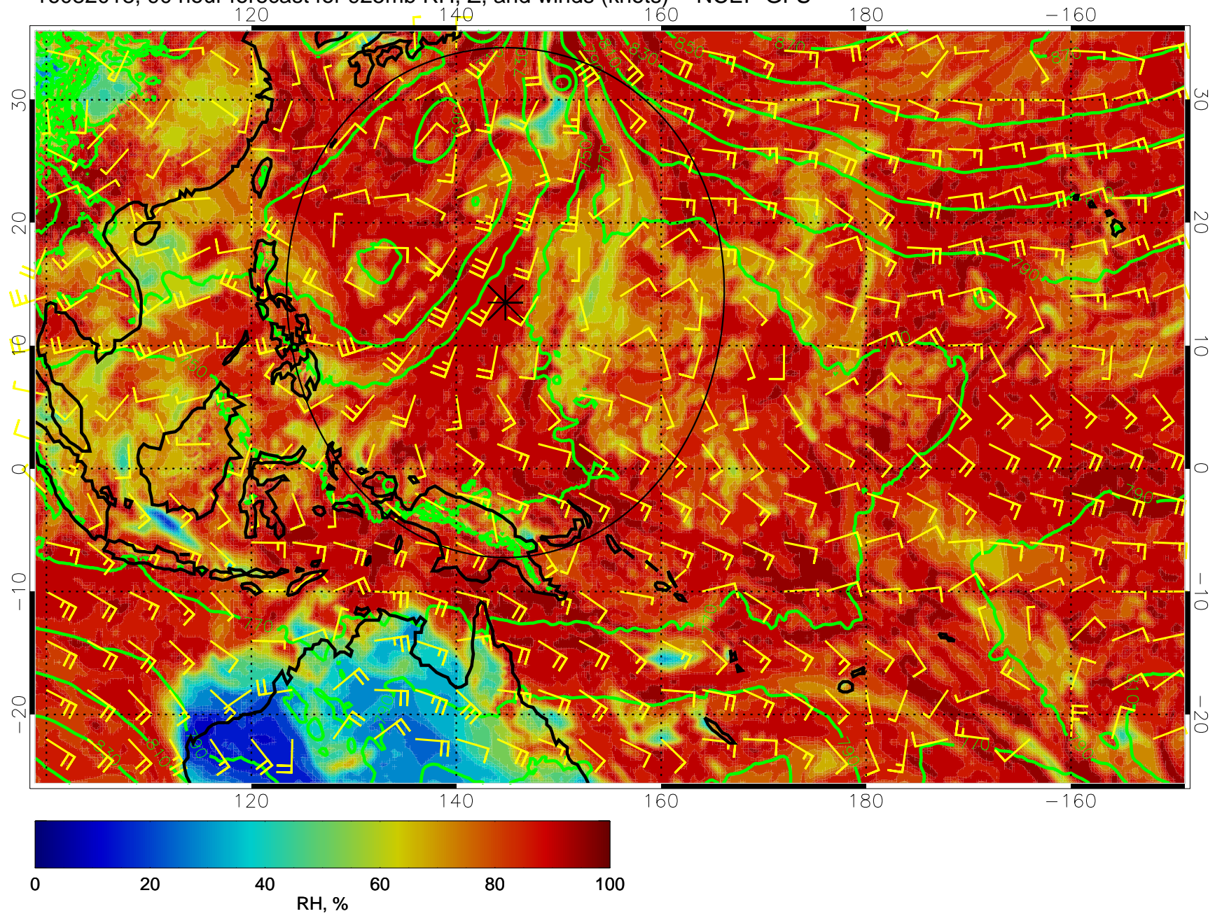
16082018, 90 hour forecast for 925mb RH, Z, and winds (knots) -- NCEP GFS
