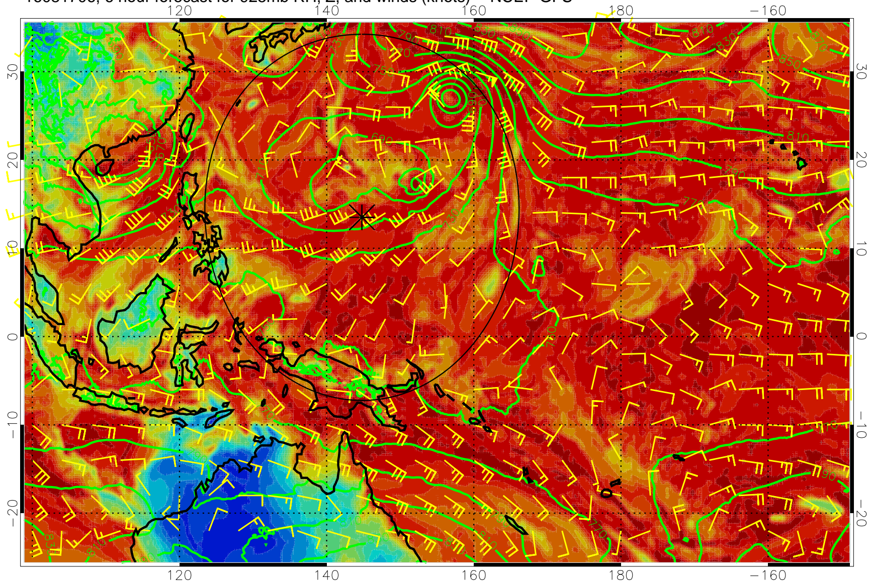
16081706, 6 hour forecast for 925mb RH, Z, and winds (knots) -- NCEP GFS
