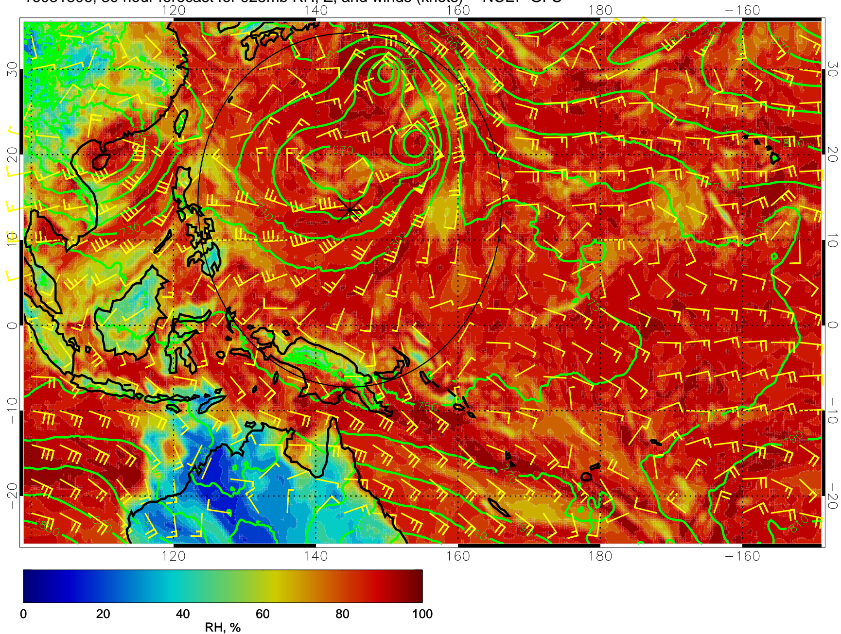
16081806, 30 hour forecast for 925mb RH, Z, and winds (knots) -- NCEP GFS
