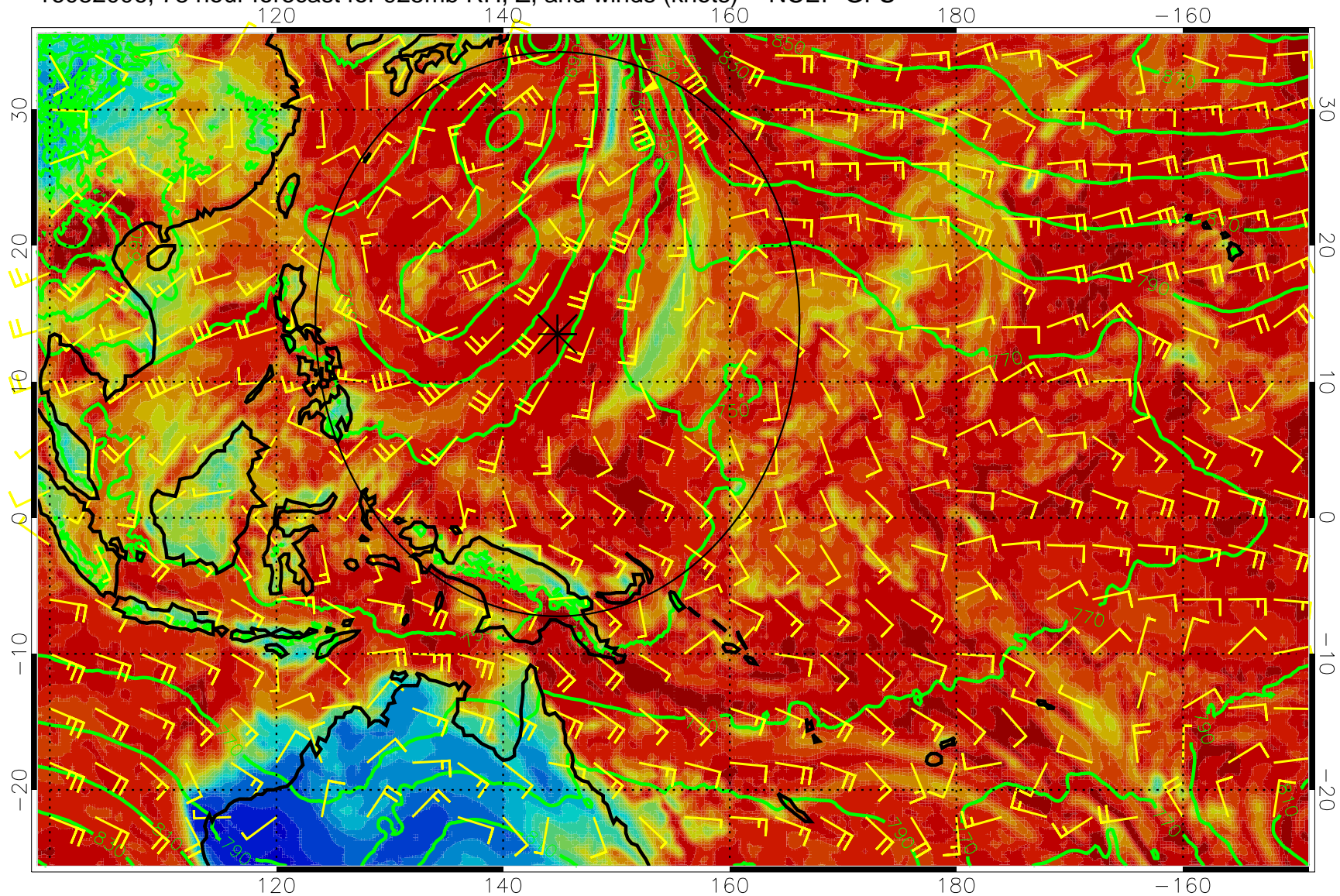
16082006, 78 hour forecast for 925mb RH, Z, and winds (knots) -- NCEP GFS
