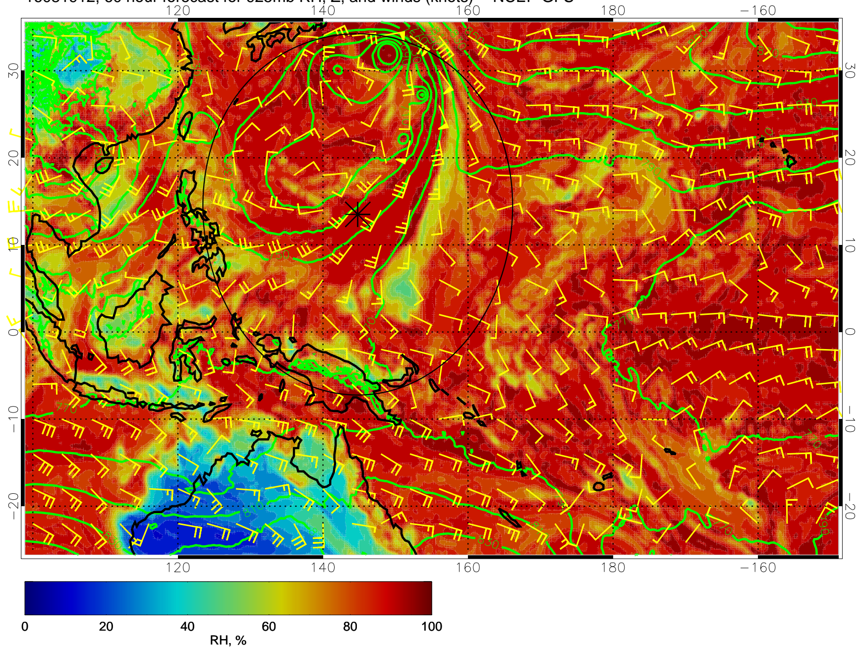
16081912, 60 hour forecast for 925mb RH, Z, and winds (knots) -- NCEP GFS
