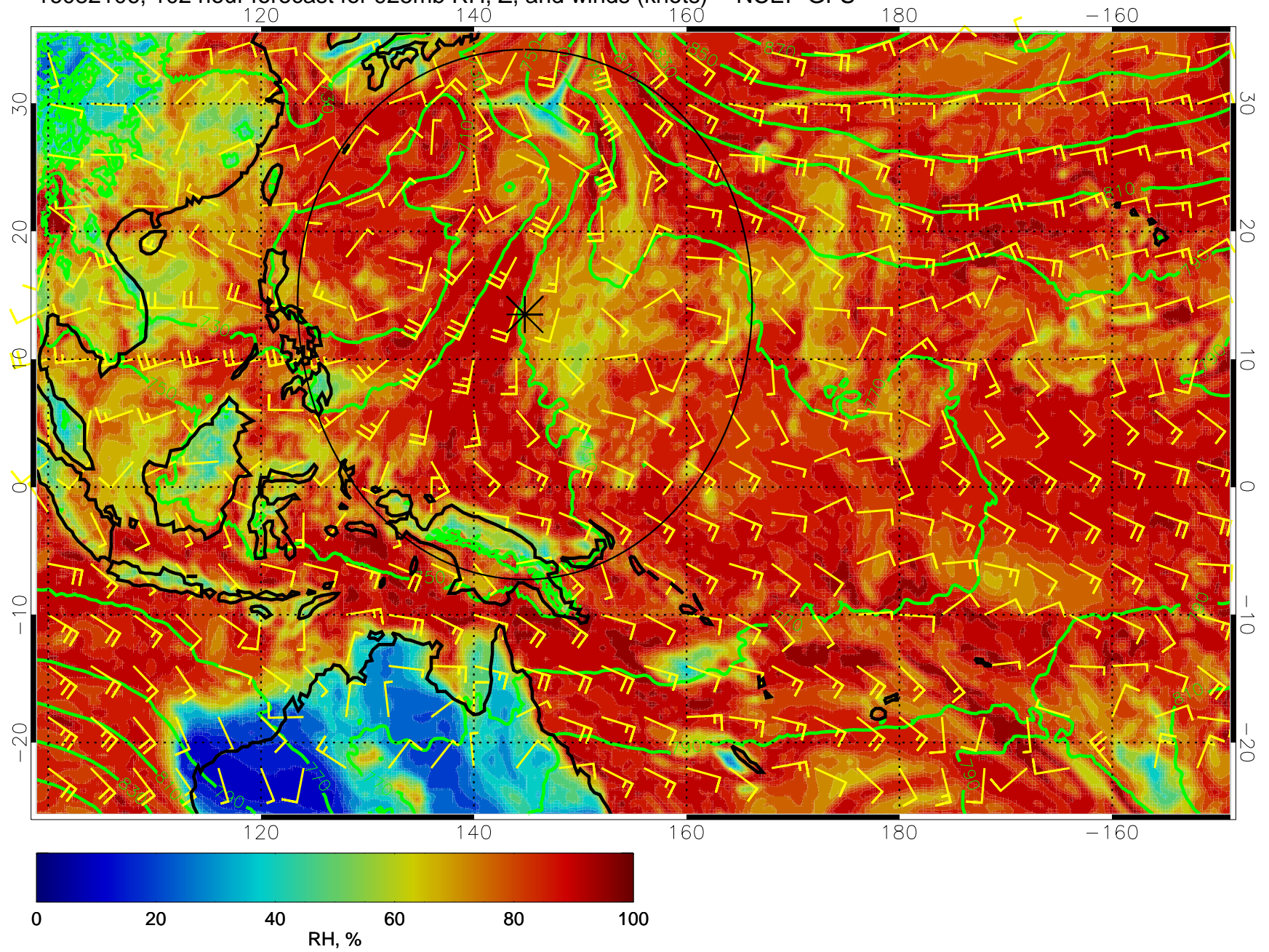
16082106, 102 hour forecast for 925mb RH, Z, and winds (knots) -- NCEP GFS
