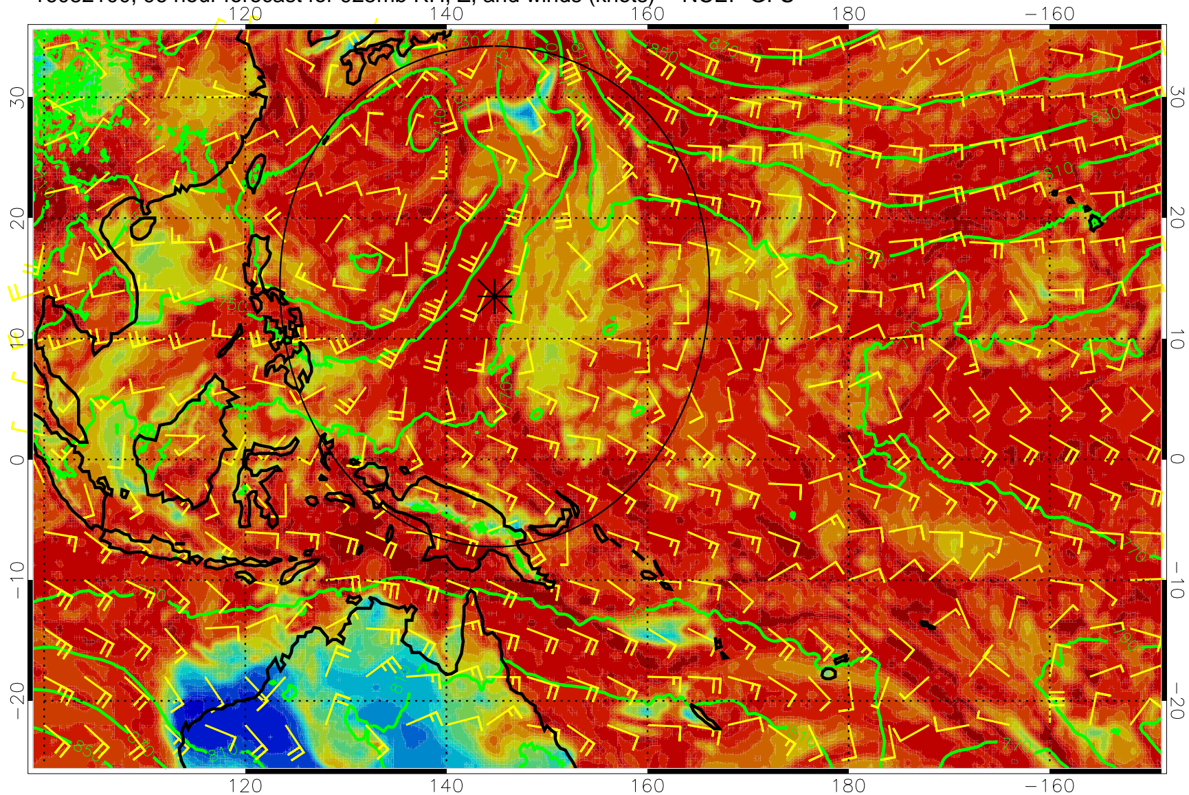
16082100, 96 hour forecast for 925mb RH, Z, and winds (knots) -- NCEP GFS
