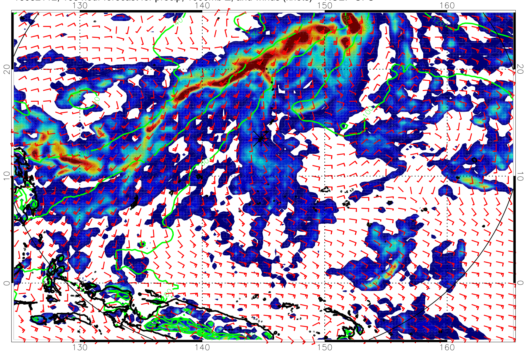
16082112, 108 hour forecast for precip, 1000mb Z, and winds (knots) -- NCEP GFS
