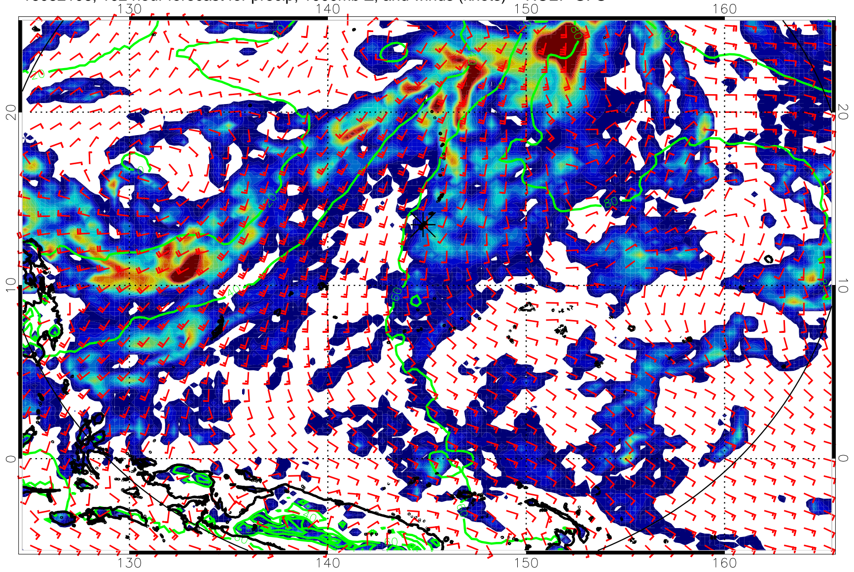
16082106, 102 hour forecast for precip, 1000mb Z, and winds (knots) -- NCEP GFS
