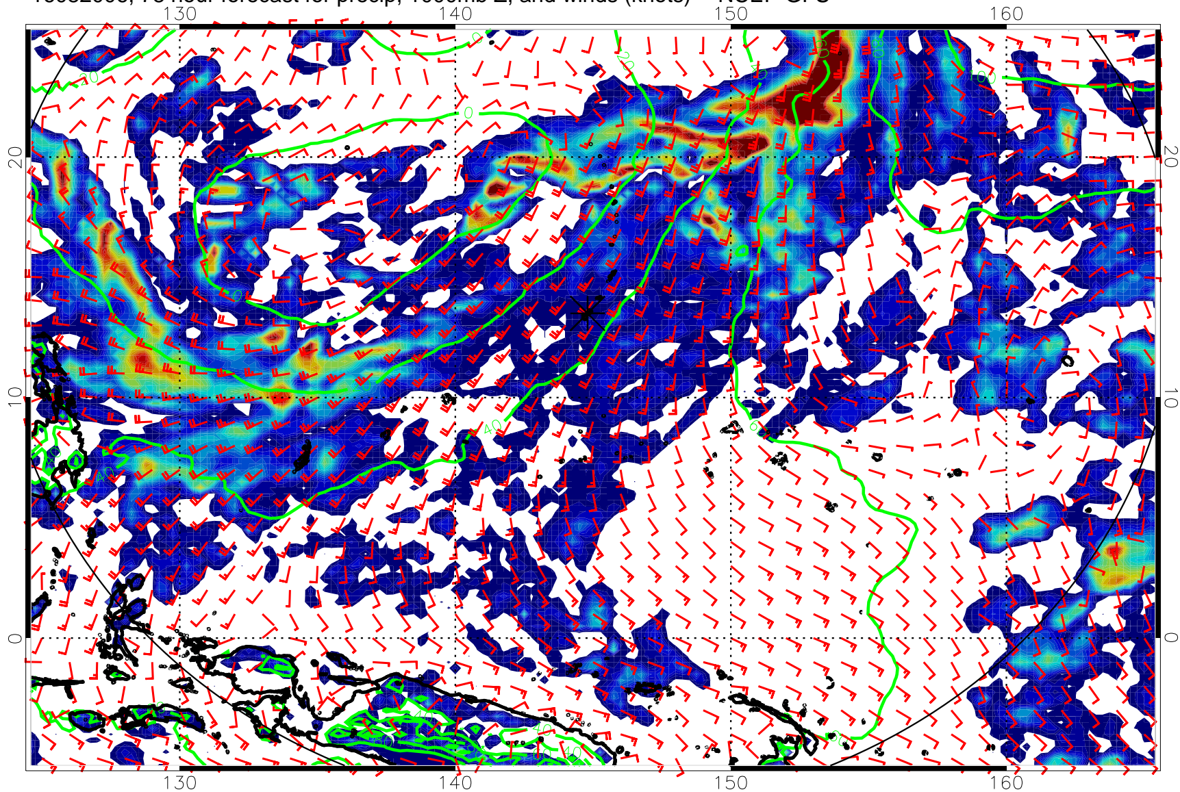
16082006, 78 hour forecast for precip, 1000mb Z, and winds (knots) -- NCEP GFS
