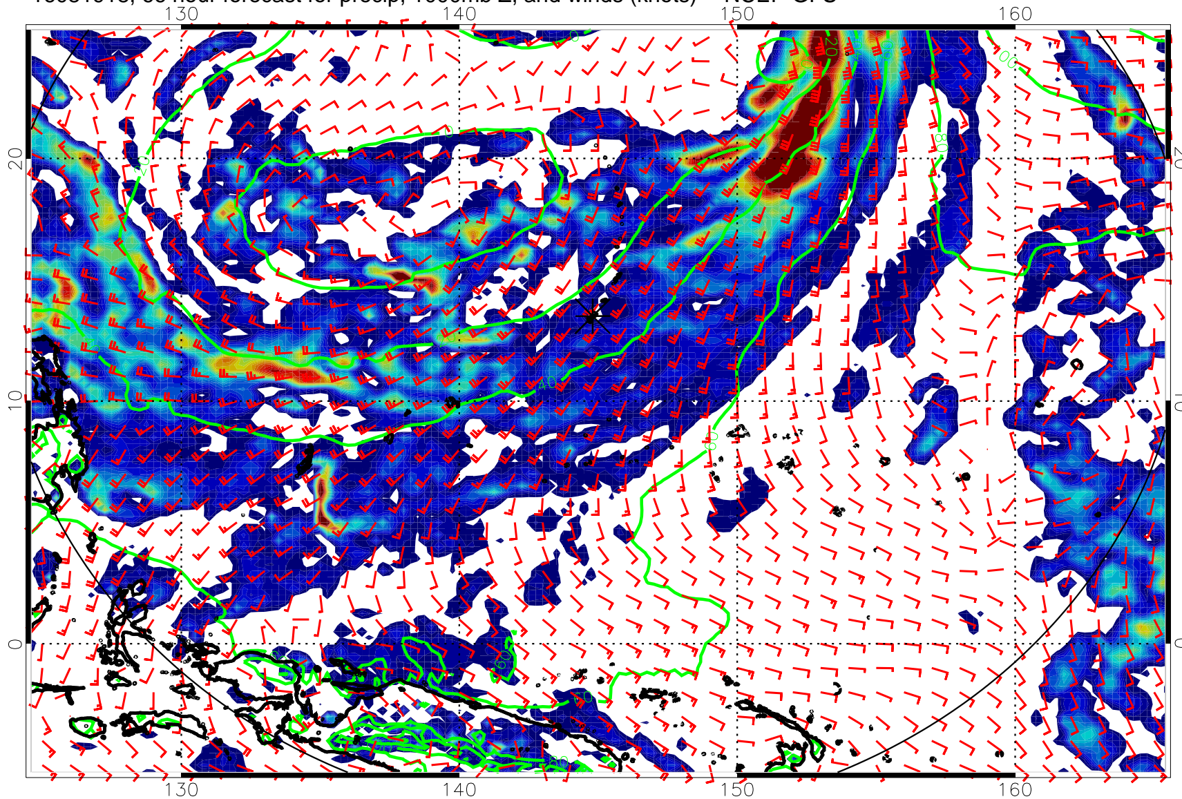
16081918, 66 hour forecast for precip, 1000mb Z, and winds (knots) -- NCEP GFS
