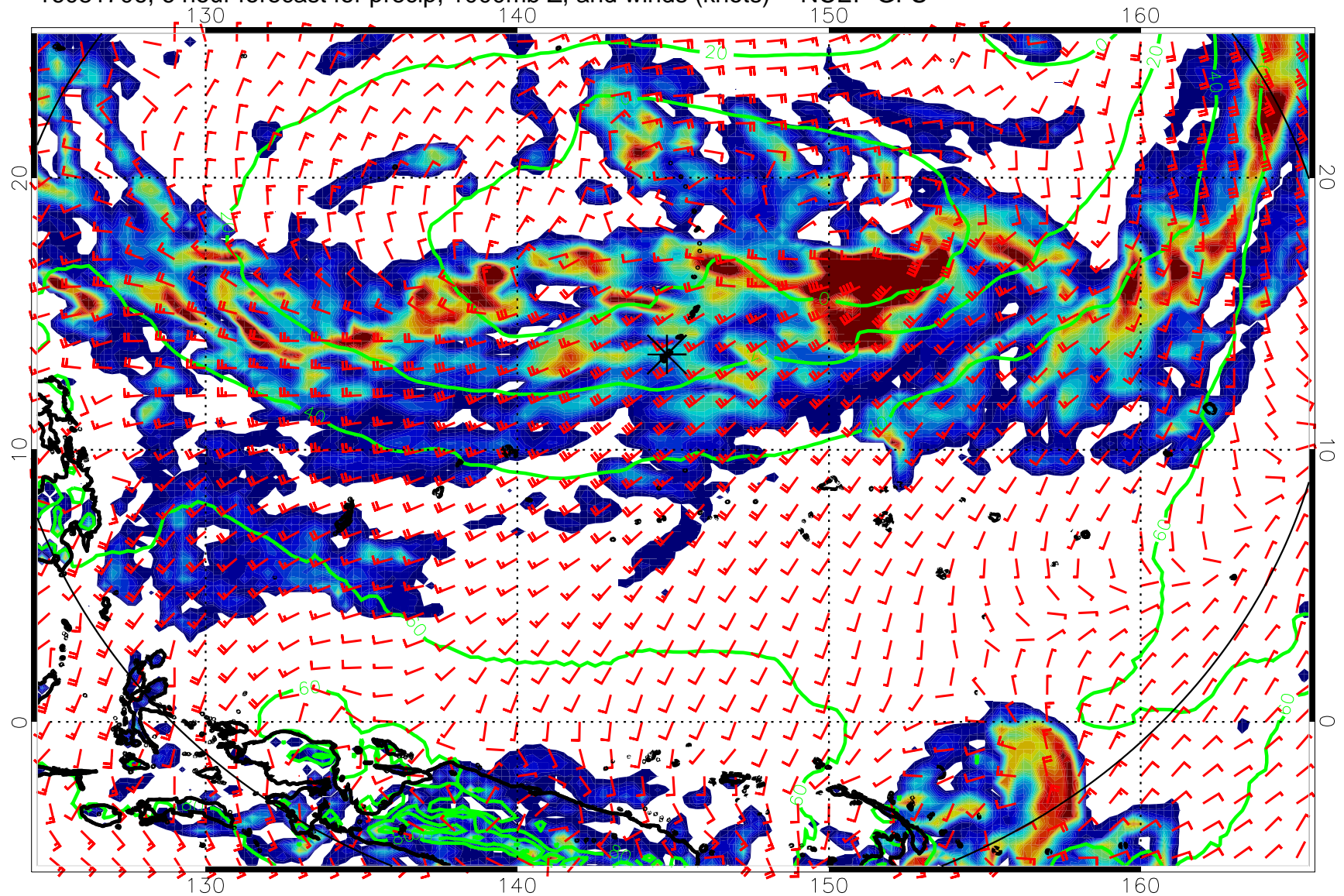
16081706, 6 hour forecast for precip, 1000mb Z, and winds (knots) -- NCEP GFS
