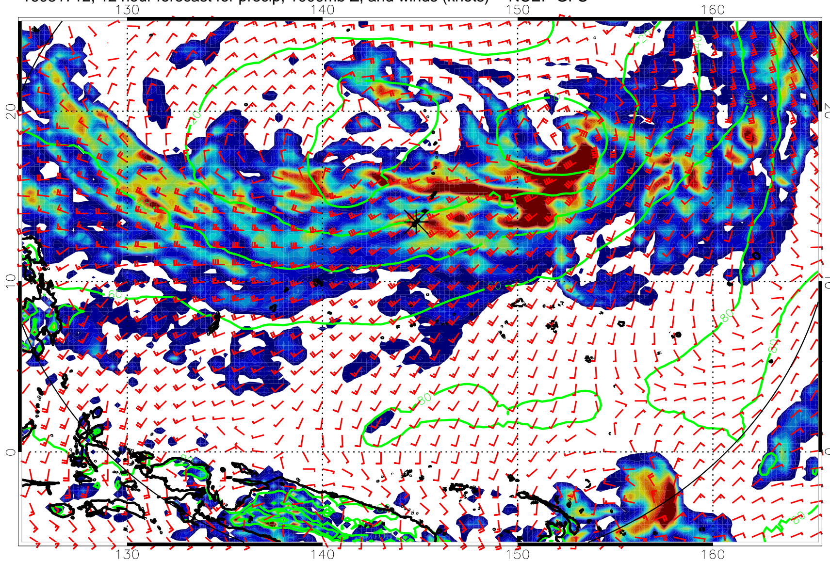
16081712, 12 hour forecast for precip, 1000mb Z, and winds (knots) -- NCEP GFS
