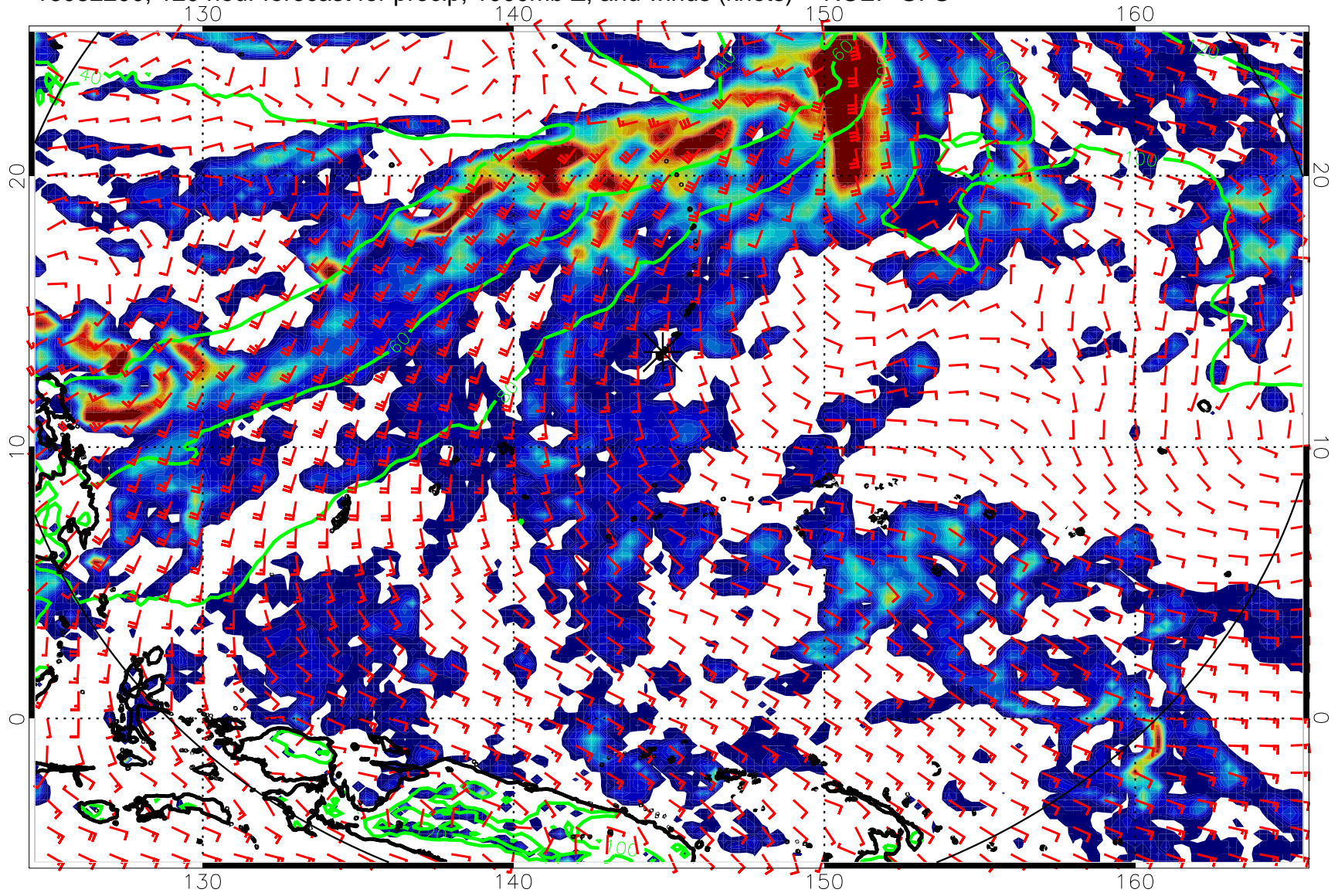
16082200, 120 hour forecast for precip, 1000mb Z, and winds (knots) -- NCEP GFS
