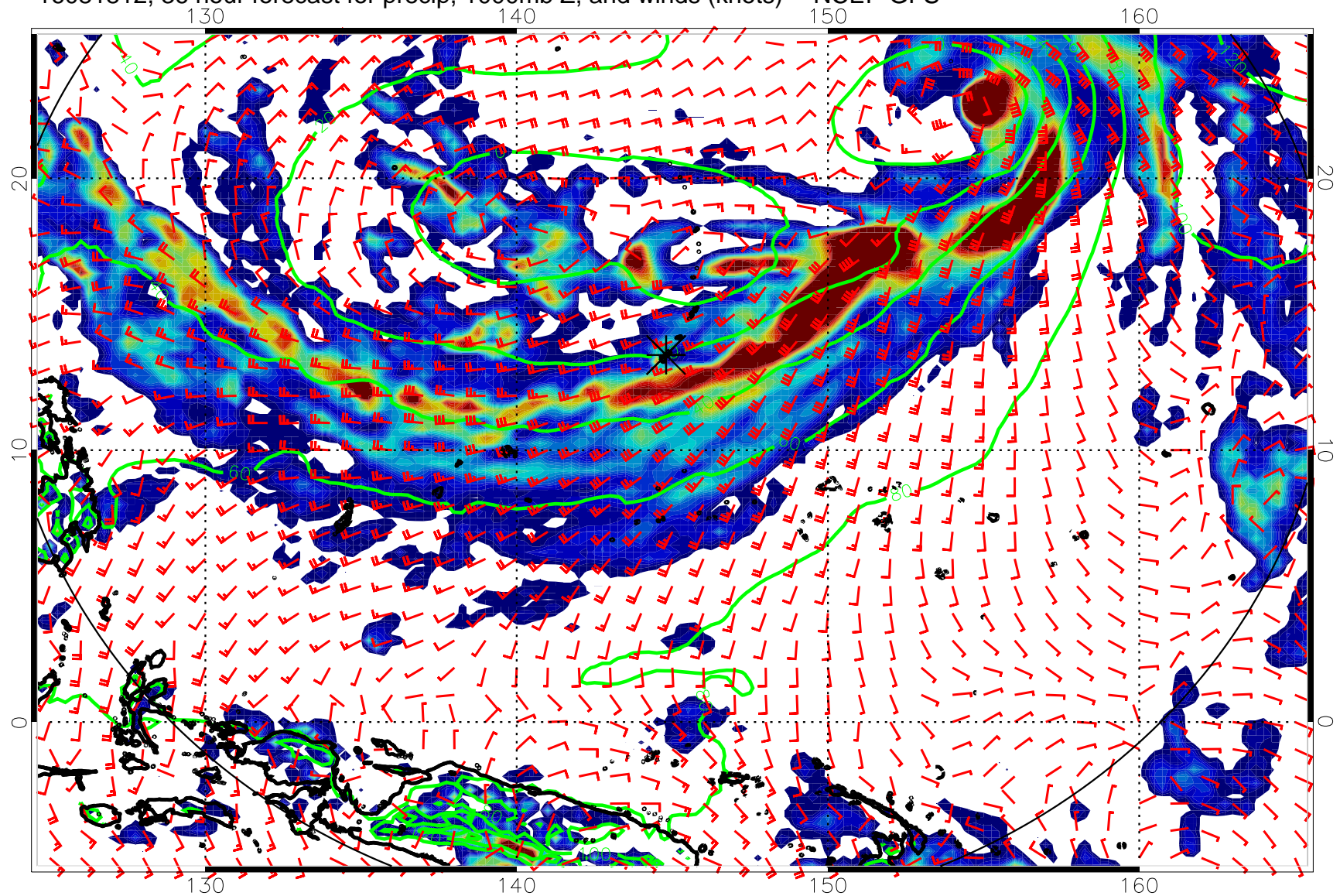
16081812, 36 hour forecast for precip, 1000mb Z, and winds (knots) -- NCEP GFS
