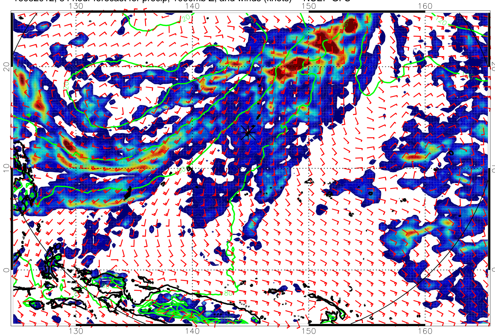
16082012, 84 hour forecast for precip, 1000mb Z, and winds (knots) -- NCEP GFS
