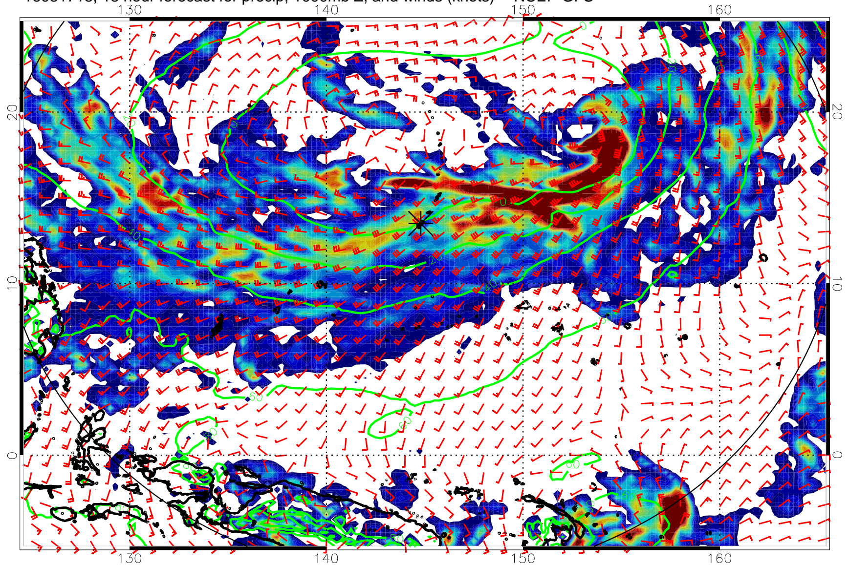
16081718, 18 hour forecast for precip, 1000mb Z, and winds (knots) -- NCEP GFS
