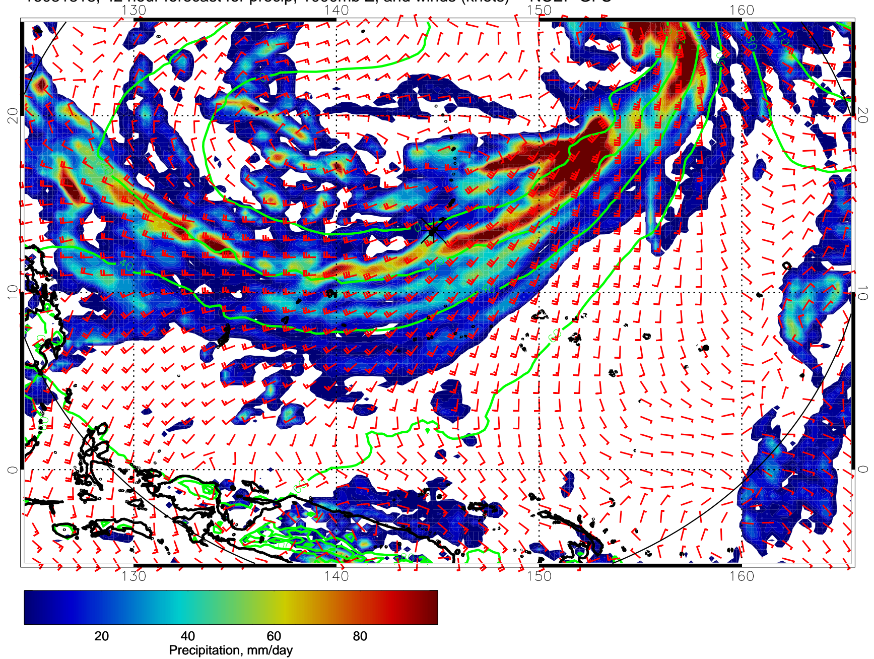
16081818, 42 hour forecast for precip, 1000mb Z, and winds (knots) -- NCEP GFS
