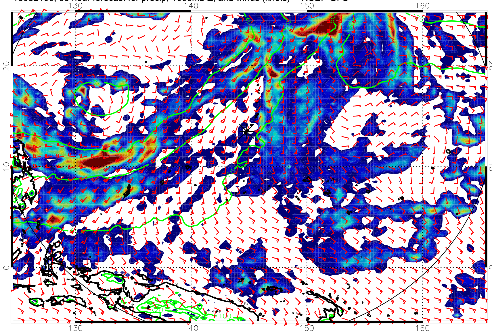
16082100, 96 hour forecast for precip, 1000mb Z, and winds (knots) -- NCEP GFS
