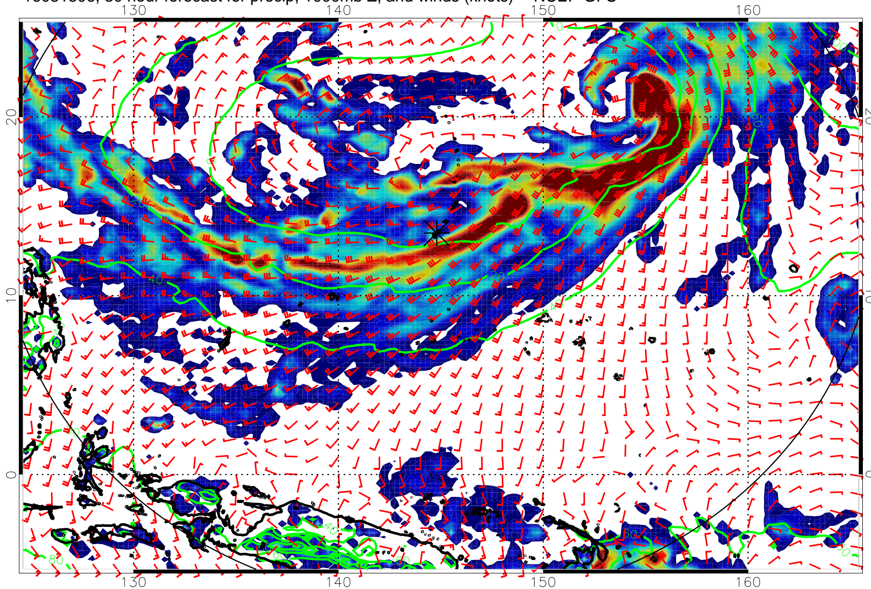
16081806, 30 hour forecast for precip, 1000mb Z, and winds (knots) -- NCEP GFS
