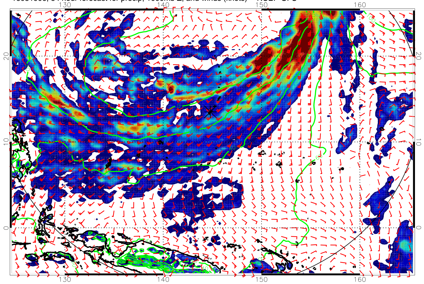
16081906, 54 hour forecast for precip, 1000mb Z, and winds (knots) -- NCEP GFS
