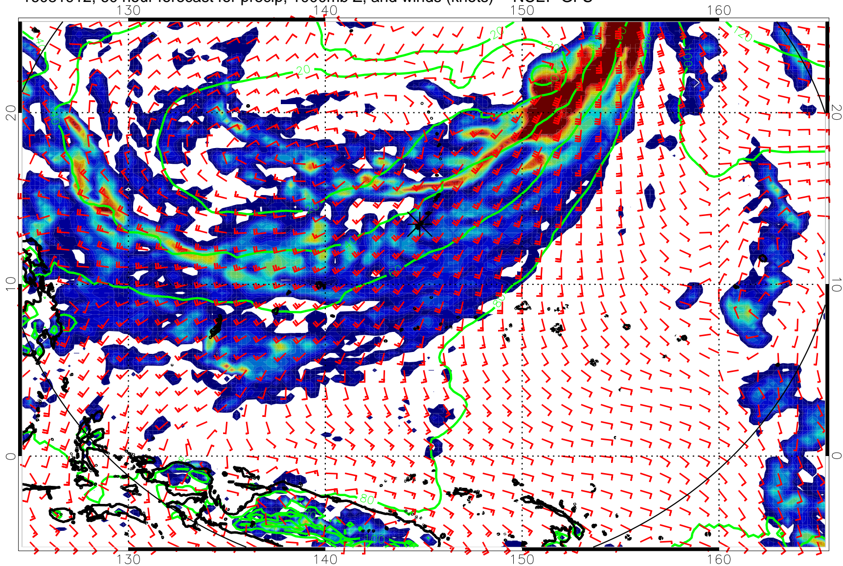
16081912, 60 hour forecast for precip, 1000mb Z, and winds (knots) -- NCEP GFS
