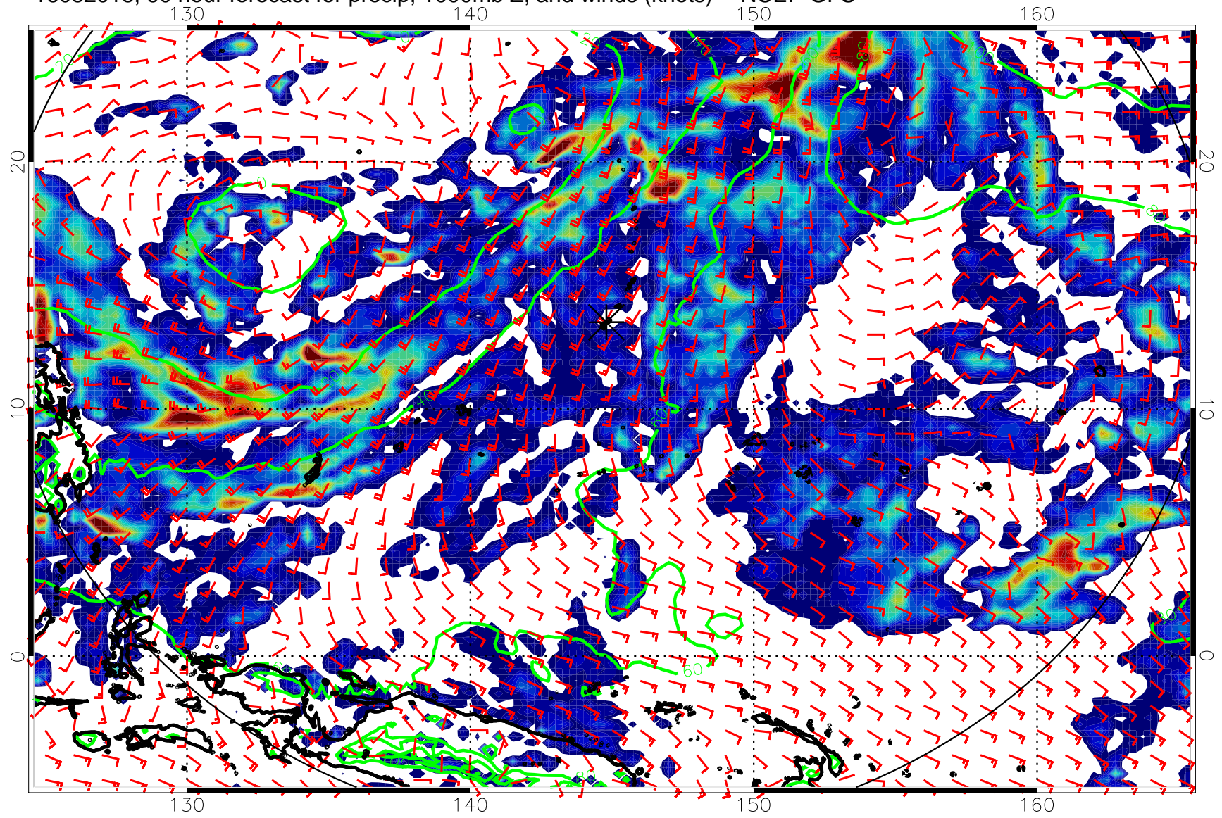
16082018, 90 hour forecast for precip, 1000mb Z, and winds (knots) -- NCEP GFS
