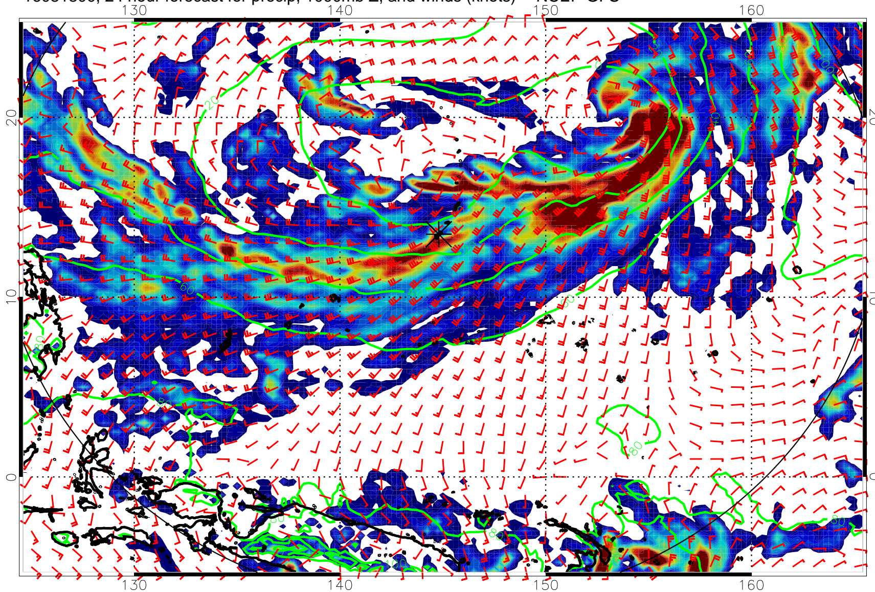
16081800, 24 hour forecast for precip, 1000mb Z, and winds (knots) -- NCEP GFS
