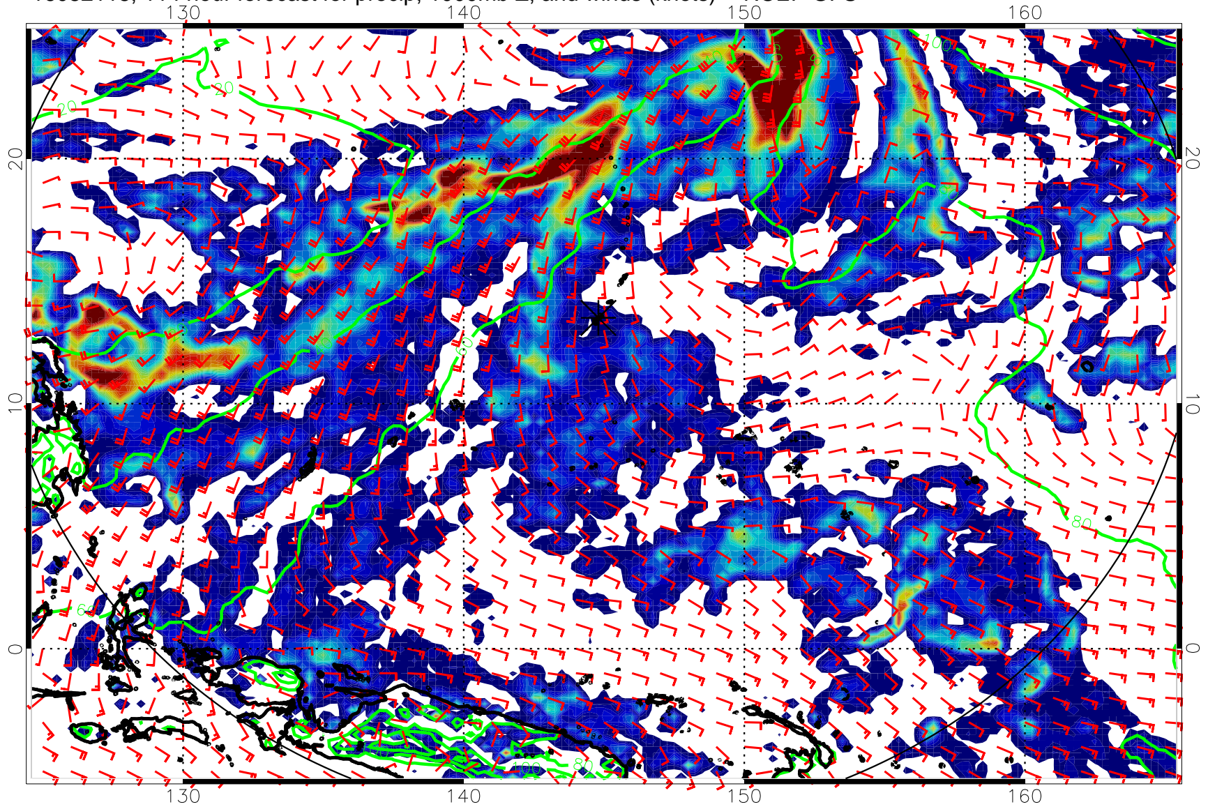
16082118, 114 hour forecast for precip, 1000mb Z, and winds (knots) -- NCEP GFS
