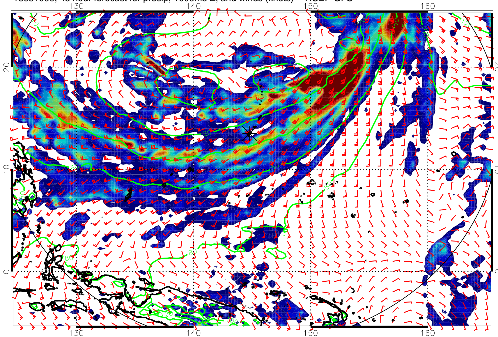
16081900, 48 hour forecast for precip, 1000mb Z, and winds (knots) -- NCEP GFS
