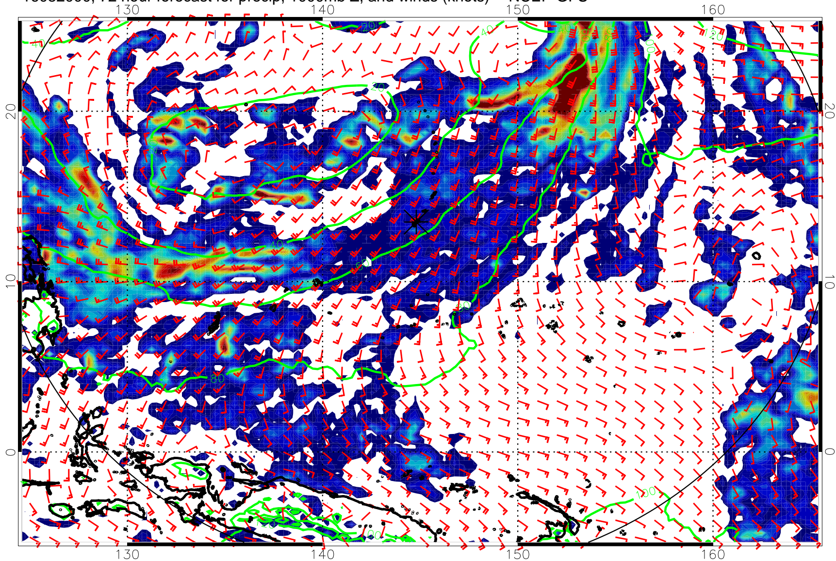
16082000, 72 hour forecast for precip, 1000mb Z, and winds (knots) -- NCEP GFS
